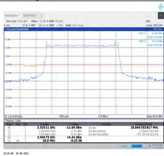
1-N78-3450-3550--30-30-H-3-DFT-16QAM-Outer_Fu II-75@0-Ant1-26.847-28.800-≤30-PASS
