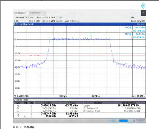
1-N78-3450-3550--30-20-L-8-CP-64QAM-Outer_Full -51@0-Ant1-18.199-19.800-<=20-PASS
