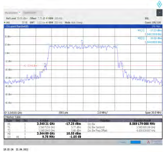
1-N78-3450-3550--30-10-H-8-CP-64QAM-Outer_Full -24@0-Ant1-8.569-9.780-<=10-PASS
