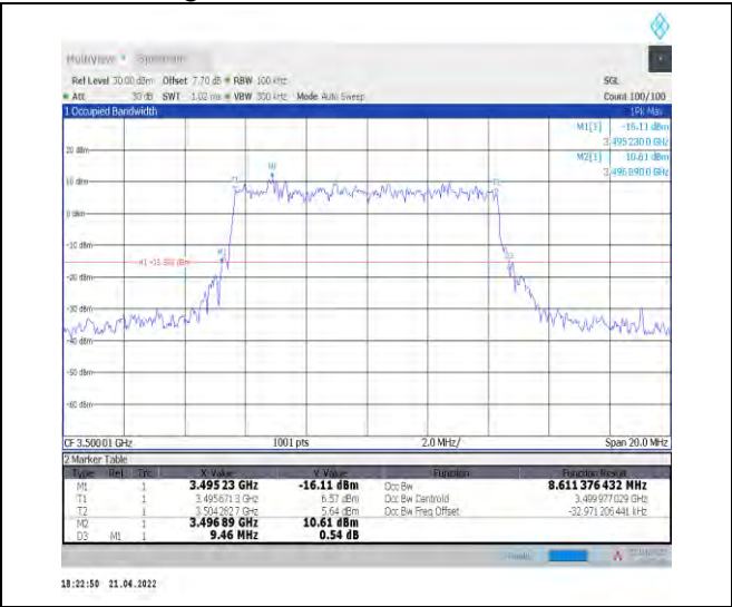
1-N78-3450-3550--30-10-M-5-DFT-256QAM-Outer_Full-24@0-Ant1-8.611-9.460-≤10-PASS
