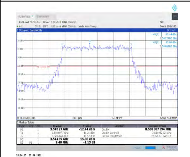
1-N78-3450-3550--30-10-H-2-DFT-PI2BPSK-Outer_Full -24@0-Ant1-8.569-9.480-≤10-PASS
