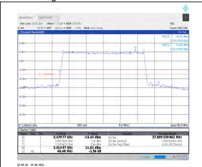
1-N78-3450-3550--30-40-M-9-CP-256QAM-Outer_F ull-106@0-Ant1-37.9-40.480-<math>\leq 40</math>-PASS
