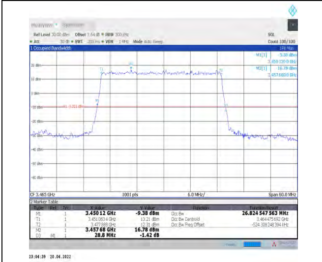
1-N78-3450-3550--30-30-L-2-DFT-PI2BPSK-Outer_Full-75@0-Ant1-26.825-28.800-<math>\leq 30</math>-PASS
