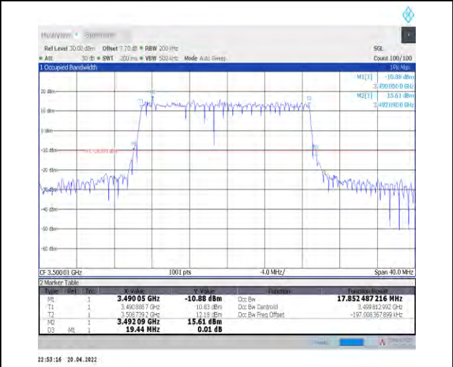
1-N78-3450-3550--30-20-M-1-DFT-QPSK-Outer_Full -50@0-Ant1-17.852-19.440-<=20-PASS
