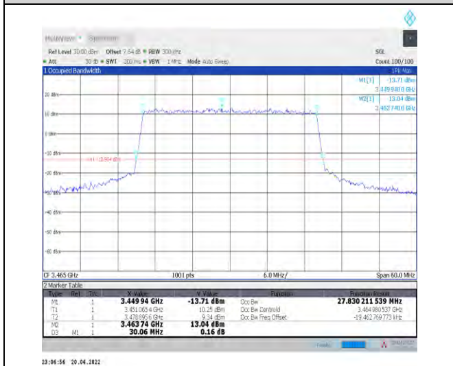
1-N78-3450-3550--30-30-L-6-CP-QPSK-Outer_Full-7 8@0-Ant1-27.83-30.060-≤30-PASS
