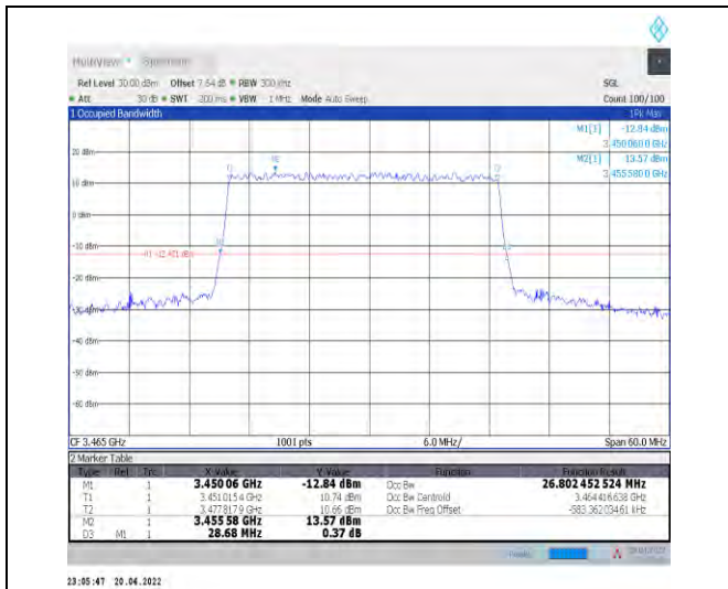
1-N78-3450-3550--30-30-L-4-DFT-64QAM-Outer_Full I-75@0-Ant1-26.802-28.680-≤30-PASS
