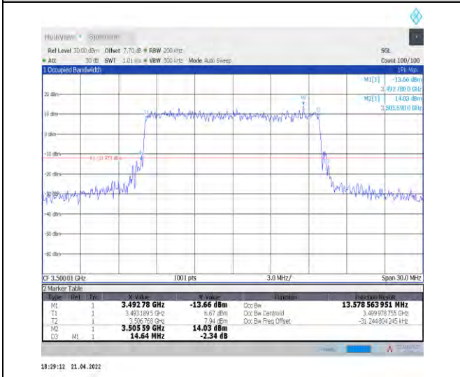
1-N78-3450-3550--30-15-M-7-CP-16QAM-Outer_Full-38@0-Ant1-13.579-14.640-≤15-PASS
