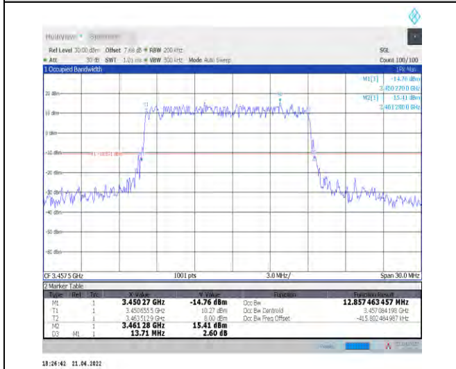
1-N78-3450-3550--30-15-L-4-DFT-64QAM-Outer_Full-36@0-Ant1-12.857-13.710-≤15-PASS
