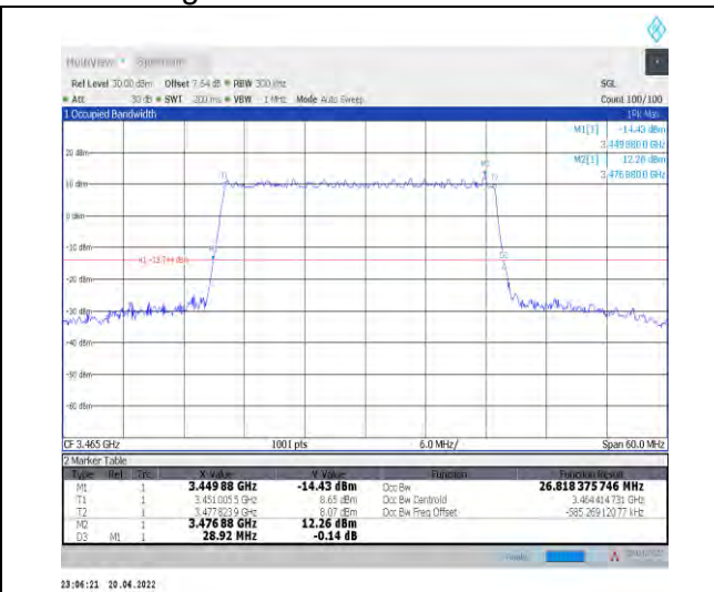
1-N78-3450-3550--30-30-L-5-DFT-256QAM-Outer_Full ull-75@0-Ant1-26.818-28.920-≤30-PASS
