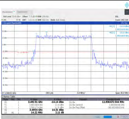
1-N78-3450-3550--30-15-M-1-DFT-QPSK-Outer_Full -36@0-Ant1-12.885-14.220-≤15-PASS
