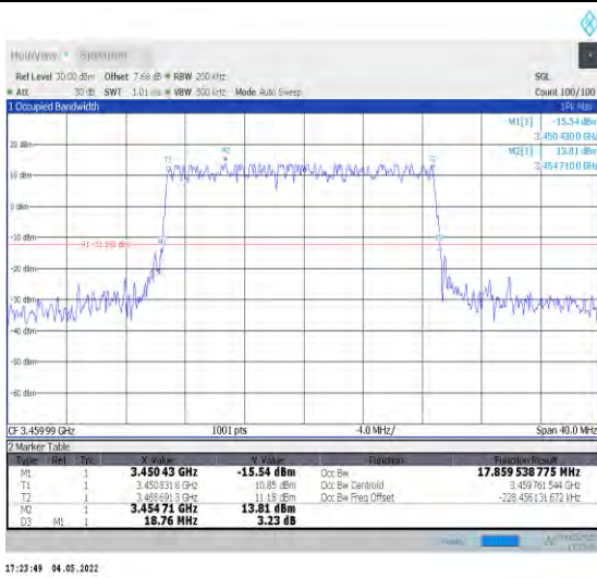
1-N78-3450-3550--30-20-L-3-DFT-16QAM-Outer_Ful I-50@0-Ant1-17.86-18.760-<math>\leq 20</math>-PASS
