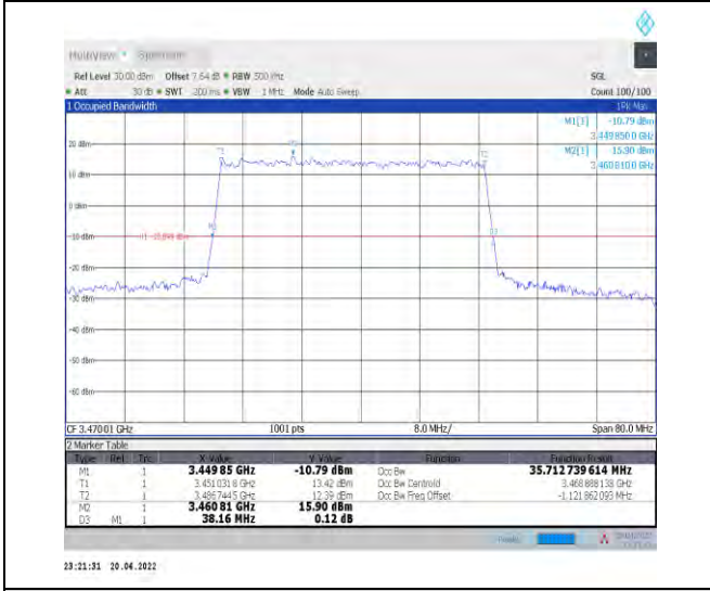
1-N78-3450-3550--30-40-L-3-DFT-16QAM-Outer_Full-100@0-Ant1-35.713-38.160-≤40-PASS
