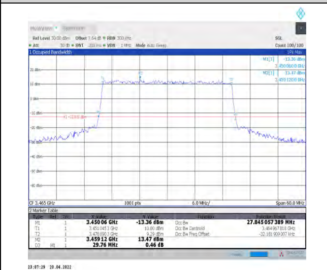
1-N78-3450-3550--30-30-L-7-CP-16QAM-Outer_Full -78@0-Ant1-27.845-29.760-≤30-PASS
