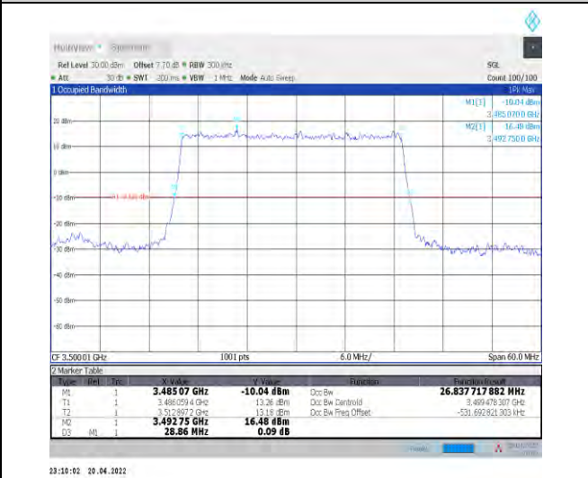
1-N78-3450-3550--30-30-M-2-DFT-PI2BPSK-Outer_Full-75@0-Ant1-26.838-28.860-<30-PASS
