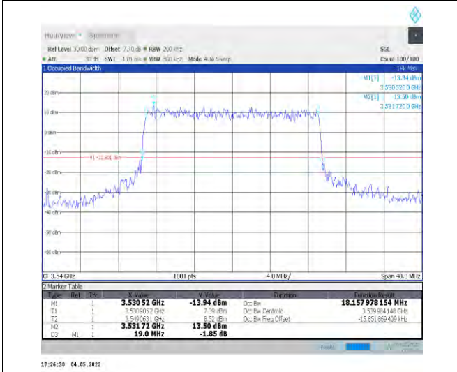
1-N78-3450-3550--30-20-H-7-CP-16QAM-Outer_Full-51@0-Ant1-18.158-19.000-≤20-PASS
