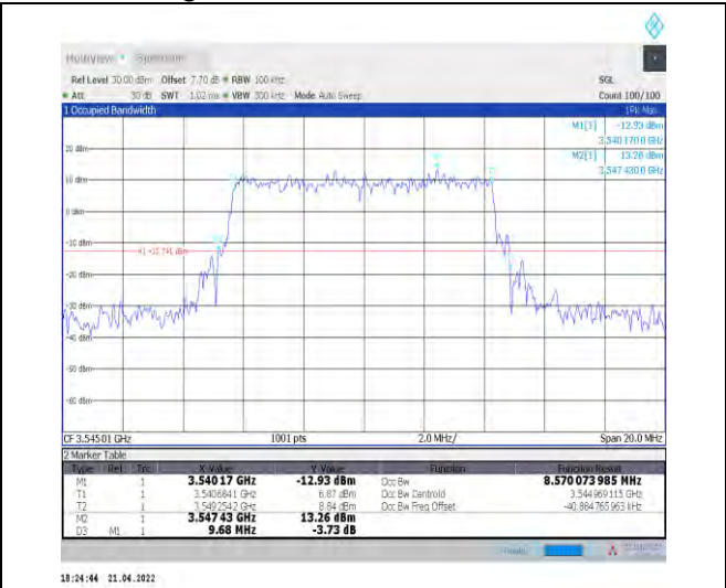
1-N78-3450-3550--30-10-H-4-DFT-64QAM-Outer_Fu II-24@0-Ant1-8.57-9.680-≤10-PASS
