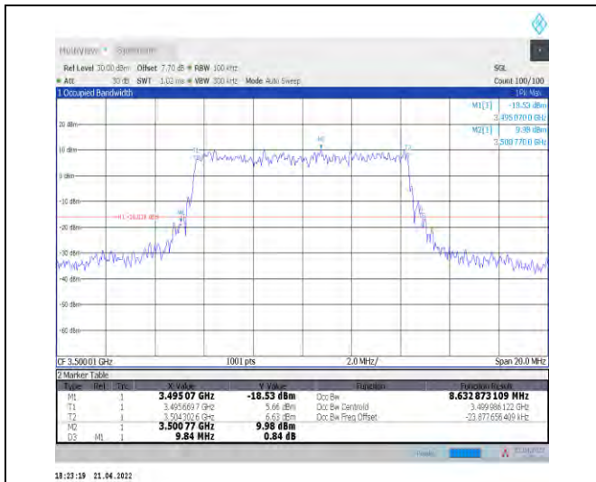
1-N78-3450-3550--30-10-M-8-CP-64QAM-Outer_Full -24@0-Ant1-8.633-9.840-≤10-PASS
