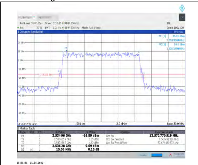
1-N78-3450-3550--30-15-H-9-CP-256QAM-Outer_Full -38@0-Ant1-13.573-15.060-≤15-PASS
