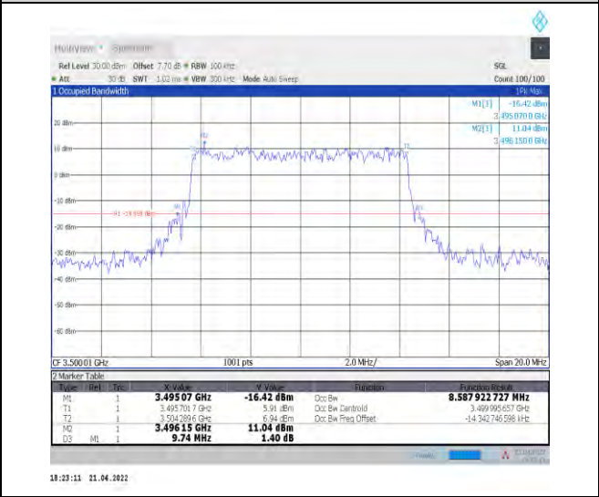
1-N78-3450-3550--30-10-M-7-CP-16QAM-Outer_Full-24@0-Ant1-8.588-9.740-≤10-PASS
