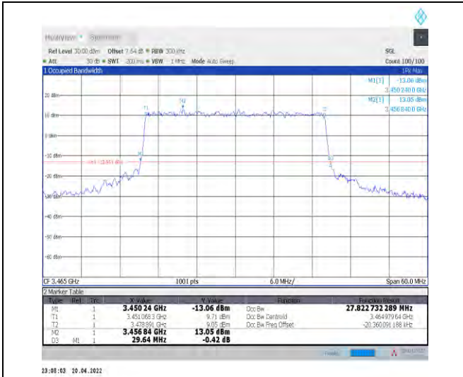
1-N78-3450-3550--30-30-L-8-CP-64QAM-Outer_Full -78@0-Ant1-27.823-29.640-<30-PASS
