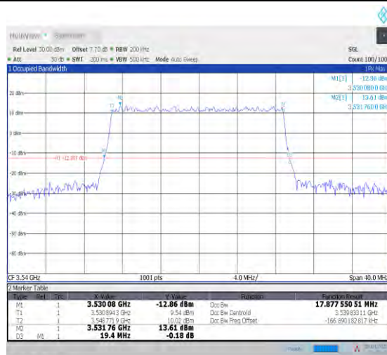
1-N78-3450-3550--30-20-H-2-DFT-PI2BPSK-Outer_Full Full-50@0-Ant1-17.844-18.720-≤20-PASS
