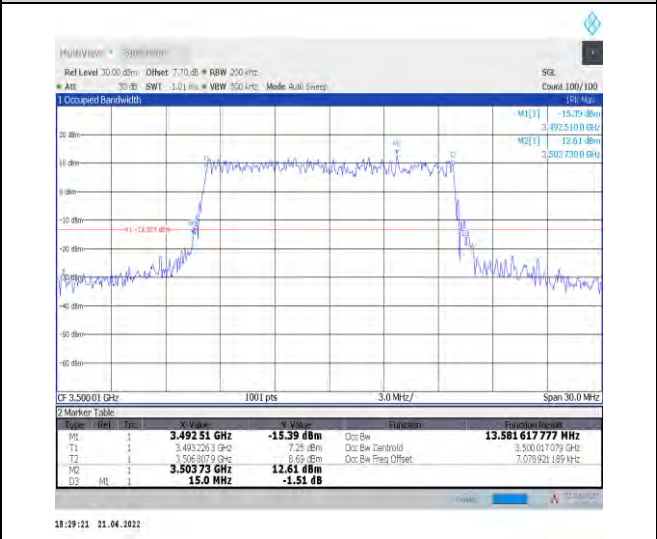
1-N78-3450-3550--30-15-M-8-CP-64QAM-Outer_Full-38@0-Ant1-13.582-15.000-≤15-PASS
