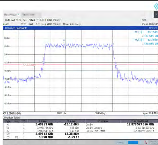
1-N78-3450-3550--30-15-M-2-DFT-PI2BPSK-Outer_Full Full-36@0-Ant1-12.846-14.430-≤15-PASS
