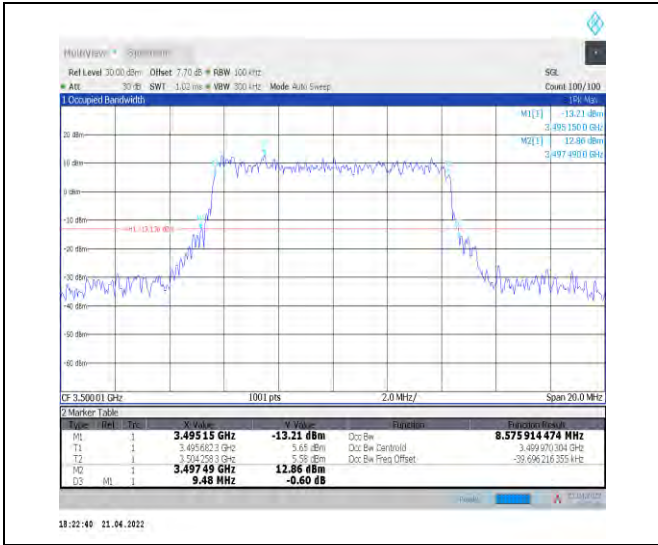
1-N78-3450-3550--30-10-M-4-DFT-64QAM-Outer_Full-24@0-Ant1-8.576-9.480-≤10-PASS
