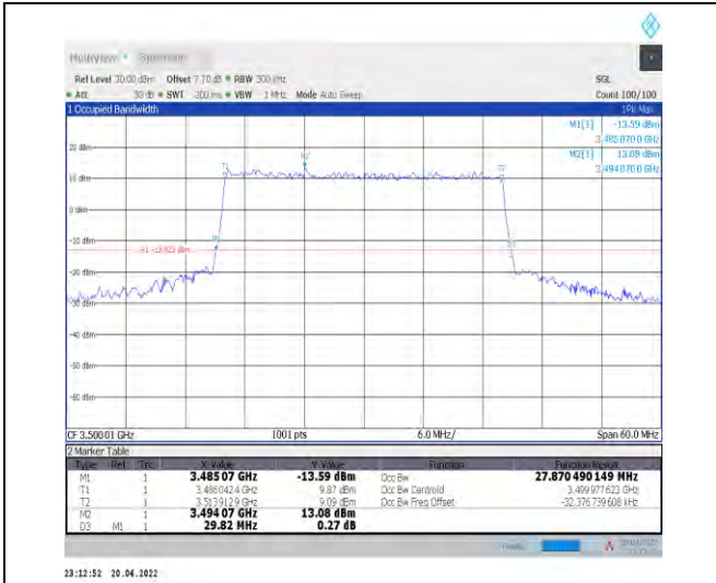
1-N78-3450-3550--30-30-M-7-CP-16QAM-Outer_Full-78@0-Ant1-27.87-29.820-≤30-PASS
