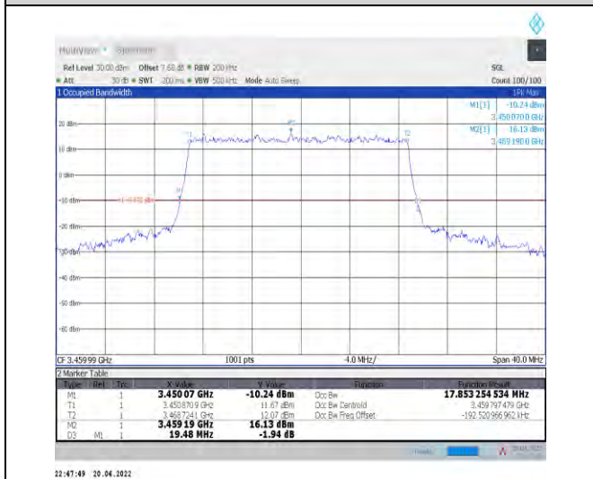
1-N78-3450-3550--30-20-L-1-DFT-QPSK-Outer_Full-50 @0-Ant1-17.853-19.480-≤20-PASS
