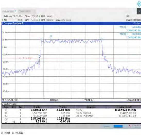
1-N78-3450-3550--30-10-H-7-CP-16QAM-Outer_Full -24@0-Ant1-8.588-9.320-<=10-PASS
