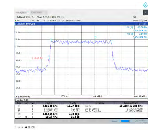
1-N78-3450-3550--30-20-L-9-CP-256QAM-Outer_Fu II-51@0-Ant1-18.218-19.240-<=20-PASS
