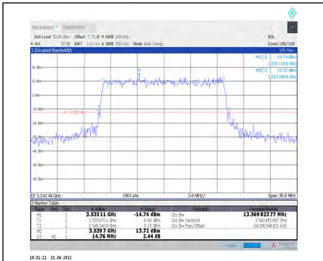
1-N78-3450-3550--30-15-H-8-CP-64QAM-Outer_Full -38@0-Ant1-13.57-14.760-≤15-PASS
