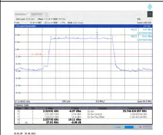
1-N78-3450-3550--30-40-H-2-DFT-PI2BPSK-Outer_ Full-100@0-Ant1-35.746-37.920-<math>\leq 40</math>-PASS
