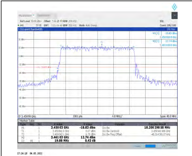
1-N78-3450-3550--30-20-L-7-CP-16QAM-Outer_Full -51@0-Ant1-18.2-19.880-<=20-PASS
