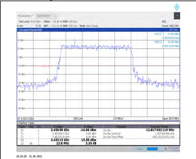
1-N78-3450-3550--30-15-L-3-DFT-16QAM-Outer_Full-36@0-Ant1-12.817-13.800-≤15-PASS
