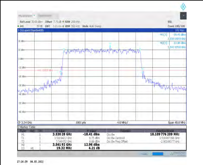
1-N78-3450-3550--30-20-H-8-CP-64QAM-Outer_Full-51@0-Ant1-18.11-19.320-≤20-PASS
