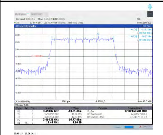
1-N78-3450-3550--30-20-L-2-DFT-PI2BPSK-Outer_Full-50 @0-Ant1-17.85-19.440-≤20-PASS
