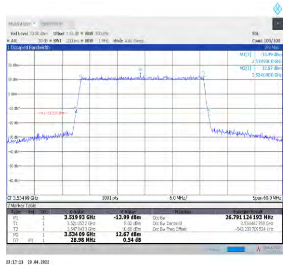
1-N78-3450-3550--30-30-H-5-DFT-256QAM-Outer_Fu ull-75@0-Ant1-26.791-28.980-≤30-PASS
