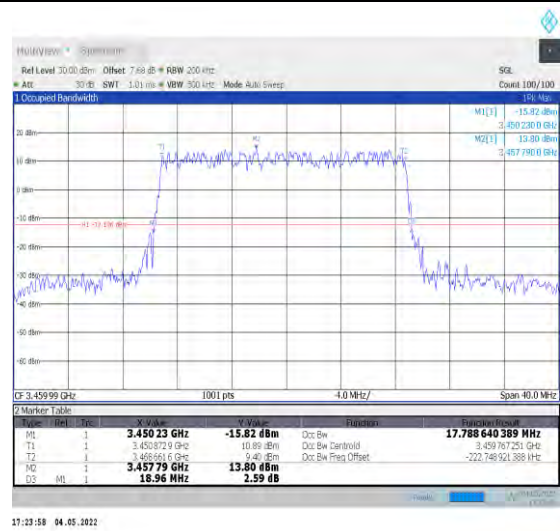
1-N78-3450-3550--30-20-L-4-DFT-64QAM-Outer_Fu II-50@0-Ant1-17.789-18.960-<math>\leq 20</math>-PASS
