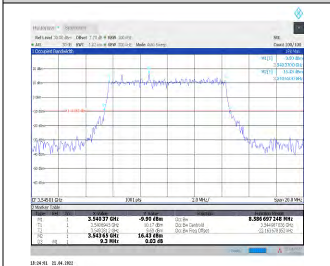
1-N78-3450-3550--30-10-H-1-DFT-QPSK-Outer_Full -24@0-Ant1-8.587-9.300-≤10-PASS
