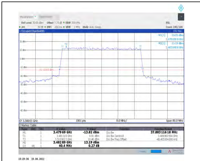
1-N78-3450-3550--30-40-M-8-CP-64QAM-Outer_Full -106@0-Ant1-37.883-40.400-<math>\leq 40</math>-PASS
