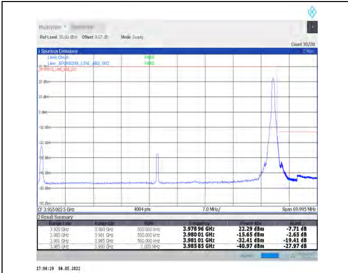
1-N77-3700-3980--30-60-H-2-DFT-PI2BPSK-Edge_1R_B_Right-1@161-Ant1-PASS-see graph
