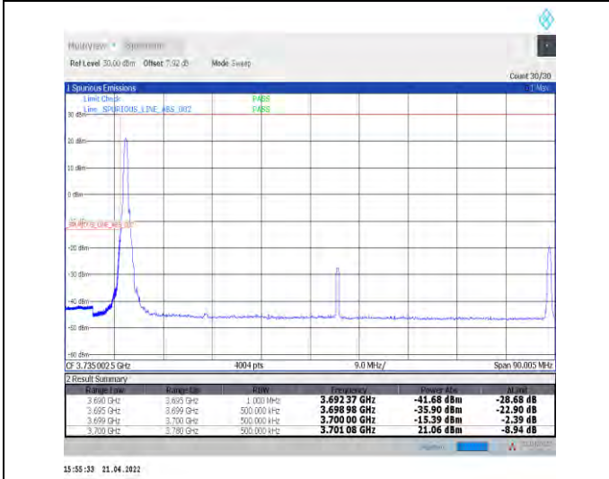
1-N77-3700-3980--30-80-L-4-CP-QPSK-Edge_1RB_L_eff-1@0-Ant1-PASS-see graph
