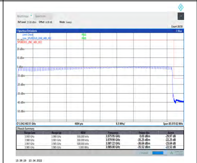
1-N77-3700-3980-PC2-30-80-H-6-CP-QPSK-Outer _Full-217@0-Ant1-PASS-see graph
