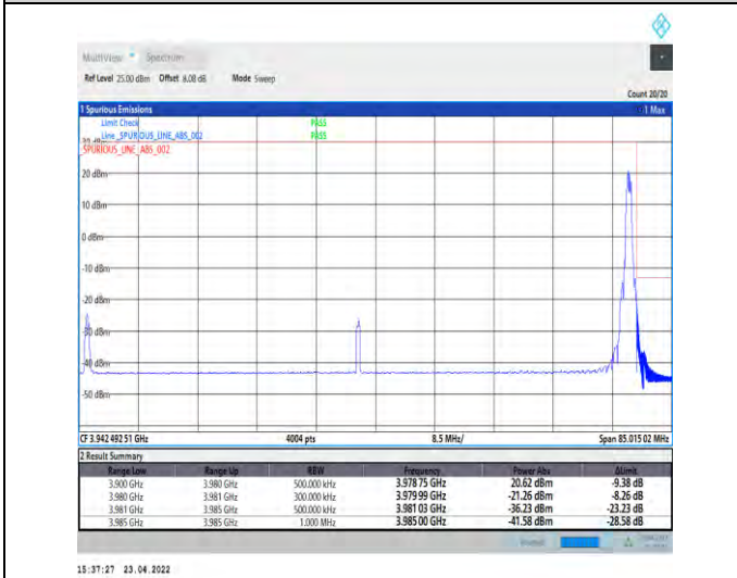
1-N77-3700-3980-PC2-30-80-H-5-CP-QPSK-Edge_1R B_Right-1@216-Ant1-PASS-see graph
