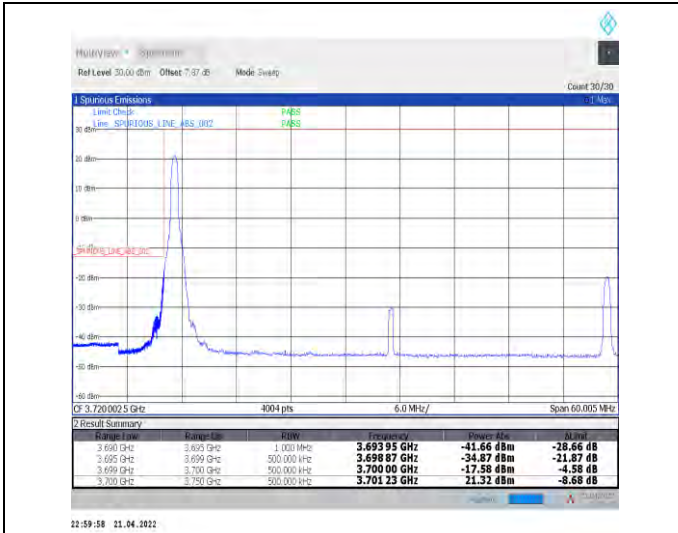
1-N77-3700-3980--30-50-L-1-DFT-PI2BPSK-Edge_1R_B_Left-1@0-Ant1-PASS-see graph
