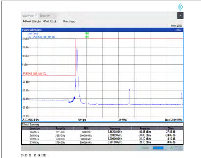
1-N77-3700-3980-PC2-30-80-L-4-CP-QPSK-Edge_1R B_Left-1@0-Ant1-PASS-see graph
