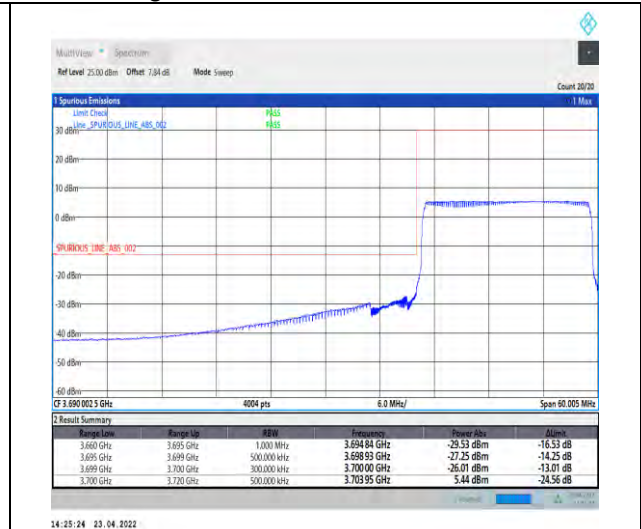
1-N77-3700-3980-PC2-30-20-L-6-CP-QPSK-Outer _Full-51@0-Ant1-PASS-see graph
