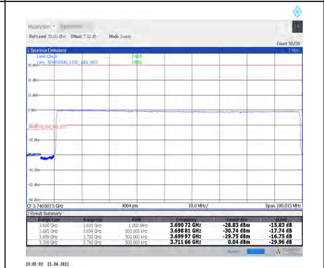
1-N77-3700-3980--30-90-L-6-CP-QPSK-Outer_Ful_I-245@0-Ant1-PASS-see graph
