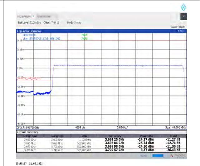
1-N77-3700-3980--30-40-L-6-CP-QPSK-Outer_Ful I-106@0-Ant1-PASS-see graph
