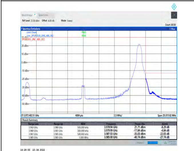
1-N77-3700-3980-PC2-30-20-H-5-CP-QPSK-Edge_1R B_Right-1@50-Ant1-PASS-see graph
