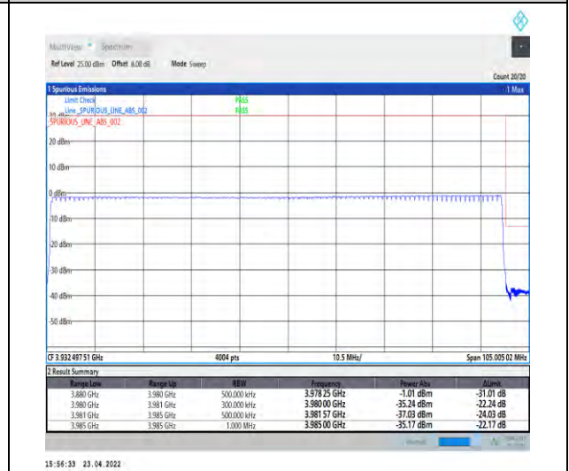
1-N77-3700-3980-PC2-30-100-H-6-CP-QPSK-Out er_Full-273@0-Ant1-PASS-see graph
