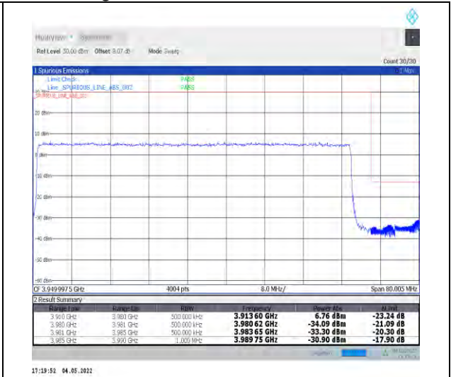
1-N77-3700-3980--30-70-H-3-DFT-PI2BPSK-Outer_Full-180@0-Ant1-PASS-see graph
