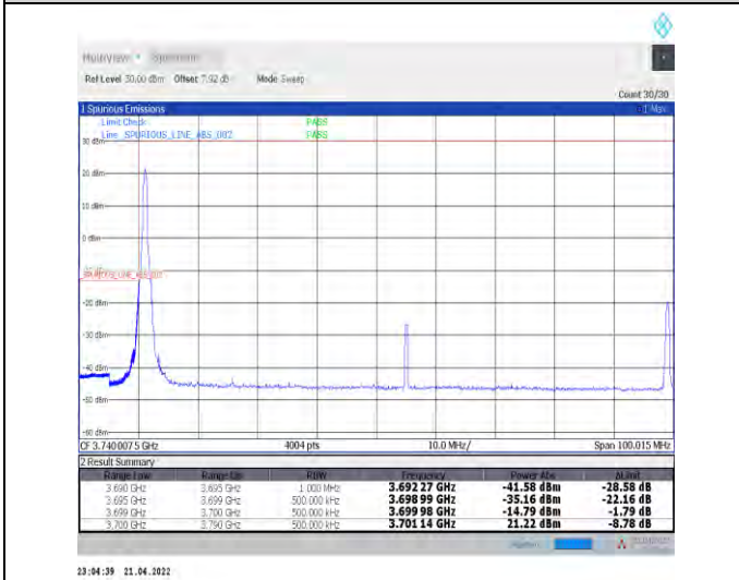
1-N77-3700-3980--30-90-L-4-CP-QPSK-Edge_1RB_L_eff-1@0-Ant1-PASS-see graph
