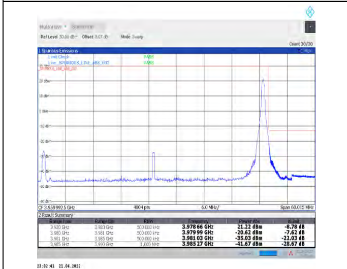
1-N77-3700-3980--30-50-H-5-CP-QPSK-Edge_1RB_R ight-1@132-Ant1-PASS-see graph
