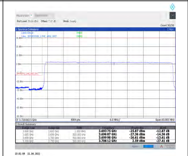
1-N77-3700-3980--30-50-L-6-CP-QPSK-Outer_Ful_I-133@0-Ant1-PASS-see graph
