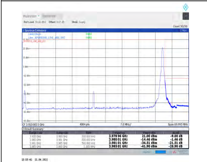
1-N77-3700-3980--30-60-H-5-CP-QPSK-Edge_1RB_Right-1@161-Ant1-PASS-see graph
