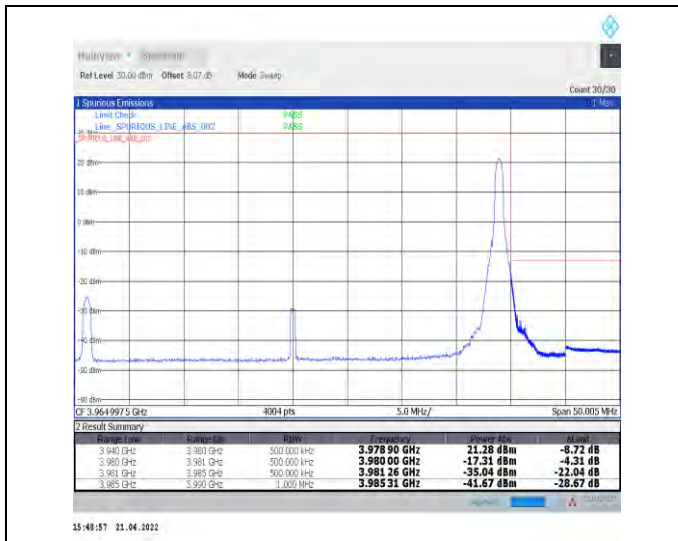
1-N77-3700-3980--30-40-H-2-DFT-PI2BPSK-Edge_1R_B_Right-1@105-Ant1-PASS-see graph
