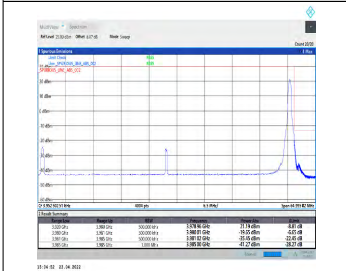
1-N77-3700-3980-PC2-30-60-H-5-CP-QPSK-Edge_1R_B_Right-1@161-Ant1-PASS-see graph
