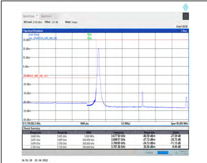
1-N77-3700-3980-PC2-30-50-L-4-CP-QPSK-Edge_1R_B_Left-1@0-Ant1-PASS-see graph
