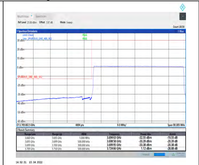
1-N77-3700-3980-PC2-30-50-L-6-CP-QPSK-Outer_Full-133@0-Ant1-PASS-see graph
