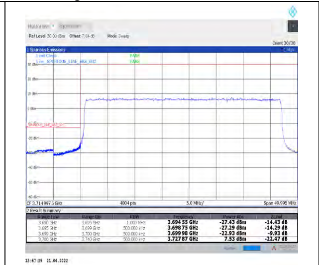
1-N77-3700-3980--30-40-L-3-DFT-PI2BPSK-Outer_Full-100@0-Ant1-PASS-see graph
