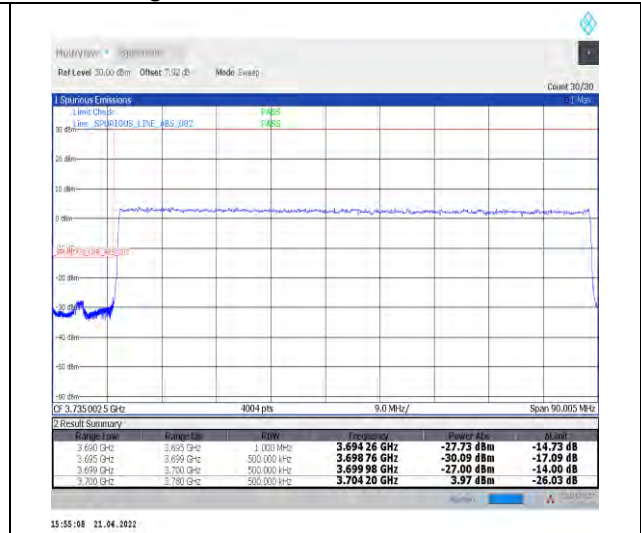
1-N77-3700-3980--30-80-L-3-DFT-PI2BPSK-Outer_Full-216@0-Ant1-PASS-see graph
