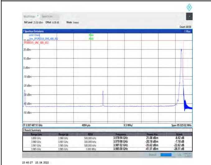
1-N77-3700-3980-PC2-30-90-H-5-CP-QPSK-Edge_1R B_Right-1@244-Ant1-PASS-see graph
