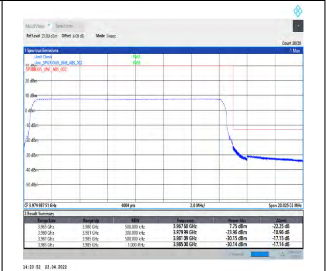
1-N77-3700-3980-PC2-30-15-H-6-CP-QPSK-Outer _Full-38@0-Ant1-PASS-see graph
