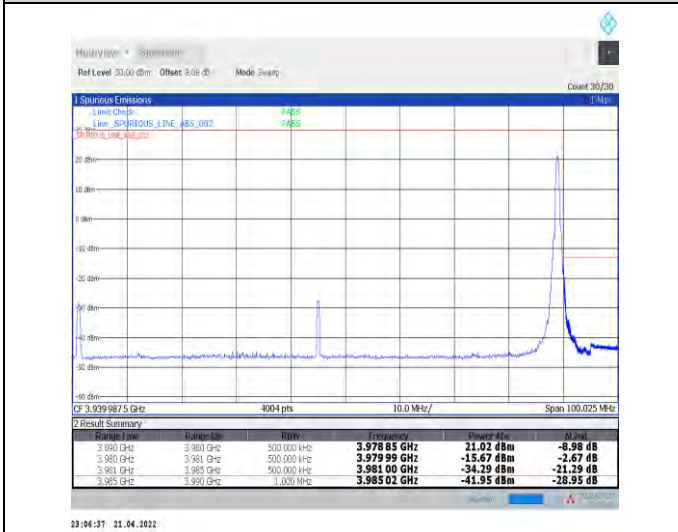
1-N77-3700-3980--30-90-H-5-CP-QPSK-Edge_1RB_R ight-1@244-Ant1-PASS-see graph
