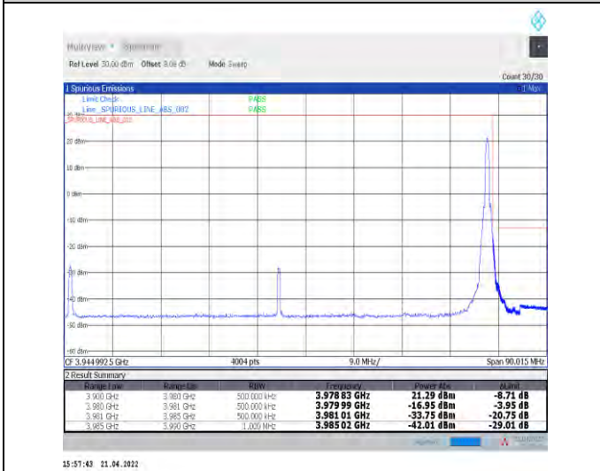
1-N77-3700-3980--30-80-H-5-CP-QPSK-Edge_1RB_Right-1@216-Ant1-PASS-see graph
