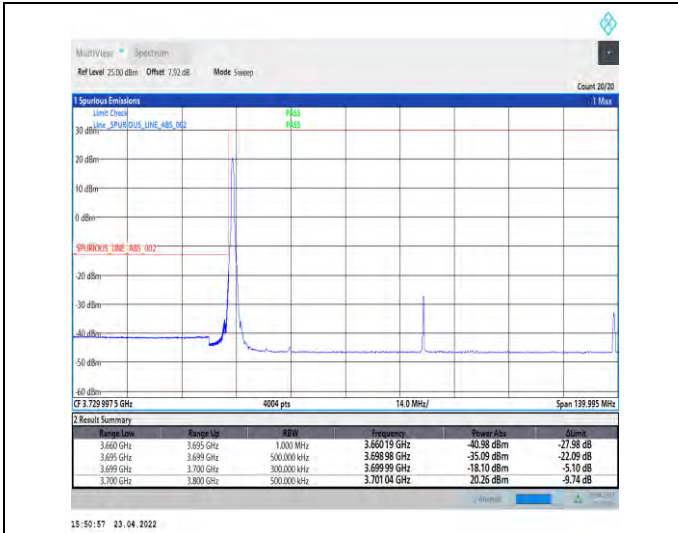
1-N77-3700-3980-PC2-30-100-L-4-CP-QPSK-Edge_1 RB_Left-1@0-Ant1-PASS-see graph
