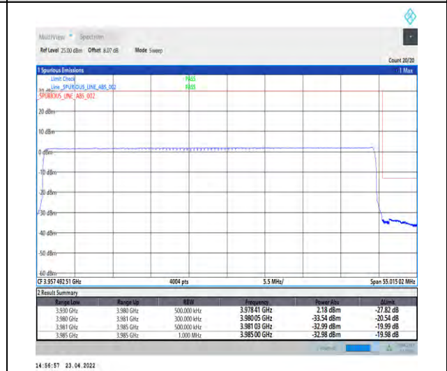
1-N77-3700-3980-PC2-30-50-H-6-CP-QPSK-Outer_Full-133@0-Ant1-PASS-see graph
