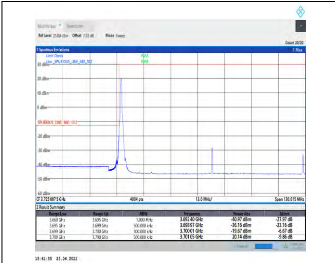
1-N77-3700-3980-PC2-30-90-L-4-CP-QPSK-Edge_1R B_Left-1@0-Ant1-PASS-see graph
