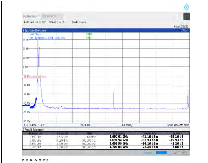
1-N77-3700-3980--30-100-L-1-DFT-PI2BPSK-Edge_1 RB_Left-1@0-Ant1-PASS-see graph
