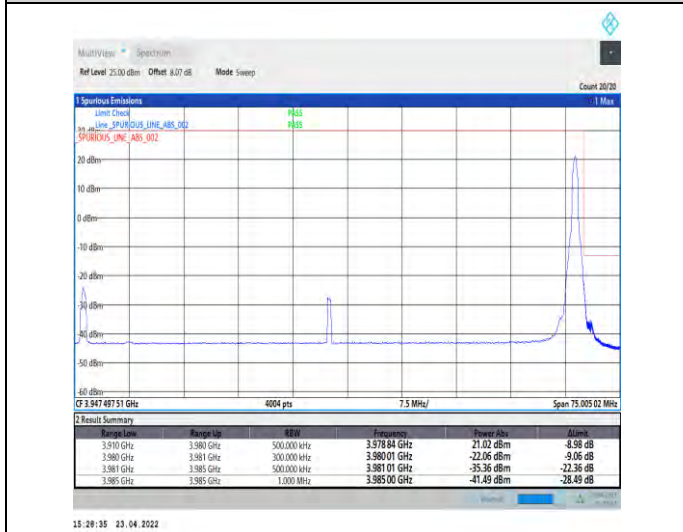
1-N77-3700-3980-PC2-30-70-H-5-CP-QPSK-Edge_1R B_Right-1@188-Ant1-PASS-see graph
