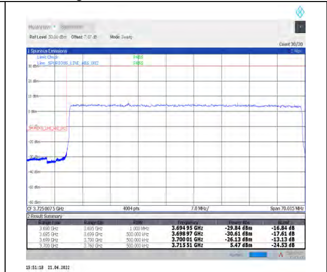
1-N77-3700-3980--30-60-L-3-DFT-PI2BPSK-Outer_Full-162@0-Ant1-PASS-see graph
