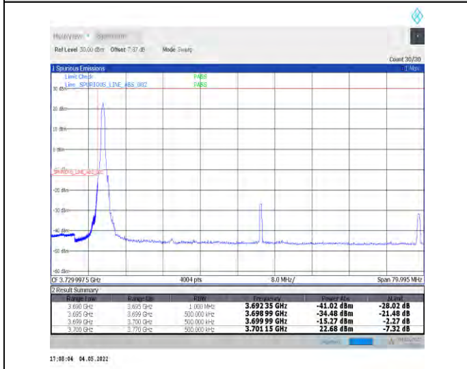
1-N77-3700-3980--30-70-L-4-CP-QPSK-Edge_1RB_L_eff-1@0-Ant1-PASS-see graph
