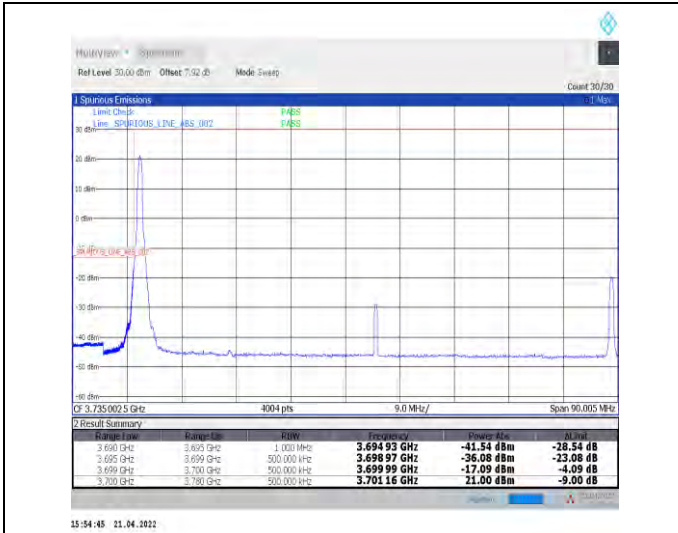
1-N77-3700-3980--30-80-L-1-DFT-PI2BPSK-Edge_1R_B_Left-1@0-Ant1-PASS-see graph
