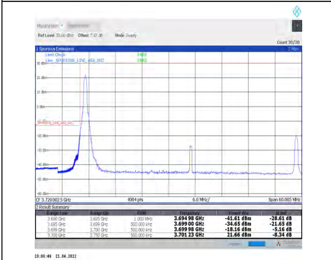
1-N77-3700-3980--30-50-L-4-CP-QPSK-Edge_1RB_L_eff-1@0-Ant1-PASS-see graph
