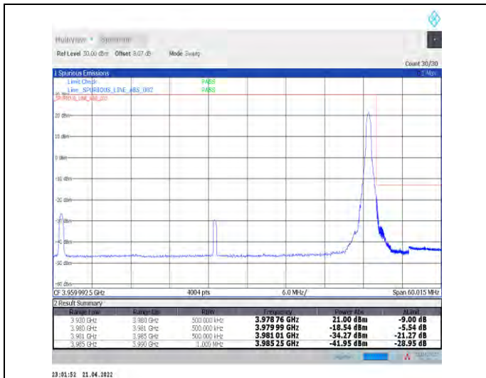
1-N77-3700-3980--30-50-H-2-DFT-PI2BPSK-Edge_1R_B_Right-1@132-Ant1-PASS-see graph
