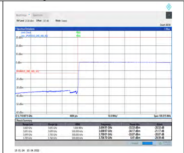
1-N77-3700-3980-PC2-30-60-L-6-CP-QPSK-Outer_Full-162@0-Ant1-PASS-see graph
