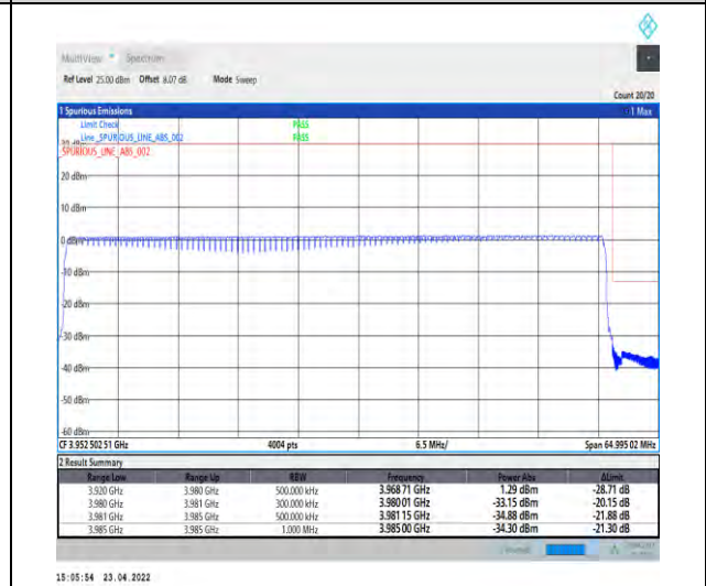
1-N77-3700-3980-PC2-30-60-H-6-CP-QPSK-Outer_Full-162@0-Ant1-PASS-see graph
