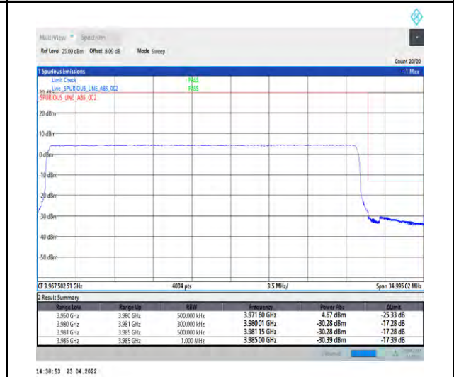
1-N77-3700-3980-PC2-30-30-H-6-CP-QPSK-Outer _Full-78@0-Ant1-PASS-see graph
