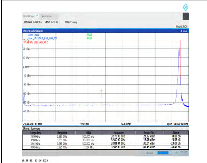
1-N77-3700-3980-PC2-30-100-H-5-CP-QPSK-Edge_1 RB_Right-1@272-Ant1-PASS-see graph
