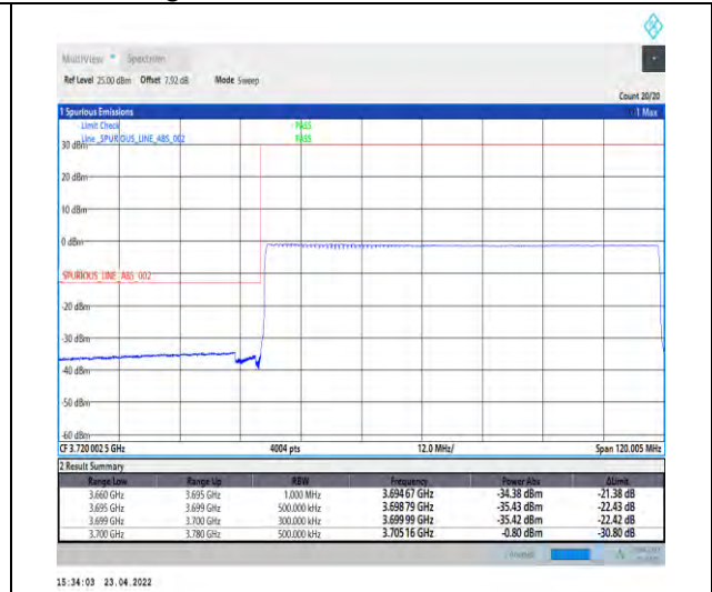
1-N77-3700-3980-PC2-30-80-L-6-CP-QPSK-Outer _Full-217@0-Ant1-PASS-see graph
