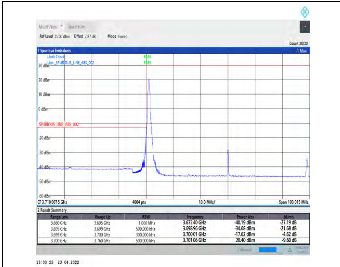
1-N77-3700-3980-PC2-30-60-L-4-CP-QPSK-Edge_1R_B_Left-1@0-Ant1-PASS-see graph
