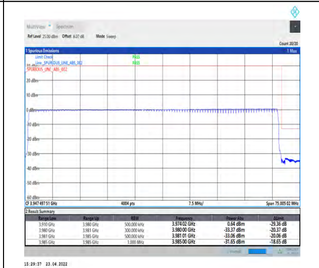
1-N77-3700-3980-PC2-30-70-H-6-CP-QPSK-Outer _Full-189@0-Ant1-PASS-see graph
