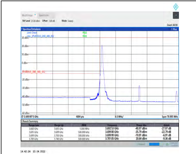
1-N77-3700-3980-PC2-30-40-L-4-CP-QPSK-Edge_1R B_Left-1@0-Ant1-PASS-see graph
