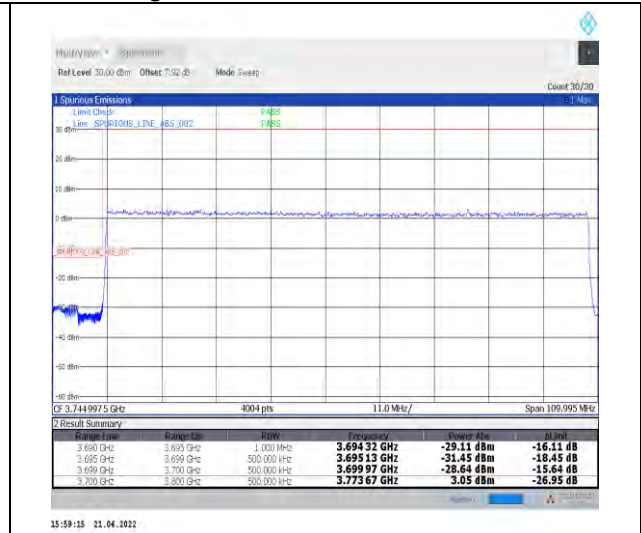
1-N77-3700-3980--30-100-L-3-DFT-PI2BPSK-Out er_Full-270@0-Ant1-PASS-see graph
