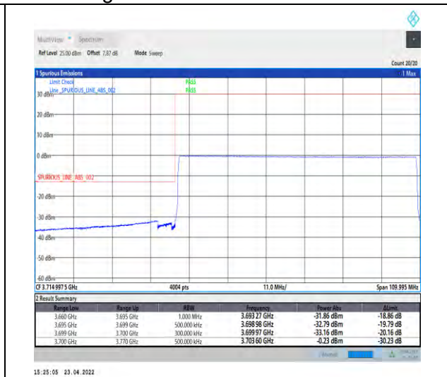
1-N77-3700-3980-PC2-30-70-L-6-CP-QPSK-Outer _Full-189@0-Ant1-PASS-see graph
