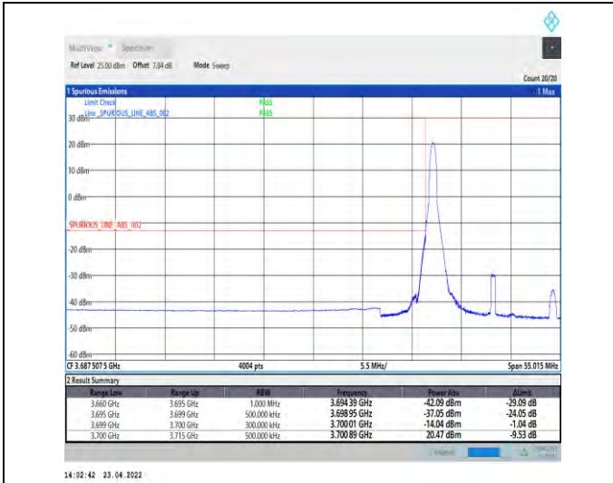
1-N77-3700-3980-PC2-30-15-L-4-CP-QPSK-Edge_1R B_Left-1@0-Ant1-PASS-see graph
