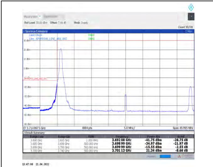
1-N77-3700-3980--30-40-L-1-DFT-PI2BPSK-Edge_1R_B_Left-1@0-Ant1-PASS-see graph
