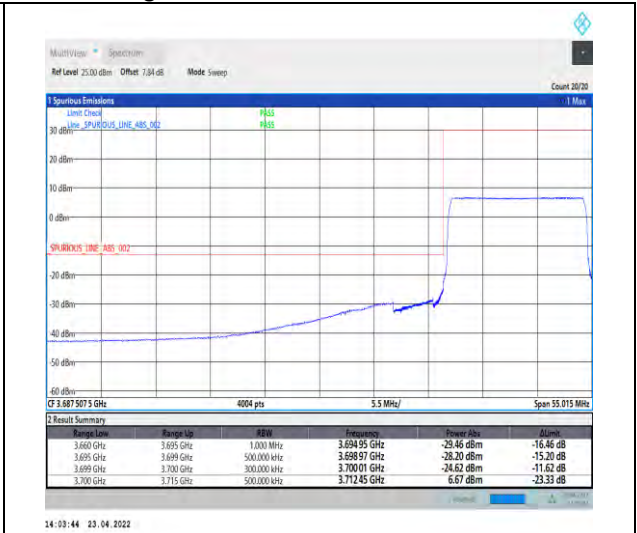
1-N77-3700-3980-PC2-30-15-L-6-CP-QPSK-Outer _Full-38@0-Ant1-PASS-see graph
