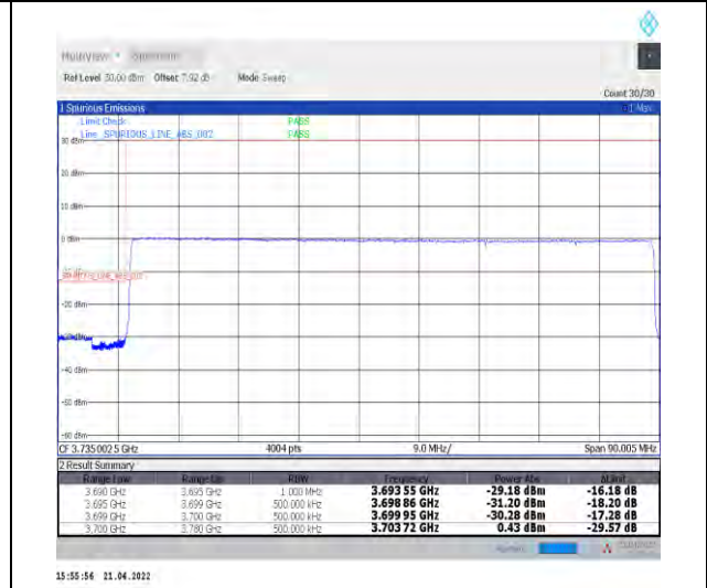
1-N77-3700-3980--30-80-L-6-CP-QPSK-Outer_Ful_I-217@0-Ant1-PASS-see graph
