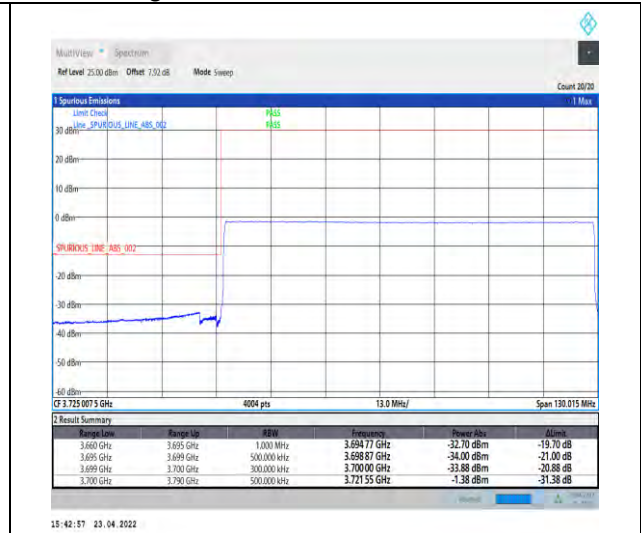
1-N77-3700-3980-PC2-30-90-L-6-CP-QPSK-Outer _Full-245@0-Ant1-PASS-see graph
