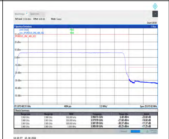
1-N77-3700-3980-PC2-30-20-H-6-CP-QPSK-Outer _Full-51@0-Ant1-PASS-see graph
