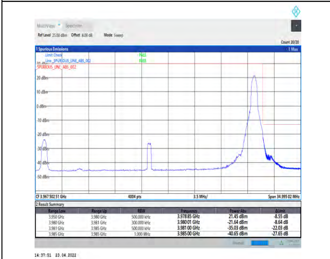
1-N77-3700-3980-PC2-30-30-H-5-CP-QPSK-Edge_1R B_Right-1@77-Ant1-PASS-see graph
