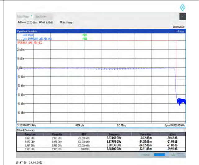
1-N77-3700-3980-PC2-30-90-H-6-CP-QPSK-Outer _Full-245@0-Ant1-PASS-see graph
