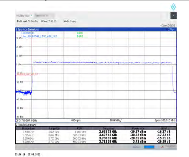
1-N77-3700-3980--30-90-L-3-DFT-PI2BPSK-Outer_Full-240@0-Ant1-PASS-see graph
