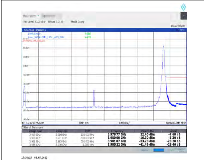
1-N77-3700-3980--30-70-H-5-CP-QPSK-Edge_1RB_R ight-1@188-Ant1-PASS-see graph
