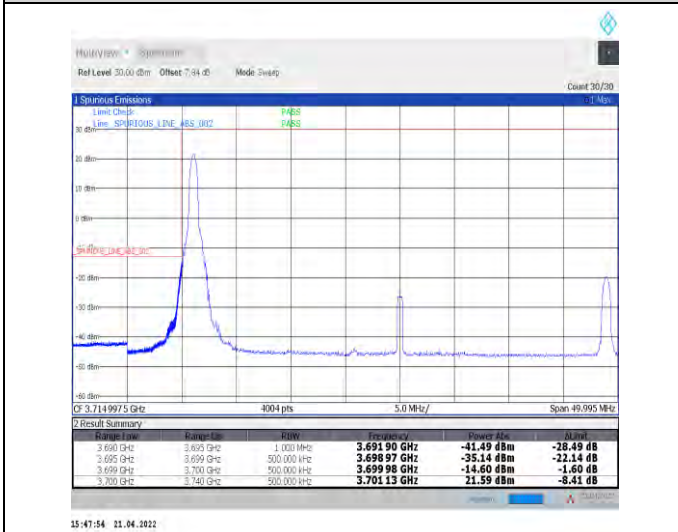
1-N77-3700-3980--30-40-L-4-CP-QPSK-Edge_1RB_L_eff-1@0-Ant1-PASS-see graph
