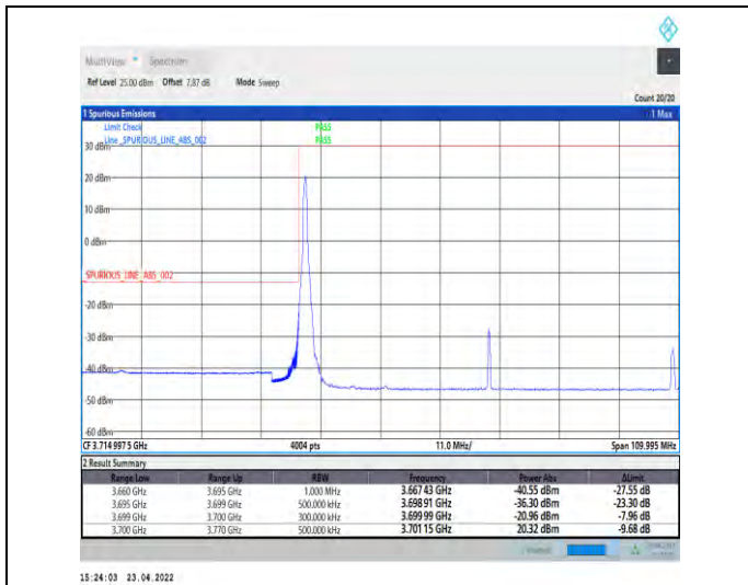
1-N77-3700-3980-PC2-30-70-L-4-CP-QPSK-Edge_1R B_Left-1@0-Ant1-PASS-see graph
