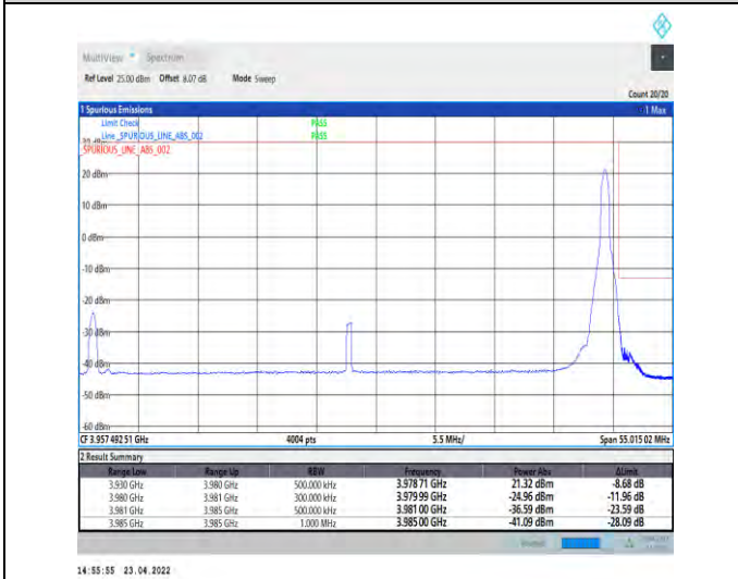
1-N77-3700-3980-PC2-30-50-H-5-CP-QPSK-Edge_1R_B_Right-1@132-Ant1-PASS-see graph
