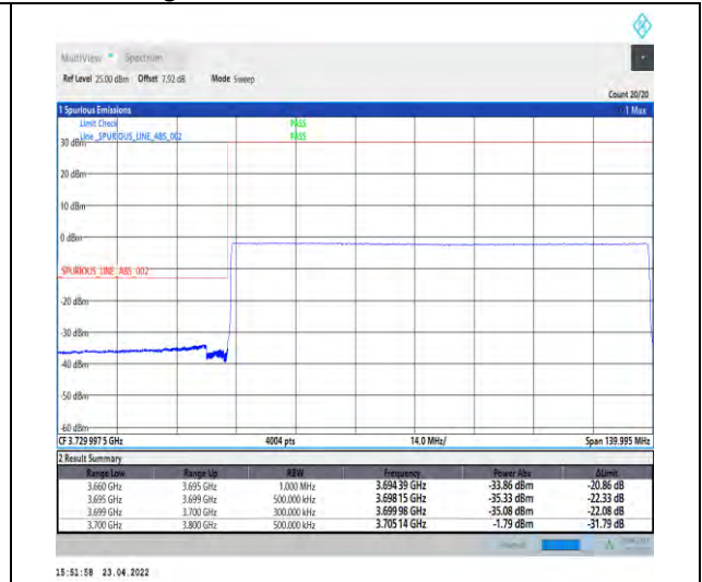
1-N77-3700-3980-PC2-30-100-L-6-CP-QPSK-Out er_Full-273@0-Ant1-PASS-see graph
