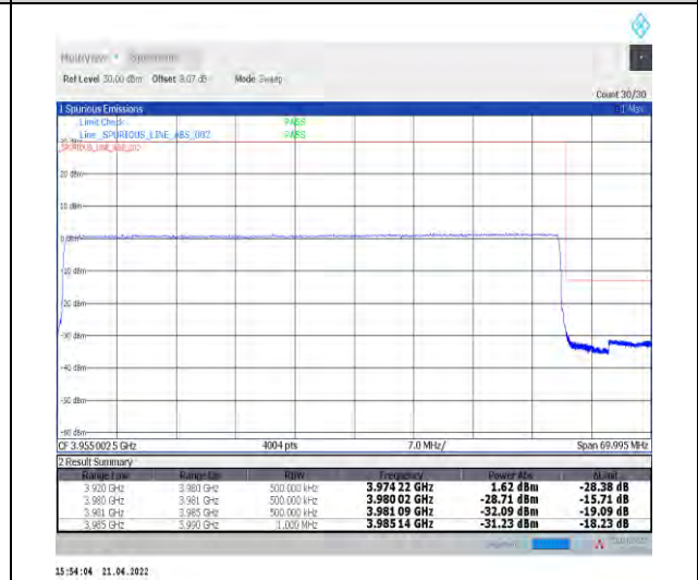
1-N77-3700-3980--30-60-H-6-CP-QPSK-Outer_Full-162@0-Ant1-PASS-see graph
