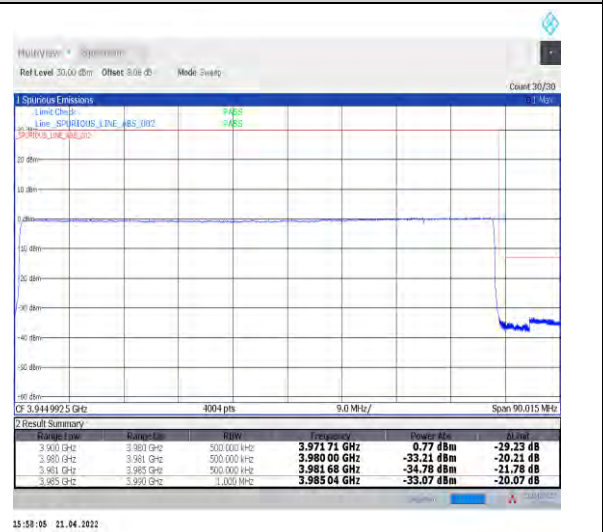
1-N77-3700-3980--30-80-H-6-CP-QPSK-Outer_Full-217@0-Ant1-PASS-see graph
