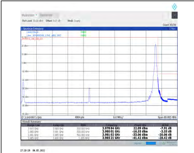
1-N77-3700-3980--30-70-H-2-DFT-PI2BPSK-Edge_1R_B_Right-1@188-Ant1-PASS-see graph
