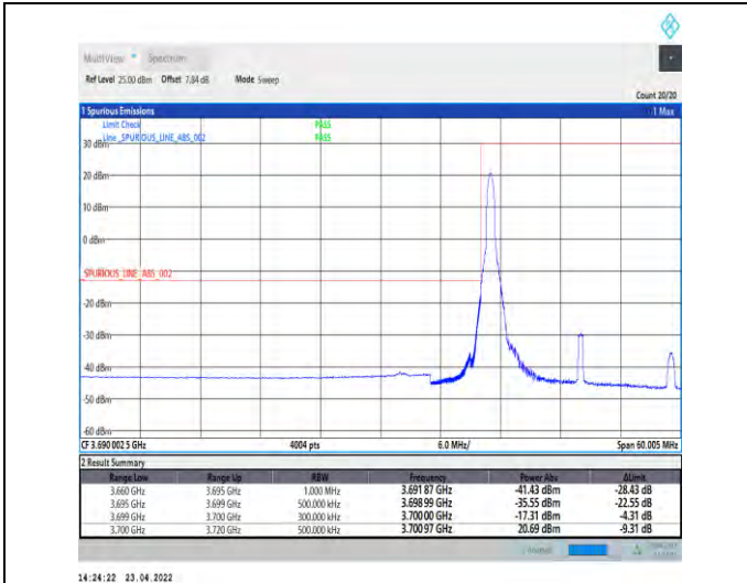
1-N77-3700-3980-PC2-30-20-L-4-CP-QPSK-Edge_1R B_Left-1@0-Ant1-PASS-see graph
