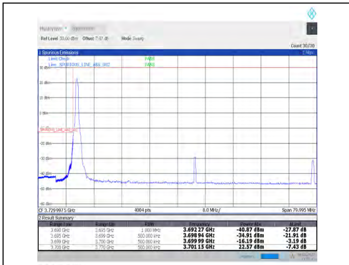
1-N77-3700-3980--30-70-L-1-DFT-PI2BPSK-Edge_1R_B_Left-1@0-Ant1-PASS-see graph
