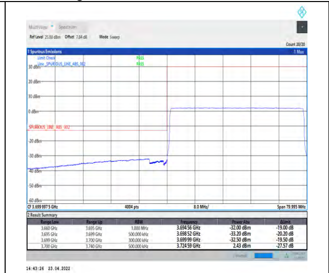
1-N77-3700-3980-PC2-30-40-L-6-CP-QPSK-Outer _Full-106@0-Ant1-PASS-see graph
