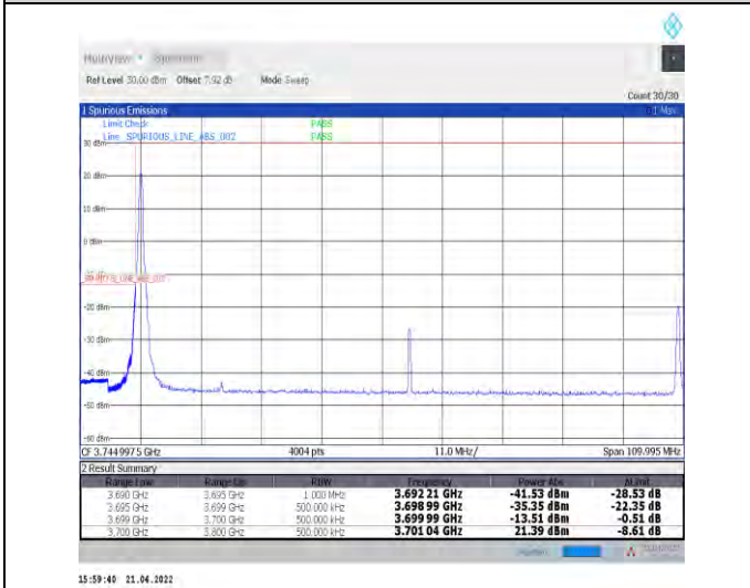
1-N77-3700-3980--30-100-L-4-CP-QPSK-Edge_1RB_Left-1@0-Ant1-PASS-see graph
