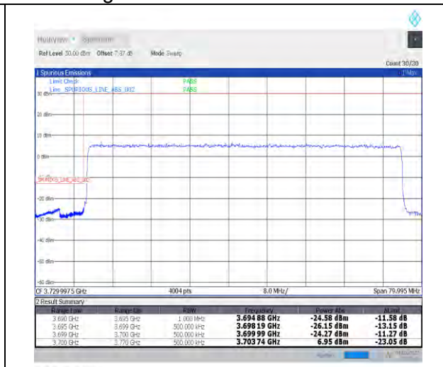
1-N77-3700-3980--30-70-L-3-DFT-PI2BPSK-Outer_Full-180@0-Ant1-PASS-see graph
