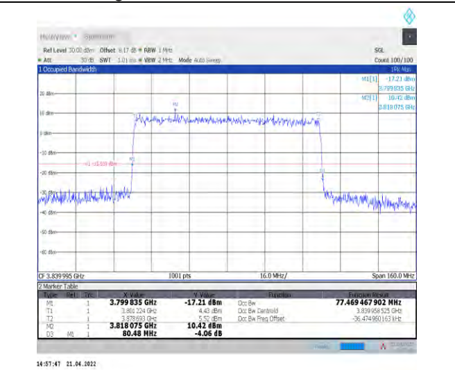
1-N77-3700-3980--30-80-M-9-CP-256QAM-Outer_Full ull-217@0-Ant1-77.469-80.480-≤80-PASS
