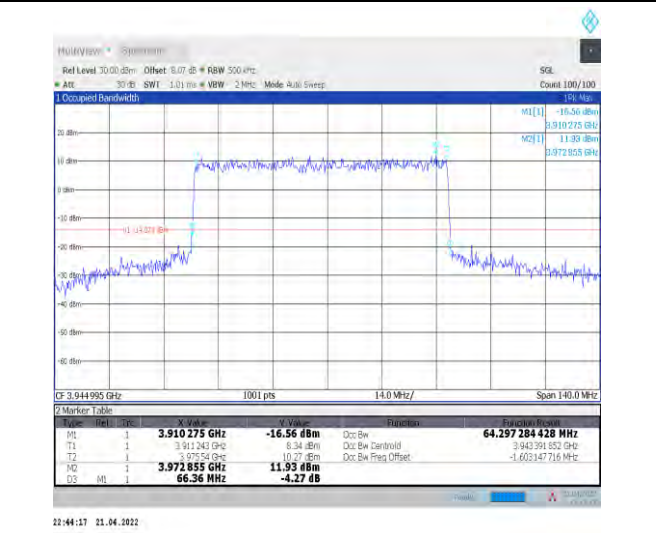
1-N77-3700-3980--30-70-H-1-DFT-QPSK-Outer_Full -180@0-Ant1-64.297-66.360-≤70-PASS
