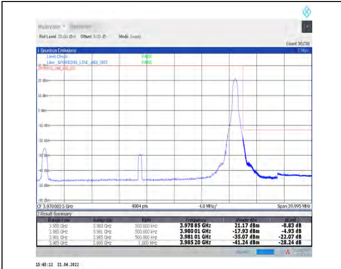
1-N77-3700-3980--30-30-H-2-DFT-PI2BPSK-Edge_1R_B_Right-1@77-Ant1-PASS-see graph
