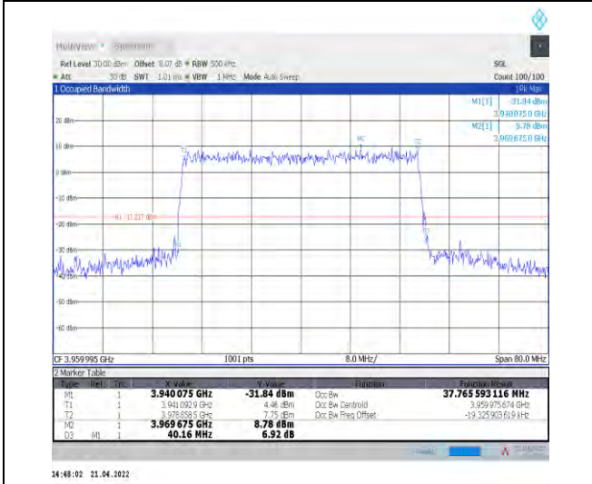
1-N77-3700-3980--30-40-H-9-CP-256QAM-Outer_Full -106@0-Ant1-37.692-40.160≤40-PASS
