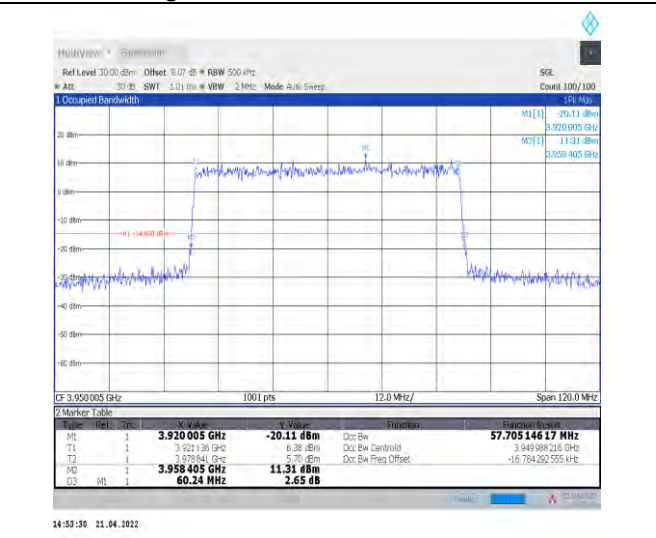
1-N77-3700-3980--30-60-H-6-CP-QPSK-Outer_Full-162@0-Ant1-57.705-60.240-≤60-PASS
