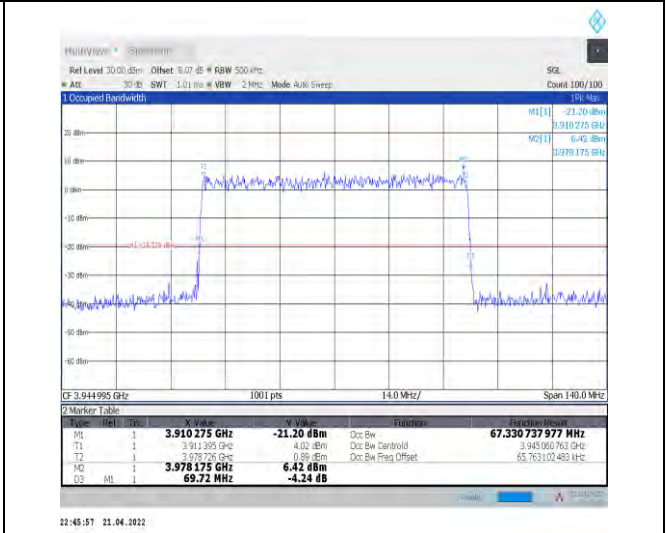
1-N77-3700-3980--30-70-H-9-CP-256QAM-Outer_Fu ll-189@0-Ant1-67.331-69.720-<=70-PASS
