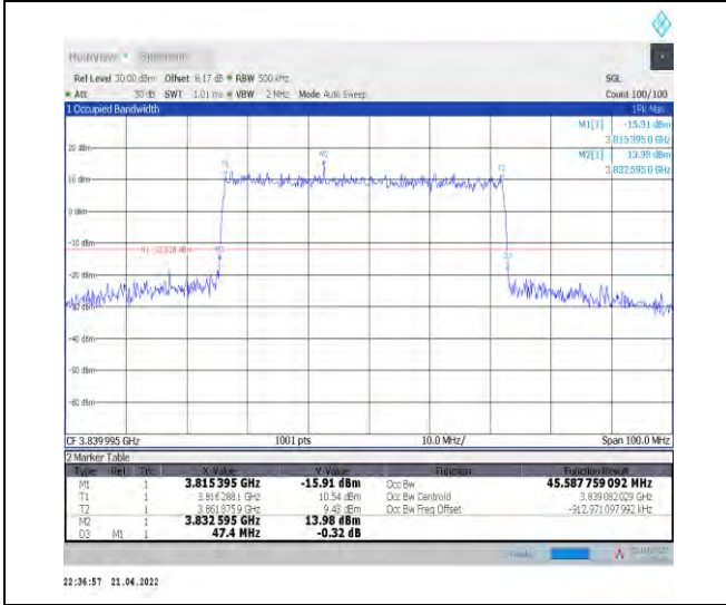
1-N77-3700-3980--30-50-M-3-DFT-16QAM-Outer_Full Full-128@0-Ant1-45.588-47.400-≤50-PASS
