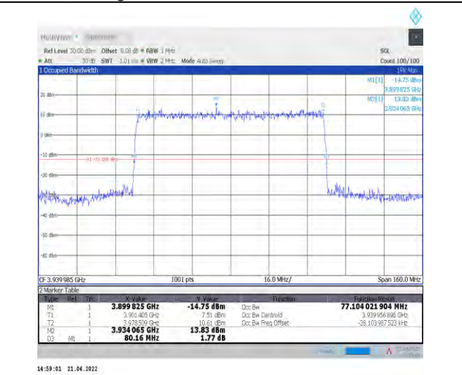
1-N77-3700-3980--30-80-H-4-DFT-64QAM-Outer_Full-216@0-Ant1-77.104-80.160-≤80-PASS
