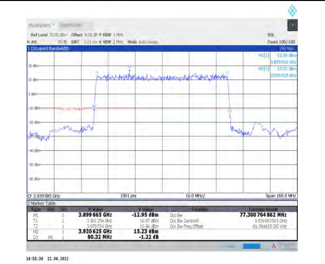
1-N77-3700-3980--30-80-H-2-DFT-PI2BPSK-Outer_Full Full-216@0-Ant1-77.301-80.320-≤80-PASS
