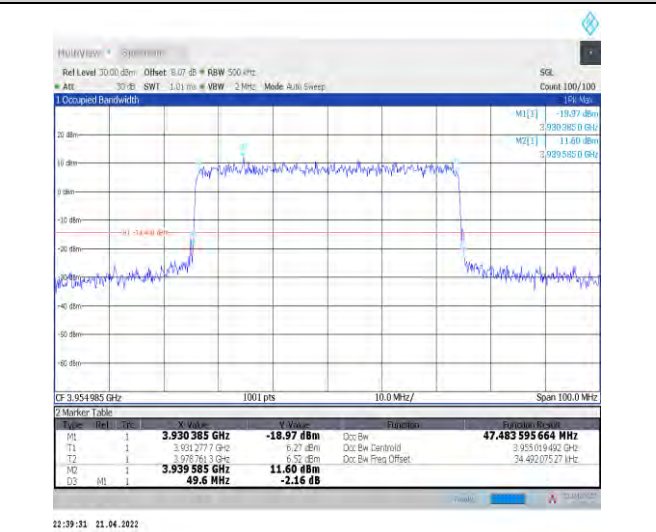
1-N77-3700-3980--30-50-H-7-CP-16QAM-Outer_Full-133@0-Ant1-47.484-49.600-≤50-PASS
