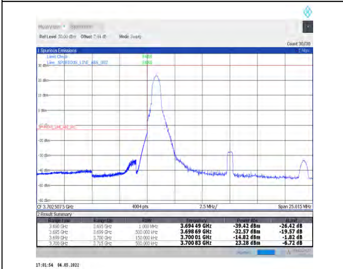
1-N77-3700-3980--30-15-L-4-CP-QPSK-Edge_1RB_L_eff-1@0-Ant1-PASS-see graph
