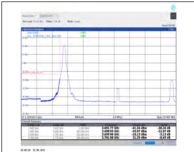
1-N77-3700-3980--30-30-L-1-DFT-PI2BPSK-Edge_1R_B_Left-1@0-Ant1-PASS-see graph
