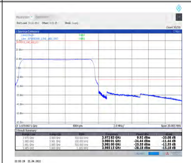
1-N77-3700-3980--30-10-H-6-CP-QPSK-Outer_Full-24@0-Ant1-PASS-see graph
