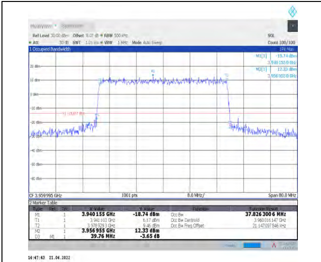
1-N77-3700-3980--30-40-H-7-CP-16QAM-Outer_Full -106@0-Ant1-37.823-39.760≤40-PASS
