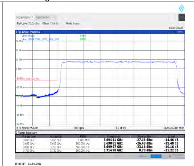
1-N77-3700-3980--30-30-L-3-DFT-PI2BPSK-Outer_Full-75@0-Ant1-PASS-see graph
