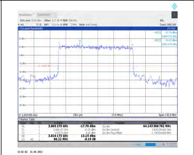
1-N77-3700-3980--30-70-M-2-DFT-PI2BPSK-Outer_Full-180@0-Ant1-64.144-66.220-<math>\leq 70</math>-PASS
