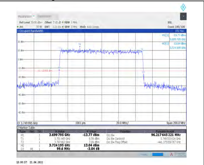
1-N77-3700-3980--30-100-L-4-DFT-64QAM-Outer_Full-270@0-Ant1-96.218-99.600-≤100-PASS
