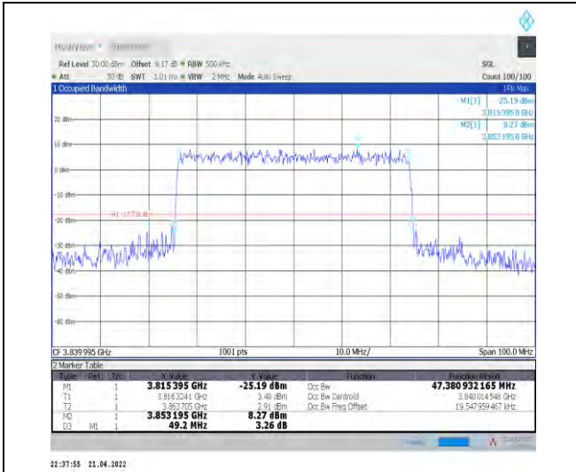
1-N77-3700-3980--30-50-M-9-CP-256QAM-Outer_Full-133@0-Ant1-47.381-49.200-≤50-PASS
