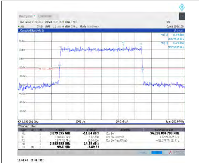
1-N77-3700-3980--30-100-H-1-DFT-QPSK-Outer_Fu II-270@0-Ant1-96.293-99.800-≤100-PASS
