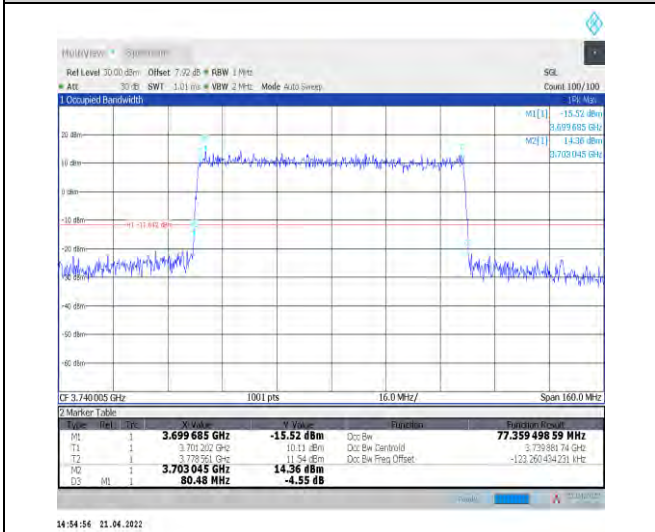
1-N77-3700-3980--30-80-L-3-DFT-16QAM-Outer_Full -216@0-Ant1-77.359-80.480-≤80-PASS
