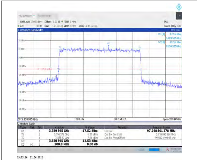
1-N77-3700-3980--30-100-M-6-CP-QPSK-Outer_Full-273@0-Ant1-97.249-100.800-≤100-PASS
