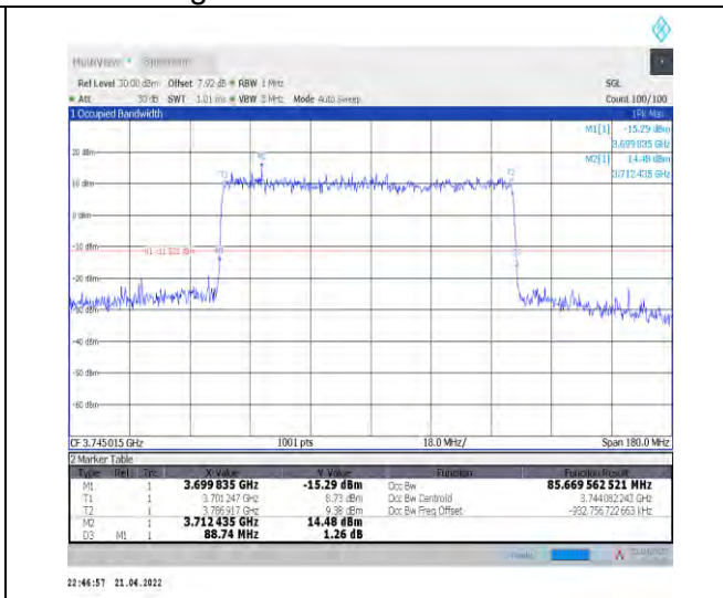
1-N77-3700-3980--30-90-L-3-DFT-16QAM-Outer_Full-240@0-Ant1-85.67-88.740-≤90-PASS
