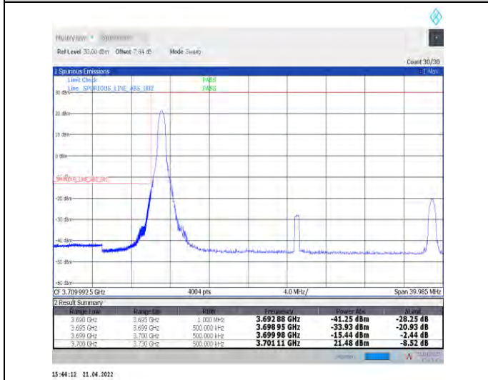
1-N77-3700-3980--30-30-L-4-CP-QPSK-Edge_1RB_L_eff-1@0-Ant1-PASS-see graph
