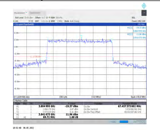
1-N77-3700-3980--30-70-M-8-CP-64QAM-Outer_Full -189@0-Ant1-67.457-69.720-≤70-PASS
