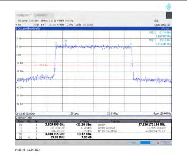
1-N77-3700-3980--30-60-M-1-DFT-QPSK-Outer_Full -162@0-Ant1-57.836-59.880-≤60-PASS
