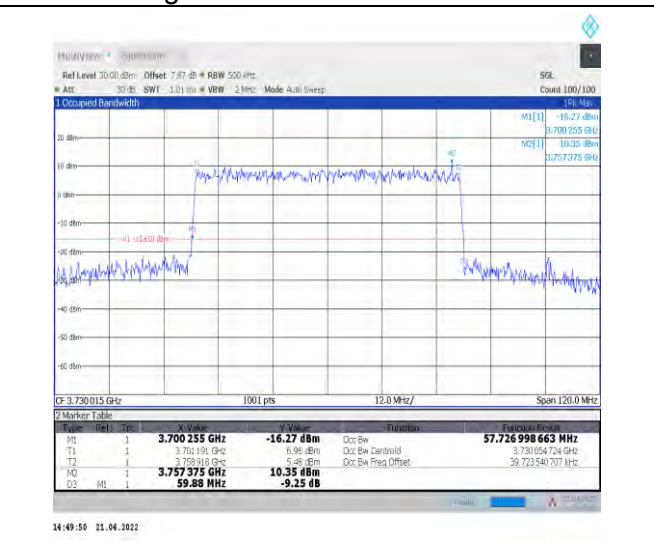
1-N77-3700-3980--30-60-L-8-CP-64QAM-Outer_Full 162@0-Ant1-57.727-59.880-≤60-PASS
