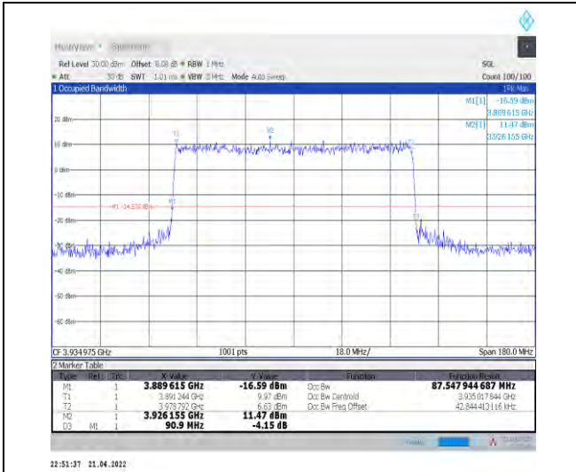
1-N77-3700-3980--30-90-H-8-CP-64QAM-Outer_Full -245@0-Ant1-87.548-90.900-≤90-PASS
