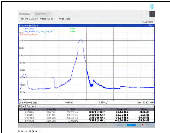
1-N77-3700-3980--30-10-H-2-DFT-PI2BPSK-Edge_1R_B_Right-1@23-Ant1-PASS-see graph
