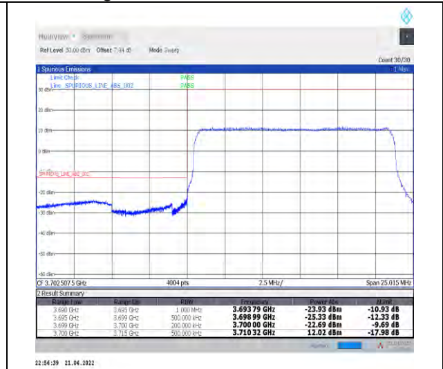
1-N77-3700-3980--30-15-L-3-DFT-PI2BPSK-Outer_Full-36@0-Ant1-PASS-see graph
