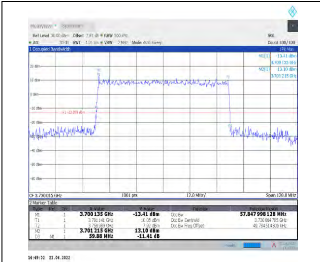
1-N77-3700-3980--30-60-L-3-DFT-16QAM-Outer_Fu II-162@0-Ant1-57.848-59.880-≤60-PASS
