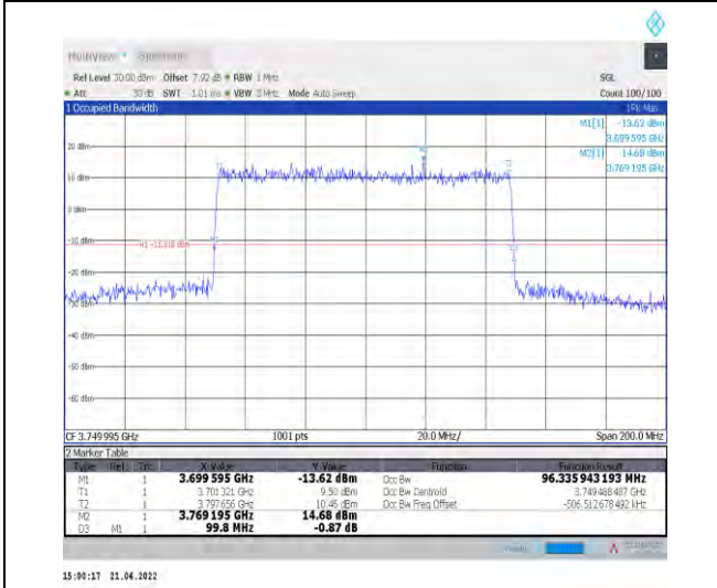
1-N77-3700-3980--30-100-L-1-DFT-QPSK-Outer_Fu ll-270@0-Ant1-96.336-99.800-≤100-PASS
