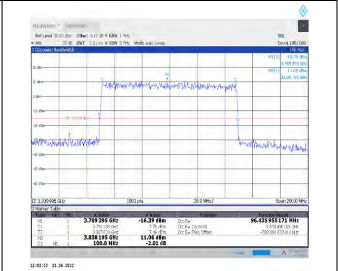
1-N77-3700-3980--30-100-M-5-DFT-256QAM-Outer_Full-270@0-Ant1-96.436-100.000-≤100-PASS
