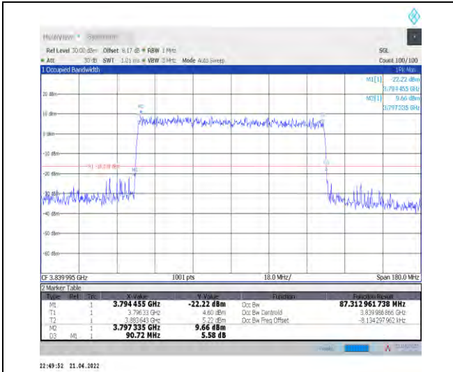
1-N77-3700-3980--30-90-M-9-CP-256QAM-Outer_Full-245@0-Ant1-87.313-90.720-<math>\leq 90</math>-PASS
