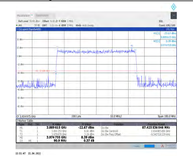
1-N77-3700-3980--30-90-H-9-CP-256QAM-Outer_Fu ll-245@0-Ant1-87.426-90.900-≤90-PASS
