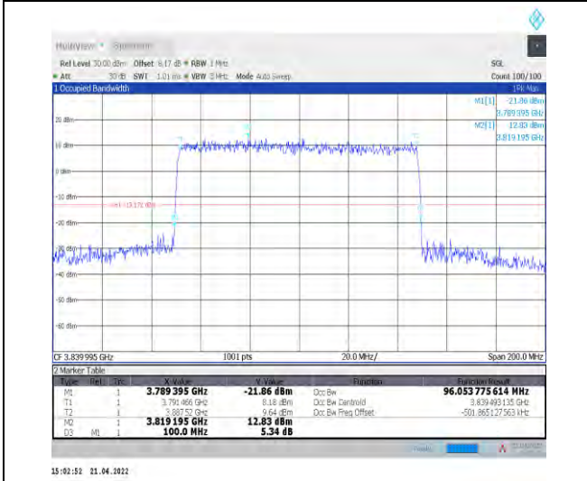
1-N77-3700-3980--30-100-M-4-DFT-64QAM-Outer_Full-270@0-Ant1-96.054-100.000-≤100-PASS
