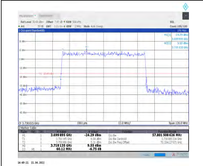
1-N77-3700-3980--30-60-L-5-DFT-256QAM-Outer_Full-162@0-Ant1-57.802-60.120-≤60-PASS
