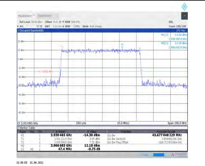
1-N77-3700-3980--30-50-H-3-DFT-16QAM-Outer_Full-128@0-Ant1-45.677-47.400-≤50-PASS
