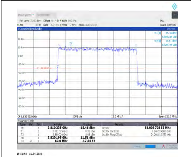
1-N77-3700-3980--30-60-M-4-DFT-64QAM-Outer_Full-162@0-Ant1-58.009-60.000-≤60-PASS
