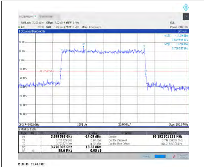
1-N77-3700-3980--30-100-L-3-DFT-16QAM-Outer_Full-270@0-Ant1-96.192-99.600-≤100-PASS
