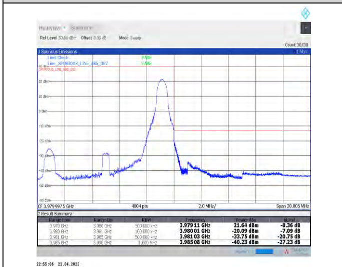
1-N77-3700-3980--30-10-H-5-CP-QPSK-Edge_1RB_Right-1@23-Ant1-PASS-see graph
