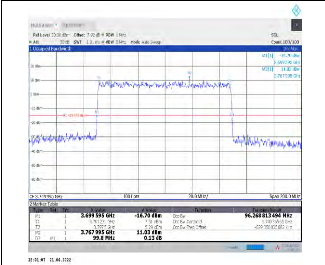
1-N77-3700-3980--30-100-L-5-DFT-256QAM-Outer_Full-270@0-Ant1-96.269-99.800-≤100-PASS
