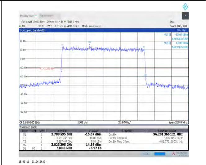
1-N77-3700-3980--30-100-M-1-DFT-QPSK-Outer_Fu I1-270@0-Ant1-96.201-100.000-≤100-PASS
