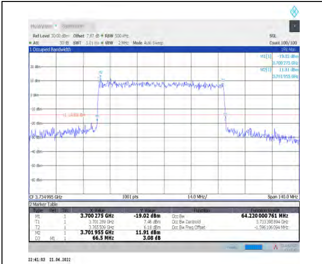
1-N77-3700-3980--30-70-L-4-DFT-64QAM-Outer_Full-180@0-Ant1-64.22-66.500-<=70-PASS
