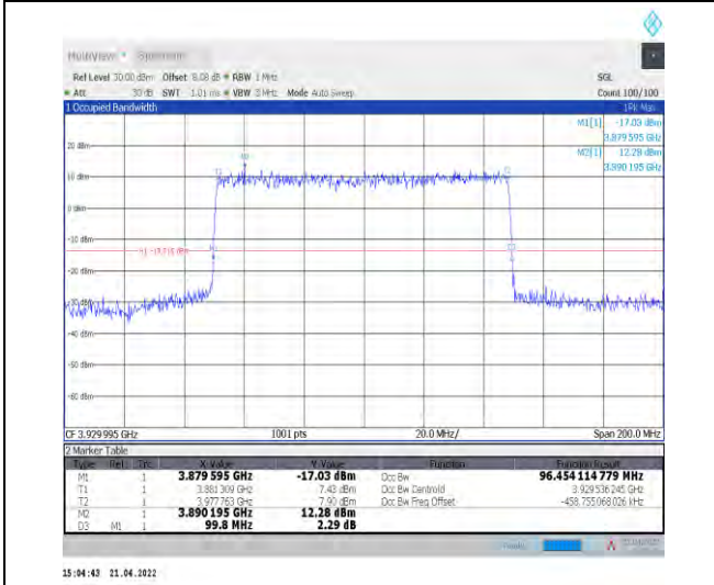
1-N77-3700-3980--30-100-H-3-DFT-16QAM-Outer_Full-270@0-Ant1-96.454-99.800-≤100-PASS
