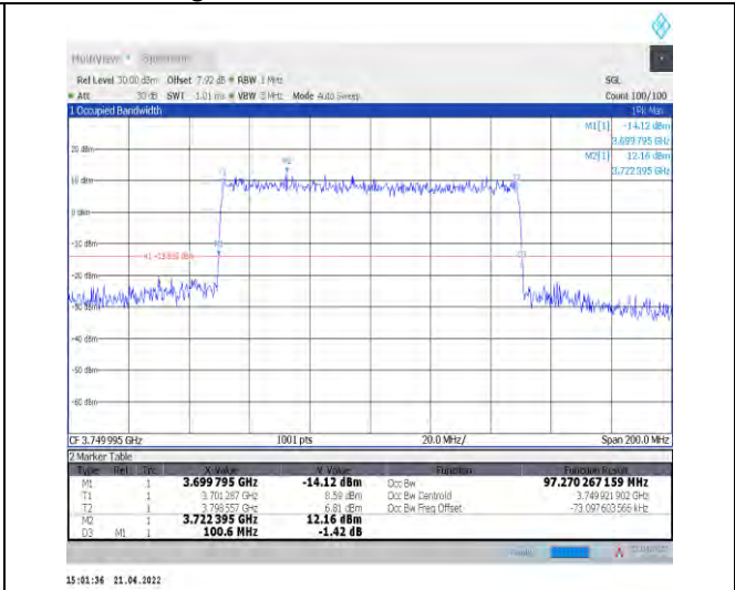
1-N77-3700-3980--30-100-L-8-CP-64QAM-Outer_Fu I-273@0-Ant1-97.27-100.600-≤100-PASS
