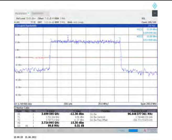
1-N77-3700-3980--30-100-L-2-DFT-PI2BPSK-Outer_Full Full-270@0-Ant1-96.448-99.800-≤100-PASS
