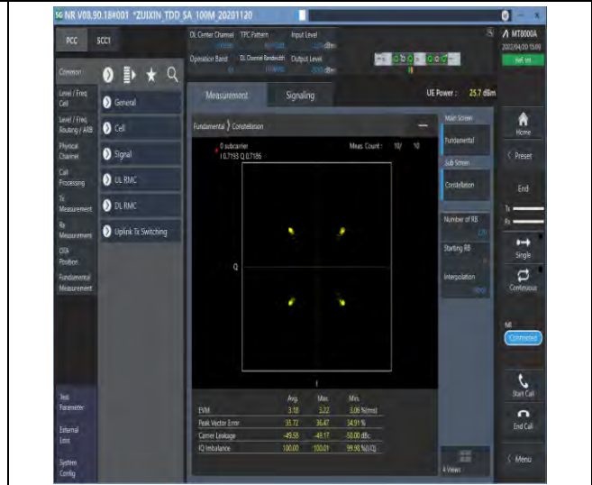
1-N41--30-100-M-2-DFT-QPSK-Outer_Full-270@0- Ant1-see graph-PASS
