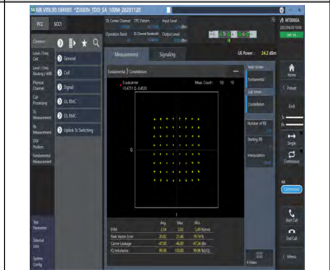
1-N41--30-100-M-4-DFT-64QAM-Outer_Full-270@0 -Ant1-see graph-PASS
