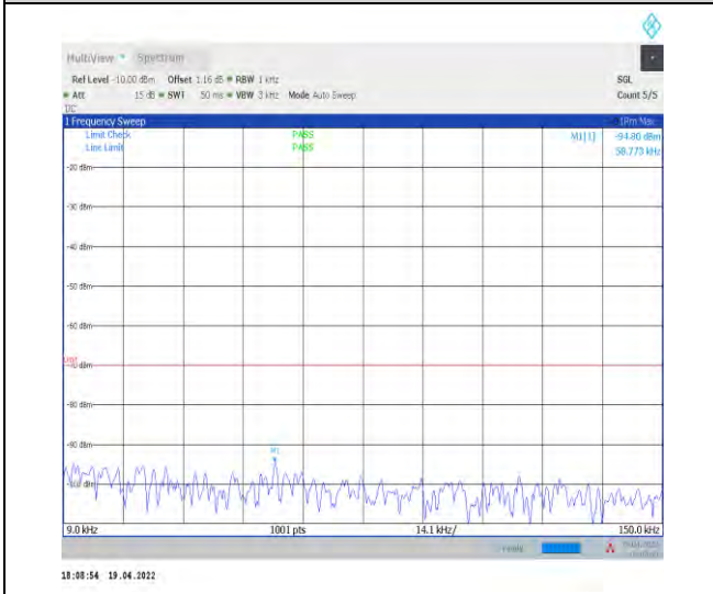
1-N30--15-10-M-1-DFT-PI2BPSK-Inner_1RB_Left-1 @1-0.009-0.15-Ant1--94.80--70-PASS
