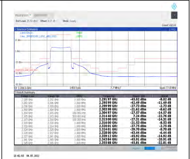
1-N30--15-10-H-6-CP-QPSK-Outer_Full-52@0-Ant1-PASS-see graph
