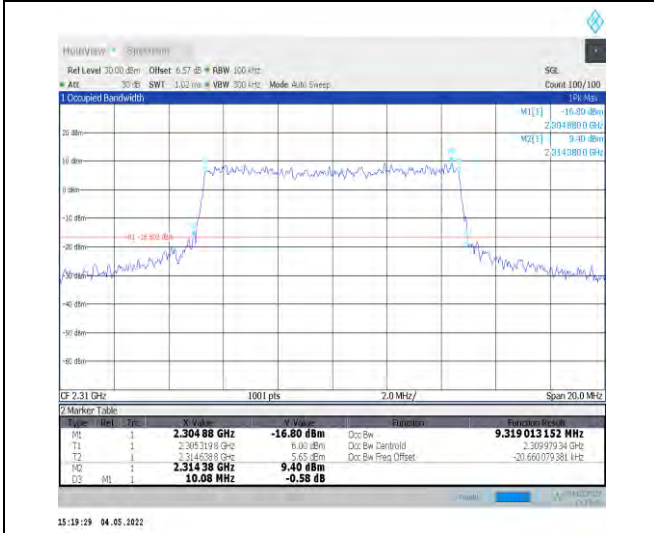
1-N30--15-10-L-8-CP-64QAM-Outer_Full-52@0-Ant1-9.319-10.080-≤10-PASS
