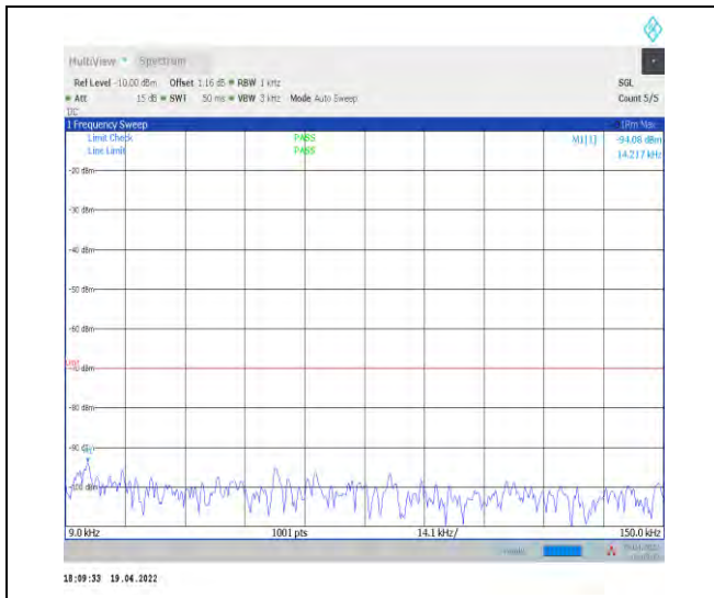
1-N30--15-10-H-1-DFT-PI2BPSK-Inner_1RB_Left-1 @1-0.009-0.15-Ant1--94.08--70-PASS
