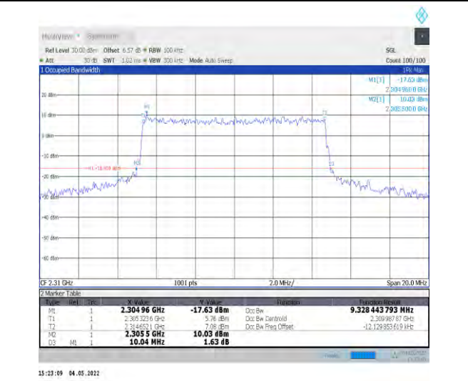
1-N30--15-10-H-7-CP-16QAM-Outer_Full-52@0-Ant 1-9.328-10.040-≤10-PASS
