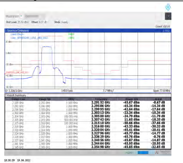
1-N30--30-10-L-3-DFT-PI2BPSK-Outer_Full-24@0-Ant1-PASS-see graph
