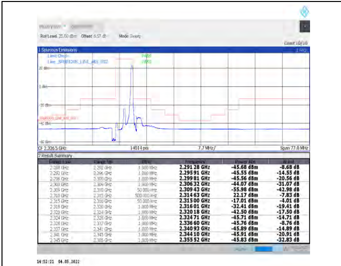
1-N30--15-5-H-2-DFT-PI2BPSK-Edge_1RB_Right-1@2 4-Ant1-PASS-see graph
