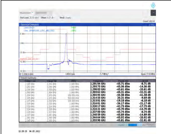
1-N30--15-10-H-5-CP-QPSK-Edge_1RB_Right-1@51-Ant1-PASS-see graph
