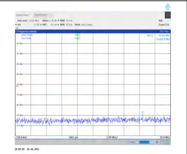
1-N30--15-10-M-1-DFT-PI2BPSK-Inner_1RB_Left-1 @1-0.15-30-Ant1--90.20--60-PASS
