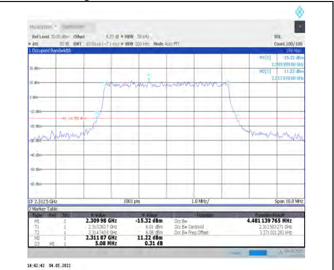
1-N30--15-5-H-4-DFT-64QAM-Outer_Full-25@0-Ant 1-4.481-5.080-≤5-PASS
