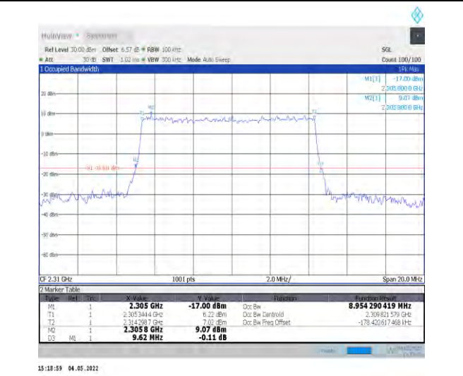
1-N30--15-10-L-5-DFT-256QAM-Outer_Full-50@0-A nt1-8.954-9.620-≤10-PASS
