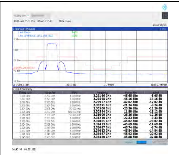
1-N30--15-5-L-3-DFT-PI2BPSK-Outer_Full-25@0-Ant1-PASS-see graph
