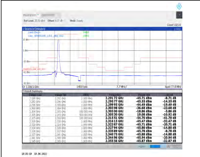
1-N30--30-10-L-4-CP-QPSK-Edge_1RB_Left-1@0-Ant1-PASS-see graph
