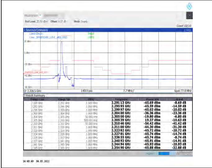
1-N30--15-5-L-4-CP-QPSK-Edge_1RB_Left-1@0-Ant1-PASS-see graph
