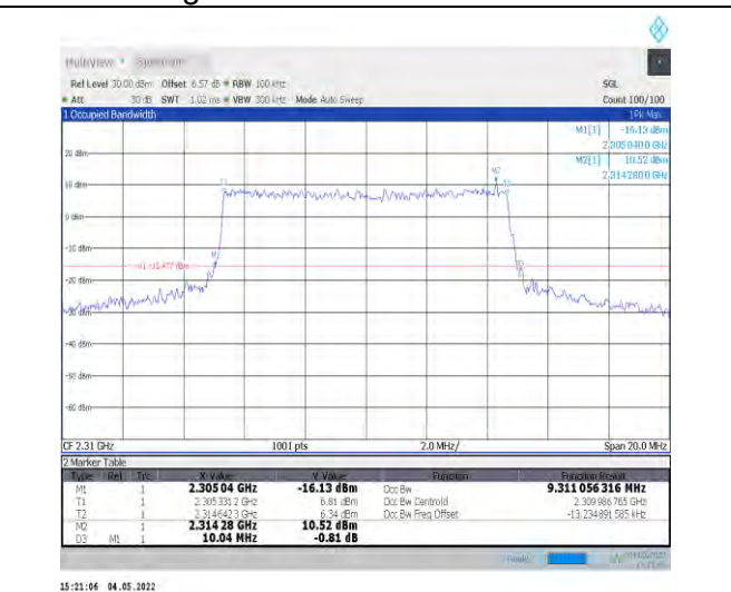
1-N30--15-10-M-6-CP-QPSK-Outer_Full-52@0-Ant1-9.311-10.040-≤10-PASS
