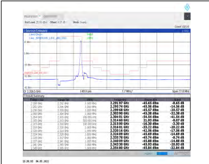
1-N30--15-10-H-2-DFT-PI2BPSK-Edge_1RB_Right-1@51-Ant1-PASS-see graph
