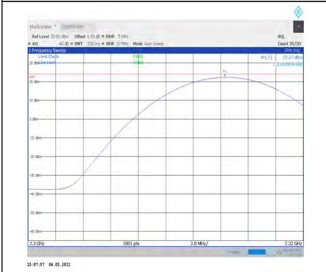
1-N30-PC3-15-10-L-2-DFT-PI2BPSK-Inner_1RB_Ri ght-1@50-2300-2320-Ant1-22.27-23.98-PASS
