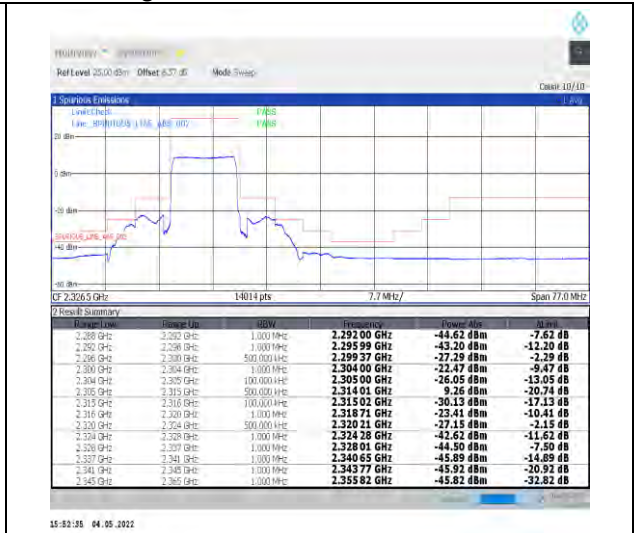
1-N30--15-10-H-3-DFT-PI2BPSK-Outer_Full-50@0-Ant1-PASS-see graph
