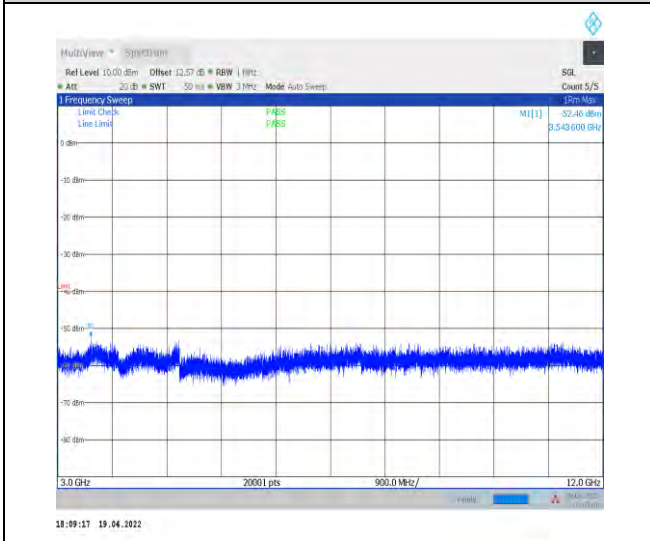
1-N30--15-10-M-1-DFT-PI2BPSK-Inner_1RB_Left-1 @1-3000-12000-Ant1--52.46--40-PASS
