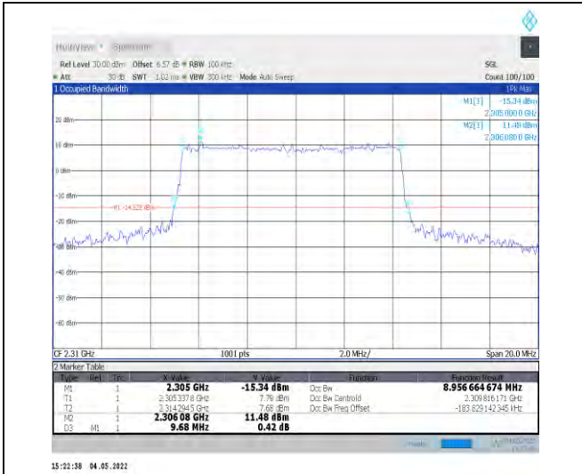
1-N30--15-10-H-4-DFT-64QAM-Outer_Full-50@0-An t1-8.957-9.680-≤10-PASS
