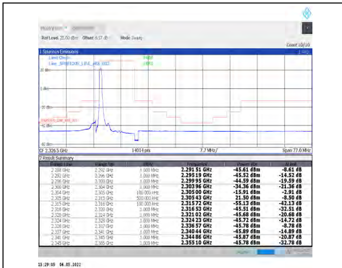
1-N30--15-10-L-1-DFT-PI2BPSK-Edge_1RB_Left-1@0-Ant1-PASS-see graph
