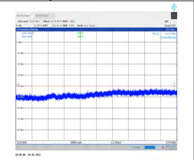
1-N30--15-10-L-1-DFT-PI2BPSK-Inner_1RB_Left-1 @1-12000-27000-Ant1--41.11--40-PASS
