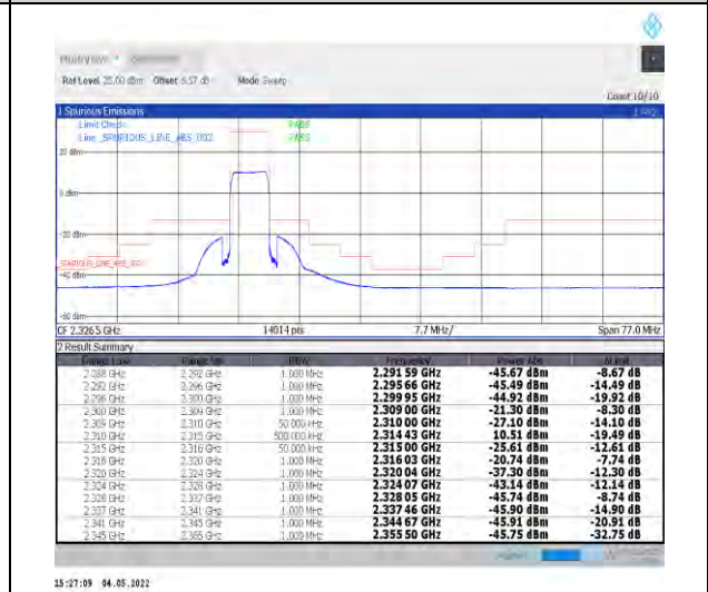
1-N30--15-5-H-6-CP-QPSK-Outer_Full-25@0-Ant 1-PASS-see graph
