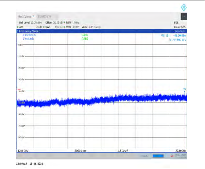
1-N30--15-10-M-1-DFT-PI2BPSK-Inner_1RB_Left-1 @1-12000-27000-Ant1--41.20--40-PASS
