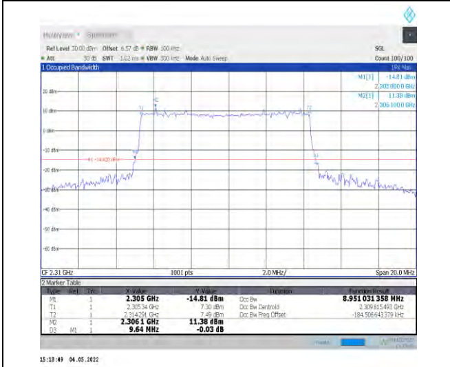
1-N30--15-10-L-4-DFT-64QAM-Outer_Full-50@0-An t1-8.951-9.640-≤10-PASS
