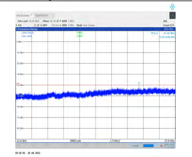
1-N30--15-10-H-1-DFT-PI2BPSK-Inner_1RB_Left-1 @1-12000-27000-Ant1--41.30--40-PASS
