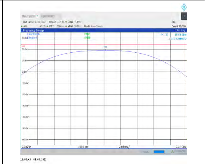
1-N30-PC3-15-10-L-3-DFT-PI2BPSK-Outer_Full-50 @0-2300-2320-Ant1-18.82-23.98-PASS
