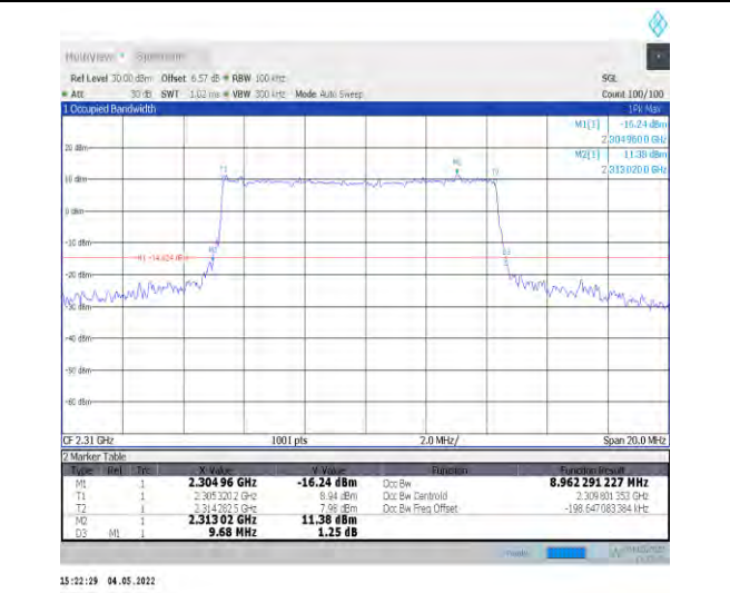
1-N30--15-10-H-3-DFT-16QAM-Outer_Full-50@0-Ant t1-8.962-9.680-≤10-PASS
