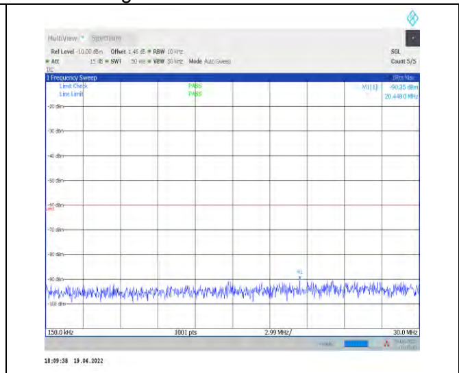
1-N30--15-10-H-1-DFT-PI2BPSK-Inner_1RB_Left-1 @1-0.15-30-Ant1--90.35--60-PASS
