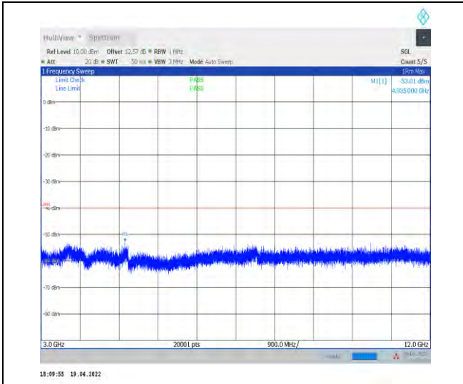
1-N30--15-10-H-1-DFT-PI2BPSK-Inner_1RB_Left-1 @1-3000-12000-Ant1--53.01--40-PASS
