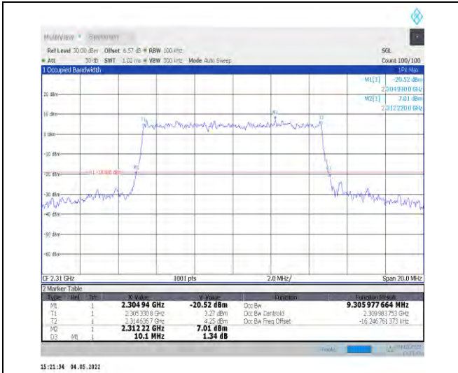
1-N30--15-10-M-9-CP-256QAM-Outer_Full-52@0-A nt1-9.306-10.100-≤10-PASS
