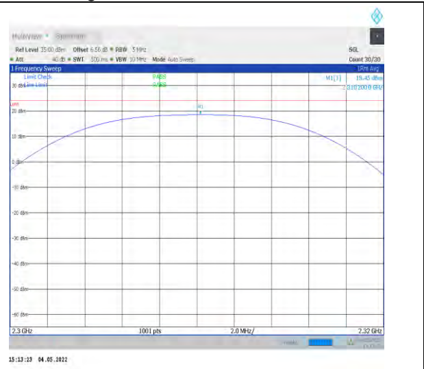
1-N30-PC3-15-10-H-3-DFT-PI2BPSK-Outer_Full-50 @0-2300-2320-Ant1-18.45-23.98-PASS
