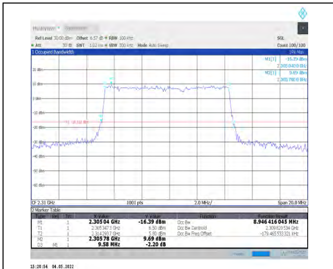
1-N30--15-10-M-5-DFT-256QAM-Outer_Full-50@0-Ant1-8.946-9.580-≤10-PASS
