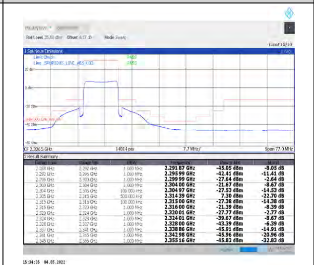
1-N30--15-10-L-6-CP-QPSK-Outer_Full-52@0-Ant1-PASS-see graph
