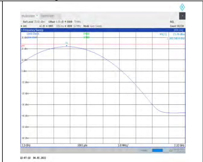
1-N30-PC3-15-10-L-1-DFT-PI2BPSK-Inner_1RB_Left -1@1-2300-2320-Ant1-21.78-23.98-PASS
