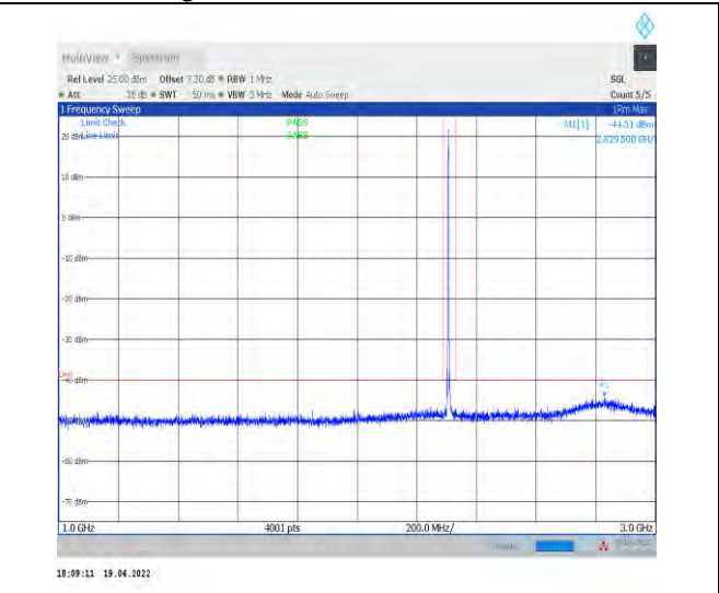
1-N30--15-10-M-1-DFT-PI2BPSK-Inner_1RB_Left-1 @1-1000-3000-Ant1--44.51--40-PASS
