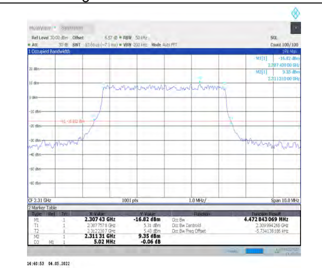
1-N30--15-5-M-5-DFT-256QAM-Outer_Full-25@0-An t1-4.473-5.020-≤5-PASS
