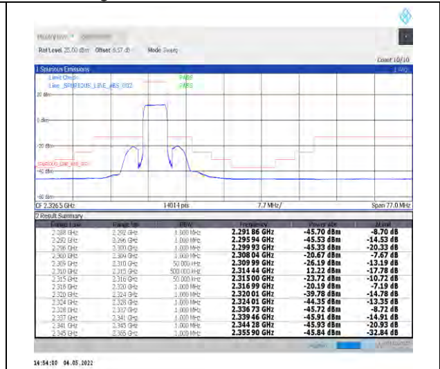
1-N30--15-5-H-3-DFT-PI2BPSK-Outer_Full-25@0 -Ant1-PASS-see graph
