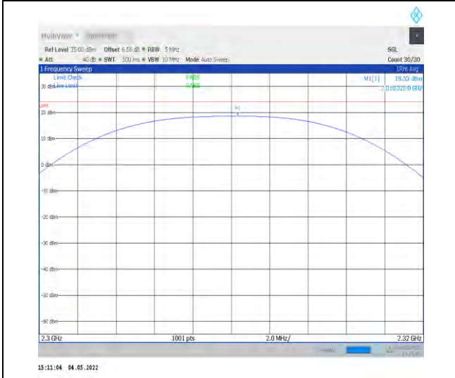
1-N30-PC3-15-10-M-3-DFT-PI2BPSK-Outer_Full-50 @0-2300-2320-Ant1-18.53-23.98-PASS
