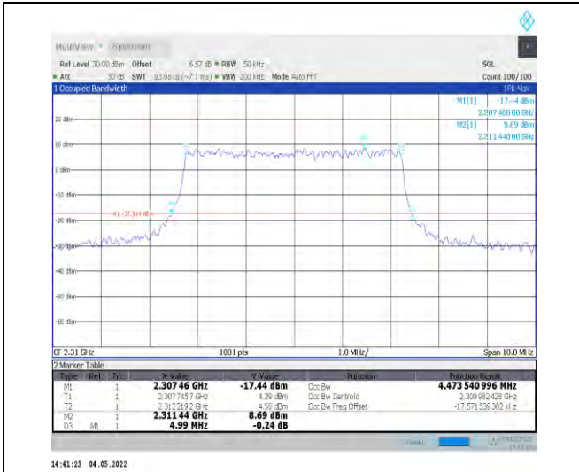
1-N30--15-5-M-8-CP-64QAM-Outer_Full-25@0-Ant1 -4.474-4.990-≤5-PASS
