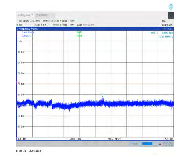
1-N30--30-15-L-1-DFT-PI2BPSK-Inner_1RB_Left-1 @1-3000-12000-Ant1--53.02--40-PASS
