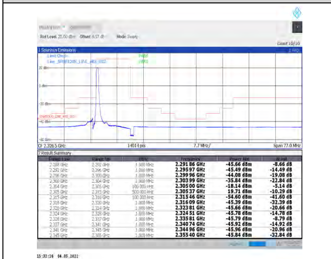
1-N30--15-10-L-4-CP-QPSK-Edge_1RB_Left-1@0-Ant1-PASS-see graph
