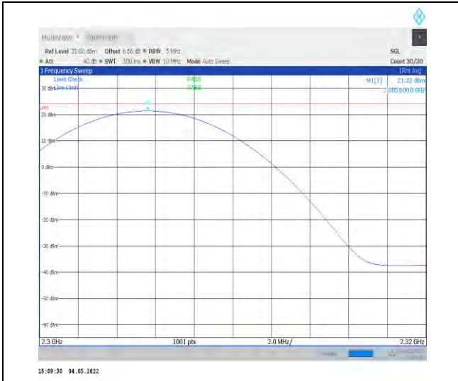
1-N30-PC3-15-10-M-1-DFT-PI2BPSK-Inner_1RB_L eff-1@1-2300-2320-Ant1-21.32-23.98-PASS
