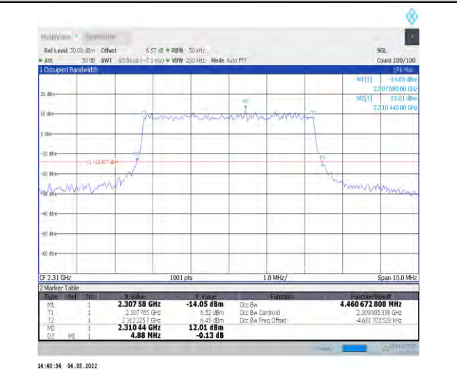
1-N30--15-5-M-3-DFT-16QAM-Outer_Full-25@0-Ant 1-4.461-4.880-≤5-PASS
