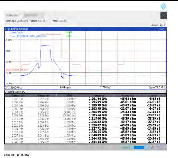
1-N30--30-10-L-6-CP-QPSK-Outer_Full-24@0-Ant1-PASS-see graph
