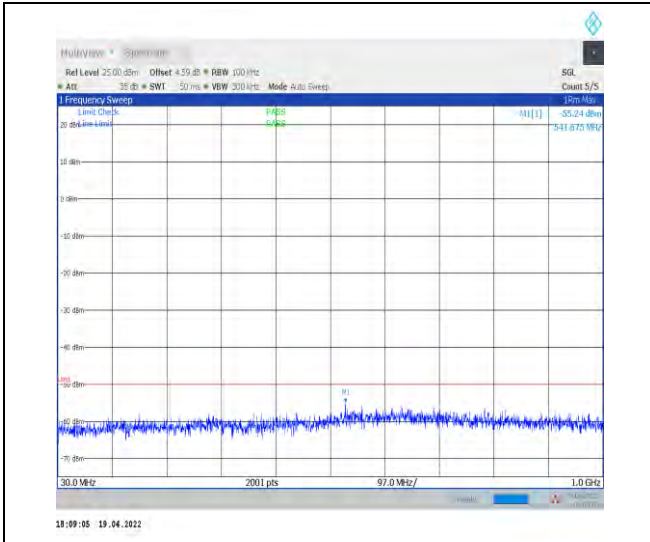
1-N30--15-10-M-1-DFT-PI2BPSK-Inner_1RB_Left-1 @1-30-1000-Ant1--55.24--50-PASS
