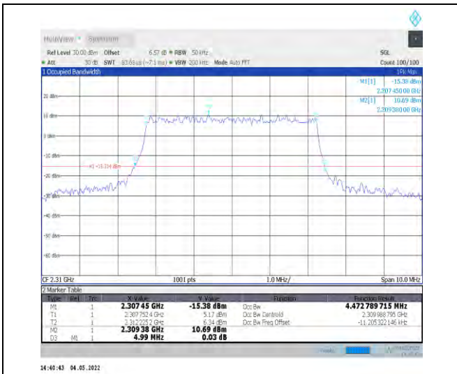
1-N30--15-5-M-4-DFT-64QAM-Outer_Full-25@0-Ant 1-4.473-4.990-≤5-PASS
