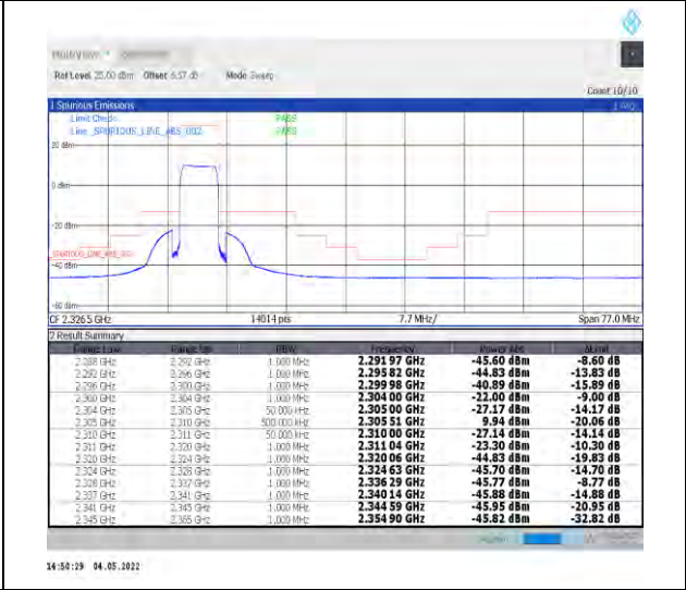
1-N30--15-5-L-6-CP-QPSK-Outer_Full-25@0-Ant1-PASS-see graph
