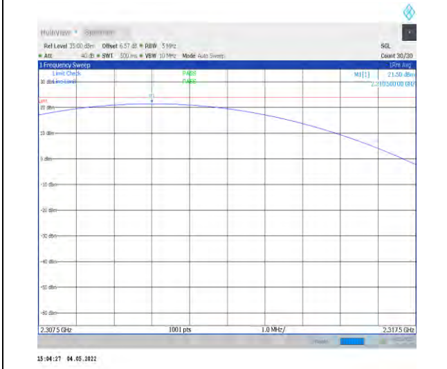
1-N30-PC3-15-5-H-1-DFT-PI2BPSK-Inner_1RB_Lef t-1@1-2307.5-2317.5-Ant1-21.50-23.98-PASS
