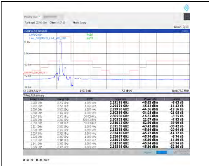
1-N30--15-5-L-1-DFT-PI2BPSK-Edge_1RB_Left-1@0-Ant1-PASS-see graph
