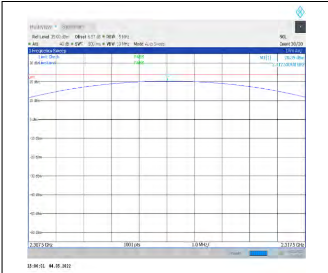
1-N30-PC3-15-5-H-3-DFT-PI2BPSK-Outer_Full-25 @0-2307.5-2317.5-Ant1-20.39-23.98-PASS
