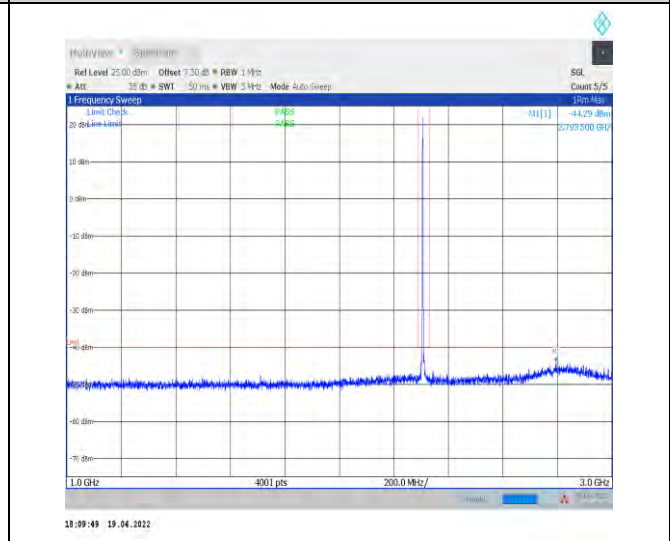
1-N30--15-10-H-1-DFT-PI2BPSK-Inner_1RB_Left-1 @1-1000-3000-Ant1--44.29--40-PASS
