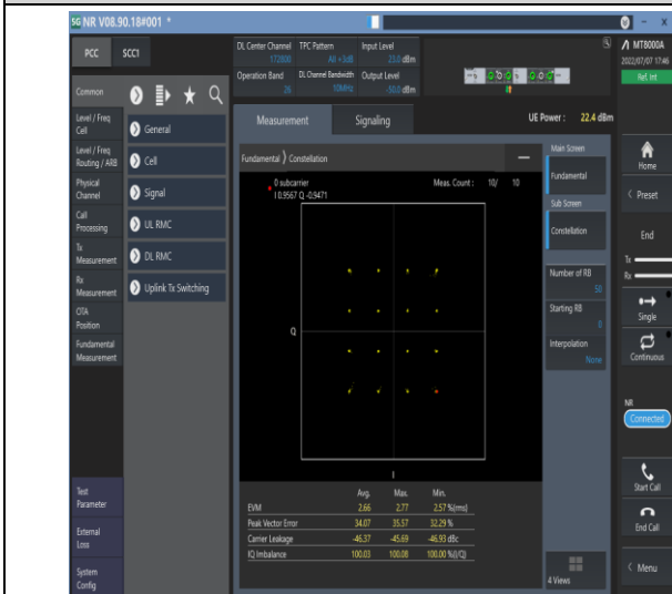
1-N26-814-824--15-10-M-3-DFT-16QAM-Outer_Full-5 0@0-Ant1-see graph-PASS
