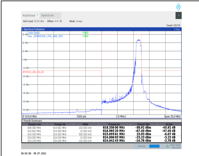
1-N26-814-824--15-5-H-2-DFT-PI2BPSK-Edge_1RB_Right-1@24-Ant1-PASS-see graph
