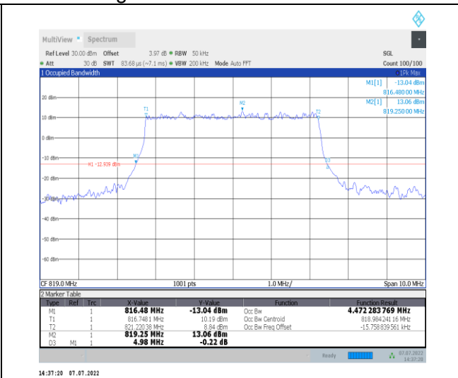
1-N26-814-824--15-5-M-1-DFT-QPSK-Outer_Full-25 @0-Ant1-4.472-4.980-≤5-PASS
