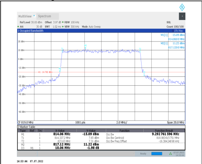
1-N26-814-824--15-10-M-7-CP-16QAM-Outer_Full-5 2@0-Ant1-9.293-10.060-≤10-PASS
