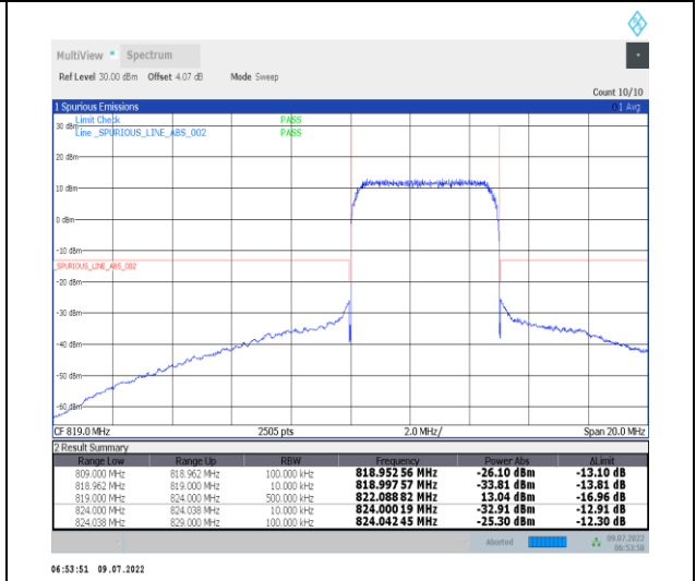
1-N26-814-824--15-5-H-6-CP-QPSK-Outer_Full-25@0-Ant1-PASS-see graph
