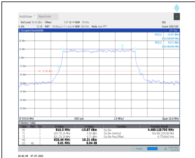
1-N26-814-824--15-5-M-8-CP-64QAM-Outer_Full-25 @0-Ant1-4.48-5.010-≤5-PASS
