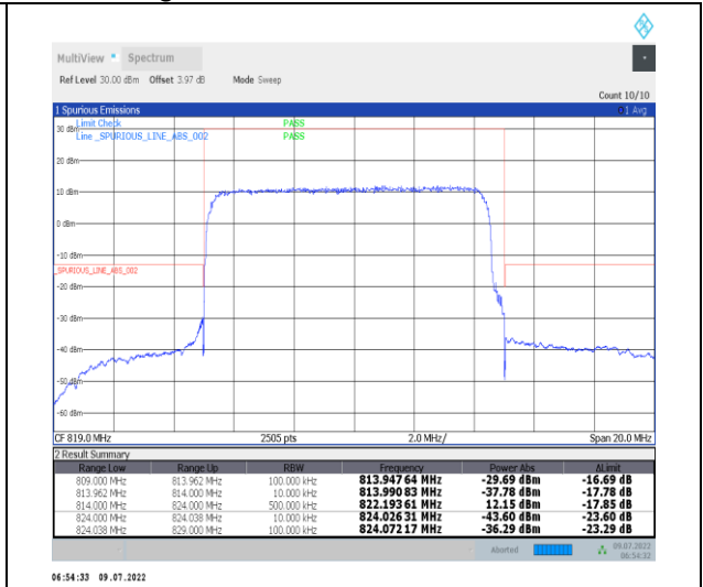
1-N26-814-824--15-10-M-3-DFT-PI2BPSK-Outer_Full-50@0-Ant1-PASS-see graph
