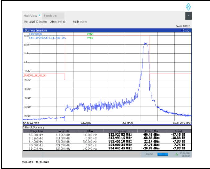
1-N26-814-824--15-10-M-5-CP-QPSK-Edge_1RB_Rig ht-1@51-Ant1-PASS-see graph
