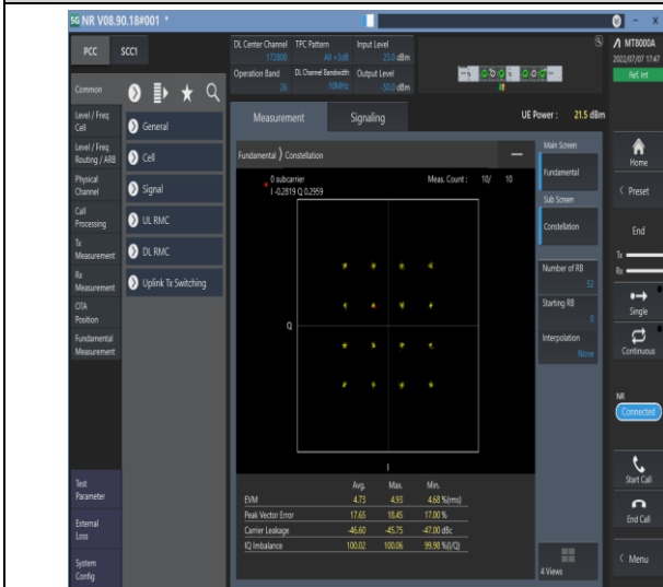
1-N26-814-824--15-10-M-7-CP-16QAM-Outer_Full-52@0-Ant1-see graph-PASS
