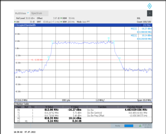
1-N26-814-824--15-5-L-8-CP-64QAM-Outer_Full-25 @0-Ant1-4.483-5.160-≤5-PASS
