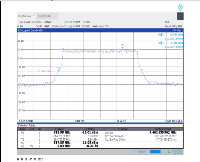
1-N26-814-824--15-5-L-6-CP-QPSK-Outer_Full-25@ 0-Ant1-4.463-5.030-≤5-PASS
