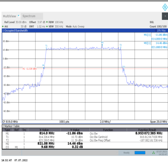
1-N26-814-824--15-10-M-2-DFT-PI2BPSK-Outer_Ful I-50@0-Ant1-8.953-9.680-≤10-PASS
