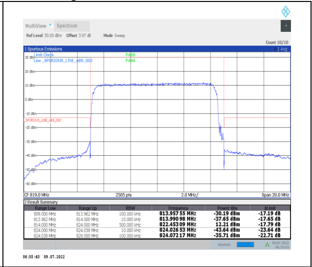
1-N26-814-824--15-10-M-3-DFT-PI2BPSK-Outer_Full-50@0-Ant1-PASS-see graph
