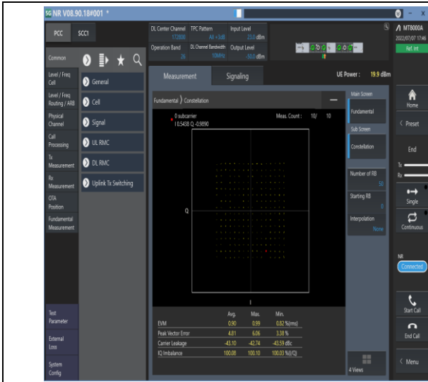
1-N26-814-824--15-10-M-5-DFT-256QAM-Outer_Full-50@0-Ant1-see graph-PASS
