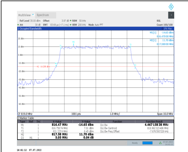
1-N26-814-824--15-5-M-4-DFT-64QAM-Outer_Full-2 5@0-Ant1-4.467-5.050-≤5-PASS
