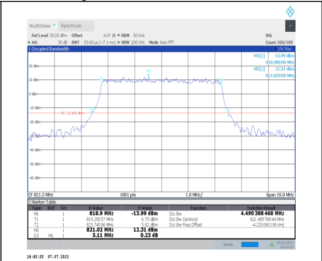
1-N26-814-824--15-5-H-4-DFT-64QAM-Outer_Full-2 5@0-Ant1-4.49-5.110-≤5-PASS
