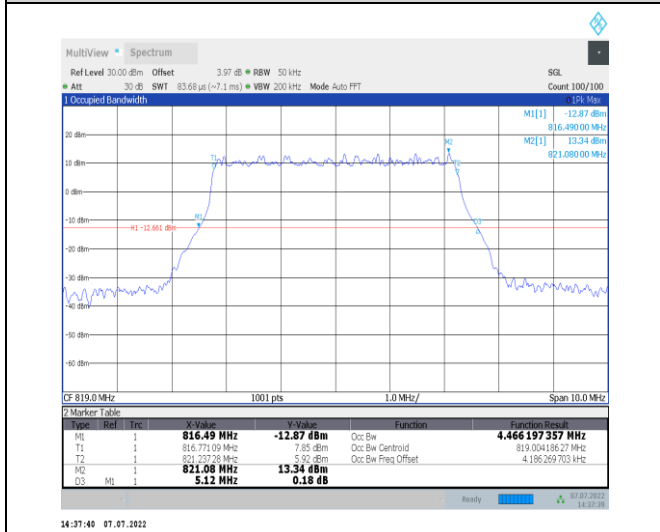
1-N26-814-824--15-5-M-2-DFT-PI2BPSK-Outer_Full-25 25@0-Ant1-4.466-5.120-≤5-PASS
