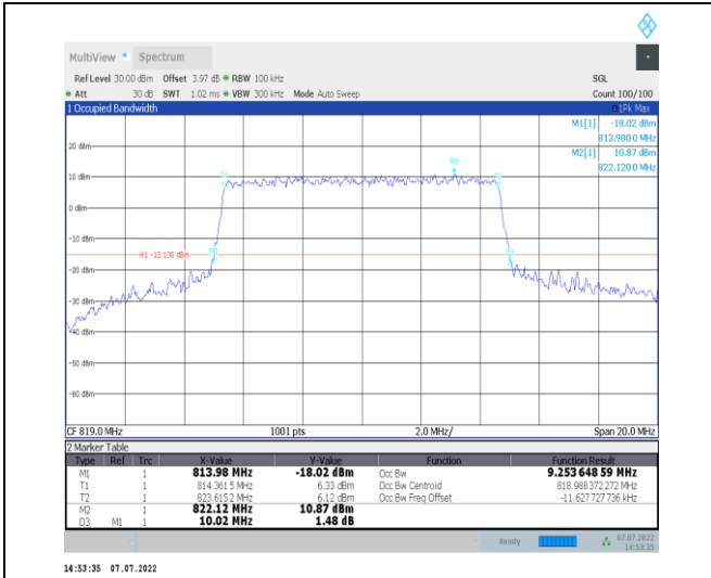
1-N26-814-824--15-10-M-6-CP-QPSK-Outer_Full-52 @0-Ant1-9.254-10.020-≤10-PASS
