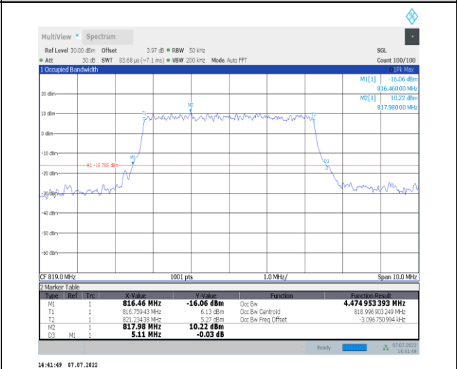
1-N26-814-824--15-5-M-7-CP-16QAM-Outer_Full-25 @0-Ant1-4.475-5.110-≤5-PASS
