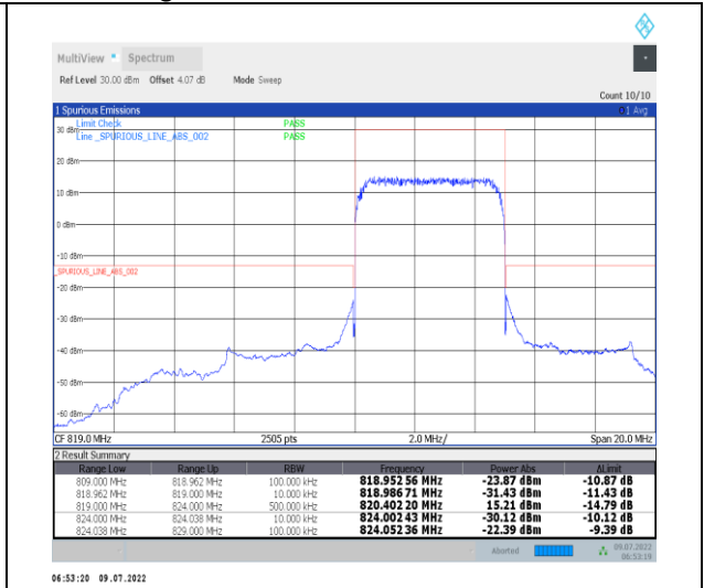
1-N26-814-824--15-5-H-3-DFT-PI2BPSK-Outer_Full-25@0-Ant1-PASS-see graph
