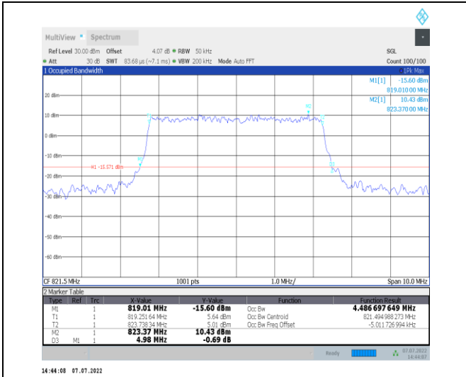
1-N26-814-824--15-5-H-7-CP-16QAM-Outer_Full-25 @0-Ant1-4.487-4.980-≤5-PASS
