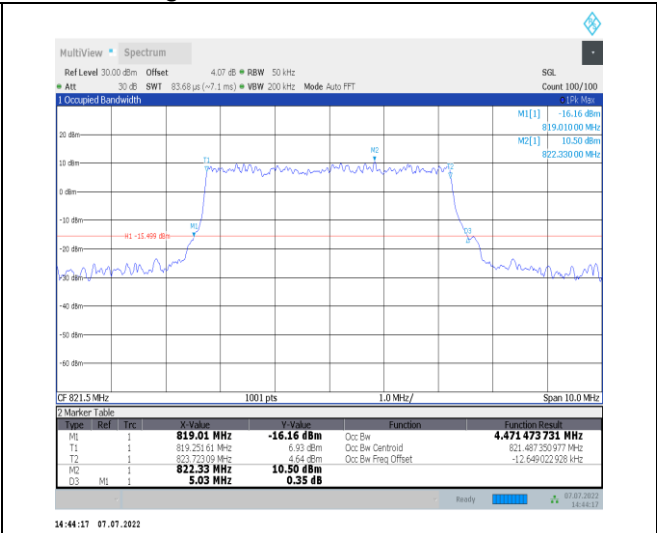
1-N26-814-824--15-5-H-8-CP-64QAM-Outer_Full-25 @0-Ant1-4.471-5.030-≤5-PASS
