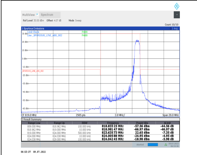
1-N26-814-824--15-5-H-5-CP-QPSK-Edge_1RB_Right-1@24-Ant1-PASS-see graph
