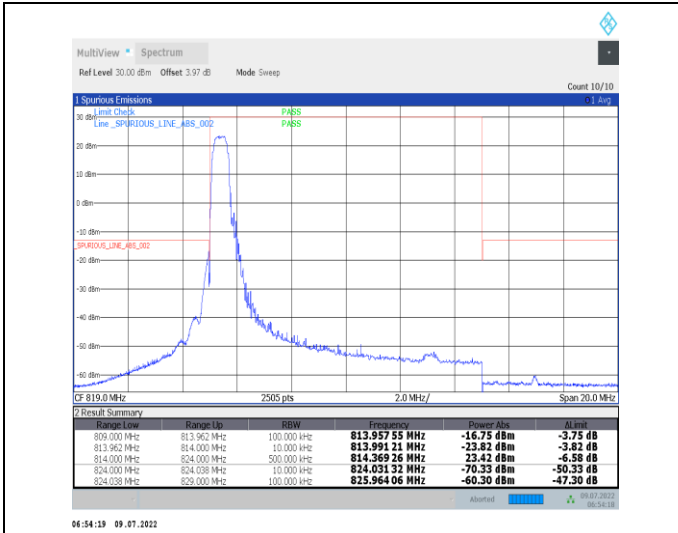
1-N26-814-824--15-10-M-1-DFT-PI2BPSK-Edge_1RB_Left-1@0-Ant1-PASS-see graph
