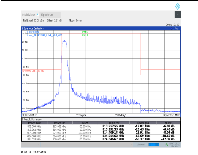
1-N26-814-824--15-10-M-4-CP-QPSK-Edge_1RB_Left-1@0-Ant1-PASS-see graph
