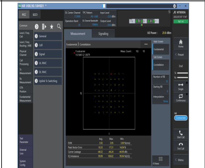
1-N26-814-824--15-10-M-8-CP-64QAM-Outer_Full-52@0-Ant1-see graph-PASS
