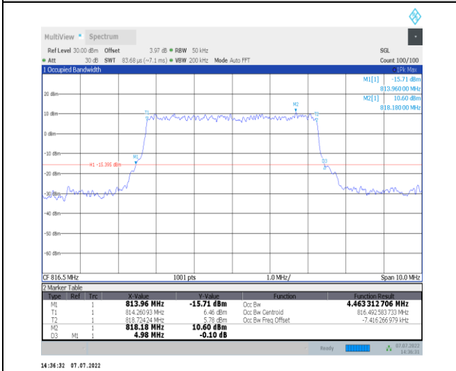
1-N26-814-824--15-5-L-7-CP-16QAM-Outer_Full-25 @0-Ant1-4.463-4.980-≤5-PASS
