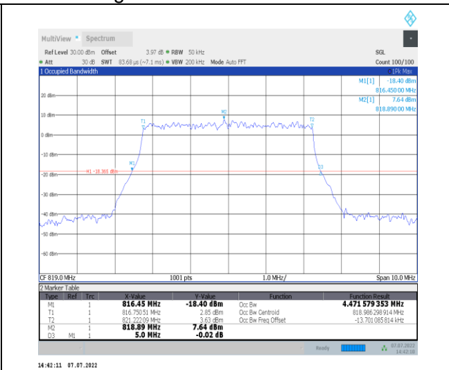
1-N26-814-824--15-5-M-9-CP-256QAM-Outer_Full-25 @0-Ant1-4.472-5.000-≤5-PASS
