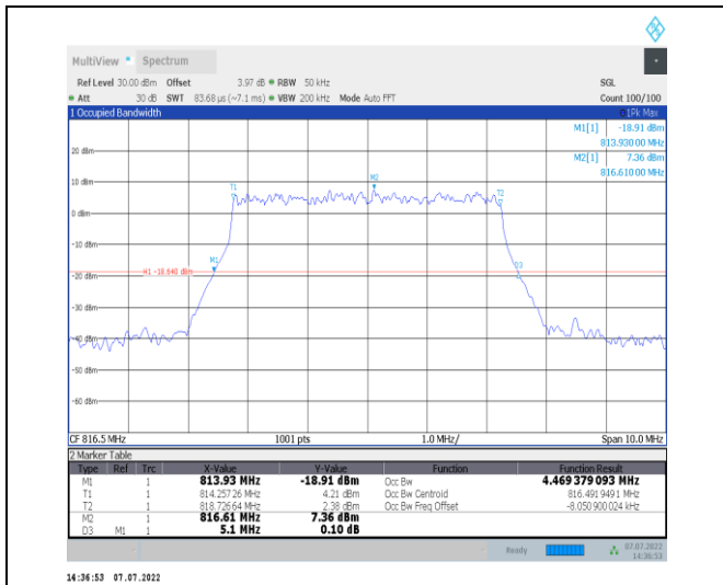
1-N26-814-824--15-5-L-9-CP-256QAM-Outer_Full-2 5@0-Ant1-4.469-5.100-≤5-PASS
