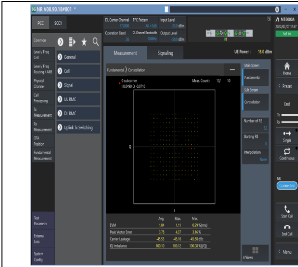
1-N26-814-824--15-10-M-9-CP-256QAM-Outer_Full-52@0-Ant1-see graph-PASS
