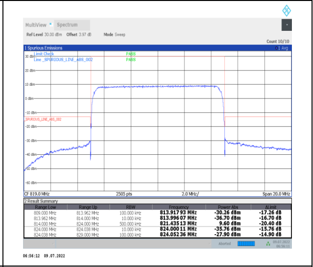
1-N26-814-824--15-10-M-6-CP-QPSK-Outer_Full-52@0-Ant1-PASS-see graph
