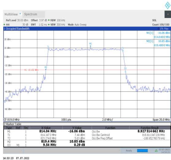
1-N26-814-824--15-10-M-5-DFT-256QAM-Outer_Ful I-50@0-Ant1-8.928-9.540-≤10-PASS
