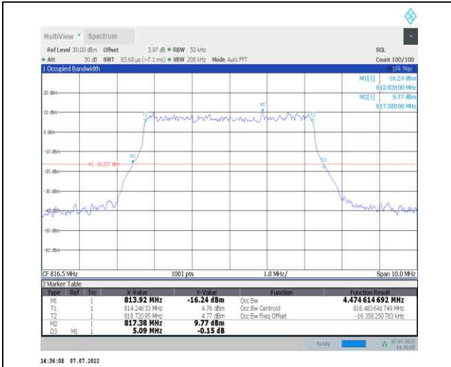
1-N26-814-824--15-5-L-5-DFT-256QAM-Outer_Full-2 5@0-Ant1-4.475-5.090-≤5-PASS
