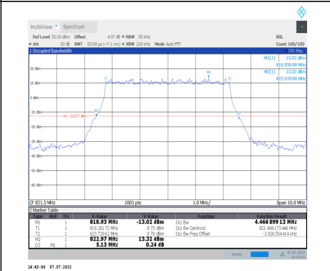
1-N26-814-824--15-5-H-2-DFT-PI2BPSK-Outer_Full-25 @0-Ant1-4.467-5.130-≤5-PASS
