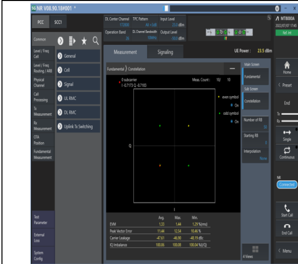
1-N26-814-824--15-10-M-1-DFT-PI2BPSK-Outer_Full -50@0-Ant1-see graph-PASS
