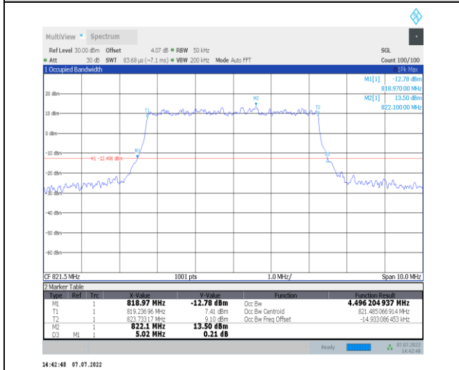
1-N26-814-824--15-5-H-1-DFT-QPSK-Outer_Full-25 @0-Ant1-4.496-5.020-≤5-PASS
