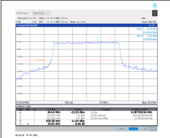
1-N26-814-824--15-10-M-8-CP-64QAM-Outer_Full-5 2@0-Ant1-9.288-10.020-≤10-PASS
