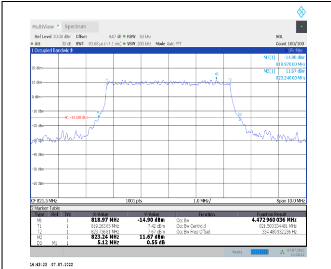
1-N26-814-824--15-5-H-3-DFT-16QAM-Outer_Full-2 5@0-Ant1-4.473-5.120-≤5-PASS
