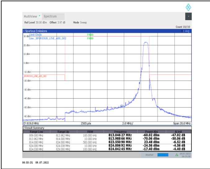
1-N26-814-824--15-10-M-2-DFT-PI2BPSK-Edge_1RB_Right-1@51-Ant1-PASS-see graph
