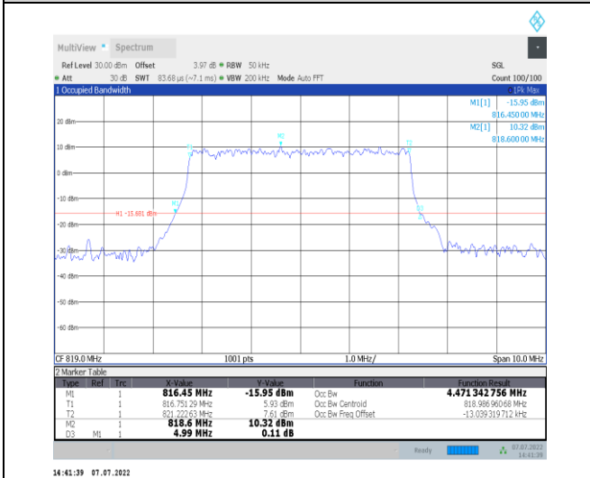
1-N26-814-824--15-5-M-6-CP-QPSK-Outer_Full-25 @0-Ant1-4.471-4.990-≤5-PASS
