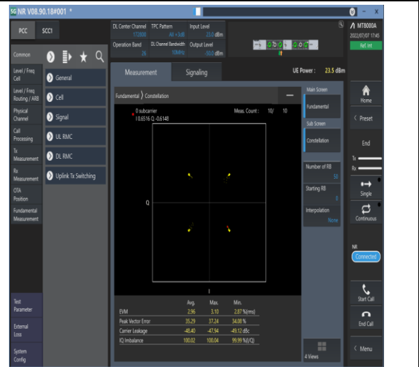
1-N26-814-824--15-10-M-2-DFT-QPSK-Outer_Full-5 0@0-Ant1-see graph-PASS
