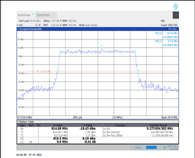
1-N26-814-824--15-10-M-9-CP-256QAM-Outer_Full- 52@0-Ant1-9.274-9.900-≤10-PASS
