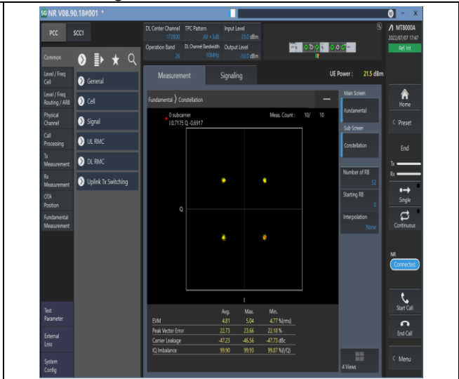
1-N26-814-824--15-10-M-6-CP-QPSK-Outer_Full-52@0-Ant1-see graph-PASS
