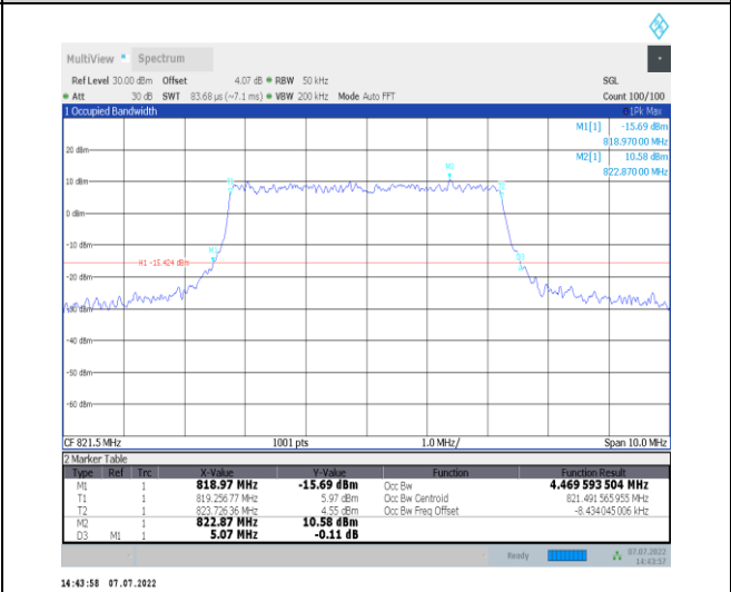
1-N26-814-824--15-5-H-6-CP-QPSK-Outer_Full-25 @0-Ant1-4.47-5.070-≤5-PASS
