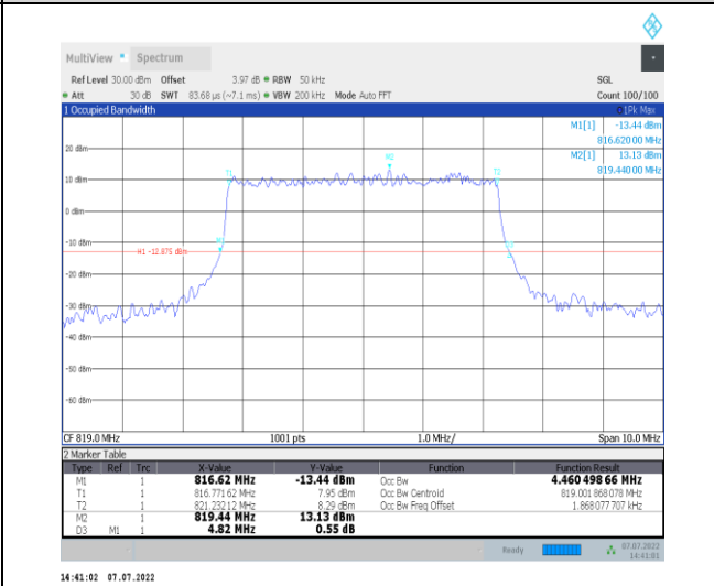
1-N26-814-824--15-5-M-3-DFT-16QAM-Outer_Full-2 5@0-Ant1-4.46-4.820-≤5-PASS
