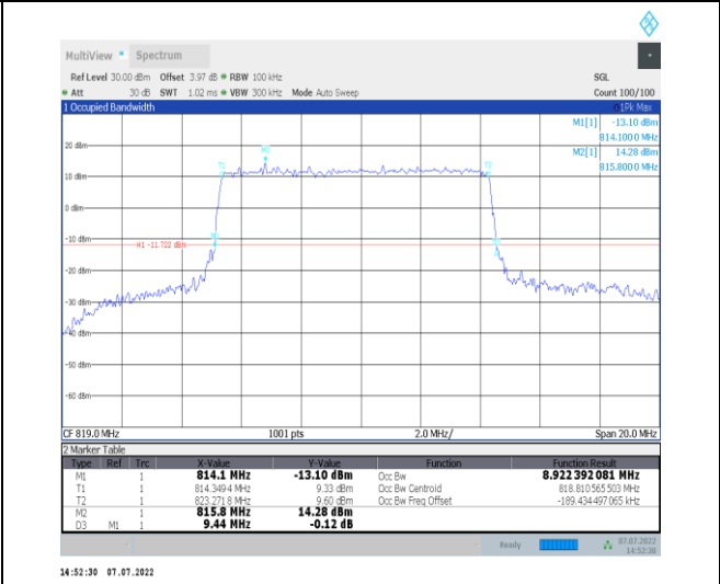
1-N26-814-824--15-10-M-1-DFT-QPSK-Outer_Full-5 0@0-Ant1-8.922-9.440-≤10-PASS
