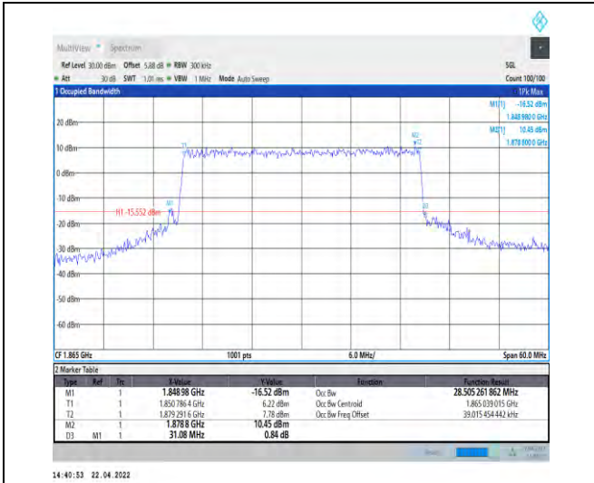
1-N25--15-30-L-6-CP-QPSK-Outer_Full-160@0-Ant1 -28.505-31.080-≤30-PASS
