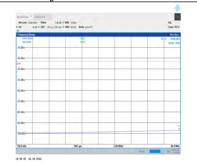
1-N25--15-40-H-1-DFT-PI2BPSK-Inner_1RB_Left-1 @1-0.15-30-Ant1--96.86--33-PASS
