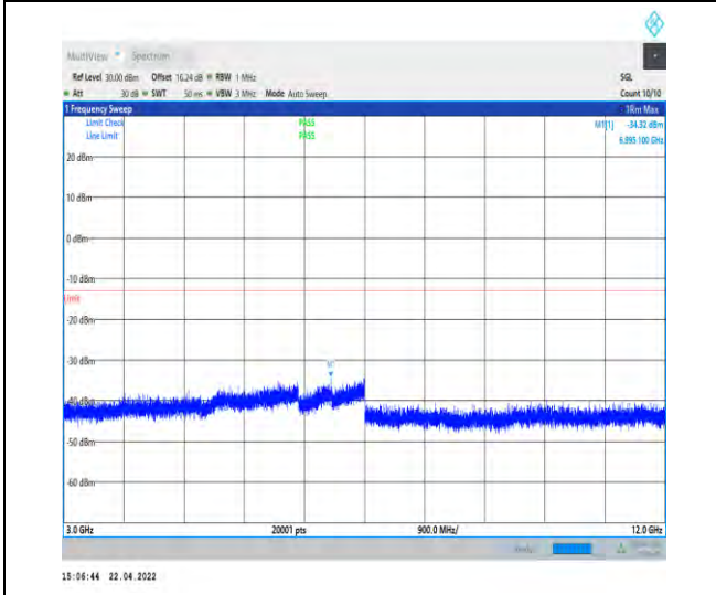
1-N25--15-40-M-1-DFT-PI2BPSK-Inner_1RB_Left-1 @1-3000-12000-Ant1--34.32--13-PASS
