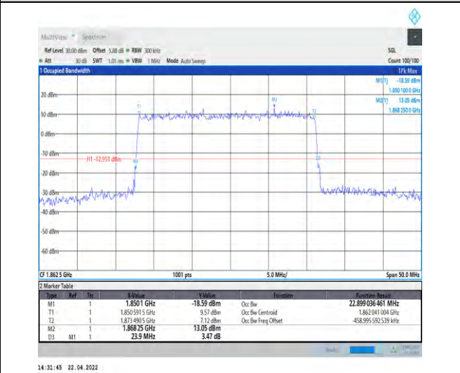
1-N25--15-25-L-4-DFT-64QAM-Outer_Full-128@0-A nt1-22.899-23.900-≤25-PASS
