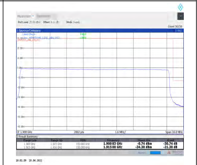
1-N25--15-15-H-6-CP-QPSK-Outer_Full-79@0-Ant1-seegraph-PASS-see graph
