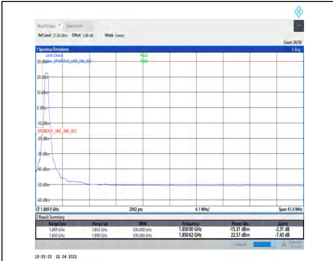
1-N25--15-40-L-1-DFT-PI2BPSK-Edge_1RB_Left-1@0-Ant1-seegraph-PASS-see graph
