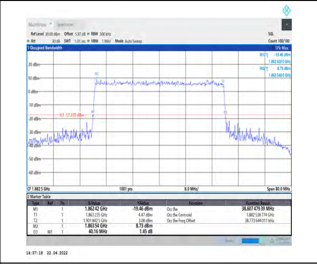
1-N25--15-40-M-9-CP-256QAM-Outer_Full-216@0-Ant Ant1-38.607-40.160-≤40-PASS
