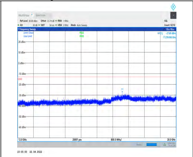
1-N25--15-40-L-1-DFT-PI2BPSK-Inner_1RB_Left-1@ 1-12000-20000-Ant1--27.80--13-PASS
