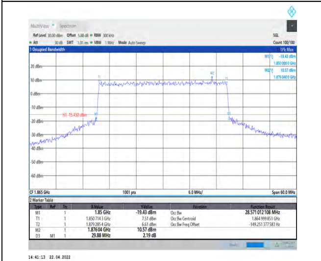
1-N25--15-30-L-8-CP-64QAM-Outer_Full-160@0-Ant1 t1-28.571-29.880-≤30-PASS
