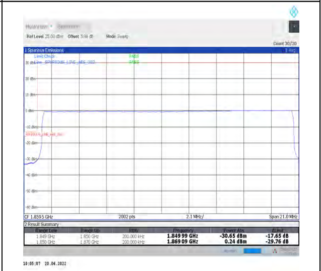
1-N25--15-20-L-6-CP-QPSK-Outer_Full-106@0-Ant1-seegraph-PASS-see graph
