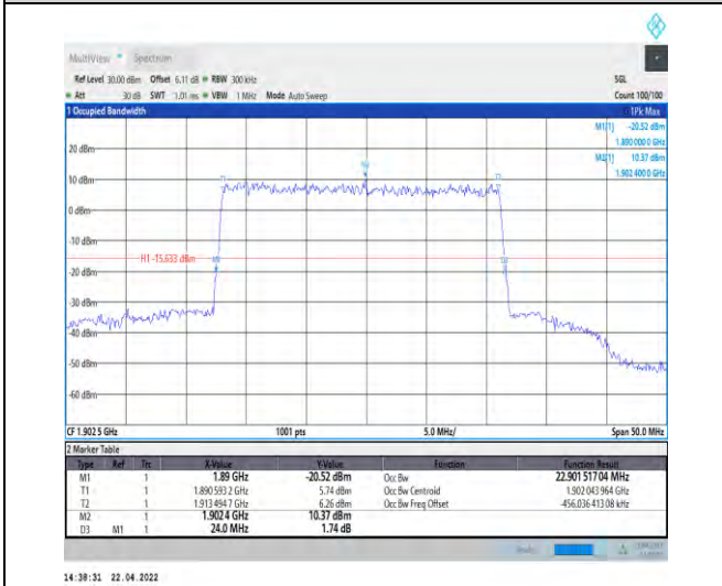
1-N25--15-25-H-5-DFT-256QAM-Outer_Full-128@0-A Ant1-22.902-24.000-≤25-PASS
