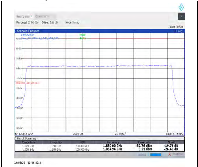
1-N25--15-20-L-3-DFT-PI2BPSK-Outer_Full-100@0-Ant1-seegraph-PASS-see graph
