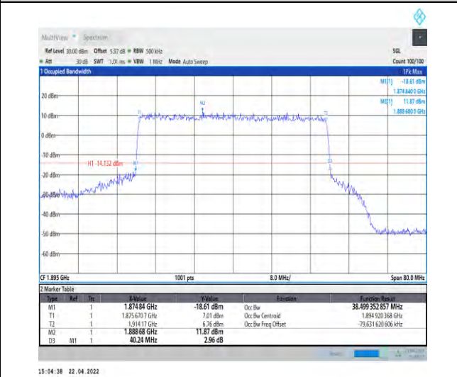
1-N25--15-40-H-8-CP-64QAM-Outer_Full-216@0-An t1-38.499-40.240-<=40-PASS
