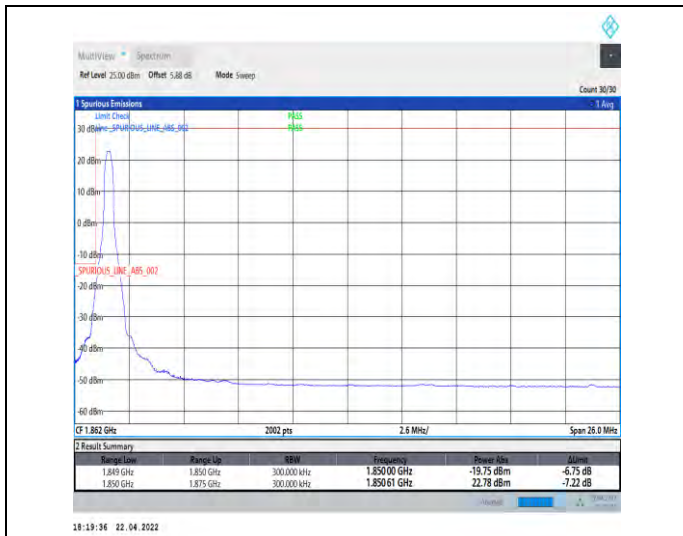
1-N25--15-25-L-1-DFT-PI2BPSK-Edge_1RB_Left-1@0-Ant1-seegraph-PASS-see graph
