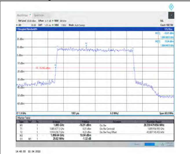
1-N25--15-30-H-5-DFT-256QAM-Outer_Full-160@0-A Ant1-28.559-29.820-≤30-PASS
