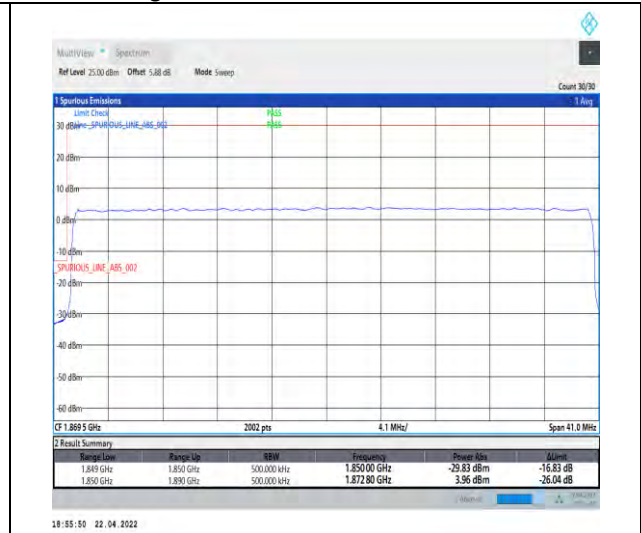
1-N25--15-40-L-3-DFT-PI2BPSK-Outer_Full-216@0-Ant1-seegraph-PASS-see graph
