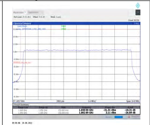
1-N25--15-15-L-3-DFT-PI2BPSK-Outer_Full-75@0-Ant1-seegraph-PASS-see graph
