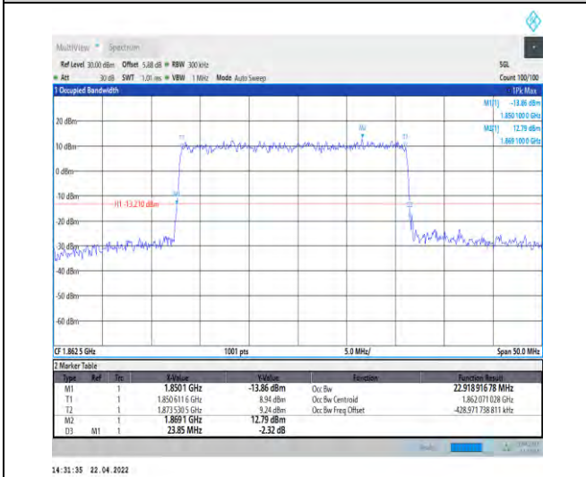
1-N25--15-25-L-3-DFT-16QAM-Outer_Full-128@0-A nt1-22.919-23.850-≤25-PASS
