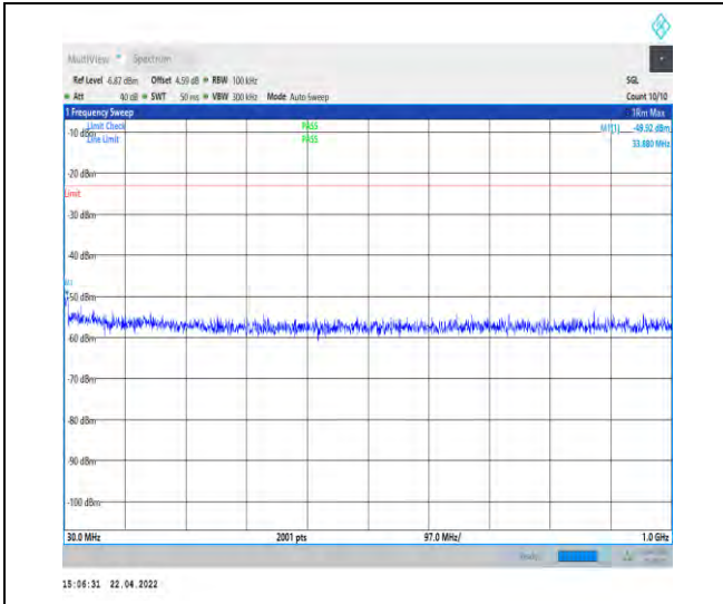
1-N25--15-40-M-1-DFT-PI2BPSK-Inner_1RB_Left-1 @1-30-1000-Ant1--49.92--23-PASS
