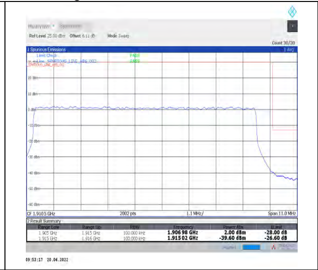
1-N25--15-10-H-3-DFT-PI2BPSK-Outer_Full-50@0-Ant1-seegraph-PASS-see graph
