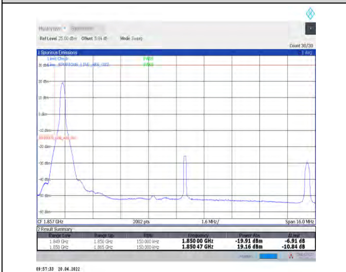
1-N25--15-15-L-4-CP-QPSK-Edge_1RB_Left-1@0-Ant1-seegraph-PASS-see graph
