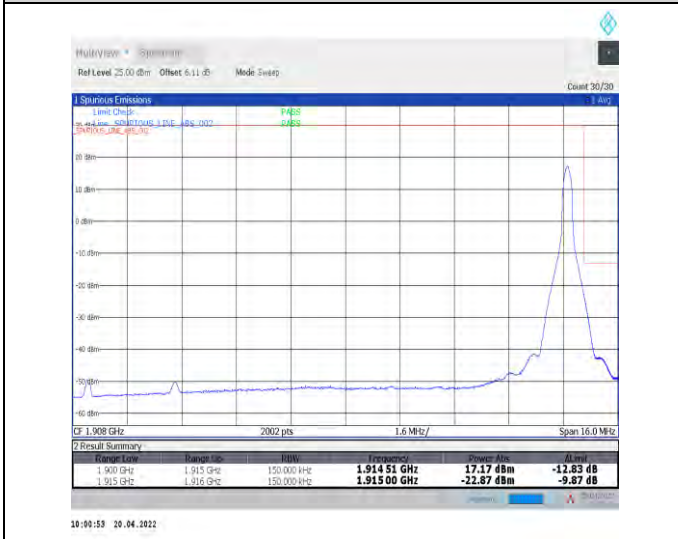
1-N25--15-15-H-5-CP-QPSK-Edge_1RB_Right-1@78-Ant1-seegraph-PASS-see graph
