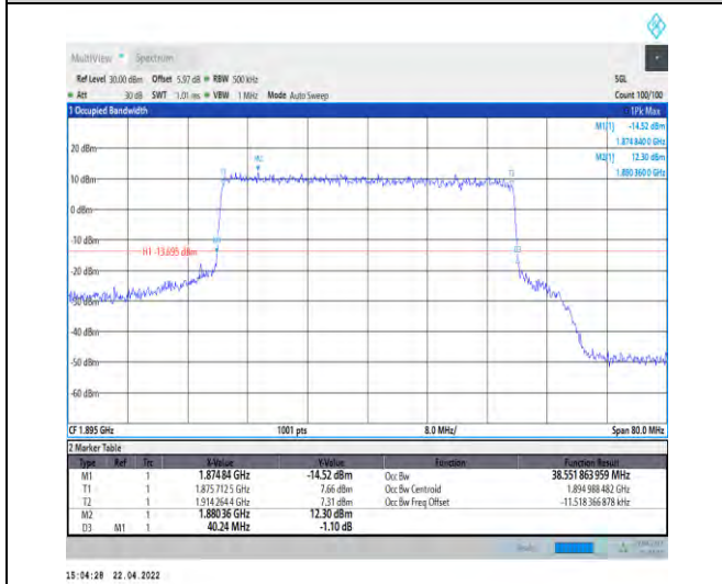
1-N25--15-40-H-7-CP-16QAM-Outer_Full-216@0-An t1-38.552-40.240-<=40-PASS
