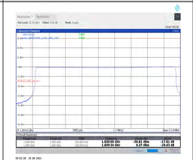
1-N25--15-10-L-6-CP-QPSK-Outer_Full-52@0-Ant1-seegraph-PASS-see graph
