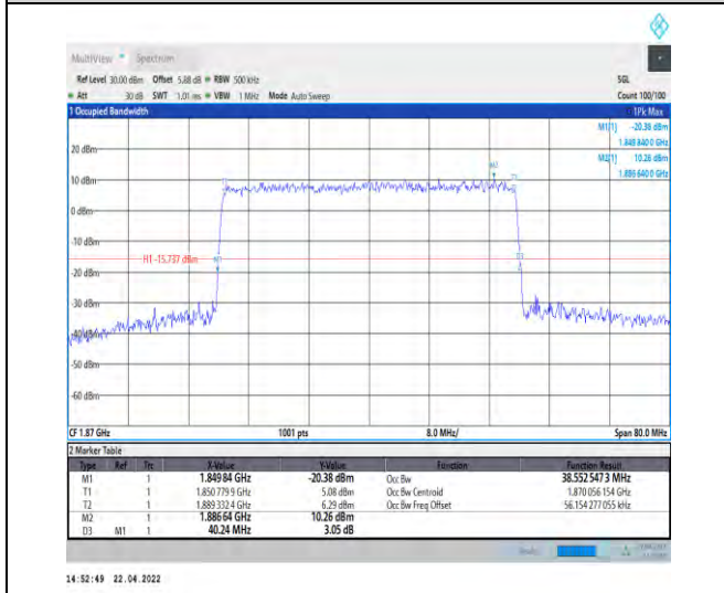
1-N25--15-40-L-5-DFT-256QAM-Outer_Full-216@0-A Ant1-38.553-40.240-≤40-PASS
