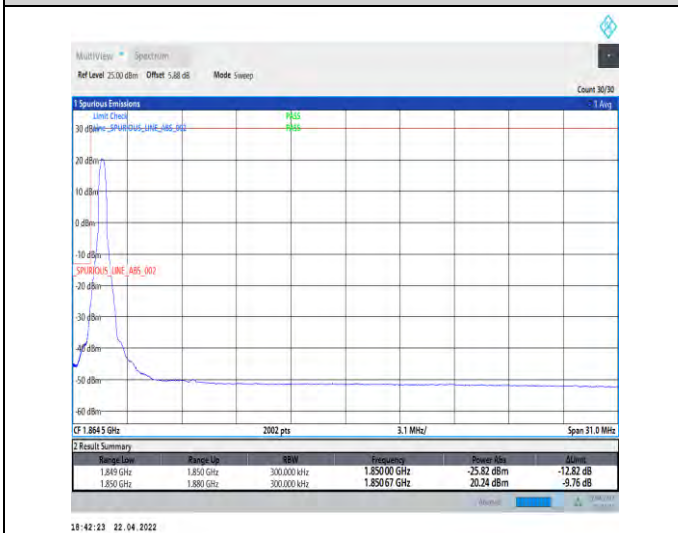
1-N25--15-30-L-4-CP-QPSK-Edge_1RB_Left-1@0-Ant1-seegraph-PASS-see graph
