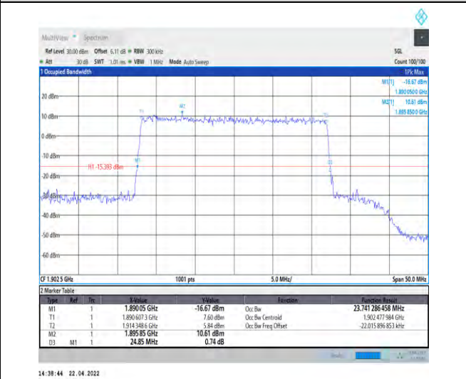
1-N25--15-25-H-6-CP-QPSK-Outer_Full-133@0-Ant 1-23.741-24.850-≤25-PASS
