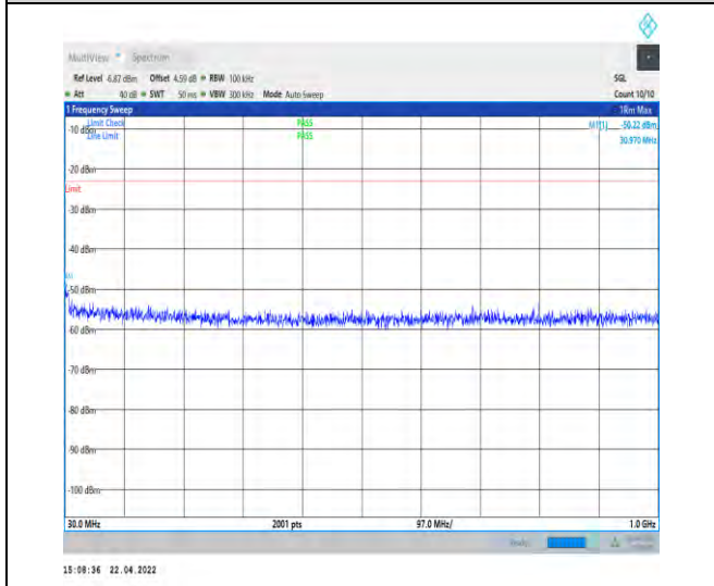
1-N25--15-40-H-1-DFT-PI2BPSK-Inner_1RB_Left-1 @1-30-1000-Ant1--50.22--23-PASS
