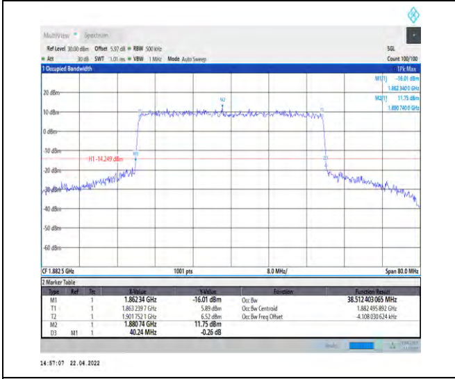
1-N25--15-40-M-8-CP-64QAM-Outer_Full-216@0-A nt1-38.512-40.240-≤40-PASS
