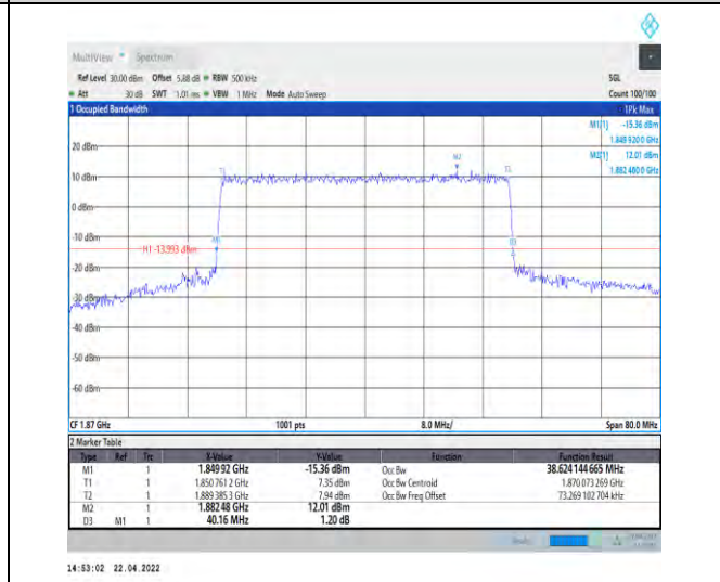
1-N25--15-40-L-6-CP-QPSK-Outer_Full-216@0-Ant1 -38.624-40.160-≤40-PASS
