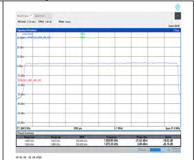
1-N25--15-30-L-3-DFT-PI2BPSK-Outer_Full-160@0-Ant1-seegraph-PASS-see graph
