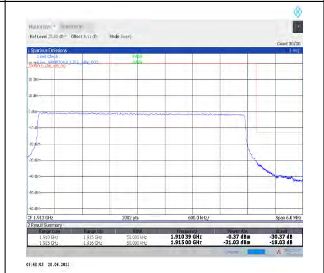
1-N25--15-5-H-6-CP-QPSK-Outer_Full-25@0-Ant1-seegraph-PASS-see graph
