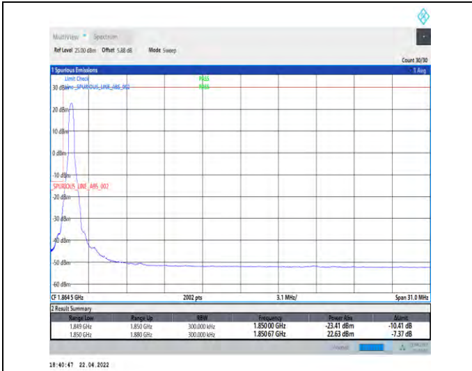
1-N25--15-30-L-1-DFT-PI2BPSK-Edge_1RB_Left-1@0-Ant1-seegraph-PASS-see graph
