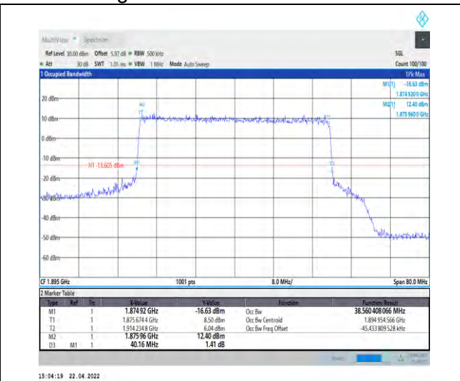
1-N25--15-40-H-6-CP-QPSK-Outer_Full-216@0-Ant 1-38.56-40.160-<=40-PASS
