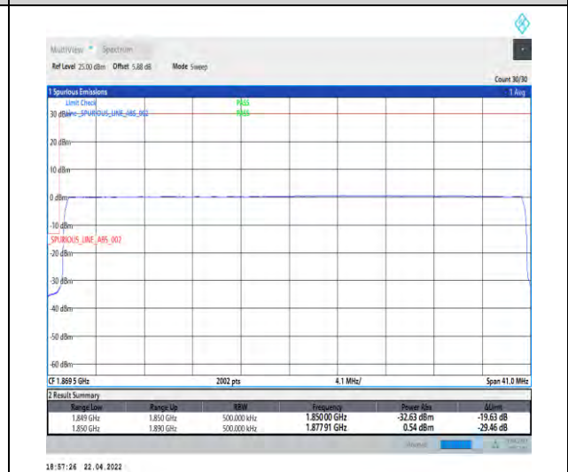
1-N25--15-40-L-6-CP-QPSK-Outer_Full-216@0-Ant1-seegraph-PASS-see graph
