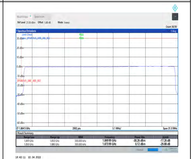
1-N25--15-30-L-6-CP-QPSK-Outer_Full-160@0-Ant1-seegraph-PASS-see graph
