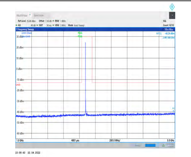
1-N25--15-40-H-1-DFT-PI2BPSK-Inner_1RB_Left-1 @1-1000-3000-Ant1--40.24--13-PASS
