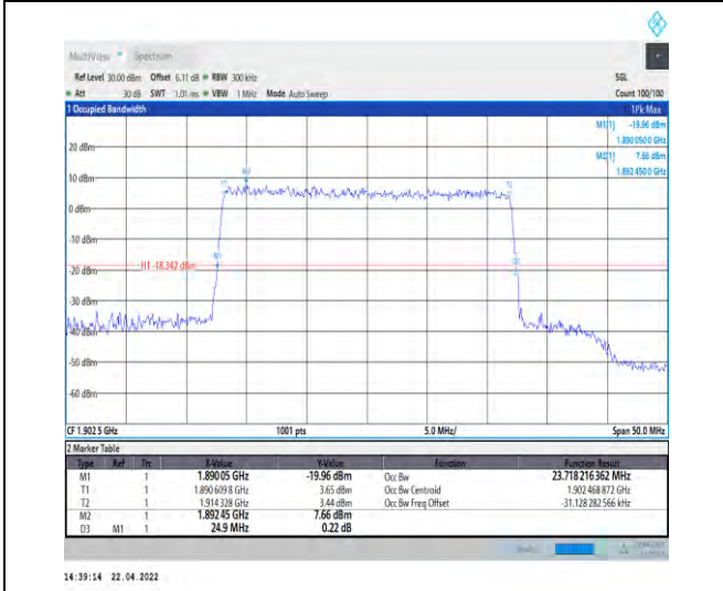
1-N25--15-25-H-9-CP-256QAM-Outer_Full-133@0-A nt1-23.718-24.900-≤25-PASS
