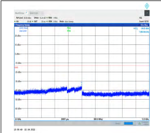
1-N25--15-40-H-1-DFT-PI2BPSK-Inner_1RB_Left-1 @1-3000-12000-Ant1--34.82--13-PASS
