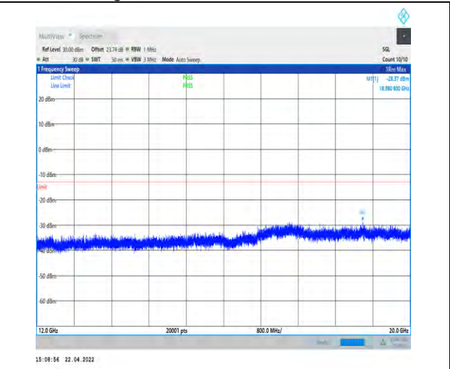
1-N25--15-40-H-1-DFT-PI2BPSK-Inner_1RB_Left-1 @1-12000-20000-Ant1--28.37--13-PASS
