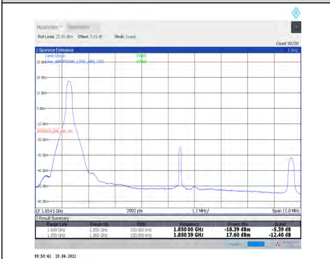
1-N25--15-10-L-4-CP-QPSK-Edge_1RB_Left-1@0-Ant1-seegraph-PASS-see graph
