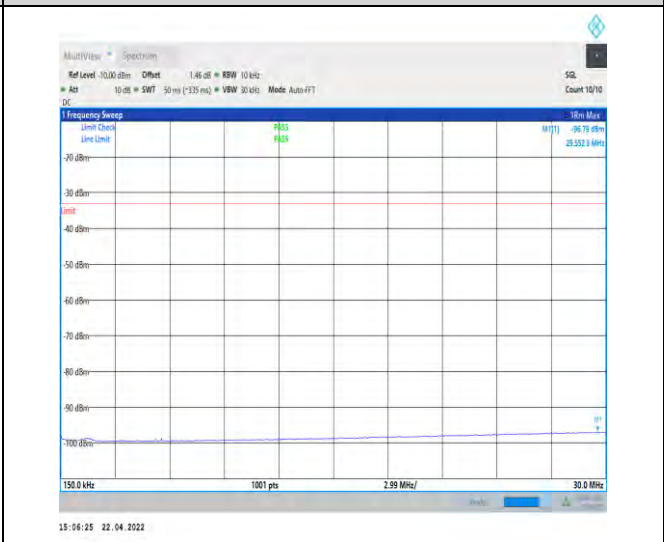
1-N25--15-40-M-1-DFT-PI2BPSK-Inner_1RB_Left-1 @1-0.15-30-Ant1--96.79--33-PASS
