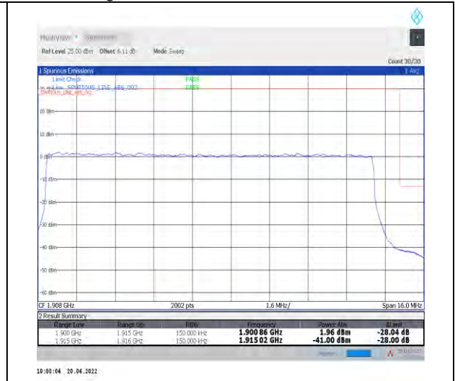
1-N25--15-15-H-3-DFT-PI2BPSK-Outer_Full-75@0-Ant1-seegraph-PASS-see graph
