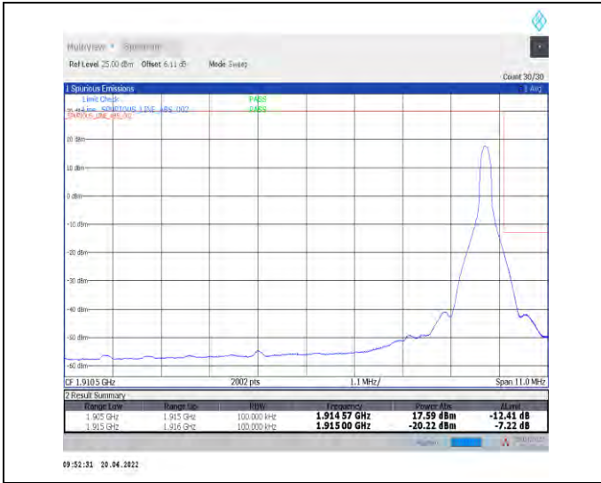
1-N25--15-10-H-2-DFT-PI2BPSK-Edge_1RB_Right-1@51-Ant1-seegraph-PASS-see graph
