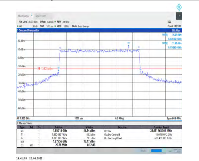
1-N25--15-30-L-7-CP-16QAM-Outer_Full-160@0-Ant1 t1-28.631-29.760-≤30-PASS
