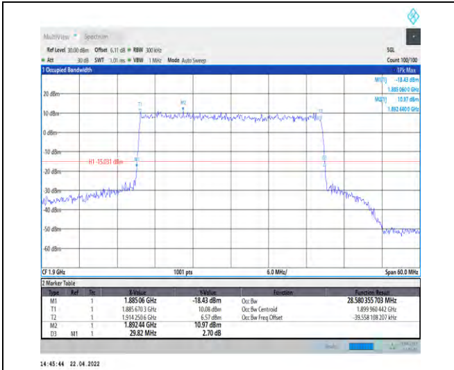
1-N25--15-30-H-4-DFT-64QAM-Outer_Full-160@0-A nt1-28.58-29.820-≤30-PASS
