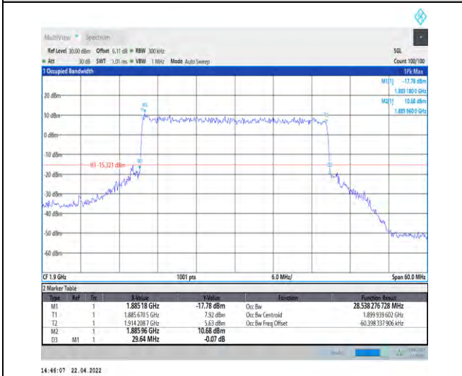
1-N25--15-30-H-6-CP-QPSK-Outer_Full-160@0-Ant 1-28.538-29.640-≤30-PASS
