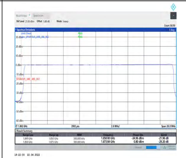
1-N25--15-25-L-6-CP-QPSK-Outer_Full-133@0-Ant1-seegraph-PASS-see graph
