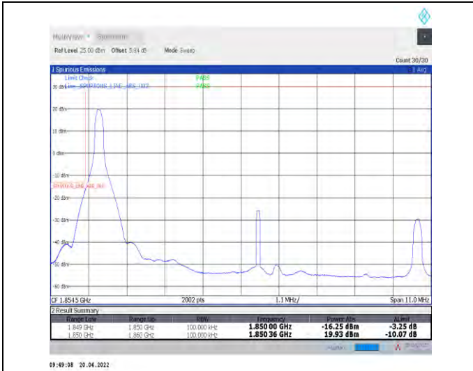
1-N25--15-10-L-1-DFT-PI2BPSK-Edge_1RB_Left-1@0-Ant1-seegraph-PASS-see graph
