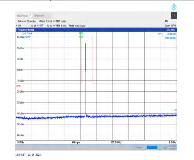
1-N25--15-40-M-1-DFT-PI2BPSK-Inner_1RB_Left-1 @1-1000-3000-Ant1--40.38--13-PASS
