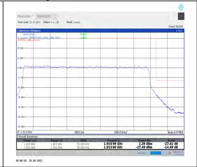
1-N25--15-5-H-3-DFT-PI2BPSK-Outer_Full-25@0-Ant1-seegraph-PASS-see graph
