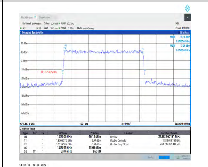
1-N25--15-25-M-3-DFT-16QAM-Outer_Full-128@0-A nt1-22.883-24.000-≤25-PASS
