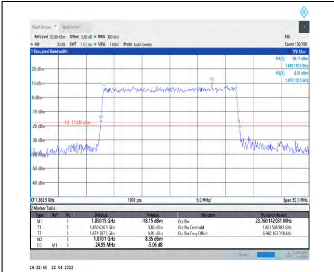
1-N25--15-25-L-9-CP-256QAM-Outer_Full-133@0-A nt1-23.76-24.950-≤25-PASS
