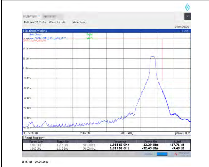
1-N25--15-5-H-5-CP-QPSK-Edge_1RB_Right-1@24-Ant1-seegraph-PASS-see graph
