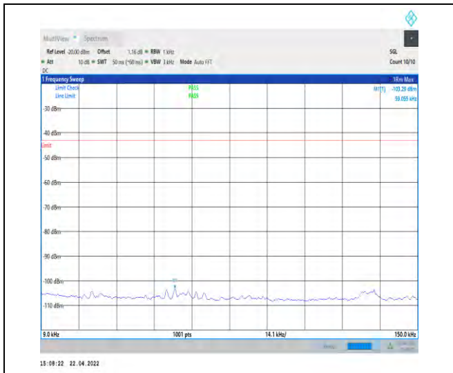
1-N25--15-40-H-1-DFT-PI2BPSK-Inner_1RB_Left-1 @1-0.009-0.15-Ant1--103.29--43-PASS
