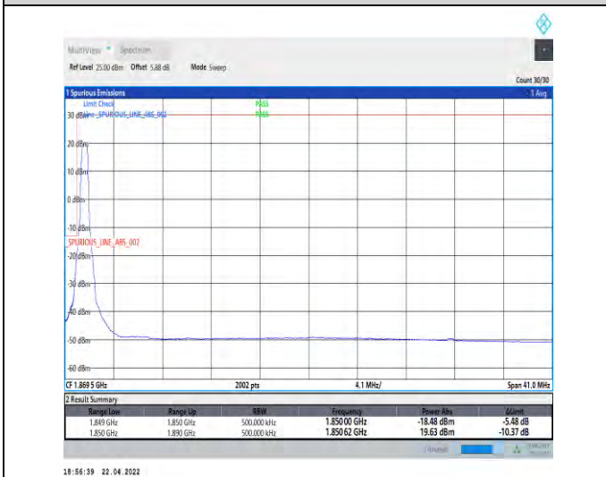
1-N25--15-40-L-4-CP-QPSK-Edge_1RB_Left-1@0-Ant1-seegraph-PASS-see graph
