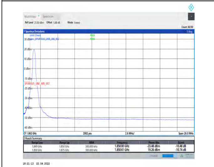
1-N25--15-25-L-4-CP-QPSK-Edge_1RB_Left-1@0-Ant1-seegraph-PASS-see graph
