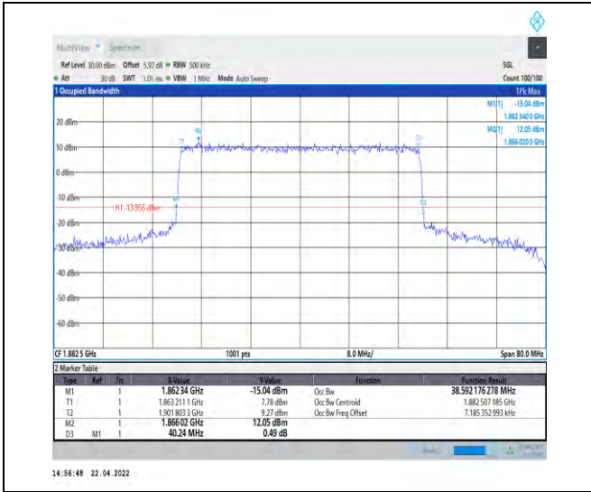
1-N25--15-40-M-6-CP-QPSK-Outer_Full-216@0-Ant 1-38.592-40.240-≤40-PASS
