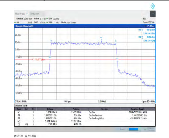
1-N25--15-25-H-4-DFT-64QAM-Outer_Full-128@0-A nt1-22.867-23.900-≤25-PASS
