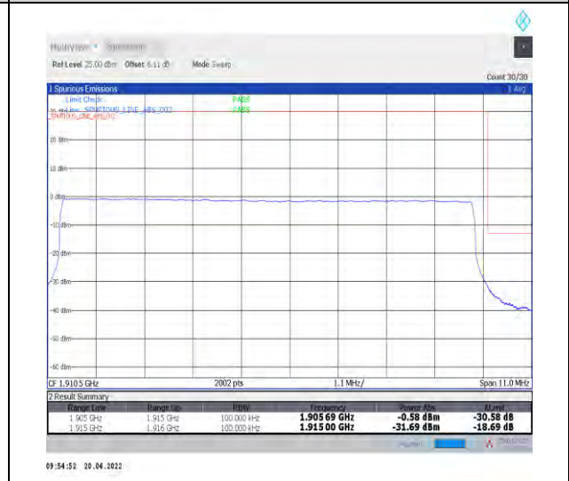
1-N25--15-10-H-6-CP-QPSK-Outer_Full-52@0-Ant1-seegraph-PASS-see graph
