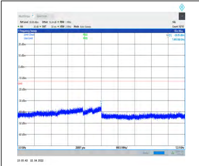
1-N25--15-40-L-1-DFT-PI2BPSK-Inner_1RB_Left-1 @1-3000-12000-Ant1--33.95--13-PASS
