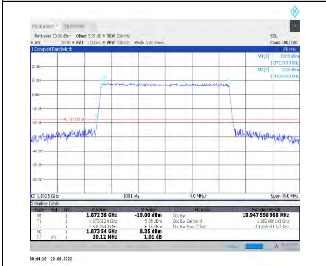
1-N25--15-20-M-9-CP-256QAM-Outer_Full-106@0-A Ant1-18.948-20.120-≤20-PASS
