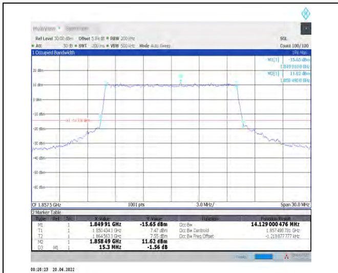
1-N25--15-15-L-7-CP-16QAM-Outer_Full-79@0-Ant 1-14.129-15.300-≤15-PASS
