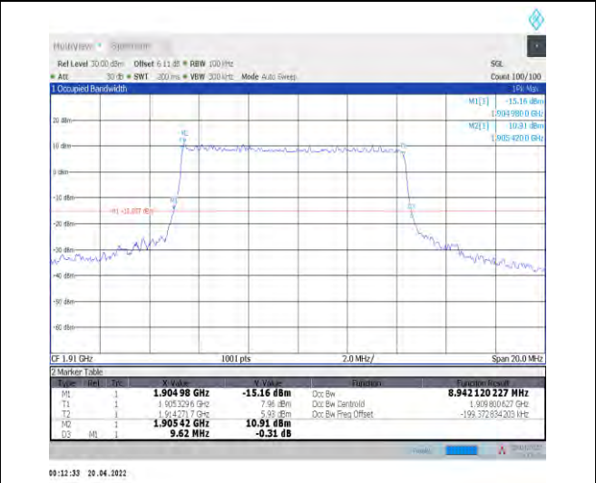
1-N25--15-10-H-3-DFT-16QAM-Outer_Full-50@0-Ant t1-8.942-9.620-≤10-PASS
