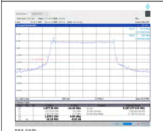
1-N25--15-10-M-7-CP-16QAM-Outer_Full-52@0-Ant 1-9.297-10.180-≤10-PASS
