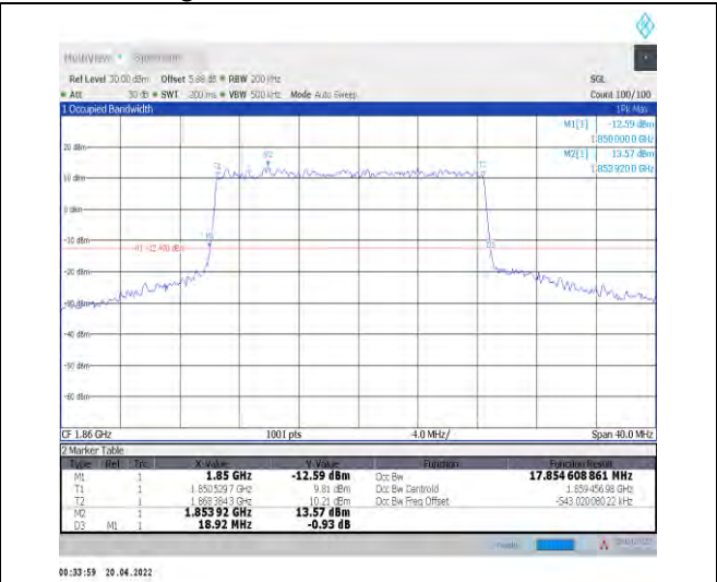
1-N25--15-20-L-1-DFT-QPSK-Outer_Full-100@0-Ant 1-17.855-18.920-≤20-PASS
