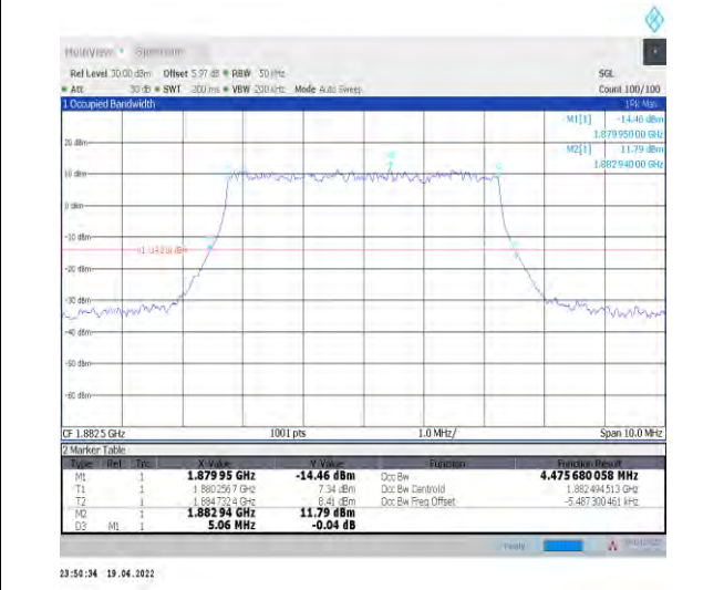
1-N25--15-5-M-3-DFT-16QAM-Outer_Full-25@0-Ant 1-4.476-5.060-≤5-PASS
