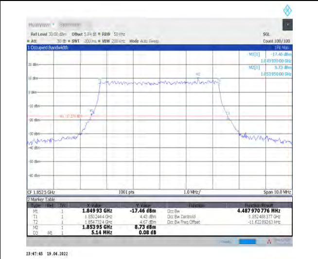
1-N25--15-5-L-8-CP-64QAM-Outer_Full-25@0-Ant1- 4.488-5.140-≤5-PASS
