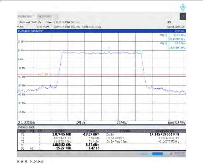
1-N25--15-15-M-9-CP-256QAM-Outer_Full-79@0-Ant -14.145-15.270-≤15-PASS
