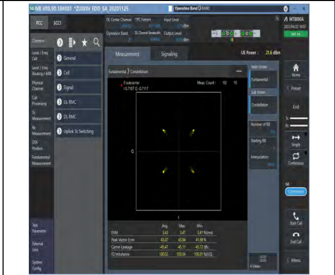
1-N25--15-40-M-2-DFT-QPSK-Outer_Full-216@0-A Ant1-see graph-PASS
