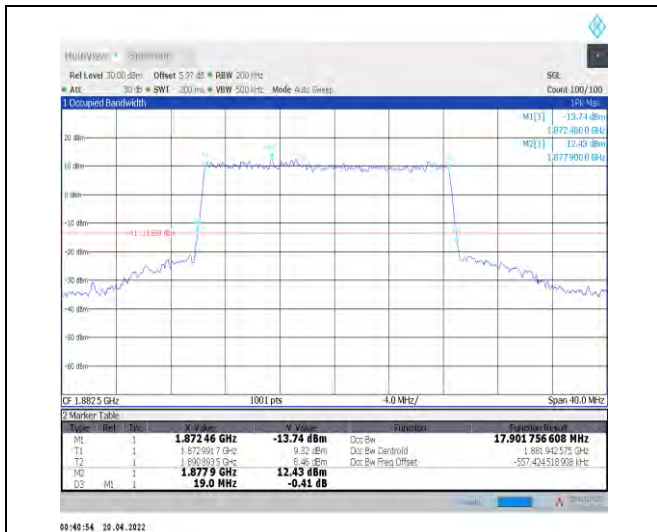
1-N25--15-20-M-3-DFT-16QAM-Outer_Full-100@0-A nt1-17.902-19.000-≤20-PASS
