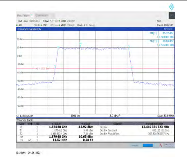
1-N25--15-15-M-5-DFT-256QAM-Outer_Full-75@0-A nt1-13.44-14.520-≤15-PASS
