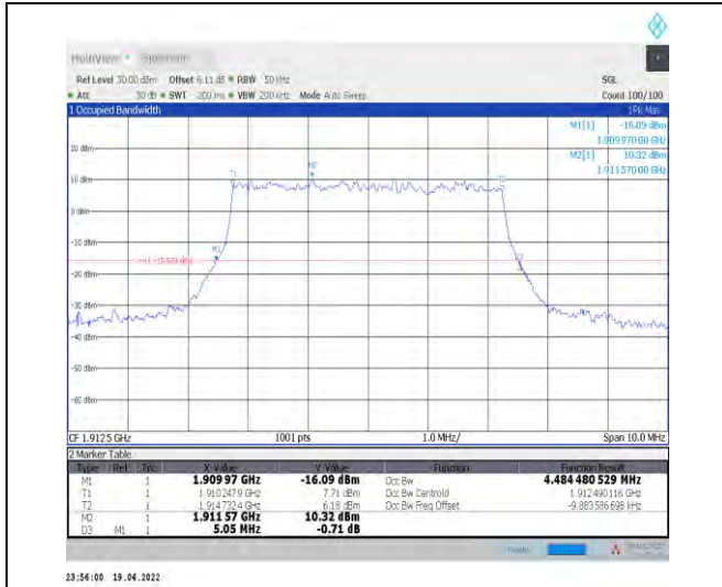
1-N25--15-5-H-3-DFT-16QAM-Outer_Full-25@0-Ant 1-4.484-5.050-≤5-PASS
