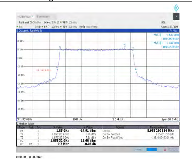
1-N25--15-10-L-3-DFT-16QAM-Outer_Full-50@0-Ant 1-8.955-9.700-≤10-PASS
