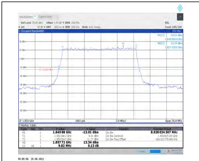
1-N25--15-10-L-2-DFT-PI2BPSK-Outer_Full-50@0-A nt1-8.938-9.820-≤10-PASS
