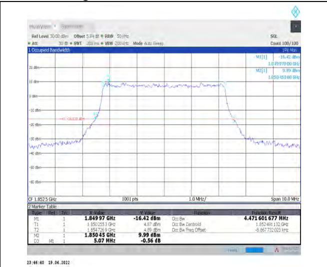
1-N25--15-5-L-6-CP-QPSK-Outer_Full-25@0-Ant1-4 .472-5.070-≤5-PASS
