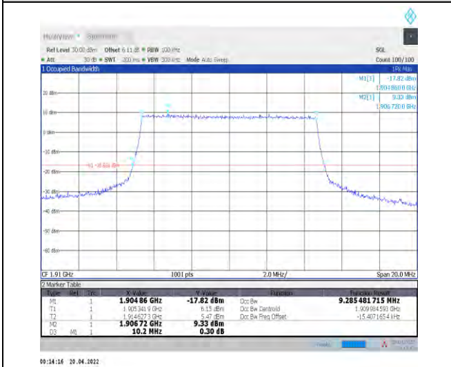
1-N25--15-10-H-6-CP-QPSK-Outer_Full-52@0-Ant1- 9.285-10.200-≤10-PASS
