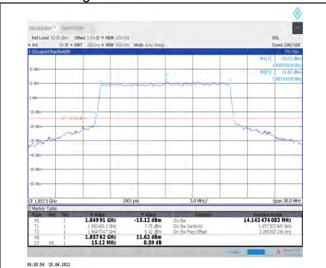
1-N25--15-15-L-8-CP-64QAM-Outer_Full-79@0-Ant 1-14.143-15.120-≤15-PASS
