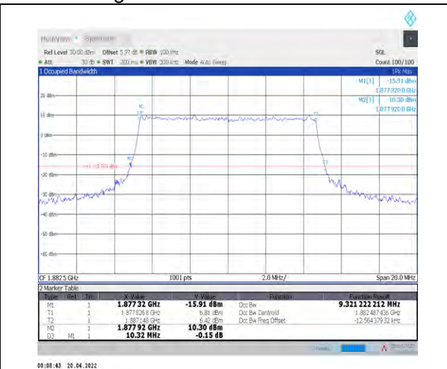
1-N25--15-10-M-6-CP-QPSK-Outer_Full-52@0-Ant1 -9.321-10.320-≤10-PASS
