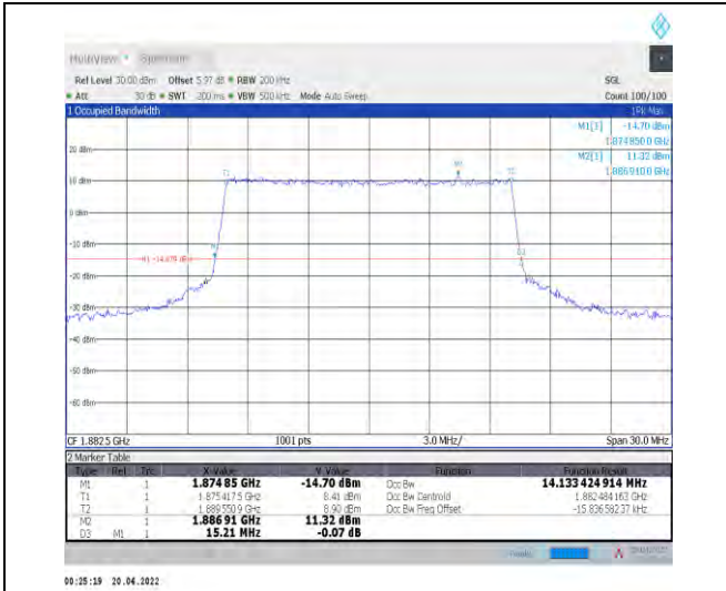
1-N25--15-15-M-6-CP-QPSK-Outer_Full-79@0-Ant1 -14.133-15.210-≤15-PASS
