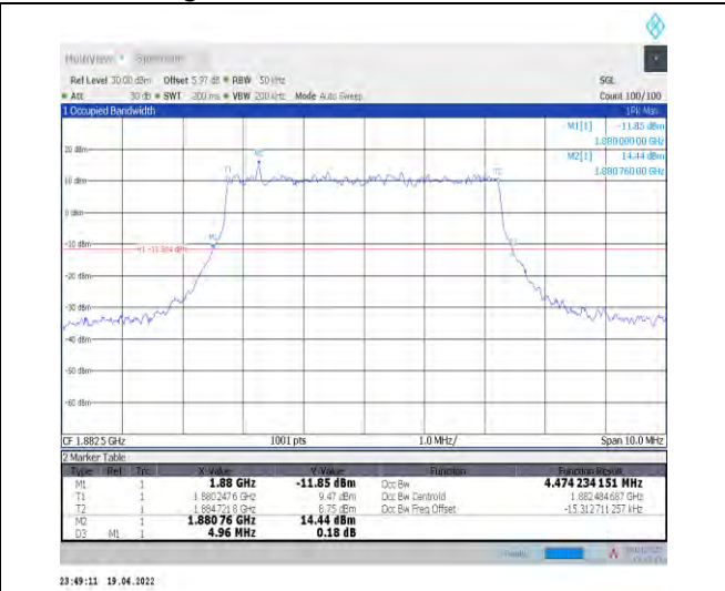
1-N25--15-5-M-1-DFT-QPSK-Outer_Full-25@0-Ant1- 4.474-4.960-≤5-PASS
