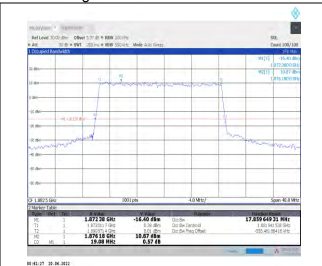
1-N25--15-20-M-4-DFT-64QAM-Outer_Full-100@0-A nt1-17.86-19.080-≤20-PASS
