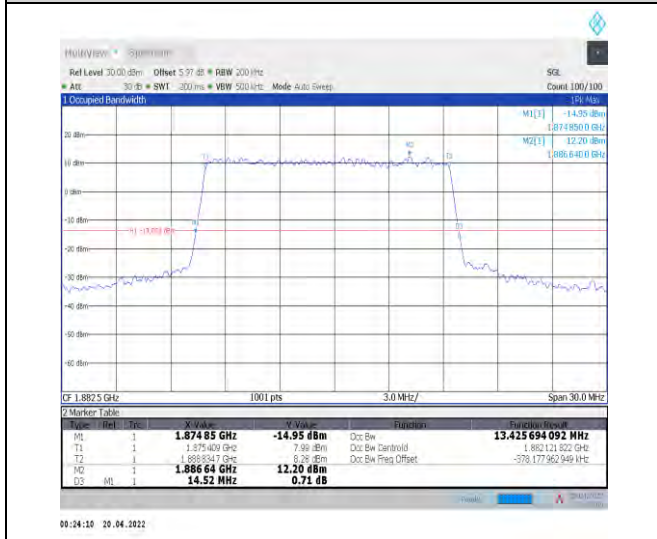
1-N25--15-15-M-4-DFT-64QAM-Outer_Full-75@0-An t1-13.426-14.520-≤15-PASS
