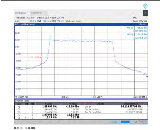
1-N25--15-15-H-7-CP-16QAM-Outer_Full-79@0-Ant 1-14.115-15.150-≤15-PASS
