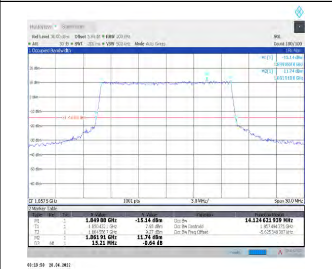
1-N25--15-15-L-6-CP-QPSK-Outer_Full-79@0-Ant1 14.125-15.210-≤15-PASS
