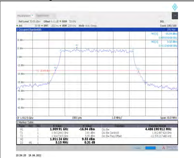
1-N25--15-5-H-4-DFT-64QAM-Outer_Full-25@0-Ant 1-4.486-5.150-≤5-PASS
