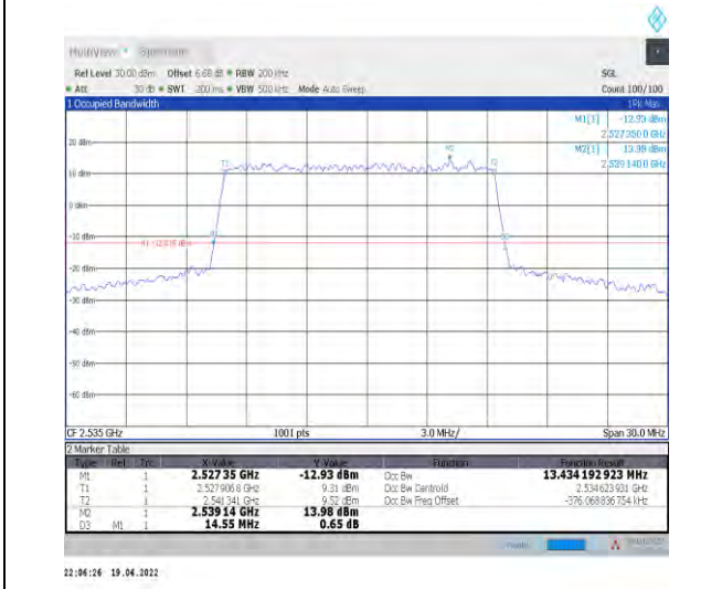
1-N7--15-15-M-4-DFT-64QAM-Outer_Full-75@0-Ant 1-13.434-14.550-≤15-PASS
