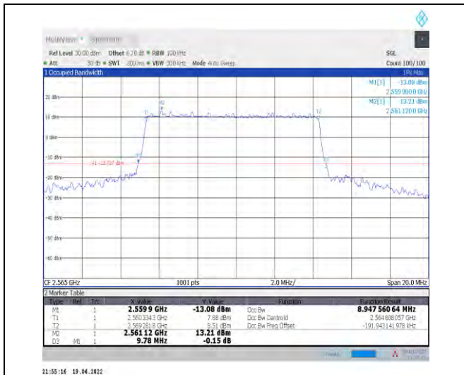
1-N7--15-10-H-4-DFT-64QAM-Outer_Full-50@0-Ant 1-8.948-9.780-≤10-PASS
