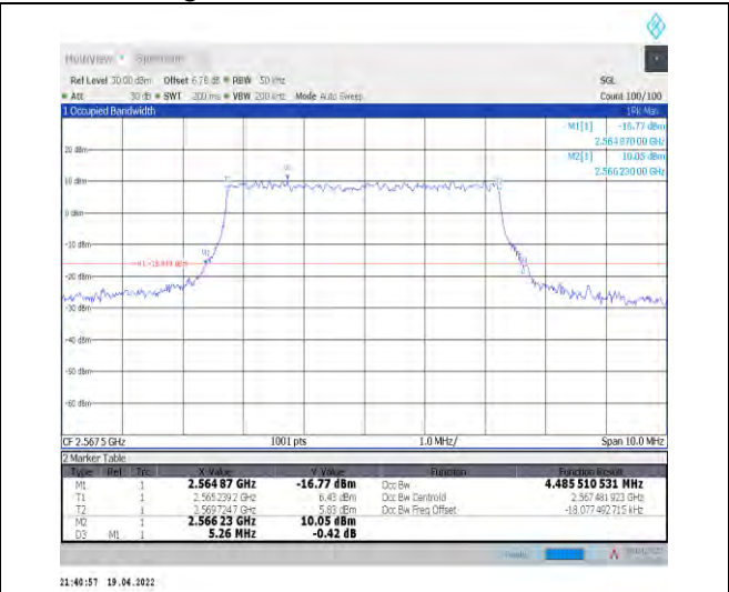
1-N7--15-5-H-8-CP-64QAM-Outer_Full-25@0-Ant1-4 .486-5.260-≤5-PASS
