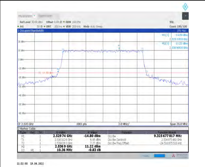
1-N7--15-10-M-8-CP-64QAM-Outer_Full-52@0-Ant1 -9.326-10.360-≤10-PASS
