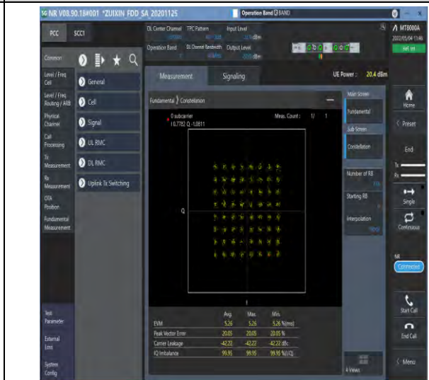
1-N7-PC3-15-40-M-8-CP-64QAM-Outer_Full-216@0-Ant1-see graph-PASS
