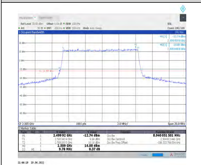
1-N7--15-10-L-4-DFT-64QAM-Outer_Full-50@0-Ant1 -8.94-9.780-≤10-PASS
