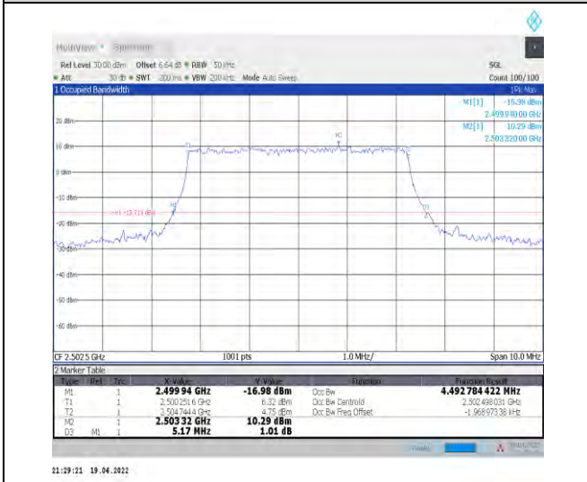
1-N7--15-5-L-7-CP-16QAM-Outer_Full-25@0-Ant1-4 .493-5.170-≤5-PASS
