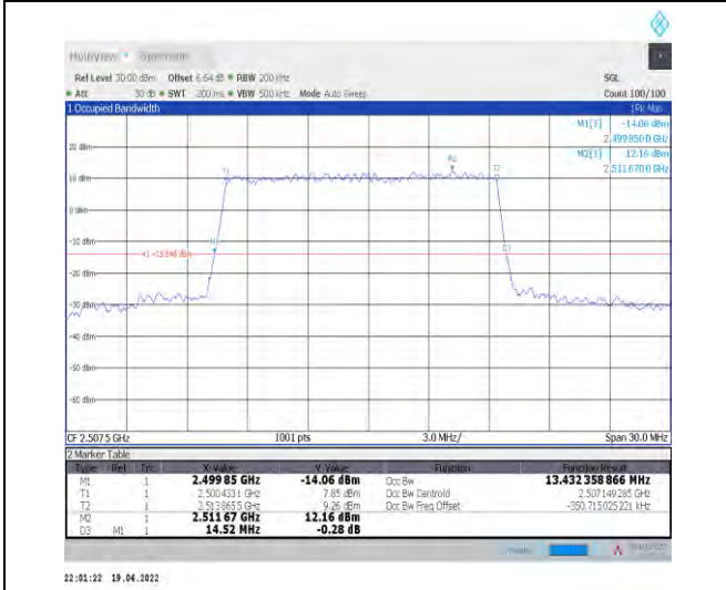
1-N7--15-15-L-5-DFT-256QAM-Outer_Full-75@0-Ant 1-13.432-14.520-≤15-PASS
