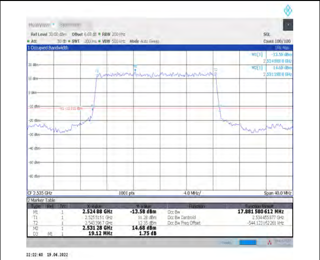
1-N7--15-20-M-2-DFT-PI2BPSK-Outer_Full-100@0-Ant Ant1-17.882-19.120-≤20-PASS
