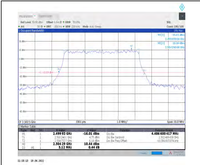
1-N7--15-5-L-5-DFT-256QAM-Outer_Full-25@0-Ant1 -4.487-5.120-≤5-PASS
