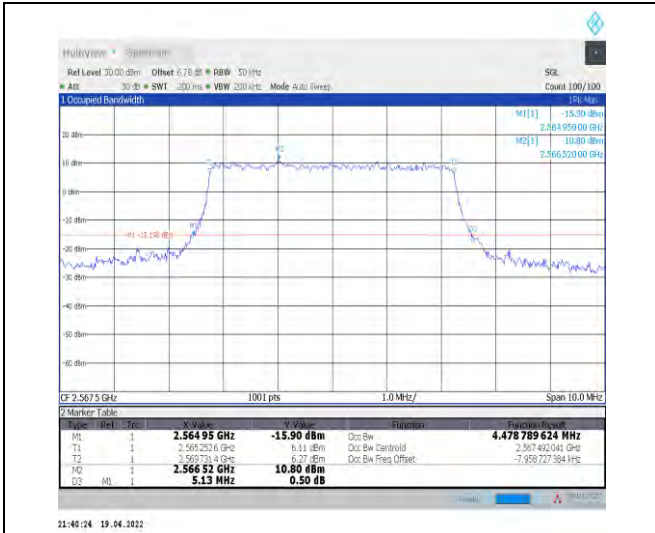
1-N7--15-5-H-7-CP-16QAM-Outer_Full-25@0-Ant1-4 .479-5.130-≤5-PASS
