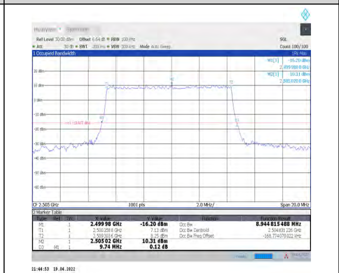
1-N7--15-10-L-5-DFT-256QAM-Outer_Full-50@0-Ant 1-8.945-9.740-≤10-PASS
