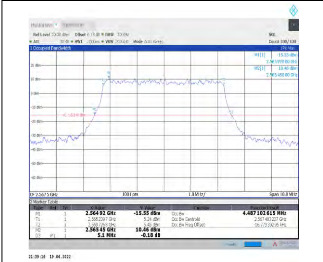
1-N7--15-5-H-5-DFT-256QAM-Outer_Full-25@0-Ant 1-4.487-5.100-≤5-PASS
