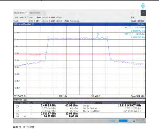
1-N7--15-15-L-4-DFT-64QAM-Outer_Full-75@0-Ant1 -13.416-14.520-≤15-PASS
