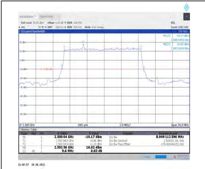
1-N7--15-10-L-2-DFT-PI2BPSK-Outer_Full-50@0-Ant t1-8.949-9.600-≤10-PASS
