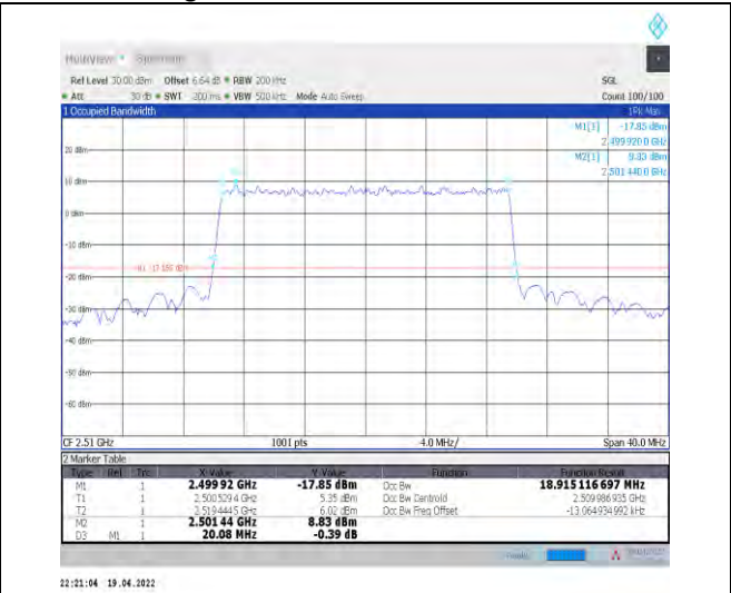
1-N7--15-20-L-9-CP-256QAM-Outer_Full-106@0-Ant t1-18.915-20.080-≤20-PASS
