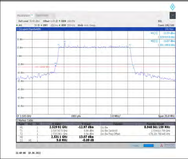
1-N7--15-10-M-4-DFT-64QAM-Outer_Full-50@0-Ant 1-8.949-9.800-≤10-PASS
