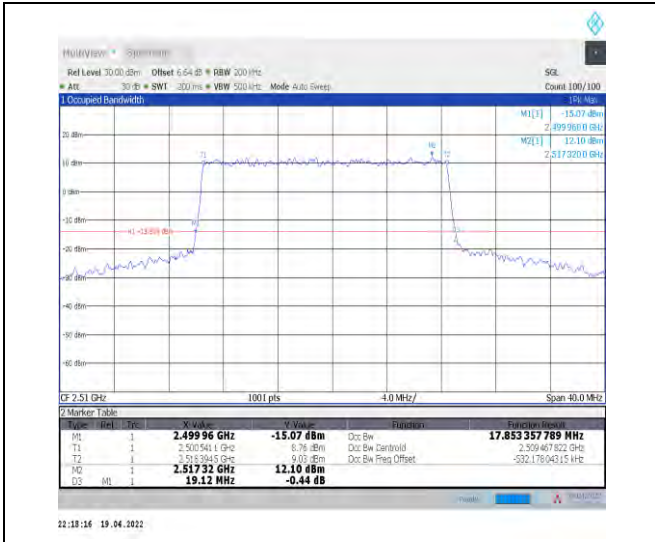
1-N7--15-20-L-4-DFT-64QAM-Outer_Full-100@0-Ant 1-17.853-19.120-≤20-PASS
