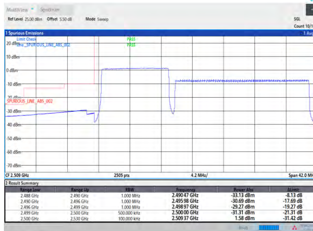
7-7-10MHz-20MHz-QPSK-QPSK-20805-20949-50RB#0-100RB#0
