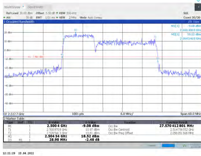
7-7-10MHz-20MHz-QPSK-QPSK-21006-21150-50RB#0-100RB#0
