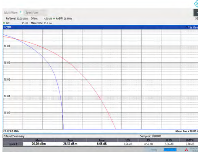
Band71-20MHz-QPSK-133222-100RB#0
