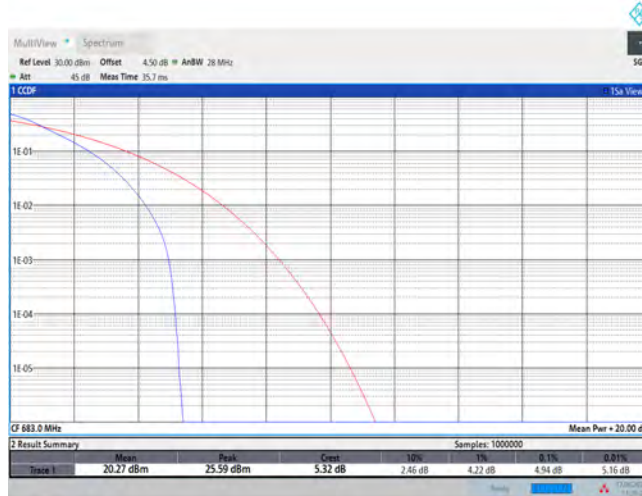
Band71-20MHz-QPSK-133322-100RB#0
