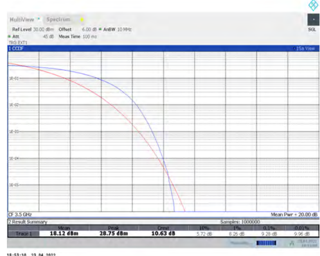
Band42-20MHz-QPSK-42590-100RB#0
