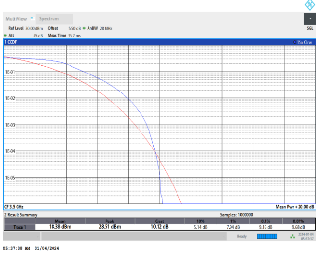
Band42-20MHz-QPSK-42590-100RB#0
