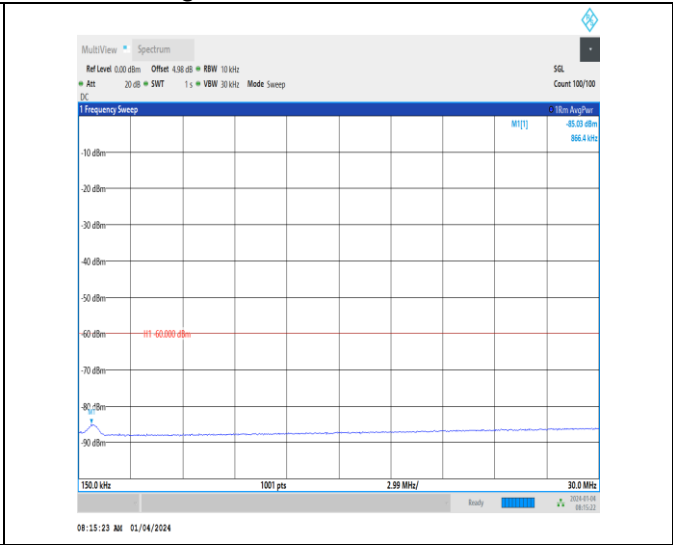
Band43_20MHz_QPSK_44490_1RB#0_0.15-30_0.15-30
