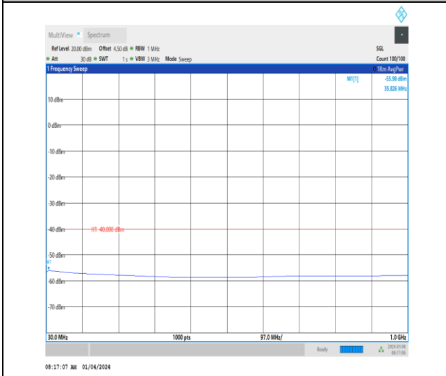
Band43_20MHz_QPSK_44490_1RB#0_30-1000_30-1000
