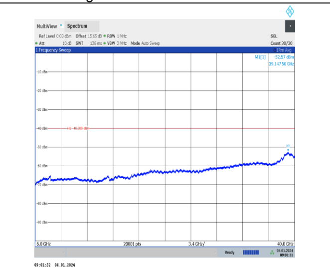
Band43_20MHz_QPSK_44490_1RB#0_6000~40000_6000~40000
