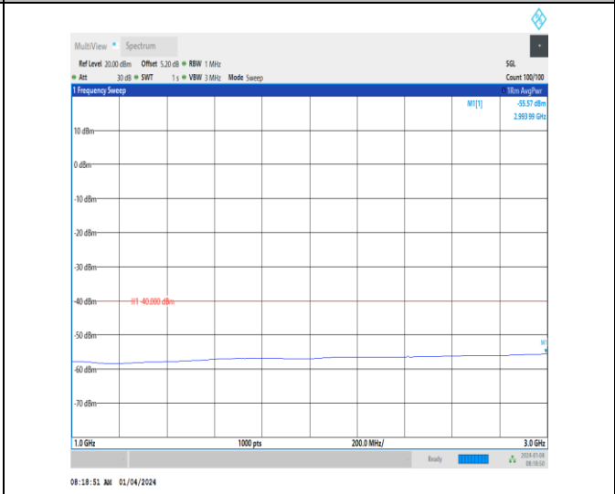
Band43_20MHz_QPSK_44490_1RB#0_1000-3000_1000-3000
