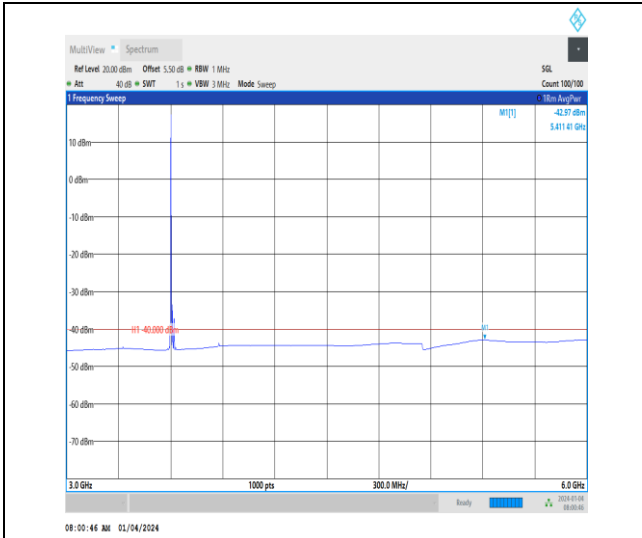
Band43_20MHz_QPSK_43690_1RB#0_3000~6000_3000~6000
