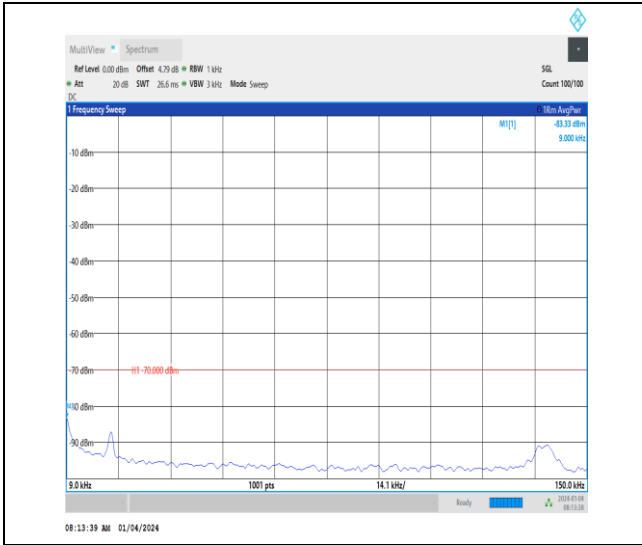
Band43_20MHz_QPSK_44490_1RB#0_0.009-0.15_0.00-9-0.15
