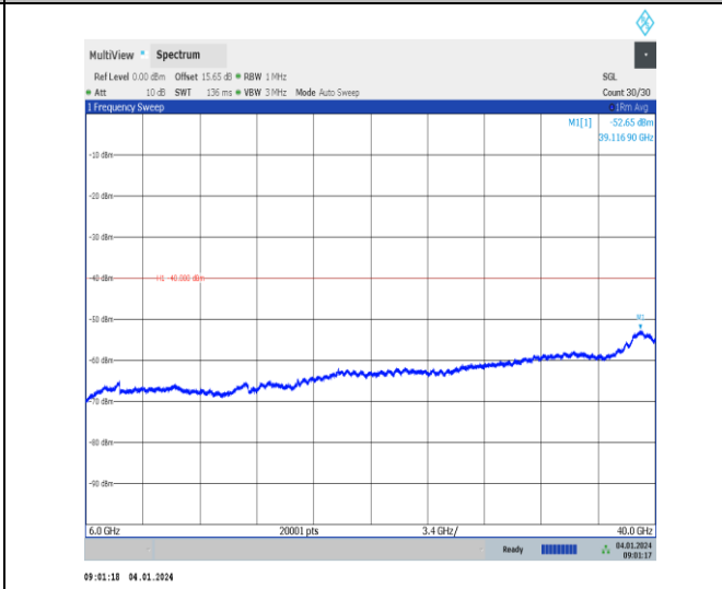
Band43_20MHz_QPSK_44090_1RB#0_6000~40000_6000~40000
