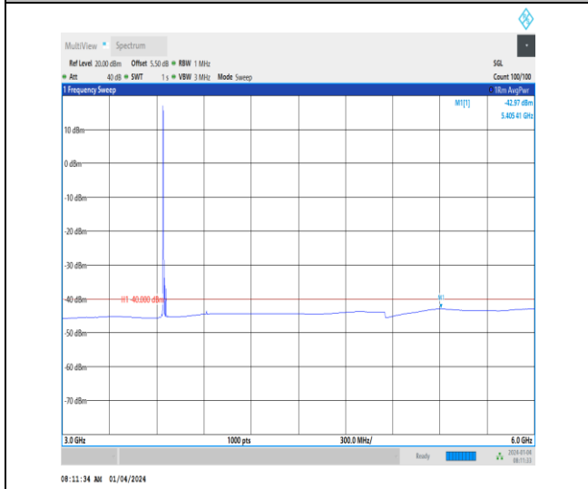
Band43_20MHz_QPSK_44090_1RB#0_3000~6000_3000~6000
