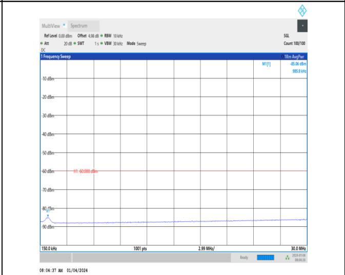
Band43_20MHz_QPSK_44090_1RB#0_0.15~30_0.15~30
