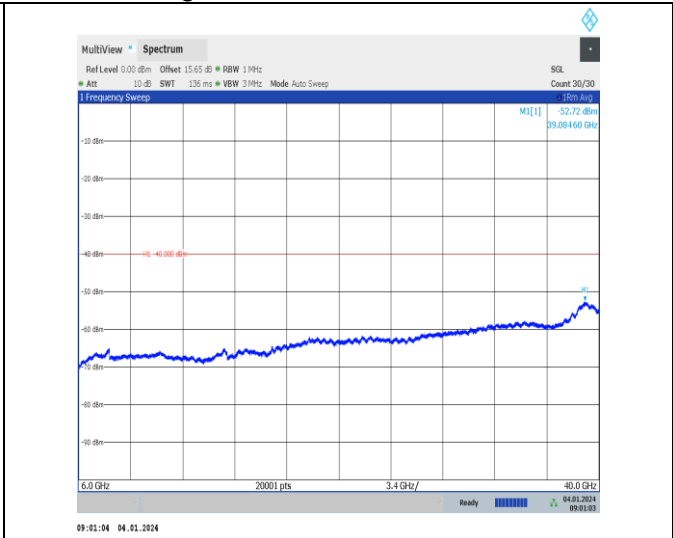
Band43_20MHz_QPSK_43690_1RB#0_6000~40000_6000~40000
