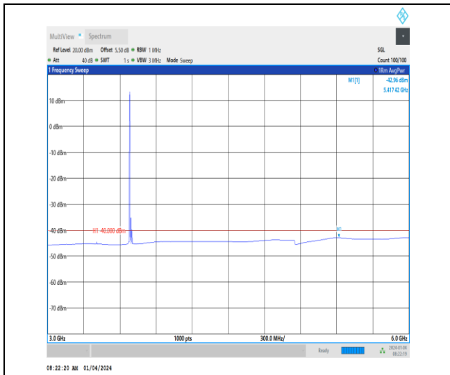
Band43_20MHz_QPSK_44490_1RB#0_3000~6000_3000~6000
