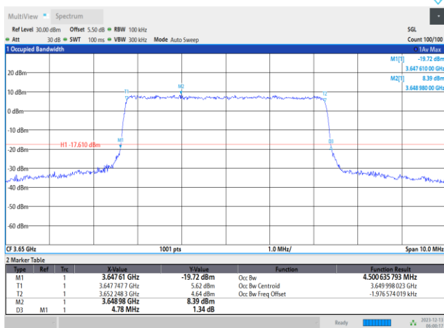
Band43-5MHz-16QAM-44090-25RB#0
