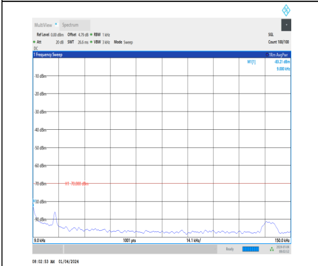
Band43_20MHz_QPSK_44090_1RB#0_0.009~0.15_0.009~0.15
