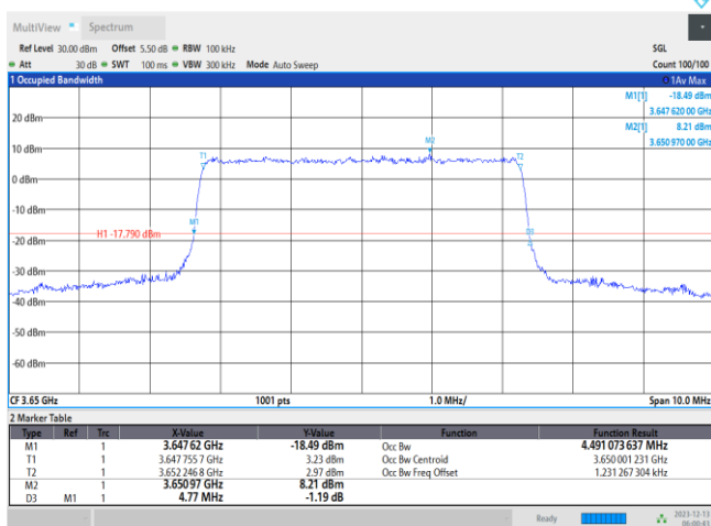
Band43-5MHz-16QAM-44090-25RB#0
