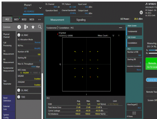
7-7-20MHz-20MHz-16QAM-16QAM -21001-21199-100RB#0-100RB#0
