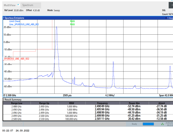
7-7-10MHz-20MHz-QPSK-QPSK-20805-20949-50RB#0-100RB#0
