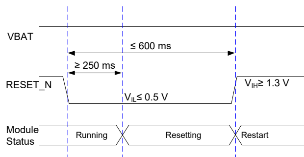
Figure 16: Reset Timing
