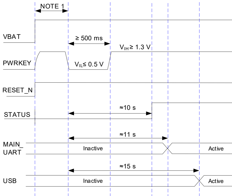
Figure 13: Power-up Timing
