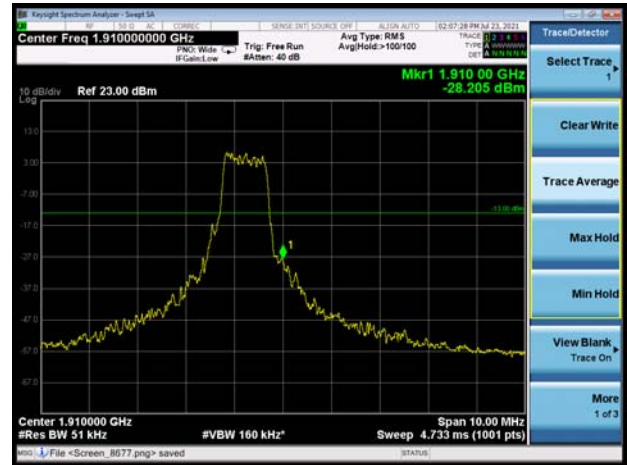
LTE-M Band 2 5MHz 16QAM 1RB CH-High
