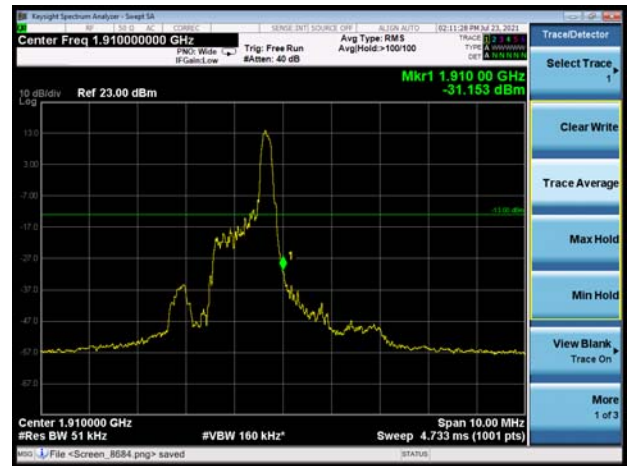
LTE-M Band 2 5MHz 16QAM 100%RB CH-High
