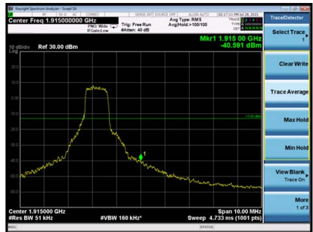
LTE-M Band 25 20MHz 16QAM 100%RB CH-High
