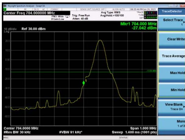
NB-IoT Band 17 BPSK 3.75KHz 1@0 CH-Low
