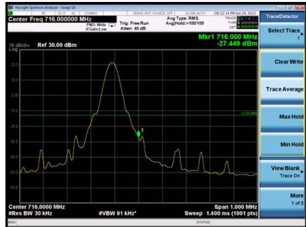
NB-IoT Band 12 QPSK 3.75KHz 1@0 CH- High
