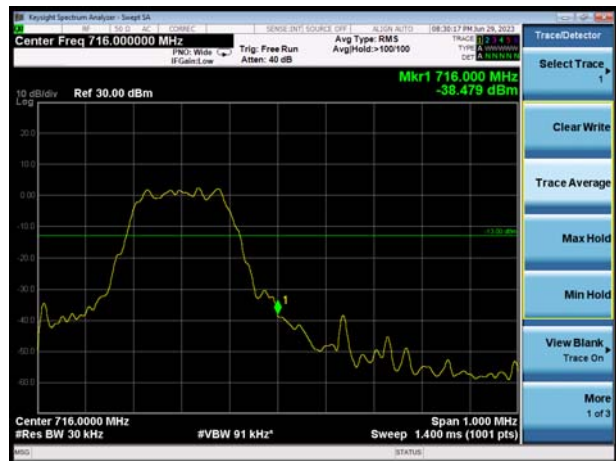
NB-IoT Band 17 BPSK 3.75KHz 1@0 CH- High
