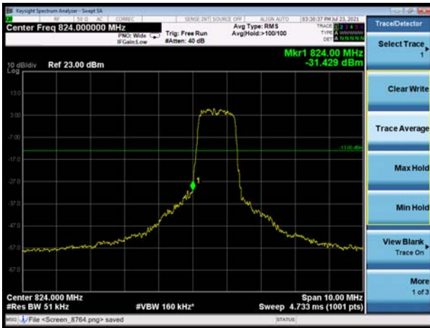
LTE-M Band 5 QPSK 3MHz CH-Low 1RB
