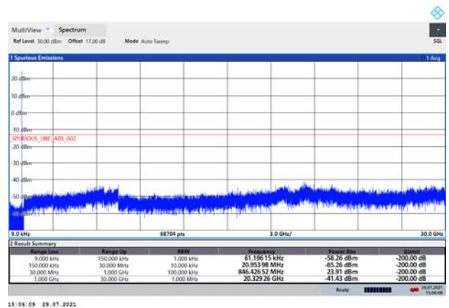
LTE-M Band 5 3MHz CH-High 9kHz~30GHz
