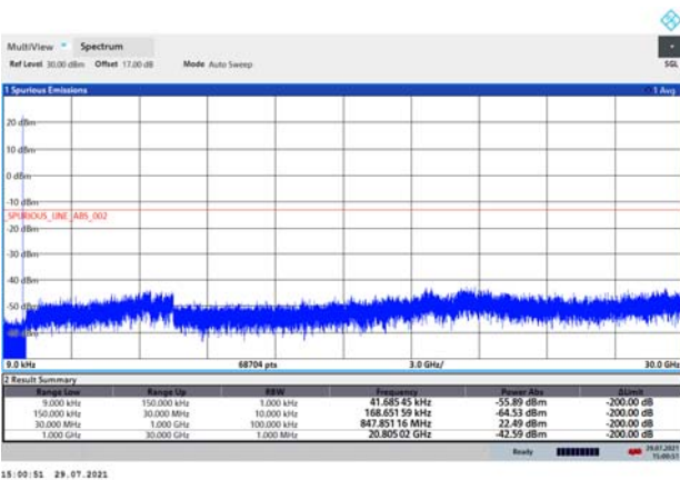
LTE-M Band 5 1.4MHz CH-High 9kHz~30GHz
