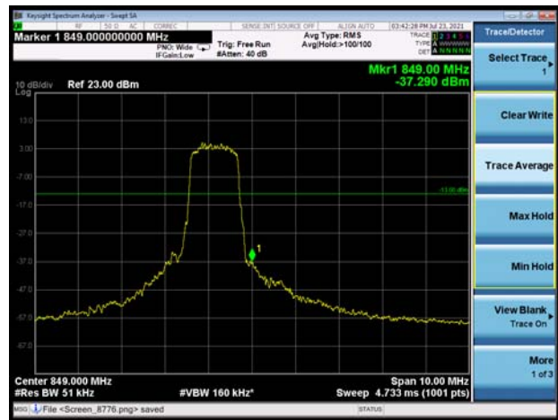
LTE-M Band 5 QPSK 5MHz CH-High 1RB
