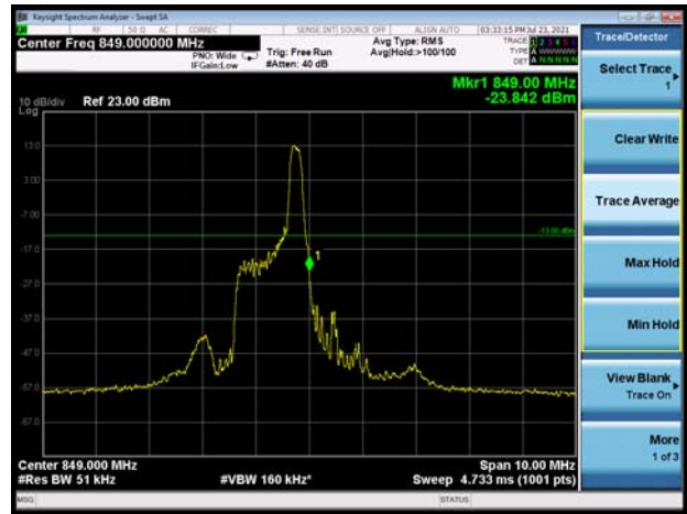
LTE-M Band 5 QPSK 1.4MHz CH-High 100%RB
