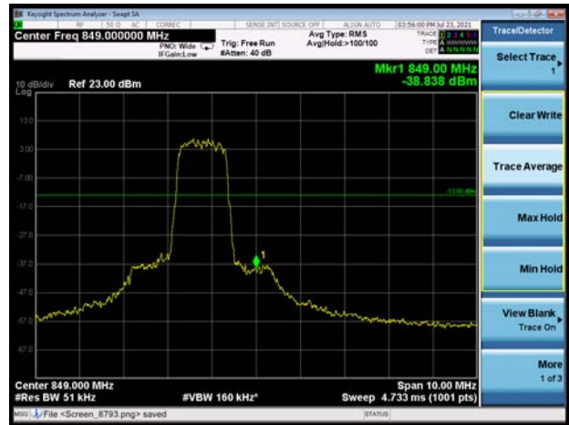
LTE-M Band 5 16QAM 1.4MHz CH-High 1RB
