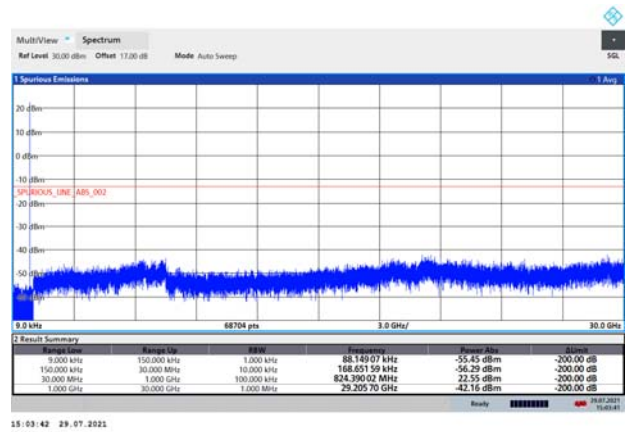
LTE-M Band 5 3MHz CH-Middle 9kHz~30GHz
