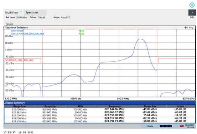
LTE Band 26 QPSK 3MHz CH-High 1RB
