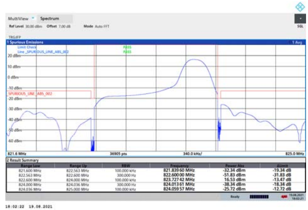
LTE Band 26 QPSK 1.4MHz CH-High 100%RB
