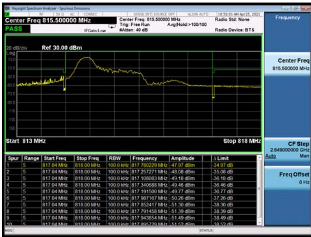
LTE-M Band 26 16QAM 3MHz CH-Low 100%RB
