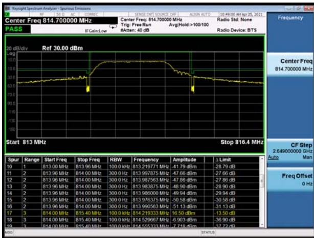
LTE-M Band 26 16QAM 3MHz CH-Low 1RB
