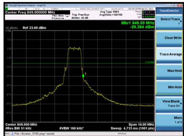
LTE-M Band 26 16QAM 1.4MHz CH-High 100%RB
