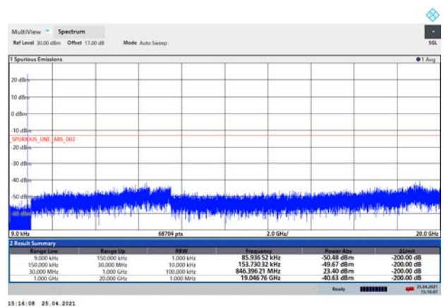
LTE-M Band 26 3MHz CH-High 9kHz~20GHz
