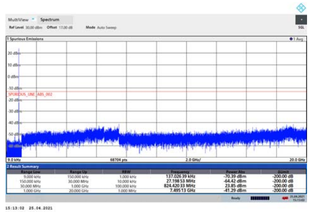
LTE-M Band 26 3MHz CH-Middle 9kHz~20GHz
