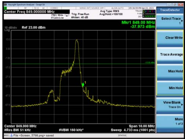
LTE-M Band 26 16QAM 3MHz CH-High 100%RB
