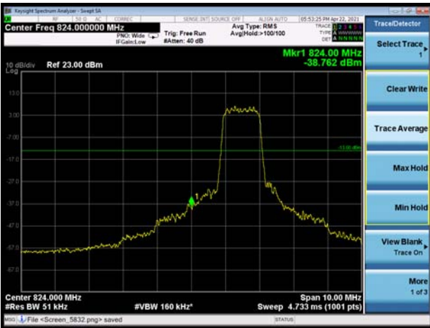
LTE-M Band 26 16QAM 1.4MHz CH-Low 1RB
