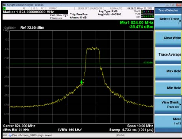
LTE-M Band 5 16QAM 3MHz CH-Low 100%RB
