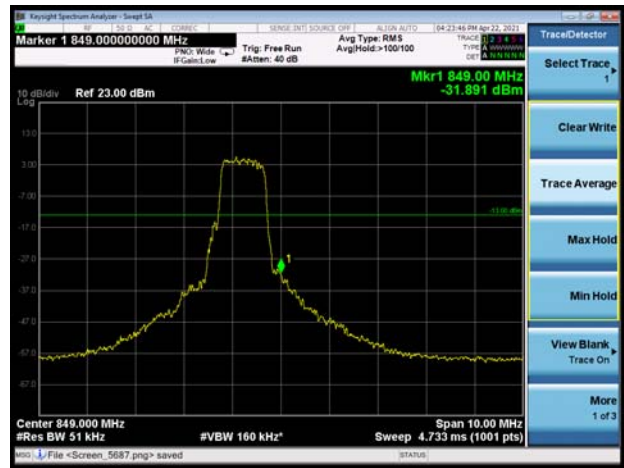
LTE-M Band 5 16QAM 3MHz CH-High 100%RB
