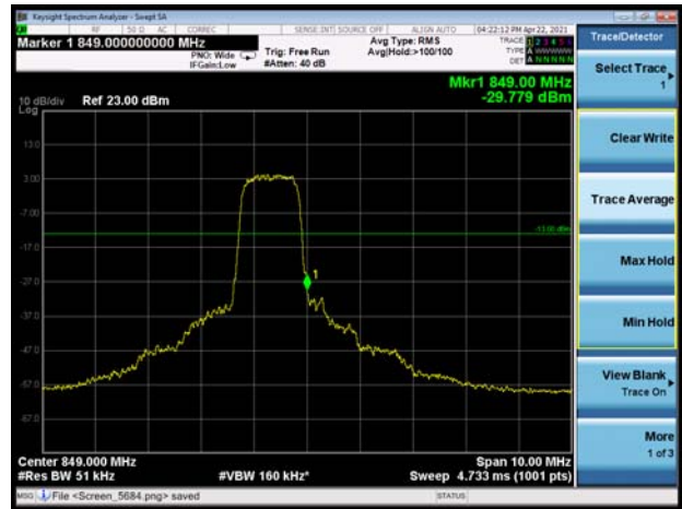
LTE-M Band 5 QPSK 3MHz CH-High 1RB
