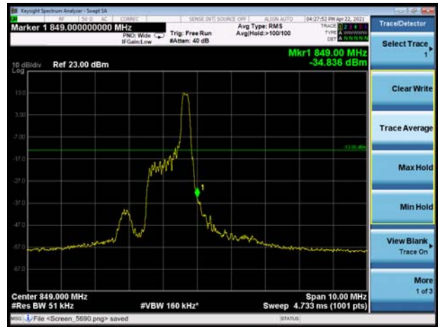
LTE-M Band 5 16QAM 5MHz CH-High 100%RB
