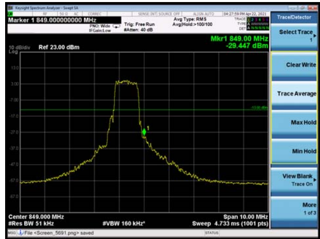
LTE-M Band 5 16QAM 10MHz CH-High 1RB
