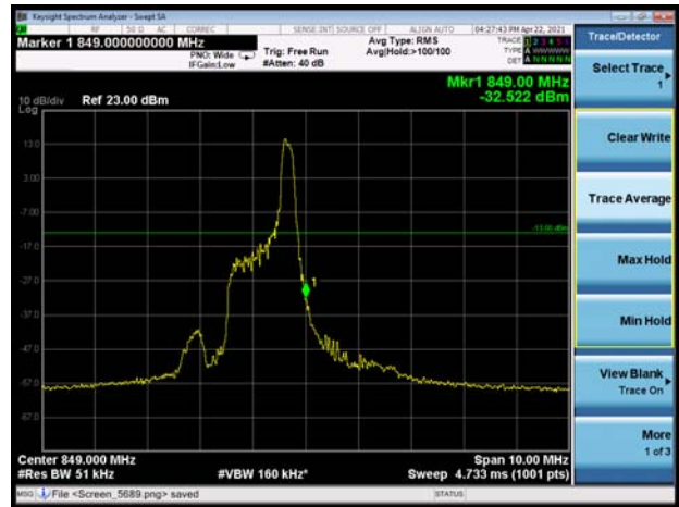
LTE-M Band 5 QPSK 5MHz CH-High 100%RB
