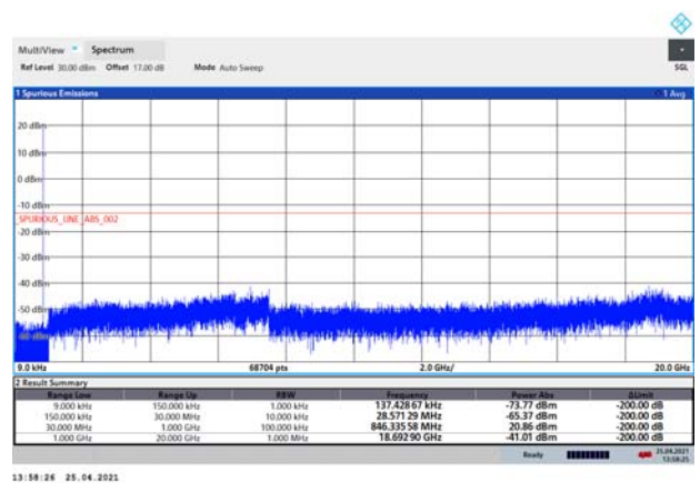
LTE-M Band 5 3MHz CH-High 9kHz~20GHz
