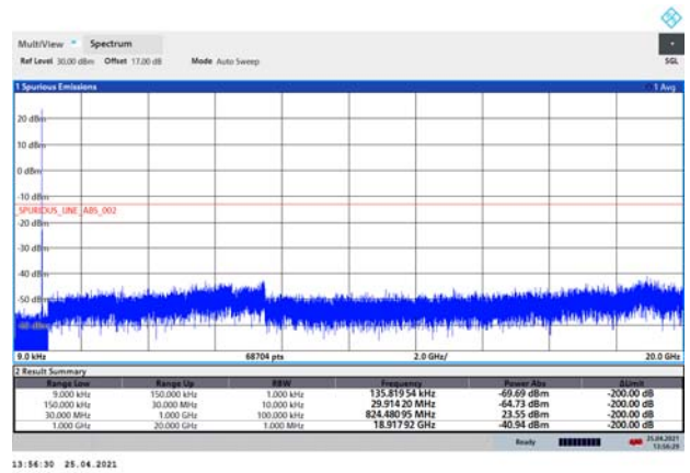
LTE-M Band 5 3MHz CH-Middle 9kHz~20GHz
