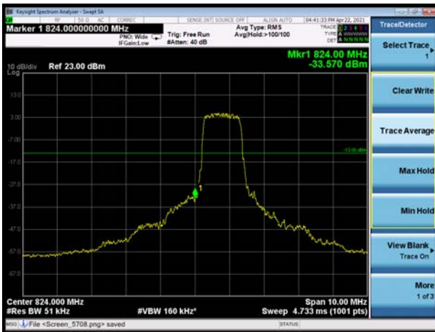
LTE-M Band 5 QPSK 5MHz CH-Low 100%RB
