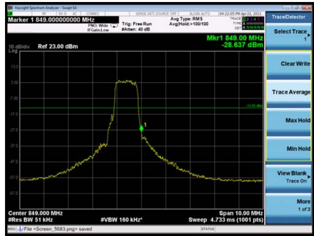
LTE-M Band 5 16QAM 3MHz CH-High 1RB
