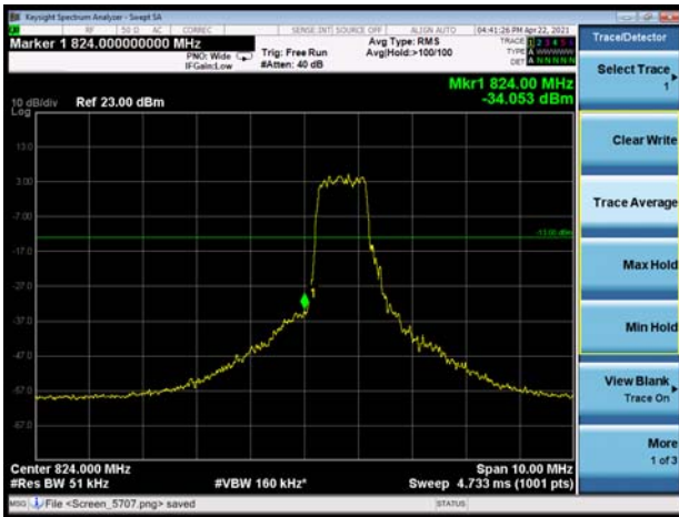
LTE-M Band 5 16QAM 10MHz CH-Low 1RB
