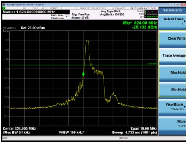
LTE-M Band 5 QPSK 1.4MHz CH-Low 100%RB
