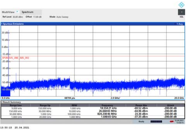
LTE-M Band 5 1.4MHz CH-Middle 9kHz~20GHz
