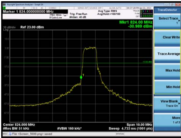
LTE-M Band 5 16QAM 3MHz CH-Low 1RB
