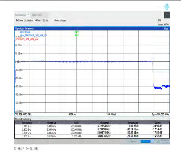
1-N78-3700-3800-30-90-H-6-CP-QPSK-Outer_Full-245@0-Ant1-1--PASS-see graph
