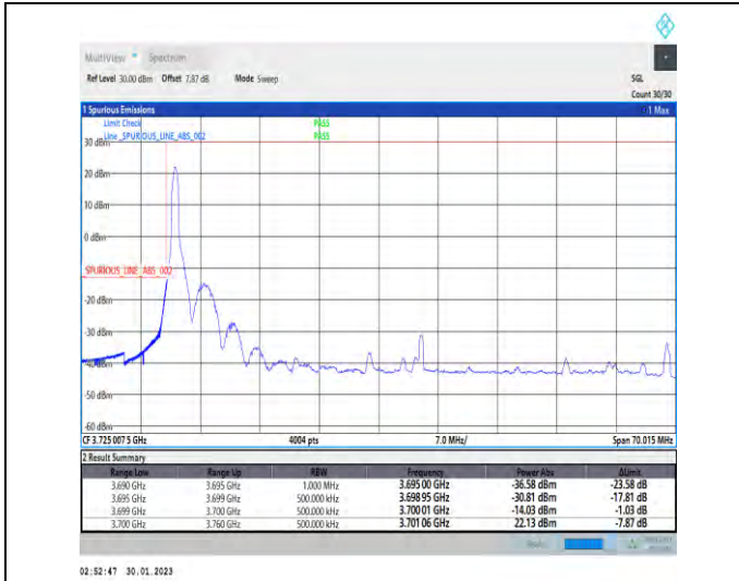
1-N78-3700-3800-30-60-L-1-DFT-PI2BPSK-Edge_1RB_Left-1@0-Ant1-1--PASS-see graph
