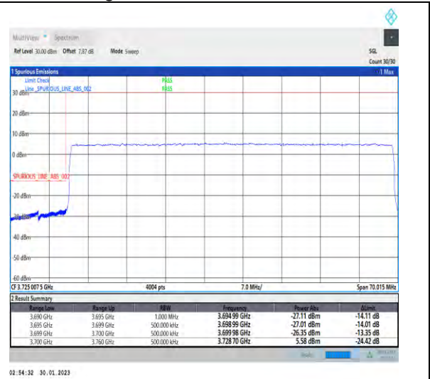
1-N78-3700-3800-30-60-L-3-DFT-PI2BPSK-Outer_Full-162@0-Ant1-1--PASS-see graph
