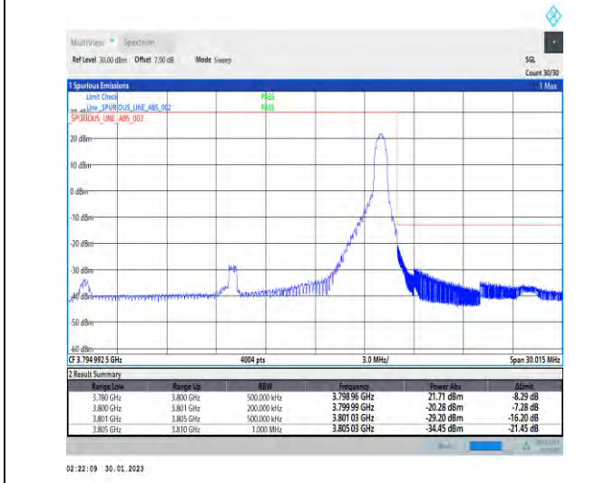
1-N78-3700-3800-30-20-H-5-CP-QPSK-Edge_1RB_Right-1@50-Ant1-1--PASS-see graph
