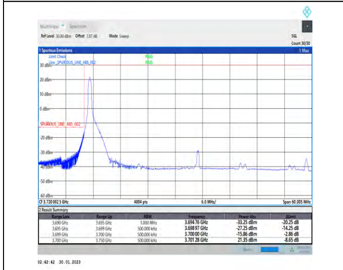
1-N78-3700-3800-30-50-L-4-CP-QPSK-Edge_1RB_Lef t-1@0-Ant1-1--PASS-see graph
