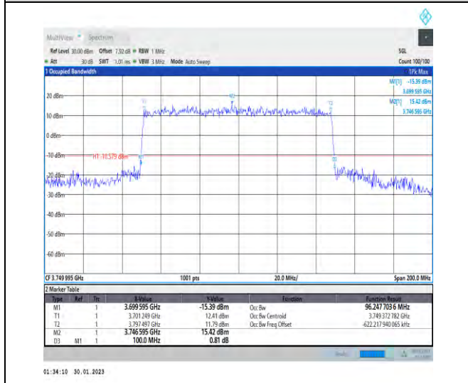
1-N78-3700-3800-30-100-H-1-DFT-QPSK-Outer_Ful l-270@0-Ant1-96.248-100.000-≤100-PASS
