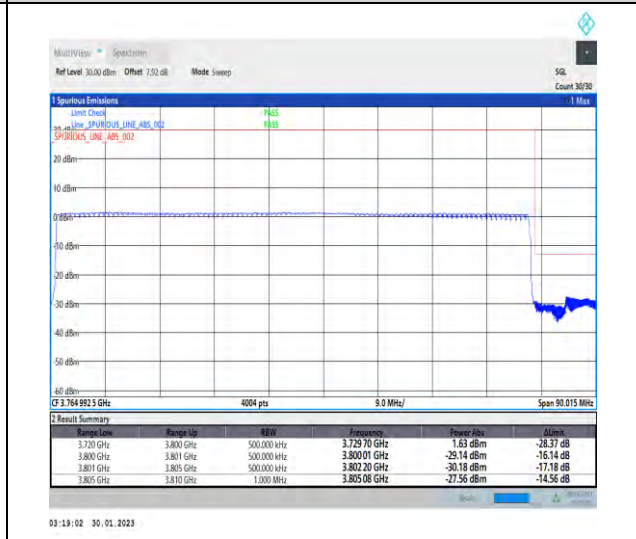
1-N78-3700-3800-30-80-H-6-CP-QPSK-Outer_Full-217@0-Ant1-1--PASS-see graph
