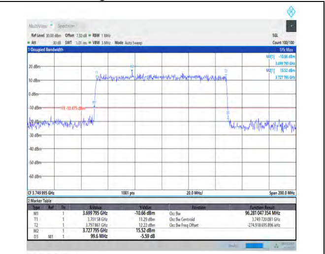
1-N78-3700-3800-30-100-M-1-DFT-QPSK-Outer_Full-270@0-Ant1-96.281-99.600-≤100-PASS
