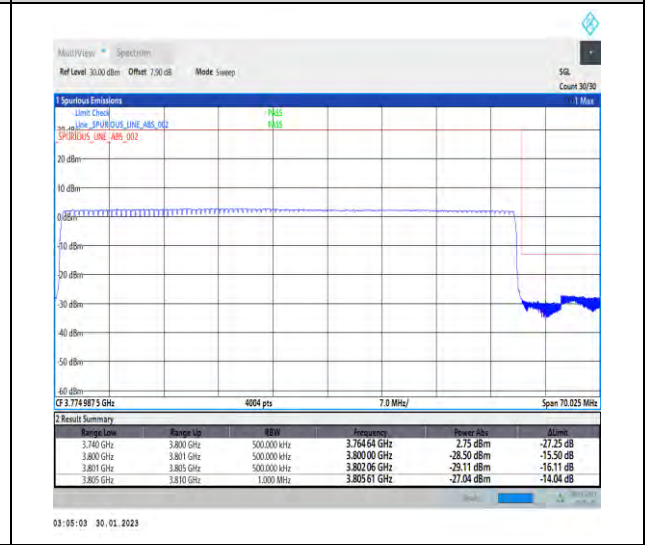
1-N78-3700-3800-30-60-H-6-CP-QPSK-Outer_Full-162@0-Ant1-1--PASS-see graph
