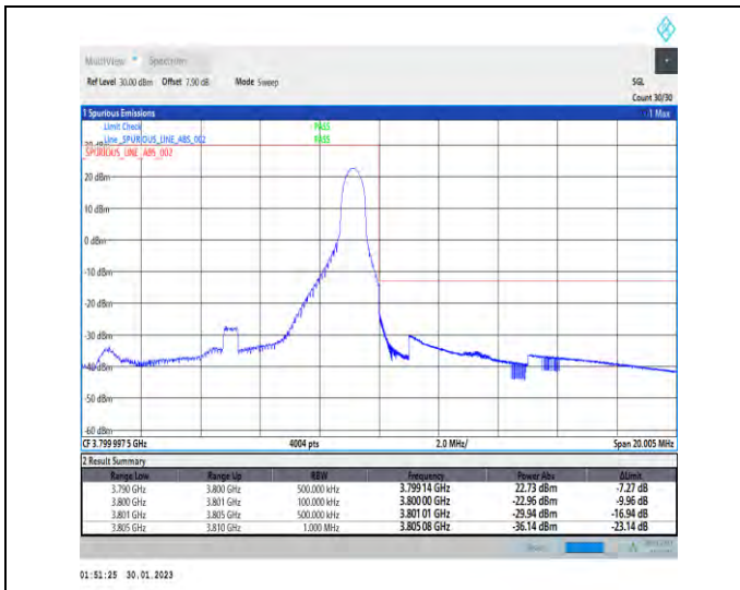
1-N78-3700-3800-30-10-H-2-DFT-PI2BPSK-Edge_1R_B_Right-1@23-Ant1-1--PASS-see graph
