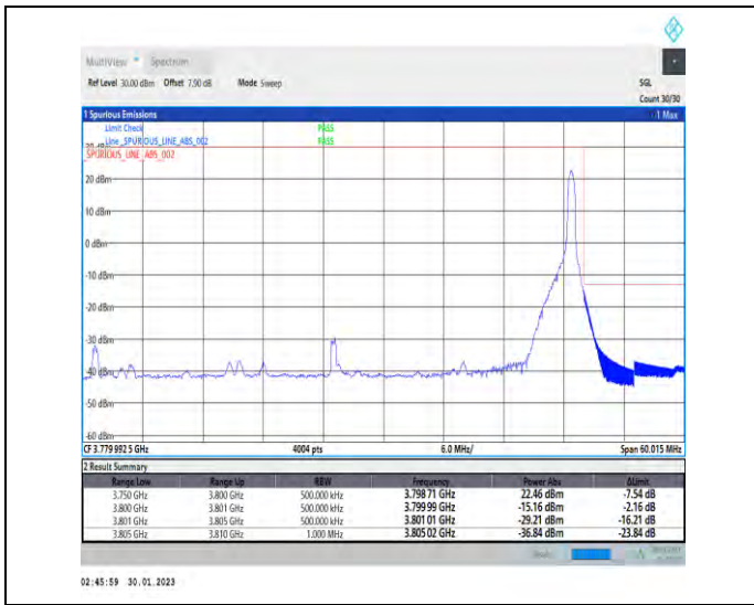
1-N78-3700-3800-30-50-H-2-DFT-PI2BPSK-Edge_1R_B_Right-1@132-Ant1-1--PASS-see graph
