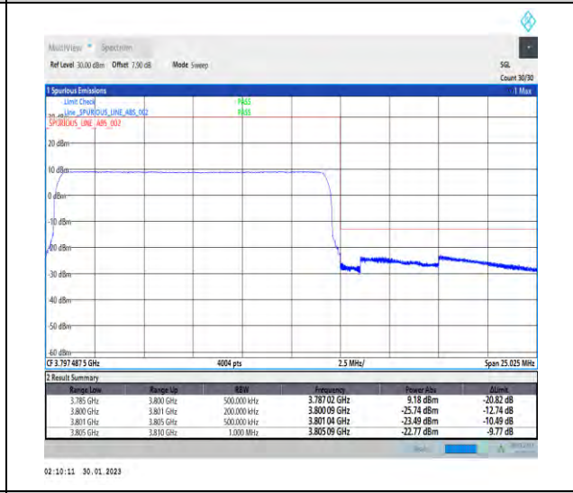
1-N78-3700-3800-30-15-H-6-CP-QPSK-Outer_Full-38@0-Ant1-1--PASS-see graph
