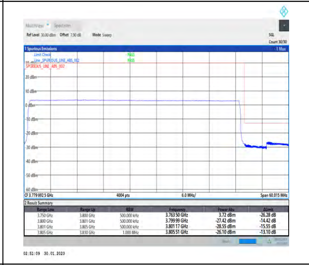
1-N78-3700-3800-30-50-H-6-CP-QPSK-Outer_Full-133@0-Ant1-1--PASS-see graph
