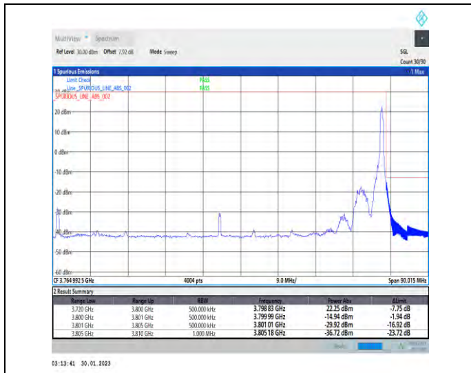
1-N78-3700-3800-30-80-H-2-DFT-PI2BPSK-Edge_1R_B_Right-1@216-Ant1-1--PASS-see graph
