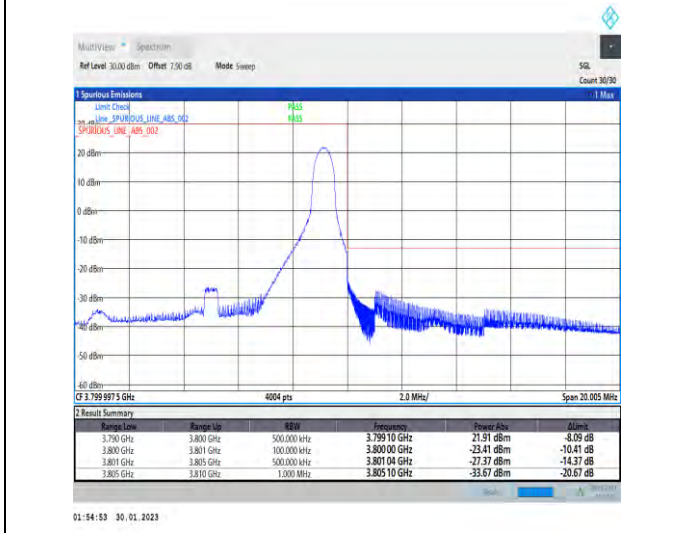
1-N78-3700-3800-30-10-H-5-CP-QPSK-Edge_1RB_Right-1@23-Ant1-1--PASS-see graph
