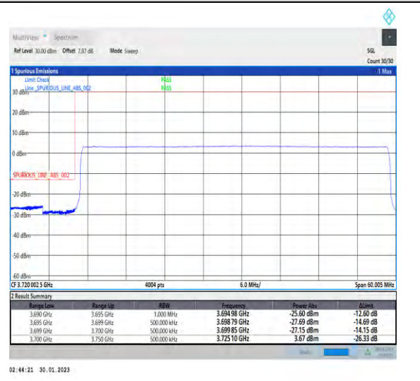
1-N78-3700-3800-30-50-L-6-CP-QPSK-Outer_Full -133@0-Ant1-1--PASS-see graph
