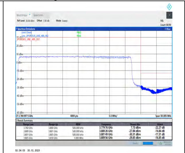
1-N78-3700-3800-30-40-H-3-DFT-PI2BPSK-Outer_Full-100@0-Ant1-1--PASS-see graph
