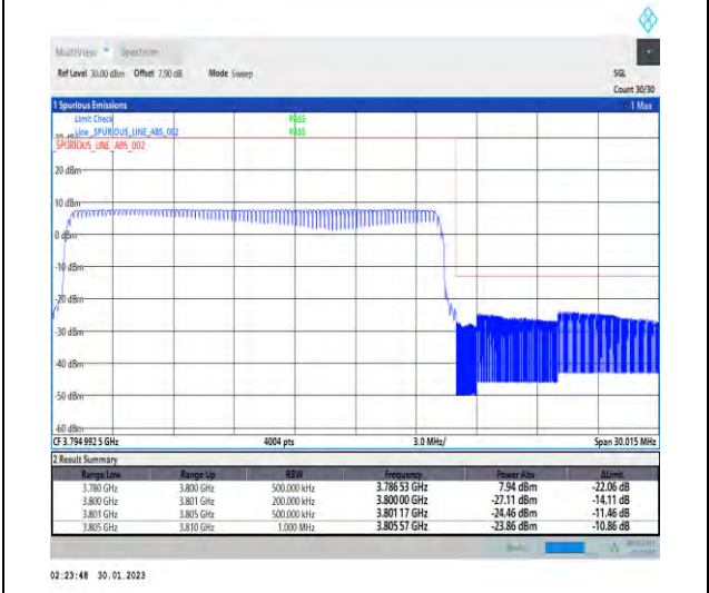
1-N78-3700-3800-30-20-H-6-CP-QPSK-Outer_Full-51@0-Ant1-1--PASS-see graph
