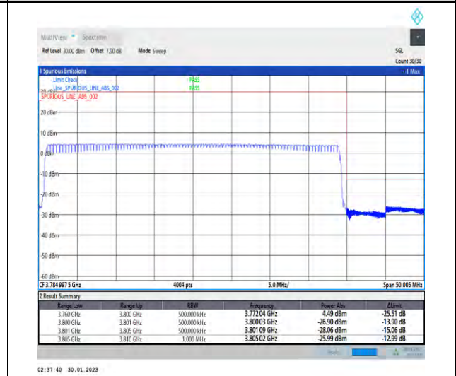
1-N78-3700-3800-30-40-H-6-CP-QPSK-Outer_Full-106@0-Ant1-1--PASS-see graph
