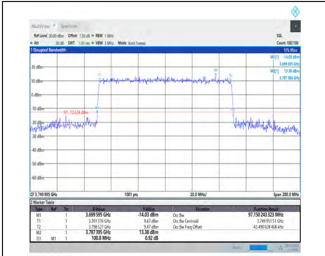
1-N78-3700-3800-30-100-H-7-CP-16QAM-Outer_Ful I-273@0-Ant1-97.15-100.800-≤100-PASS
