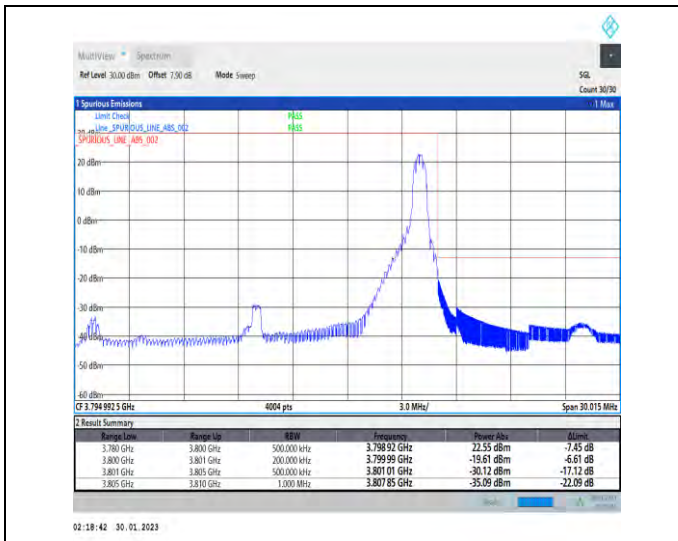
1-N78-3700-3800-30-20-H-2-DFT-PI2BPSK-Edge_1R_B_Right-1@50-Ant1-1--PASS-see graph
