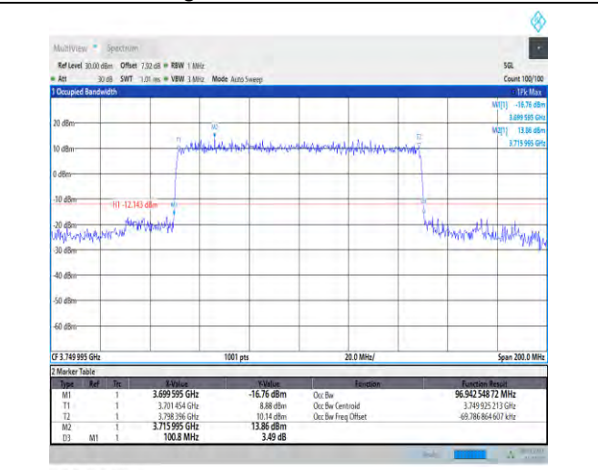
1-N78-3700-3800-30-100-L-6-CP-QPSK-Outer_Full-273@0-Ant1-96.943-100.800-≤100-PASS
