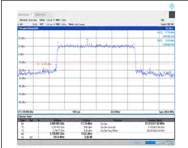
1-N78-3700-3800-30-100-L-7-CP-16QAM-Outer_Ful I-273@0-Ant1-97.314-101.000-≤100-PASS
