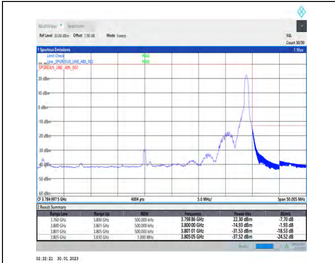
1-N78-3700-3800-30-40-H-2-DFT-PI2BPSK-Edge_1R_B_Right-1@105-Ant1-1--PASS-see graph
