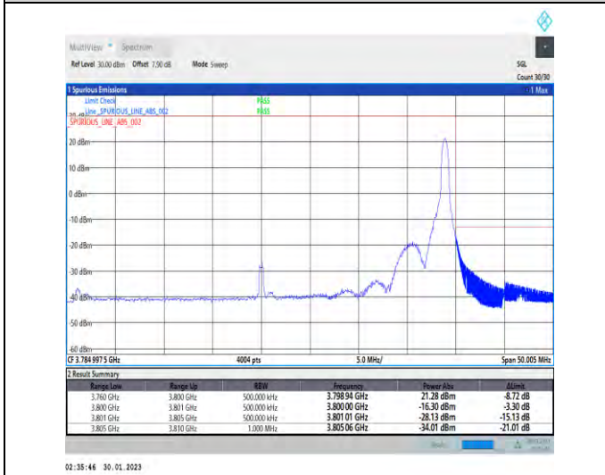
1-N78-3700-3800-30-40-H-5-CP-QPSK-Edge_1RB_Right-1@105-Ant1-1--PASS-see graph
