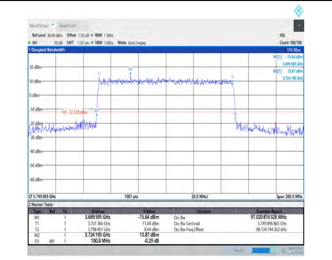
1-N78-3700-3800-30-100-L-8-CP-64QAM-Outer_Full -273@0-Ant1-97.021-100.800-≤100-PASS
