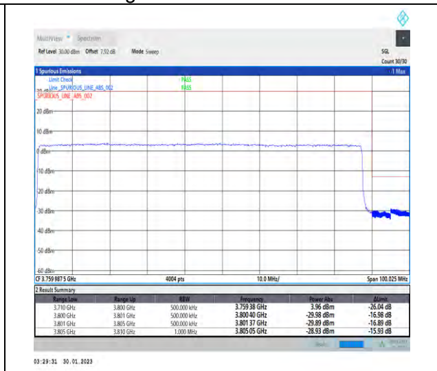
1-N78-3700-3800-30-90-H-3-DFT-PI2BPSK-Outer_Full-240@0-Ant1-1--PASS-see graph
