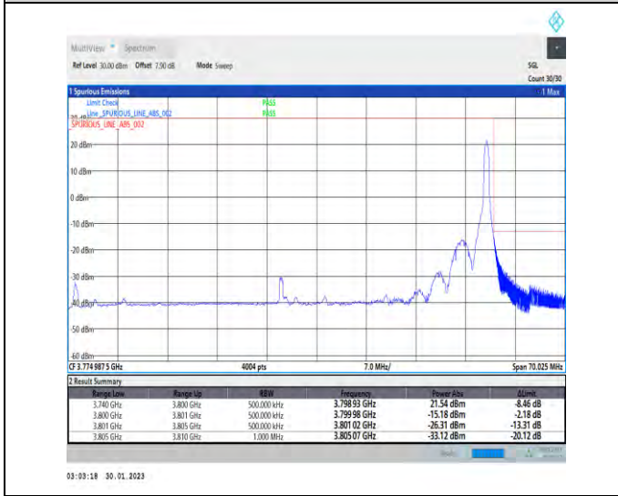
1-N78-3700-3800-30-60-H-5-CP-QPSK-Edge_1RB_Right-1@161-Ant1-1--PASS-see graph
