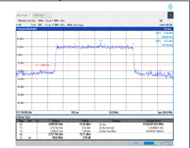
1-N78-3700-3800-30-100-H-8-CP-64QAM-Outer_Ful I-273@0-Ant1-97.053-100.800-≤100-PASS
