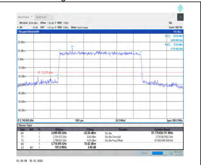
1-N78-3700-3800-30-100-M-9-CP-256QAM-Outer_F ull-273@0-Ant1-97.18-101.000-≤100-PASS
