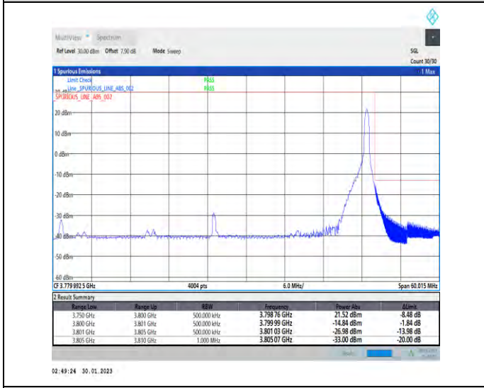
1-N78-3700-3800-30-50-H-5-CP-QPSK-Edge_1RB_Right-1@132-Ant1-1--PASS-see graph
