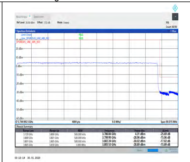
1-N78-3700-3800-30-80-H-3-DFT-PI2BPSK-Outer_Full-216@0-Ant1-1--PASS-see graph
