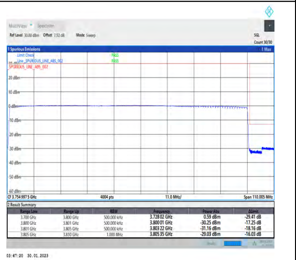
1-N78-3700-3800-30-100-H-6-CP-QPSK-Outer_Full-273@0-Ant1-1--PASS-see graph
