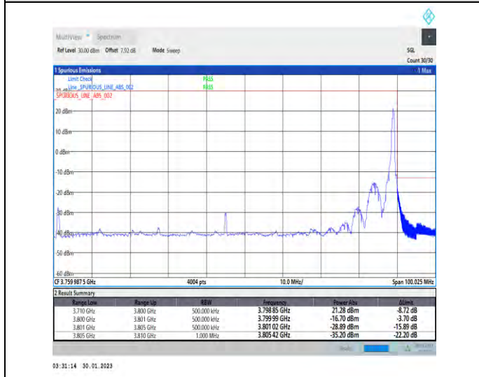
1-N78-3700-3800-30-90-H-5-CP-QPSK-Edge_1RB_Right-1@244-Ant1-1--PASS-see graph
