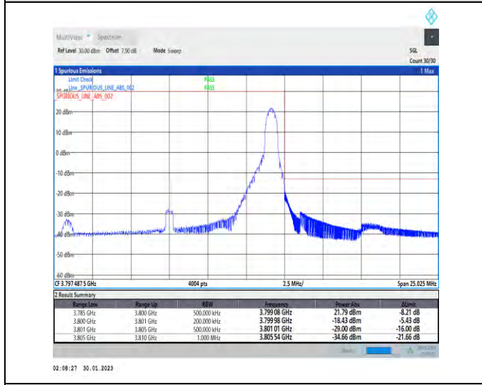
1-N78-3700-3800-30-15-H-5-CP-QPSK-Edge_1RB_Right-1@37-Ant1-1--PASS-see graph
