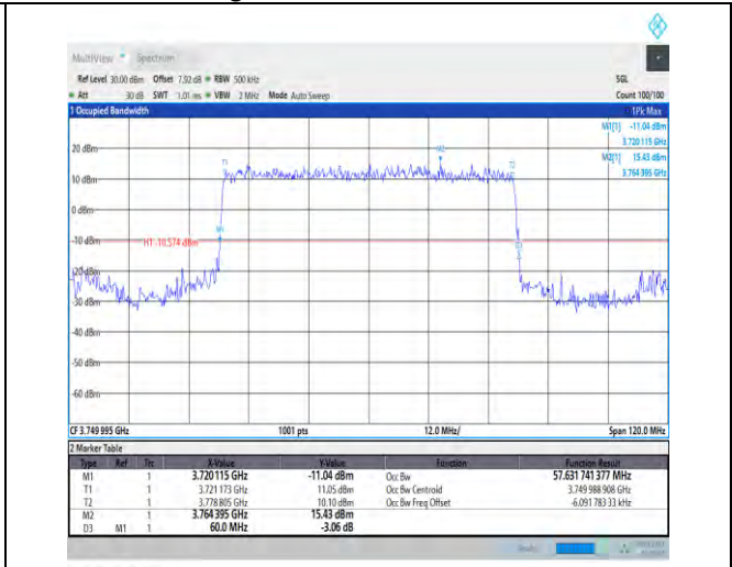
1-N78-3700-3800-30-60-M-2-DFT-PI2BPSK-Outer_Full-162@0-Ant1-57.632-60.000-≤60-PASS
