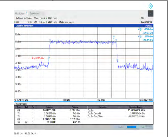
1-N78-3700-3800-30-90-L-5-DFT-256QAM-Outer_Fu ll-240@0-Ant1-85.578-89.100-≤90-PASS
