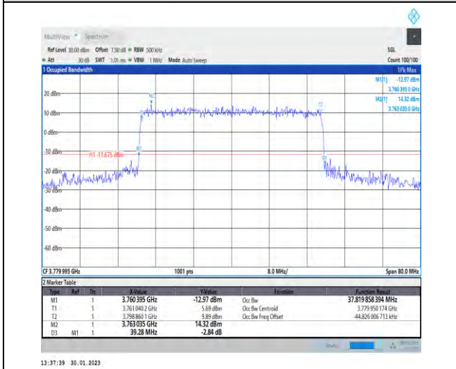
1-N78-3700-3800-30-40-H-8-CP-64QAM-Outer_Full-106@0-Ant1-37.82-39.280-≤40-PASS
