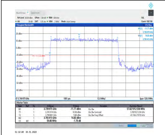
1-N78-3700-3800-30-60-H-2-DFT-PI2BPSK-Outer_Full-162@0-Ant1-57.827-59.880-≤60-PASS
