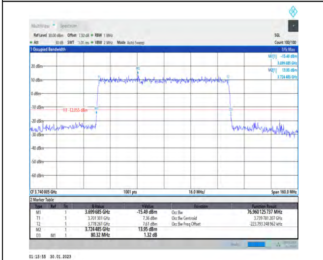
1-N78-3700-3800-30-80-L-5-DFT-256QAM-Outer_Full -216@0-Ant1-76.96-80.320-≤80-PASS
