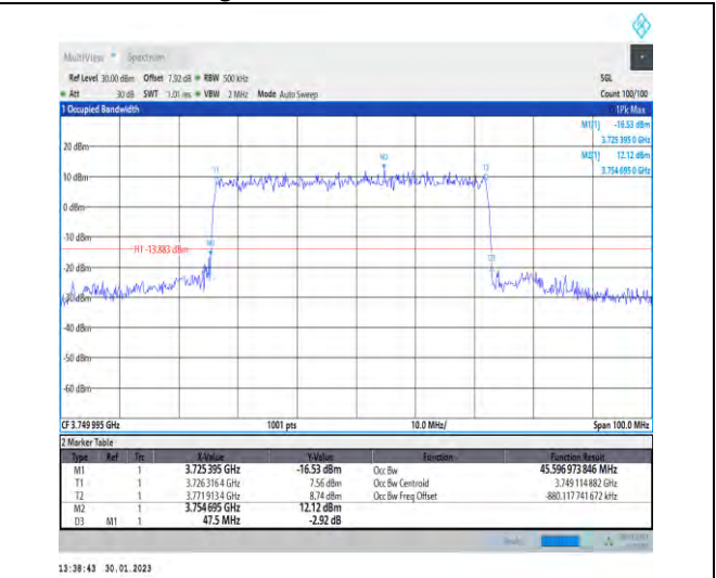
1-N78-3700-3800-30-50-M-5-DFT-256QAM-Outer_F uII-128@0-Ant1-45.597-47.500-≤50-PASS
