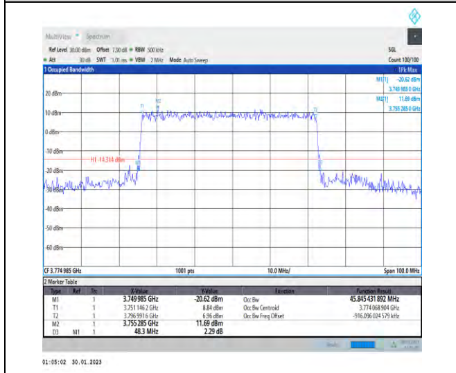
1-N78-3700-3800-30-50-H-5-DFT-256QAM-Outer_Full-128@0-Ant1-45.845-48.300-≤50-PASS
