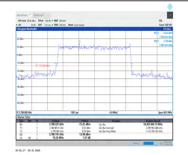
1-N78-3700-3800-30-20-H-8-CP-64QAM-Outer_Full-51@0-Ant1-18.203-19.240-≤20-PASS
