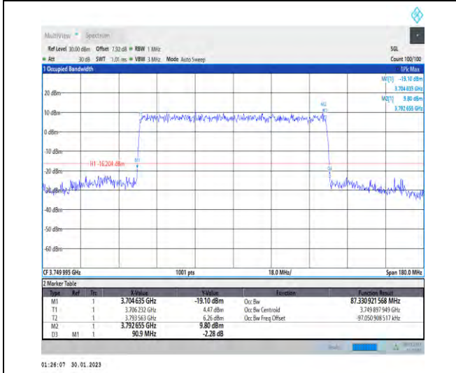
1-N78-3700-3800-30-90-M-9-CP-256QAM-Outer_Fu II-245@0-Ant1-87.331-90.900-≤90-PASS
