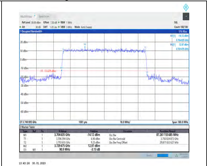
1-N78-3700-3800-30-90-M-8-CP-64QAM-Outer_Full -245@0-Ant1-87.261-90.900-≤90-PASS
