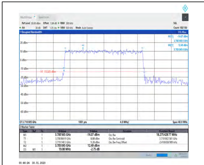
1-N78-3700-3800-30-20-L-7-CP-16QAM-Outer_Full-51@0-Ant1-18.275-19.080-≤20-PASS
