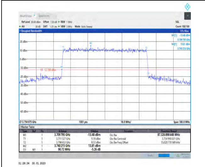
1-N78-3700-3800-30-90-H-8-CP-64QAM-Outer_Full-245@0-Ant1-87.327-90.720-<=90-PASS
