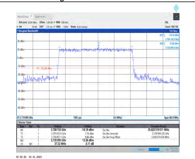
1-N78-3700-3800-30-40-L-5-DFT-256QAM-Outer_Fu ll-100@0-Ant1-35.826-37.520-≤40-PASS
