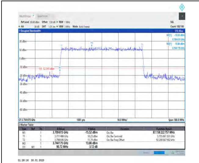
1-N78-3700-3800-30-90-H-6-CP-QPSK-Outer_Full-245@0-Ant1-87.158-90.720-<=90-PASS
