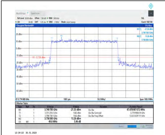
1-N78-3700-3800-30-50-H-7-CP-16QAM-Outer_Full-133@0-Ant1-47.479-49.800-≤50-PASS
