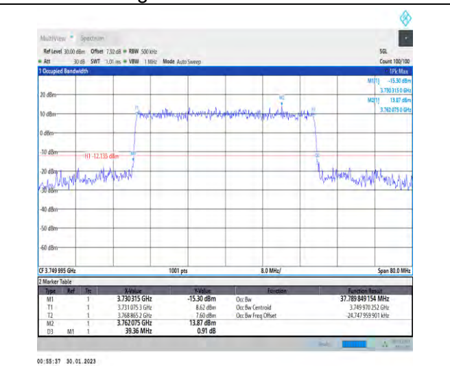
1-N78-3700-3800-30-40-M-8-CP-64QAM-Outer_Full 106@0-Ant1-37.79-39.360-≤40-PASS
