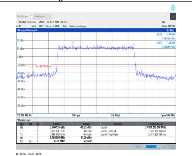
1-N78-3700-3800-30-40-H-7-CP-16QAM-Outer_Full-106@0-Ant1-37.811-39.680-≤40-PASS
