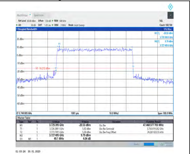
1-N78-3700-3800-30-50-M-9-CP-256QAM-Outer_Ful I-133@0-Ant1-47.46-49.100-≤50-PASS
