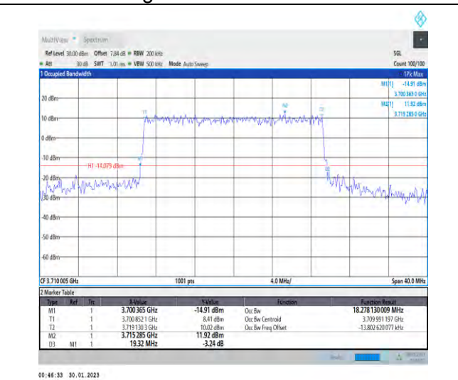
1-N78-3700-3800-30-20-L-8-CP-64QAM-Outer_Full-51@0-Ant1-18.278-19.320-≤20-PASS
