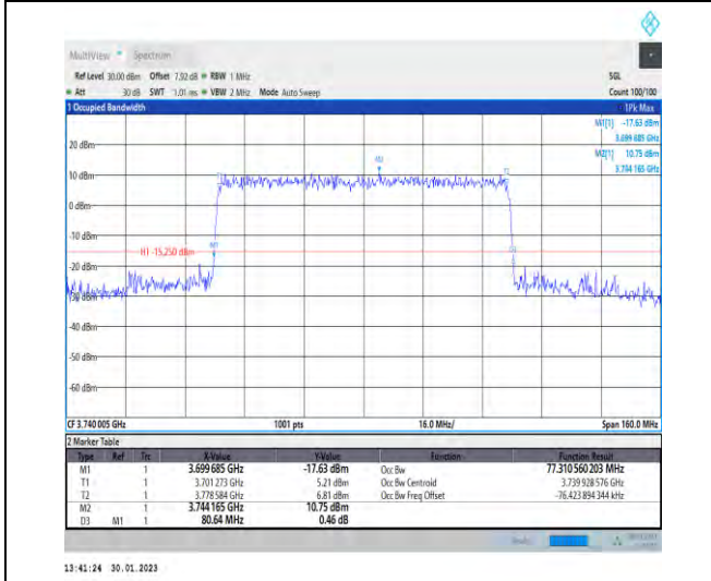
1-N78-3700-3800-30-80-L-9-CP-256QAM-Outer_Ful-l-217@0-Ant1-77.311-80.640-≤80-PASS
