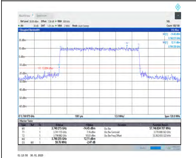
1-N78-3700-3800-30-60-H-6-CP-QPSK-Outer_Full-162@0-Ant1-57.747-59.760-≤60-PASS
