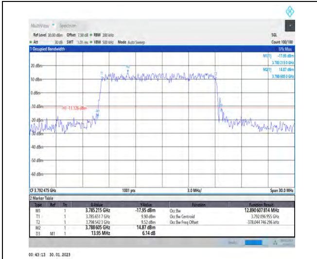
1-N78-3700-3800-30-15-H-4-DFT-64QAM-Outer_Full-36@0-Ant1-12.891-13.950-≤15-PASS
