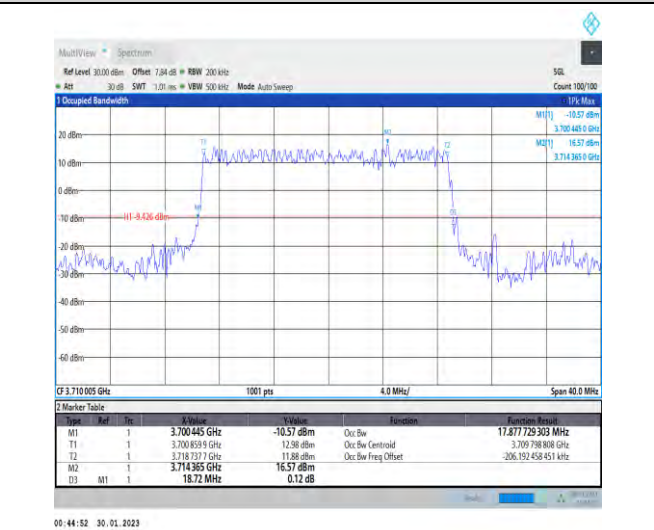
1-N78-3700-3800-30-20-L-2-DFT-PI2BPSK-Outer_Full-50@0-Ant1-17.878-18.720-≤20-PASS
