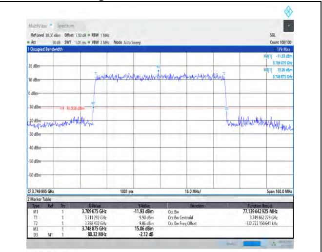
1-N78-3700-3800-30-80-M-3-DFT-16QAM-Outer_Full-216@0-Ant1-77.14-80.320-≤80-PASS
