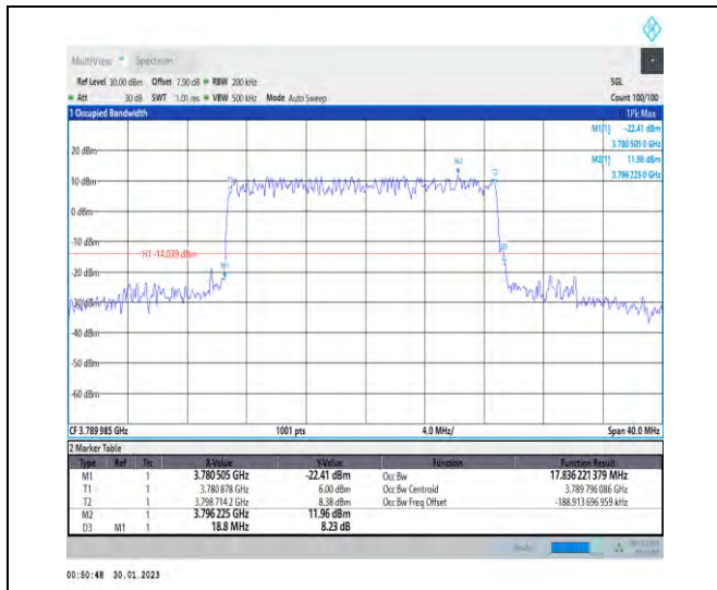
1-N78-3700-3800-30-20-H-5-DFT-256QAM-Outer_Full-50@0-Ant1-17.836-18.800-≤20-PASS
