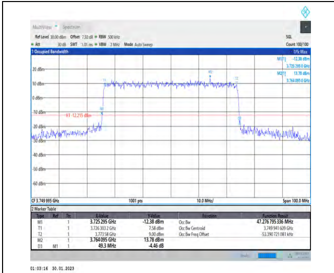
1-N78-3700-3800-30-50-M-8-CP-64QAM-Outer_Full -133@0-Ant1-47.277-49.300-≤50-PASS
