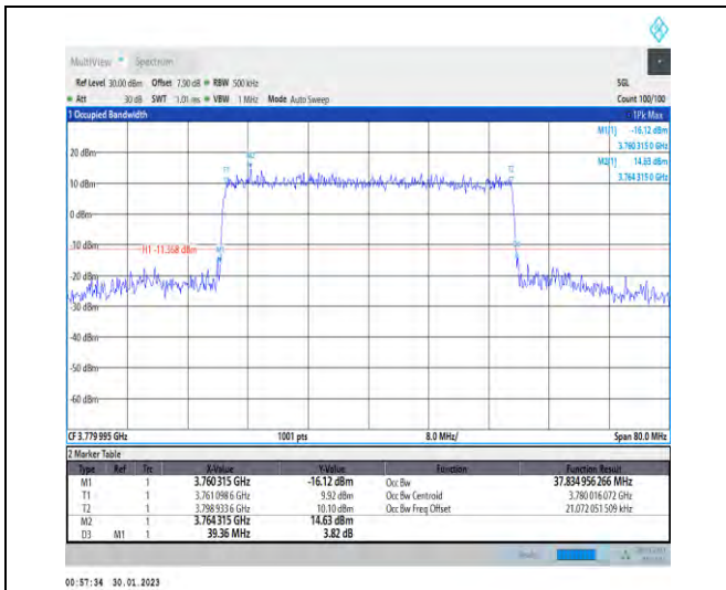
1-N78-3700-3800-30-40-H-6-CP-QPSK-Outer_Full-106@0-Ant1-37.835-39.360-≤40-PASS
