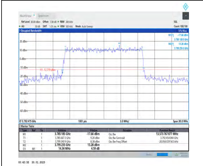
1-N78-3700-3800-30-15-H-6-CP-QPSK-Outer_Full-38@0-Ant1-13.574-14.340-≤15-PASS
