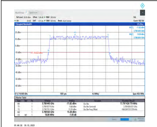
1-N78-3700-3800-30-20-L-1-DFT-QPSK-Outer_Full-50@0-Ant1-17.797-18.840-≤20-PASS
