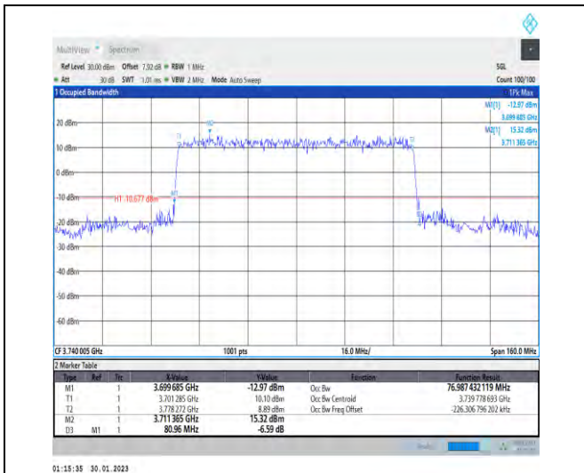
1-N78-3700-3800-30-80-L-3-DFT-16QAM-Outer_Full -216@0-Ant1-76.987-80.960-≤80-PASS
