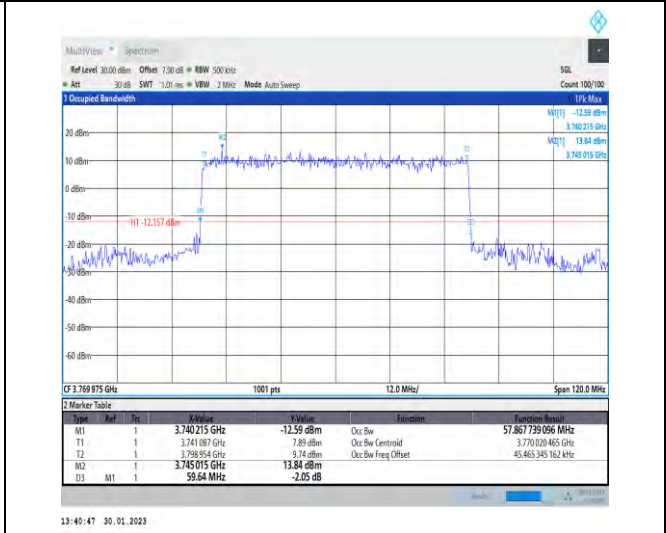
1-N78-3700-3800-30-60-H-3-DFT-16QAM-Outer_Full-162@0-Ant1-57.868-59.640-≤60-PASS
