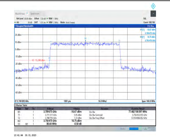
1-N78-3700-3800-30-80-M-9-CP-256QAM-Outer_Full-217@0-Ant1-77.482-80.640-≤80-PASS
