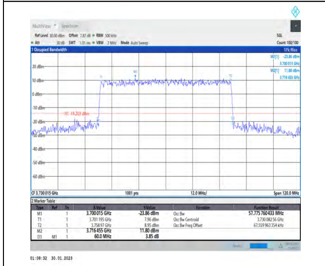
1-N78-3700-3800-30-60-L-8-CP-64QAM-Outer_Full-162@0-Ant1-57.776-60.000-≤60-PASS
