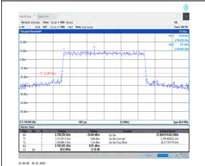
1-N78-3700-3800-30-40-M-9-CP-256QAM-Outer_Fu II-106@0-Ant1-37.835-39.600-≤40-PASS
