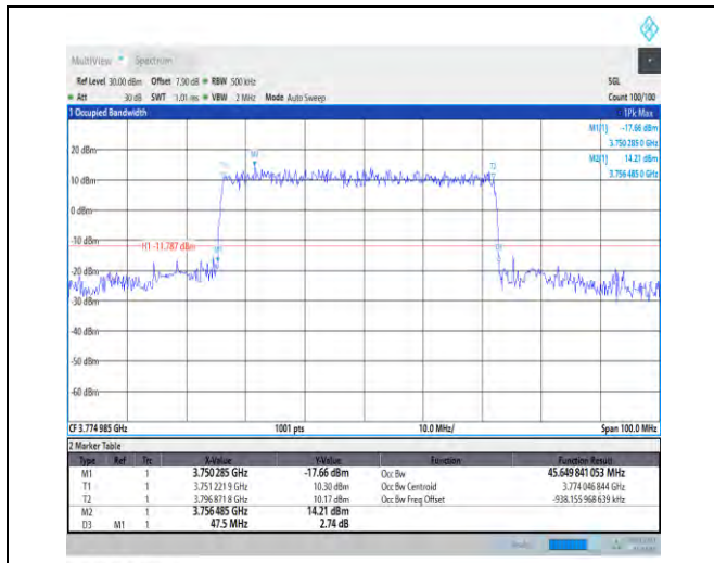
1-N78-3700-3800-30-50-H-3-DFT-16QAM-Outer_Full-128@0-Ant1-45.65-47.500-≤50-PASS
