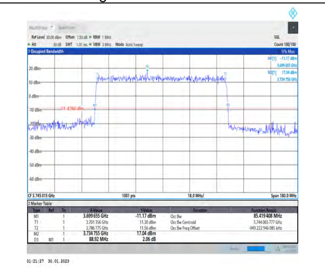
1-N78-3700-3800-30-90-L-1-DFT-QPSK-Outer_Full-240@0-Ant1-85.419-88.920-≤90-PASS
