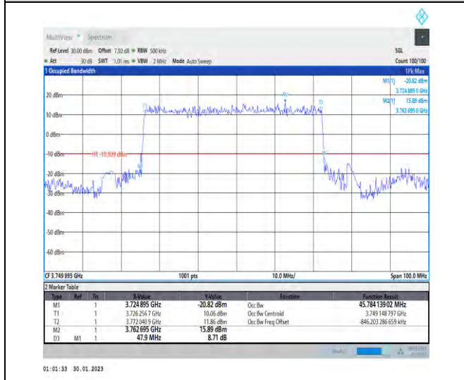
1-N78-3700-3800-30-50-M-2-DFT-16QAM-Outer_Ful- Full-128@0-Ant1-45.784-47.900-≤50-PASS
