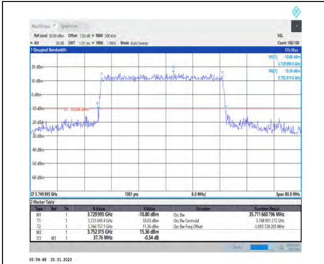
1-N78-3700-3800-30-40-M-3-DFT-16QAM-Outer_Fu II-100@0-Ant1-35.712-37.760-≤40-PASS
