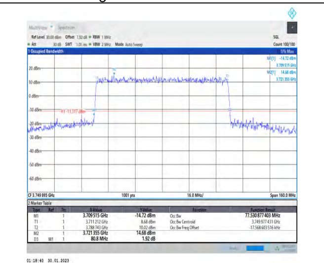
1-N78-3700-3800-30-80-M-7-CP-16QAM-Outer_Full-217@0-Ant1-77.531-80.800-≤80-PASS
