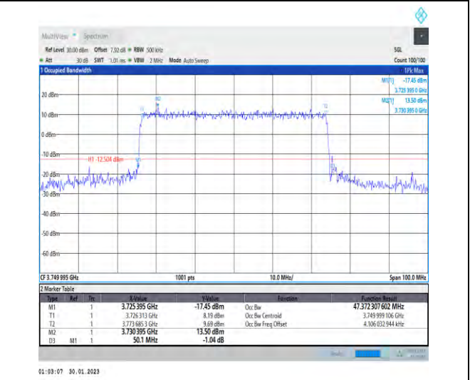
1-N78-3700-3800-30-50-M-7-CP-16QAM-Outer_Full-133@0-Ant1-47.372-50.100-≤50-PASS
