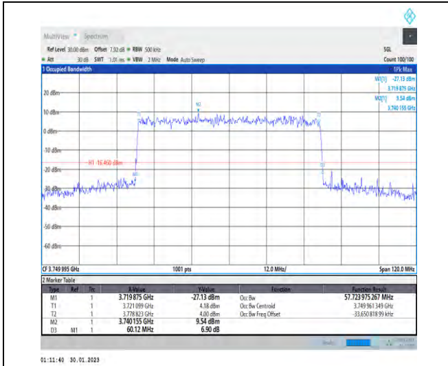
1-N78-3700-3800-30-60-M-9-CP-256QAM-Outer_Fu II-162@0-Ant1-57.724-60.120-≤60-PASS
