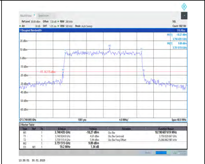
1-N78-3700-3800-30-20-M-9-CP-256QAM-Outer_Full-51@0-Ant1-18.191-19.200-≤20-PASS
