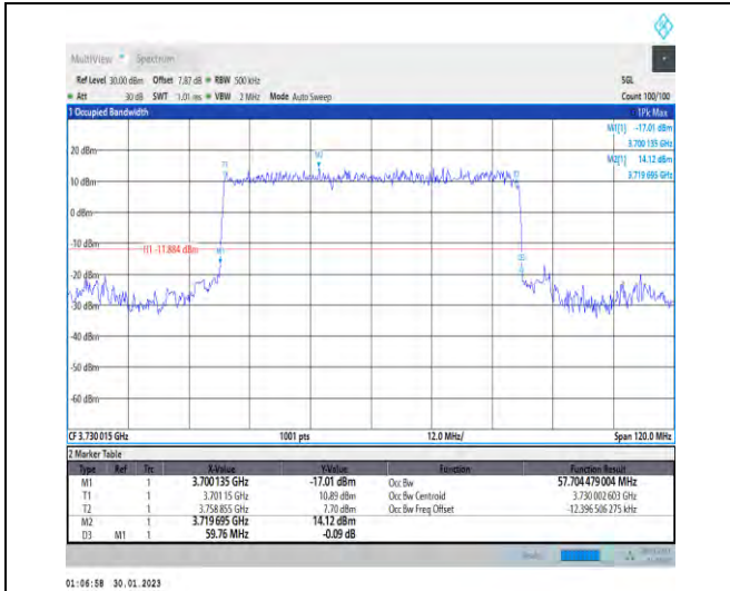
1-N78-3700-3800-30-60-L-2-DFT-PI2BPSK-Outer_Full-162@0-Ant1-57.704-59.760-≤60-PASS
