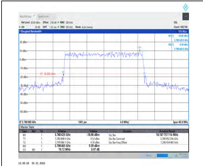
1-N78-3700-3800-30-20-H-9-CP-256QAM-Outer_Full-I51@0-Ant1-18.188-19.120-<=20-PASS
