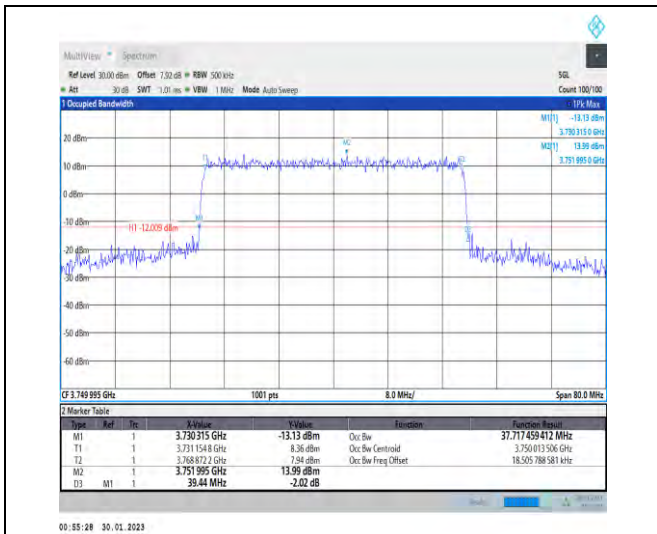
1-N78-3700-3800-30-40-M-7-CP-16QAM-Outer_Full -106@0-Ant1-37.717-39.440-≤40-PASS
