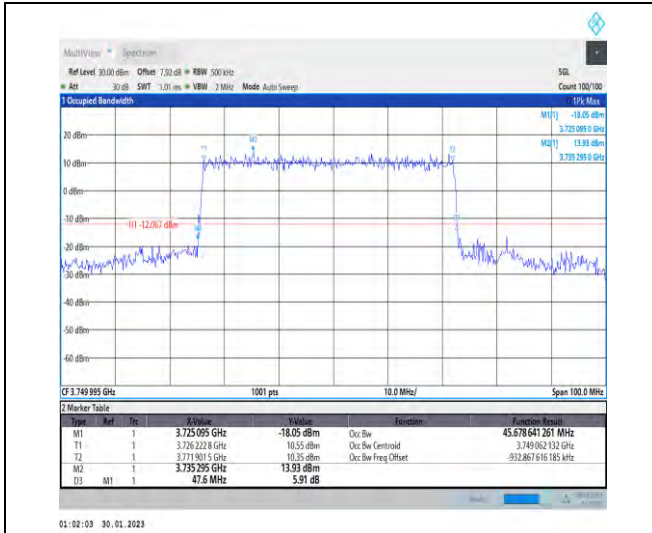
1-N78-3700-3800-30-50-M-4-DFT-64QAM-Outer_Fu II-128@0-Ant1-45.679-47.600-≤50-PASS
