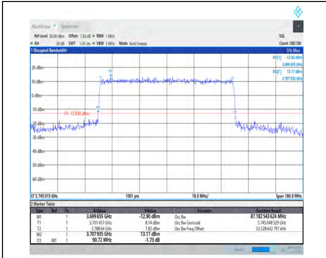
1-N78-3700-3800-30-90-L-8-CP-64QAM-Outer_Full-245@0-Ant1-87.183-90.720-≤90-PASS
