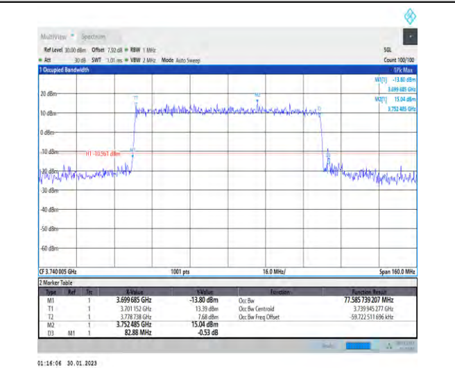
1-N78-3700-3800-30-80-L-6-CP-QPSK-Outer_Full-2 17@0-Ant1-77.586-82.880-≤80-PASS
