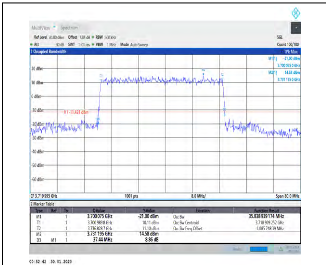
1-N78-3700-3800-30-40-L-4-DFT-64QAM-Outer_Full -100@0-Ant1-35.839-37.440-≤40-PASS
