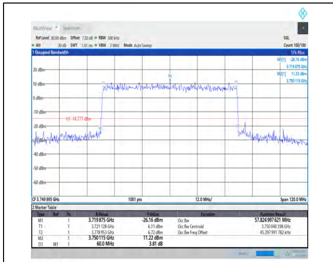
1-N78-3700-3800-30-60-M-5-DFT-256QAM-Outer_Full-162@0-Ant1-57.825-60.000-≤60-PASS
