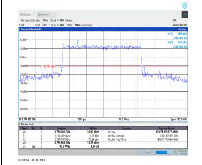
1-N78-3700-3800-30-50-H-1-DFT-QPSK-Outer_Full 128@0-Ant1-45.672-47.600-≤50-PASS
