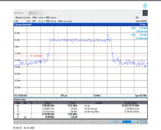
1-N78-3700-3800-30-20-L-6-CP-QPSK-Outer_Full-5 1@0-Ant1-18.209-19.480-≤20-PASS
