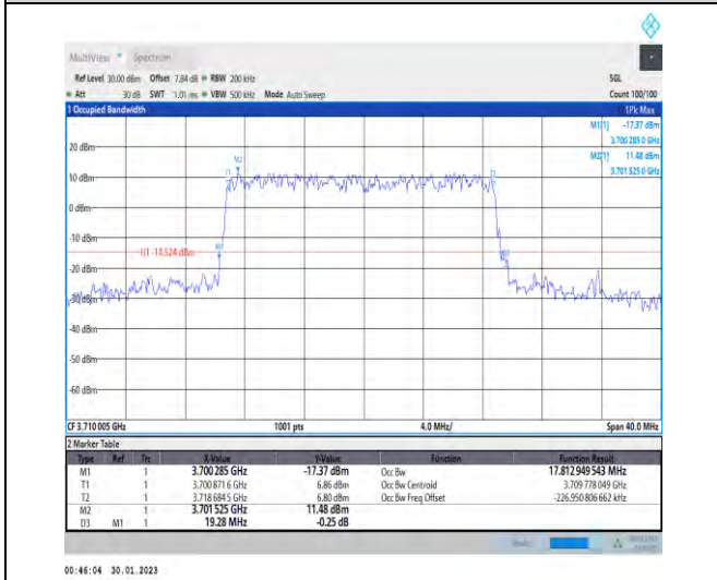
1-N78-3700-3800-30-20-L-5-DFT-256QAM-Outer_Full -50@0-Ant1-17.813-19.280-≤20-PASS
