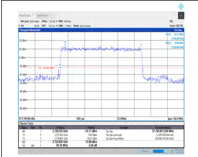
1-N78-3700-3800-30-60-M-3-DFT-16QAM-Outer_Full-162@0-Ant1-57.766-59.760-≤60-PASS
