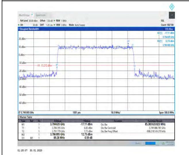
1-N78-3700-3800-30-90-M-5-DFT-256QAM-Outer_F ull-240@0-Ant1-85.384-89.280-≤90-PASS
