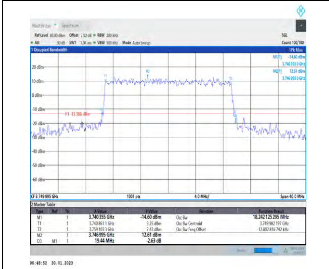
1-N78-3700-3800-30-20-M-8-CP-64QAM-Outer_Full-51@0-Ant1-18.242-19.440-≤20-PASS
