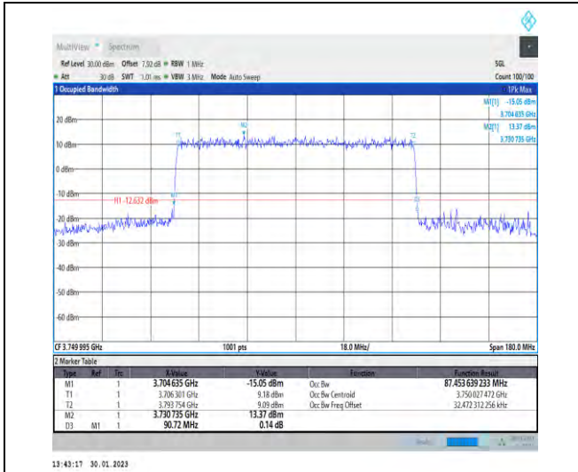
1-N78-3700-3800-30-90-M-7-CP-16QAM-Outer_Full -245@0-Ant1-87.454-90.720-≤90-PASS
