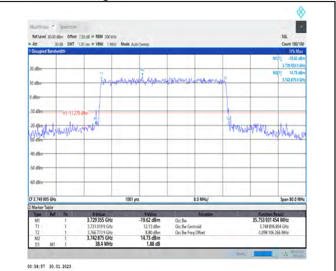
1-N78-3700-3800-30-40-M-4-DFT-64QAM-Outer_Ful I-100@0-Ant1-35.754-38.400-≤40-PASS
