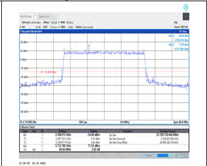
1-N78-3700-3800-30-40-L-9-CP-256QAM-Outer_Full-106@0-Ant1-37.793-39.360-≤40-PASS
