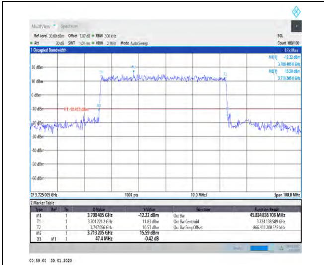
1-N78-3700-3800-30-50-L-1-DFT-QPSK-Outer_Full-128@0-Ant1-45.835-47.400-≤50-PASS
