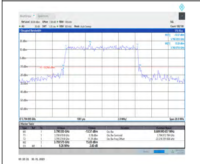
1-N78-3700-3800-30-10-H-1-DFT-QPSK-Outer_Full- 24@0-Ant1-8.604-9.260-≤10-PASS
