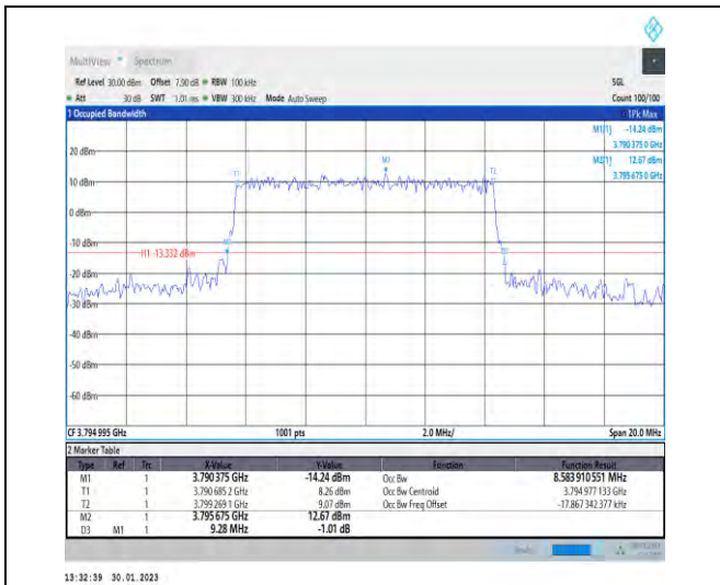
1-N78-3700-3800-30-10-H-7-CP-16QAM-Outer_Full-24@0-Ant1-8.584-9.280-≤10-PASS
