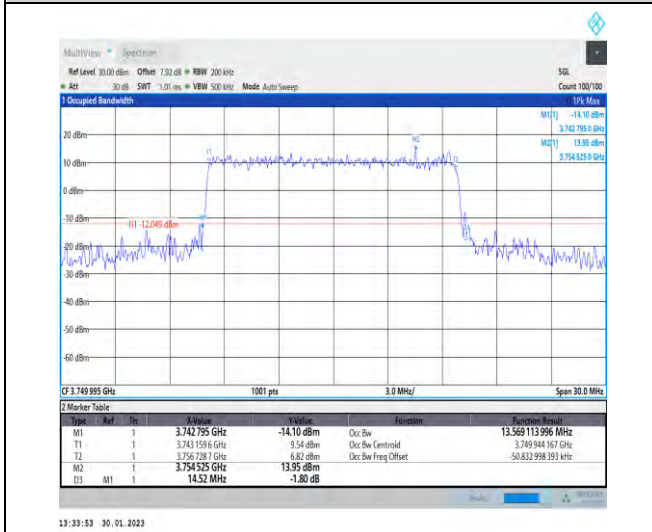
1-N78-3700-3800-30-15-M-7-CP-16QAM-Outer_Full-38@0-Ant1-13.569-14.520-≤15-PASS
