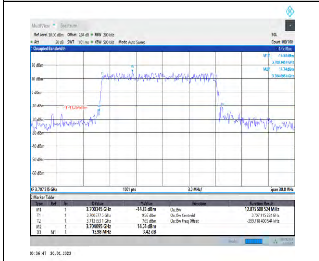
1-N78-3700-3800-30-15-L-4-DFT-64QAM-Outer_Full-36@0-Ant1-12.876-13.980-≤15-PASS
