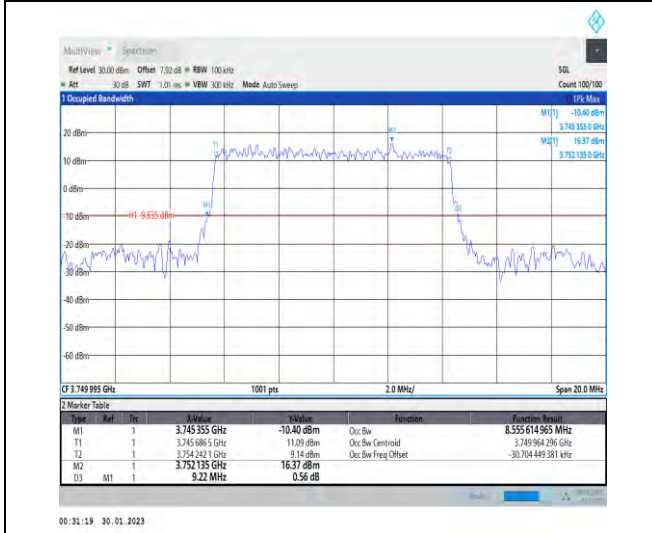
1-N78-3700-3800-30-10-M-2-DFT-16QAM-Outer_Full I-24@0-Ant1-8.556-9.220-≤10-PASS
