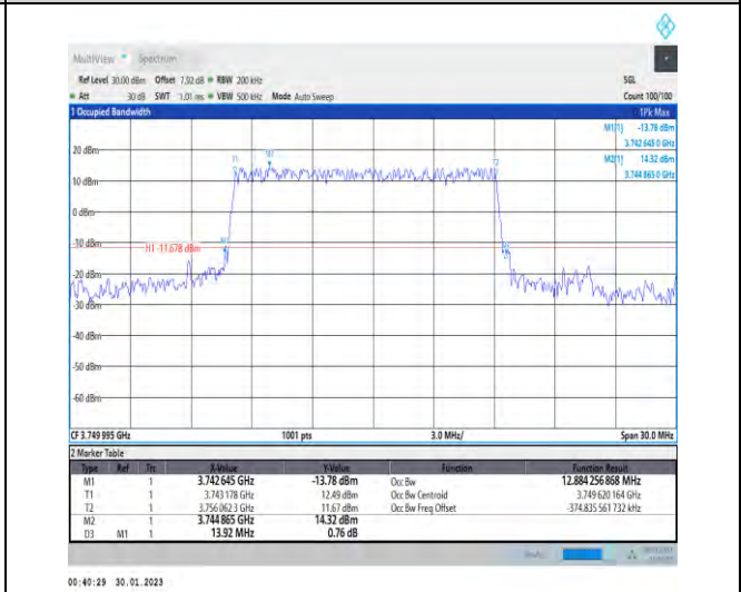
1-N78-3700-3800-30-15-M-4-DFT-64QAM-Outer_Full-36@0-Ant1-12.884-13.920-≤15-PASS
