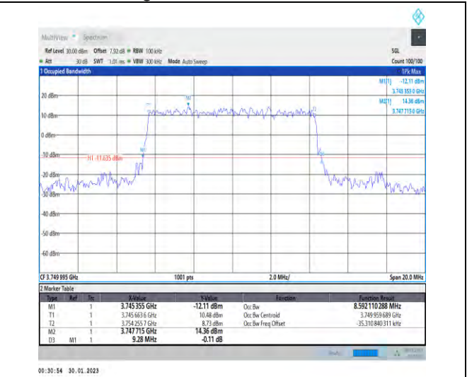
1-N78-3700-3800-30-10-M-1-DFT-QPSK-Outer_Full I-24@0-Ant1-8.592-9.280-≤10-PASS
