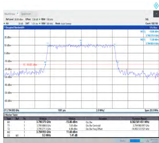
1-N78-3700-3800-30-10-H-4-DFT-64QAM-Outer_Ful I-24@0-Ant1-8.604-9.420-≤10-PASS
