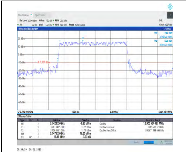
1-N78-3700-3800-30-15-M-1-DFT-QPSK-Outer_Full-36@0-Ant1-12.906-13.830-≤15-PASS
