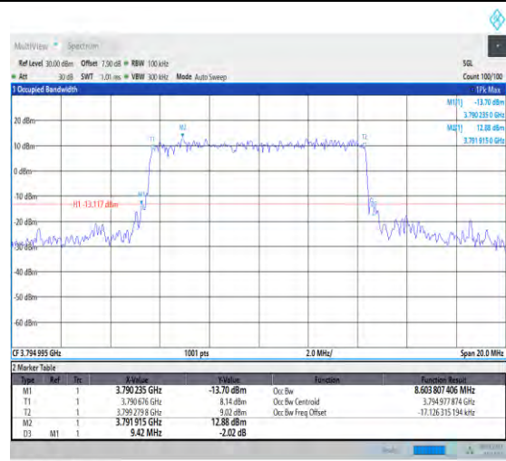
1-N78-3700-3800-30-10-H-4-DFT-64QAM-Outer_Ful I-24@0-Ant1-8.604-9.420-≤10-PASS
