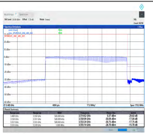
1-N78-3450-3550-30-100-H-3-DFT-PI2BPSK-Outer_Full-270@0-Ant1-1--PASS-see graph
