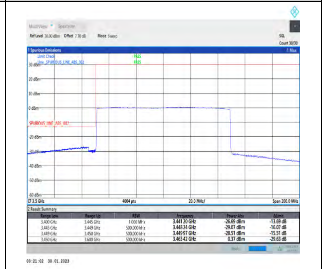
1-N78-3450-3550-30-100-L-6-CP-QPSK-Outer_Full-273@0-Ant1-1--PASS-see graph
