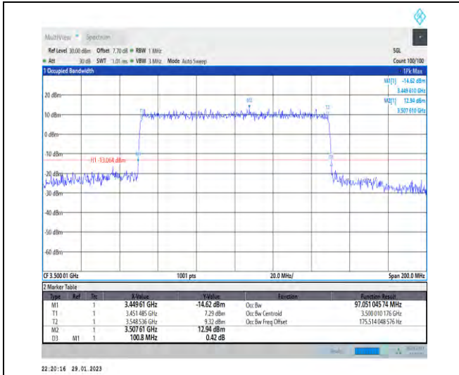
1-N78-3450-3550-30-100-M-8-CP-64QAM-Outer_Fu II-273@0-Ant1-97.051-100.800-≤100-PASS
