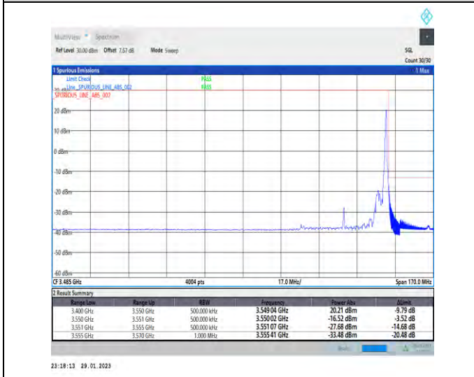
1-N78-3450-3550-30-40-H-5-CP-QPSK-Edge_1RB_Right-1@105-Ant1-1--PASS-see graph
