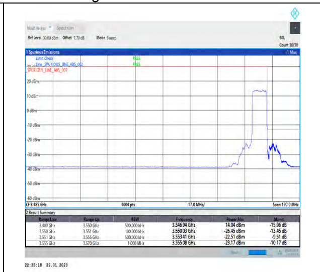
1-N78-3450-3550-30-10-H-3-DFT-PI2BPSK-Outer_Full-24@0-Ant1-1--PASS-see graph
