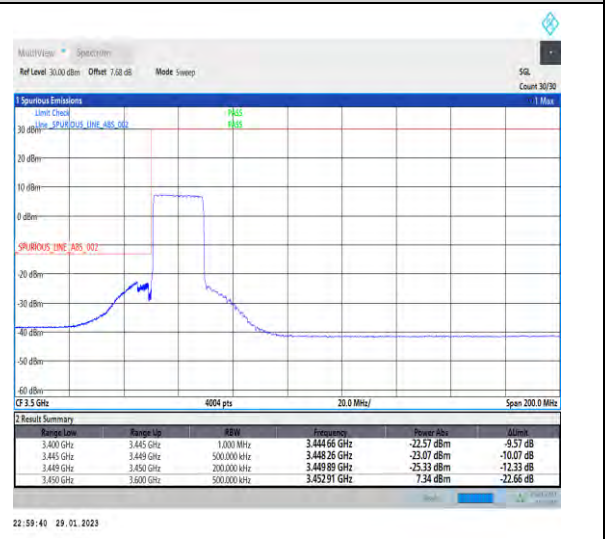
1-N78-3450-3550-30-20-L-6-CP-QPSK-Outer_Full -51@0-Ant1-1--PASS-see graph
