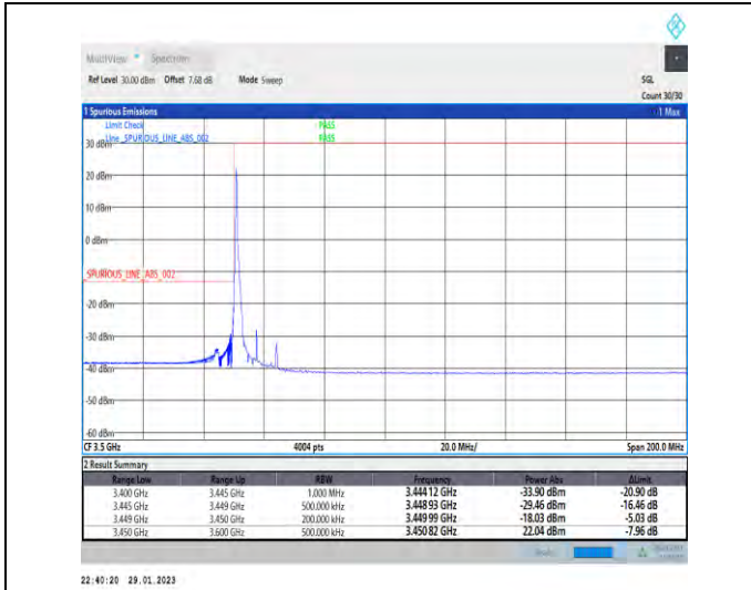
1-N78-3450-3550-30-15-L-1-DFT-PI2BPSK-Edge_1RB_Left-1@0-Ant1-1--PASS-see graph
