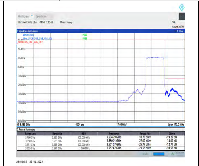
1-N78-3450-3550-30-20-H-3-DFT-PI2BPSK-Outer_Full-50@0-Ant1-1--PASS-see graph
