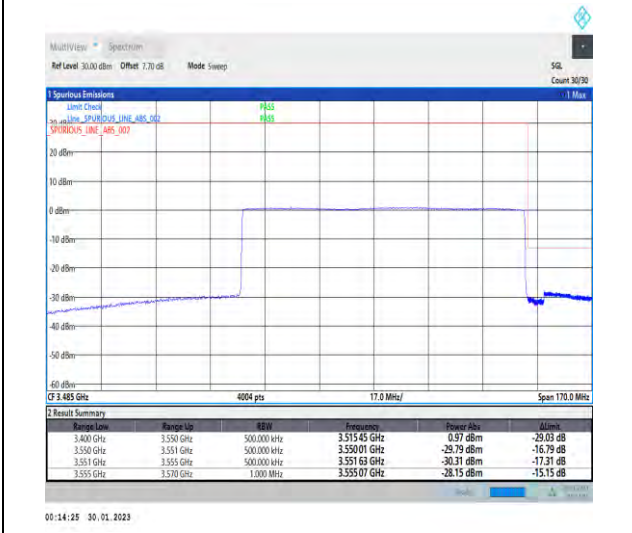
1-N78-3450-3550-30-90-H-6-CP-QPSK-Outer_Full-245@0-Ant1-1--PASS-see graph
