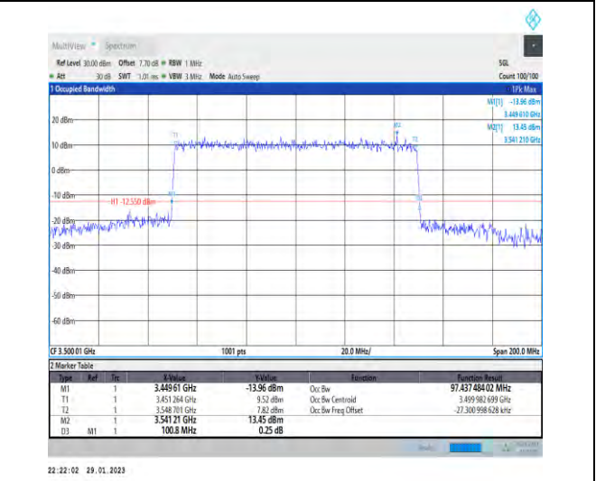
1-N78-3450-3550-30-100-H-6-CP-QPSK-Outer_Full-273@0-Ant1-97.437-100.800-≤100-PASS
