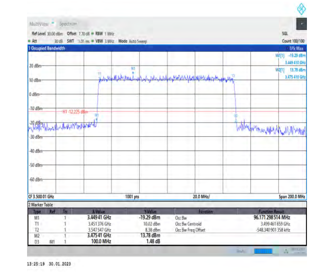
1-N78-3450-3550-30-100-M-3-DFT-16QAM-Outer_Full-270@0-Ant1-96.171-100.000-≤100-PASS
