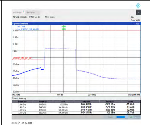
1-N78-3450-3550-30-50-L-6-CP-QPSK-Outer_Full -133@0-Ant1-1--PASS-see graph
