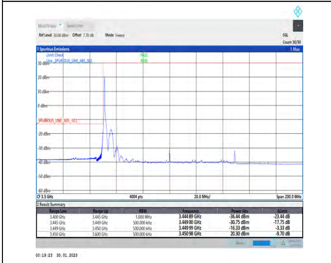
1-N78-3450-3550-30-100-L-4-CP-QPSK-Edge_1RB_Left-1@0-Ant1-1--PASS-see graph
