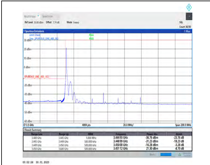
1-N78-3450-3550-30-90-L-1-DFT-PI2BPSK-Edge_1RB _Left-1@0-Ant1-1--PASS-see graph
