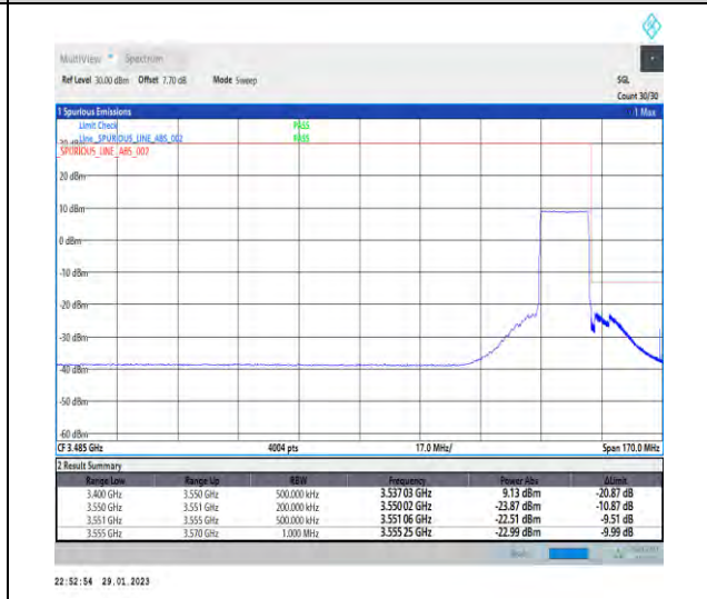
1-N78-3450-3550-30-15-H-6-CP-QPSK-Outer_Full-38@0-Ant1-1--PASS-see graph
