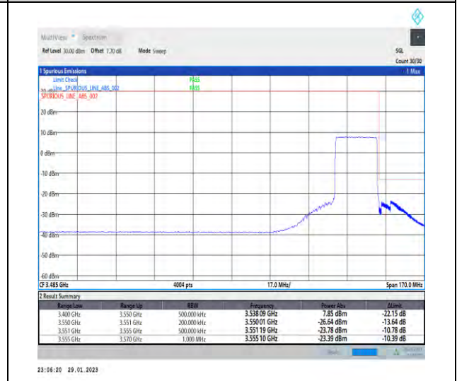
1-N78-3450-3550-30-20-H-6-CP-QPSK-Outer_Full-51@0-Ant1-1--PASS-see graph
