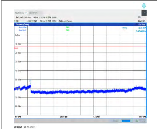
1-N78-3450-3550-30-100-H-1-DFT-PI2BPSK-Inner_1RB_Left-1@1-6000-18000-Ant1-7465.44--55.03--1 3-PASS
