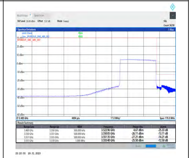
1-N78-3450-3550-30-40-H-6-CP-QPSK-Outer_Full-106@0-Ant1-1--PASS-see graph
