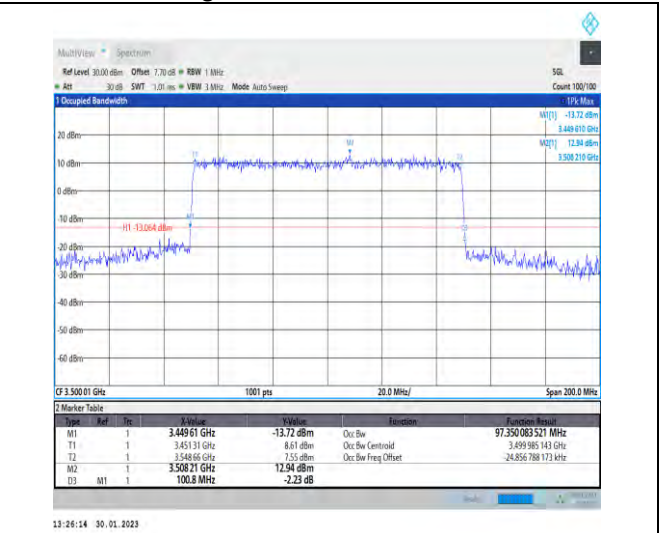
1-N78-3450-3550-30-100-H-8-CP-64QAM-Outer_Ful I-273@0-Ant1-97.35-100.800-≤100-PASS
