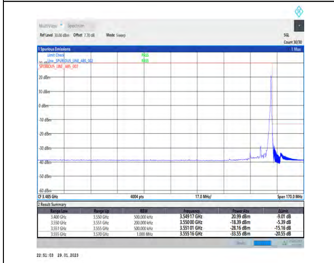
1-N78-3450-3550-30-15-H-5-CP-QPSK-Edge_1RB_Right-1@37-Ant1-1--PASS-see graph
