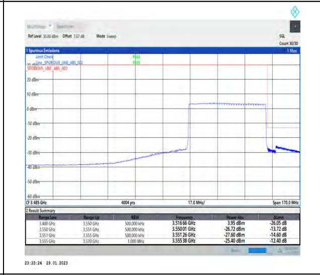
1-N78-3450-3550-30-50-H-6-CP-QPSK-Outer_Full-133@0-Ant1-1--PASS-see graph
