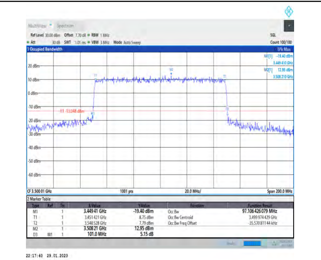
1-N78-3450-3550-30-100-L-8-CP-64QAM-Outer_Full-273@0-Ant1-97.106-101.000-≤100-PASS
