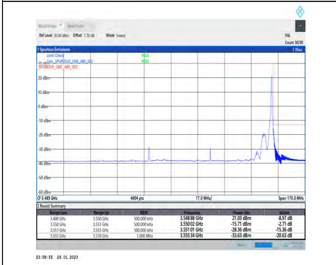
1-N78-3450-3550-30-80-H-5-CP-QPSK-Edge_1RB_Right-1@216-Ant1-1--PASS-see graph
