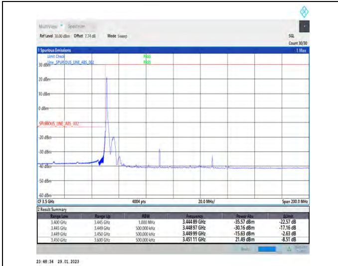
1-N78-3450-3550-30-80-L-1-DFT-PI2BPSK-Edge_1RB_Left-1@0-Ant1-1--PASS-see graph
