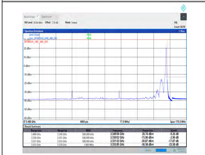
1-N78-3450-3550-30-100-H-2-DFT-PI2BPSK-Edge_1R_B_Right-1@272-Ant1-1--PASS-see graph
