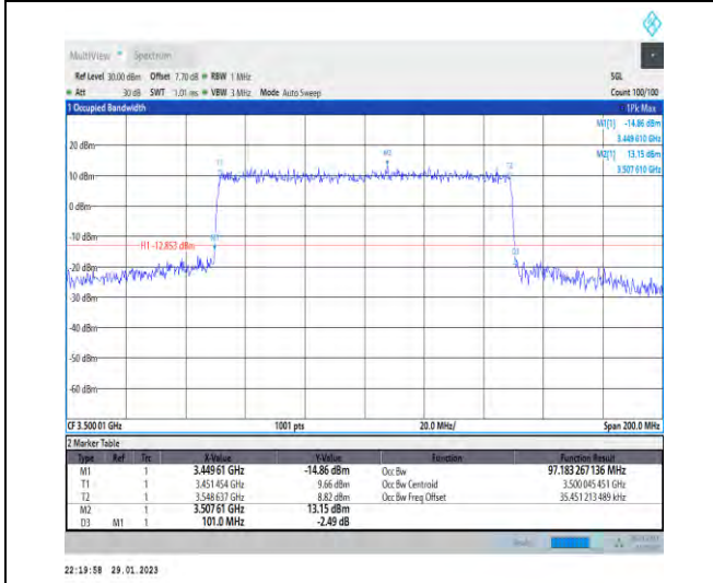
1-N78-3450-3550-30-100-M-6-CP-QPSK-Outer_Full-273@0-Ant1-97.183-101.000-≤100-PASS
