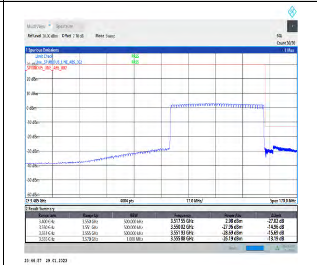
1-N78-3450-3550-30-60-H-6-CP-QPSK-Outer_Full-162@0-Ant1-1--PASS-see graph
