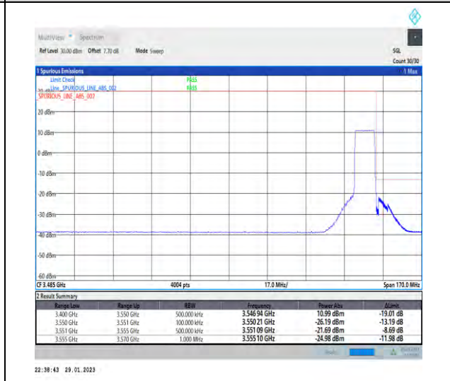
1-N78-3450-3550-30-10-H-6-CP-QPSK-Outer_Full-24@0-Ant1-1--PASS-see graph
