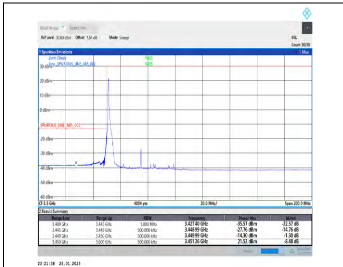
1-N78-3450-3550-30-50-L-1-DFT-PI2BPSK-Edge_1RB _Left-1@0-Ant1-1--PASS-see graph
