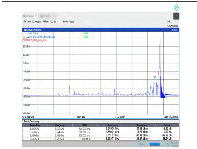
1-N78-3450-3550-30-100-H-2-DFT-PI2BPSK-Edge_1R_B_Right-1@272-Ant1-1--PASS-see graph
