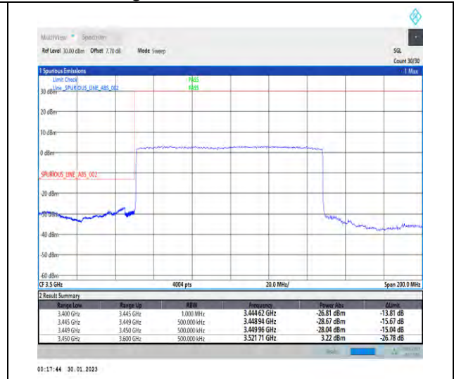
1-N78-3450-3550-30-100-L-3-DFT-PI2BPSK-Outer_Full-270@0-Ant1-1--PASS-see graph
