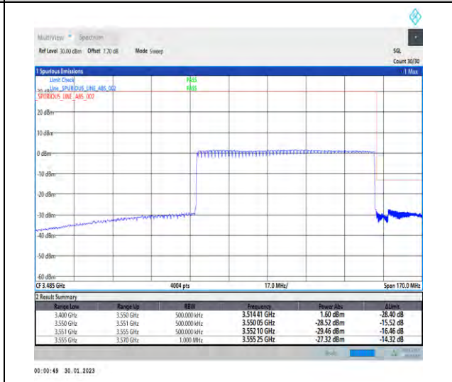
1-N78-3450-3550-30-80-H-6-CP-QPSK-Outer_Full-217@0-Ant1-1--PASS-see graph
