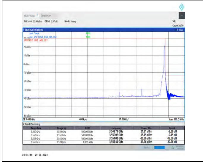
1-N78-3450-3550-30-50-H-5-CP-QPSK-Edge_1RB_Right-1@132-Ant1-1--PASS-see graph
