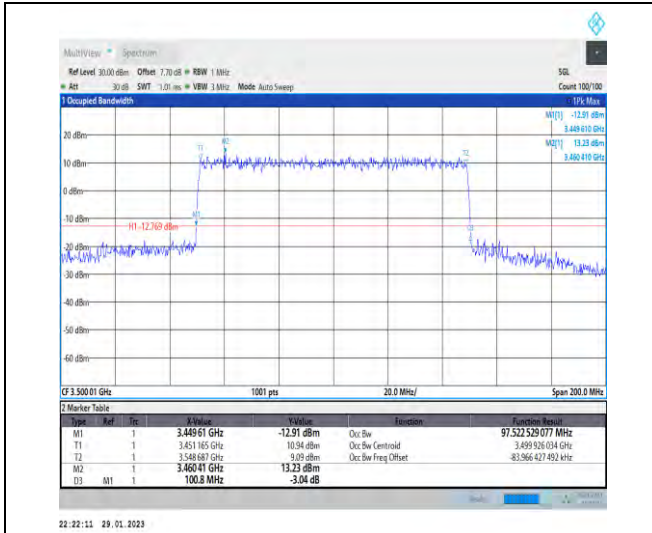
1-N78-3450-3550-30-100-H-7-CP-16QAM-Outer_Fu II-273@0-Ant1-97.523-100.800-≤100-PASS
