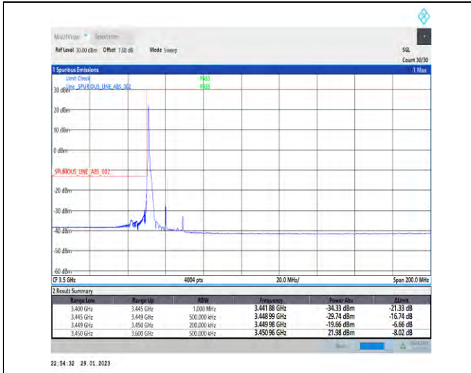
1-N78-3450-3550-30-20-L-1-DFT-PI2BPSK-Edge_1RB _Left-1@0-Ant1-1--PASS-see graph
