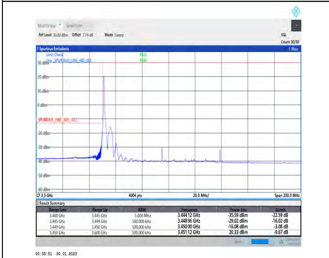
1-N78-3450-3550-30-90-L-4-CP-QPSK-Edge_1RB_Lef t-1@0-Ant1-1--PASS-see graph
