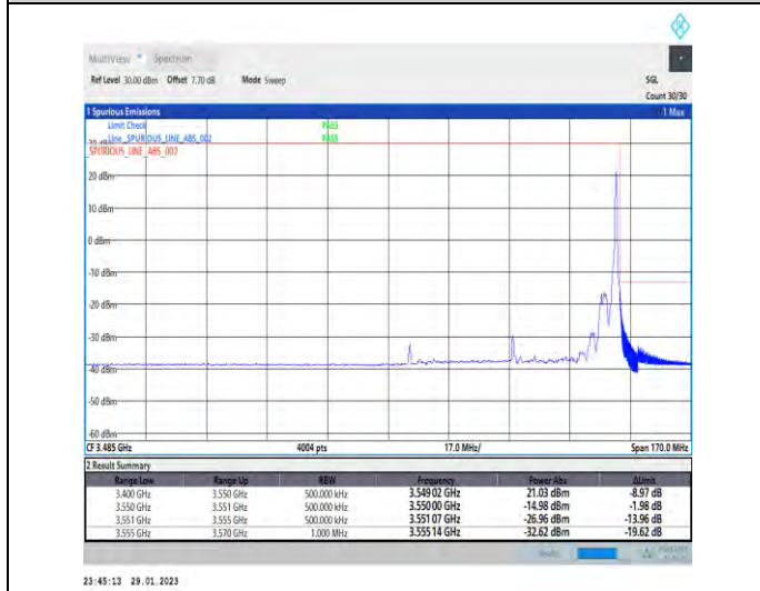
1-N78-3450-3550-30-60-H-5-CP-QPSK-Edge_1RB_Right-1@161-Ant1-1--PASS-see graph
