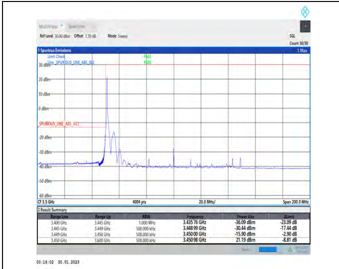
1-N78-3450-3550-30-100-L-1-DFT-PI2BPSK-Edge_1R_B_Left-1@0-Ant1-1--PASS-see graph
