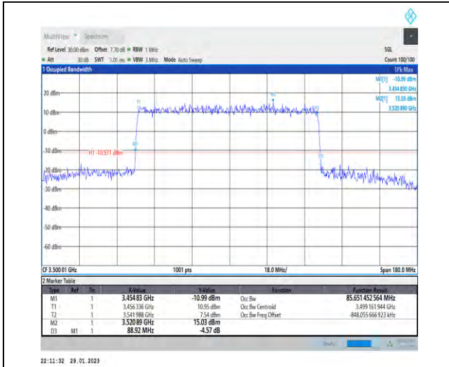
1-N78-3450-3550-30-90-M-3-DFT-16QAM-Outer_Fu II-240@0-Ant1-85.651-88.920-≤90-PASS
