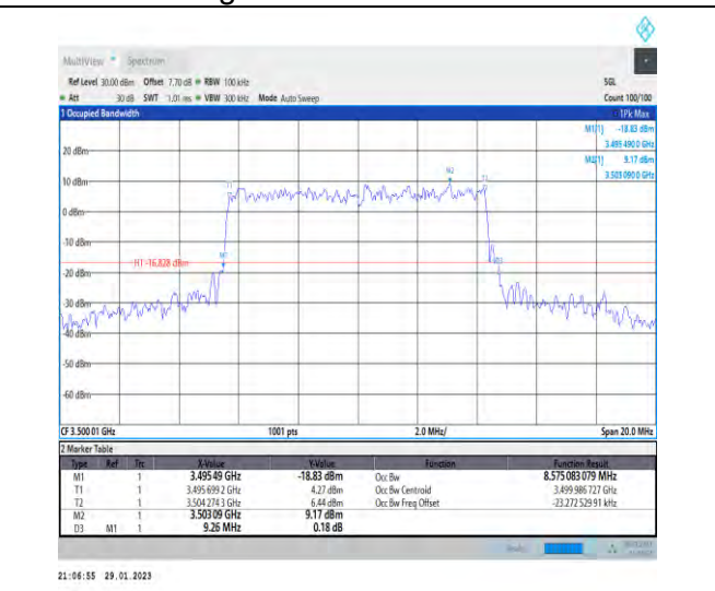
1-N78-3450-3550-30-10-M-9-CP-256QAM-Outer_Ful I-24@0-Ant1-8.575-9.260-≤10-PASS
