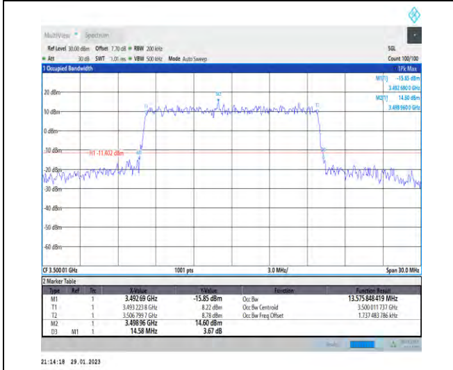
1-N78-3450-3550-30-15-M-7-CP-16QAM-Outer_Full-38@0-Ant1-13.576-14.580-≤15-PASS
