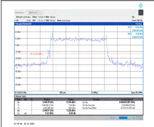
1-N78-3450-3550-30-10-H-5-DFT-256QAM-Outer_F ull-24@0-Ant1-8.607-9.220-≤10-PASS
