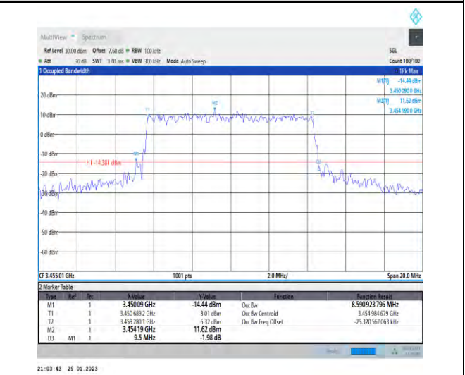
1-N78-3450-3550-30-10-L-8-CP-64QAM-Outer_Full-24@0-Ant1-8.591-9.500-≤10-PASS
