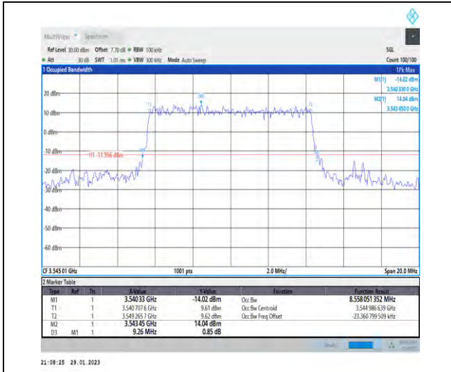
1-N78-3450-3550-30-10-H-3-DFT-16QAM-Outer_Ful I-24@0-Ant1-8.558-9.260-≤10-PASS
