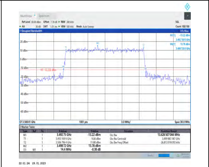
1-N78-3450-3550-30-15-M-8-CP-64QAM-Outer_Full-38@0-Ant1-13.627-14.400-≤15-PASS
