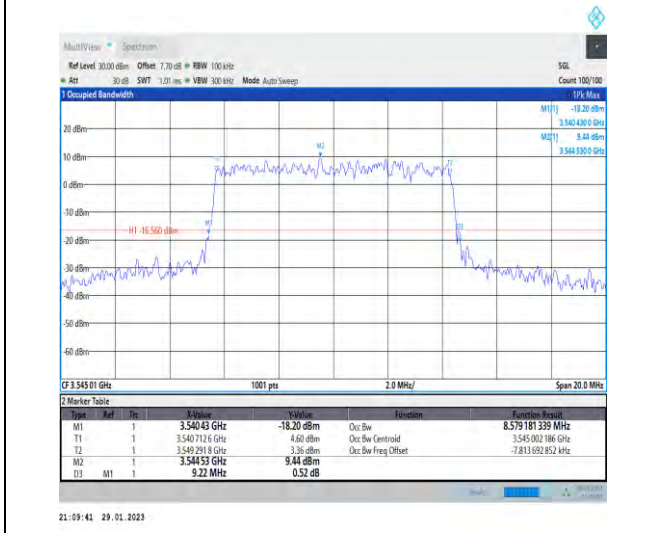
1-N78-3450-3550-30-10-H-9-CP-256QAM-Outer_Fu-ll-24@0-Ant1-8.579-9.220-≤10-PASS
