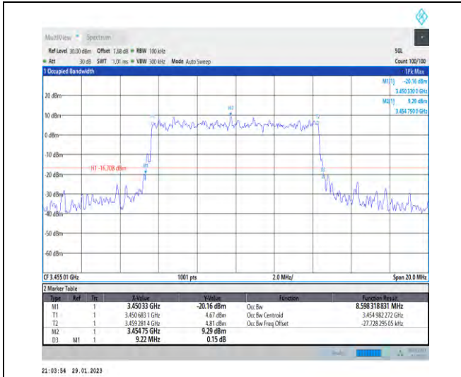
1-N78-3450-3550-30-10-L-9-CP-256QAM-Outer_Ful I-24@0-Ant1-8.598-9.220-≤10-PASS
