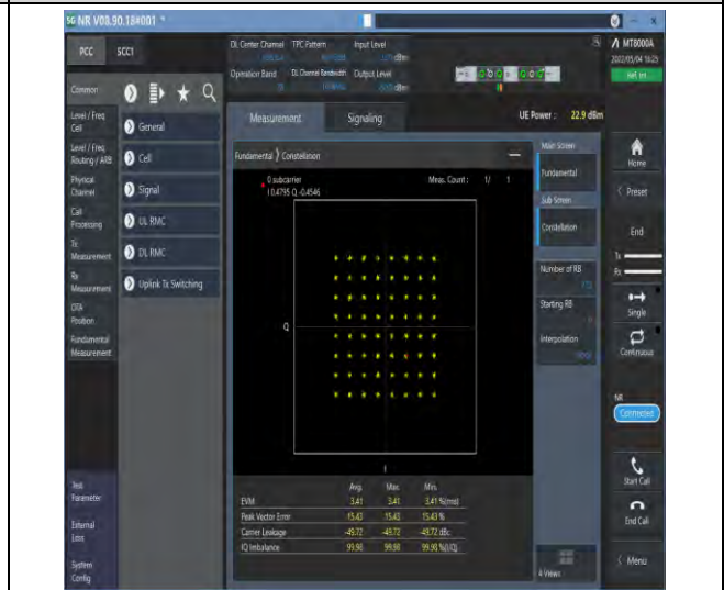
1-N78-3450-3550--30-100-M-8-CP-64QAM-Outer_F ull-273@0-Ant1-see graph-PASS
