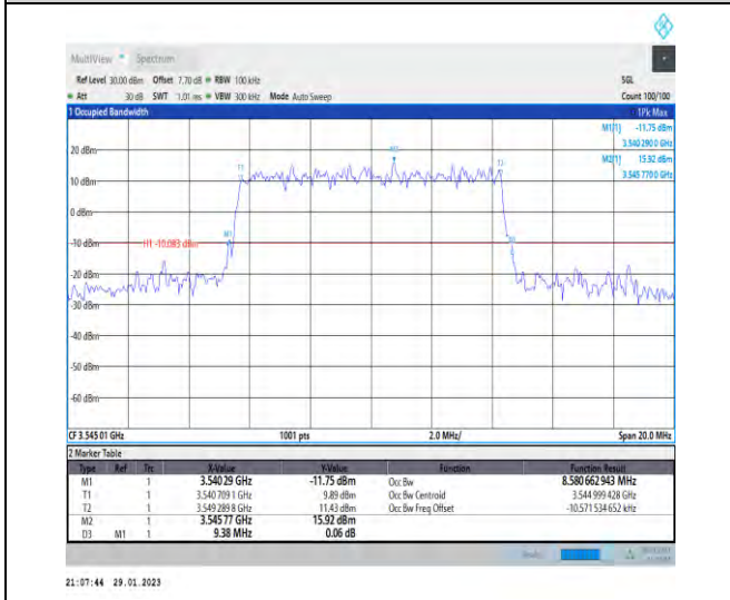
1-N78-3450-3550-30-10-H-1-DFT-QPSK-Outer_Full 24@0-Ant1-8.581-9.380-≤10-PASS
