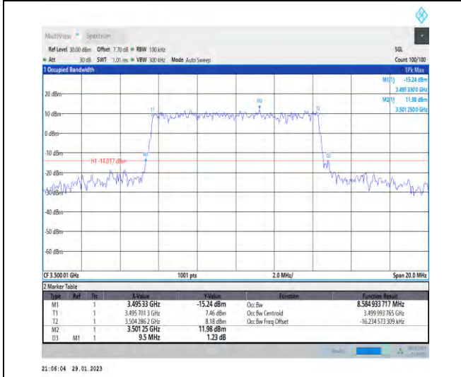
1-N78-3450-3550-30-10-M-6-CP-QPSK-Outer_Full- 24@0-Ant1-8.585-9.500-≤10-PASS
