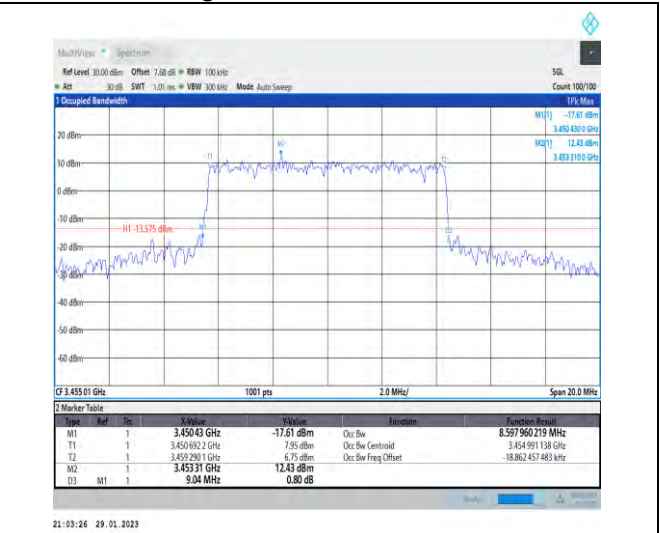
1-N78-3450-3550-30-10-L-6-CP-QPSK-Outer_Full-24@0-Ant1-8.598-9.040-≤10-PASS
