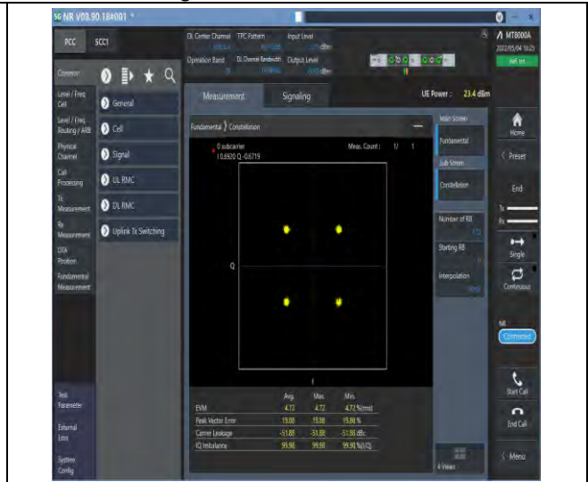
1-N78-3450-3550--30-100-M-6-CP-QPSK-Outer_Fu ll-273@0-Ant1-see graph-PASS
