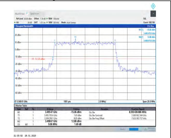
1-N78-3450-3550-30-10-M-5-DFT-256QAM-Outer_F ull-24@0-Ant1-8.593-9.060-≤10-PASS
