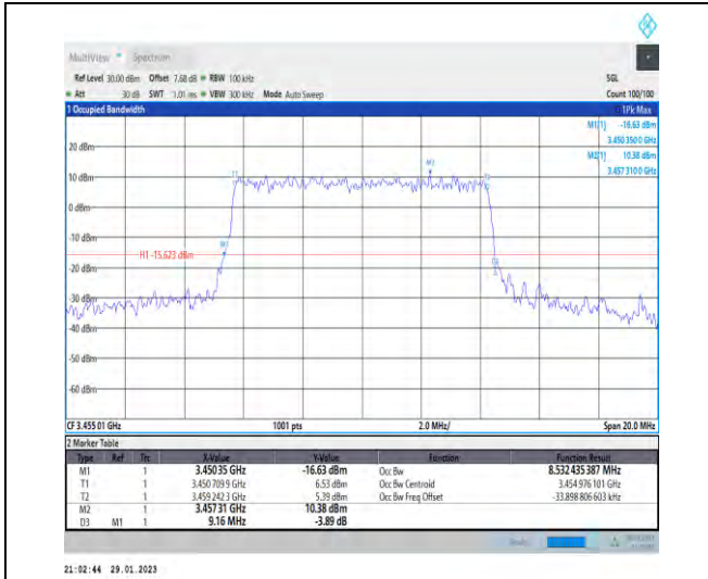
1-N78-3450-3550-30-10-L-5-DFT-256QAM-Outer_Full-24@0-Ant1-8.532-9.160-≤10-PASS
