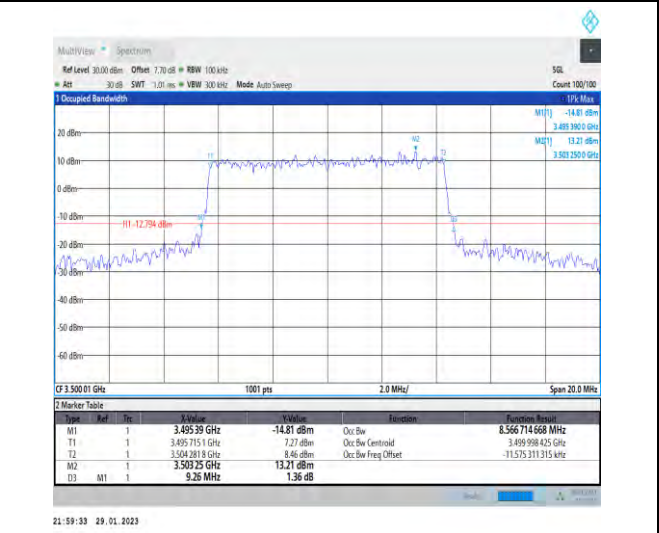
1-N78-3450-3550-30-10-M-7-CP-16QAM-Outer_Full- 24@0-Ant1-8.567-9.260-≤10-PASS
