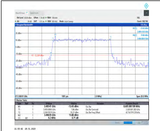
1-N78-3450-3550-30-10-M-4-DFT-64QAM-Outer_Fu ll-24@0-Ant1-8.605-9.200-≤10-PASS
