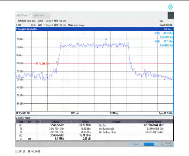
1-N78-3450-3550-30-10-H-2-DFT-PI2BPSK-Outer_F ull-24@0-Ant1-8.578-9.400-≤10-PASS
