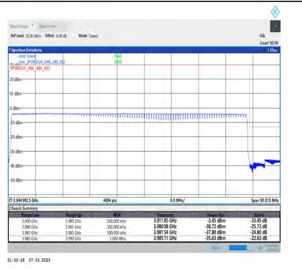
1-N77-3700-3980-PC3-30-80-H-6-CP-QPSK-Outer_Full-217@0-Ant1-1--PASS-see graph
