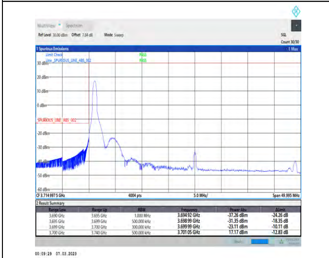
1-N77-3700-3980-PC3-30-40-L-4-CP-QPSK-Edge_1RB_Left-1@0-Ant1-1--PASS-see graph
