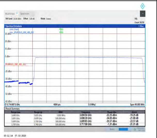
1-N77-3700-3980-PC3-30-40-L-6-CP-QPSK-Outer_Full-106@0-Ant1-1--PASS-see graph
