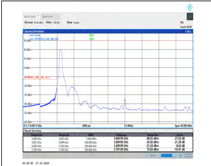
1-N77-3700-3980-PC3-30-40-L-1-DFT-PI2BPSK-Edge_1RB_Left-1@0-Ant1-1--PASS-see graph
