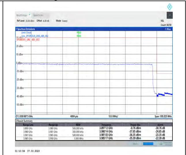
1-N77-3700-3980-PC3-30-90-H-3-DFT-PI2BPSK-Outer_Full-240@0-Ant1-1--PASS-see graph
