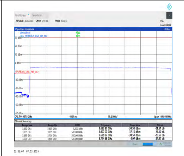
1-N77-3700-3980-PC3-30-100-L-6-CP-QPSK-Outer_Full-273@0-Ant1-1--PASS-see graph
