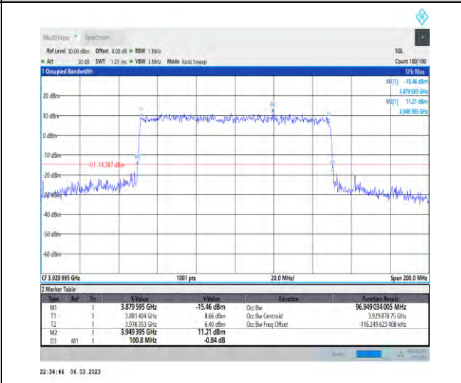
1-N77-3700-3980-PC3-30-100-H-6-CP-QPSK-Outer_Full-273@0-Ant1-96.949-100.800-≤100-PASS
