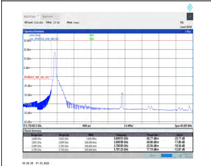
1-N77-3700-3980-PC3-30-50-L-4-CP-QPSK-Edge_1RB_Left-1@0-Ant1-1--PASS-see graph
