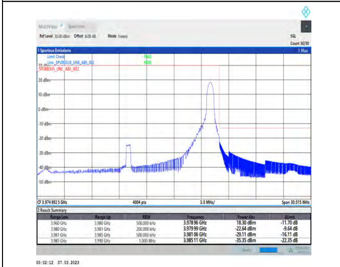
1-N77-3700-3980-PC3-30-20-H-5-CP-QPSK-Edge_1RB_Right-1@50-Ant1-1--PASS-see graph
