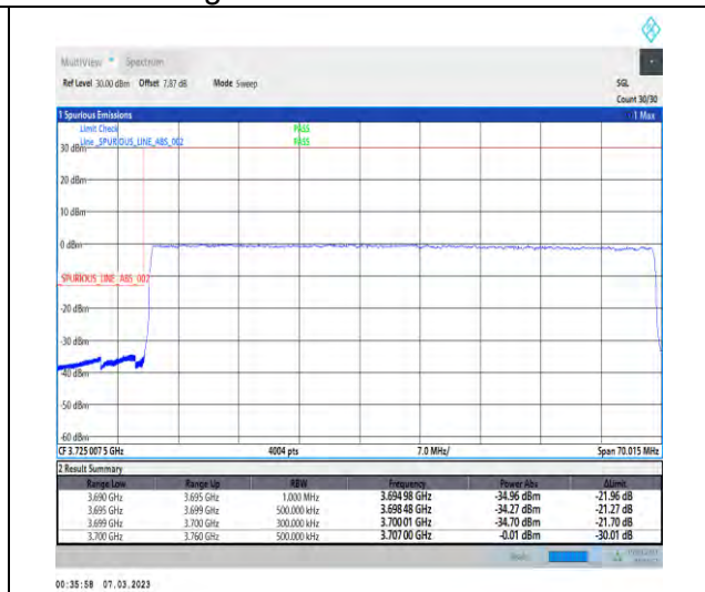
1-N77-3700-3980-PC3-30-60-L-3-DFT-PI2BPSK-Outer_Full-162@0-Ant1-1--PASS-see graph
