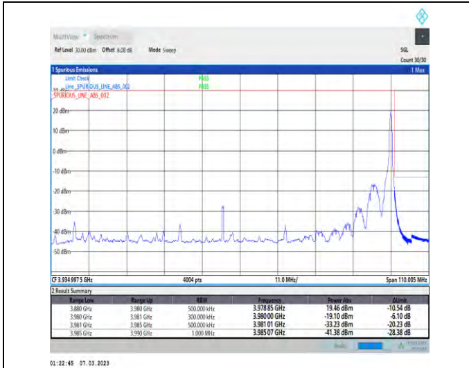
1-N77-3700-3980-PC3-30-100-H-2-DFT-PI2BPSK-Edge_1_RB_Right-1@272-Ant1-1--PASS-see graph
