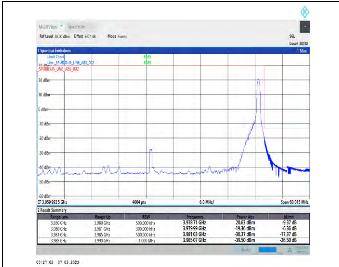
1-N77-3700-3980-PC3-30-50-H-2-DFT-PI2BPSK-Edge_1RB_Right-1@132-Ant1-1--PASS-see graph
