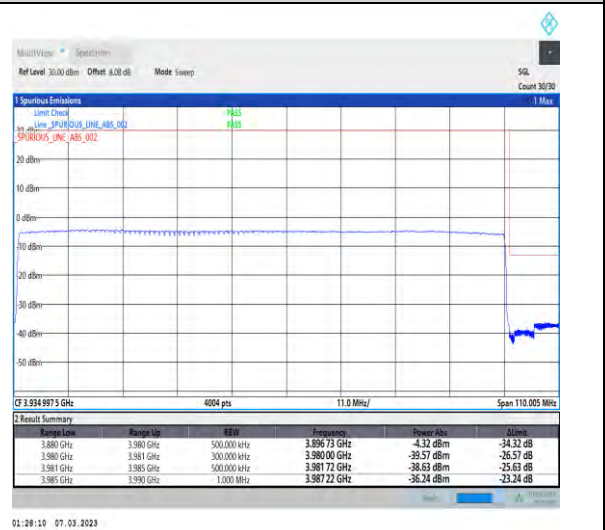
1-N77-3700-3980-PC3-30-100-H-6-CP-QPSK-Outer_Full-273@0-Ant1-1--PASS-see graph
