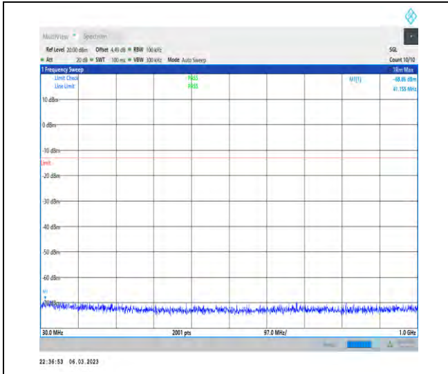
1-N77-3700-3980-PC3-30-100-M-1-DFT-PI2BPSK- nner_1RB_Left-1@1-30-1000-Ant1-41.16--68.86--1 3-PASS
