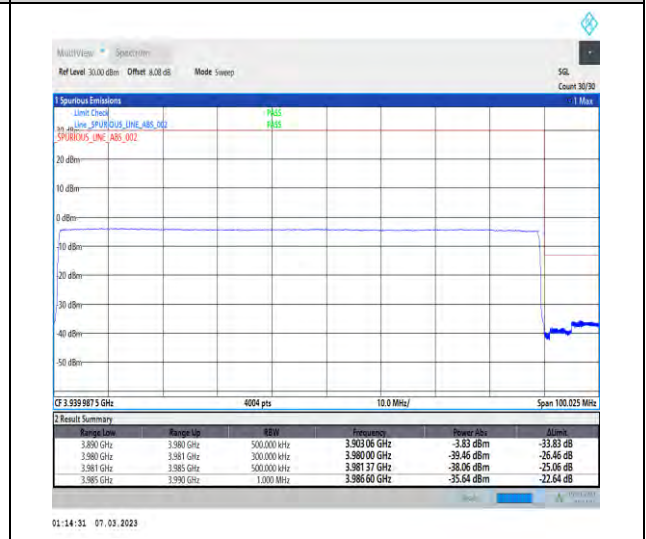
1-N77-3700-3980-PC3-30-90-H-6-CP-QPSK-Outer_Full-245@0-Ant1-1--PASS-see graph
