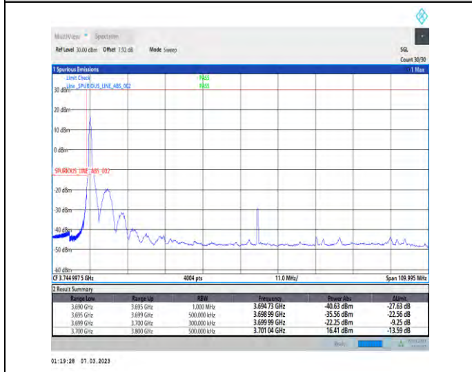
1-N77-3700-3980-PC3-30-100-L-4-CP-QPSK-Edge_1RB_Left-1@0-Ant1-1--PASS-see graph
