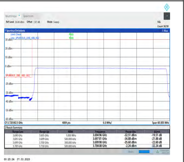
1-N77-3700-3980-PC3-30-50-L-6-CP-QPSK-Outer_Full-133@0-Ant1-1--PASS-see graph
