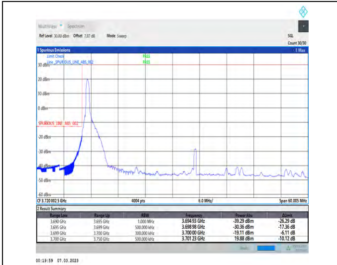
1-N77-3700-3980-PC3-30-50-L-1-DFT-PI2BPSK-Edge_1RB_Left-1@0-Ant1-1--PASS-see graph
