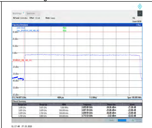
1-N77-3700-3980-PC3-30-100-L-3-DFT-PI2BPSK-Outer_Full-270@0-Ant1-1--PASS-see graph
