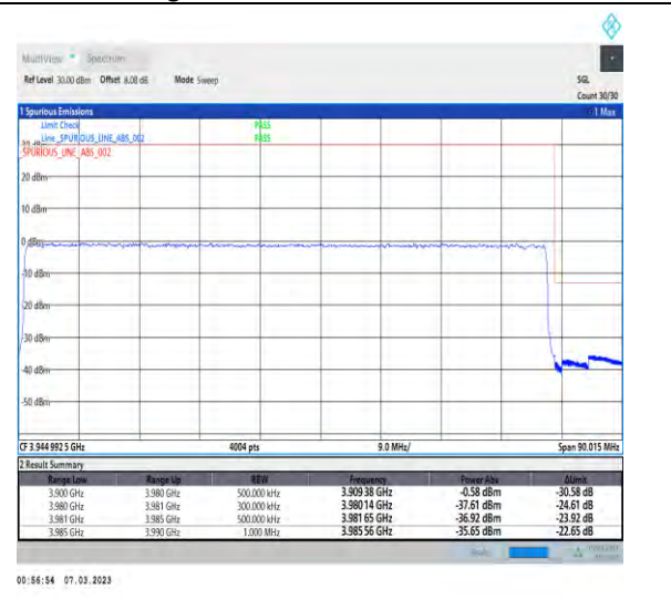
1-N77-3700-3980-PC3-30-80-H-3-DFT-PI2BPSK-Outer_Full-216@0-Ant1-1--PASS-see graph
