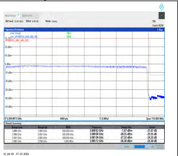
1-N77-3700-3980-PC3-30-100-H-3-DFT-PI2BPSK-Outer_Full-270@0-Ant1-1--PASS-see graph
