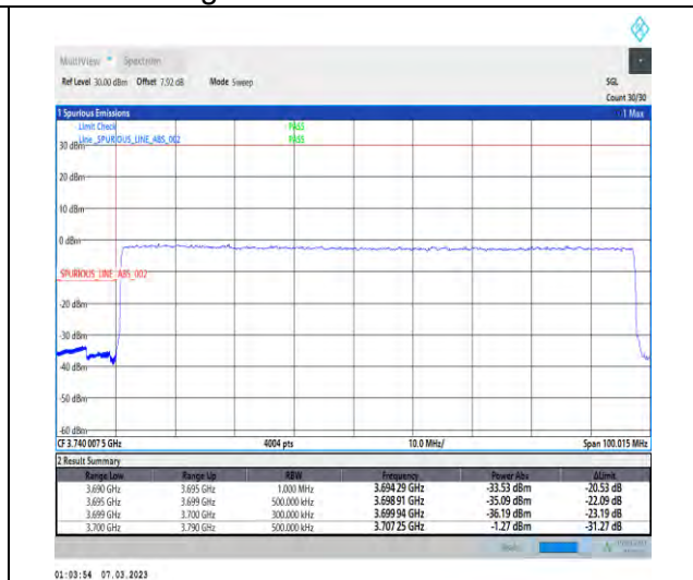
1-N77-3700-3980-PC3-30-90-L-3-DFT-PI2BPSK-Outer_Full-240@0-Ant1-1--PASS-see graph
