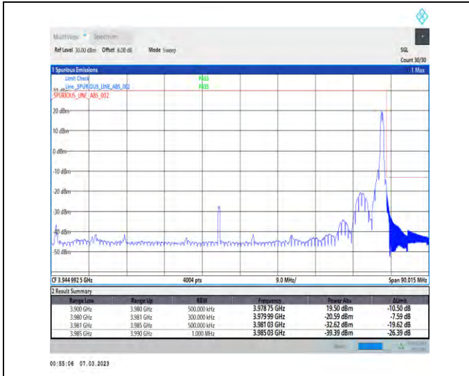
1-N77-3700-3980-PC3-30-80-H-2-DFT-PI2BPSK-Edge_1RB_Right-1@216-Ant1-1--PASS-see graph
