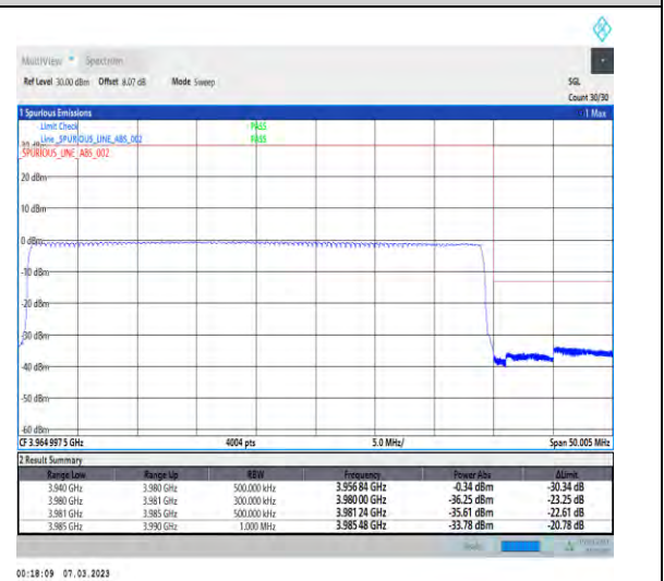
1-N77-3700-3980-PC3-30-40-H-6-CP-QPSK-Outer_Full-106@0-Ant1-1--PASS-see graph
