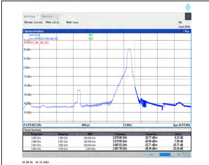
1-N77-3700-3980-PC3-30-20-H-2-DFT-PI2BPSK-Edge_1RB_Right-1@50-Ant1-1--PASS-see graph
