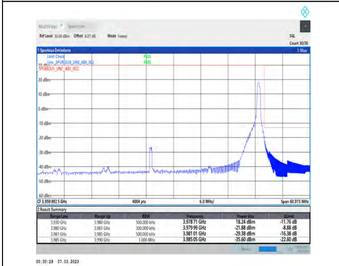
1-N77-3700-3980-PC3-30-50-H-5-CP-QPSK-Edge_1RB_Right-1@132-Ant1-1--PASS-see graph
