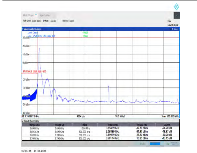
1-N77-3700-3980-PC3-30-90-L-4-CP-QPSK-Edge_1RB_Left-1@0-Ant1-1--PASS-see graph
