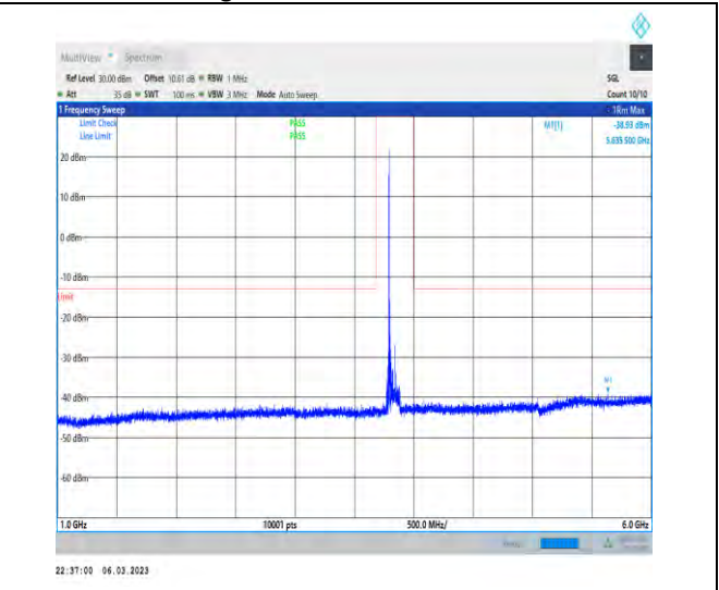
1-N77-3700-3980-PC3-30-100-M-1-DFT-PI2BPSK-In ner_1RB_Left-1@1-1000-6000-Ant1-5635.50--38.93- -13-PASS
