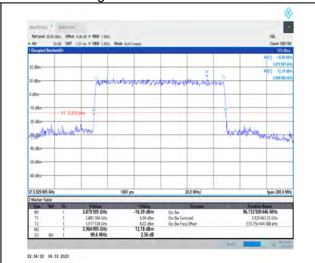
1-N77-3700-3980-PC3-30-100-H-4-DFT-64QAM-Out er_Full-270@0-Ant1-96.154-99.600-≤100-PASS
