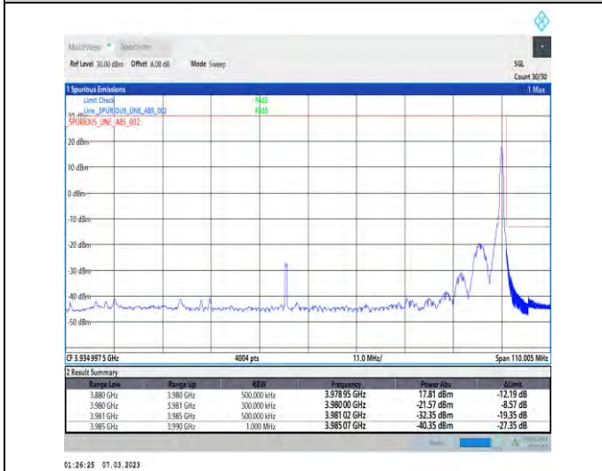
1-N77-3700-3980-PC3-30-100-H-5-CP-QPSK-Edge_1_RB_Right-1@272-Ant1-1--PASS-see graph
