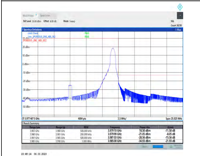
1-N77-3700-3980-PC3-30-15-H-5-CP-QPSK-Edge_1RB_Right-1@37-Ant1-1--PASS-see graph
