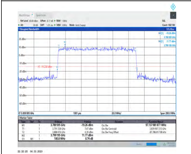
1-N77-3700-3980-PC3-30-100-M-6-CP-QPSK-Outer_Full-273@0-Ant1-97.138-100.800-≤100-PASS
