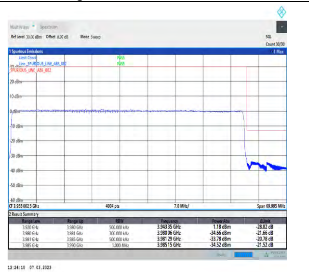
1-N77-3700-3980-PC3-30-60-H-3-DFT-PI2BPSK-Outer_Full-162@0-Ant1-1--PASS-see graph
