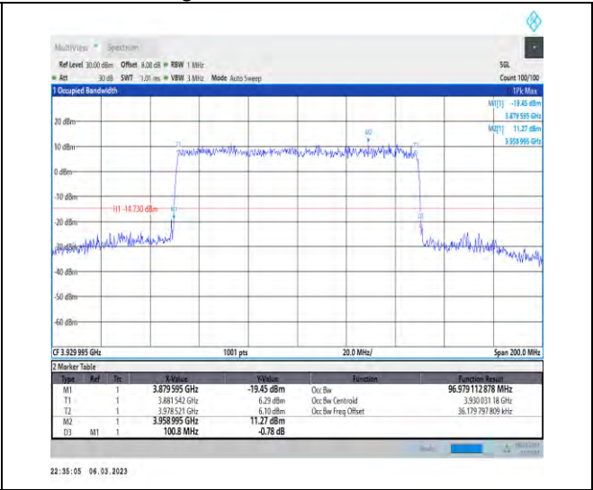
1-N77-3700-3980-PC3-30-100-H-8-CP-64QAM-Outer_Full-273@0-Ant1-96.979-100.800-≤100-PASS
