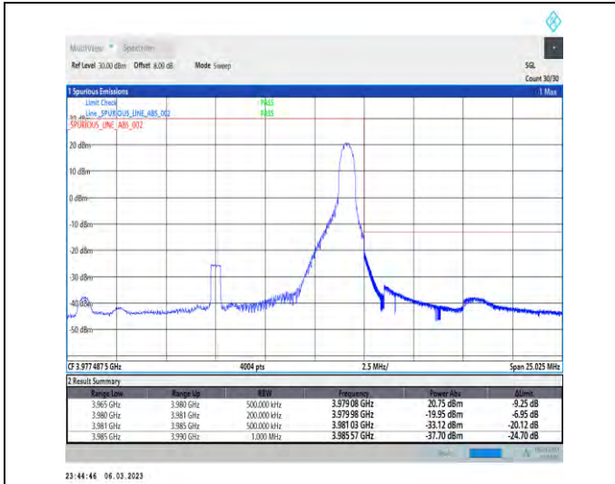
1-N77-3700-3980-PC3-30-15-H-2-DFT-PI2BPSK-Edge_1RB_Right-1@37-Ant1-1--PASS-see graph
