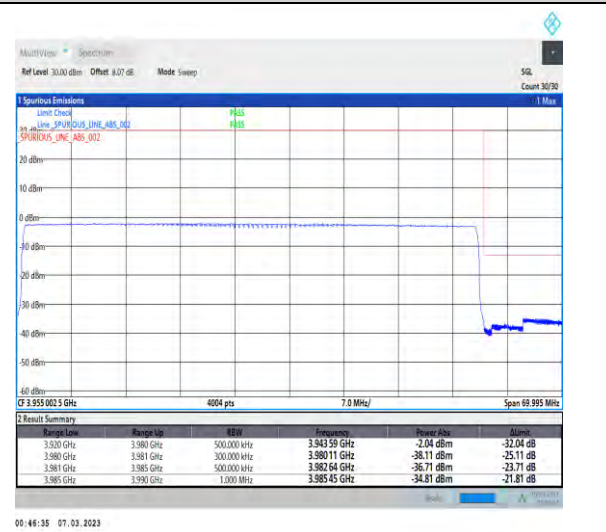
1-N77-3700-3980-PC3-30-60-H-6-CP-QPSK-Outer_Full-162@0-Ant1-1--PASS-see graph
