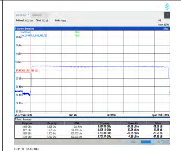
1-N77-3700-3980-PC3-30-90-L-6-CP-QPSK-Outer_Full-245@0-Ant1-1--PASS-see graph
