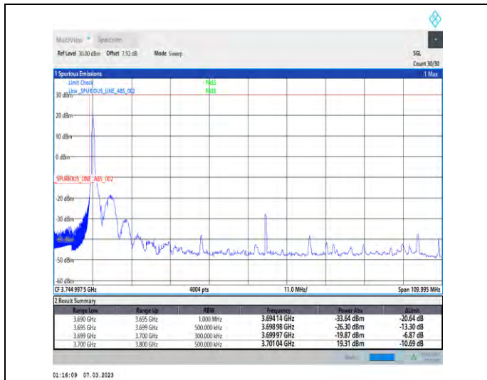
1-N77-3700-3980-PC3-30-100-L-1-DFT-PI2BPSK-Edge_1RB_Left-1@0-Ant1-1--PASS-see graph
