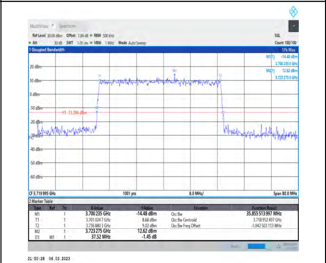
1-N77-3700-3980-PC3-30-40-L-3-DFT-16QAM-Outer_Full-100@0-Ant1-35.856-37.520-≤40-PASS
