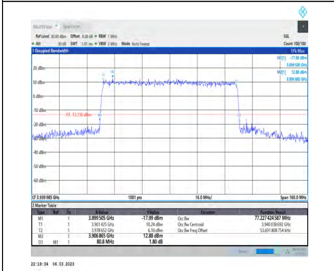
1-N77-3700-3980-PC3-30-80-H-7-CP-16QAM-Outer _Full-217@0-Ant1-77.227-80.800-≤80-PASS
