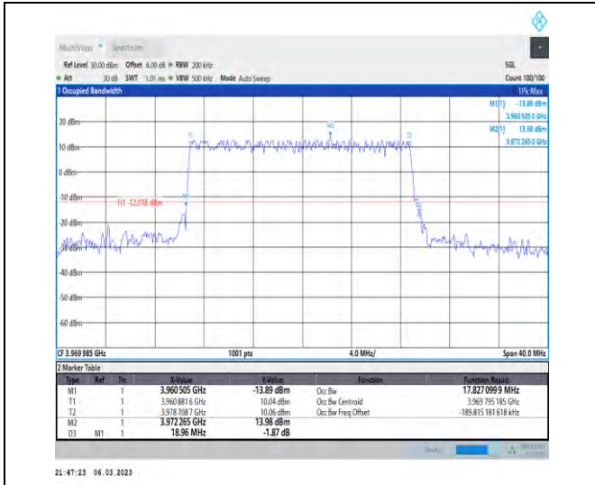
1-N77-3700-3980-PC3-30-20-H-1-DFT-QPSK-Outer_Full-50@0-Ant1-17.827-18.960-≤20-PASS
