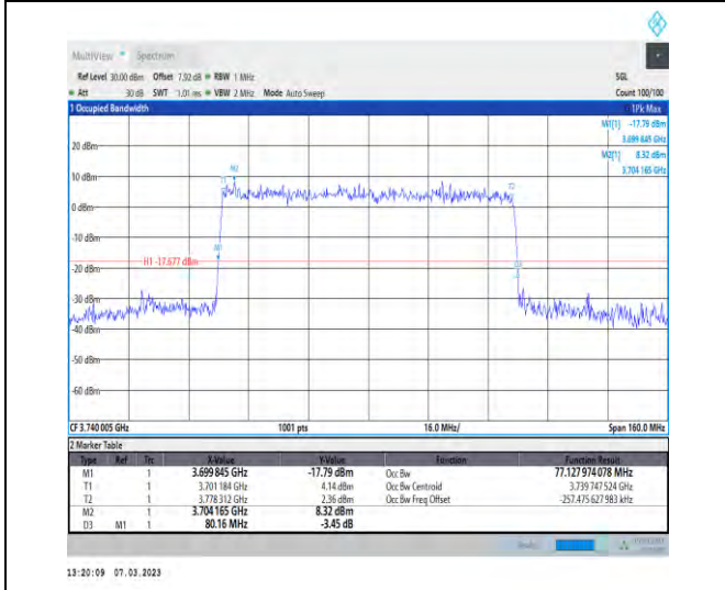
1-N77-3700-3980-PC3-30-80-L-5-DFT-256QAM-Outer_Full-216@0-Ant1-77.128-80.160-≤80-PASS
