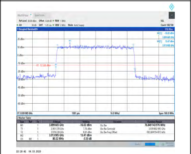
1-N77-3700-3980-PC3-30-80-H-4-DFT-64QAM-Outer_Full-216@0-Ant1-76.849-80.320-≤80-PASS
