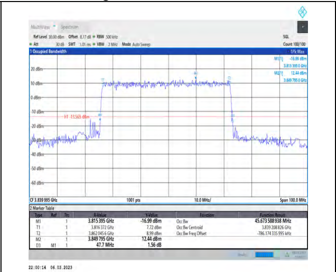
1-N77-3700-3980-PC3-30-50-M-1-DFT-QPSK-Outer_Full-128@0-Ant1-45.674-47.700-≤50-PASS
