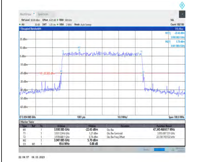
1-N77-3700-3980-PC3-30-50-H-9-CP-256QAM-Outer_Full-133@0-Ant1-47.345-49.600-≤50-PASS
