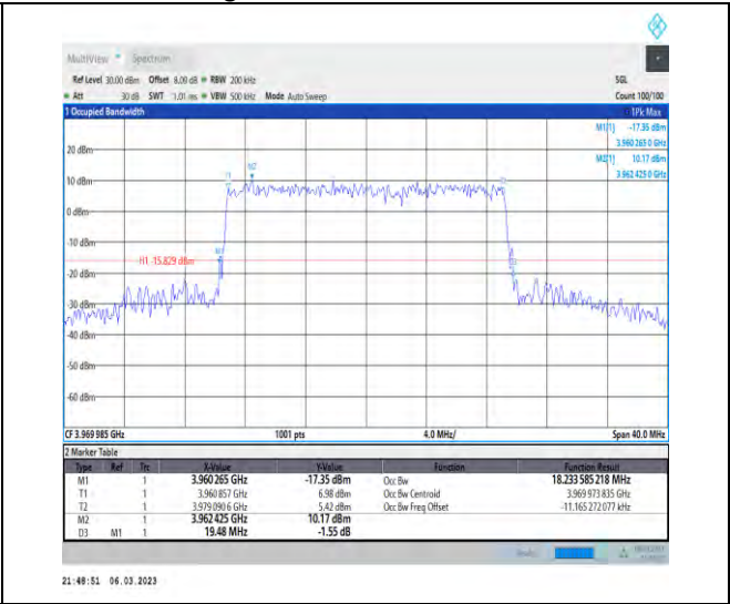
1-N77-3700-3980-PC3-30-20-H-6-CP-QPSK-Outer _Full-51@0-Ant1-18.234-19.480-≤20-PASS
