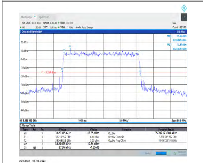
1-N77-3700-3980-PC3-30-40-M-5-DFT-256QAM-Outer_Full-100@0-Ant1-35.707-37.360-≤40-PASS
