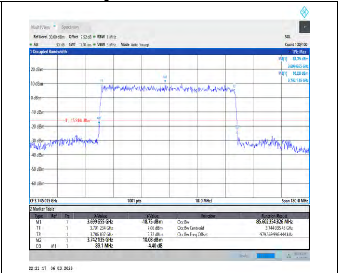
1-N77-3700-3980-PC3-30-90-L-5-DFT-256QAM-Outer_Full-240@0-Ant1-85.602-89.100-≤90-PASS
