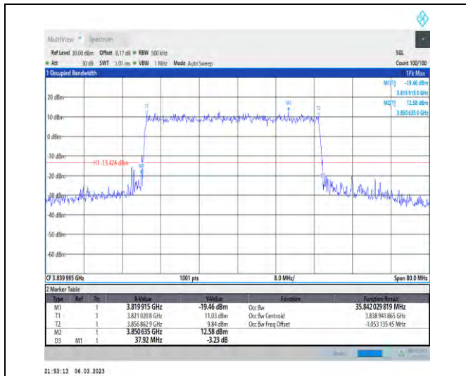
1-N77-3700-3980-PC3-30-40-M-3-DFT-16QAM-Outer_Full-100@0-Ant1-35.842-37.920-≤40-PASS
