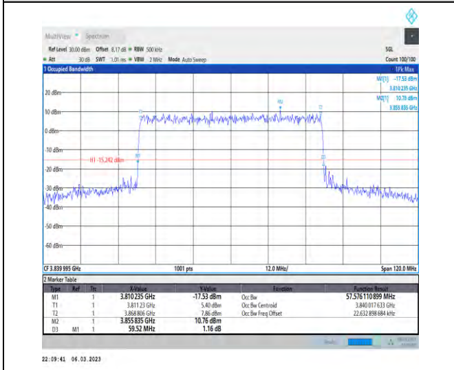
1-N77-3700-3980-PC3-30-60-M-7-CP-16QAM-Outer _Full-162@0-Ant1-57.576-59.520-≤60-PASS
