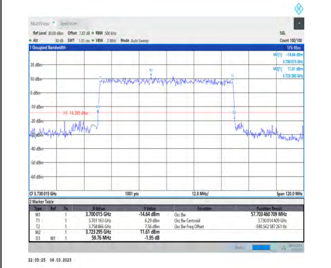
1-N77-3700-3980-PC3-30-60-L-1-DFT-QPSK-Outer_Full-162@0-Ant1-57.703-59.760-≤60-PASS
