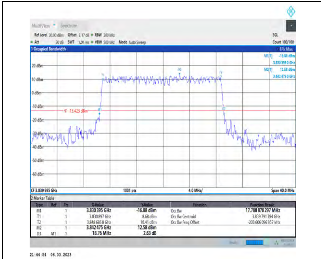
1-N77-3700-3980-PC3-30-20-M-2-DFT-PI2BPSK-Out_Full-50@0-Ant1-17.789-18.760-≤20-PASS
