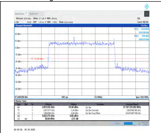
1-N77-3700-3980-PC3-30-60-M-6-CP-QPSK-Outer_ Full-162@0-Ant1-57.767-59.640-≤60-PASS
