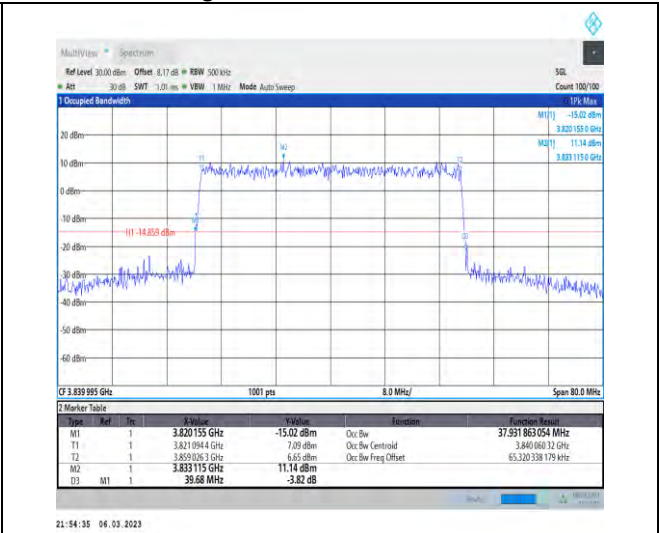
1-N77-3700-3980-PC3-30-40-M-8-CP-64QAM-Outer_Full-106@0-Ant1-37.932-39.680-≤40-PASS
