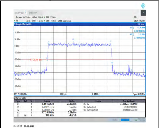
1-N77-3700-3980-PC3-30-40-L-9-CP-256QAM-Outer_Full-106@0-Ant1-37.834-39.600-≤40-PASS
