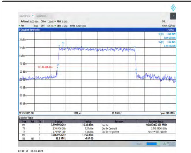
1-N77-3700-3980-PC3-30-100-L-3-DFT-16QAM-Outer_Full-270@0-Ant1-96.029-99.800-≤100-PASS
