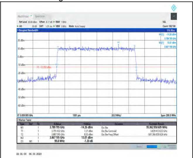
1-N77-3700-3980-PC3-30-100-M-1-DFT-QPSK-Outer_Full-270@0-Ant1-95.963-99.800-≤100-PASS
