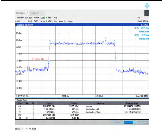
1-N77-3700-3980-PC3-30-80-H-5-DFT-256QAM-Out er_Full-216@0-Ant1-76.994-80.480-≤80-PASS
