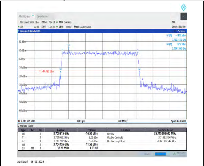
1-N77-3700-3980-PC3-30-40-L-5-DFT-256QAM-Outer_Full-100@0-Ant1-35.716-37.280-≤40-PASS
