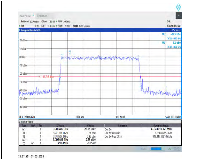
1-N77-3700-3980-PC3-30-50-L-9-CP-256QAM-Outer_Full-133@0-Ant1-47.343-49.600-≤50-PASS
