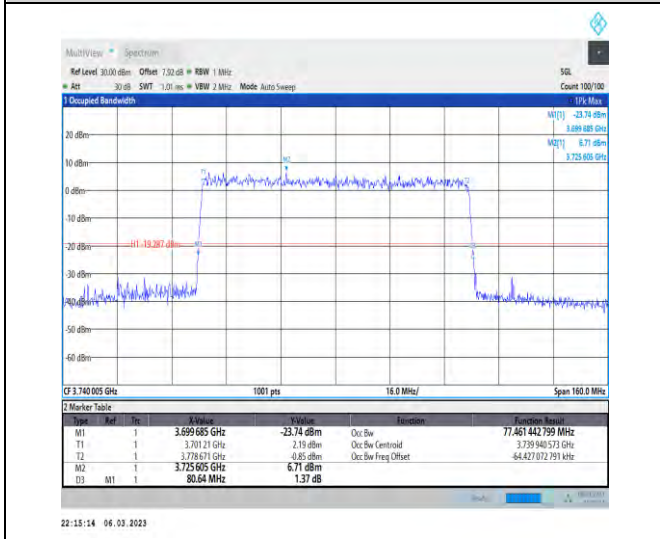
1-N77-3700-3980-PC3-30-80-L-9-CP-256QAM-Outer_Full-217@0-Ant1-77.461-80.640-≤80-PASS
