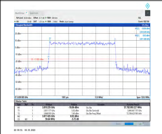
1-N77-3700-3980-PC3-30-60-M-8-CP-64QAM-Outer _Full-162@0-Ant1-57.782-59.640-≤60-PASS
