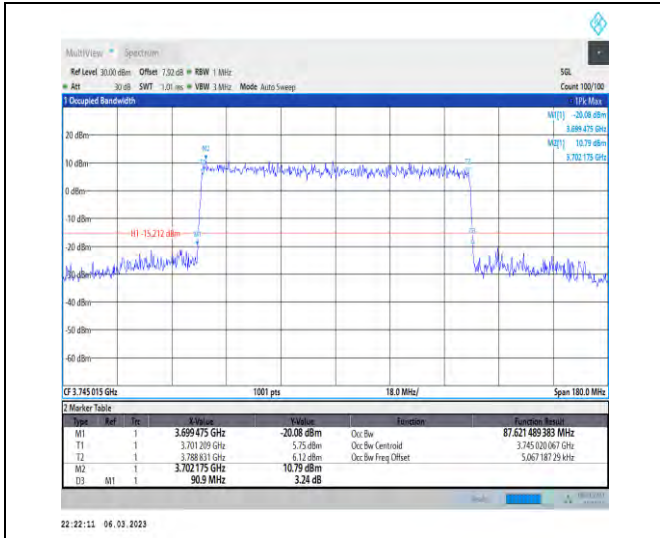
1-N77-3700-3980-PC3-30-90-L-8-CP-64QAM-Outer_Full-245@0-Ant1-87.621-90.900-≤90-PASS
