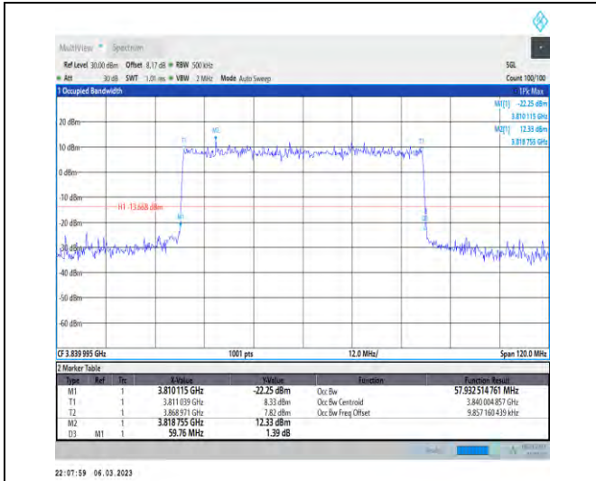
1-N77-3700-3980-PC3-30-60-M-1-DFT-QPSK-Outer_Full-162@0-Ant1-57.933-59.760-≤60-PASS
