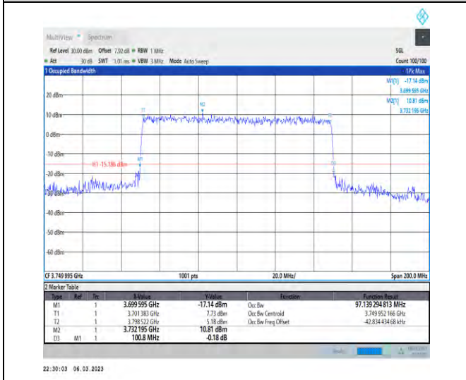
1-N77-3700-3980-PC3-30-100-L-7-CP-16QAM-Outer_Full-273@0-Ant1-97.139-100.800-≤100-PASS
