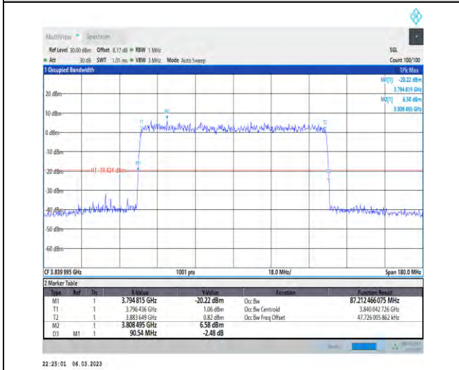
1-N77-3700-3980-PC3-30-90-M-9-CP-256QAM-Outer_Full-245@0-Ant1-87.212-90.540-≤90-PASS
