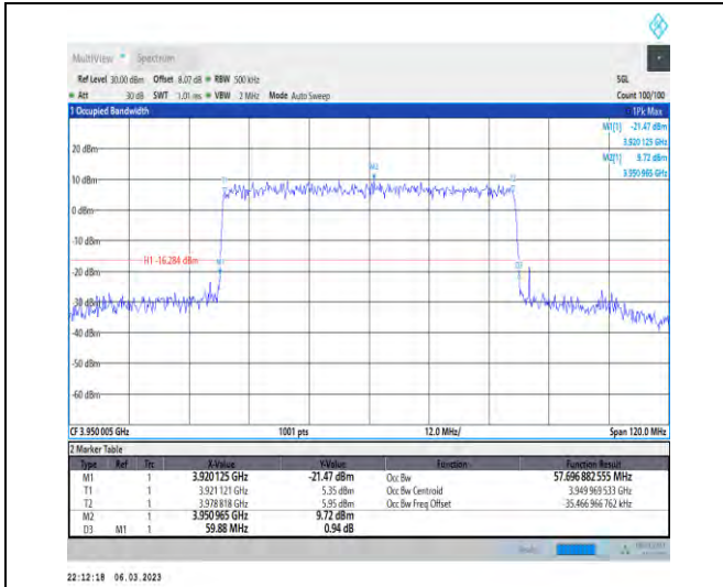
1-N77-3700-3980-PC3-30-60-H-8-CP-64QAM-Outer_Full-162@0-Ant1-57.697-59.880-≤60-PASS
