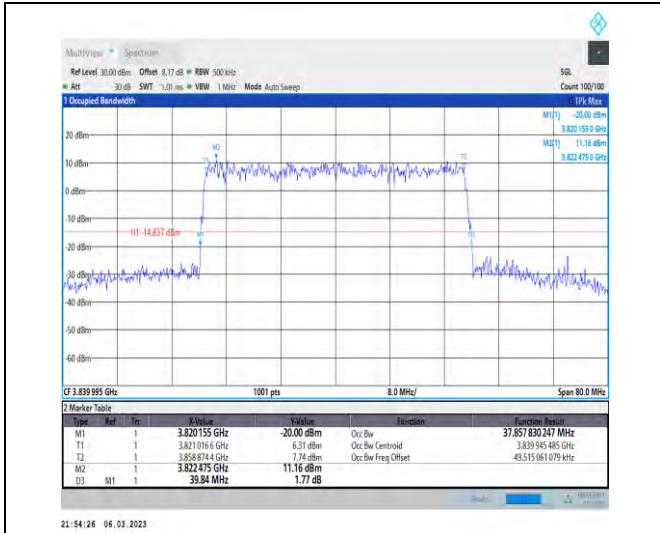
1-N77-3700-3980-PC3-30-40-M-7-CP-16QAM-Outer_Full-106@0-Ant1-37.858-39.840-≤40-PASS
