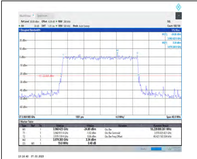
1-N77-3700-3980-PC3-30-20-H-9-CP-256QAM-Outer_Full-51@0-Ant1-18.228-19.000-≤20-PASS
