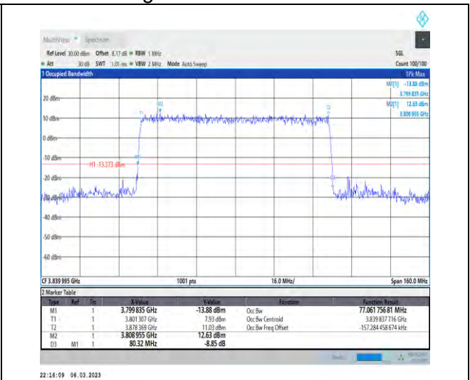
1-N77-3700-3980-PC3-30-80-M-3-DFT-16QAM-Outer_Full-216@0-Ant1-77.062-80.320-≤80-PASS
