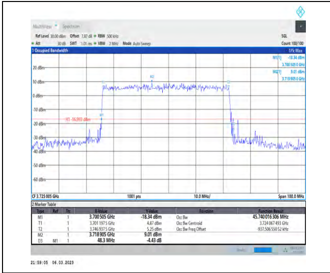
1-N77-3700-3980-PC3-30-50-L-5-DFT-256QAM-Out_er_Full-128@0-Ant1-45.74-48.300-≤50-PASS
