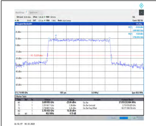
1-N77-3700-3980-PC3-30-40-L-8-CP-64QAM-Outer_Full-106@0-Ant1-37.818-40.000-≤40-PASS
