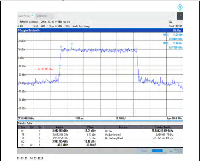
1-N77-3700-3980-PC3-30-50-H-4-DFT-64QAM-Outer_Full-128@0-Ant1-45.589-47.900-≤50-PASS
