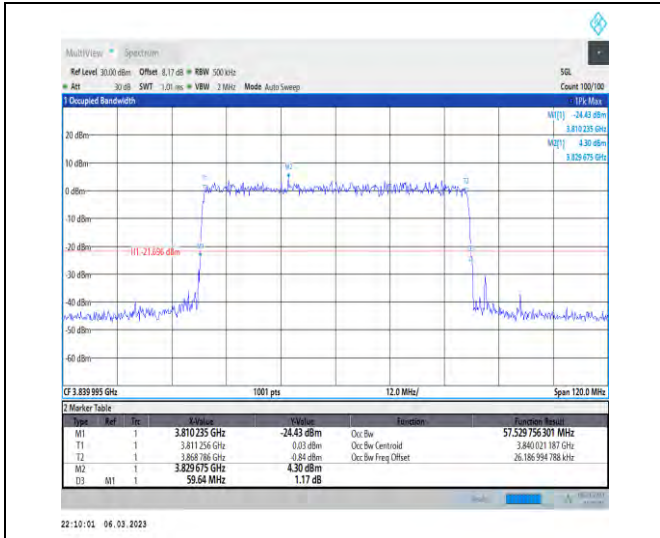
1-N77-3700-3980-PC3-30-60-M-9-CP-256QAM-Outer_Full-162@0-Ant1-57.53-59.640-≤60-PASS
