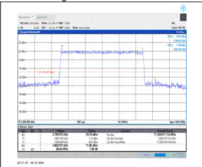
1-N77-3700-3980-PC3-30-80-M-7-CP-16QAM-Outer_Full-217@0-Ant1-77.344-80.640-<math>\leq 80</math>-PASS
