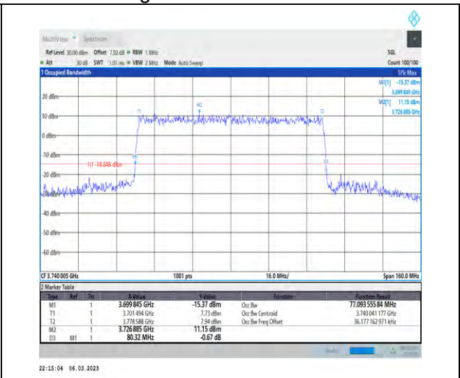
1-N77-3700-3980-PC3-30-80-L-8-CP-64QAM-Outer_Full-217@0-Ant1-77.094-80.320-≤80-PASS
