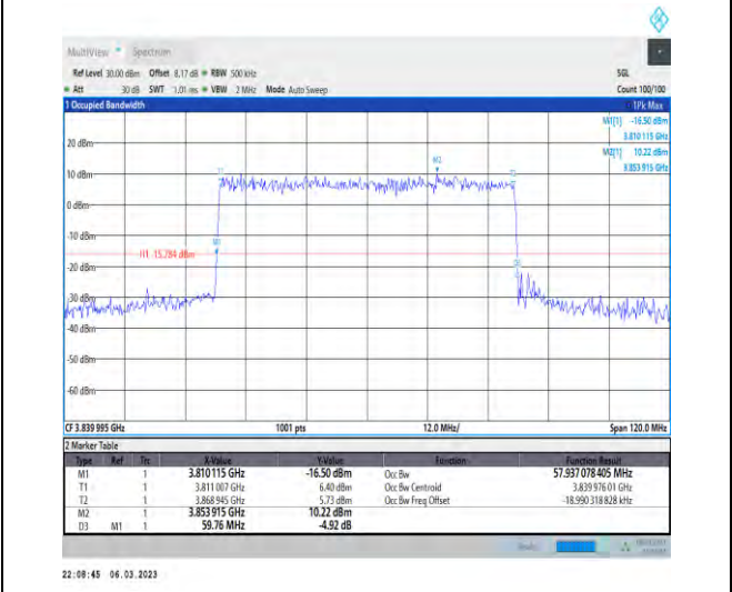
1-N77-3700-3980-PC3-30-60-M-4-DFT-64QAM-Outer_Full-162@0-Ant1-57.937-59.760-≤60-PASS
