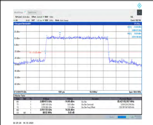
1-N77-3700-3980-PC3-30-90-H-1-DFT-QPSK-Outer_Full-240@0-Ant1-85.422-88.920-≤90-PASS
