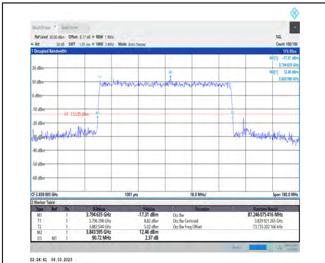
1-N77-3700-3980-PC3-30-90-M-7-CP-16QAM-Outer_Full-245@0-Ant1-87.246-90.720-≤90-PASS
