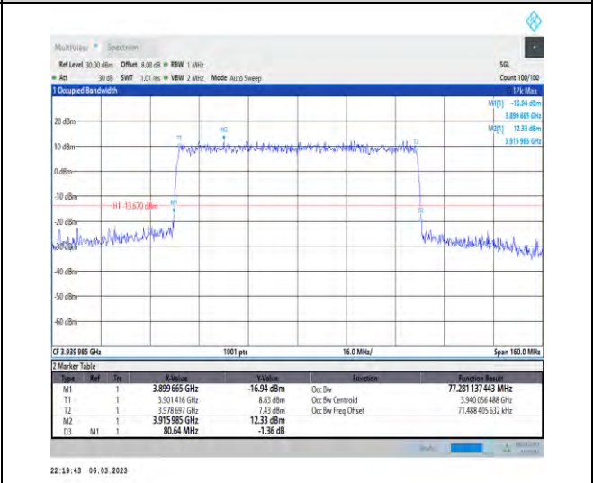
1-N77-3700-3980-PC3-30-80-H-8-CP-64QAM-Outer _Full-217@0-Ant1-77.281-80.640-≤80-PASS
