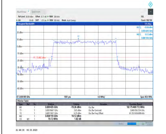
1-N77-3700-3980-PC3-30-20-M-8-CP-64QAM-Outer_Full-51@0-Ant1-18.175-19.120-≤20-PASS
