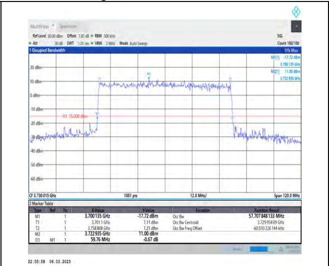
1-N77-3700-3980-PC3-30-60-L-3-DFT-16QAM-Outer_Full-162@0-Ant1-57.708-59.760-<math>\leq 60</math>-PASS
