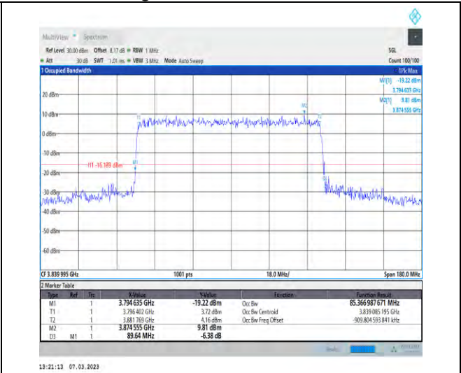
1-N77-3700-3980-PC3-30-90-M-4-DFT-64QAM-Outer_Full-240@0-Ant1-85.367-89.640-≤90-PASS
