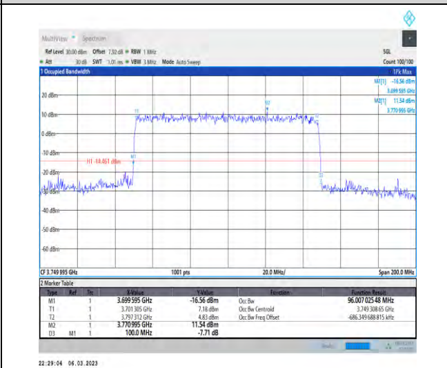
1-N77-3700-3980-PC3-30-100-L-4-DFT-64QAM-Outer_Full-270@0-Ant1-96.007-100.000-≤100-PASS
