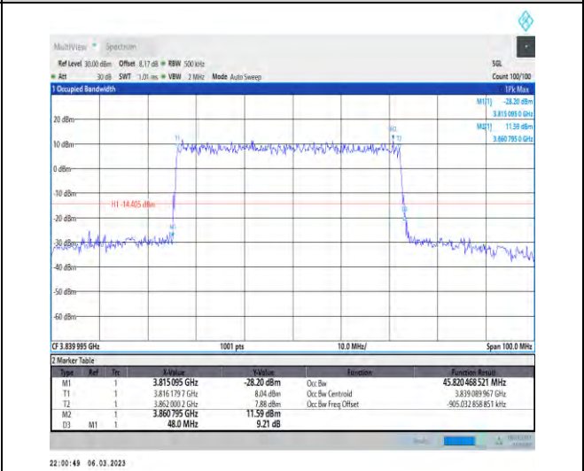
1-N77-3700-3980-PC3-30-50-M-3-DFT-16QAM-Outer_Full-128@0-Ant1-45.82-48.000-≤50-PASS
