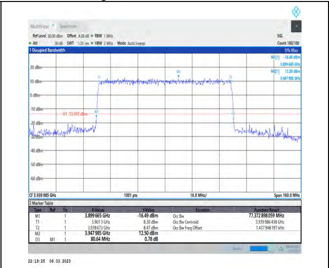
1-N77-3700-3980-PC3-30-80-H-6-CP-QPSK-Outer_ Full-217@0-Ant1-77.373-80.640-≤80-PASS
