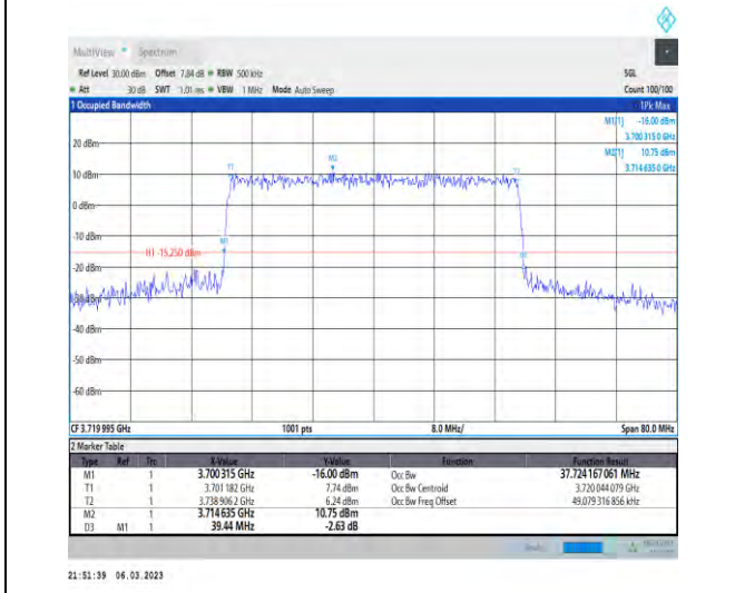
1-N77-3700-3980-PC3-30-40-L-6-CP-QPSK-Outer_Full-106@0-Ant1-37.724-39.440-≤40-PASS
