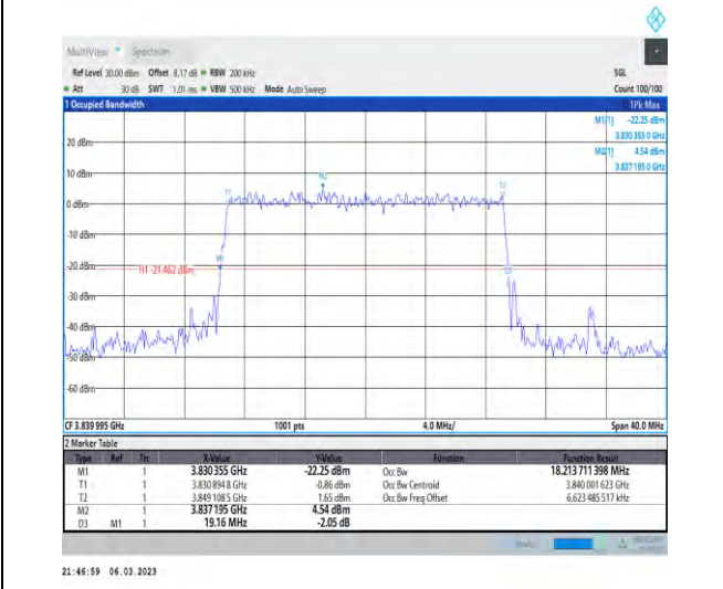
1-N77-3700-3980-PC3-30-20-M-9-CP-256QAM-Outer_Full-51@0-Ant1-18.214-19.160-≤20-PASS
