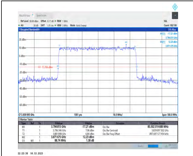
1-N77-3700-3980-PC3-30-90-M-3-DFT-16QAM-Outer_Full-240@0-Ant1-85.502-88.740-≤90-PASS
