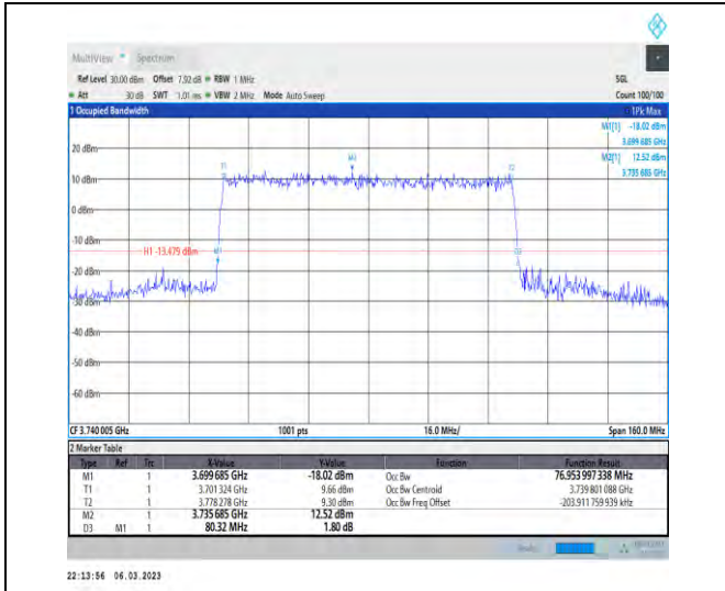
1-N77-3700-3980-PC3-30-80-L-3-DFT-16QAM-Outer_Full-216@0-Ant1-76.954-80.320-≤80-PASS
