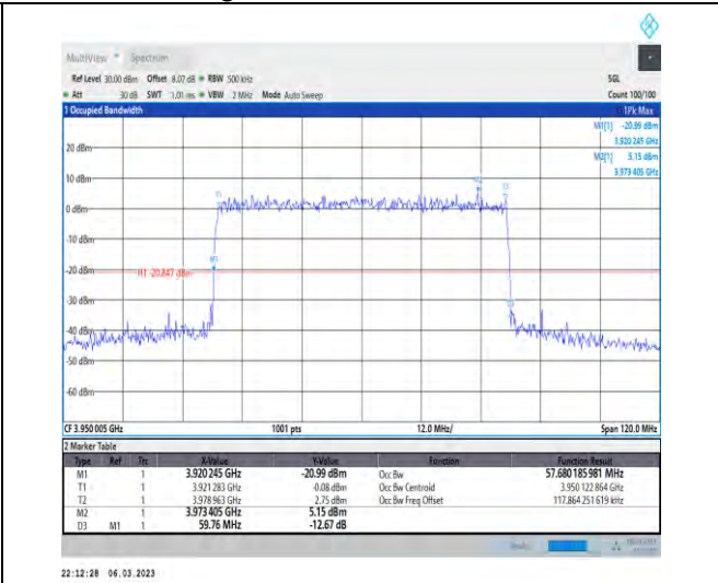
1-N77-3700-3980-PC3-30-60-H-9-CP-256QAM-Outer_Full-162@0-Ant1-57.68-59.760-≤60-PASS
