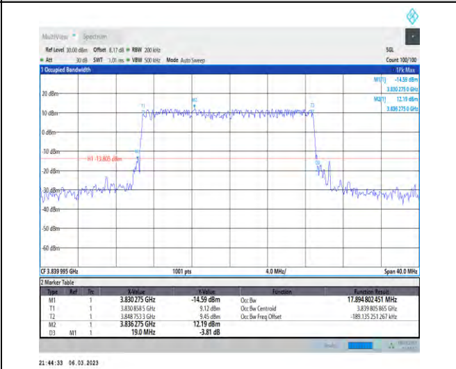
1-N77-3700-3980-PC3-30-20-M-1-DFT-QPSK-Outer_Full-50@0-Ant1-17.895-19.000-≤20-PASS
