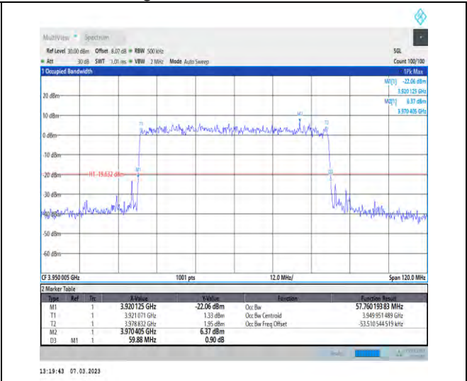
1-N77-3700-3980-PC3-30-60-H-5-DFT-256QAM-Outer_Full-162@0-Ant1-57.76-59.880-≤60-PASS
