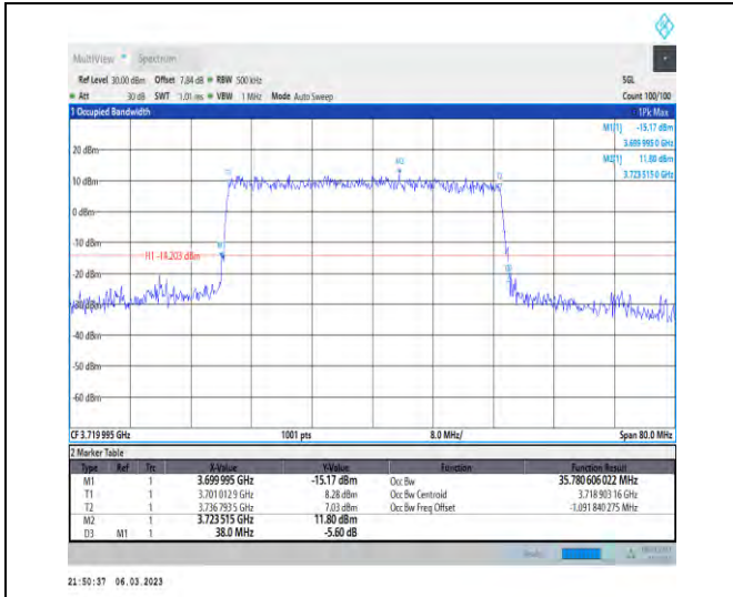
1-N77-3700-3980-PC3-30-40-L-4-DFT-64QAM-Outer_Full-100@0-Ant1-35.781-38.000-≤40-PASS
