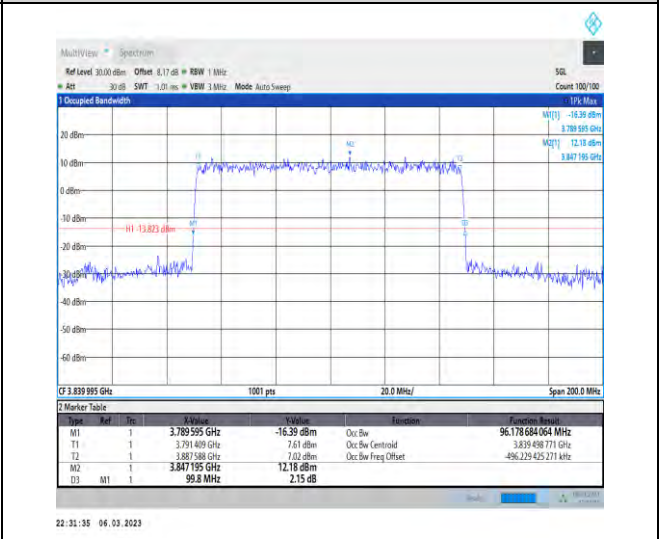
1-N77-3700-3980-PC3-30-100-M-3-DFT-16QAM-Outer_Full-270@0-Ant1-96.179-99.800-≤100-PASS
