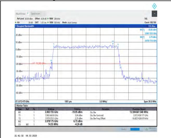
1-N77-3700-3980-PC3-30-15-H-9-CP-256QAM-Outer_Full-38@0-Ant1-13.595-14.550-≤15-PASS
