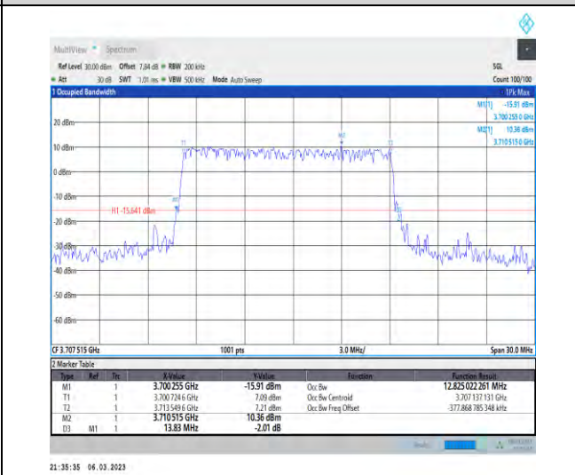
1-N77-3700-3980-PC3-30-15-L-5-DFT-256QAM-Out er_Full-36@0-Ant1-12.825-13.830-≤15-PASS
