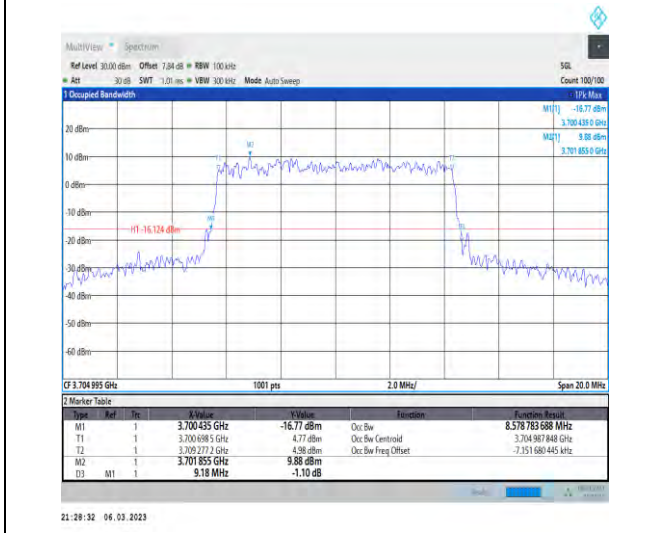
1-N77-3700-3980-PC3-30-10-L-7-CP-16QAM-Outer Full-24@0-Ant1-8.579-9.180-≤10-PASS
