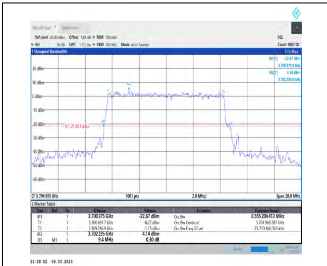
1-N77-3700-3980-PC3-30-10-L-9-CP-256QAM-Outer_Full-24@0-Ant1-8.555-9.400-≤10-PASS
