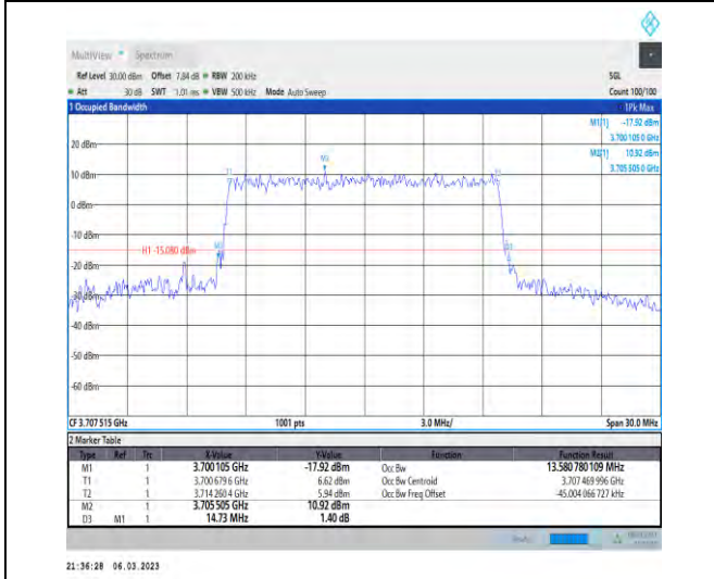
1-N77-3700-3980-PC3-30-15-L-8-CP-64QAM-Outer_Full-38@0-Ant1-13.581-14.730-≤15-PASS
