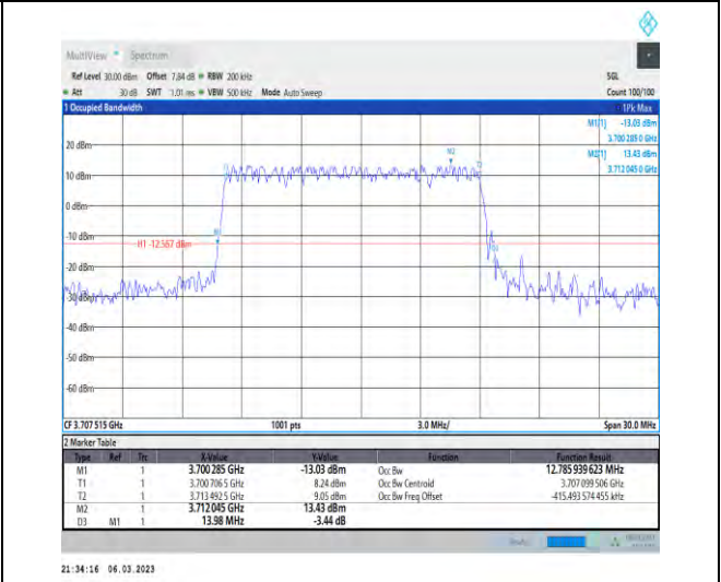
1-N77-3700-3980-PC3-30-15-L-1-DFT-QPSK-Outer _Full-36@0-Ant1-12.786-13.980-≤15-PASS
