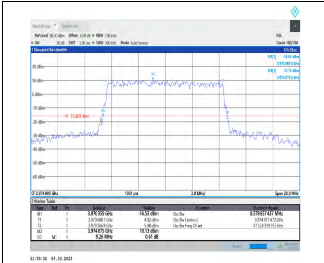
1-N77-3700-3980-PC3-30-10-H-7-CP-16QAM-Outer _Full-24@0-Ant1-8.579-9.260-≤10-PASS
