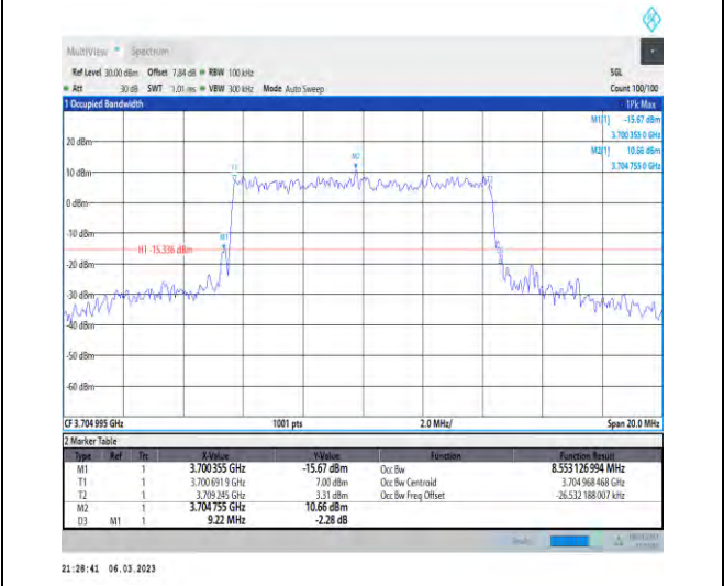
1-N77-3700-3980-PC3-30-10-L-8-CP-64QAM-Outer Full-24@0-Ant1-8.553-9.220-≤10-PASS
