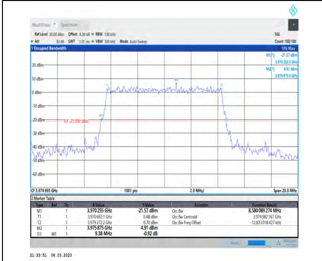
1-N77-3700-3980-PC3-30-10-H-9-CP-256QAM-Outer _Full-24@0-Ant1-8.58-9.380-≤10-PASS
