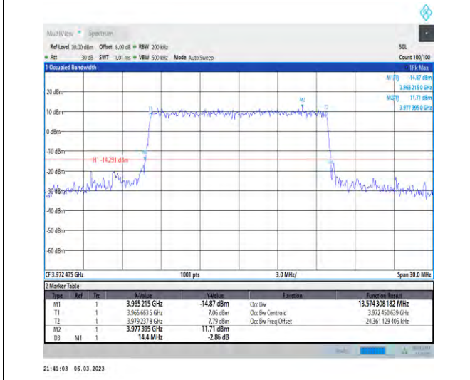
1-N77-3700-3980-PC3-30-15-H-6-CP-QPSK-Outer_Full-38@0-Ant1-13.574-14.400-≤15-PASS
