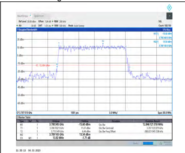
1-N77-3700-3980-PC3-30-15-L-3-DFT-16QAM-Out er_Full-36@0-Ant1-12.846-13.920-≤15-PASS
