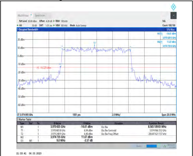
1-N77-3700-3980-PC3-30-10-H-8-CP-64QAM-Outer _Full-24@0-Ant1-8.565-9.000-≤10-PASS
