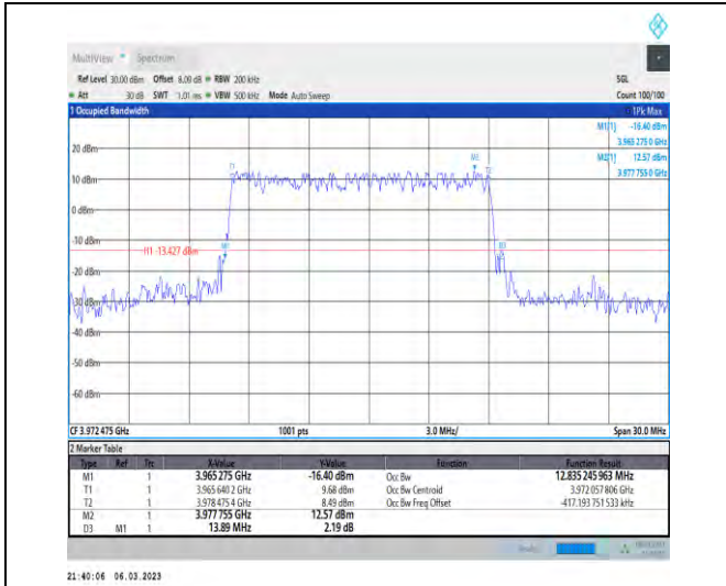
1-N77-3700-3980-PC3-30-15-H-4-DFT-64QAM-Outer_Full-36@0-Ant1-12.835-13.890-≤15-PASS
