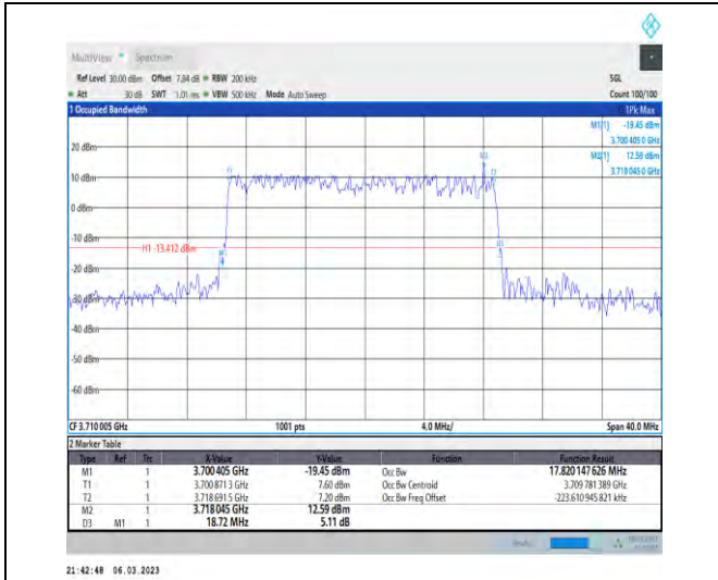
1-N77-3700-3980-PC3-30-20-L-3-DFT-16QAM-Outer_Full-50@0-Ant1-17.82-18.720-≤20-PASS
