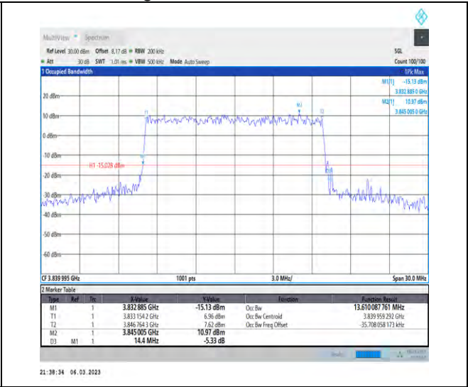
1-N77-3700-3980-PC3-30-15-M-6-CP-QPSK-Outer Full-38@0-Ant1-13.61-14.400-≤15-PASS
