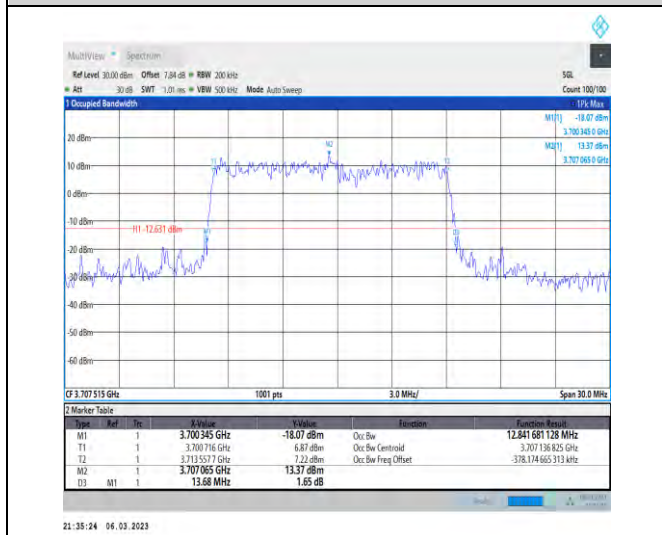
1-N77-3700-3980-PC3-30-15-L-4-DFT-64QAM-Out er_Full-36@0-Ant1-12.842-13.680-≤15-PASS
