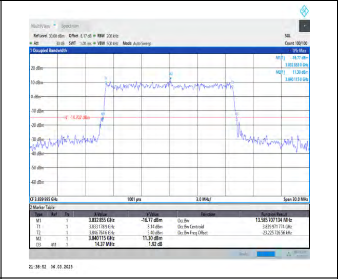
1-N77-3700-3980-PC3-30-15-M-8-CP-64QAM-Outer Full-38@0-Ant1-13.586-14.370-≤15-PASS
