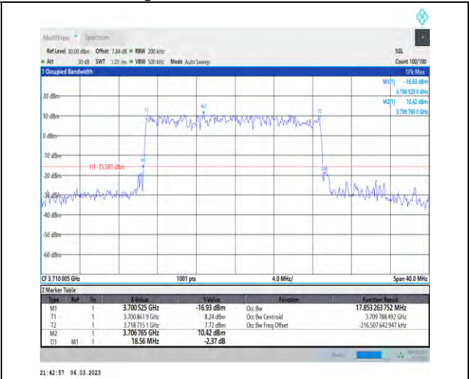
1-N77-3700-3980-PC3-30-20-L-4-DFT-64QAM-Outer_Full-50@0-Ant1-17.853-18.560-≤20-PASS
