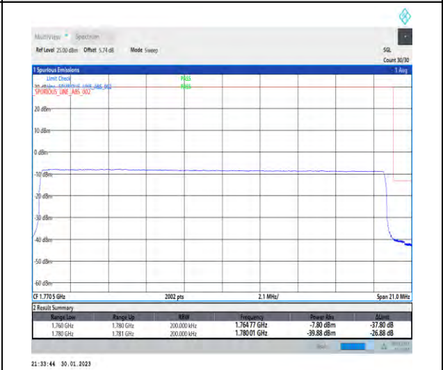
1-N66-PC3-15-20-H-6-CP-QPSK-Outer_Full-106@0-Ant1-1-seegraph-PASS-see graph
