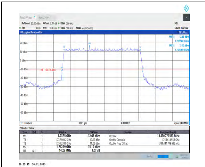
1-N66-PC3-15-15-M-2-DFT-PI2BPSK-Outer_Full-75 @0-Ant1-13.431-14.250-≤15-PASS
