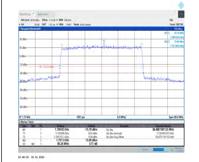
1-N66-PC3-15-40-L-3-DFT-16QAM-Outer_Full-216 @0-Ant1-38.488-40.240-≤40-PASS
