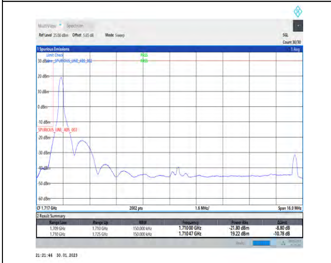
1-N66-PC3-15-15-L-4-CP-QPSK-Edge_1RB_Left-1@0-Ant1-1-seegraph-PASS-see graph
