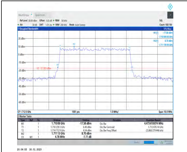
1-N66-PC3-15-5-L-5-DFT-256QAM-Outer_Full-25@0-Ant1-4.474-4.780-≤5-PASS
