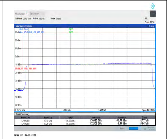
1-N66-PC3-15-15-L-6-CP-QPSK-Outer_Full-79@0-Ant1-1-seegraph-PASS-see graph
