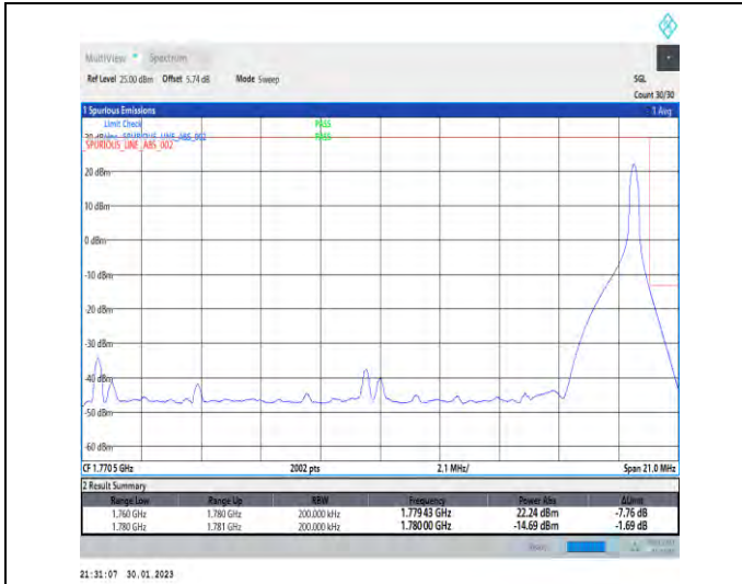
1-N66-PC3-15-20-H-2-DFT-PI2BPSK-Edge_1RB_Right-t-1@105-Ant1-1-seegraph-PASS-see graph
