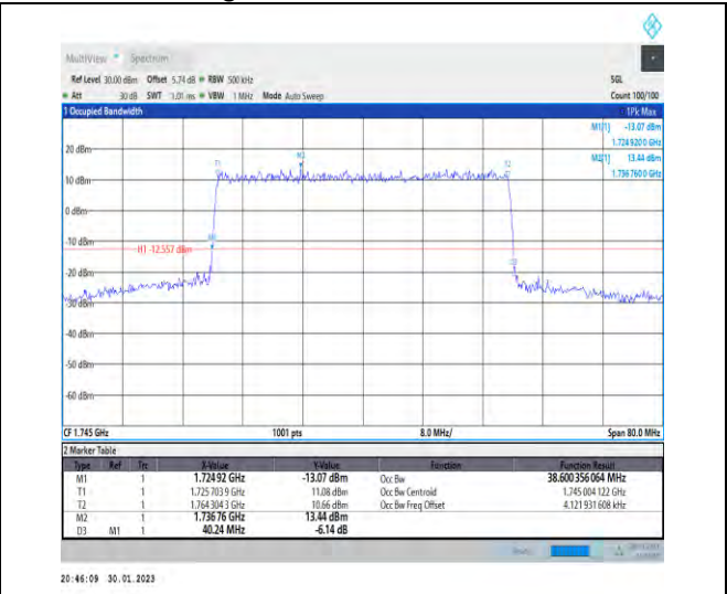
1-N66-PC3-15-40-M-1-DFT-QPSK-Outer_Full-216 @0-Ant1-38.6-40.240-≤40-PASS
