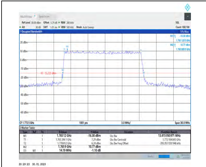
1-N66-PC3-15-15-H-5-DFT-256QAM-Outer_Full-75 @0-Ant1-13.416-14.190-≤15-PASS
