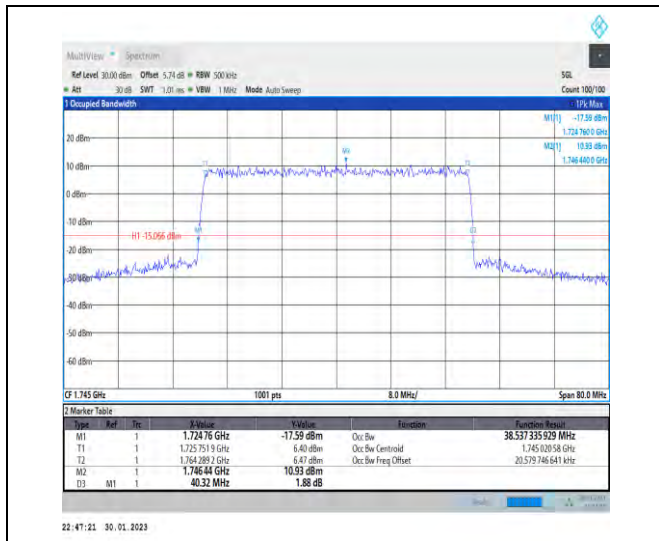
1-N66-PC3-15-40-M-8-CP-64QAM-Outer_Full-216@ 0-Ant1-38.537-40.320-≤40-PASS
