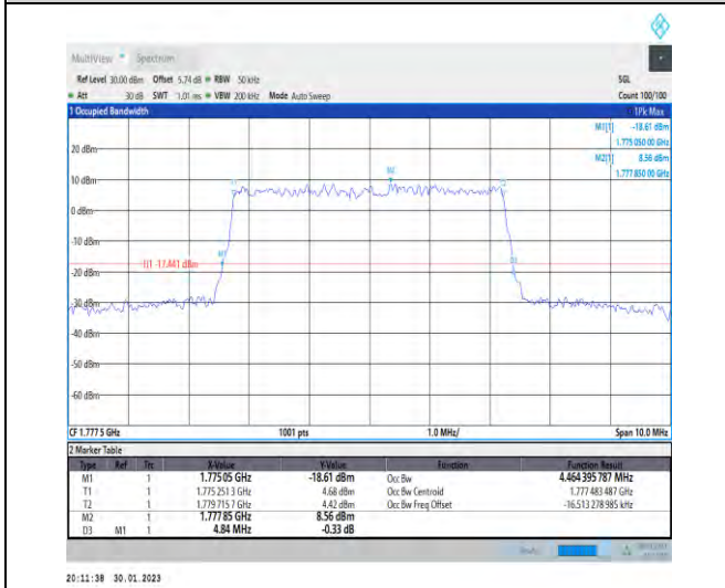
1-N66-PC3-15-5-H-5-DFT-256QAM-Outer_Full-25@0 0-Ant1-4.464-4.840-<math>\leq</math>5-PASS
