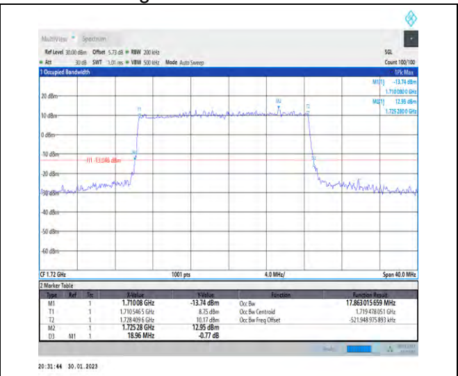
1-N66-PC3-15-20-L-1-DFT-QPSK-Outer_Full-100@ 0-Ant1-17.863-18.960-≤20-PASS
