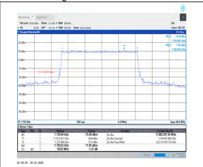
1-N66-PC3-15-20-M-4-DFT-64QAM-Outer_Full-100 @0-Ant1-17.882-18.920-≤20-PASS
