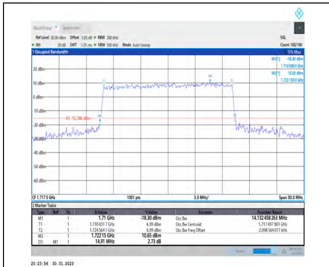
1-N66-PC3-15-15-L-7-CP-16QAM-Outer_Full-79@0-Ant1-14.132-14.910-≤15-PASS
