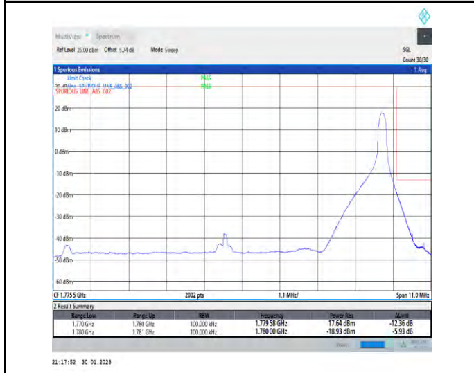
1-N66-PC3-15-10-H-5-CP-QPSK-Edge_1RB_Right-1@51-Ant1-1-seegraph-PASS-see graph
