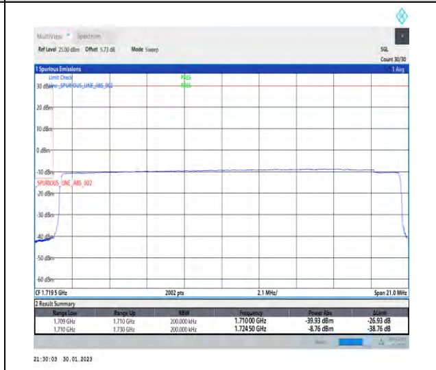
1-N66-PC3-15-20-L-6-CP-QPSK-Outer_Full-106@0-Ant1-1-seegraph-PASS-see graph
