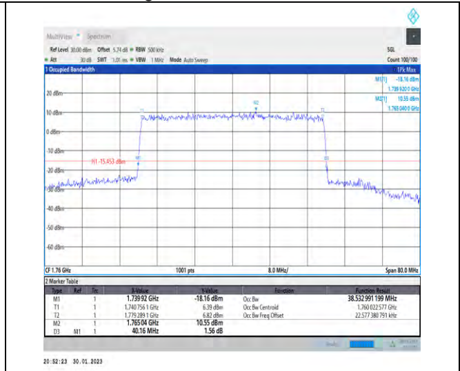
1-N66-PC3-15-40-H-8-CP-64QAM-Outer_Full-216@ 0-Ant1-38.533-40.160-≤40-PASS
