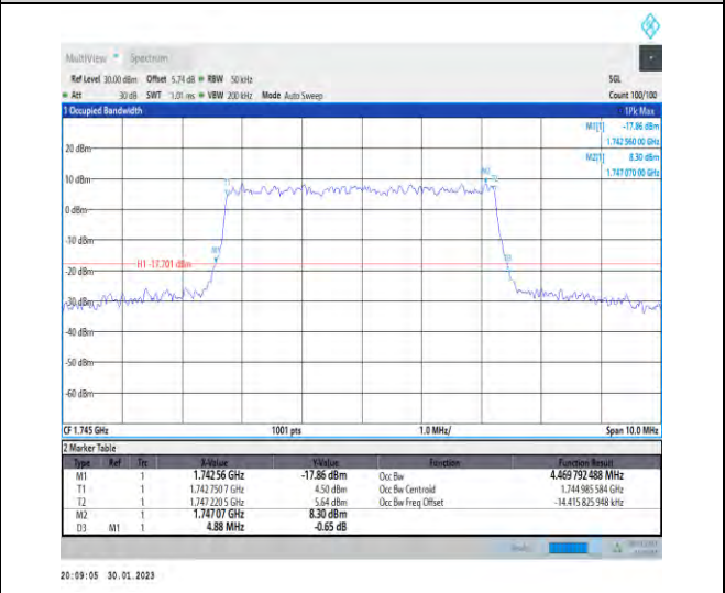
1-N66-PC3-15-5-M-7-CP-16QAM-Outer_Full-25@0-Ant1-4.47-4.880-≤5-PASS
