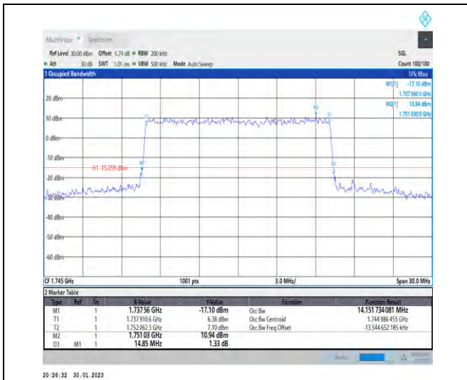
1-N66-PC3-15-15-M-6-CP-QPSK-Outer_Full-79@0-Ant1-14.152-14.850-≤15-PASS
