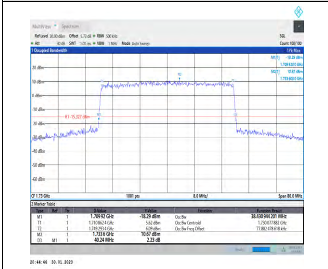
1-N66-PC3-15-40-L-7-CP-16QAM-Outer_Full-216@0-Ant1-38.431-40.240-≤40-PASS
