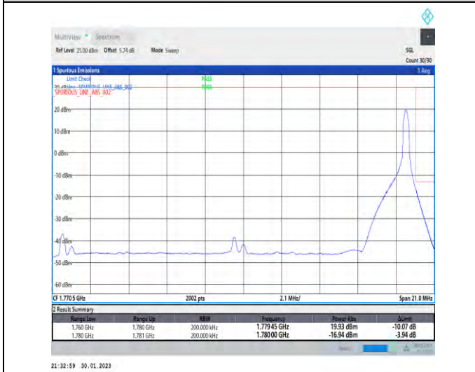
1-N66-PC3-15-20-H-5-CP-QPSK-Edge_1RB_Right-1@105-Ant1-1-seegraph-PASS-see graph
