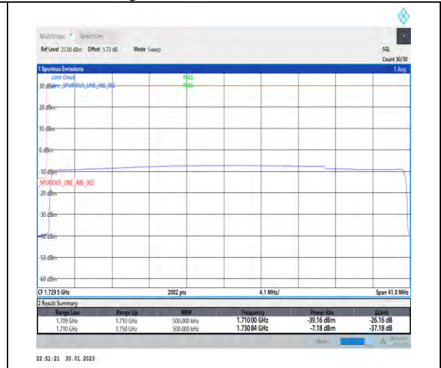
1-N66-PC3-15-40-L-3-DFT-PI2BPSK-Outer_Full-216@0-Ant1-1-seegraph-PASS-see graph
