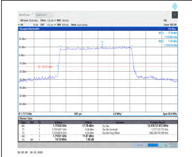
1-N66-PC3-15-15-L-5-DFT-256QAM-Outer_Full-75 @0-Ant1-13.418-14.190-≤15-PASS
