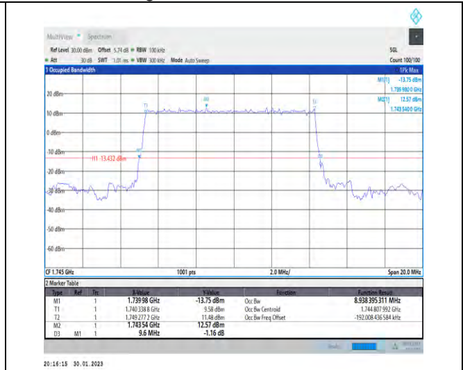
1-N66-PC3-15-10-M-2-DFT-PI2BPSK-Outer_Full-50@0-Ant1-8.938-9.600-≤10-PASS
