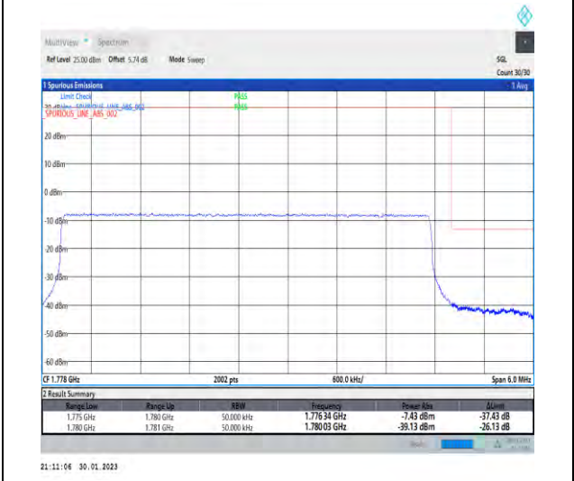
1-N66-PC3-15-5-H-6-CP-QPSK-Outer_Full-25@0-Ant1-1-seegraph-PASS-see graph
