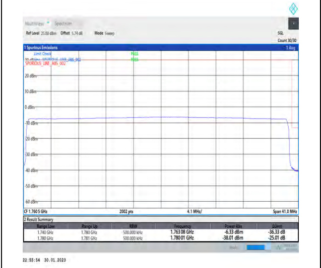
1-N66-PC3-15-40-H-6-CP-QPSK-Outer_Full-216@0-Ant1-1-seegraph-PASS-see graph
