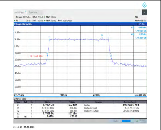
1-N66-PC3-15-10-H-3-DFT-16QAM-Outer_Full-50@ 0-Ant1-8.903-9.600-≤10-PASS
