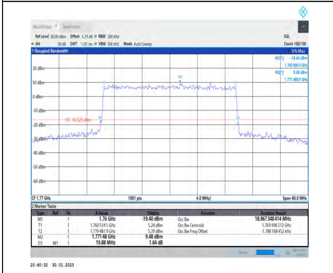
1-N66-PC3-15-20-H-8-CP-64QAM-Outer_Full-106@0 -Ant1-18.967-19.880-≤20-PASS
