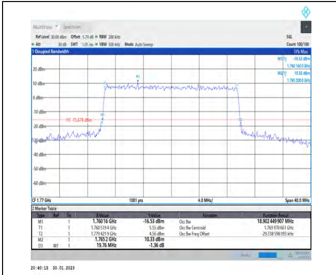
1-N66-PC3-15-20-H-6-CP-QPSK-Outer_Full-106@0 -Ant1-18.902-19.760-≤20-PASS
