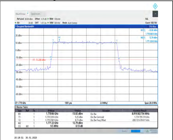
1-N66-PC3-15-10-H-1-DFT-QPSK-Outer_Full-50@0- Ant1-8.919-9.500-≤10-PASS
