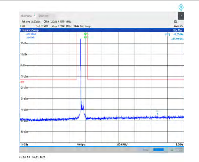
1-N66-PC3-15-40-H-1-DFT-PI2BPSK-Inner_1RB_Lef t-1@1-1000-3000-Ant1-2677.00--45.00--13-PASS
