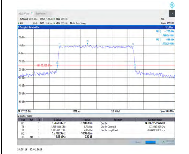
1-N66-PC3-15-15-H-7-CP-16QAM-Outer_Full-79@0 -Ant1-14.067-14.820-≤15-PASS
