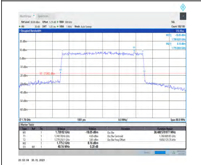
1-N66-PC3-15-40-H-9-CP-256QAM-Outer_Full-216 @0-Ant1-38.481-40.160-≤40-PASS
