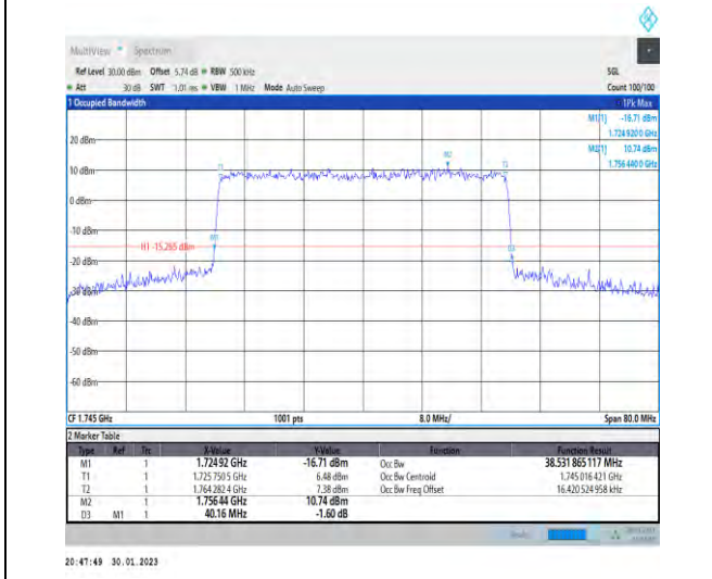
1-N66-PC3-15-40-M-6-CP-QPSK-Outer_Full-216@0-Ant1-38.532-40.160-<math>\leq 40</math>-PASS
