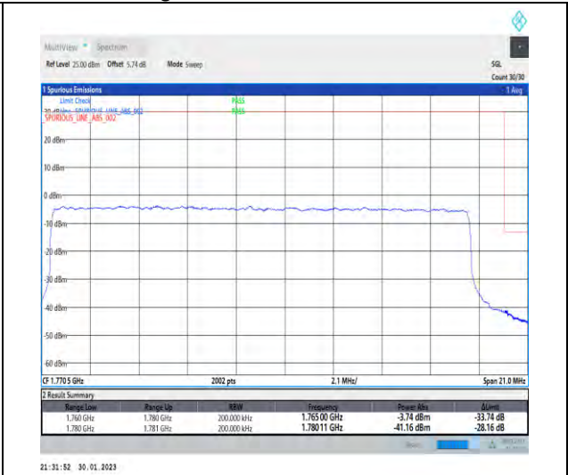
1-N66-PC3-15-20-H-3-DFT-PI2BPSK-Outer_Full-100@0-Ant1-1-seegraph-PASS-see graph
