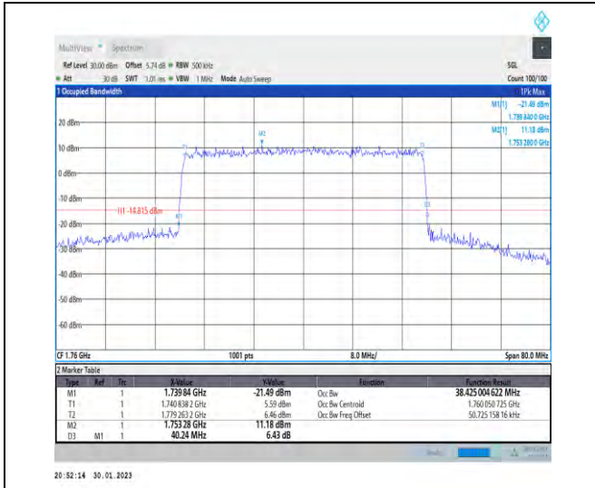
1-N66-PC3-15-40-H-7-CP-16QAM-Outer_Full-216@ 0-Ant1-38.425-40.240-≤40-PASS
