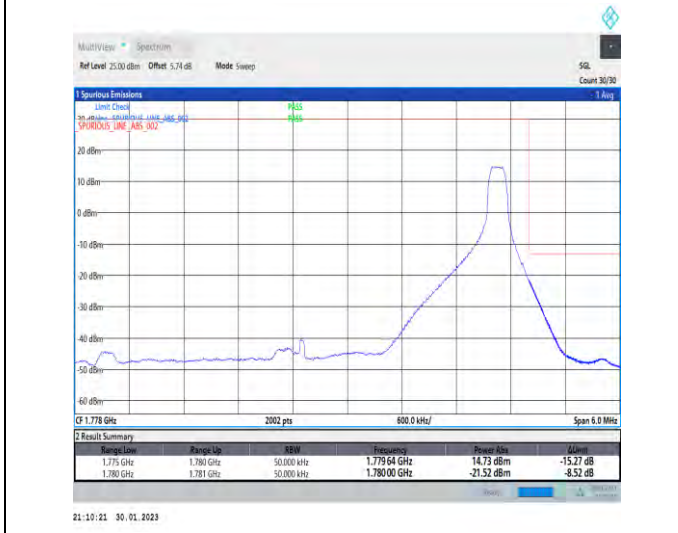
1-N66-PC3-15-5-H-5-CP-QPSK-Edge_1RB_Right-1@24-Ant1-1-seegraph-PASS-see graph
