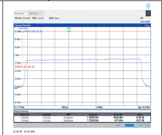
1-N66-PC3-15-15-L-3-DFT-PI2BPSK-Outer_Full-75@0-Ant1-1-seegraph-PASS-see graph
