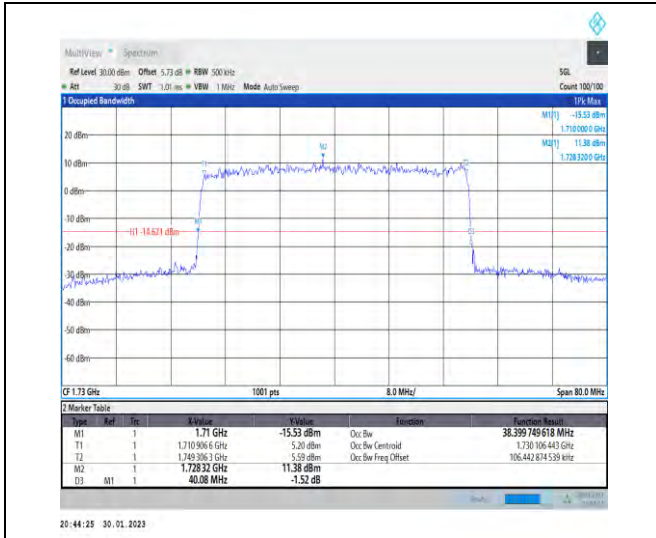
1-N66-PC3-15-40-L-5-DFT-256QAM-Outer_Full-216 @0-Ant1-38.4-40.080-≤40-PASS
