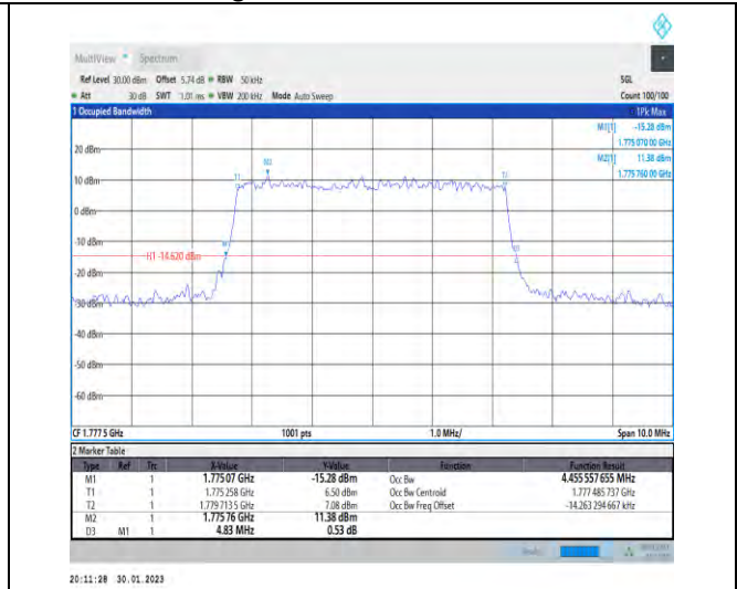
1-N66-PC3-15-5-H-4-DFT-64QAM-Outer_Full-25@0 -Ant1-4.456-4.830-<math>\leq</math>5-PASS
