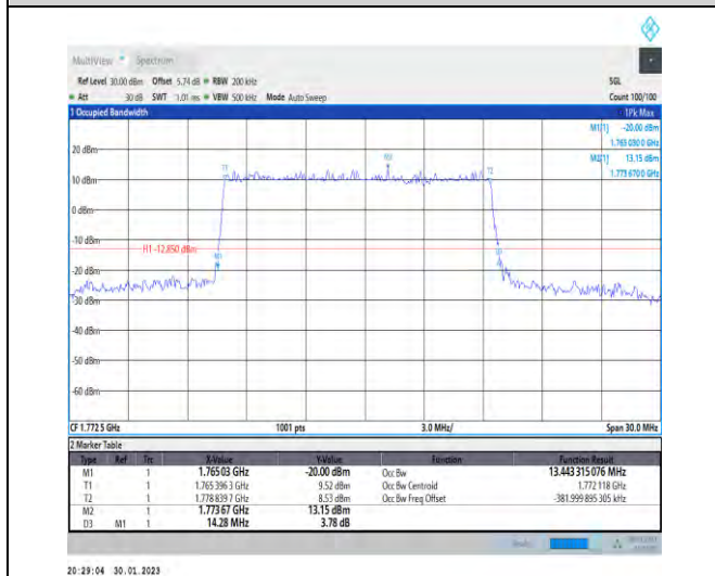
1-N66-PC3-15-15-H-3-DFT-16QAM-Outer_Full-75@0-Ant1-13.443-14.280-≤15-PASS
