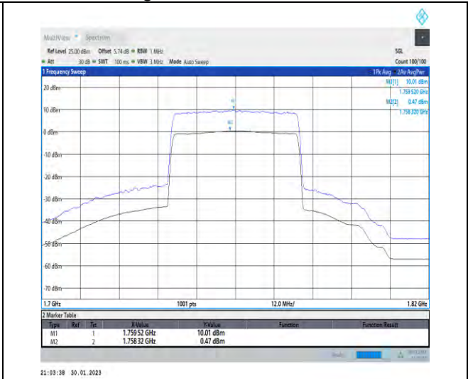
1-N66-PC3-15-40-H-2-CP-256QAM-Outer_Full-216 @0-Ant1-9.54-100%-0.00-9.54-PASS-≤13
