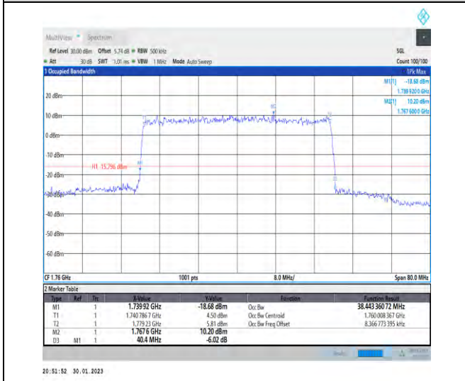
1-N66-PC3-15-40-H-5-DFT-256QAM-Outer_Full-216 @0-Ant1-38.443-40.400-≤40-PASS
