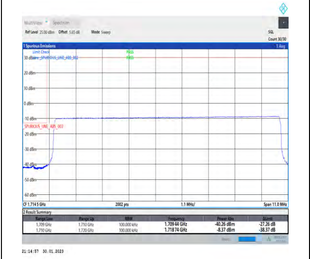
1-N66-PC3-15-10-L-6-CP-QPSK-Outer_Full-52@0-Ant1-1-seegraph-PASS-see graph
