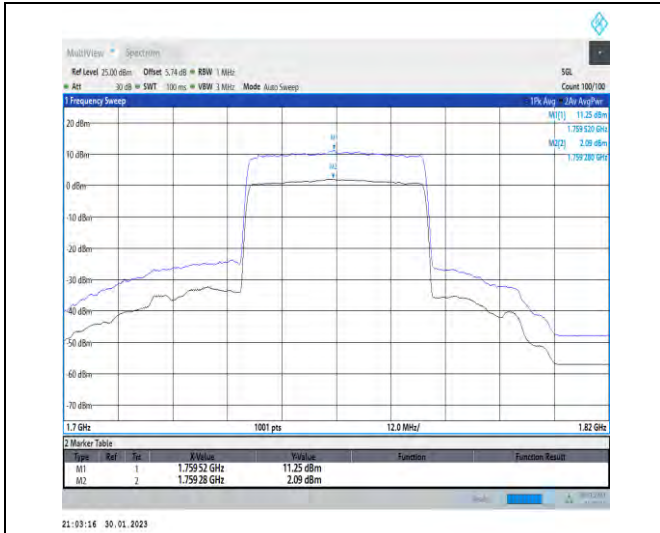
1-N66-PC3-15-40-H-1-DFT-256QAM-Outer_Full-216 @0-Ant1-9.16-100%-0.00-9.16-PASS-≤13
