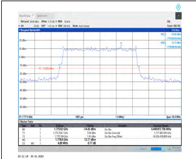
1-N66-PC3-15-5-H-3-DFT-16QAM-Outer_Full-25@0 -Ant1-4.45-4.890-<math>\leq</math>5-PASS
