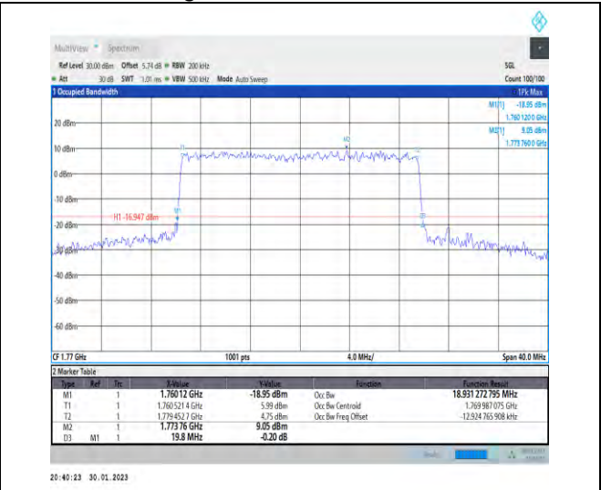
1-N66-PC3-15-20-H-7-CP-16QAM-Outer_Full-106@0 -Ant1-18.931-19.800-≤20-PASS
