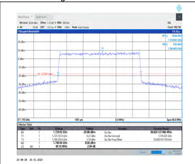
1-N66-PC3-15-40-M-9-CP-256QAM-Outer_Full-216 @0-Ant1-38.603-40.160-≤40-PASS
