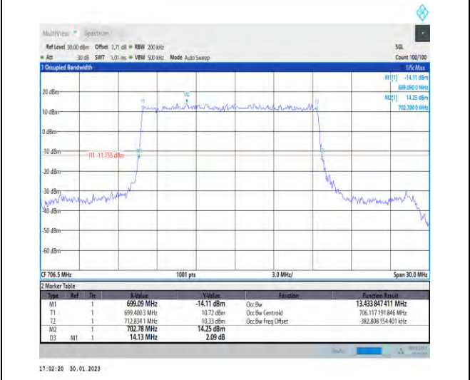
1-N12-PC3-15-15-L-2-DFT-PI2BPSK-Outer_Full-75@0- Ant1-13.434-14.130-≤15-PASS
