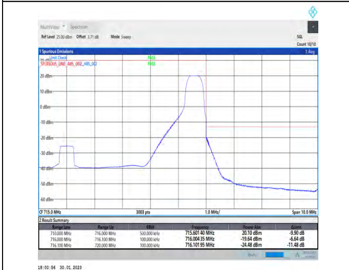
1-N12-PC3-15-10-H-5-CP-QPSK-Edge_1RB_Right-1@51-Ant1-1--PASS-see graph
