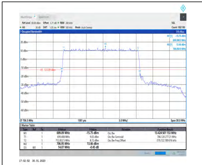
1-N12-PC3-15-15-L-3-DFT-16QAM-Outer_Full-75@ 0-Ant1-13.425-14.070-≤15-PASS
