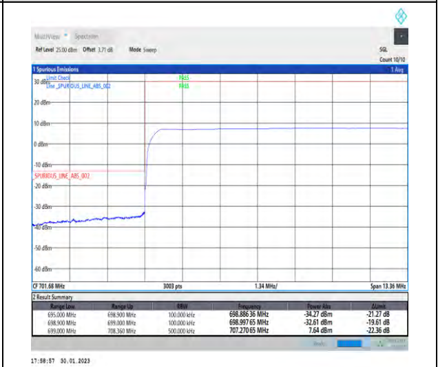
1-N12-PC3-15-10-L-6-CP-QPSK-Outer_Full-52@0-Ant1-1--PASS-see graph
