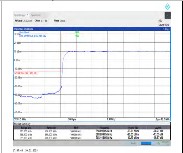
1-N12-PC3-15-10-L-3-DFT-PI2BPSK-Outer_Full-50@0-Ant1-1--PASS-see graph
