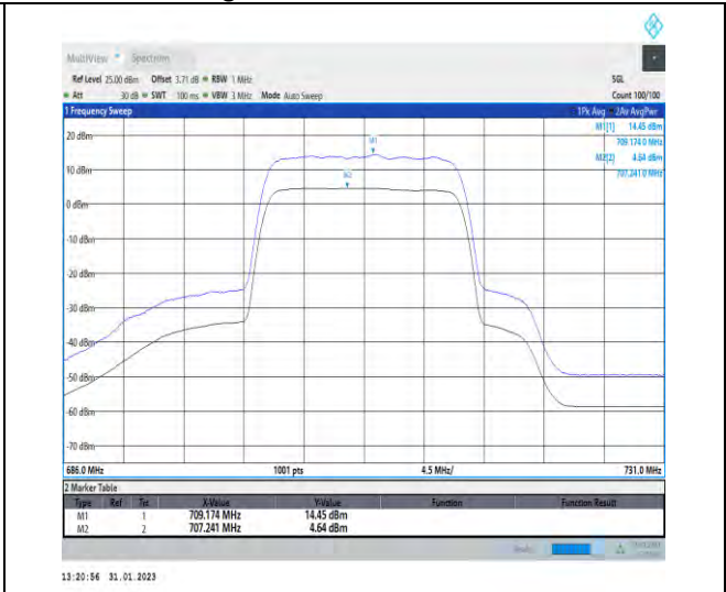
1-N12-PC3-15-15-H-2-CP-256QAM-Outer_Full-79@ 0-Ant1-9.81-100%-0.00-9.81-PASS-≤13
