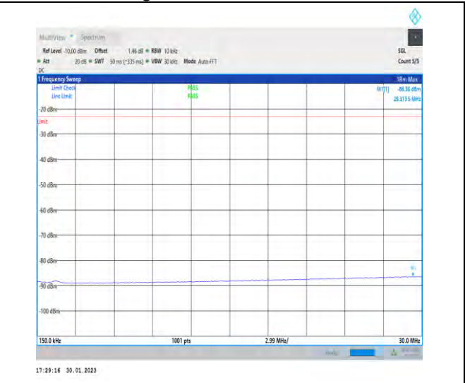
1-N12-PC3-15-15-H-1-DFT-PI2BPSK-Inner_1RB_Lef t-1@1-0.15-30-Ant1-29.31--86.36--23-PASS
