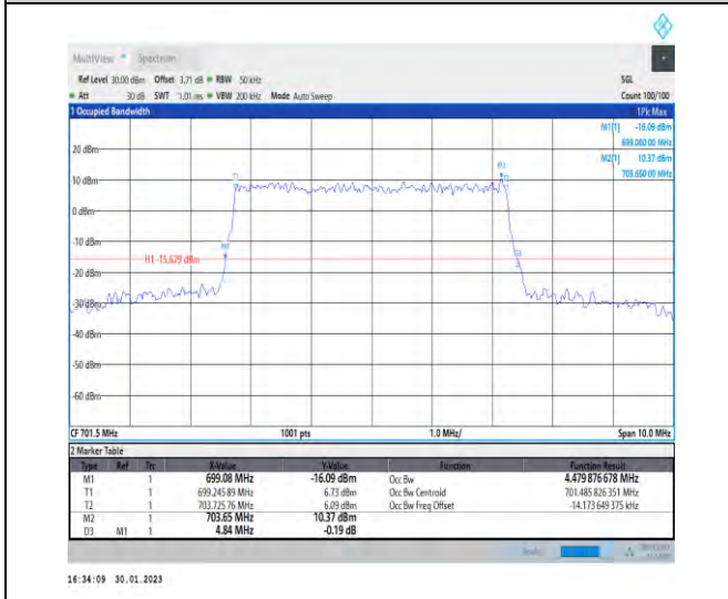
1-N12-PC3-15-5-L-7-CP-16QAM-Outer_Full-25@0-Ant1-4.48-4.840-≤5-PASS
