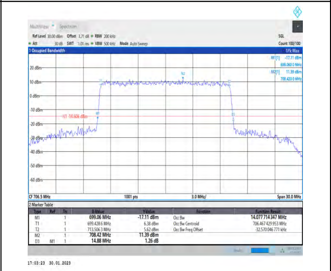
1-N12-PC3-15-15-L-6-CP-QPSK-Outer_Full-79@0- Ant1-14.078-14.880-≤15-PASS
