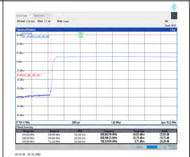
1-N12-PC3-15-15-L-6-CP-QPSK-Outer_Full-79@0-Ant1-1--PASS-see graph
