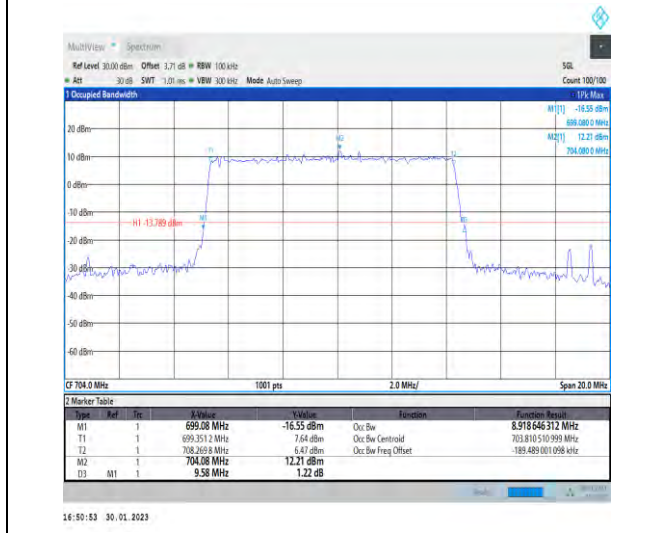
1-N12-PC3-15-10-L-4-DFT-64QAM-Outer_Full-50 @0-Ant1-8.919-9.580-≤10-PASS
