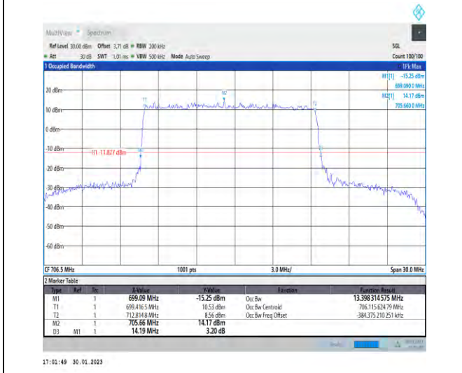
1-N12-PC3-15-15-L-1-DFT-QPSK-Outer_Full-75@0- Ant1-13.398-14.190-≤15-PASS
