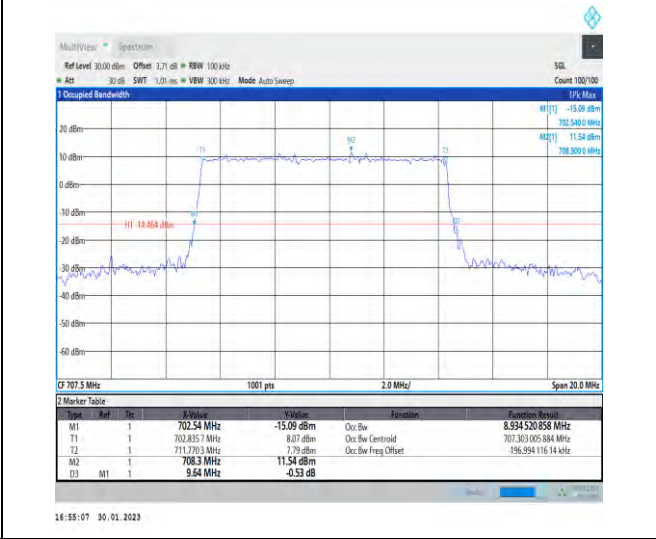
1-N12-PC3-15-10-M-4-DFT-64QAM-Outer_Full-50@0-Ant1-8.935-9.640-≤10-PASS
