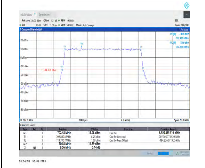
1-N12-PC3-15-10-M-3-DFT-16QAM-Outer_Full-50@0-Ant1-8.93-9.560-≤10-PASS
