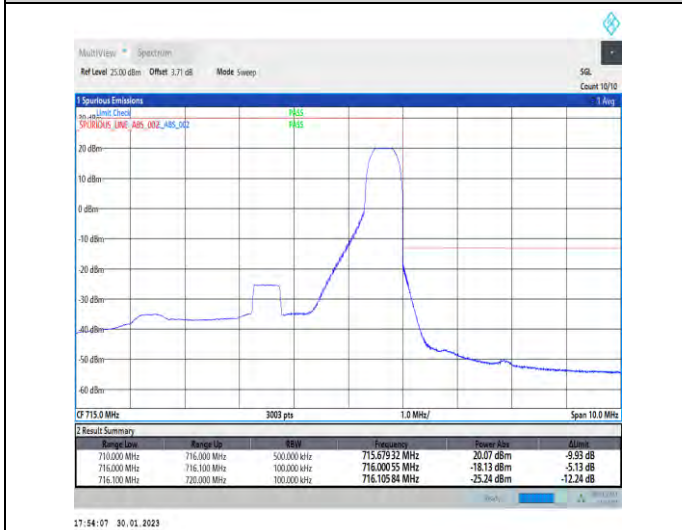
1-N12-PC3-15-5-H-5-CP-QPSK-Edge_1RB_Right-1@24-Ant1-1--PASS-see graph
