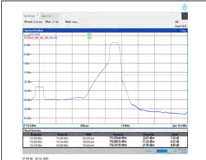
1-N12-PC3-15-10-H-2-DFT-PI2BPSK-Edge_1RB_Right-t-1@51-Ant1-1--PASS-see graph
