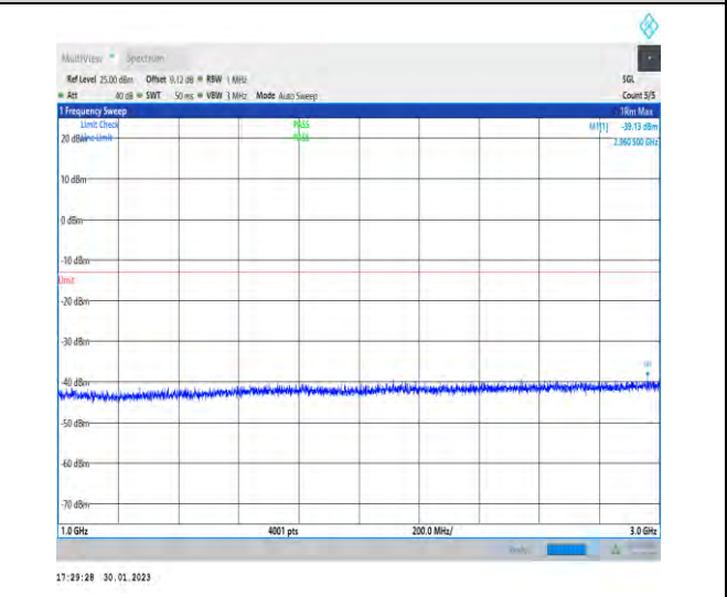
1-N12-PC3-15-15-H-1-DFT-PI2BPSK-Inner_1RB_Lef t-1@1-1000-3000-Ant1-2960.50--39.13--13-PASS
