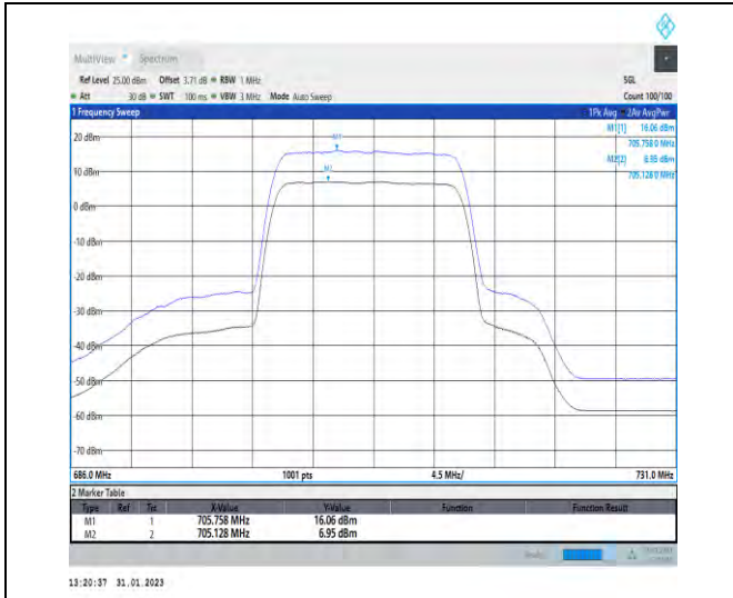
1-N12-PC3-15-15-H-1-DFT-256QAM-Outer_Full-75 @0-Ant1-9.11-100%-0.00-9.11-PASS-≤13
