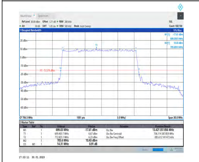
1-N12-PC3-15-15-L-5-DFT-256QAM-Outer_Full-75 @0-Ant1-13.421-14.310-≤15-PASS
