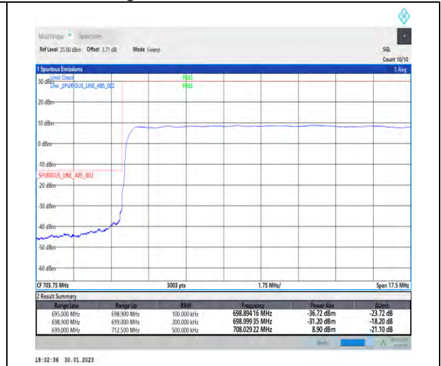
1-N12-PC3-15-15-L-3-DFT-PI2BPSK-Outer_Full-75@0-Ant1-1--PASS-see graph
