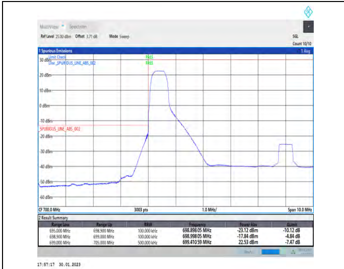
1-N12-PC3-15-10-L-1-DFT-PI2BPSK-Edge_1RB_Left-1@0-Ant1-1--PASS-see graph
