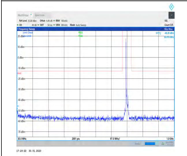
1-N12-PC3-15-15-H-1-DFT-PI2BPSK-Inner_1RB_L eft-1@1-30-1000-Ant1-30.97--49.29--13-PASS
