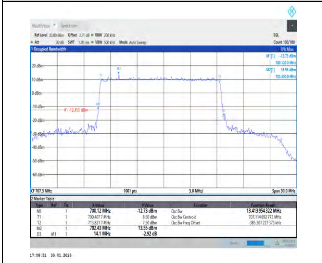
1-N12-PC3-15-15-M-4-DFT-64QAM-Outer_Full-75 @0-Ant1-13.414-14.100-≤15-PASS
