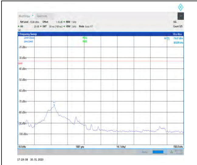
1-N12-PC3-15-15-H-1-DFT-PI2BPSK-Inner_1RB_L eft-1@1-0.009-0.15-Ant1-0.04--74.47--33-PASS
