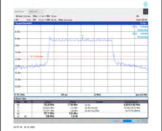
1-N12-PC3-15-10-M-8-CP-64QAM-Outer_Full-52@0-Ant1-9.284-9.860-≤10-PASS
