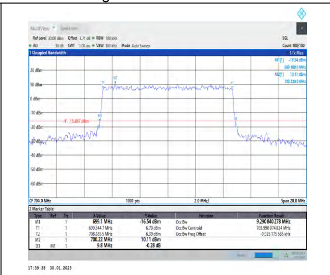
1-N12-PC3-15-10-L-7-CP-16QAM-Outer_Full-52@0-0 Ant1-9.291-9.800-≤10-PASS
