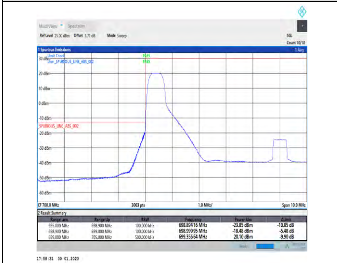
1-N12-PC3-15-10-L-4-CP-QPSK-Edge_1RB_Left-1@0-Ant1-1--PASS-see graph
