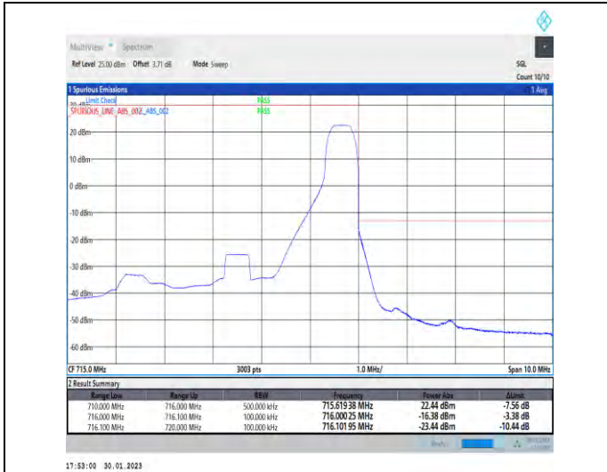
1-N12-PC3-15-5-H-2-DFT-PI2BPSK-Edge_1RB_Right-1@24-Ant1-1--PASS-see graph
