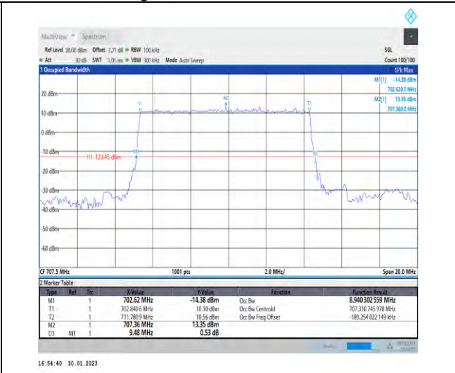
1-N12-PC3-15-10-M-2-DFT-PI2BPSK-Outer_Full-50@0-Ant1-8.94-9.480-≤10-PASS
