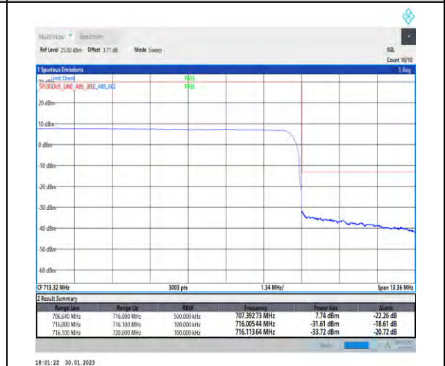
1-N12-PC3-15-10-H-6-CP-QPSK-Outer_Full-52@0-Ant1-1--PASS-see graph
