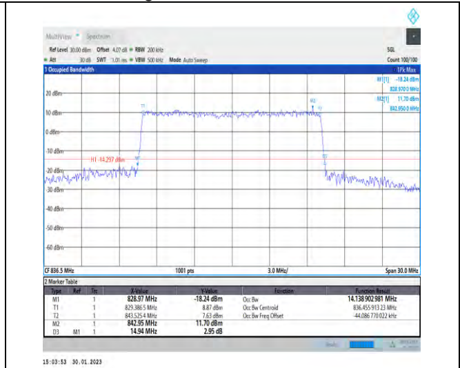
1-N5-PC3-15-15-M-7-CP-16QAM-Outer_Full-79@0- Ant1-14.139-14.940-≤15-PASS
