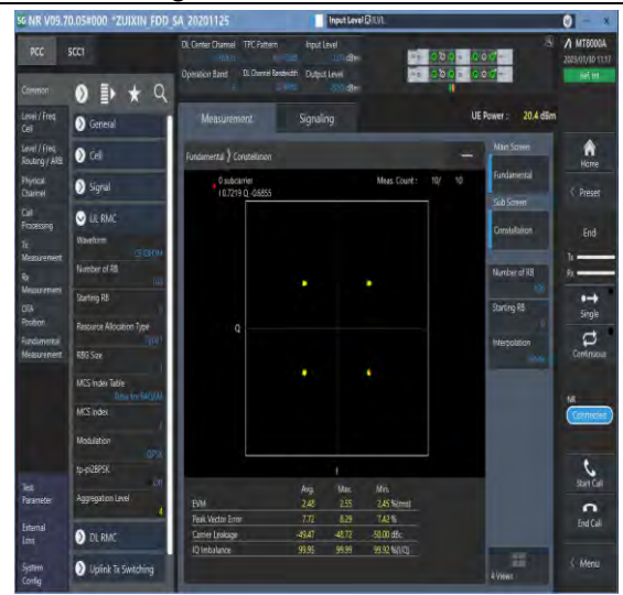
1-N5-PC3-15-20-M-6-CP-QPSK-Outer_Full-106@0-Ant1-see graph-PASS
