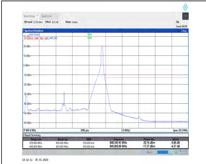
1-N5-PC3-15-10-H-2-DFT-PI2BPSK-Edge_1RB_Right-1@51-Ant1-1-seegraph-PASS-see graph
