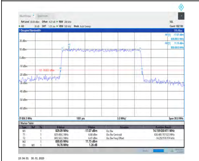
1-N5-PC3-15-15-M-8-CP-64QAM-Outer_Full-79@0- Ant1-14.159-14.760-≤15-PASS
