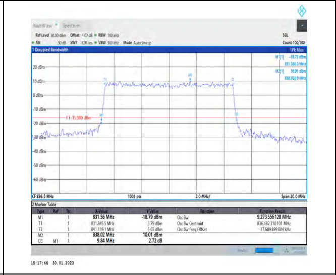
1-N5-PC3-15-10-M-8-CP-64QAM-Outer_Full-52@0-Ant1-9.274-9.840-≤10-PASS
