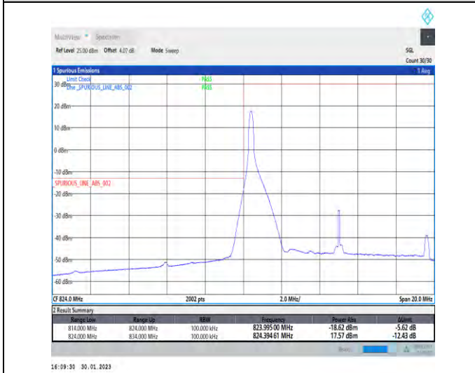
1-N5-PC3-15-10-L-4-CP-QPSK-Edge_1RB_Left-1@0-Ant1-1-seegraph-PASS-see graph
