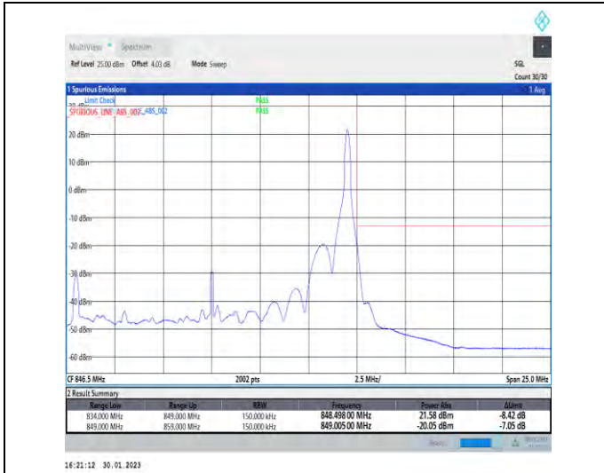
1-N5-PC3-15-15-H-2-DFT-PI2BPSK-Edge_1RB_Right-1@78-Ant1-1-seegraph-PASS-see graph
