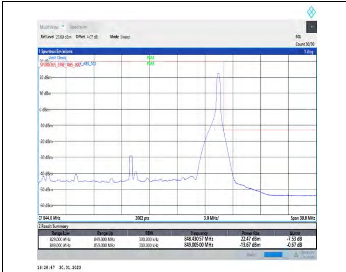
1-N5-PC3-15-20-H-2-DFT-PI2BPSK-Edge_1RB_Right-1@105-Ant1-1-seegraph-PASS-see graph
