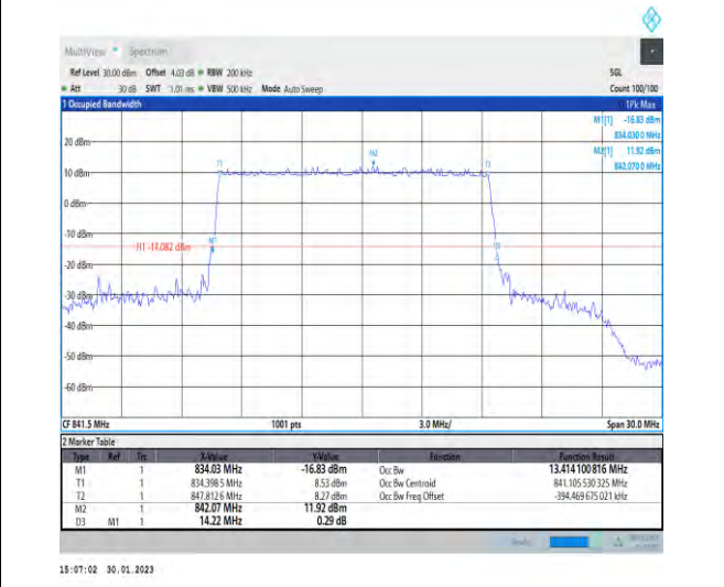
1-N5-PC3-15-15-H-4-DFT-64QAM-Outer_Full-75@0-Ant1-13.414-14.220-≤15-PASS
