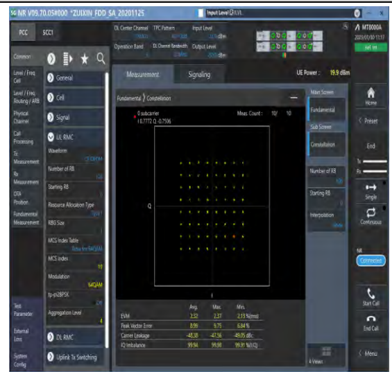
1-N5-PC3-15-20-M-8-CP-64QAM-Outer_Full-106@0-Ant1-see graph-PASS
