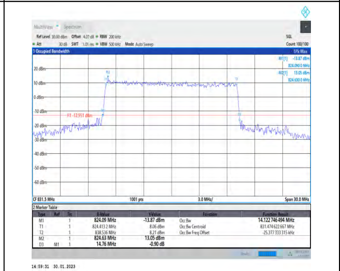
1-N5-PC3-15-15-L-6-CP-QPSK-Outer_Full-79@0-Ant1-14.123-14.760-≤15-PASS
