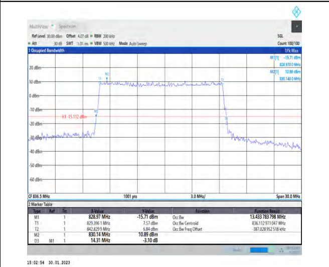
1-N5-PC3-15-15-M-5-DFT-256QAM-Outer_Full-75@0-Ant1-13.434-14.310-≤15-PASS
