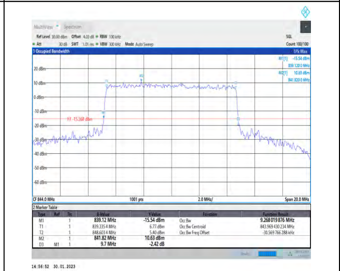
1-N5-PC3-15-10-H-7-CP-16QAM-Outer_Full-52@0- Ant1-9.268-9.700-≤10-PASS
