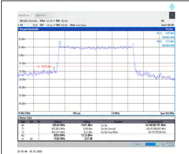
1-N5-PC3-15-15-M-6-CP-QPSK-Outer_Full-79@0-A Ant1-14.141-14.820-≤15-PASS
