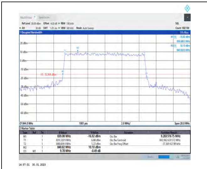
1-N5-PC3-15-10-H-8-CP-64QAM-Outer_Full-52@0-Ant1-9.284-9.780-≤10-PASS
