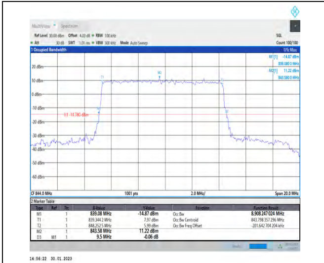
1-N5-PC3-15-10-H-4-DFT-64QAM-Outer_Full-50@0 -Ant1-8.908-9.500-≤10-PASS
