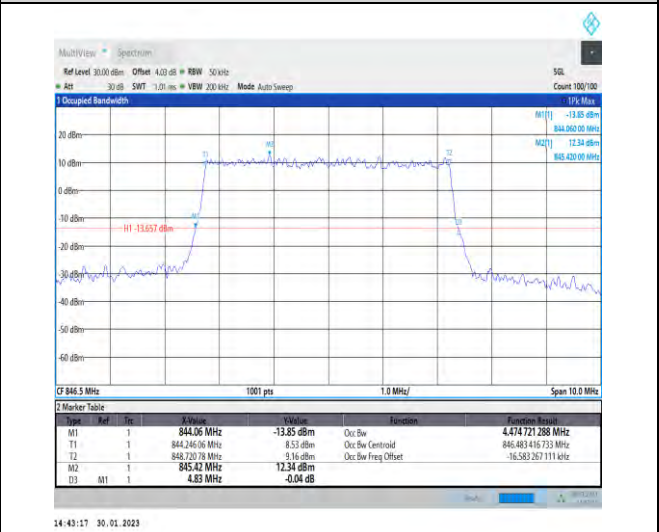
1-N5-PC3-15-5-H-2-DFT-PI2BPSK-Outer_Full-25@0-A -Ant1-4.475-4.830-≤5-PASS
