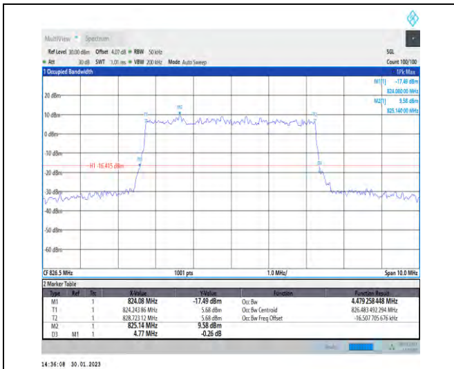
1-N5-PC3-15-5-L-5-DFT-256QAM-Outer_Full-25@0-Ant1-4.479-4.770-≤5-PASS
