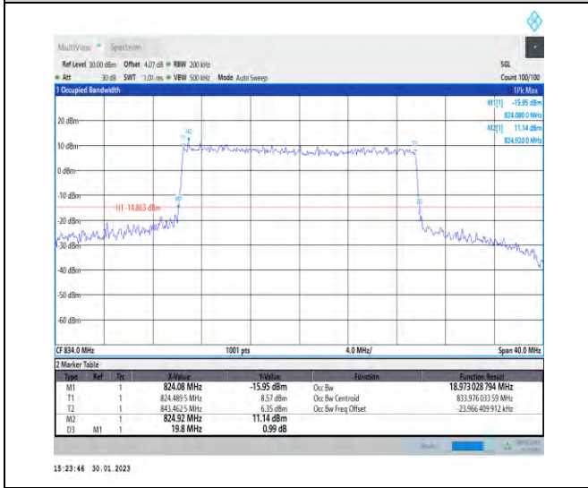
1-N5-PC3-15-20-L-6-CP-QPSK-Outer_Full-106@0-Ant1-18.973-19.800-<math>\leq 20</math>-PASS
