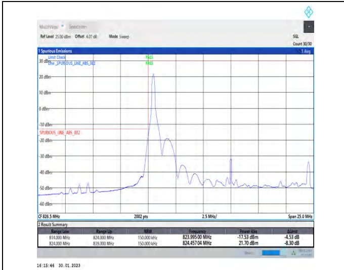
1-N5-PC3-15-15-L-1-DFT-PI2BPSK-Edge_1RB_Left-1 @0-Ant1-1-seegraph-PASS-see graph
