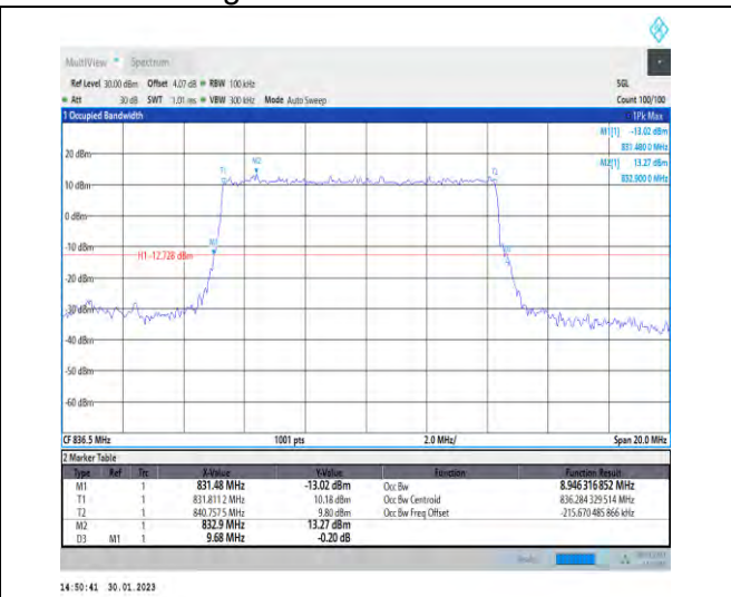
1-N5-PC3-15-10-M-2-DFT-PI2BPSK-Outer_Full-50@0-Ant1-8.946-9.680-≤10-PASS
