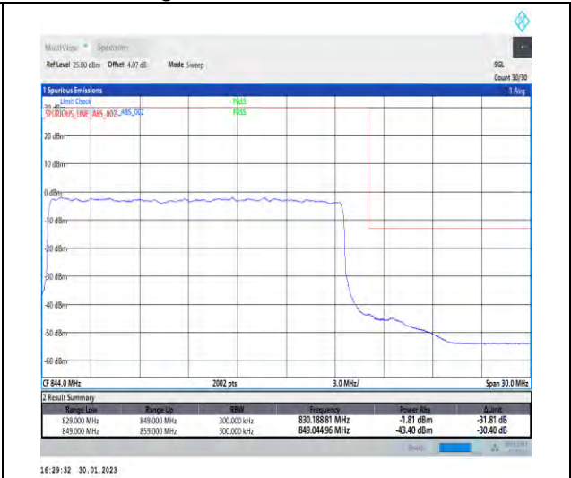
1-N5-PC3-15-20-H-3-DFT-PI2BPSK-Outer_Full-100@0-Ant1-1-seegraph-PASS-see graph
