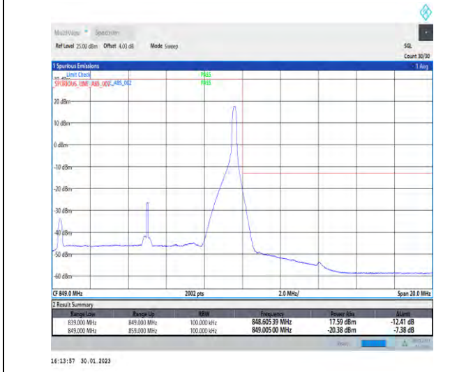
1-N5-PC3-15-10-H-5-CP-QPSK-Edge_1RB_Right-1@51-Ant1-1-seegraph-PASS-see graph
