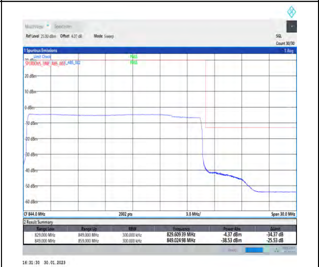
1-N5-PC3-15-20-H-6-CP-QPSK-Outer_Full-106@0-Ant1-1-seegraph-PASS-see graph
