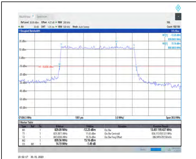
1-N5-PC3-15-15-M-2-DFT-PI2BPSK-Outer_Full-75 @0-Ant1-13.451-14.190-≤15-PASS
