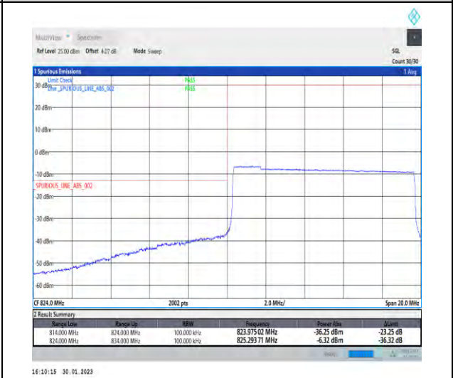
1-N5-PC3-15-10-L-6-CP-QPSK-Outer_Full-52@0-Ant1-1-seegraph-PASS-see graph
