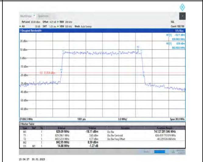
1-N5-PC3-15-15-M-9-CP-256QAM-Outer_Full-79@0- -Ant1-14.127-14.880-≤15-PASS
