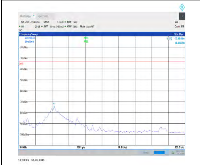
1-N5-PC3-15-20-H-1-DFT-PI2BPSK-Inner_1RB_Left -1@1-0.009-0.15-Ant1-0.04--75.19--33-PASS
