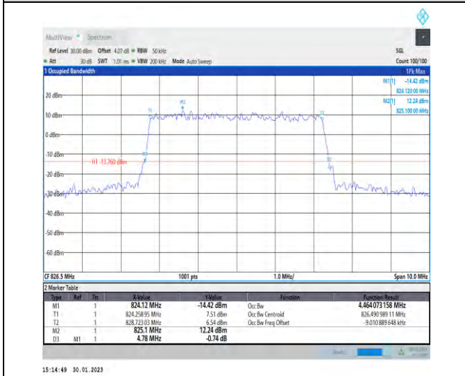
1-N5-PC3-15-5-L-7-CP-16QAM-Outer_Full-25@0-A nt1-4.464-4.780-≤5-PASS
