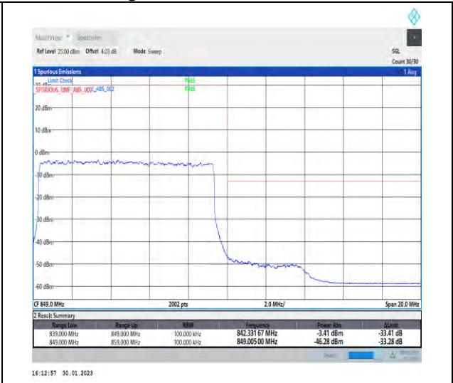
1-N5-PC3-15-10-H-3-DFT-PI2BPSK-Outer_Full-50@0-Ant1-1-seegraph-PASS-see graph
