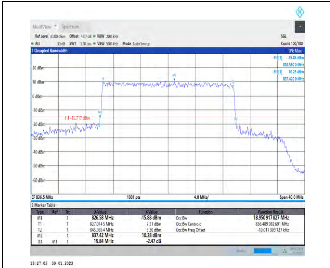
1-N5-PC3-15-20-M-7-CP-16QAM-Outer_Full-106@0 -Ant1-18.951-19.840-≤20-PASS
