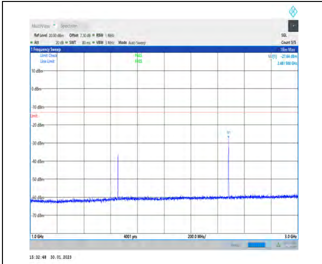
1-N5-PC3-15-20-M-1-DFT-PI2BPSK-Inner_1RB_Left -1@1-1000-3000-Ant1-2481.50--27.64--13-PASS
