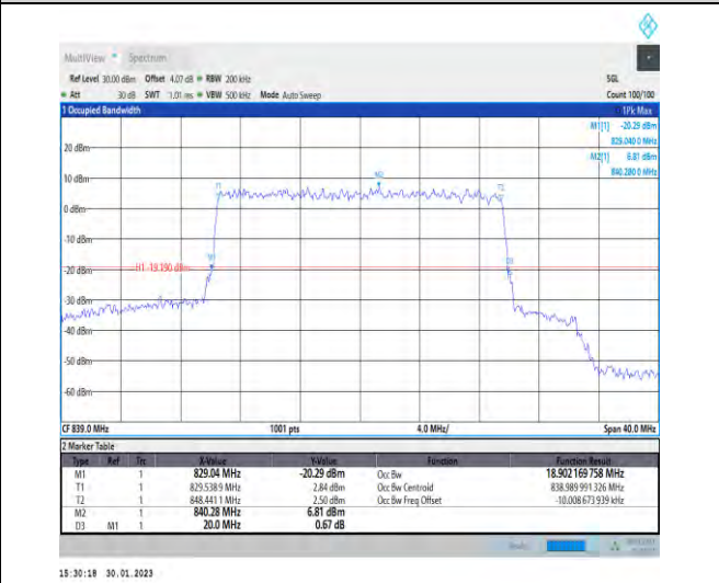
1-N5-PC3-15-20-H-9-CP-256QAM-Outer_Full-106@0-Ant1-18.902-20.000-<=20-PASS
