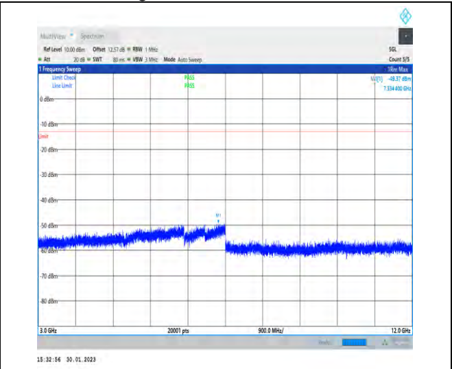
1-N5-PC3-15-20-M-1-DFT-PI2BPSK-Inner_1RB_Left -1@1-3000-12000-Ant1-7334.40--49.37--13-PASS
