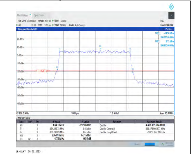
1-N5-PC3-15-5-M-9-CP-256QAM-Outer_Full-25@0-A Ant1-4.466-4.780-≤5-PASS
