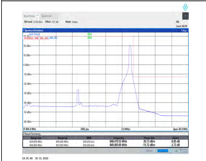
1-N5-PC3-15-20-H-5-CP-QPSK-Edge_1RB_Right-1@105-Ant1-1-seegraph-PASS-see graph
