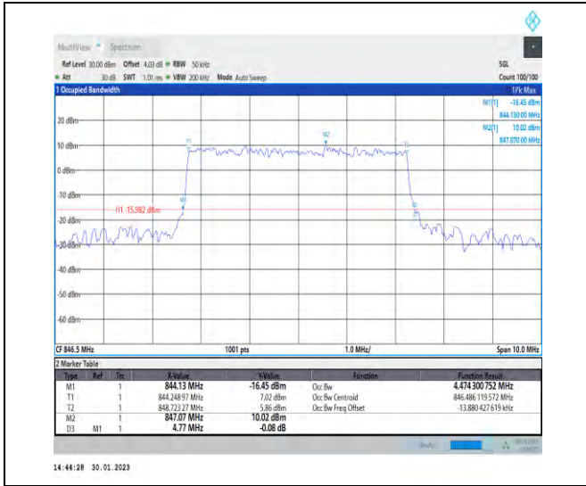
1-N5-PC3-15-5-H-7-CP-16QAM-Outer_Full-25@0-A nt1-4.474-4.770-≤5-PASS
