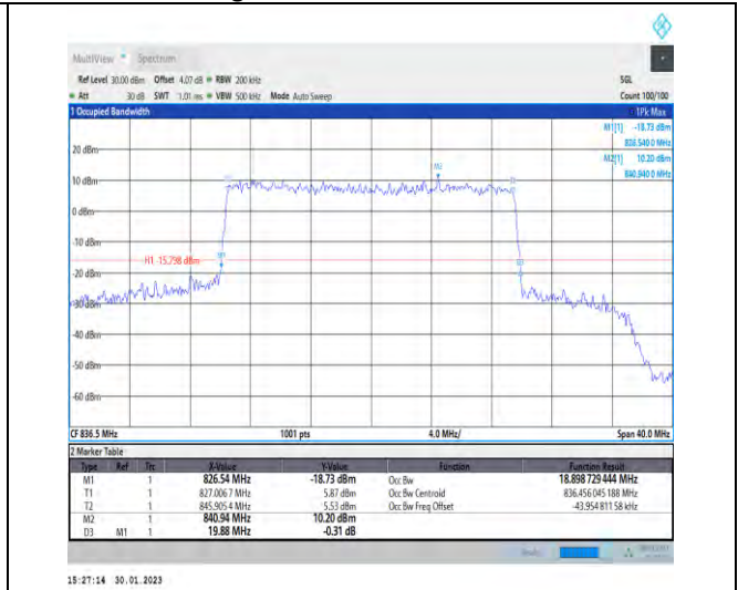
1-N5-PC3-15-20-M-8-CP-64QAM-Outer_Full-106@0 -Ant1-18.899-19.880-≤20-PASS
