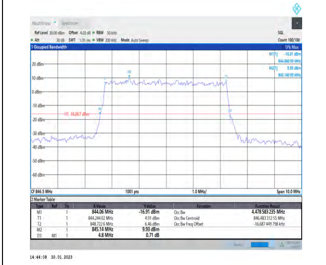
1-N5-PC3-15-5-H-5-DFT-256QAM-Outer_Full-25@0-Ant1-4.479-4.800-≤5-PASS
