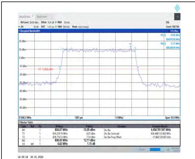
1-N5-PC3-15-5-M-4-DFT-64QAM-Outer_Full-25@0-Ant1-4.457-4.820-≤5-PASS
