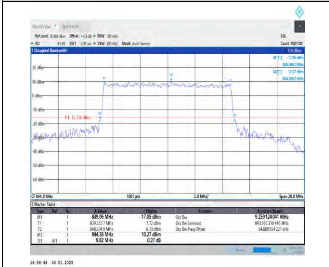
1-N5-PC3-15-10-H-6-CP-QPSK-Outer_Full-52@0-A nt1-9.259-9.820-≤10-PASS
