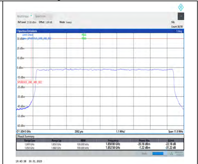
1-N2-PC3-15-10-L-3-DFT-PI2BPSK-Outer_Full-50 @0-Ant1-1-seegraph-PASS-see graph
