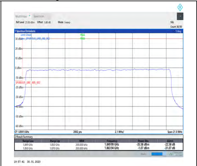
1-N2-PC3-15-20-L-3-DFT-PI2BPSK-Outer_Full-10 0@0-Ant1-1-seegraph-PASS-see graph
