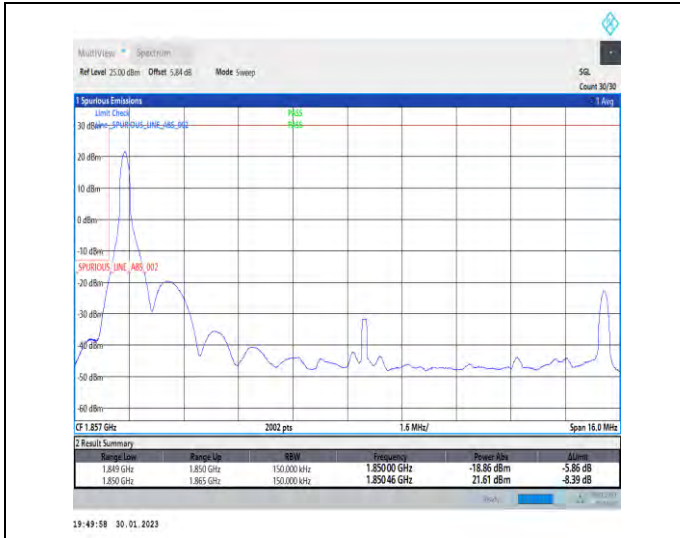
1-N2-PC3-15-15-L-1-DFT-PI2BPSK-Edge_1RB_Left-1 @0-Ant1-1-seegraph-PASS-see graph
