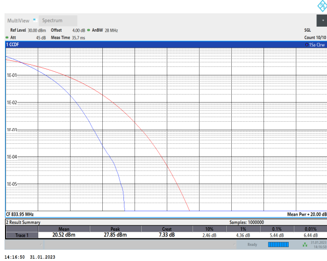
5-5-10MHz-10MHz-QPSK-QPSK-20476-20575-50RB#0-50RB#0
