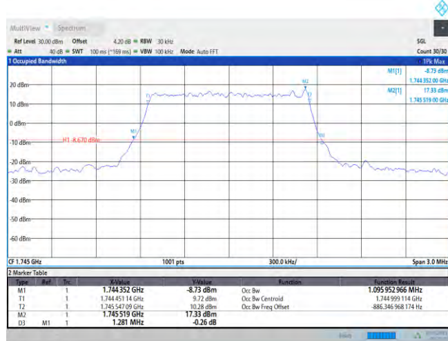
Band66-1.4MHz-QPSK-132322-6RB#0
