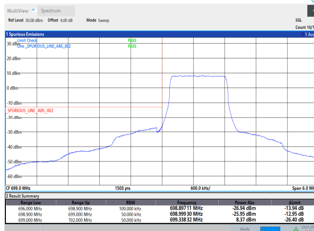
Band12-1.4MHz-QPSK-23017-6RB#0
