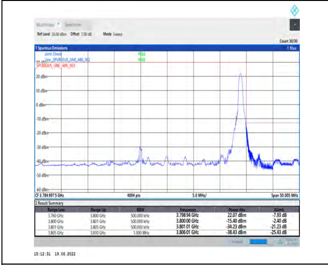
1-N78-3700-3800-PC2-30-40-H-5-CP-QPSK-Edge_1RB_Right-1@105-Ant1-PASS-see graph
