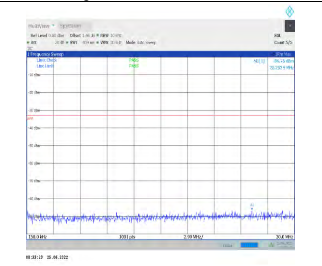
1-N78-3700-3800-PC2-30-100-H-1-DFT-PI2BPSK-In ner_1RB_Left-1@1-0.15-30-Ant1--86.76--33-PASS
