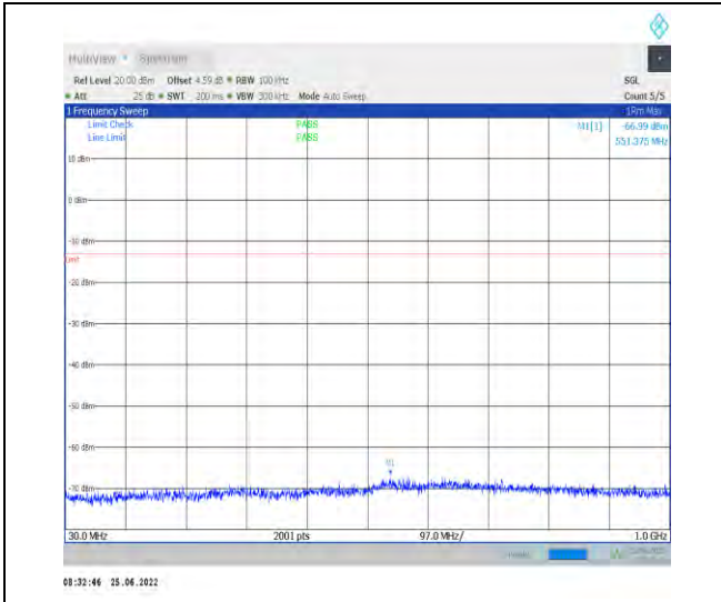
1-N78-3700-3800-PC2-30-100-M-1-DFT-PI2BPSK- Inner_1RB_Left-1@1-30-1000-Ant1--66.99--13-PAS S
