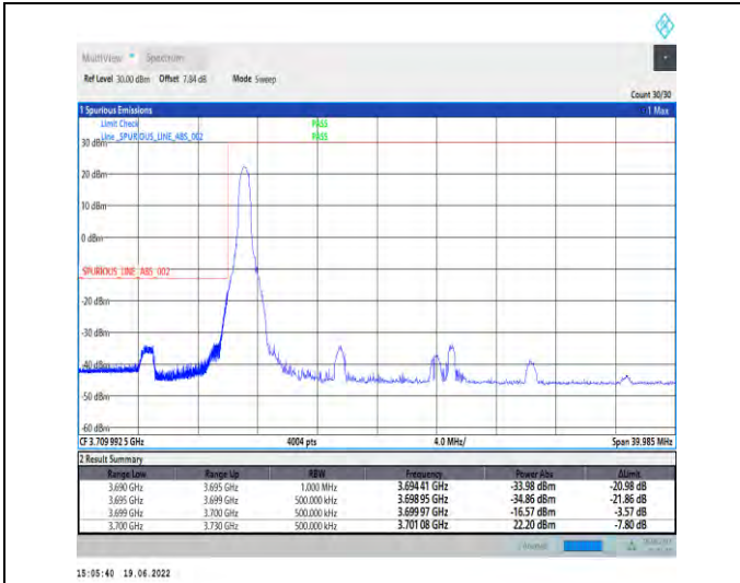
1-N78-3700-3800-PC2-30-30-L-1-DFT-PI2BPSK-Edge_1RB_Left-1@0-Ant1-PASS-see graph
