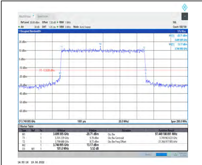
1-N78-3700-3800-PC2-30-100-H-7-CP-16QAM-Outer_Full-273@0-Ant1-97.449-101.000-≤100-PASS
