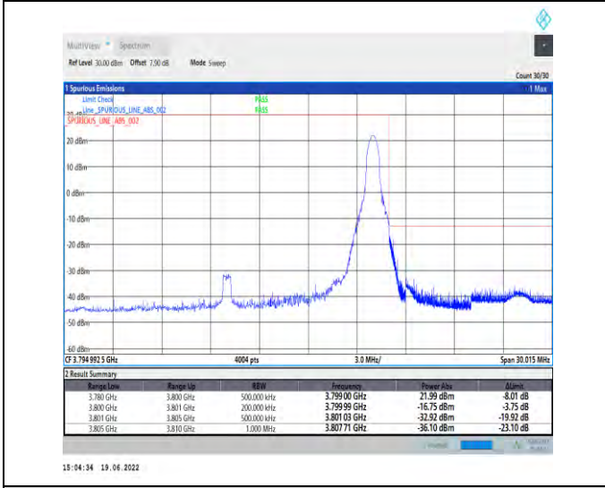
1-N78-3700-3800-PC2-30-20-H-5-CP-QPSK-Edge_1RB_Right-1@50-Ant1-PASS-see graph
