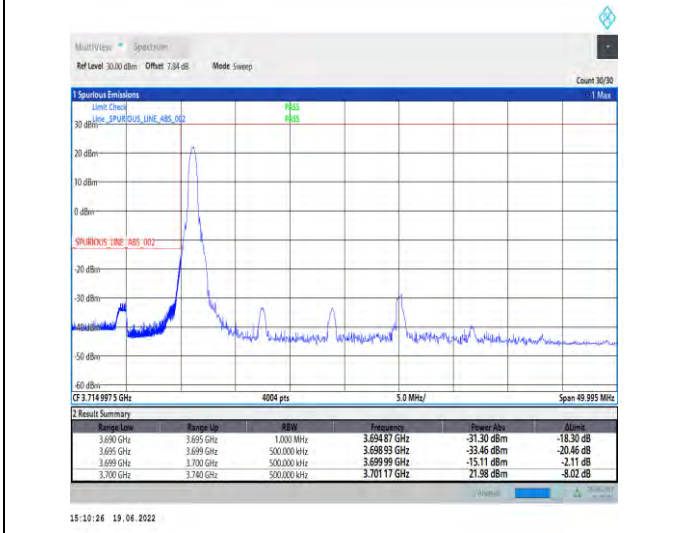
1-N78-3700-3800-PC2-30-40-L-4-CP-QPSK-Edge_1RB_Left-1@0-Ant1-PASS-see graph
