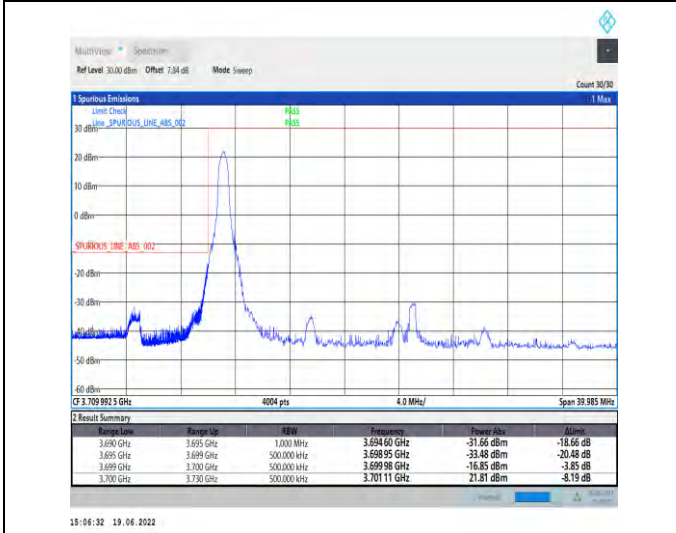
1-N78-3700-3800-PC2-30-30-L-4-CP-QPSK-Edge_1RB_Left-1@0-Ant1-PASS-see graph
