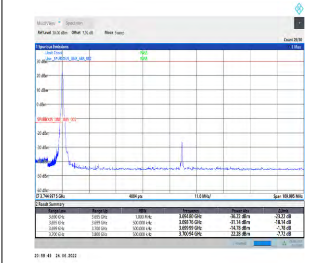
1-N78-3700-3800-PC2-30-100-L-4-CP-QPSK-Edge_1RB_Left-1@0-Ant1-PASS-see graph
