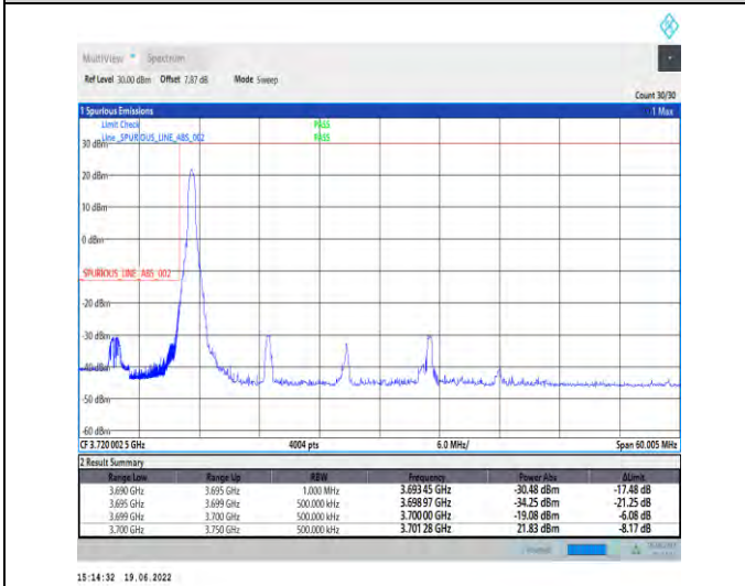
1-N78-3700-3800-PC2-30-50-L-4-CP-QPSK-Edge_1RB_Left-1@0-Ant1-PASS-see graph
