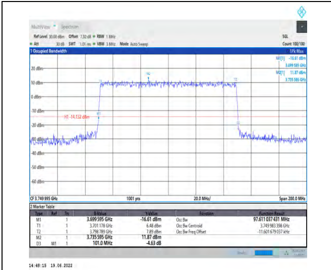
1-N78-3700-3800-PC2-30-100-M-8-CP-64QAM-Out er_Full-273@0-Ant1-97.611-101.000-≤100-PASS
