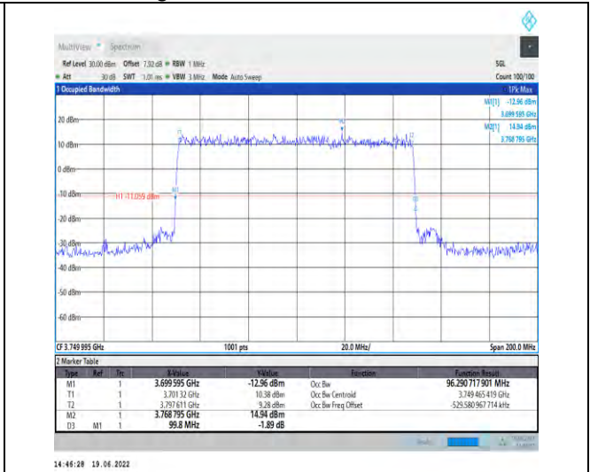
1-N78-3700-3800-PC2-30-100-M-1-DFT-QPSK-Outer_Full-270@0-Ant1-96.291-99.800-≤100-PASS
