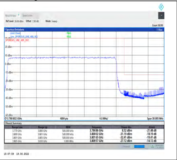
1-N78-3700-3800-PC2-30-30-H-3-DFT-PI2BPSK-Outer_Full-75@0-Ant1-PASS-see graph
