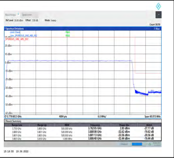
1-N78-3700-3800-PC2-30-50-H-6-CP-QPSK-Outer_Full-133@0-Ant1-PASS-see graph
