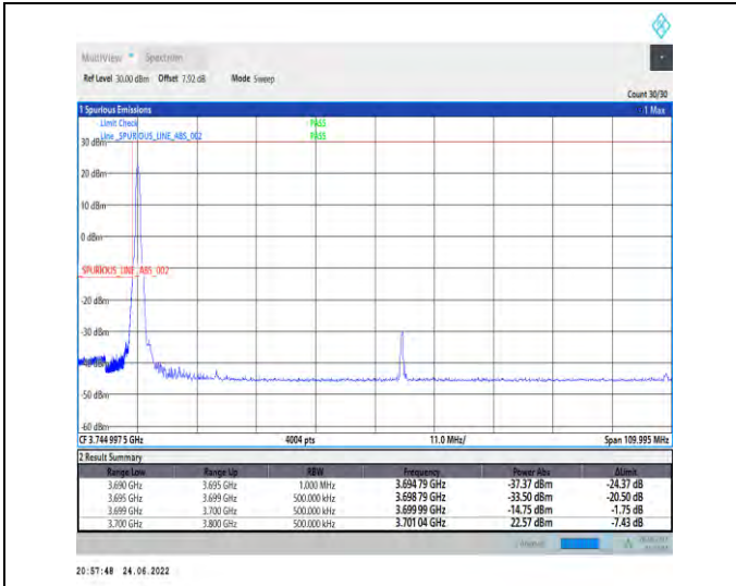
1-N78-3700-3800-PC2-30-100-L-1-DFT-PI2BPSK-Edge_1RB_Left-1@0-Ant1-PASS-see graph
