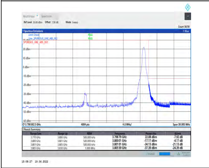
1-N78-3700-3800-PC2-30-30-H-5-CP-QPSK-Edge_1RB_Right-1@77-Ant1-PASS-see graph
