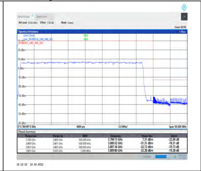
1-N78-3700-3800-PC2-30-40-H-3-DFT-PI2BPSK-Outer_Full-100@0-Ant1-PASS-see graph
