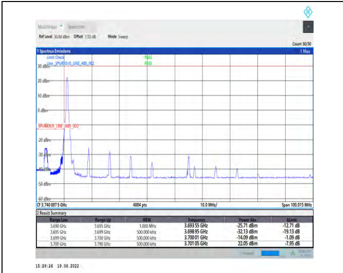
1-N78-3700-3800-PC2-30-90-L-1-DFT-PI2BPSK-Edge_1RB_Left-1@0-Ant1-PASS-see graph
