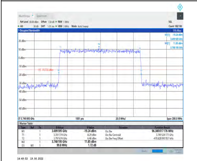
1-N78-3700-3800-PC2-30-100-H-5-DFT-256QAM-Out er_Full-270@0-Ant1-96.3-99.800-≤100-PASS
