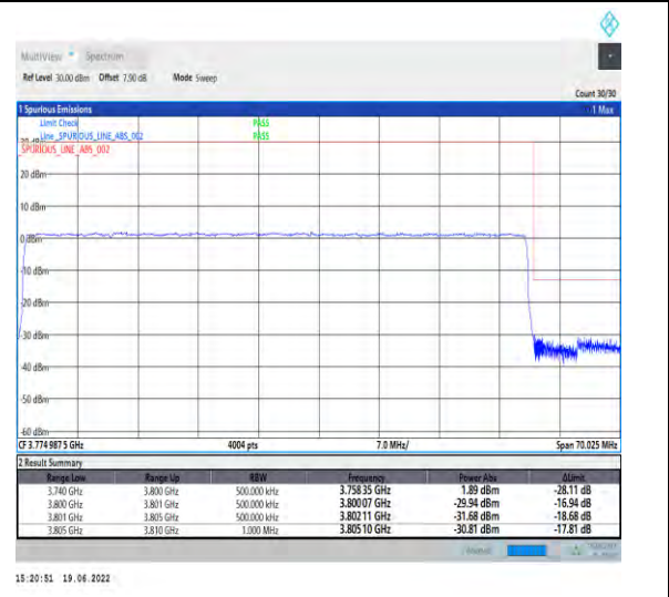
1-N78-3700-3800-PC2-30-60-H-6-CP-QPSK-Outer_Full-162@0-Ant1-PASS-see graph
