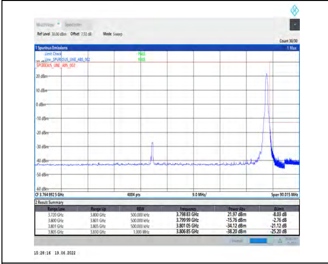
1-N78-3700-3800-PC2-30-80-H-5-CP-QPSK-Edge_1RB_Right-1@216-Ant1-PASS-see graph
