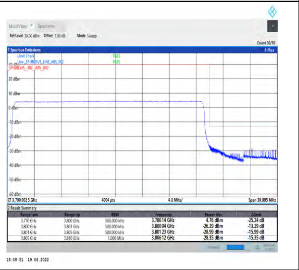
1-N78-3700-3800-PC2-30-30-H-6-CP-QPSK-Outer_Full-78@0-Ant1-PASS-see graph
