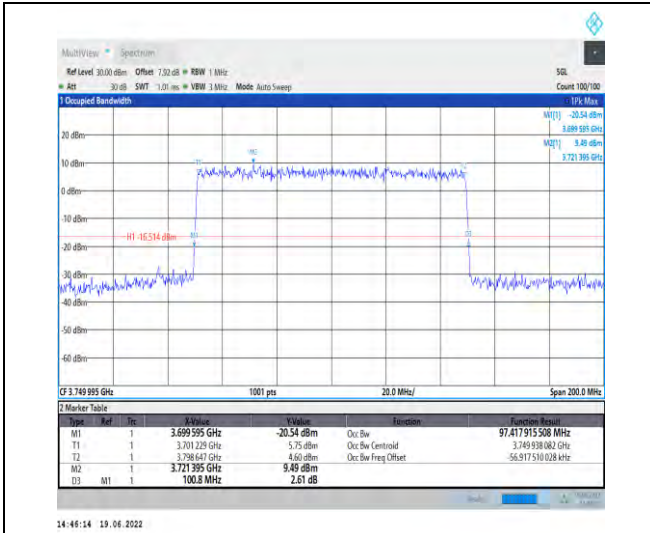
1-N78-3700-3800-PC2-30-100-L-9-CP-256QAM-Out er_Full-273@0-Ant1-97.418-100.800-≤100-PASS
