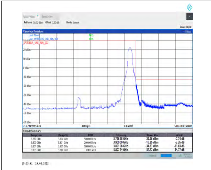
1-N78-3700-3800-PC2-30-20-H-2-DFT-PI2BPSK-Edge_1RB_Right-1@50-Ant1-PASS-see graph
