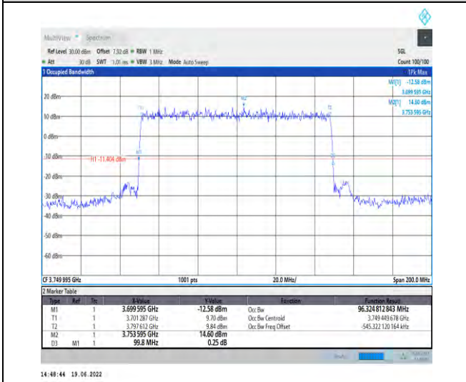
1-N78-3700-3800-PC2-30-100-H-1-DFT-QPSK-Out er_Full-270@0-Ant1-96.325-99.800-≤100-PASS
