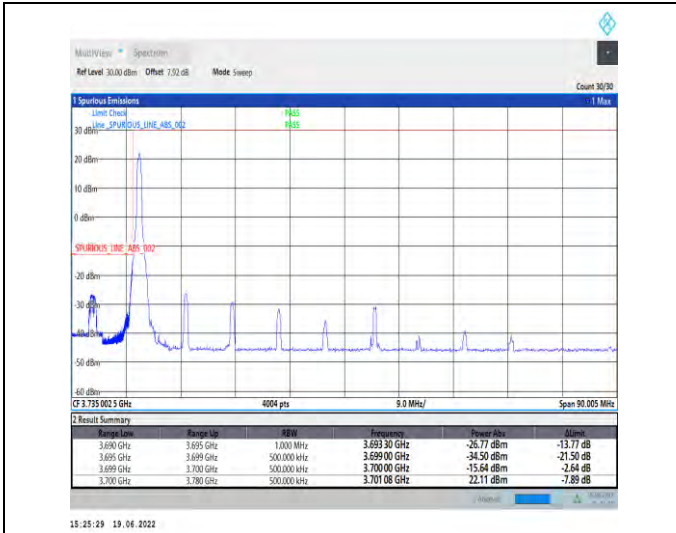
1-N78-3700-3800-PC2-30-80-L-1-DFT-PI2BPSK-Edge_1RB_Left-1@0-Ant1-PASS-see graph
