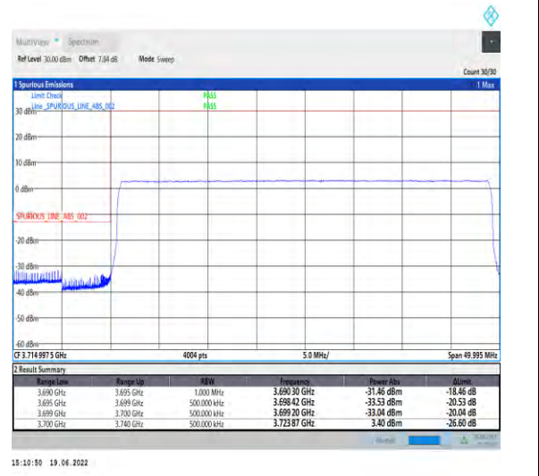
1-N78-3700-3800-PC2-30-40-L-6-CP-QPSK-Outer_Full-106@0-Ant1-PASS-see graph
