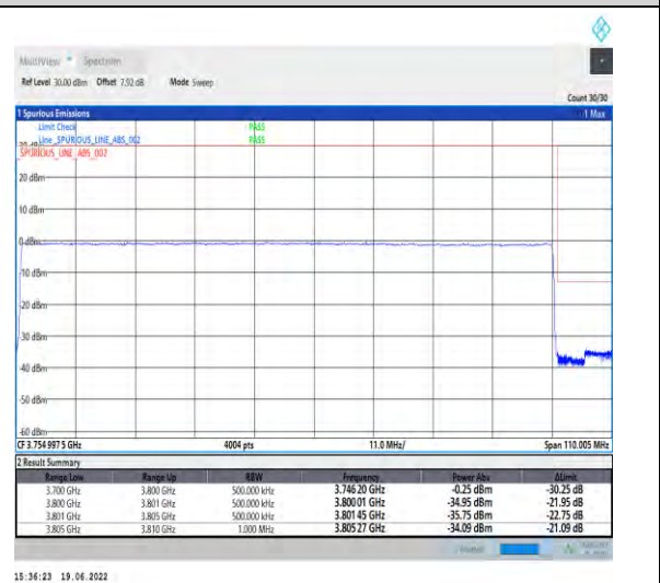
1-N78-3700-3800-PC2-30-100-H-6-CP-QPSK-Outer_Full-273@0-Ant1-PASS-see graph
