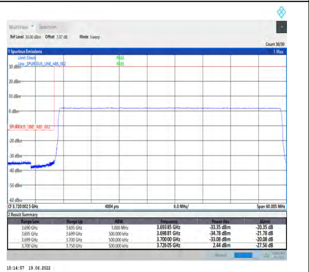
1-N78-3700-3800-PC2-30-50-L-6-CP-QPSK-Outer_Full-133@0-Ant1-PASS-see graph
