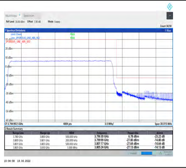
1-N78-3700-3800-PC2-30-20-H-6-CP-QPSK-Outer_Full-51@0-Ant1-PASS-see graph
