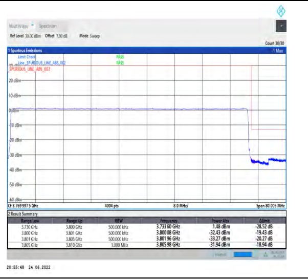
1-N78-3700-3800-PC2-30-70-H-6-CP-QPSK-Outer_Full-189@0-Ant1-PASS-see graph
