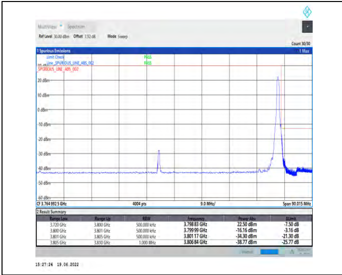
1-N78-3700-3800-PC2-30-80-H-2-DFT-PI2BPSK-Edge_1RB_Right-1@216-Ant1-PASS-see graph
