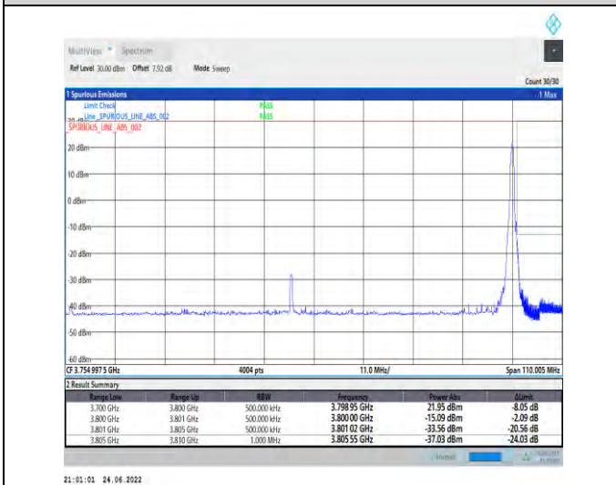
1-N78-3700-3800-PC2-30-100-H-5-CP-QPSK-Edge_1_RB_Right-1@272-Ant1-PASS-see graph
