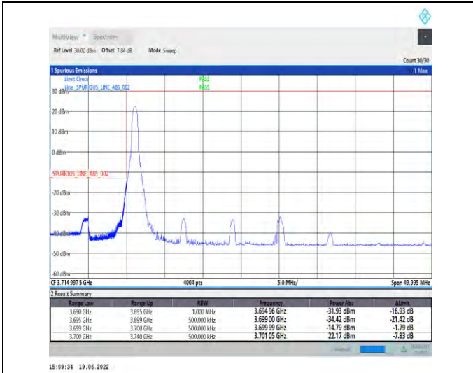
1-N78-3700-3800-PC2-30-40-L-1-DFT-PI2BPSK-Edge_1RB_Left-1@0-Ant1-PASS-see graph
