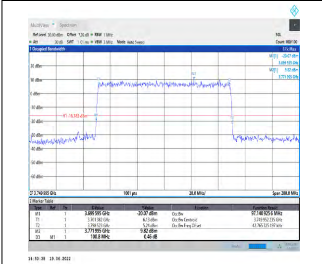
1-N78-3700-3800-PC2-30-100-H-9-CP-256QAM-Outer_Full-273@0-Ant1-97.141-100.800-≤100-PASS
