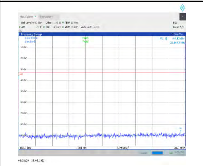
1-N78-3700-3800-PC2-30-100-M-1-DFT-PI2BPSK-In ner_1RB_Left-1@1-0.15-30-Ant1--87.13--33-PASS
