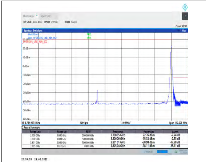
1-N78-3700-3800-PC2-30-100-H-2-DFT-PI2BPSK-Edge_1_RB_Right-1@272-Ant1-PASS-see graph
