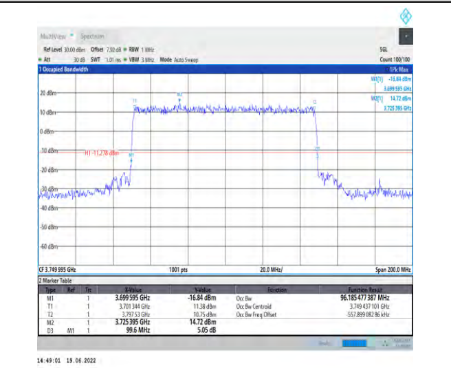
1-N78-3700-3800-PC2-30-100-H-2-DFT-PI2BPSK-Out er_Full-270@0-Ant1-96.185-99.600-≤100-PASS
