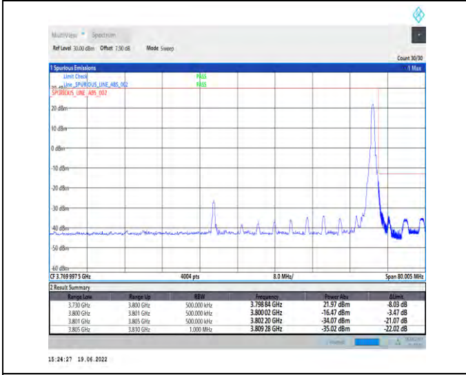
1-N78-3700-3800-PC2-30-70-H-5-CP-QPSK-Edge_1RB_Right-1@188-Ant1-PASS-see graph
