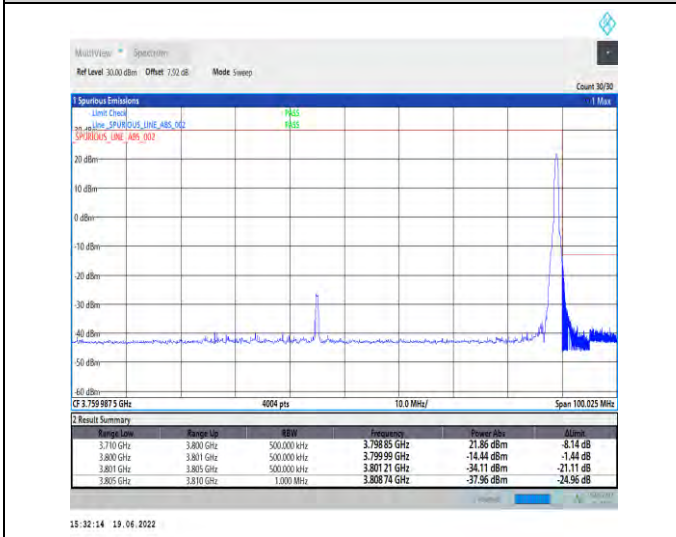
1-N78-3700-3800-PC2-30-90-H-5-CP-QPSK-Edge_1RB_Right-1@244-Ant1-PASS-see graph
