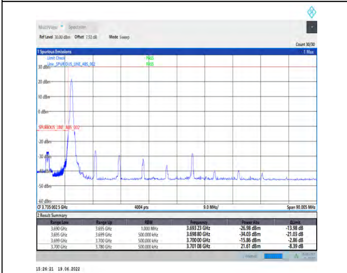
1-N78-3700-3800-PC2-30-80-L-4-CP-QPSK-Edge_1RB_Left-1@0-Ant1-PASS-see graph
