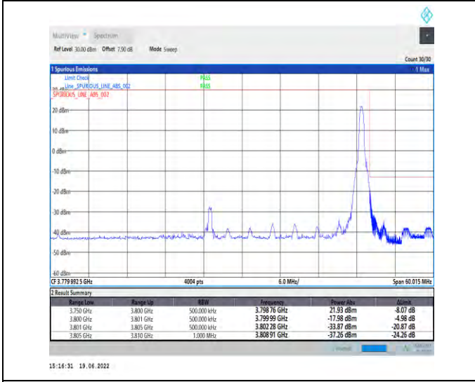
1-N78-3700-3800-PC2-30-50-H-5-CP-QPSK-Edge_1RB_Right-1@132-Ant1-PASS-see graph
