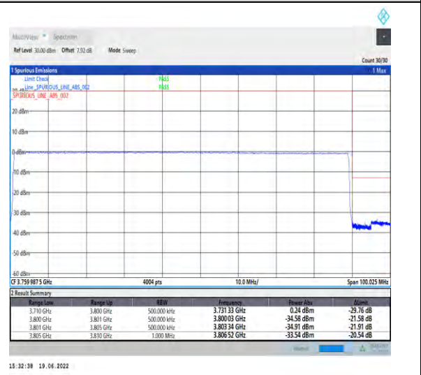
1-N78-3700-3800-PC2-30-90-H-6-CP-QPSK-Outer_Full-245@0-Ant1-PASS-see graph
