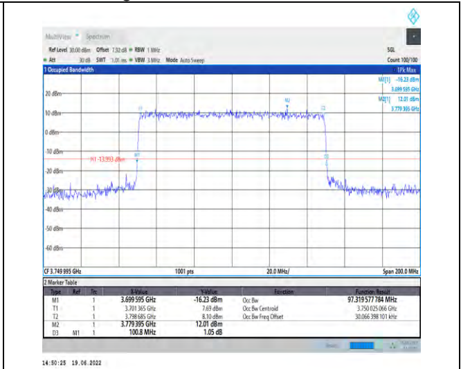
1-N78-3700-3800-PC2-30-100-H-8-CP-64QAM-Outer_Full-273@0-Ant1-97.32-100.800-≤100-PASS
