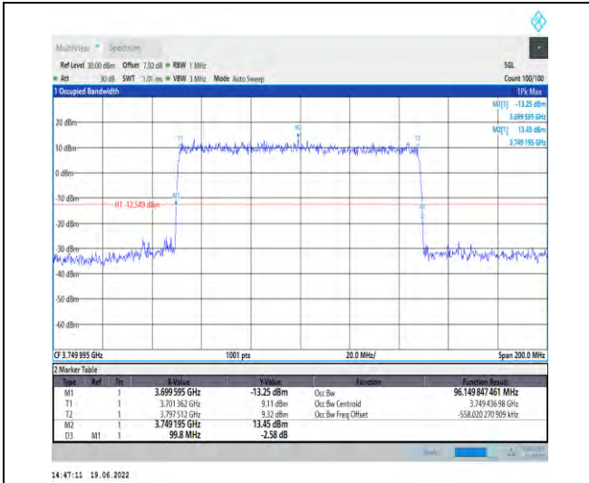
1-N78-3700-3800-PC2-30-100-M-4-DFT-64QAM-Outer_Full-270@0-Ant1-96.15-99.800-≤100-PASS
