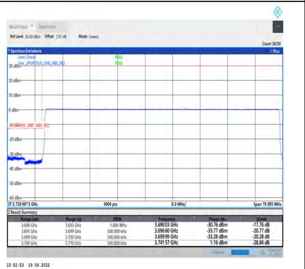
1-N78-3700-3800-PC2-30-70-L-6-CP-QPSK-Outer_Full-189@0-Ant1-PASS-see graph
