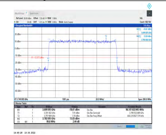
1-N78-3700-3800-PC2-30-100-H-4-DFT-64QAM-Out er_Full-270@0-Ant1-96.102-99.800-≤100-PASS
