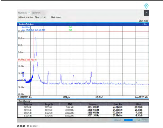
1-N78-3700-3800-PC2-30-70-L-4-CP-QPSK-Edge_1RB_Left-1@0-Ant1-PASS-see graph
