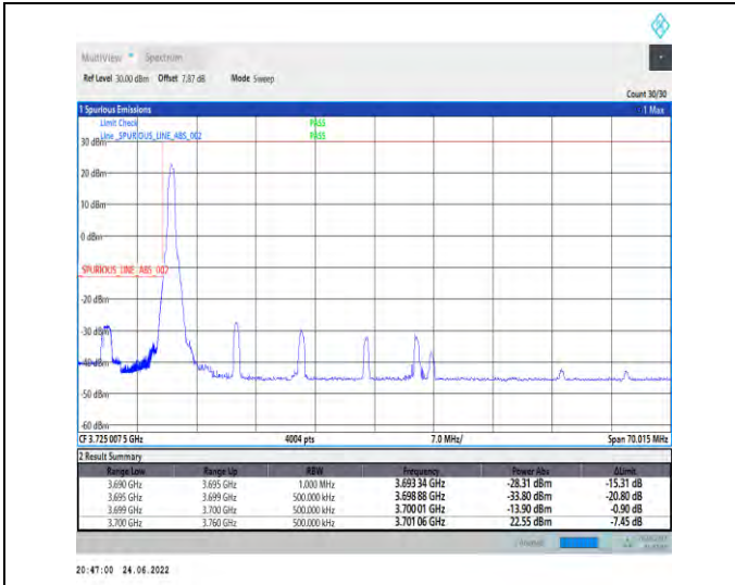
1-N78-3700-3800-PC2-30-60-L-1-DFT-PI2BPSK-Edge_1RB_Left-1@0-Ant1-PASS-see graph
