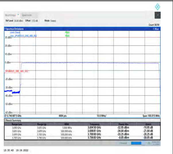
1-N78-3700-3800-PC2-30-90-L-6-CP-QPSK-Outer_Full-245@0-Ant1-PASS-see graph
