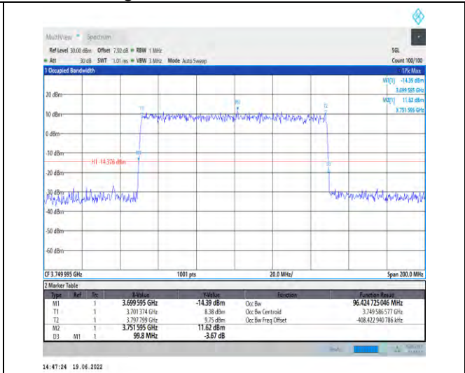
1-N78-3700-3800-PC2-30-100-M-5-DFT-256QAM-Outer_Full-270@0-Ant1-96.425-99.800-≤100-PASS
