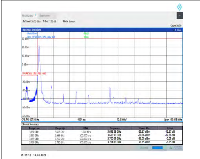
1-N78-3700-3800-PC2-30-90-L-4-CP-QPSK-Edge_1RB_Left-1@0-Ant1-PASS-see graph
