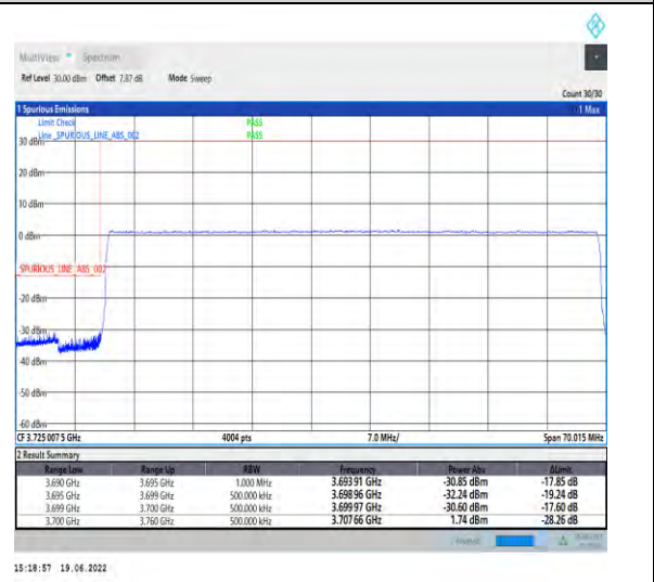
1-N78-3700-3800-PC2-30-60-L-6-CP-QPSK-Outer_Full-162@0-Ant1-PASS-see graph
