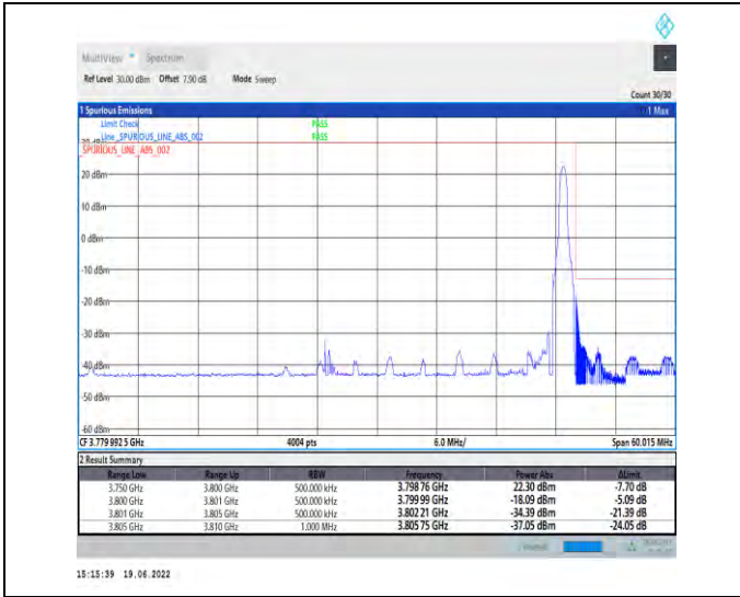
1-N78-3700-3800-PC2-30-50-H-2-DFT-PI2BPSK-Edge_1RB_Right-1@132-Ant1-PASS-see graph
