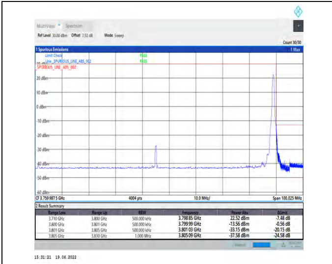
1-N78-3700-3800-PC2-30-90-H-2-DFT-PI2BPSK-Edge_1RB_Right-1@244-Ant1-PASS-see graph
