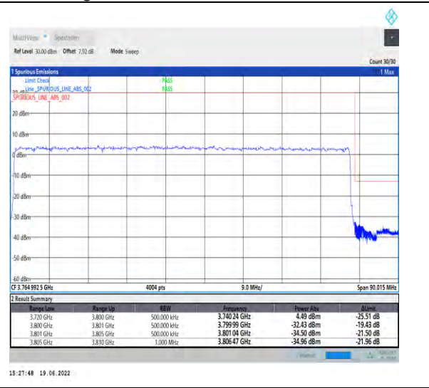
1-N78-3700-3800-PC2-30-80-H-3-DFT-PI2BPSK-Outer_Full-216@0-Ant1-PASS-see graph
