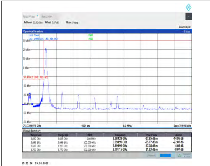
1-N78-3700-3800-PC2-30-70-L-1-DFT-PI2BPSK-Edge_1RB_Left-1@0-Ant1-PASS-see graph
