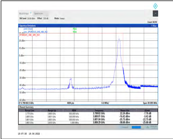
1-N78-3700-3800-PC2-30-30-H-2-DFT-PI2BPSK-Edge_1RB_Right-1@77-Ant1-PASS-see graph
