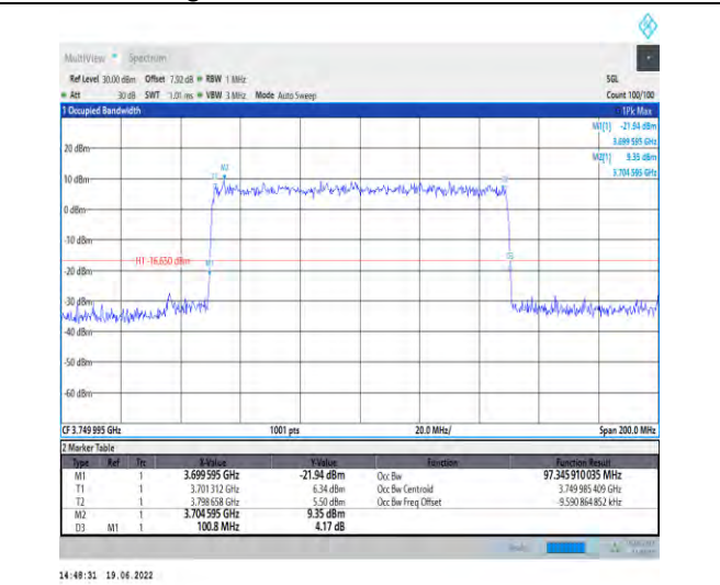
1-N78-3700-3800-PC2-30-100-M-9-CP-256QAM-Out er_Full-273@0-Ant1-97.346-100.800-≤100-PASS
