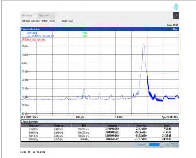
1-N78-3700-3800-PC2-30-40-H-2-DFT-PI2BPSK-Edge_1RB_Right-1@105-Ant1-PASS-see graph
