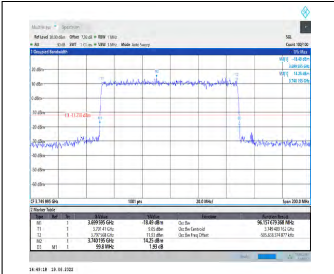
1-N78-3700-3800-PC2-30-100-H-3-DFT-16QAM-Out er_Full-270@0-Ant1-96.158-99.800-≤100-PASS
