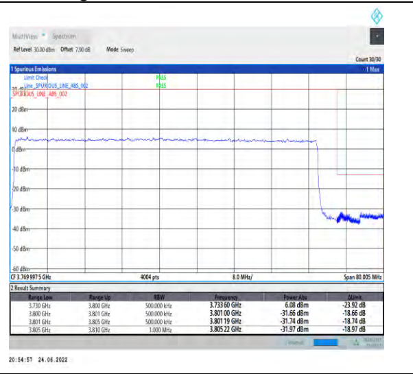
1-N78-3700-3800-PC2-30-70-H-3-DFT-PI2BPSK-Outer_Full-180@0-Ant1-PASS-see graph
