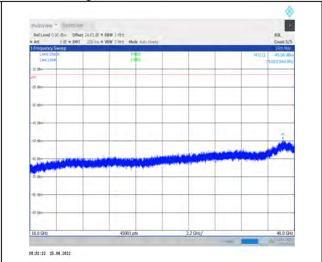
1-N78-3700-3800-PC2-30-100-L-1-DFT-PI2BPSK-In ner_1RB_Left-1@1-18000-40000-Ant1--49.56--13-P ASS
