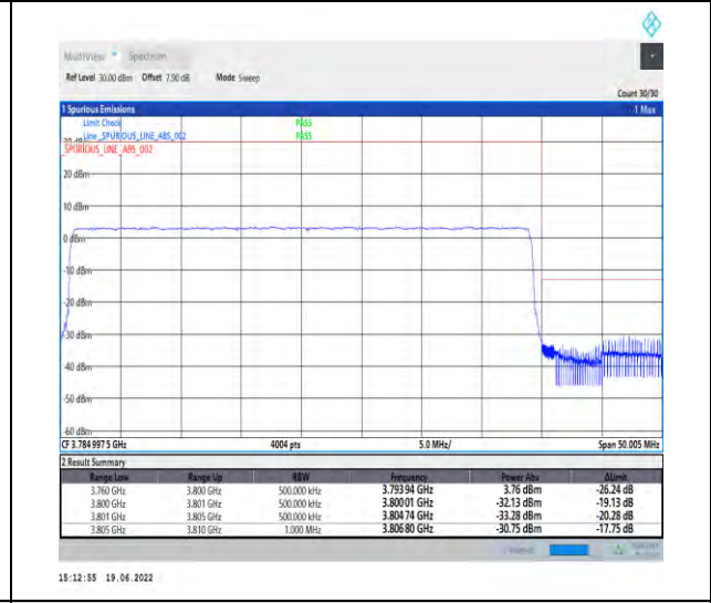
1-N78-3700-3800-PC2-30-40-H-6-CP-QPSK-Outer_Full-106@0-Ant1-PASS-see graph
