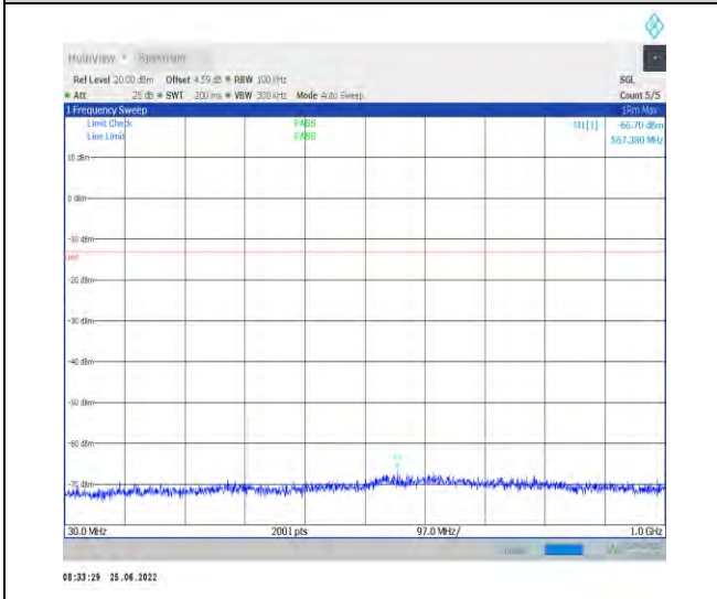
1-N78-3700-3800-PC2-30-100-H-1-DFT-PI2BPSK-In ner_1RB_Left-1@1-30-1000-Ant1--66.70--13-PASS
