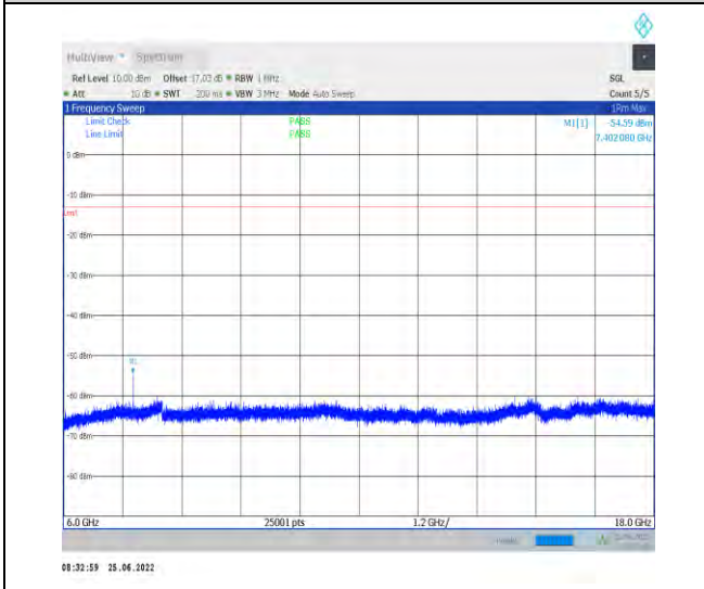
1-N78-3700-3800-PC2-30-100-M-1-DFT-PI2BPSK-I nner_1RB_Left-1@1-6000-18000-Ant1--54.59--13-P ASS
