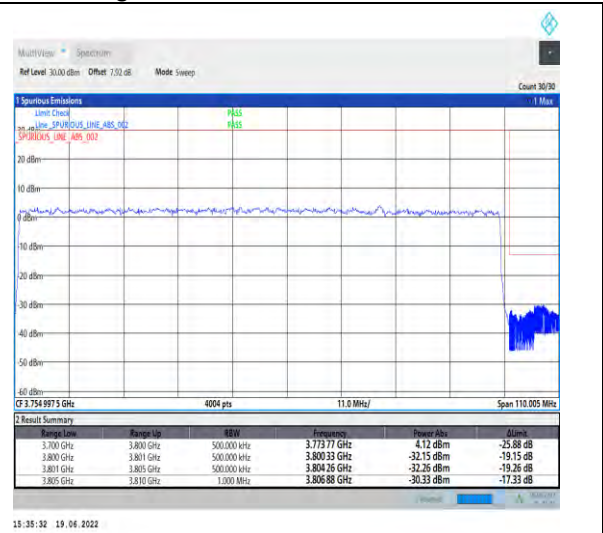
1-N78-3700-3800-PC2-30-100-H-3-DFT-PI2BPSK-Outer_Full-270@0-Ant1-PASS-see graph
