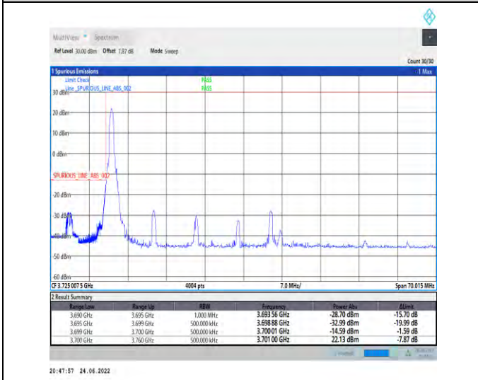
1-N78-3700-3800-PC2-30-60-L-4-CP-QPSK-Edge_1RB_Left-1@0-Ant1-PASS-see graph
