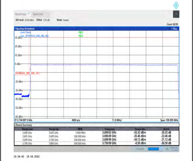
1-N78-3700-3800-PC2-30-100-L-6-CP-QPSK-Outer_Full-273@0-Ant1-PASS-see graph
