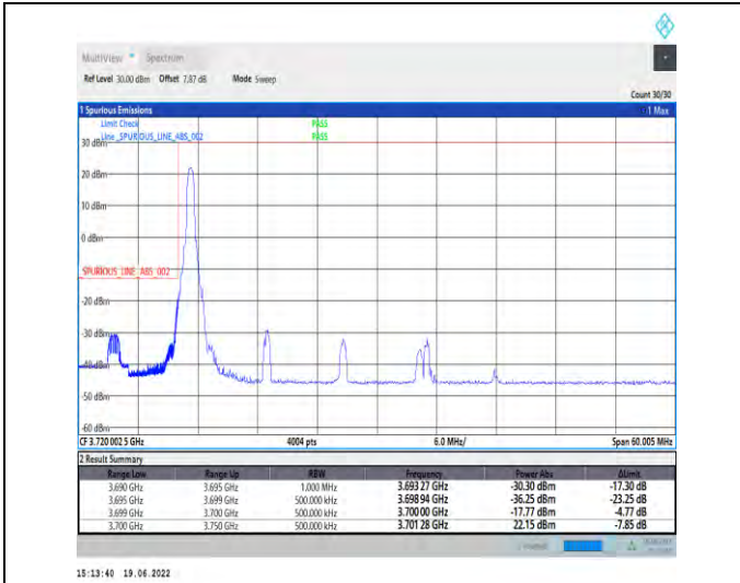
1-N78-3700-3800-PC2-30-50-L-1-DFT-PI2BPSK-Edge_1RB_Left-1@0-Ant1-PASS-see graph
