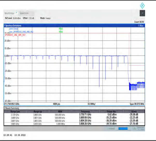
1-N78-3700-3800-PC2-30-80-H-6-CP-QPSK-Outer_Full-217@0-Ant1-PASS-see graph
