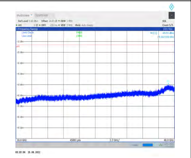
1-N78-3700-3800-PC2-30-100-M-1-DFT-PI2BPSK-In ner_1RB_Left-1@1-18000-40000-Ant1--49.91--13-P ASS
