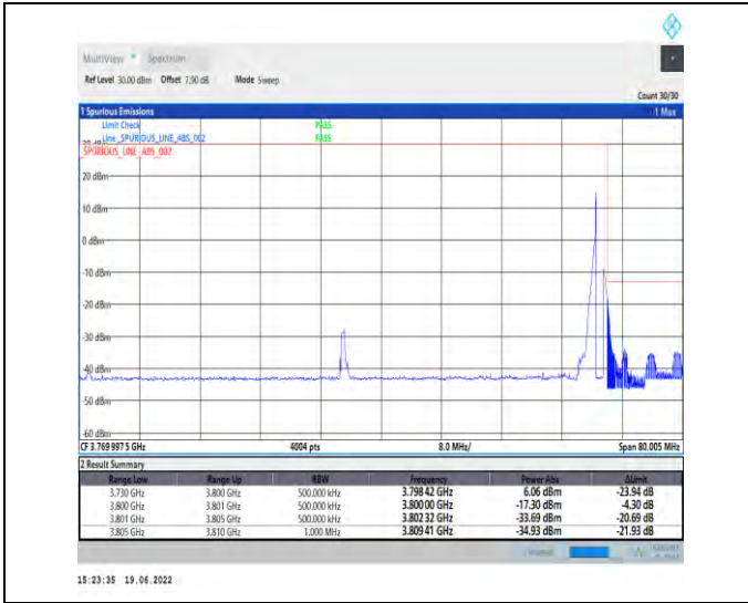
1-N78-3700-3800-PC2-30-70-H-2-DFT-PI2BPSK-Edge_1RB_Right-1@188-Ant1-PASS-see graph
