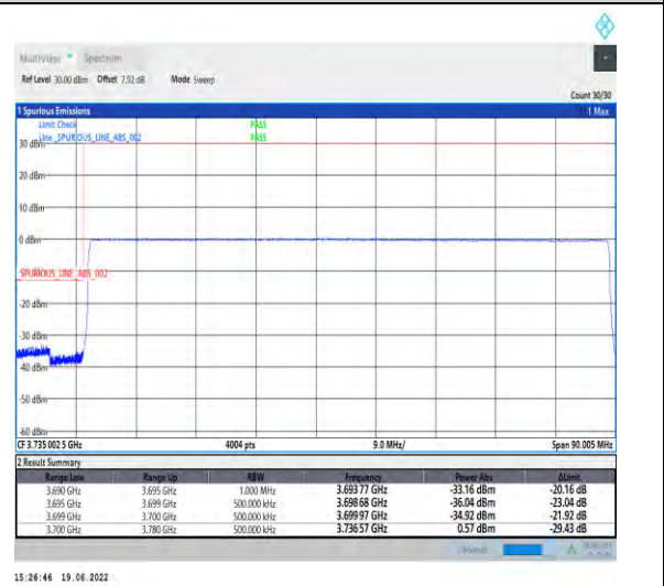
1-N78-3700-3800-PC2-30-80-L-6-CP-QPSK-Outer_Full-217@0-Ant1-PASS-see graph
