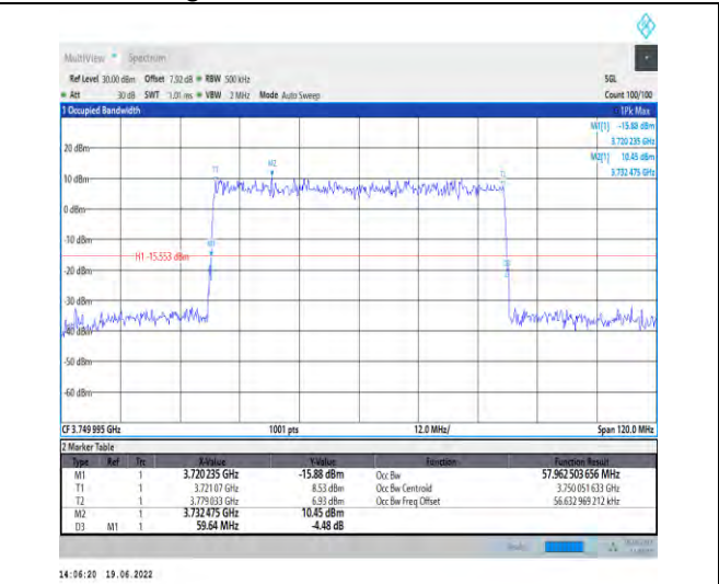
1-N78-3700-3800-PC2-30-60-M-5-DFT-256QAM-Out er_Full-162@0-Ant1-57.963-59.640-≤60-PASS
