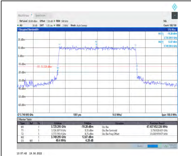
1-N78-3700-3800-PC2-30-50-M-7-CP-16QAM-Outer_Full-133@0-Ant1-47.437-49.400-≤50-PASS
