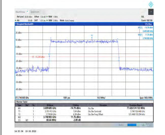
1-N78-3700-3800-PC2-30-80-L-9-CP-256QAM-Outer_Full-217@0-Ant1-77.427-80.640-≤80-PASS
