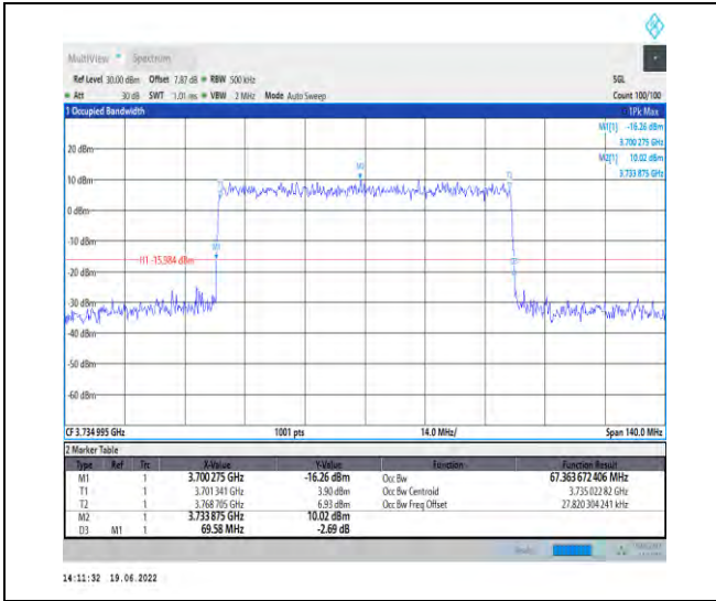
1-N78-3700-3800-PC2-30-70-L-6-CP-QPSK-Outer_Full-189@0-Ant1-67.364-69.580-≤70-PASS
