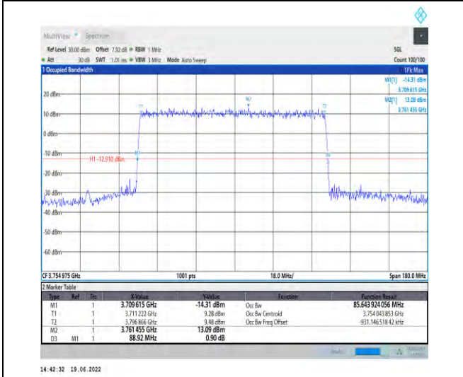
1-N78-3700-3800-PC2-30-90-H-4-DFT-64QAM-Outer_Full-240@0-Ant1-85.644-88.920-≤90-PASS
