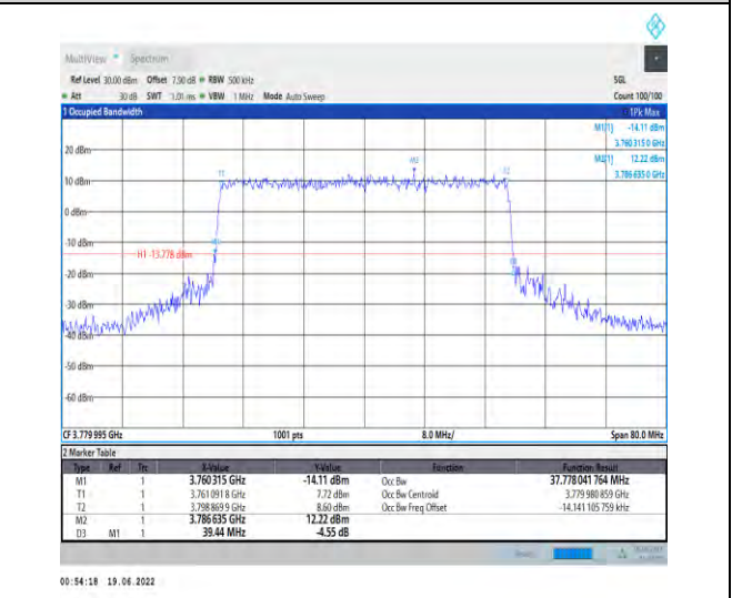
1-N78-3700-3800-PC2-30-40-H-8-CP-64QAM-Outer_Full-106@0-Ant1-37.778-39.440-≤40-PASS
