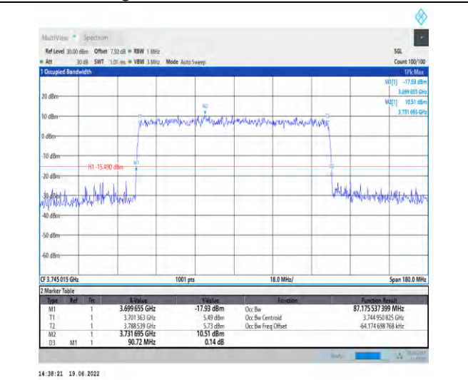
1-N78-3700-3800-PC2-30-90-L-9-CP-256QAM-Outer_Full-245@0-Ant1-87.176-90.720-≤90-PASS
