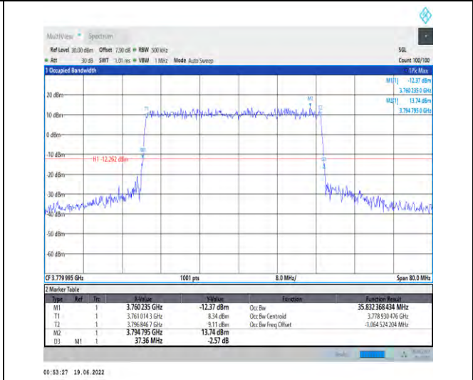
1-N78-3700-3800-PC2-30-40-H-4-DFT-64QAM-Outer_Full-100@0-Ant1-35.832-37.360-≤40-PASS
