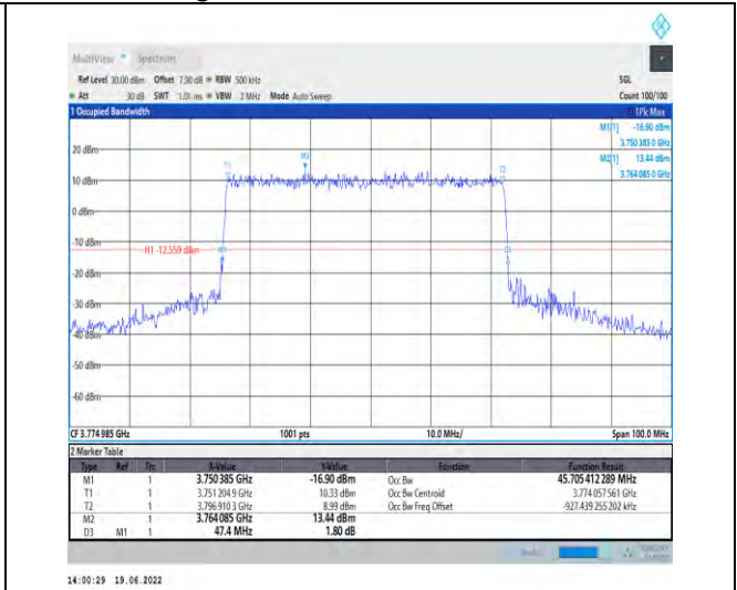
1-N78-3700-3800-PC2-30-50-H-3-DFT-16QAM-Outer_Full-128@0-Ant1-45.705-47.400-≤50-PASS
