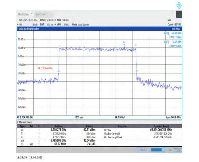
1-N78-3700-3800-PC2-30-70-H-3-DFT-16QAM-Outer_Full-180@0-Ant1-64.374-66.220-≤70-PASS
