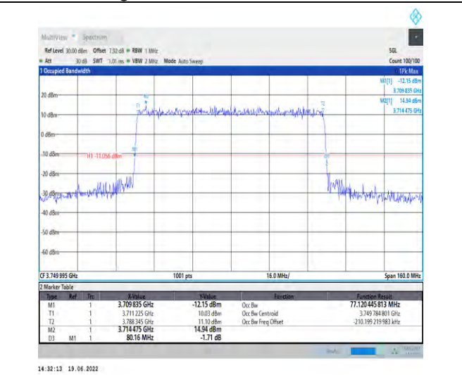
1-N78-3700-3800-PC2-30-80-M-3-DFT-16QAM-Outer_Full-216@0-Ant1-77.12-80.160-≤80-PASS
