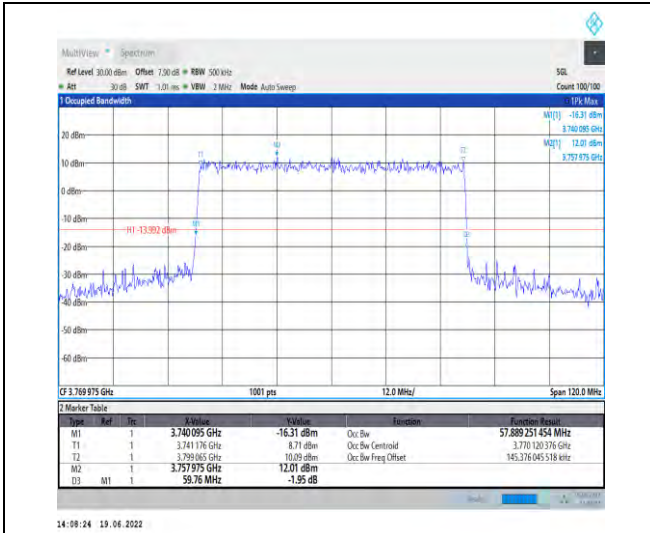
1-N78-3700-3800-PC2-30-60-H-3-DFT-16QAM-Outer_Full-162@0-Ant1-57.889-59.760-≤60-PASS
