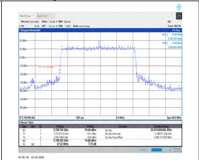
1-N78-3700-3800-PC2-30-40-M-3-DFT-16QAM-Outer_Full-100@0-Ant1-35.675-37.520-≤40-PASS
