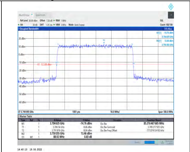
1-N78-3700-3800-PC2-30-90-M-4-DFT-64QAM-Out er_Full-240@0-Ant1-85.316-88.920-≤90-PASS
