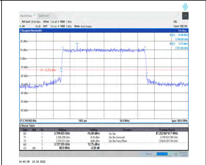
1-N78-3700-3800-PC2-30-90-M-6-CP-QPSK-Out er_Full-245@0-Ant1-87.253-90.900-≤90-PASS
