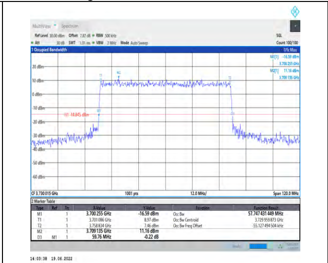
1-N78-3700-3800-PC2-30-60-L-6-CP-QPSK-Outer_F ull-162@0-Ant1-57.747-59.760-≤60-PASS
