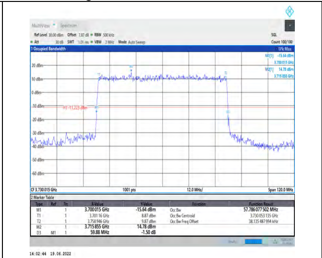
1-N78-3700-3800-PC2-30-60-L-2-DFT-PI2BPSK-Outer_Full-162@0-Ant1-57.786-59.880-≤60-PASS
