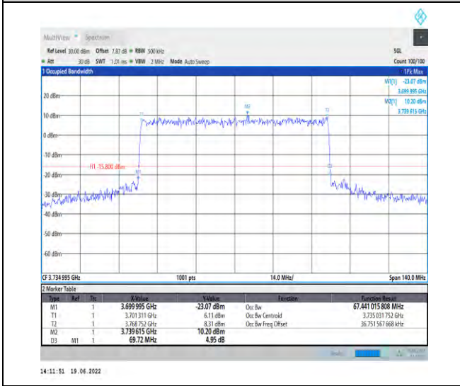
1-N78-3700-3800-PC2-30-70-L-8-CP-64QAM-Outer_Full-189@0-Ant1-67.441-69.720-≤70-PASS
