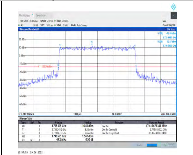
1-N78-3700-3800-PC2-30-50-M-8-CP-64QAM-Outer_Full-133@0-Ant1-47.417-49.200-≤50-PASS
