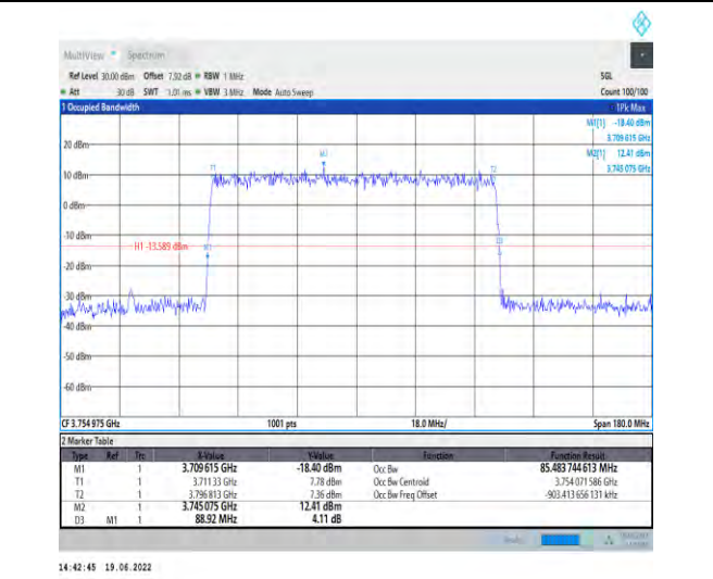
1-N78-3700-3800-PC2-30-90-H-5-DFT-256QAM-Outer_Full-240@0-Ant1-85.484-88.920-≤90-PASS
