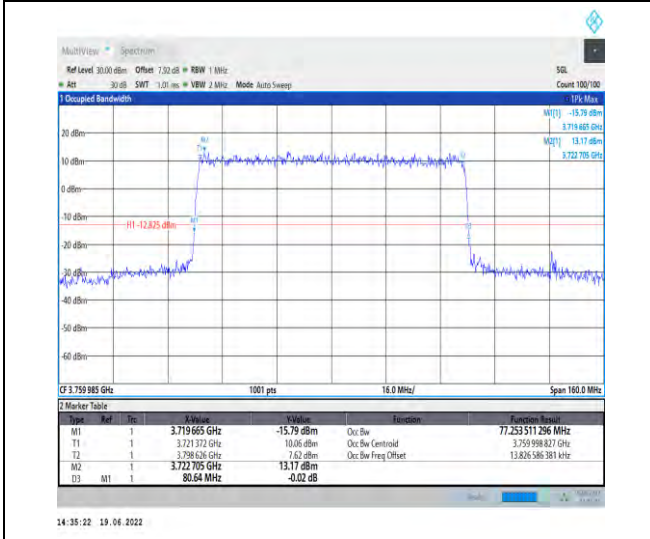
1-N78-3700-3800-PC2-30-80-H-7-CP-16QAM-Outer_Full-217@0-Ant1-77.254-80.640-≤80-PASS
