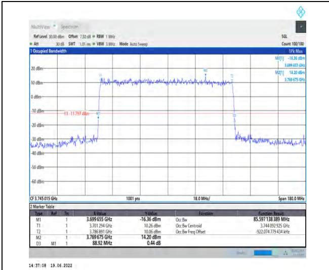
1-N78-3700-3800-PC2-30-90-L-4-DFT-64QAM-Outer_Full-240@0-Ant1-85.597-88.920-≤90-PASS
