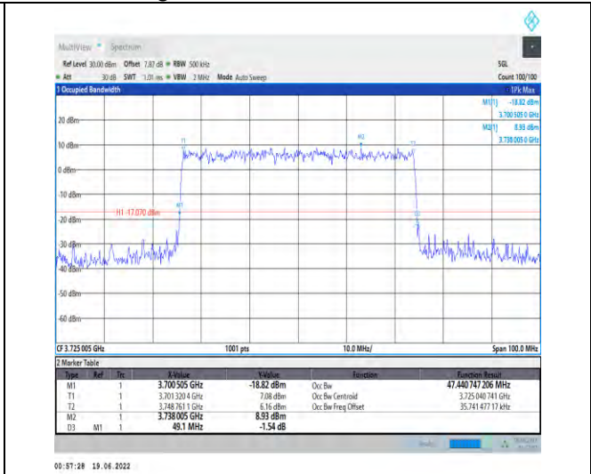
1-N78-3700-3800-PC2-30-50-L-9-CP-256QAM-Outer _Full-133@0-Ant1-47.441-49.100-≤50-PASS
