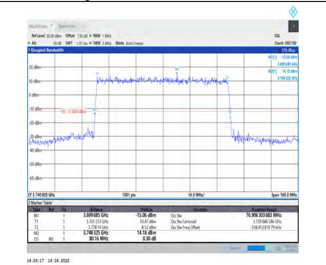
1-N78-3700-3800-PC2-30-80-L-4-DFT-64QAM-Outer_Full-216@0-Ant1-76.906-80.160-≤80-PASS
