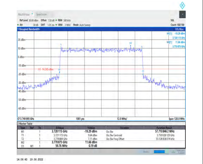
1-N78-3700-3800-PC2-30-60-M-7-CP-16QAM-Outer_Full-162@0-Ant1-57.711-59.760-≤60-PASS
