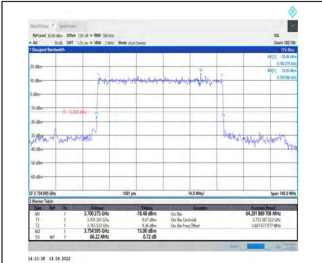
1-N78-3700-3800-PC2-30-70-L-2-DFT-PI2BPSK-Out er_Full-180@0-Ant1-64.292-66.220-≤70-PASS
