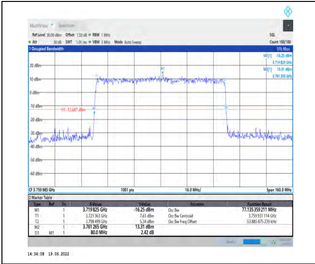
1-N78-3700-3800-PC2-30-80-H-5-DFT-256QAM-Out er_Full-216@0-Ant1-77.135-80.000-≤80-PASS
