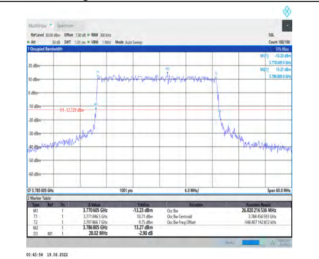
1-N78-3700-3800-PC2-30-30-H-1-DFT-QPSK-Outer_Full-75@0-Ant1-26.82-28.020-≤30-PASS
