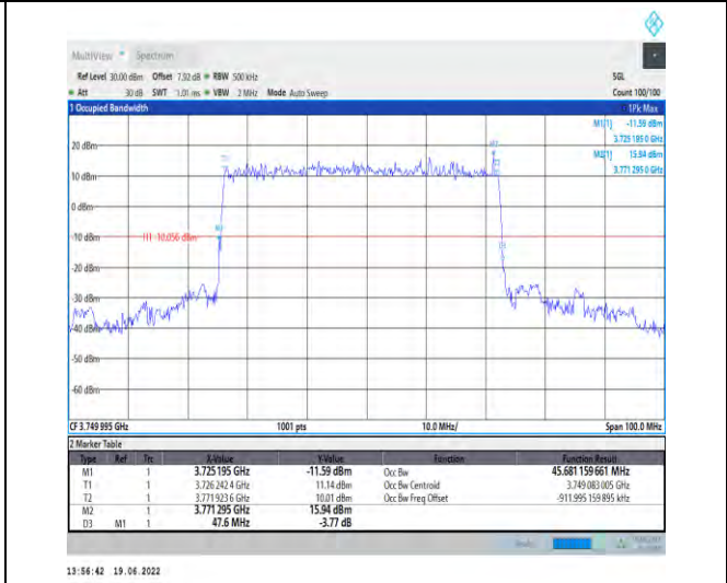
1-N78-3700-3800-PC2-30-50-M-2-DFT-PI2BPSK-Outer _Full-128@0-Ant1-45.681-47.600-≤50-PASS
