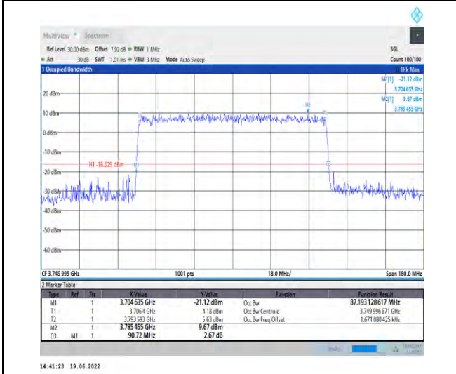
1-N78-3700-3800-PC2-30-90-M-9-CP-256QAM-Outer_Full-245@0-Ant1-87.193-90.720-<math>\leq 90</math>-PASS
