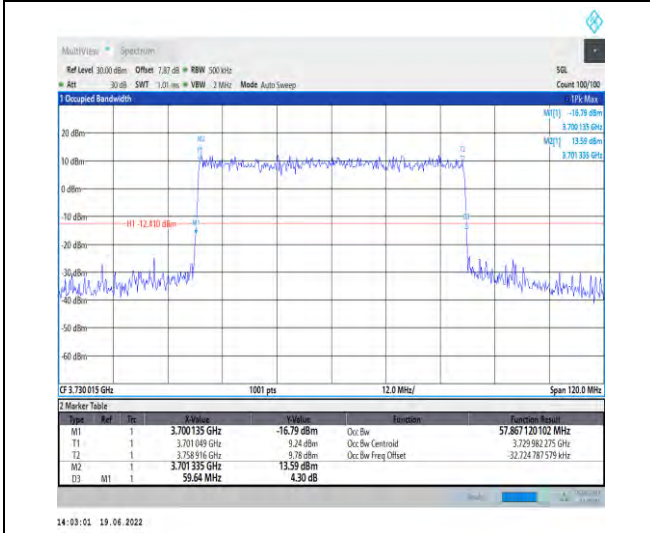
1-N78-3700-3800-PC2-30-60-L-3-DFT-16QAM-Outer_Full-162@0-Ant1-57.867-59.640-≤60-PASS
