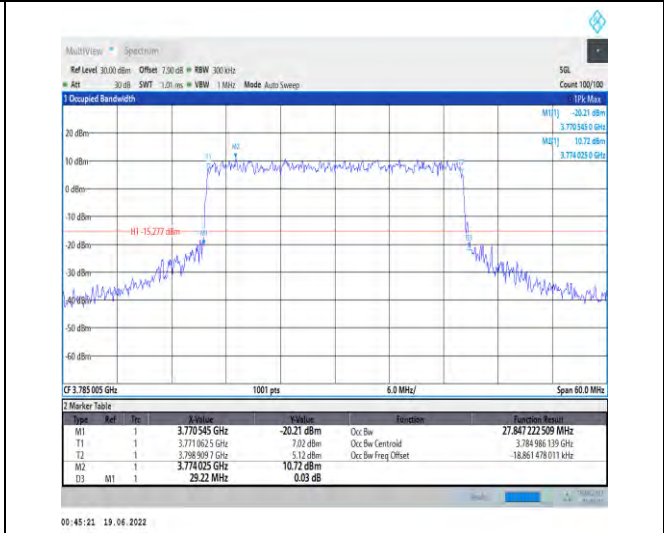
1-N78-3700-3800-PC2-30-30-H-7-CP-16QAM-Outer_Full-78@0-Ant1-27.847-29.220-≤30-PASS
