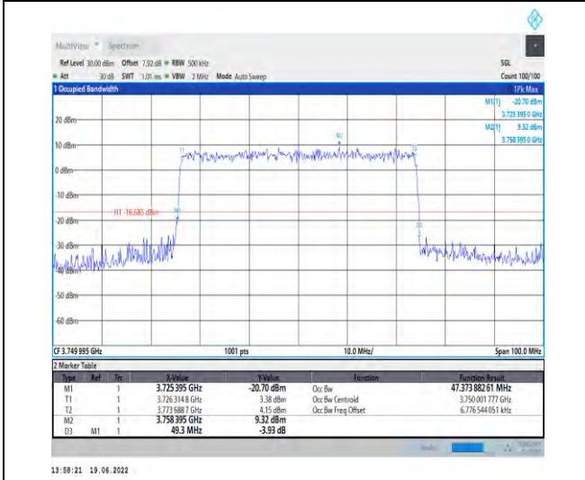
1-N78-3700-3800-PC2-30-50-M-9-CP-256QAM-Outer_Full-133@0-Ant1-47.374-49.300-≤50-PASS
