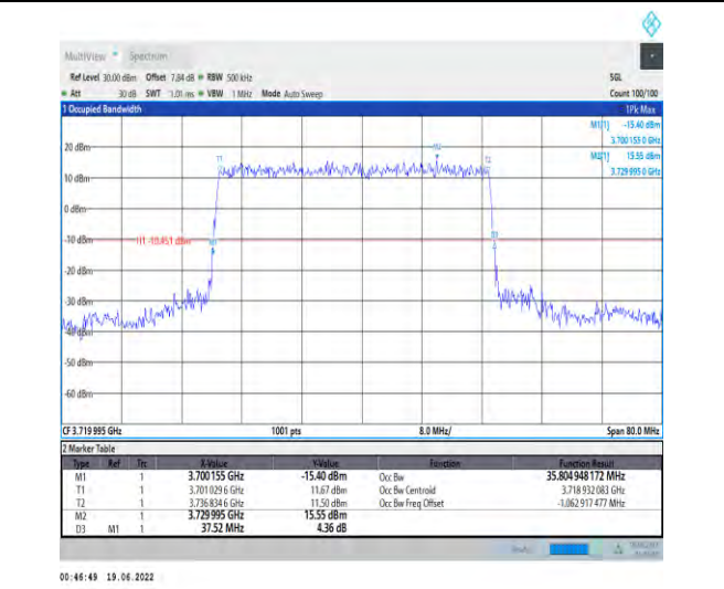
1-N78-3700-3800-PC2-30-40-L-2-DFT-PI2BPSK-Outer_Full-100@0-Ant1-35.805-37.520-≤40-PASS
