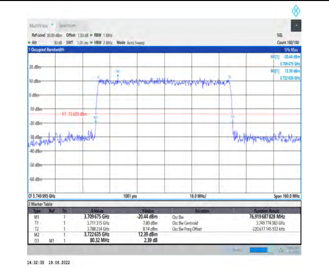
1-N78-3700-3800-PC2-30-80-M-5-DFT-256QAM-Outer_Full-216@0-Ant1-76.92-80.320-≤80-PASS
