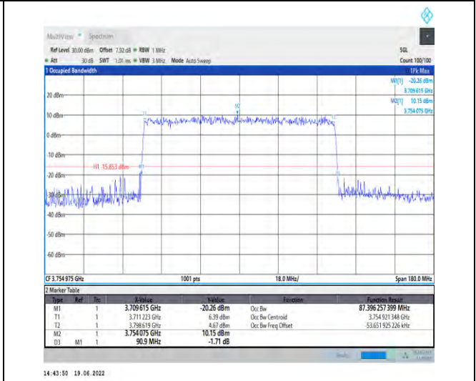
1-N78-3700-3800-PC2-30-90-H-9-CP-256QAM-Outer_Full-245@0-Ant1-87.396-90.900-≤90-PASS
