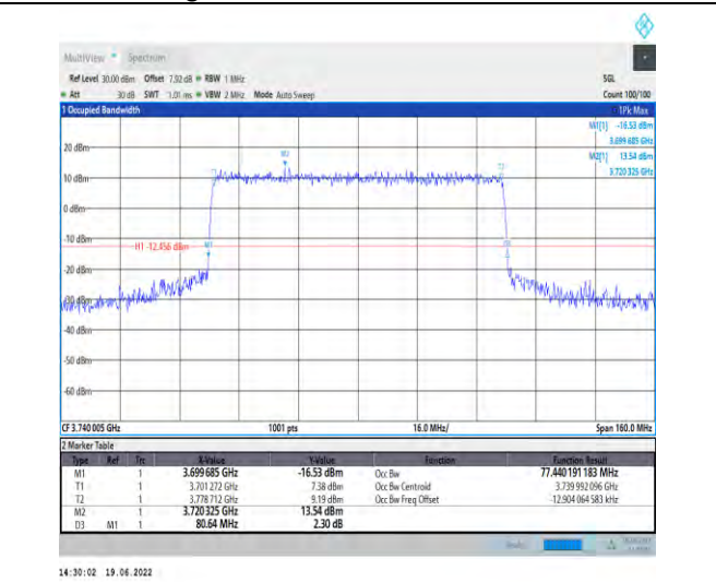
1-N78-3700-3800-PC2-30-80-L-8-CP-64QAM-Outer_Full-217@0-Ant1-77.44-80.640-≤80-PASS
