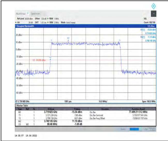
1-N78-3700-3800-PC2-30-80-H-9-CP-256QAM-Outer_Full-217@0-Ant1-77.499-80.480-≤80-PASS
