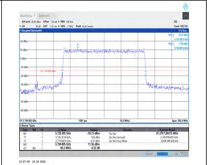
1-N78-3700-3800-PC2-30-50-M-6-CP-QPSK-Outer_Full-133@0-Ant1-47.37-49.200-≤50-PASS
