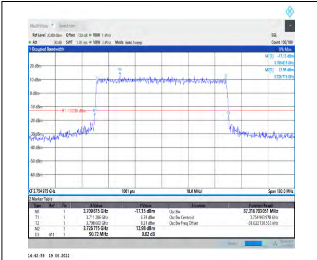
1-N78-3700-3800-PC2-30-90-H-6-CP-QPSK-Outer_Full-245@0-Ant1-87.317-90.720-≤90-PASS
