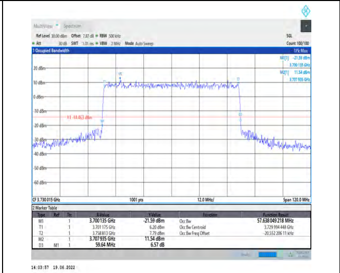
1-N78-3700-3800-PC2-30-60-L-8-CP-64QAM-Outer_ Full-162@0-Ant1-57.638-59.640-≤60-PASS
