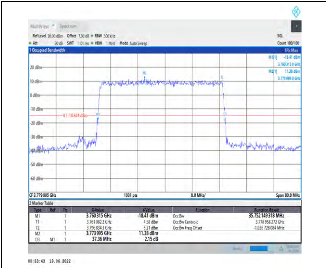
1-N78-3700-3800-PC2-30-40-H-5-DFT-256QAM-Out_er_Full-100@0-Ant1-35.752-37.360-≤40-PASS
