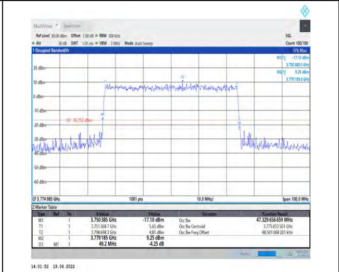
1-N78-3700-3800-PC2-30-50-H-9-CP-256QAM-Outer_Full-133@0-Ant1-47.33-49.200-≤50-PASS
