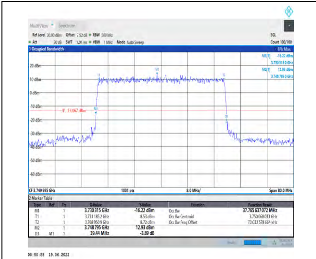
1-N78-3700-3800-PC2-30-40-M-6-CP-QPSK-Outer_Full-106@0-Ant1-37.766-39.440-≤40-PASS
