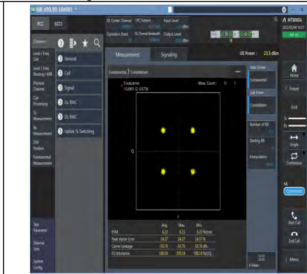
1-N78-3700-3800--30-100-M-6-CP-QPSK-Outer_Fu I1-273@0-Ant1-see graph-PASS
