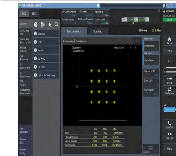
1-N78-3700-3800--30-100-M-7-CP-16QAM-Outer_Fu I1-273@0-Ant1-see graph-PASS
