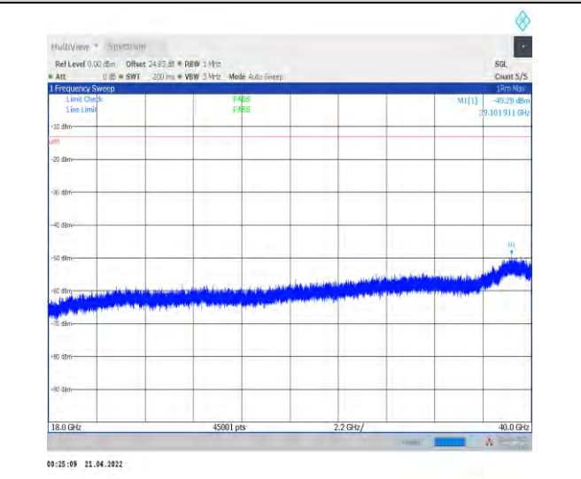
1-N78-3450-3550--30-100-M-1-DFT-PI2BPSK-Inner_ 1RB_Left-1@1-18000-40000-Ant1--49.28--13-PASS
