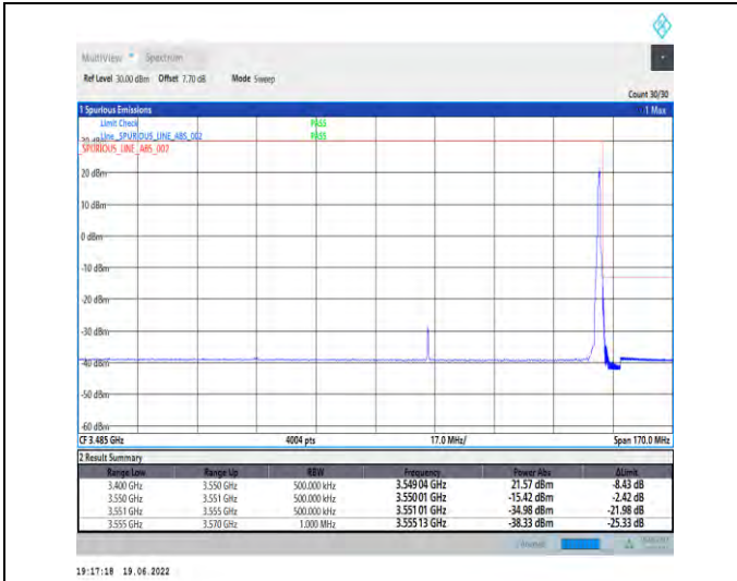
1-N78-3450-3550-PC2-30-100-H-2-DFT-PI2BPSK-Edge_1RB_Right-1@272-Ant1-PASS-see graph
