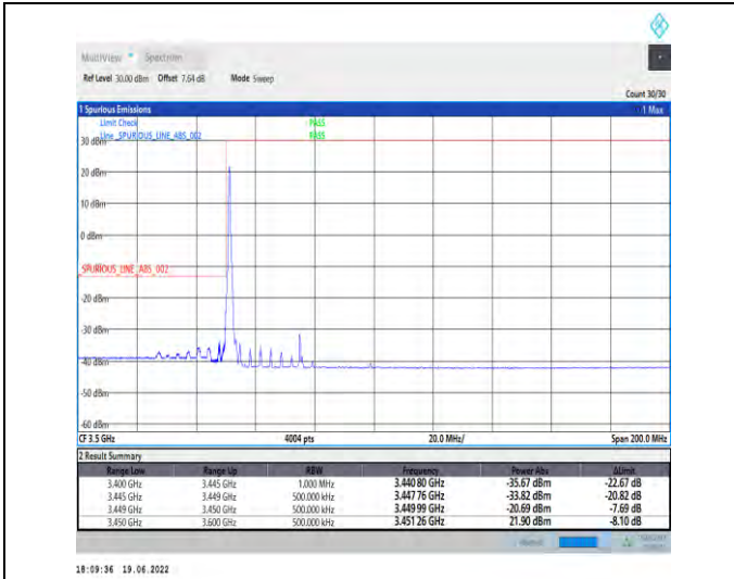
1-N78-3450-3550-PC2-30-50-L-1-DFT-PI2BPSK-Edge_1RB_Left-1@0-Ant1-PASS-see graph
