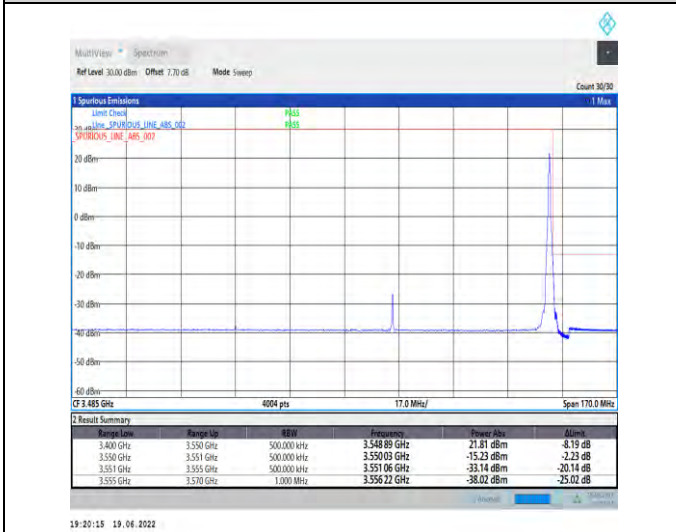
1-N78-3450-3550-PC2-30-100-H-5-CP-QPSK-Edge_1RB_Right-1@272-Ant1-PASS-see graph
