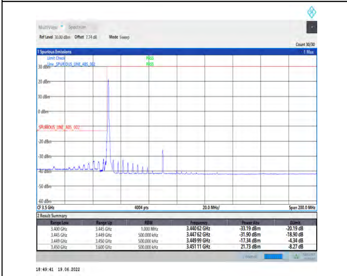
1-N78-3450-3550-PC2-30-80-L-4-CP-QPSK-Edge_1RB_Left-1@0-Ant1-PASS-see graph
