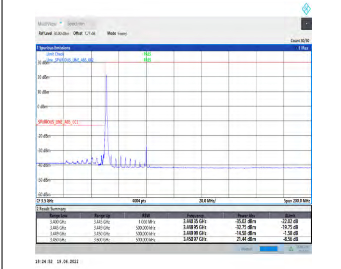
1-N78-3450-3550-PC2-30-60-L-4-CP-QPSK-Edge_1RB_Left-1@0-Ant1-PASS-see graph
