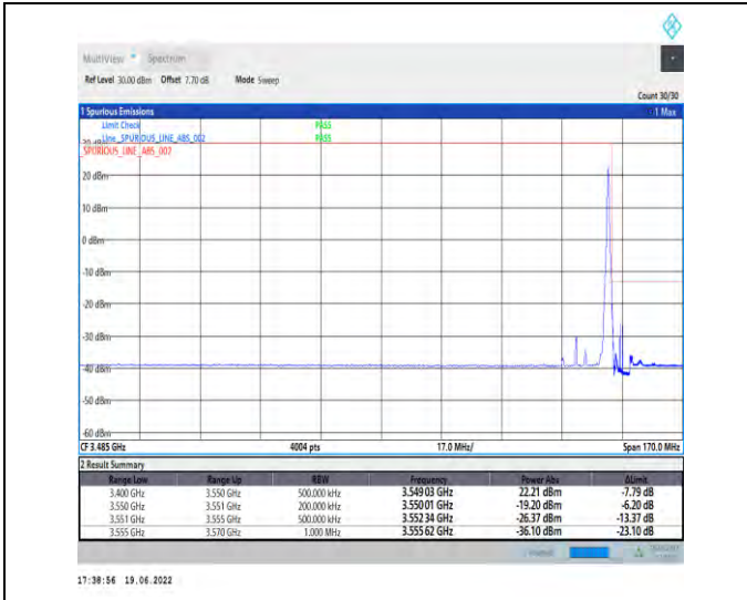
1-N78-3450-3550-PC2-30-20-H-2-DFT-PI2BPSK-Edge_1RB_Right-1@50-Ant1-PASS-see graph
