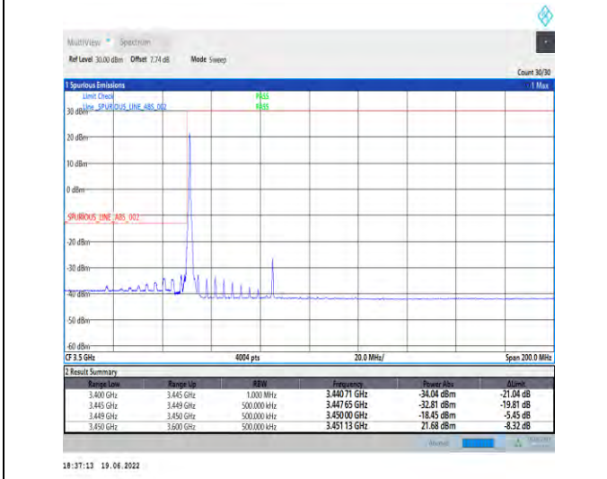
1-N78-3450-3550-PC2-30-70-L-4-CP-QPSK-Edge_1RB_Left-1@0-Ant1-PASS-see graph
