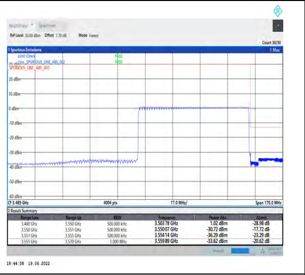
1-N78-3450-3550-PC2-30-70-H-6-CP-QPSK-Outer_Full-189@0-Ant1-PASS-see graph
