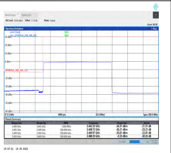
1-N78-3450-3550-PC2-30-90-L-6-CP-QPSK-Outer_Full-245@0-Ant1-PASS-see graph
