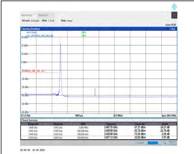
1-N78-3450-3550-PC2-30-90-L-1-DFT-PI2BPSK-Edge_1RB_Left-1@0-Ant1-PASS-see graph
