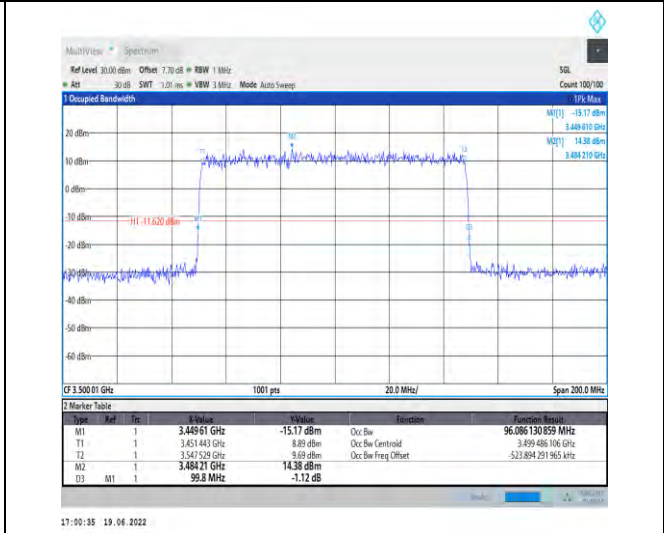
1-N78-3450-3550-PC2-30-100-H-3-DFT-16QAM-Outer_Full-270@0-Ant1-96.086-99.800-≤100-PASS
