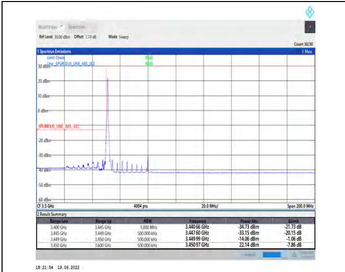
1-N78-3450-3550-PC2-30-60-L-1-DFT-PI2BPSK-Edge_1RB_Left-1@0-Ant1-PASS-see graph
