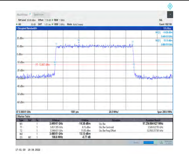
1-N78-3450-3550-PC2-30-100-H-7-CP-16QAM-Outer _Full-273@0-Ant1-97.257-100.800-≤100-PASS
