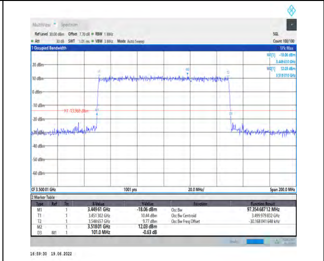
1-N78-3450-3550-PC2-30-100-M-8-CP-64QAM-Outer_Full-273@0-Ant1-97.355-101.000-≤100-PASS
