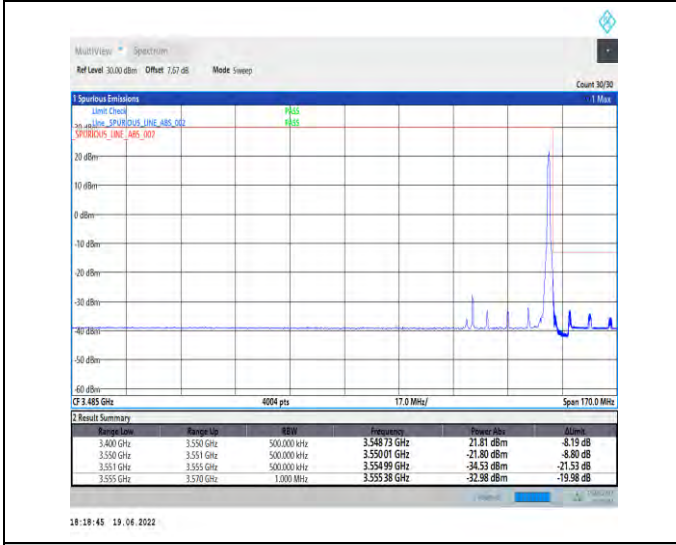
1-N78-3450-3550-PC2-30-50-H-5-CP-QPSK-Edge_1RB_Right-1@132-Ant1-PASS-see graph
