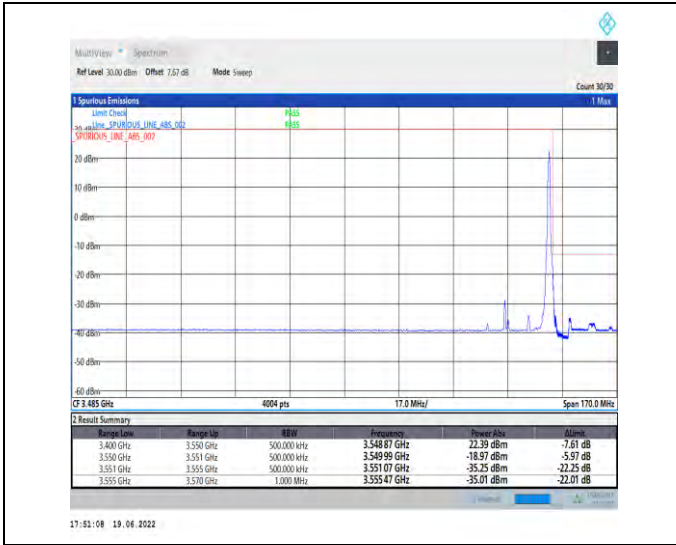
1-N78-3450-3550-PC2-30-30-H-2-DFT-PI2BPSK-Edge_1RB_Right-1@77-Ant1-PASS-see graph
