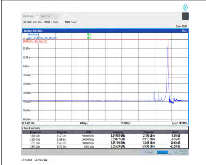
1-N78-3450-3550-PC2-30-20-H-5-CP-QPSK-Edge_1RB_Right-1@50-Ant1-PASS-see graph
