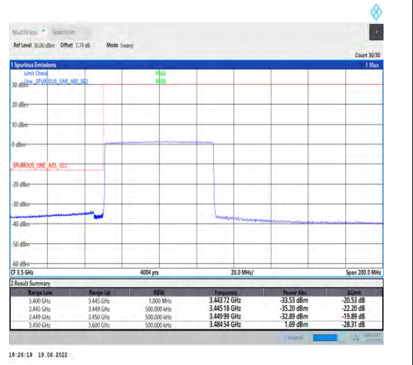
1-N78-3450-3550-PC2-30-60-L-6-CP-QPSK-Outer_Full-162@0-Ant1-PASS-see graph
