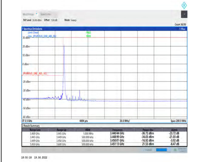
1-N78-3450-3550-PC2-30-40-L-4-CP-QPSK-Edge_1RB_Left-1@0-Ant1-PASS-see graph
