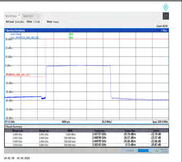
1-N78-3450-3550-PC2-30-80-L-6-CP-QPSK-Outer_Full-217@0-Ant1-PASS-see graph
