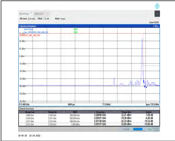
1-N78-3450-3550-PC2-30-70-H-2-DFT-PI2BPSK-Edge_1RB_Right-1@188-Ant1-PASS-see graph
