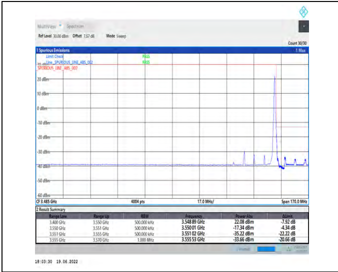
1-N78-3450-3550-PC2-30-40-H-2-DFT-PI2BPSK-Edge_1RB_Right-1@105-Ant1-PASS-see graph
