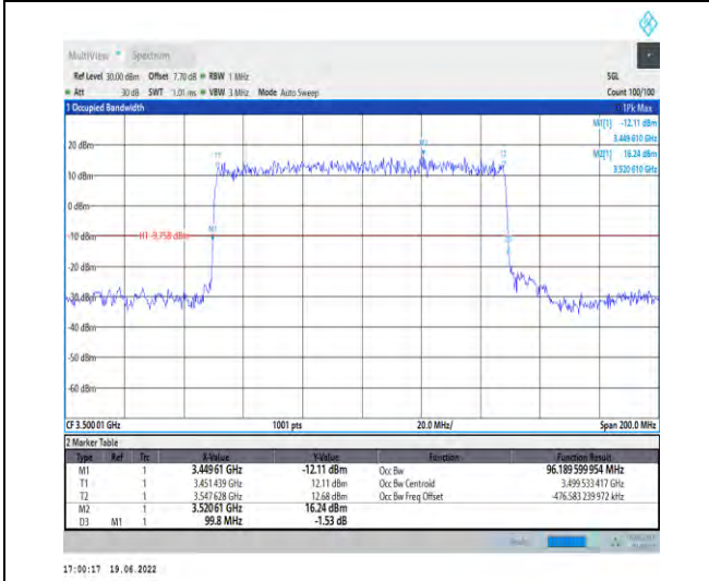
1-N78-3450-3550-PC2-30-100-H-2-DFT-PI2BPSK-Outer_Full-270@0-Ant1-96.19-99.800-≤100-PASS
