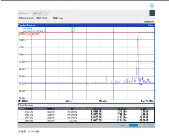
1-N78-3450-3550-PC2-30-80-H-2-DFT-PI2BPSK-Edge_1RB_Right-1@216-Ant1-PASS-see graph
