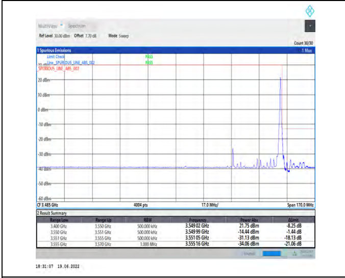
1-N78-3450-3550-PC2-30-60-H-5-CP-QPSK-Edge_1RB_Right-1@161-Ant1-PASS-see graph
