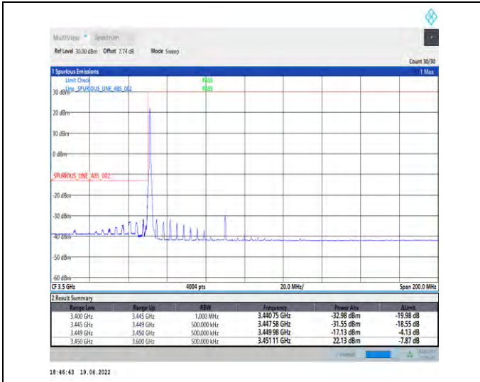
1-N78-3450-3550-PC2-30-80-L-1-DFT-PI2BPSK-Edge_1RB_Left-1@0-Ant1-PASS-see graph
