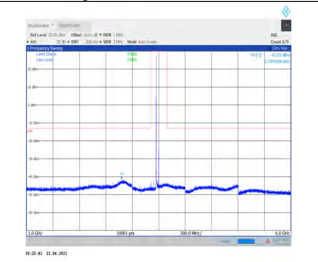
1-N78-3450-3550--30-100-M-1-DFT-PI2BPSK-Inner_ 1RB_Left-1@1-1000-6000-Ant1--41.68--13-PASS
