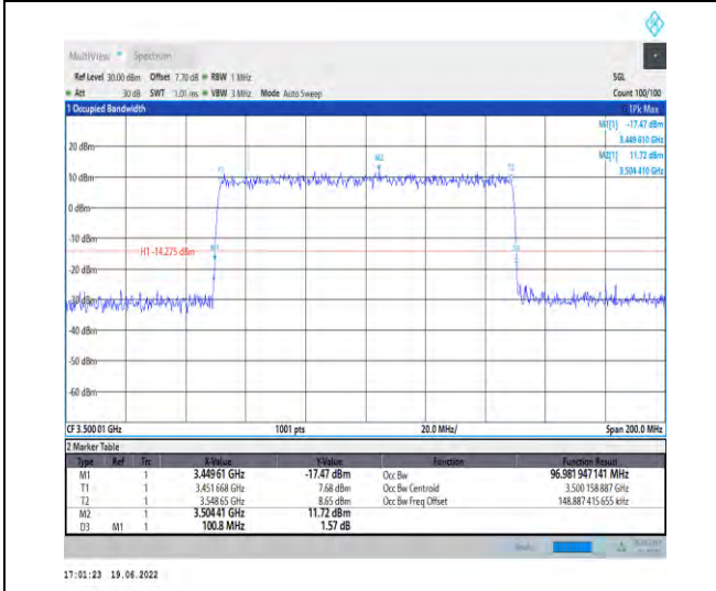
1-N78-3450-3550-PC2-30-100-H-6-CP-QPSK-Outer _Full-273@0-Ant1-96.982-100.800-≤100-PASS
