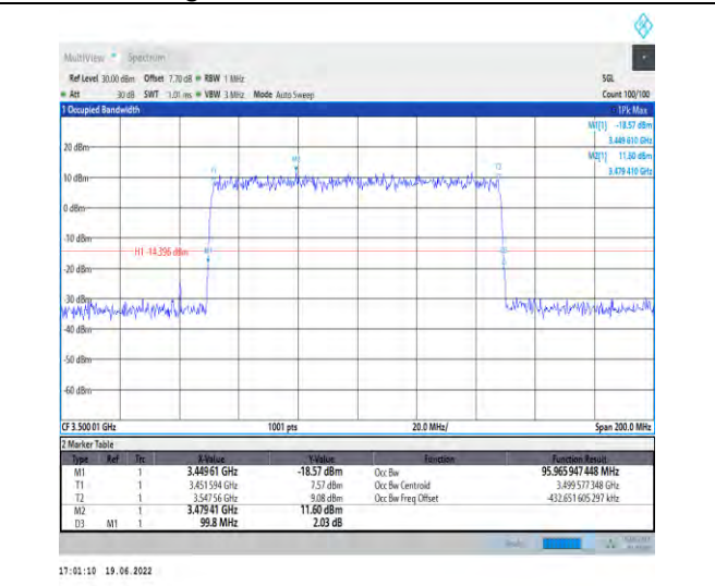
1-N78-3450-3550-PC2-30-100-H-5-DFT-256QAM-O uter_Full-270@0-Ant1-95.966-99.800-≤100-PASS
