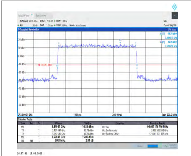
1-N78-3450-3550-PC2-30-100-M-1-DFT-QPSK-Outer_Full-270@0-Ant1-96.097-99.800-≤100-PASS
