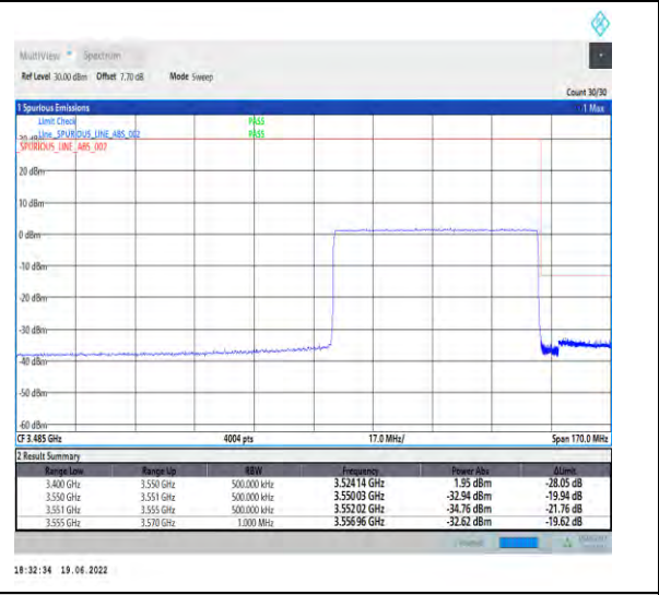
1-N78-3450-3550-PC2-30-60-H-6-CP-QPSK-Outer_Full-162@0-Ant1-PASS-see graph
