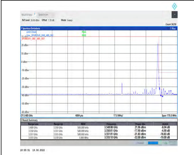
1-N78-3450-3550-PC2-30-80-H-5-CP-QPSK-Edge_1RB_Right-1@216-Ant1-PASS-see graph
