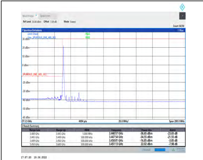
1-N78-3450-3550-PC2-30-40-L-1-DFT-PI2BPSK-Edge_1RB_Left-1@0-Ant1-PASS-see graph
