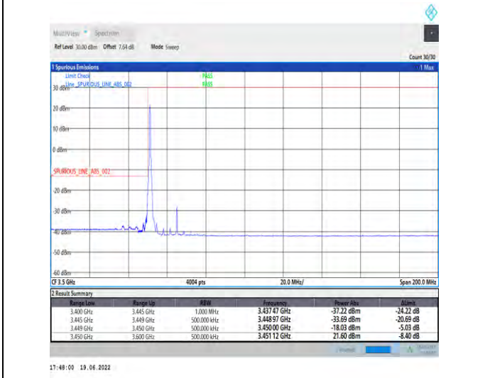
1-N78-3450-3550-PC2-30-30-L-4-CP-QPSK-Edge_1RB_Left-1@0-Ant1-PASS-see graph
