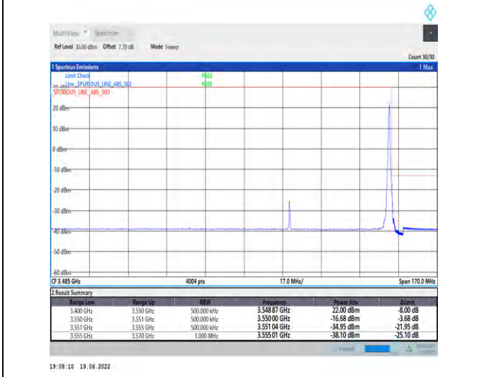
1-N78-3450-3550-PC2-30-90-H-5-CP-QPSK-Edge_1RB_Right-1@244-Ant1-PASS-see graph
