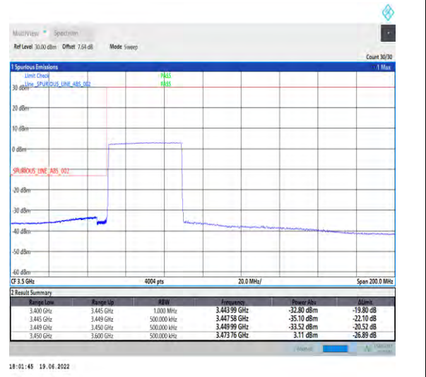
1-N78-3450-3550-PC2-30-40-L-6-CP-QPSK-Outer_Full-106@0-Ant1-PASS-see graph
