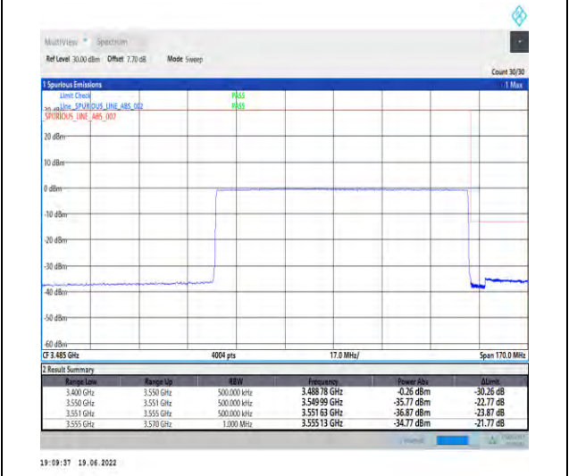
1-N78-3450-3550-PC2-30-90-H-6-CP-QPSK-Outer_Full-245@0-Ant1-PASS-see graph
