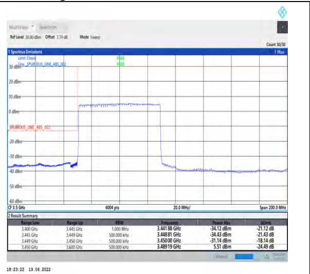
1-N78-3450-3550-PC2-30-60-L-3-DFT-PI2BPSK-Outer_Full-162@0-Ant1-PASS-see graph
