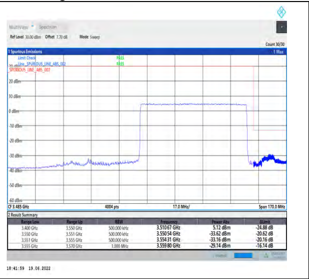
1-N78-3450-3550-PC2-30-70-H-3-DFT-PI2BPSK-Outer_Full-180@0-Ant1-PASS-see graph
