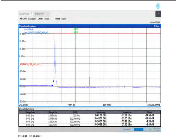
1-N78-3450-3550-PC2-30-100-L-4-CP-QPSK-Edge_1RB_Left-1@0-Ant1-PASS-see graph
