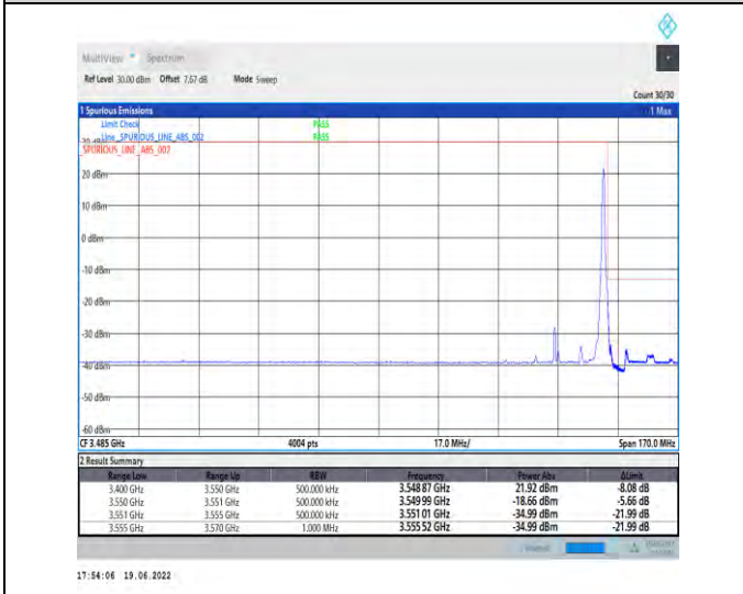
1-N78-3450-3550-PC2-30-30-H-5-CP-QPSK-Edge_1RB_Right-1@77-Ant1-PASS-see graph
