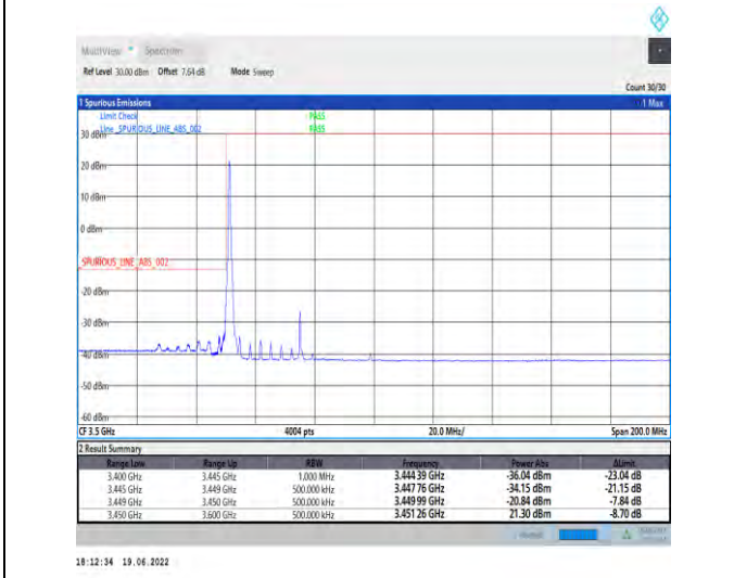
1-N78-3450-3550-PC2-30-50-L-4-CP-QPSK-Edge_1RB_Left-1@0-Ant1-PASS-see graph
