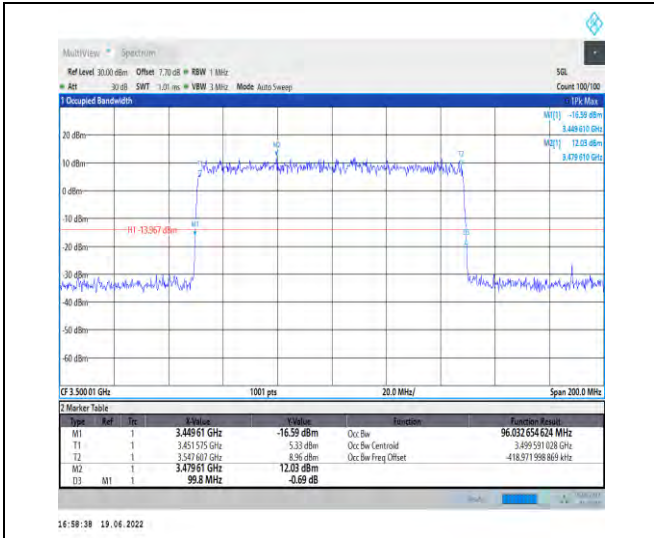
1-N78-3450-3550-PC2-30-100-M-5-DFT-256QAM-Outer_Full-270@0-Ant1-96.033-99.800-≤100-PASS
