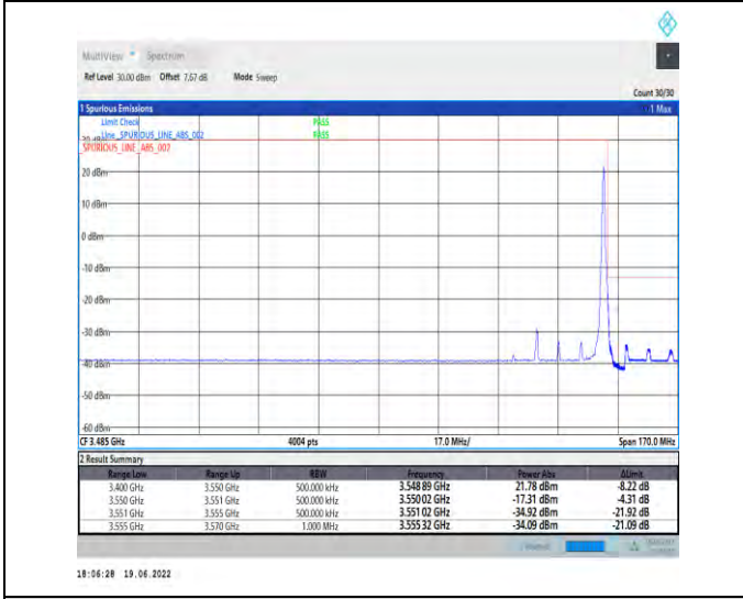
1-N78-3450-3550-PC2-30-40-H-5-CP-QPSK-Edge_1RB_Right-1@105-Ant1-PASS-see graph
