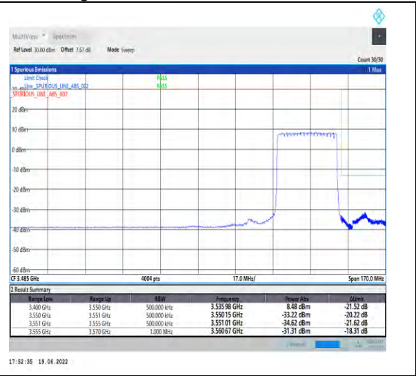
1-N78-3450-3550-PC2-30-30-H-3-DFT-PI2BPSK-Outer_Full-75@0-Ant1-PASS-see graph
