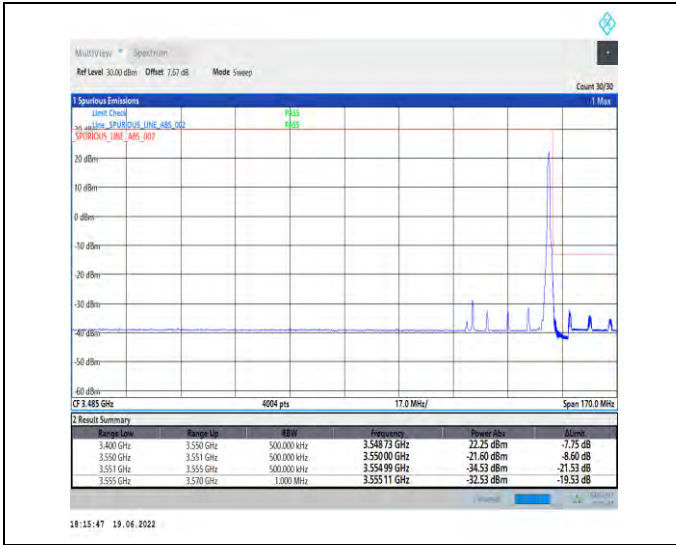
1-N78-3450-3550-PC2-30-50-H-2-DFT-PI2BPSK-Edge_1RB_Right-1@132-Ant1-PASS-see graph
