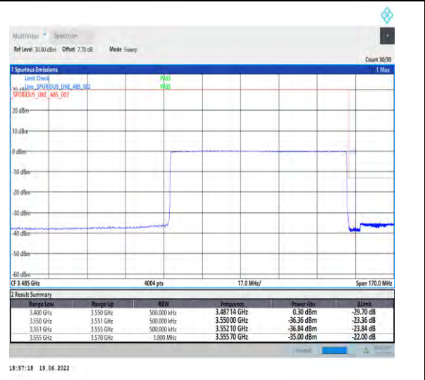
1-N78-3450-3550-PC2-30-80-H-6-CP-QPSK-Outer_Full-217@0-Ant1-PASS-see graph
