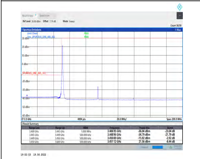
1-N78-3450-3550-PC2-30-90-L-4-CP-QPSK-Edge_1RB_Left-1@0-Ant1-PASS-see graph
