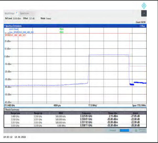
1-N78-3450-3550-PC2-30-50-H-6-CP-QPSK-Outer_Full-133@0-Ant1-PASS-see graph
