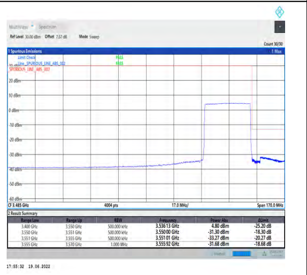
1-N78-3450-3550-PC2-30-30-H-6-CP-QPSK-Outer_Full-78@0-Ant1-PASS-see graph
