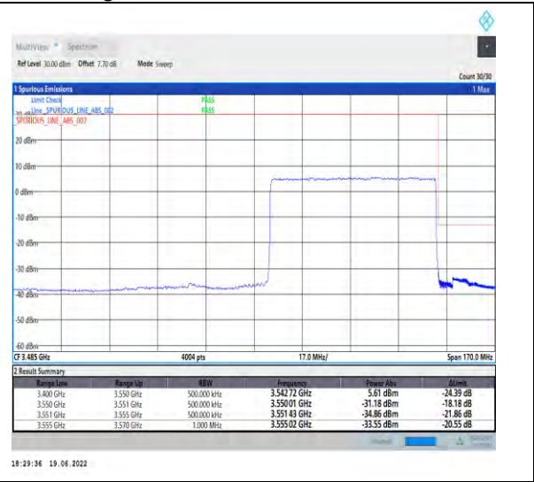
1-N78-3450-3550-PC2-30-60-H-3-DFT-PI2BPSK-Outer_Full-162@0-Ant1-PASS-see graph
