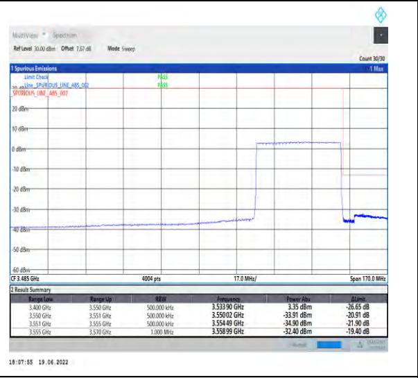
1-N78-3450-3550-PC2-30-40-H-6-CP-QPSK-Outer_Full-106@0-Ant1-PASS-see graph
