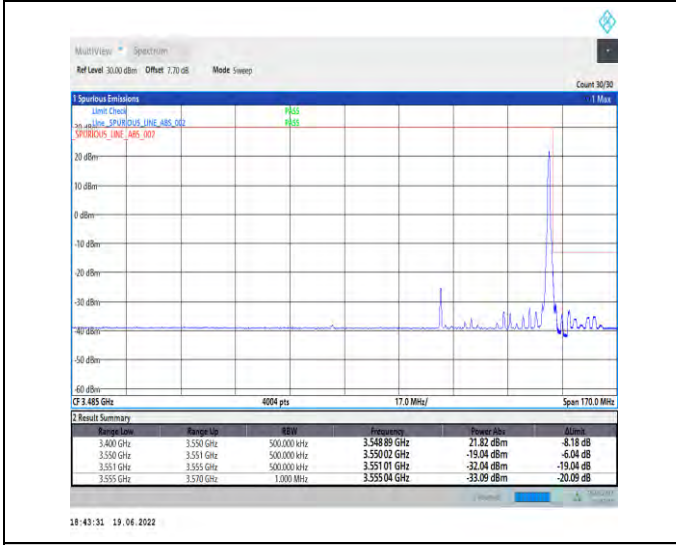
1-N78-3450-3550-PC2-30-70-H-5-CP-QPSK-Edge_1RB_Right-1@188-Ant1-PASS-see graph
