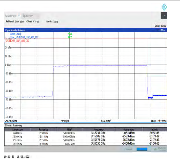
1-N78-3450-3550-PC2-30-100-H-6-CP-QPSK-Outer_Full-273@0-Ant1-PASS-see graph
