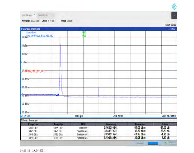
1-N78-3450-3550-PC2-30-100-L-1-DFT-PI2BPSK-Edge_e_1RB_Left-1@0-Ant1-PASS-see graph
