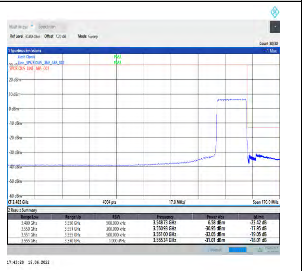
1-N78-3450-3550-PC2-30-20-H-6-CP-QPSK-Outer_Full-51@0-Ant1-PASS-see graph
