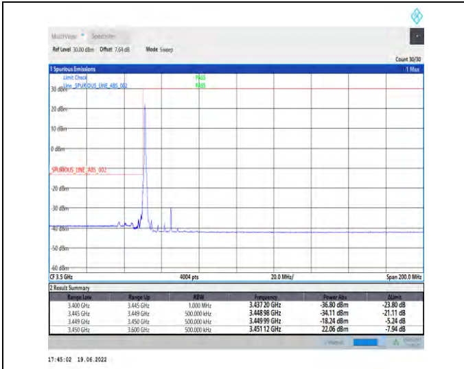
1-N78-3450-3550-PC2-30-30-L-1-DFT-PI2BPSK-Edge_1RB_Left-1@0-Ant1-PASS-see graph
