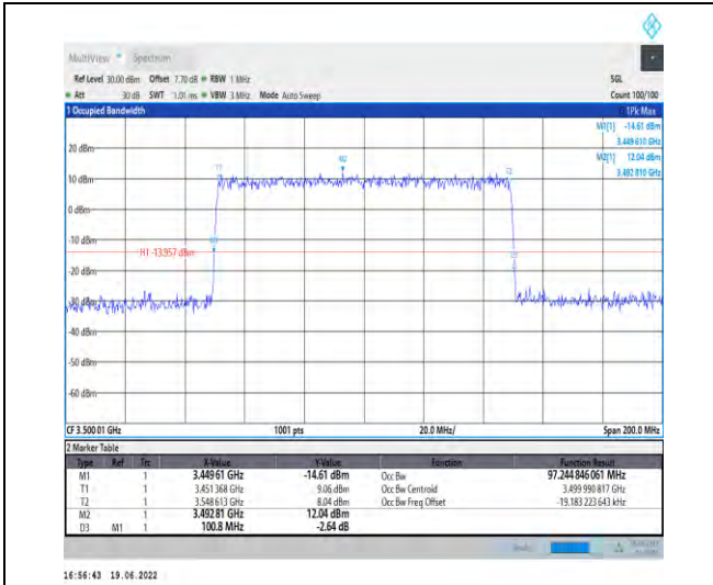
1-N78-3450-3550-PC2-30-100-L-6-CP-QPSK-Outer_Full-273@0-Ant1-97.245-100.800-≤100-PASS
