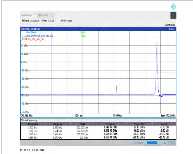
1-N78-3450-3550-PC2-30-90-H-2-DFT-PI2BPSK-Edge_1RB_Right-1@244-Ant1-PASS-see graph
