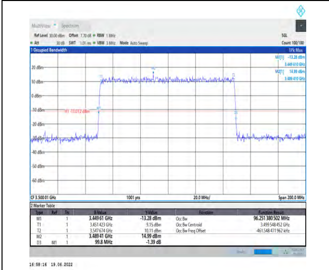
1-N78-3450-3550-PC2-30-100-M-3-DFT-16QAM-Outer_Full-270@0-Ant1-96.251-99.800-≤100-PASS
