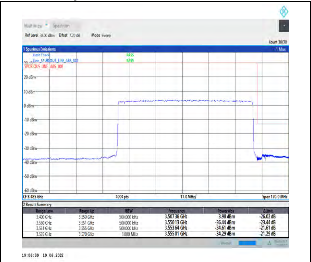
1-N78-3450-3550-PC2-30-90-H-3-DFT-PI2BPSK-Outer_Full-240@0-Ant1-PASS-see graph
