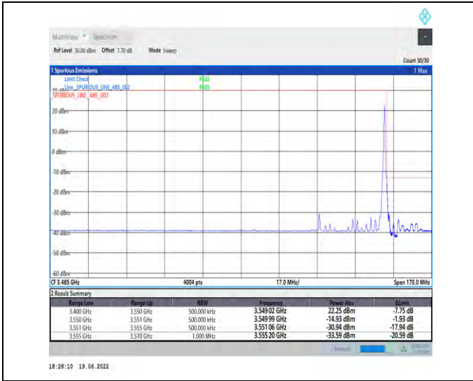
1-N78-3450-3550-PC2-30-60-H-2-DFT-PI2BPSK-Edge_1RB_Right-1@161-Ant1-PASS-see graph
