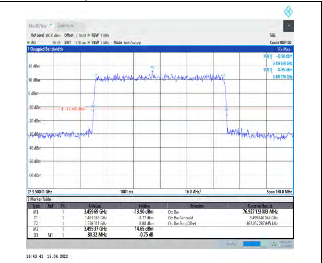
1-N78-3450-3550-PC2-30-80-M-4-DFT-64QAM-Out er_Full-216@0-Ant1-76.927-80.320-≤80-PASS
