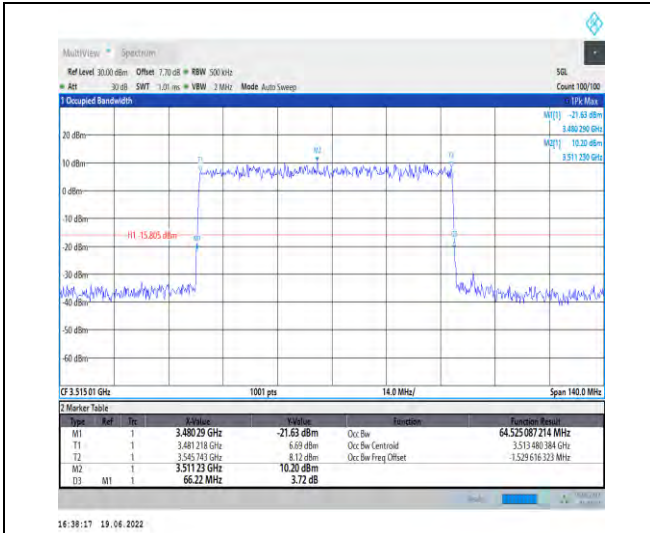
1-N78-3450-3550-PC2-30-70-H-5-DFT-256QAM-Out er_Full-180@0-Ant1-64.525-66.220-≤70-PASS
