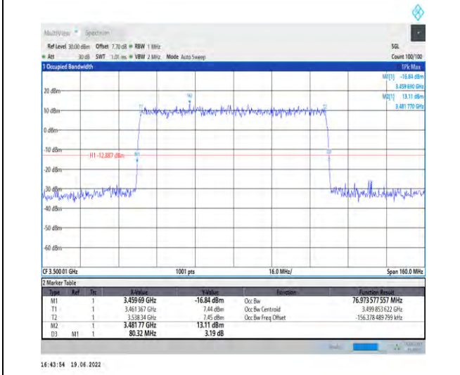
1-N78-3450-3550-PC2-30-80-M-5-DFT-256QAM-Out er_Full-216@0-Ant1-76.974-80.320-≤80-PASS
