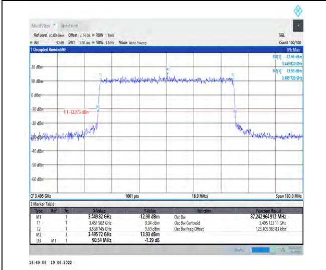
1-N78-3450-3550-PC2-30-90-L-7-CP-16QAM-Outer _Full-245@0-Ant1-87.243-90.540-≤90-PASS
