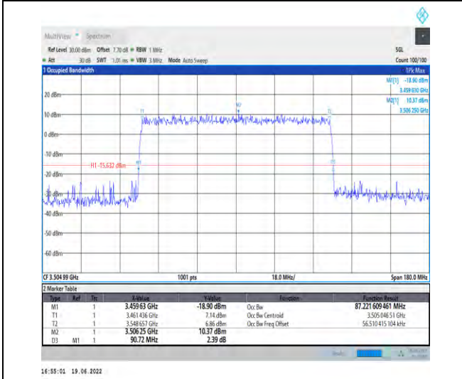
1-N78-3450-3550-PC2-30-90-H-9-CP-256QAM-Outer _Full-245@0-Ant1-87.222-90.720-≤90-PASS
