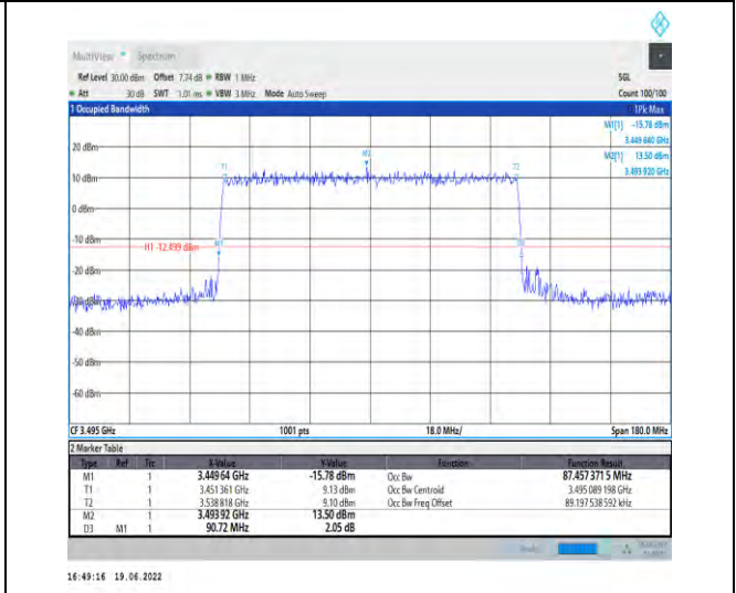
1-N78-3450-3550-PC2-30-90-L-8-CP-64QAM-Outer _Full-245@0-Ant1-87.457-90.720-≤90-PASS
