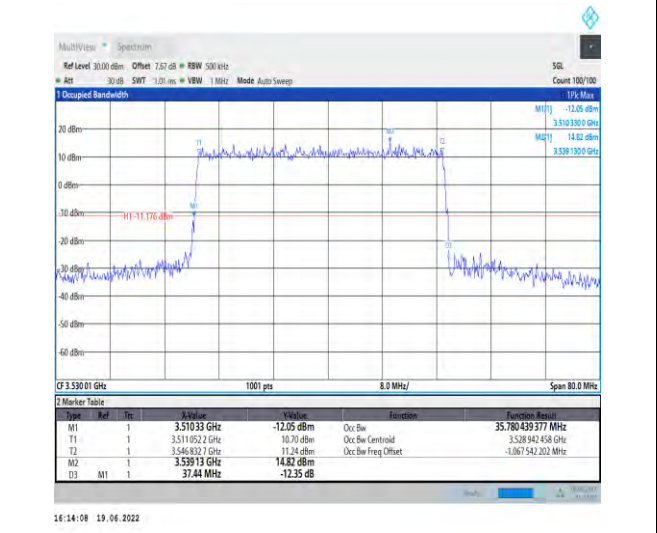
1-N78-3450-3550-PC2-30-40-H-4-DFT-64QAM-Oute r_Full-100@0-Ant1-35.78-37.440-≤40-PASS
