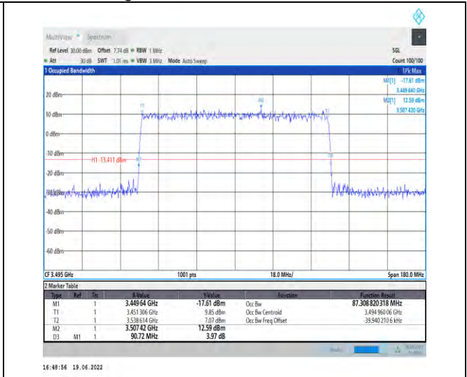
1-N78-3450-3550-PC2-30-90-L-6-CP-QPSK-Outer Full-245@0-Ant1-87.309-90.720-≤90-PASS
