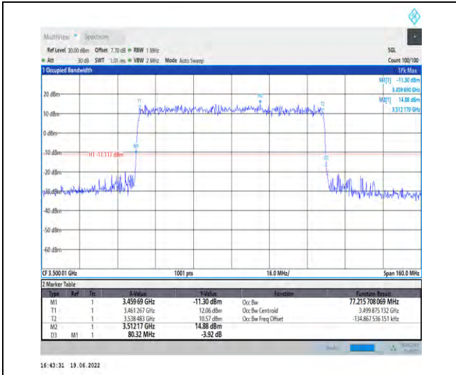
1-N78-3450-3550-PC2-30-80-M-3-DFT-16QAM-Out er_Full-216@0-Ant1-77.216-80.320-≤80-PASS
