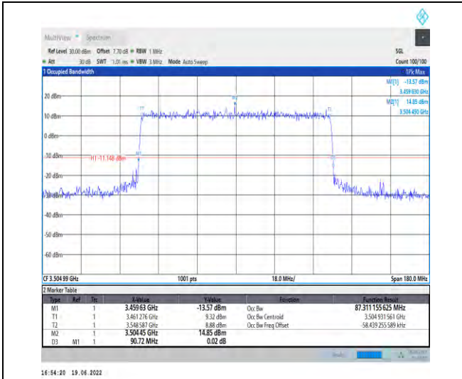
1-N78-3450-3550-PC2-30-90-H-7-CP-16QAM-Outer _Full-245@0-Ant1-87.311-90.720-≤90-PASS
