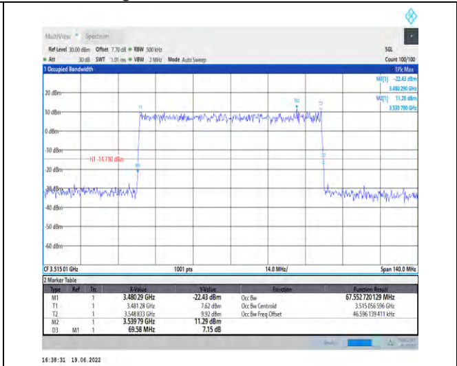
1-N78-3450-3550-PC2-30-70-H-6-CP-QPSK-Outer Full-189@0-Ant1-67.553-69.580-≤70-PASS
