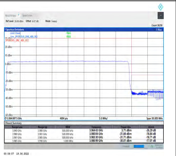
1-N77-3700-3980--30-40-H-6-CP-QPSK-Outer_Full-106@0-Ant1-PASS-see graph
