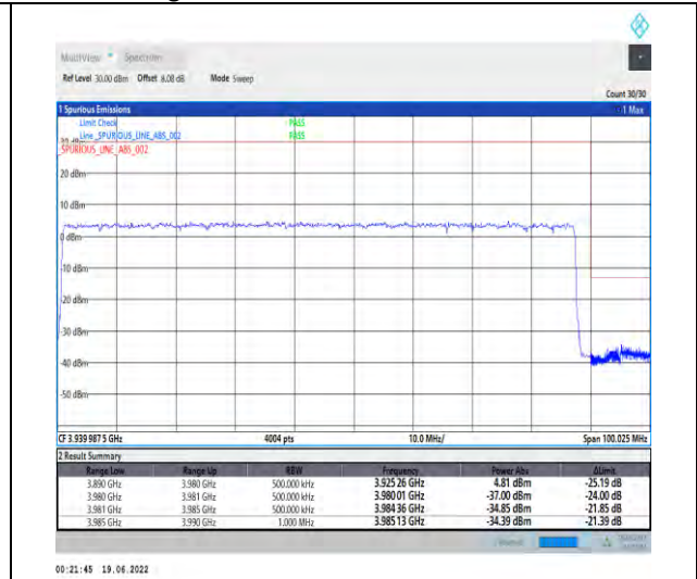
1-N77-3700-3980--30-90-H-3-DFT-PI2BPSK-Outer_Full-240@0-Ant1-PASS-see graph
