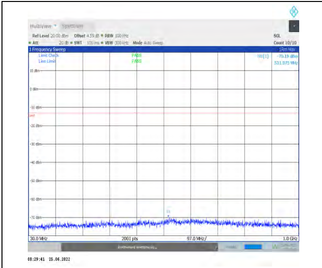
1-N77-3700-3980--30-100-M-1-DFT-PI2BPSK-Inner _1RB_Left-1@1-30-1000-Ant1--70.18--13-PASS
