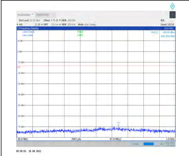
1-N77-3700-3980--30-100-H-1-DFT-PI2BPSK-Inner _1RB_Left-1@1-30-1000-Ant1--69.59--13-PASS
