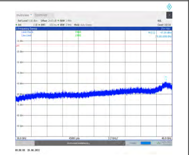
1-N77-3700-3980--30-100-M-1-DFT-PI2BPSK-Inner_ 1RB_Left-1@1-18000-40000-Ant1--47.16--13-PASS
