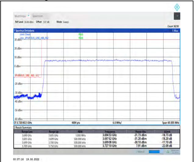
1-N77-3700-3980--30-50-L-3-DFT-PI2BPSK-Outer_Full-128@0-Ant1-PASS-see graph
