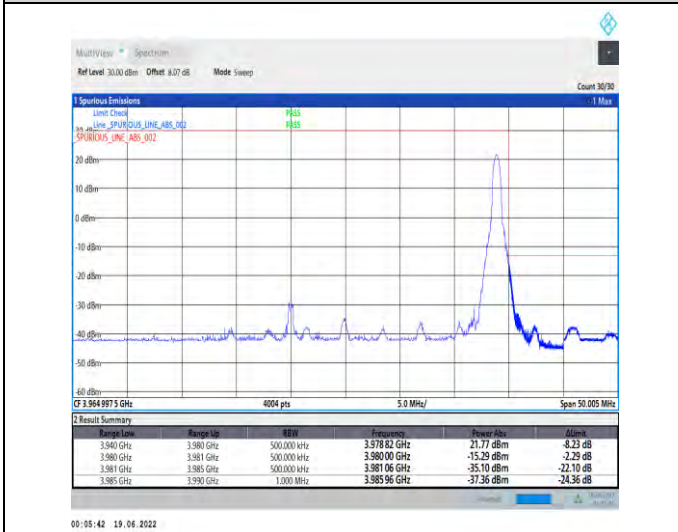
1-N77-3700-3980--30-40-H-5-CP-QPSK-Edge_1RB_Right-1@105-Ant1-PASS-see graph
