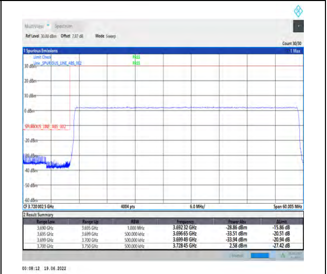
1-N77-3700-3980--30-50-L-6-CP-QPSK-Outer_Ful_I-133@0-Ant1-PASS-see graph
