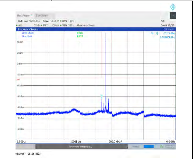
1-N77-3700-3980--30-100-M-1-DFT-PI2BPSK-Inner_ 1RB_Left-1@1-1000-6000-Ant1--32.22--13-PASS
