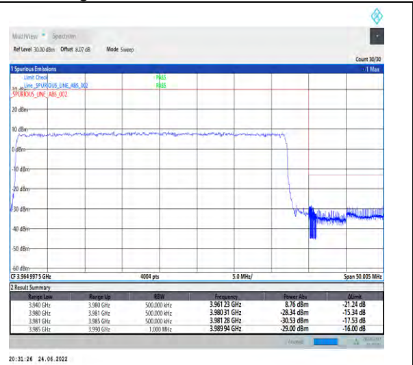
1-N77-3700-3980--30-40-H-3-DFT-PI2BPSK-Outer_Full-100@0-Ant1-PASS-see graph
