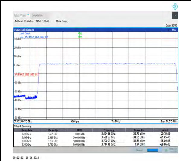
1-N77-3700-3980--30-60-L-6-CP-QPSK-Outer_Ful_I-162@0-Ant1-PASS-see graph
