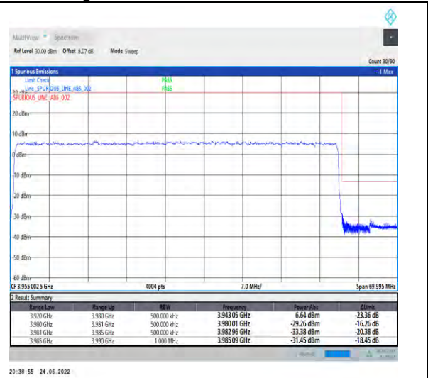
1-N77-3700-3980--30-60-H-3-DFT-PI2BPSK-Outer_Full-162@0-Ant1-PASS-see graph
