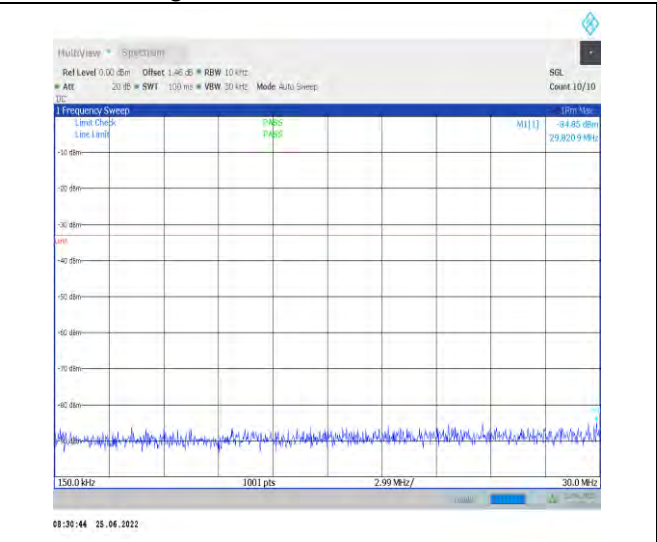
1-N77-3700-3980--30-100-H-1-DFT-PI2BPSK-Inner_ 1RB_Left-1@1-0.15-30-Ant1--84.85--33-PASS
