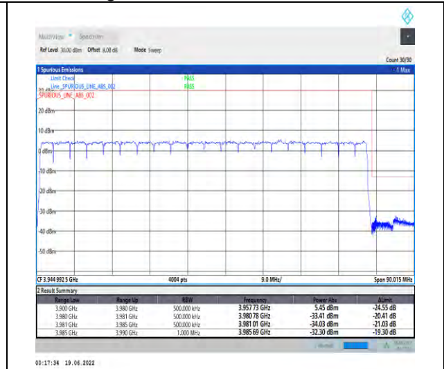
1-N77-3700-3980--30-80-H-3-DFT-PI2BPSK-Outer_Full-216@0-Ant1-PASS-see graph
