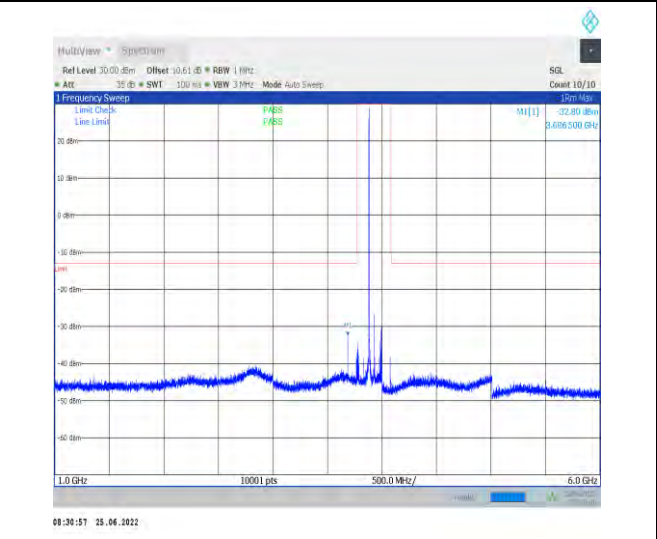
1-N77-3700-3980--30-100-H-1-DFT-PI2BPSK-Inner_ 1RB_Left-1@1-1000-6000-Ant1--32.80--13-PASS
