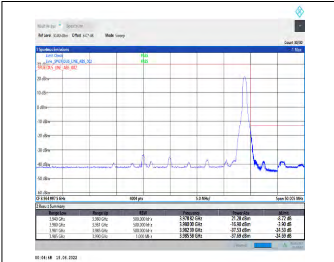
1-N77-3700-3980--30-40-H-2-DFT-PI2BPSK-Edge_1R_B_Right-1@105-Ant1-PASS-see graph
