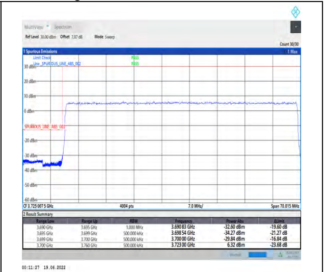
1-N77-3700-3980--30-60-L-3-DFT-PI2BPSK-Outer_Full-162@0-Ant1-PASS-see graph
