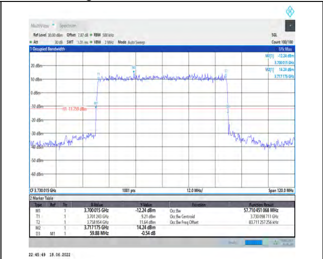
1-N77-3700-3980--30-60-L-2-DFT-PI2BPSK-Outer_Full-162@0-Ant1-57.71-59.880-≤60-PASS
