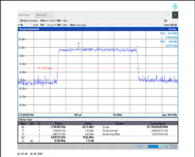
1-N77-3700-3980--30-90-M-9-CP-256QAM-Outer_Full-245@0-Ant1-87.136-91.080-<=90-PASS
