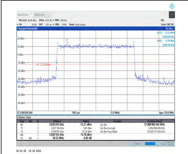
1-N77-3700-3980--30-60-H-1-DFT-QPSK-Outer_Full -162@0-Ant1-57.801-59.520-≤60-PASS
