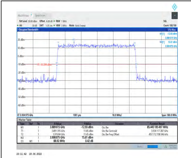
1-N77-3700-3980--30-90-H-1-DFT-QPSK-Outer_Full-240@0-Ant1-85.445-88.920-<=90-PASS
