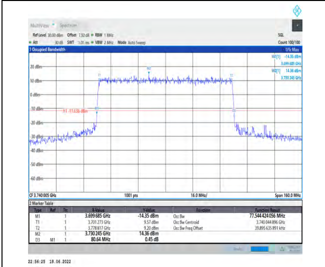
1-N77-3700-3980--30-80-L-8-CP-64QAM-Outer_Full-217@0-Ant1-77.544-80.640-<math>\leq 80</math>-PASS
