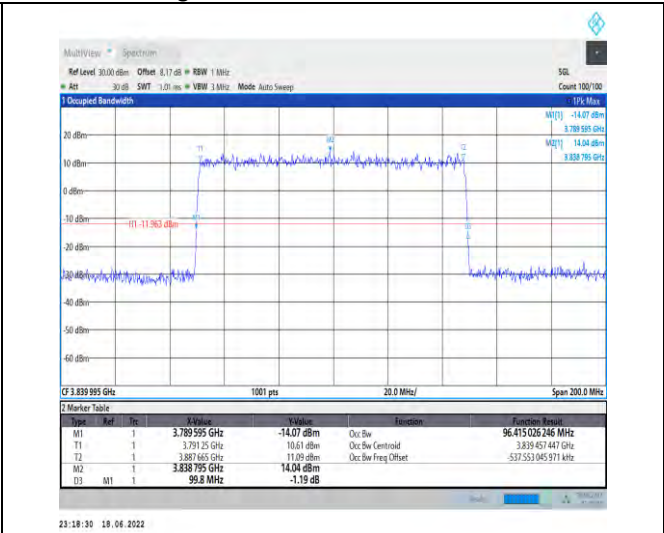
1-N77-3700-3980--30-100-M-4-DFT-64QAM-Outer_Full-270@0-Ant1-96.415-99.800-≤100-PASS
