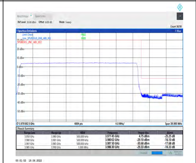
1-N77-3700-3980--30-30-H-6-CP-QPSK-Outer_Full-78@0-Ant1-PASS-see graph
