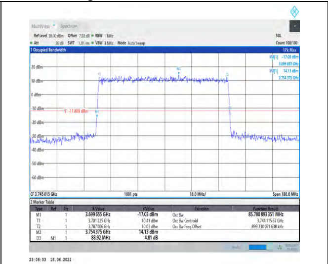
1-N77-3700-3980--30-90-L-4-DFT-64QAM-Outer_Ful I-240@0-Ant1-85.781-88.920-≤90-PASS
