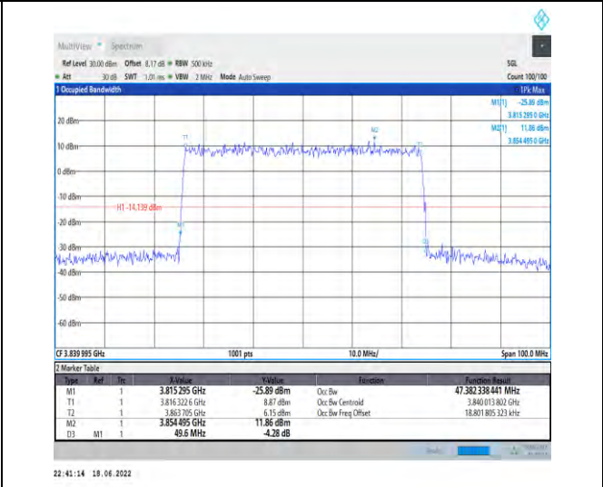
1-N77-3700-3980--30-50-M-6-CP-QPSK-Outer_Full-133@0-Ant1-47.382-49.600-<math>\leq 50</math>-PASS
