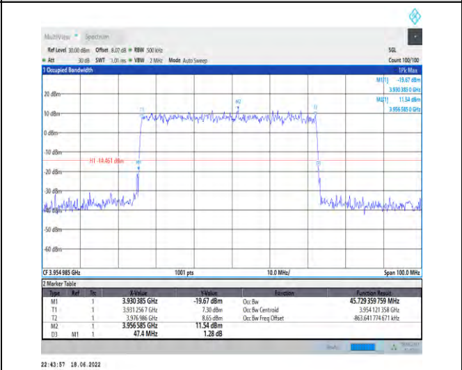
1-N77-3700-3980--30-50-H-5-DFT-256QAM-Outer_Full-128@0-Ant1-45.729-47.400-≤50-PASS
