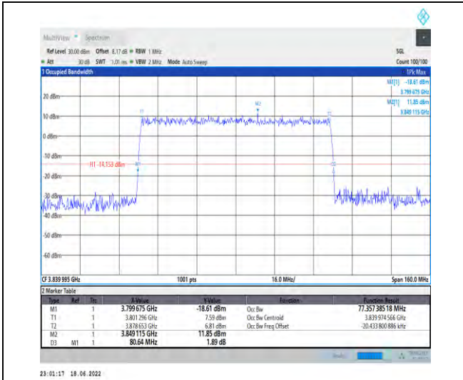
1-N77-3700-3980--30-80-M-9-CP-256QAM-Outer_Full-217@0-Ant1-77.357-80.640-≤80-PASS
