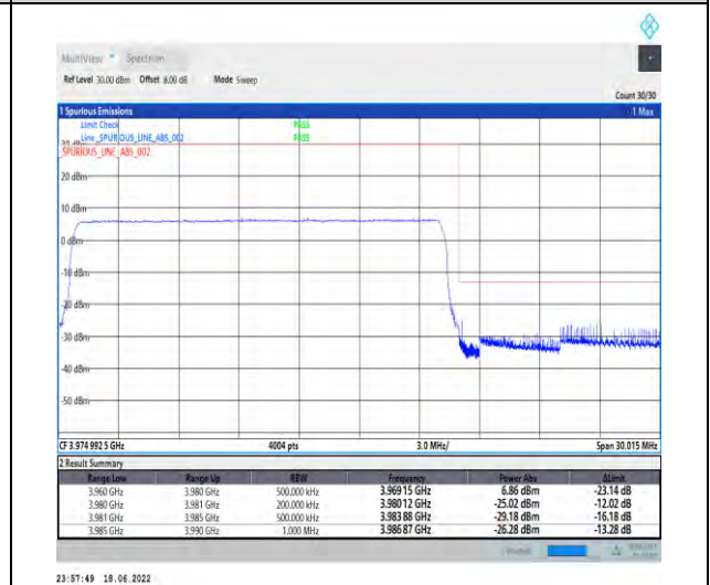
1-N77-3700-3980--30-20-H-6-CP-QPSK-Outer_Fu ll-51@0-Ant1-PASS-see graph
