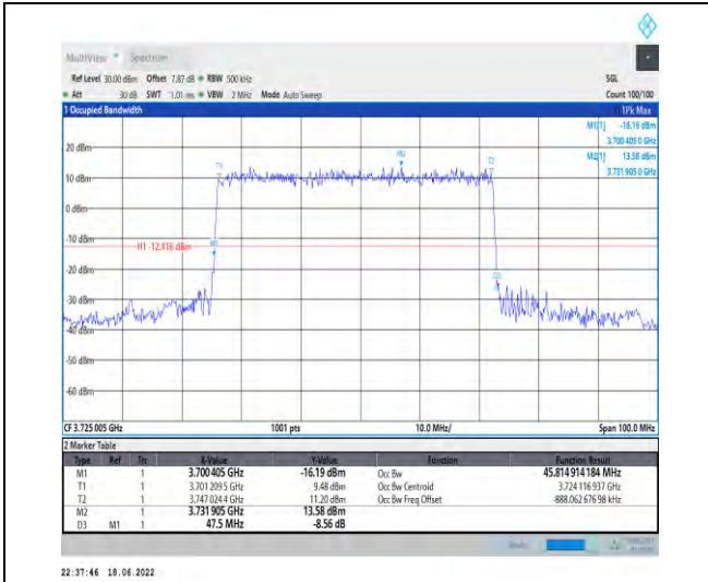
1-N77-3700-3980--30-50-L-4-DFT-64QAM-Outer_Fu II-128@0-Ant1-45.815-47.500-≤50-PASS
