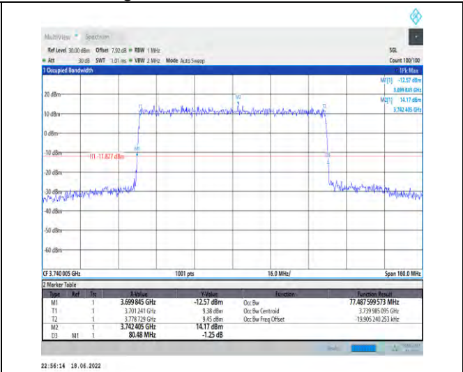
1-N77-3700-3980--30-80-L-7-CP-16QAM-Outer_Full-217@0-Ant1-77.488-80.480-<math>\leq 80</math>-PASS
