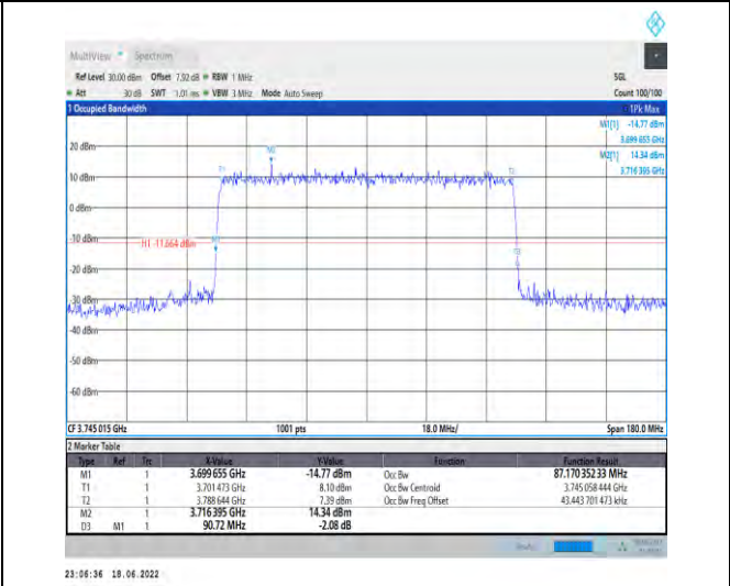
1-N77-3700-3980--30-90-L-6-CP-QPSK-Outer_Full-245@0-Ant1-87.17-90.720-≤90-PASS
