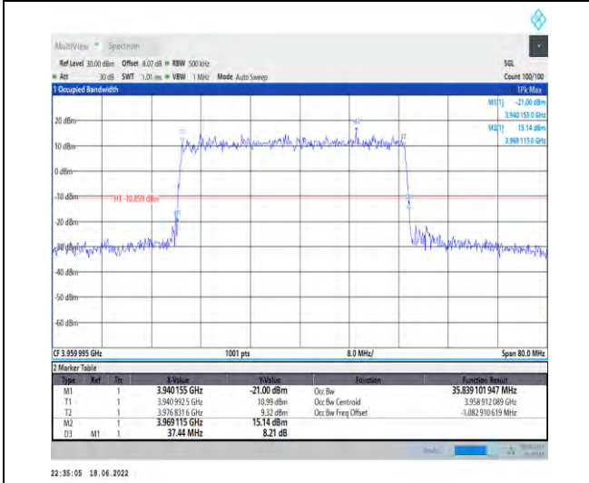
1-N77-3700-3980--30-40-H-3-DFT-16QAM-Outer_Full -100@0-Ant1-35.839-37.440-≤40-PASS
