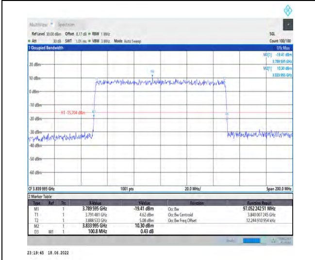
1-N77-3700-3980--30-100-M-9-CP-256QAM-Outer_Full-273@0-Ant1-97.052-100.800-≤100-PASS
