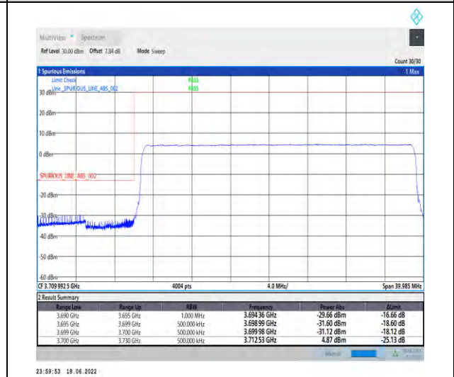
1-N77-3700-3980--30-30-L-6-CP-QPSK-Outer_Ful_l-78@0-Ant1-PASS-see graph
