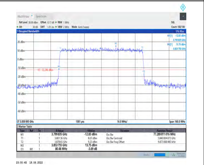
1-N77-3700-3980--30-80-M-8-CP-64QAM-Outer_Full-217@0-Ant1-77.29-80.480-<math>\leq</math>80-PASS
