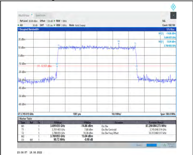
1-N77-3700-3980--30-90-L-8-CP-64QAM-Outer_Full -245@0-Ant1-87.29-90.720-≤90-PASS
