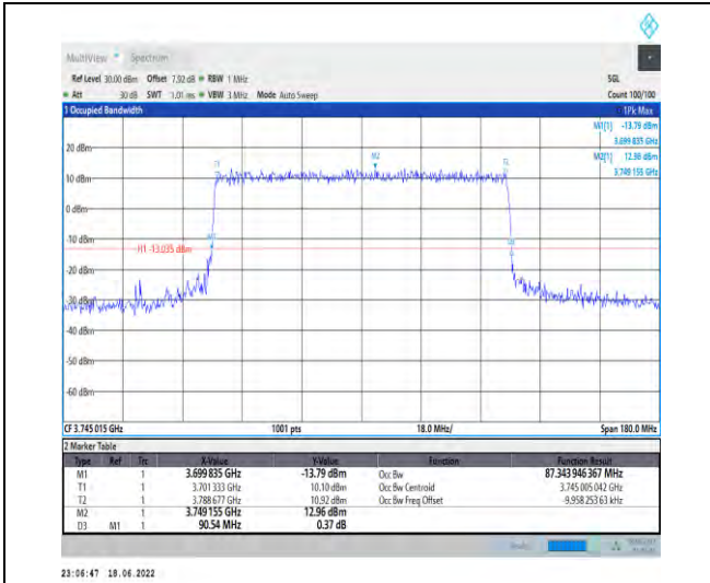
1-N77-3700-3980--30-90-L-7-CP-16QAM-Outer_Full -245@0-Ant1-87.344-90.540-≤90-PASS
