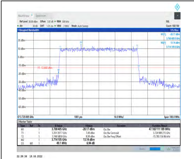
1-N77-3700-3980--30-50-L-8-CP-64QAM-Outer_Full -I-133@0-Ant1-47.183-49.100-≤50-PASS
