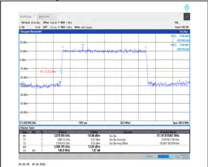
1-N77-3700-3980--30-100-H-7-CP-16QAM-Outer_Fu II-273@0-Ant1-97.142-100.800-≤100-PASS
