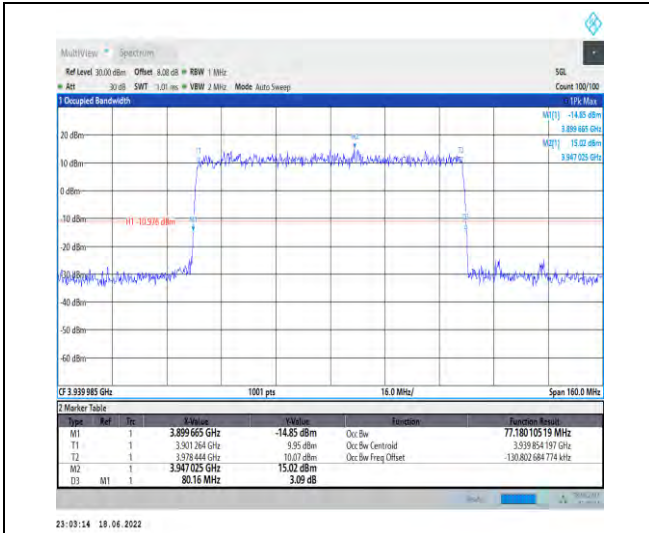
1-N77-3700-3980--30-80-H-4-DFT-64QAM-Outer_Full-216@0-Ant1-77.18-80.160-<math>\leq</math>80-PASS
