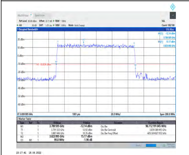
1-N77-3700-3980--30-100-M-1-DFT-QPSK-Outer_F ull-270@0-Ant1-96.112-99.800-≤100-PASS
