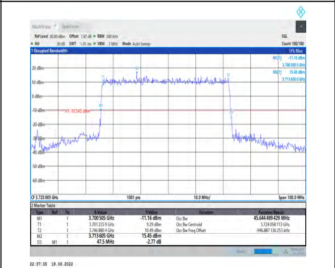
1-N77-3700-3980--30-50-L-3-DFT-16QAM-Outer_Full-128@0-Ant1-45.644-47.500-≤50-PASS
