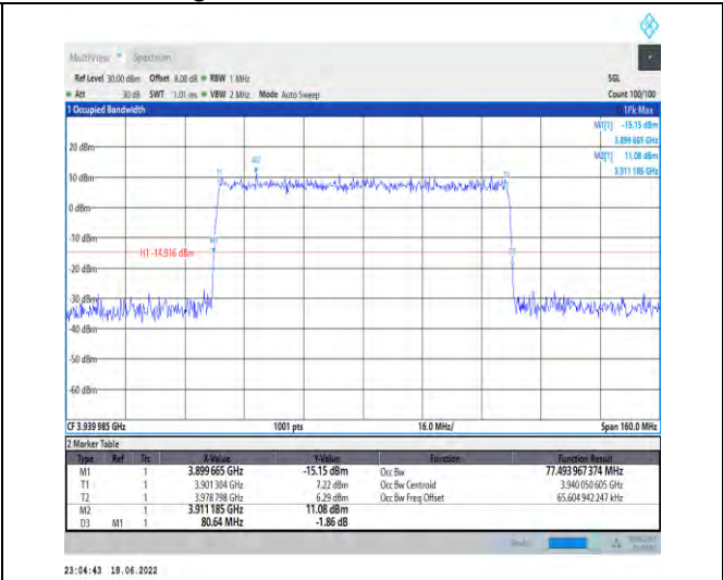
1-N77-3700-3980--30-80-H-9-CP-256QAM-Outer_Fu II-217@0-Ant1-77.494-80.640-<math>\leq 80</math>-PASS
