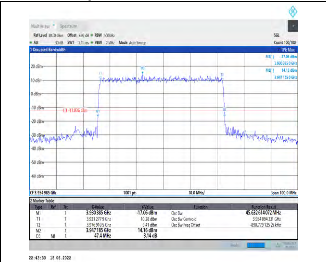
1-N77-3700-3980--30-50-H-3-DFT-16QAM-Outer_Full-128@0-Ant1-45.633-47.400-≤50-PASS
