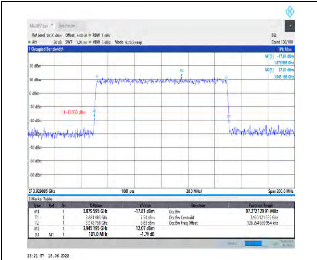
1-N77-3700-3980--30-100-H-6-CP-QPSK-Outer_Ful I-273@0-Ant1-97.272-101.000-≤100-PASS
