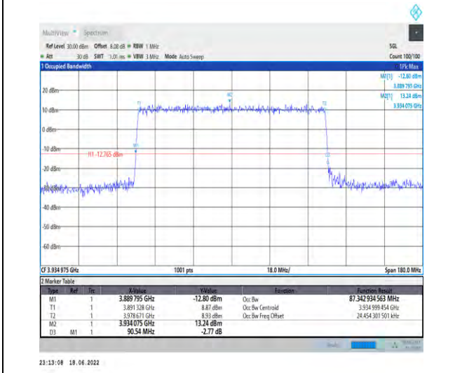
1-N77-3700-3980--30-90-H-7-CP-16QAM-Outer_Full-245@0-Ant1-87.343-90.540-<=90-PASS
