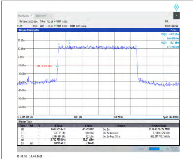
1-N77-3700-3980--30-90-L-3-DFT-16QAM-Outer_Fu II-240@0-Ant1-85.664-88.920-≤90-PASS
