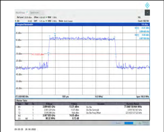
1-N77-3700-3980--30-80-H-3-DFT-16QAM-Outer_Full-216@0-Ant1-77.068-80.320-≤80-PASS
