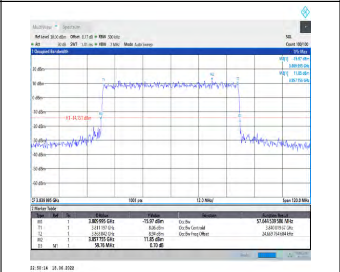
1-N77-3700-3980--30-60-M-7-CP-16QAM-Outer_Full-162@0-Ant1-57.645-59.760-≤60-PASS
