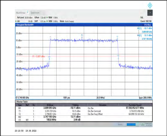
1-N77-3700-3980--30-100-L-7-CP-16QAM-Outer_Full-273@0-Ant1-97.592-100.800-≤100-PASS
