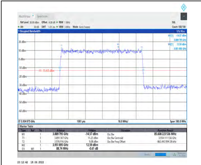
1-N77-3700-3980--30-90-H-5-DFT-256QAM-Outer_Full-240@0-Ant1-85.608-88.740-<=90-PASS
