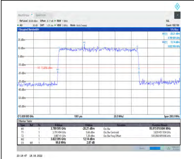
1-N77-3700-3980--30-100-M-5-DFT-256QAM-Outer_Full-270@0-Ant1-95.916-99.800-≤100-PASS
