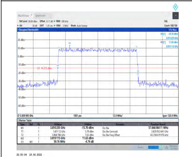
1-N77-3700-3980--30-60-M-6-CP-QPSK-Outer_Full-162@0-Ant1-57.666-59.760-≤60-PASS
