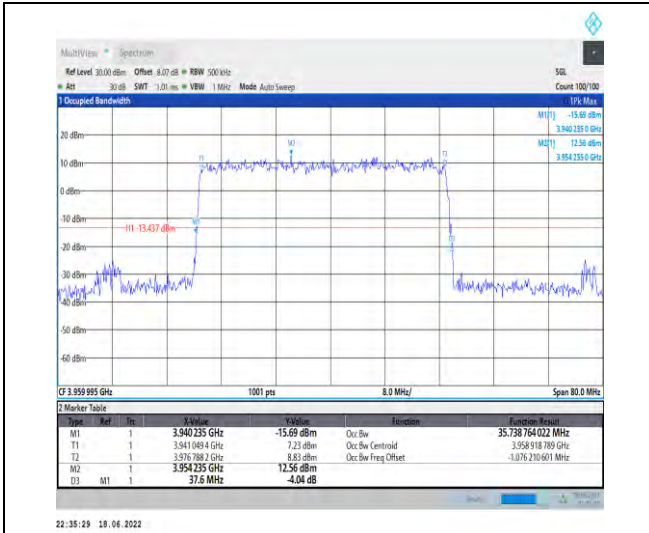
1-N77-3700-3980--30-40-H-5-DFT-256QAM-Outer_Full-100@0-Ant1-35.739-37.600-≤40-PASS
