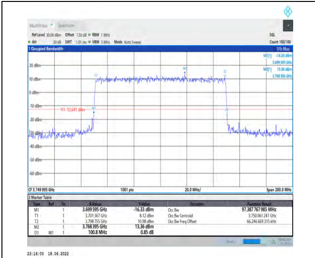
1-N77-3700-3980--30-100-L-8-CP-64QAM-Outer_F ull-273@0-Ant1-97.388-100.800-≤100-PASS
