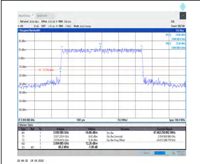
1-N77-3700-3980--30-50-H-8-CP-64QAM-Outer_Full-133@0-Ant1-47.463-49.200-<math>\leq 50</math>-PASS
