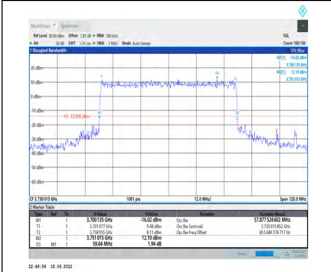
1-N77-3700-3980--30-60-L-7-CP-16QAM-Outer_Full-162@0-Ant1-57.878-59.640-≤60-PASS
