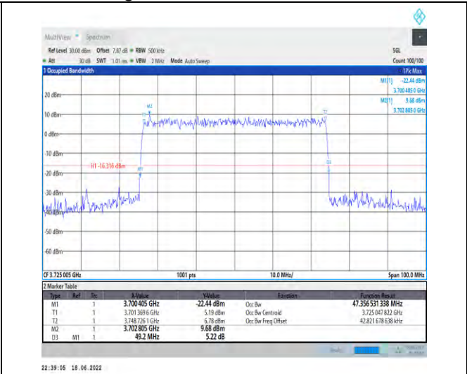
1-N77-3700-3980--30-50-L-9-CP-256QAM-Outer_Ful I-133@0-Ant1-47.357-49.200-≤50-PASS
