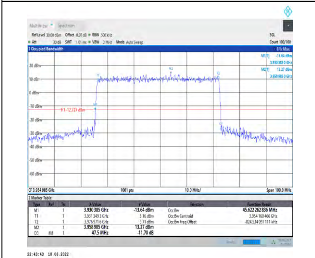
1-N77-3700-3980--30-50-H-4-DFT-64QAM-Outer_Full-128@0-Ant1-45.622-47.500-≤50-PASS
