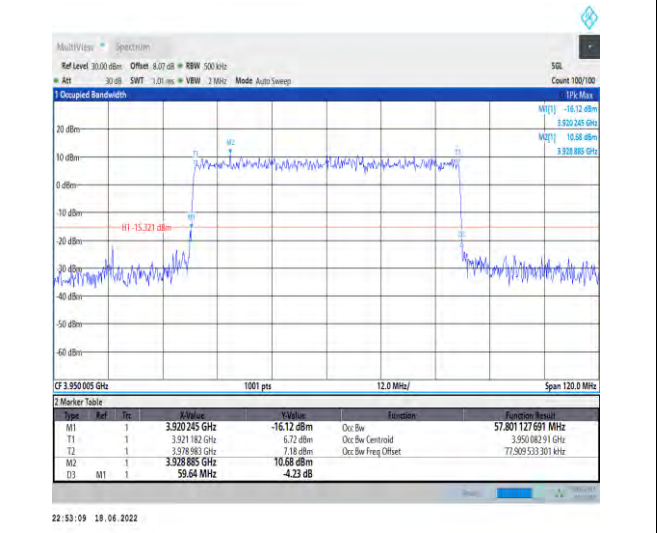
1-N77-3700-3980--30-60-H-6-CP-QPSK-Outer_Full-162@0-Ant1-57.801-59.640-≤60-PASS
