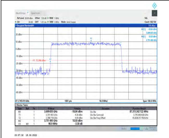
1-N77-3700-3980--30-90-L-9-CP-256QAM-Outer_Full -245@0-Ant1-87.315-90.900-≤90-PASS
