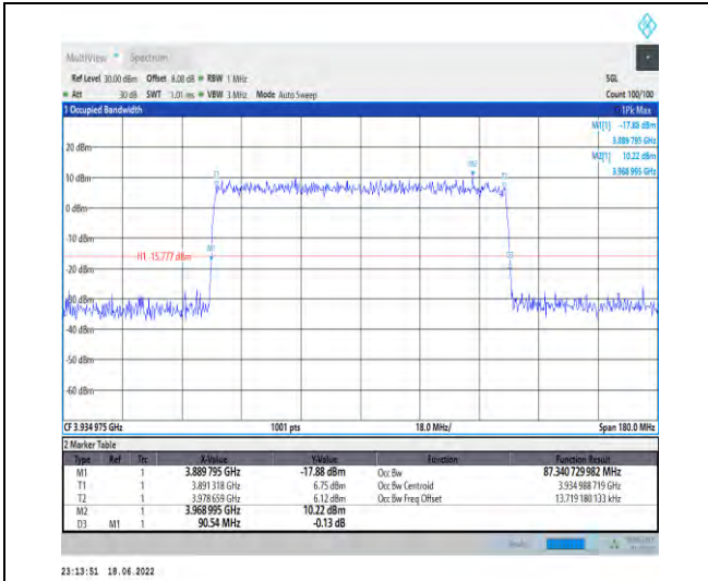
1-N77-3700-3980--30-90-H-9-CP-256QAM-Outer_Full-245@0-Ant1-87.341-90.540-≤90-PASS
