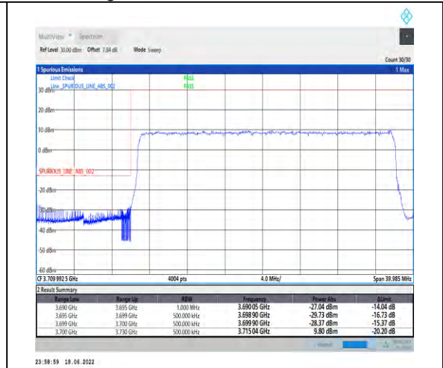
1-N77-3700-3980--30-30-L-3-DFT-PI2BPSK-Outer_Full-75@0-Ant1-PASS-see graph
