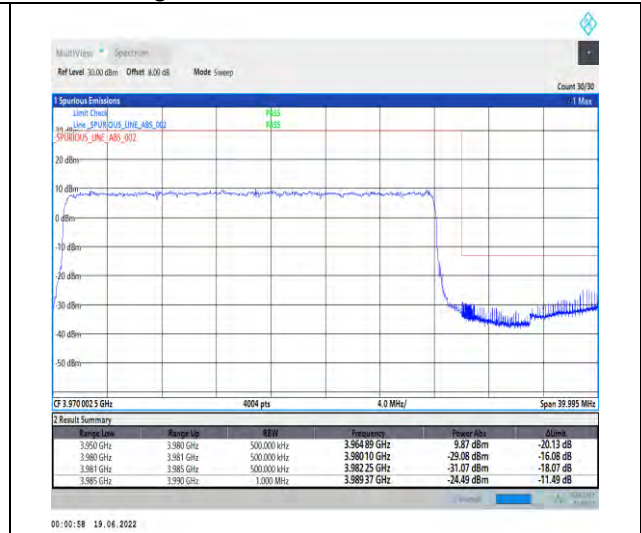
1-N77-3700-3980--30-30-H-3-DFT-PI2BPSK-Outer_Full-75@0-Ant1-PASS-see graph
