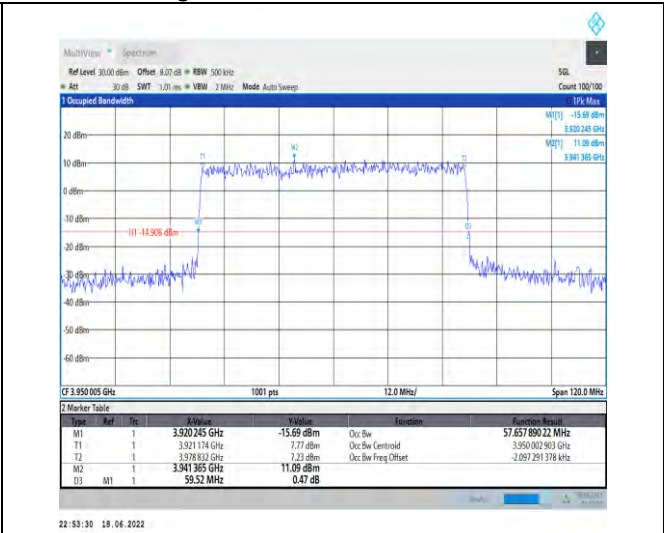
1-N77-3700-3980--30-60-H-8-CP-64QAM-Outer_Full -162@0-Ant1-57.658-59.520-≤60-PASS
