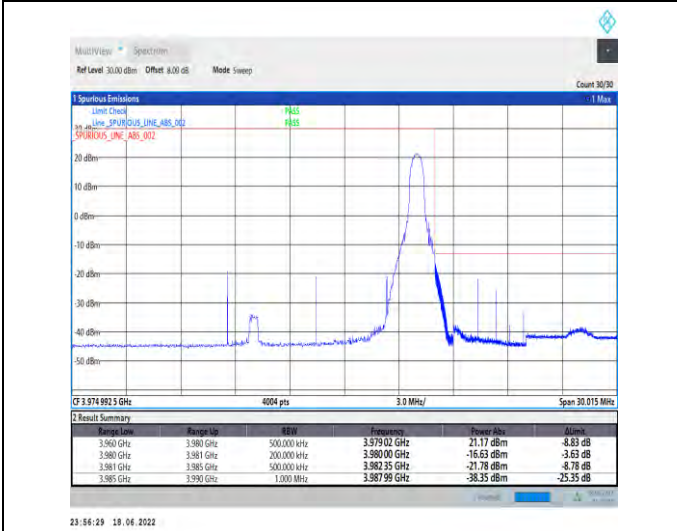
1-N77-3700-3980--30-20-H-2-DFT-PI2BPSK-Edge_1R_B_Right-1@50-Ant1-PASS-see graph
