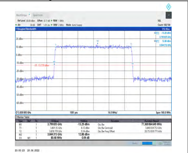
1-N77-3700-3980--30-80-M-6-CP-QPSK-Outer_Full-217@0-Ant1-77.369-80.480-<math>\leq</math>80-PASS
