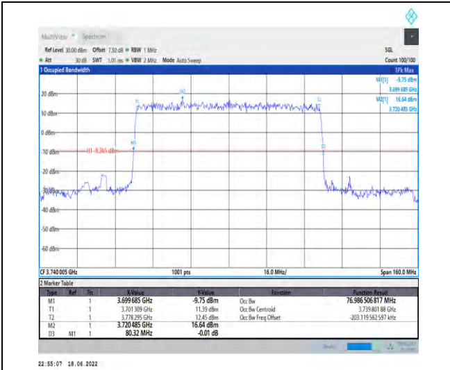
1-N77-3700-3980--30-80-L-2-DFT-PI2BPSK-Outer_Full-216@0-Ant1-76.987-80.320-<math>\leq 80</math>-PASS
