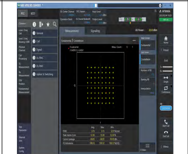
1-N77-3700-3980--30-100-M-8-CP-64QAM-Outer_F ull-273@0-Ant1-see graph-PASS
