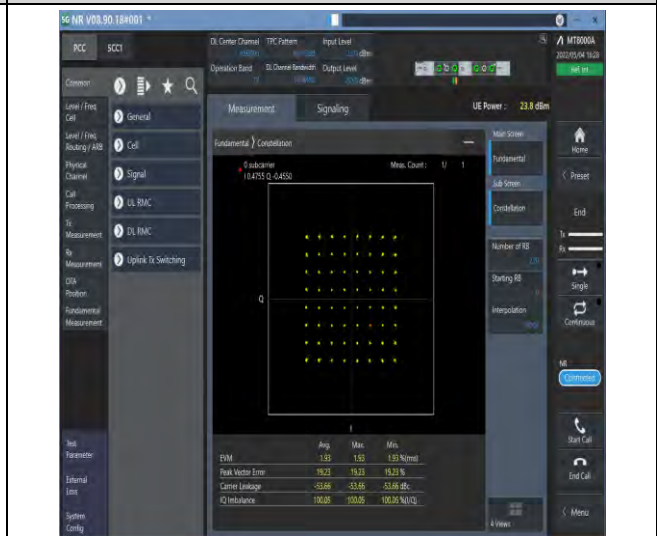
1-N77-3700-3980--30-100-M-4-DFT-64QAM-Outer_Full-270@0-Ant1-see graph-PASS
