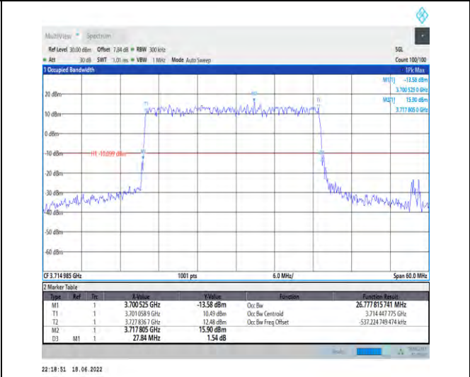
1-N77-3700-3980--30-30-L-1-DFT-QPSK-Outer_Full- 75@0-Ant1-26.778-27.840-<=30-PASS
