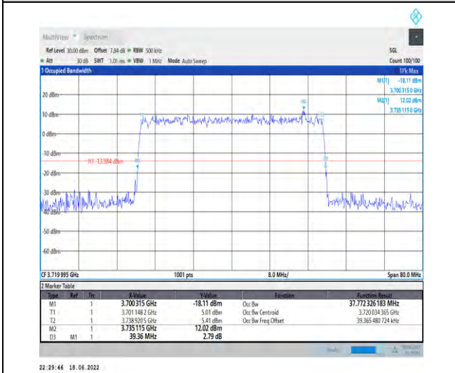
1-N77-3700-3980--30-40-L-9-CP-256QAM-Outer_Full ull-106@0-Ant1-37.772-39.360-≤40-PASS
