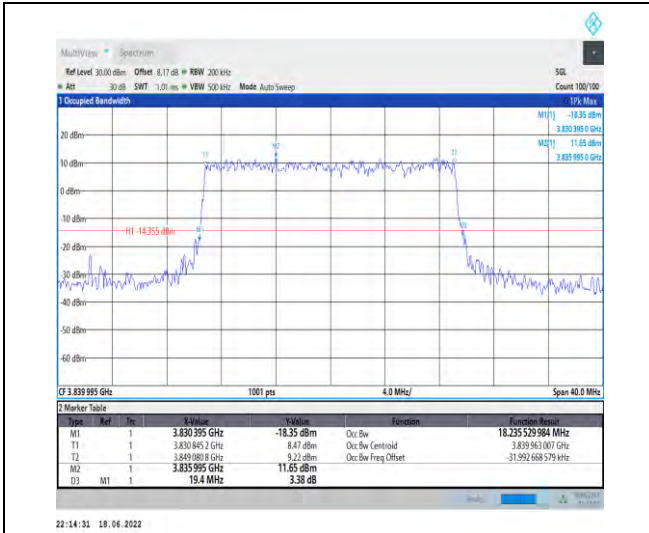
1-N77-3700-3980--30-20-M-8-CP-64QAM-Outer_Ful I-51@0-Ant1-18.236-19.400-<20-PASS
