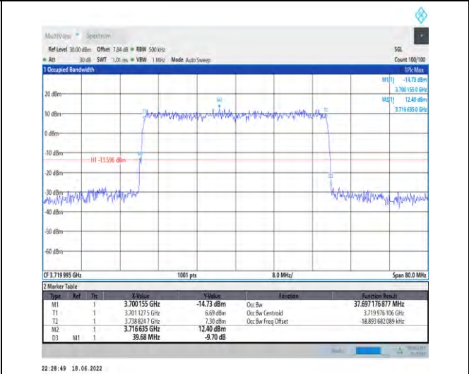
1-N77-3700-3980--30-40-L-6-CP-QPSK-Outer_Full-1 06@0-Ant1-37.697-39.680-≤40-PASS
