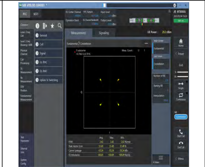
1-N77-3700-3980--30-100-M-2-DFT-QPSK-Outer_Full-270@0-Ant1-see graph-PASS
