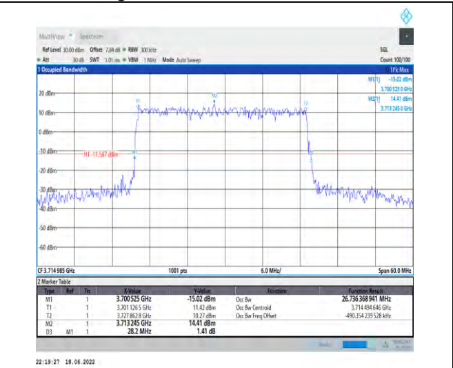
1-N77-3700-3980--30-30-L-3-DFT-16QAM-Outer_Full-75@0-Ant1-26.736-28.200-<math>\leq</math>30-PASS
