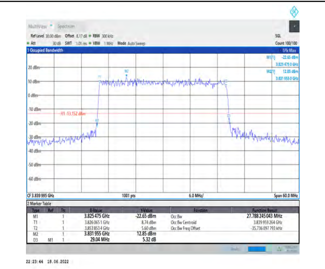
1-N77-3700-3980--30-30-M-8-CP-64QAM-Outer_Full-78@0-Ant1-27.788-29.040-<=30-PASS
