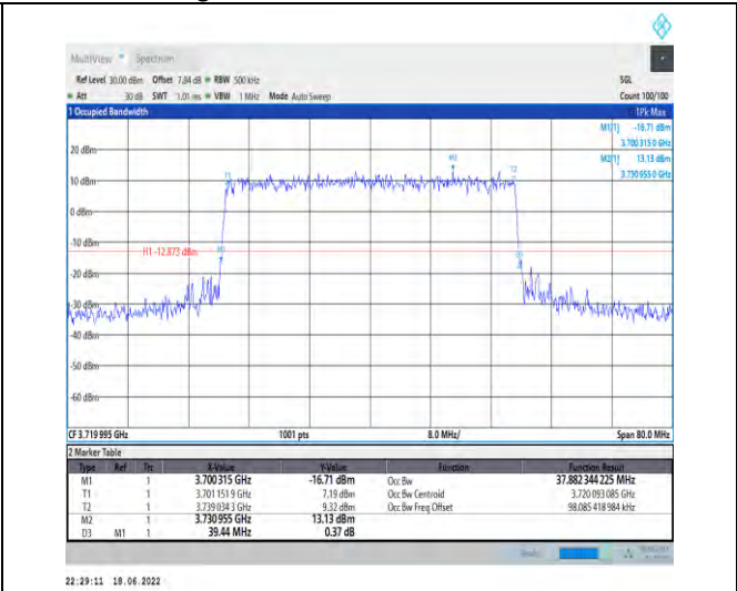
1-N77-3700-3980--30-40-L-8-CP-64QAM-Outer_Full 106@0-Ant1-37.882-39.440-≤40-PASS
