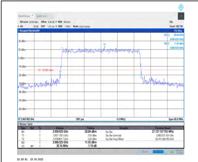
1-N77-3700-3980--30-30-H-8-CP-64QAM-Outer_Ful I-78@0-Ant1-27.721-29.160-<30-PASS
