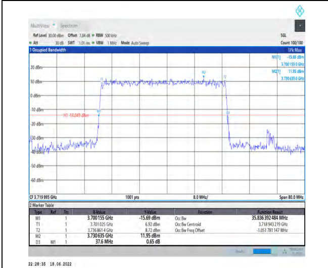
1-N77-3700-3980--30-40-L-5-DFT-256QAM-Outer_F ull-100@0-Ant1-35.836-37.600-≤40-PASS
