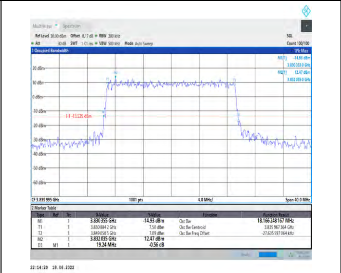
1-N77-3700-3980--30-20-M-7-CP-16QAM-Outer_Full-51@0-Ant1-18.166-19.240-≤20-PASS
