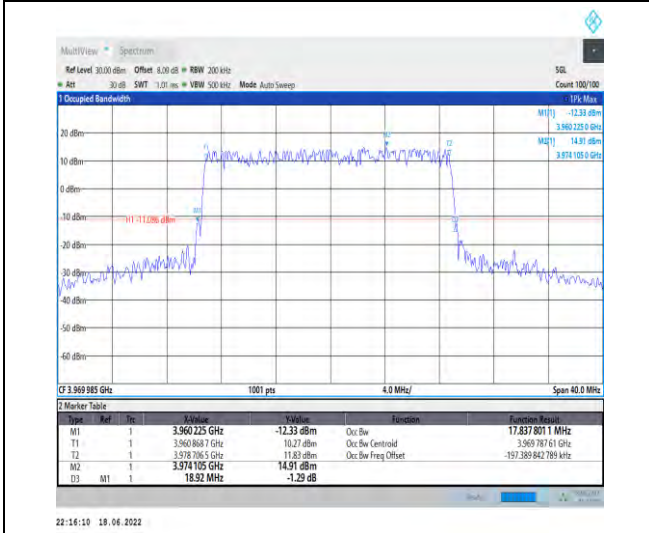
1-N77-3700-3980--30-20-H-1-DFT-QPSK-Outer_Full -50@0-Ant1-17.838-18.920-<20-PASS
