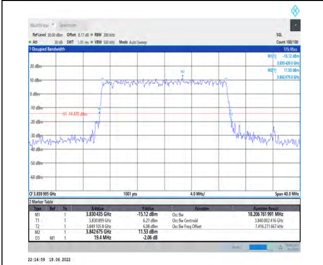
1-N77-3700-3980--30-20-M-6-CP-QPSK-Outer_Full-51@0-Ant1-18.207-19.400-≤20-PASS
