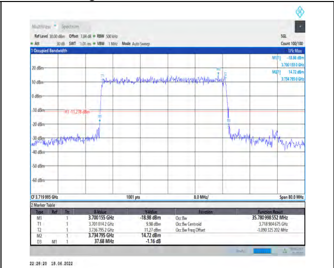
1-N77-3700-3980--30-40-L-4-DFT-64QAM-Outer_Ful I-100@0-Ant1-35.781-37.680-≤40-PASS
