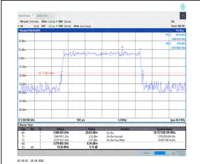
1-N77-3700-3980--30-20-H-9-CP-256QAM-Outer_F ull-51@0-Ant1-18.158-19.360-<=20-PASS
