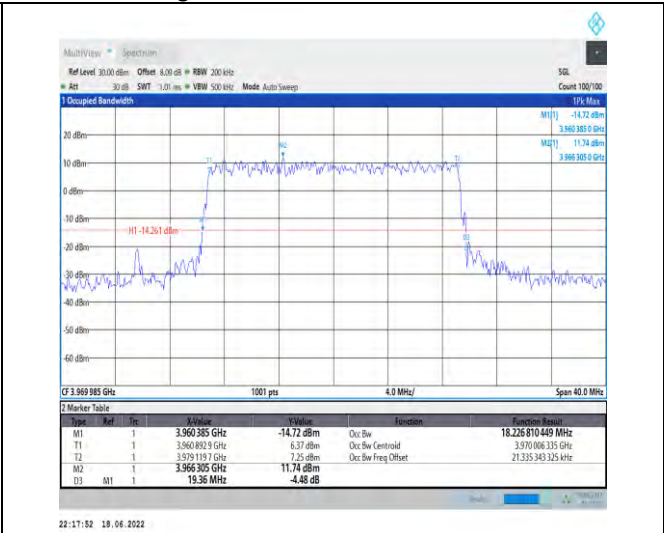
1-N77-3700-3980--30-20-H-8-CP-64QAM-Outer_Full -51@0-Ant1-18.227-19.360-<=20-PASS
