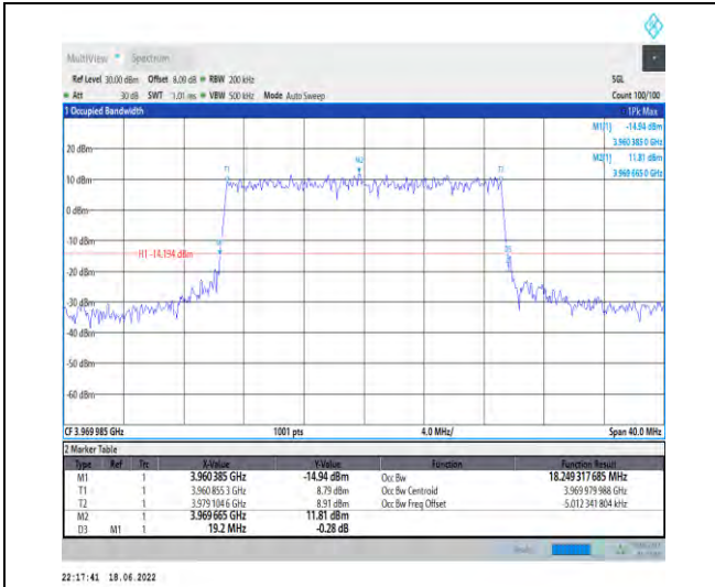
1-N77-3700-3980--30-20-H-7-CP-16QAM-Outer_Full I-51@0-Ant1-18.249-19.200-<=20-PASS
