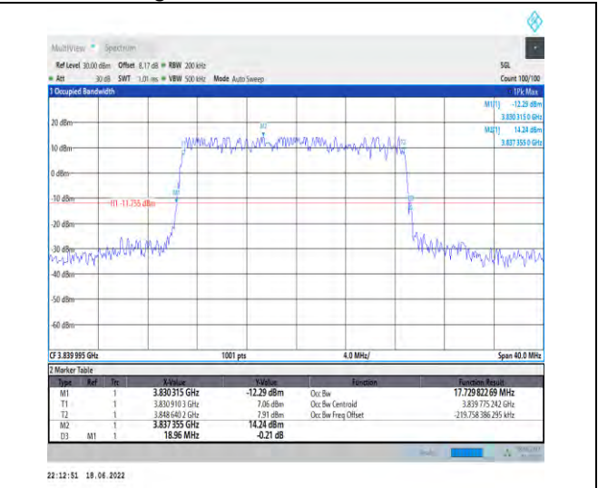
1-N77-3700-3980--30-20-M-1-DFT-QPSK-Outer_Full-50@0-Ant1-17.73-18.960-≤20-PASS
