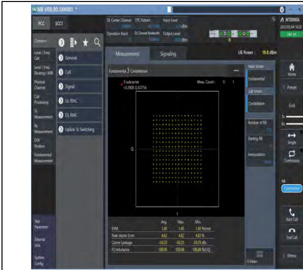
1-N77-3700-3980--30-100-M-9-CP-256QAM-Outer_F ull-273@0-Ant1-see graph-PASS
