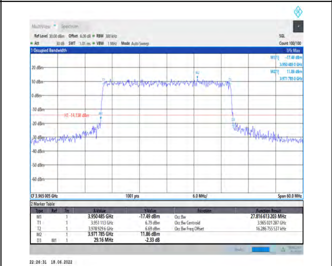
1-N77-3700-3980--30-30-H-7-CP-16QAM-Outer_Full-78@0-Ant1-27.817-29.160-≤30-PASS
