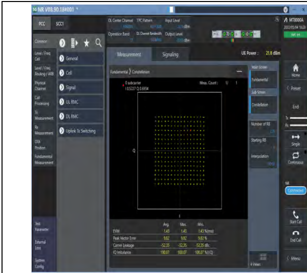
1-N77-3700-3980--30-100-M-5-DFT-256QAM-Outer_ Full-270@0-Ant1-see graph-PASS
