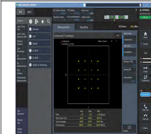
1-N77-3700-3980--30-100-M-3-DFT-16QAM-Outer_Full-270@0-Ant1-see graph-PASS
