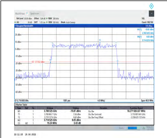
1-N77-3700-3980--30-20-L-9-CP-256QAM-Outer_Full-51@0-Ant1-18.272-19.240-≤20-PASS
