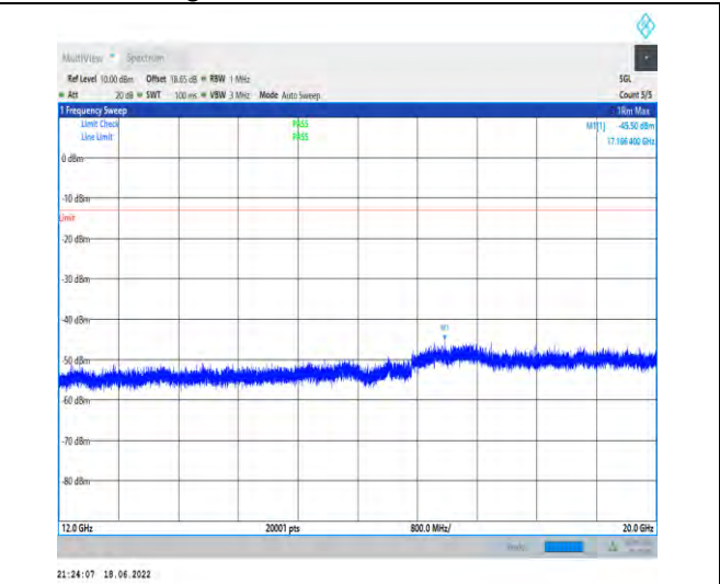
1-N71--15-20-H-1-DFT-PI2BPSK-Inner_1RB_Left-1 @1-12000-20000-Ant1--45.50--13-PASS
