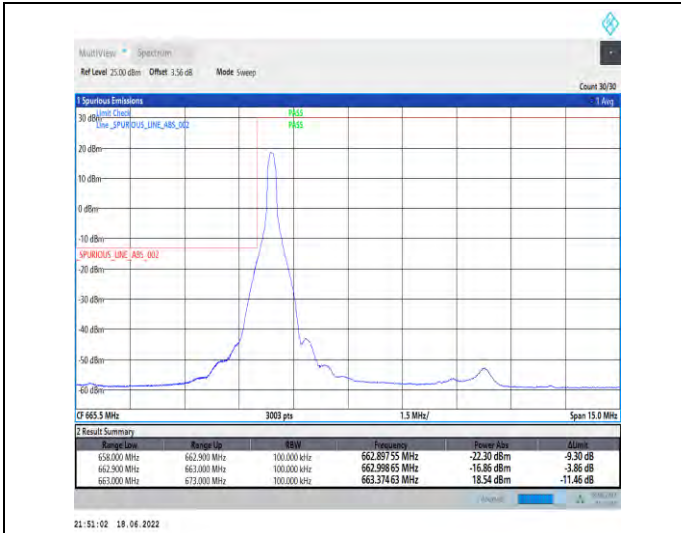
1-N71--15-10-L-1-DFT-PI2BPSK-Edge_1RB_Left-1@0-Ant1-PASS-see graph
