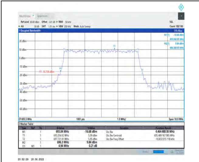
1-N71--15-5-H-7-CP-16QAM-Outer_Full-25@0-Ant1 4.464-4.940-≤5-PASS
