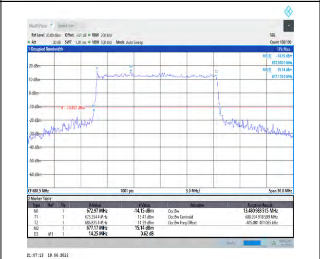
1-N71--15-15-M-1-DFT-QPSK-Outer_Full-75@0-Ant 1-13.481-14.250-≤15-PASS
