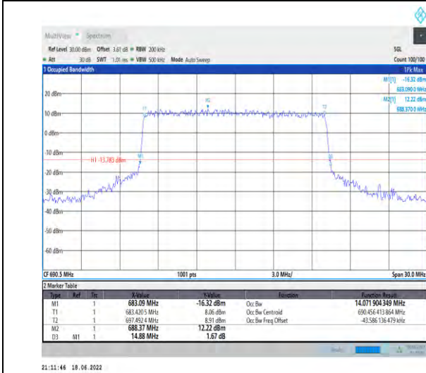
1-N71--15-15-H-7-CP-16QAM-Outer_Full-79@0-Ant 1-14.072-14.880-≤15-PASS
