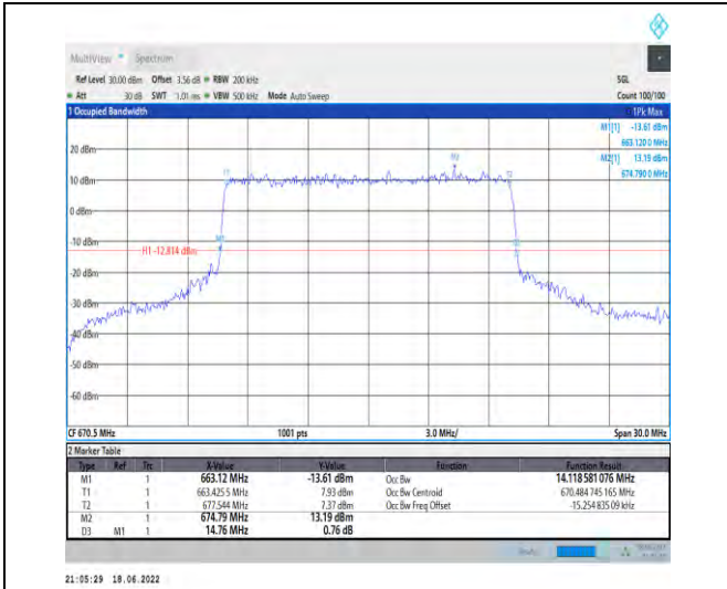
1-N71--15-15-L-7-CP-16QAM-Outer_Full-79@0-Ant1 -14.119-14.760-≤15-PASS
