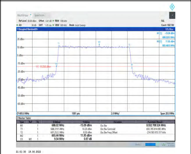
1-N71--15-10-H-3-DFT-16QAM-Outer_Full-50@0-Ant t1-8.933-9.540-≤10-PASS
