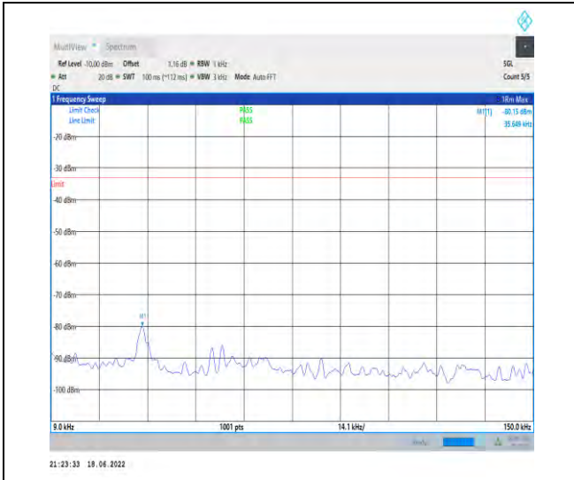
1-N71--15-20-H-1-DFT-PI2BPSK-Inner_1RB_Left-1 @1-0.009-0.15-Ant1--80.15--33-PASS
