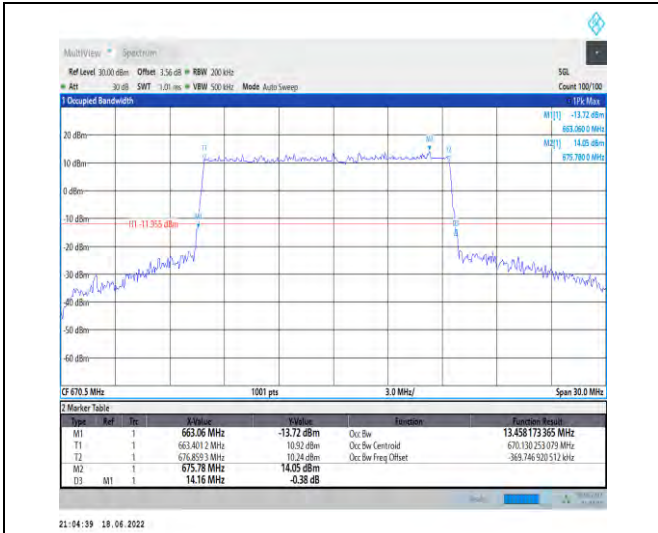
1-N71--15-15-L-3-DFT-16QAM-Outer_Full-75@0-Ant 1-13.458-14.160-≤15-PASS
