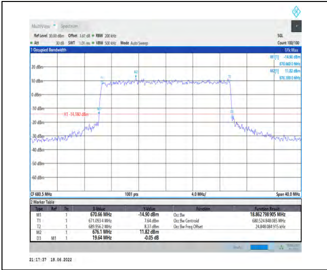
1-N71--15-20-M-7-CP-16QAM-Outer_Full-106@0-An t1-18.863-19.640-<=20-PASS
