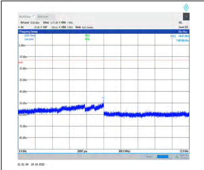
1-N71--15-20-L-1-DFT-PI2BPSK-Inner_1RB_Left-1 @1-3000-12000-Ant1--48.87--13-PASS
