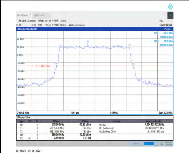
1-N71--15-5-M-3-DFT-16QAM-Outer_Full-25@0-Ant1 -4.464-4.890-≤5-PASS
