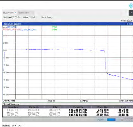
1-N71-PC3-15-20-H-6-CP-QPSK-Outer_Full-106@0-Ant1-PASS-see graph
