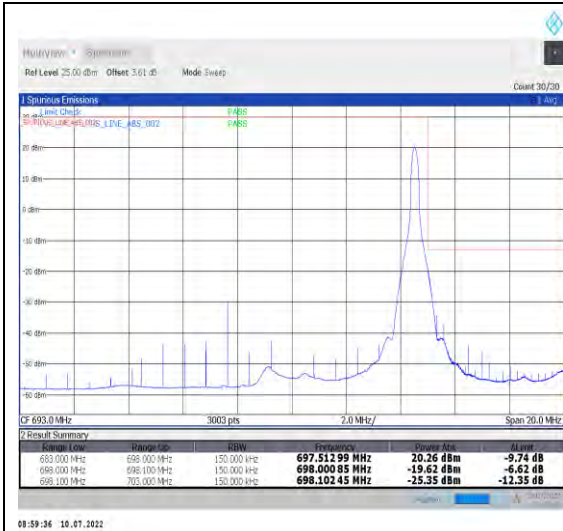
1-N71-PC3-15-15-H-2-DFT-PI2BPSK-Edge_1RB_Right-1@78-Ant1-PASS-see graph
