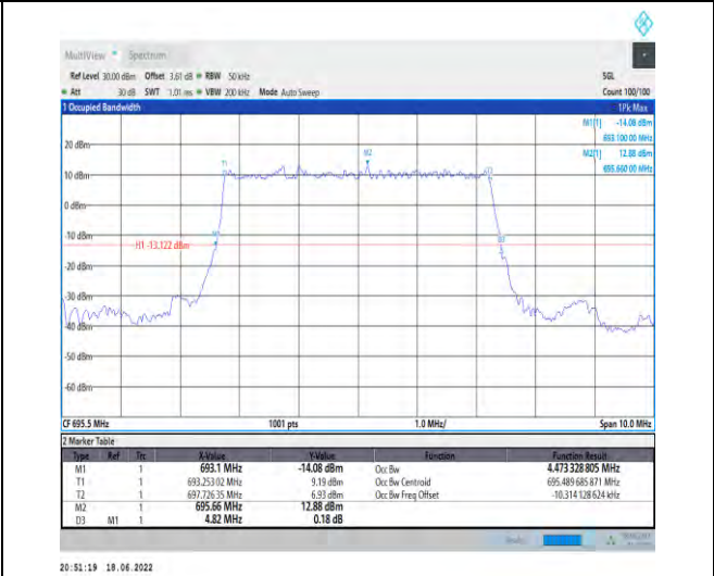
1-N71--15-5-H-2-DFT-PI2BPSK-Outer_Full-25@0-A nt1-4.473-4.820-≤5-PASS
