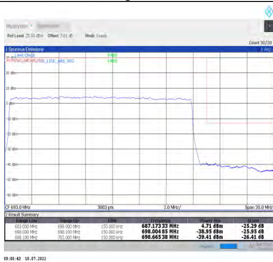
1-N71-PC3-15-15-H-3-DFT-PI2BPSK-Outer_Full-75@0-Ant1-PASS-see graph
