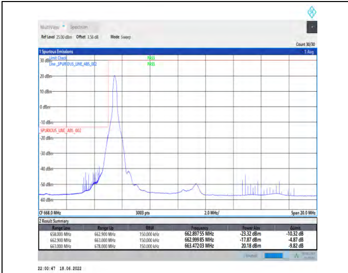
1-N71--15-15-L-1-DFT-PI2BPSK-Edge_1RB_Left-1@0-Ant1-PASS-see graph
