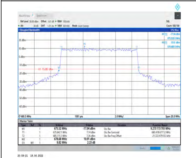
1-N71--15-10-M-7-CP-16QAM-Outer_Full-52@0-Ant 1-9.273-9.820-≤10-PASS
