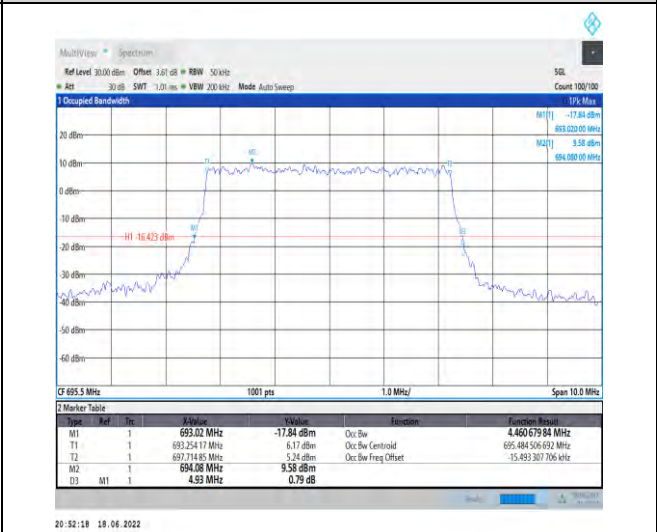
1-N71--15-5-H-6-CP-QPSK-Outer_Full-25@0-Ant1-4 .461-4.930-≤5-PASS
