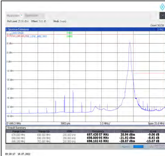
1-N71-PC3-15-20-H-2-DFT-PI2BPSK-Edge_1RB_Right-1@105-Ant1-PASS-see graph
