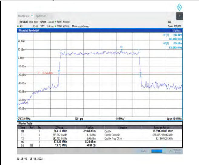
1-N71--15-20-L-9-CP-256QAM-Outer_Full-106@0-Ant nt1-18.891-19.760-≤20-PASS
