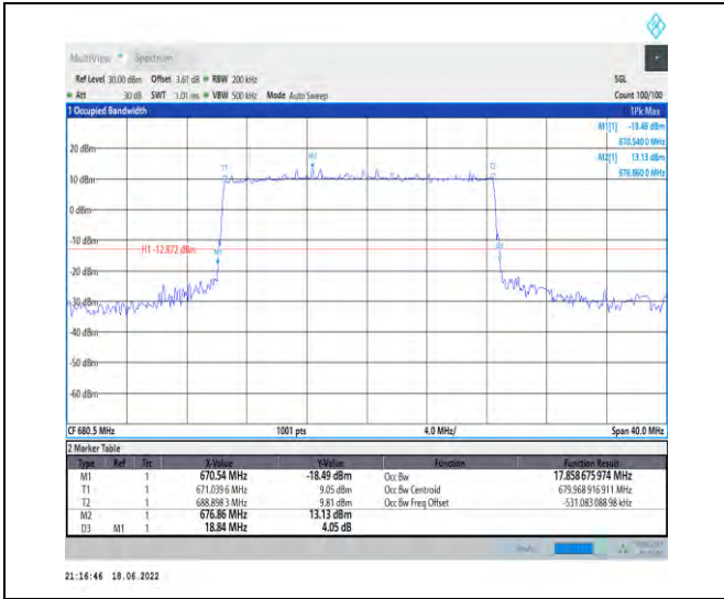
1-N71--15-20-M-3-DFT-16QAM-Outer_Full-100@0-A nt1-17.859-18.840-≤20-PASS
