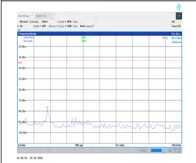
1-N71--15-20-M-1-DFT-PI2BPSK-Inner_1RB_Left-1 @1-0.009-0.15-Ant1--80.13--33-PASS
