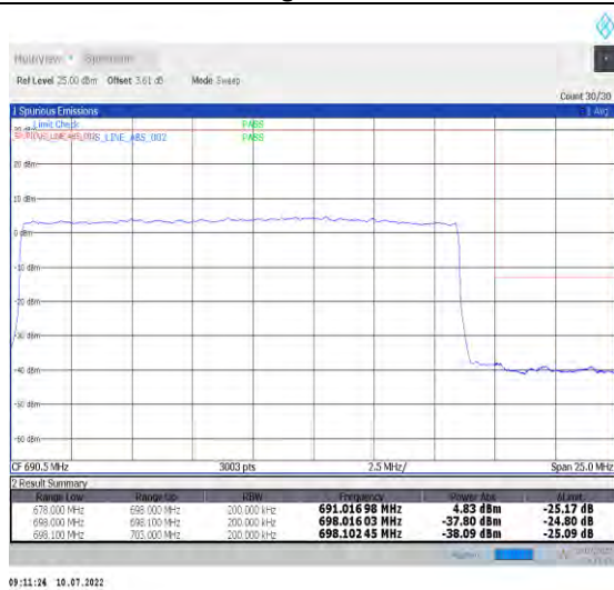
1-N71-PC3-15-20-H-3-DFT-PI2BPSK-Outer_Full-100@0-Ant1-PASS-see graph
