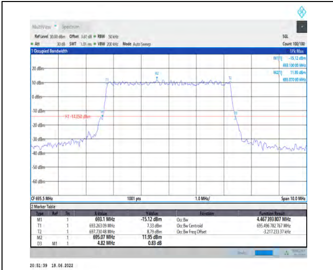
1-N71--15-5-H-3-DFT-16QAM-Outer_Full-25@0-Ant 1-4.467-4.820-≤5-PASS
