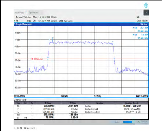
1-N71--15-20-H-9-CP-256QAM-Outer_Full-106@0-A nt1-18.842-19.800-≤20-PASS
