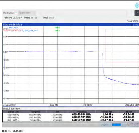
1-N71-PC3-15-15-H-6-CP-QPSK-Outer_Full-79@0-Ant1-PASS-see graph
