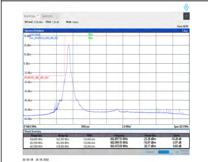
1-N71--15-15-L-4-CP-QPSK-Edge_1RB_Left-1@0-Ant1-PASS-see graph
