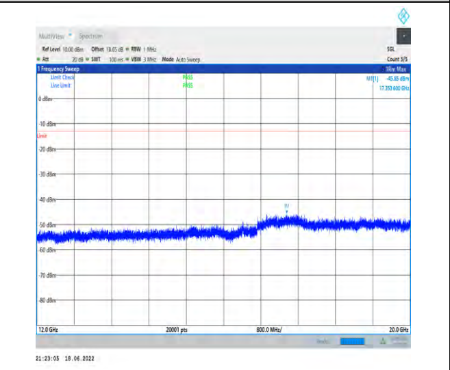
1-N71--15-20-M-1-DFT-PI2BPSK-Inner_1RB_Left-1 @1-12000-20000-Ant1--45.85--13-PASS
