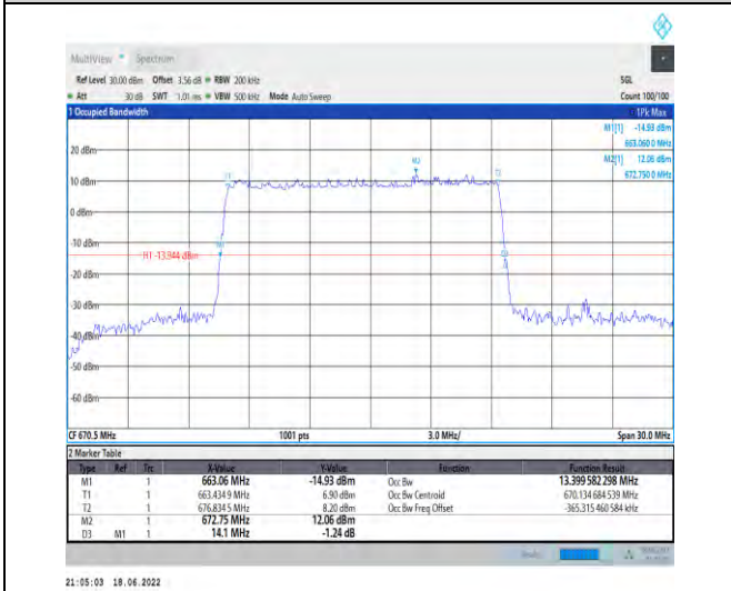
1-N71--15-15-L-5-DFT-256QAM-Outer_Full-75@0-A nt1-13.4-14.100-≤15-PASS
