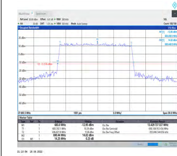
1-N71--15-15-H-3-DFT-16QAM-Outer_Full-75@0-An t1-13.43-14.250-≤15-PASS
