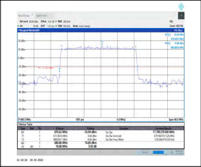
1-N71--15-20-M-2-DFT-PI2BPSK-Outer_Full-100@0-Ant -Ant1-17.79-18.680-≤20-PASS
