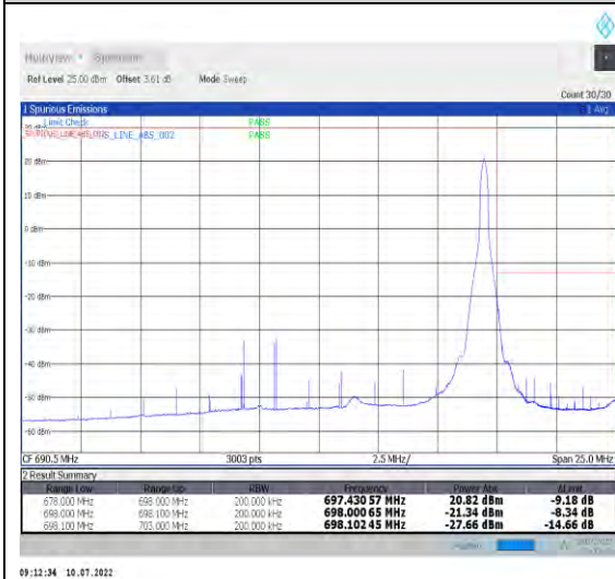
1-N71-PC3-15-20-H-5-CP-QPSK-Edge_1RB_Right-1@105-Ant1-PASS-see graph
