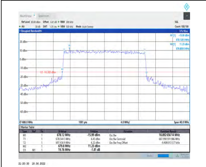
1-N71--15-20-H-8-CP-64QAM-Outer_Full-106@0-An t1-18.893-19.760-≤20-PASS
