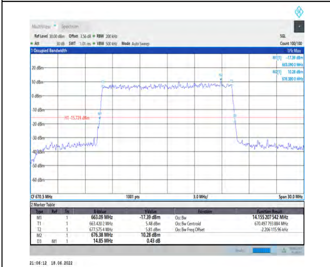
1-N71--15-15-L-9-CP-256QAM-Outer_Full-79@0-Ant 1-14.155-14.850-≤15-PASS
