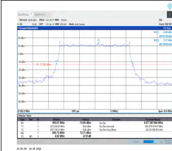
1-N71--15-5-H-1-DFT-QPSK-Outer_Full-25@0-Ant1- 4.477-4.920-≤5-PASS
