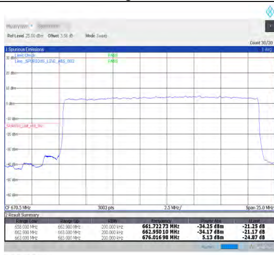
1-N71-PC3-15-20-L-3-DFT-PI2BPSK-Outer_Full-100@0-Ant1-PASS-see graph
