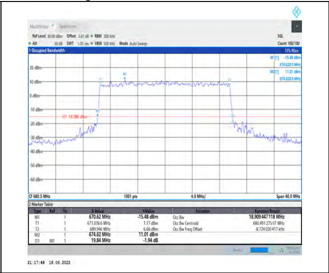
1-N71--15-20-M-8-CP-64QAM-Outer_Full-106@0-A nt1-18.909-19.840-<=20-PASS
