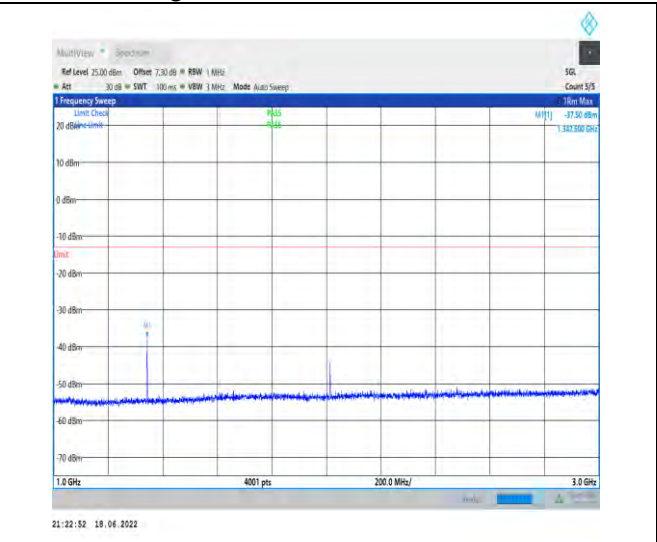
1-N71--15-20-M-1-DFT-PI2BPSK-Inner_1RB_Left-1 @1-1000-3000-Ant1--37.50--13-PASS
