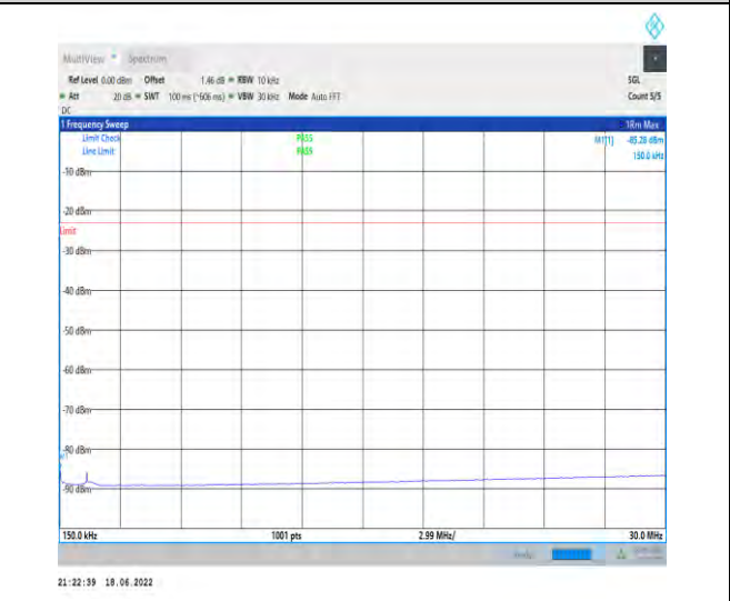
1-N71--15-20-M-1-DFT-PI2BPSK-Inner_1RB_Left-1 @1-0.15-30-Ant1--85.28--23-PASS
