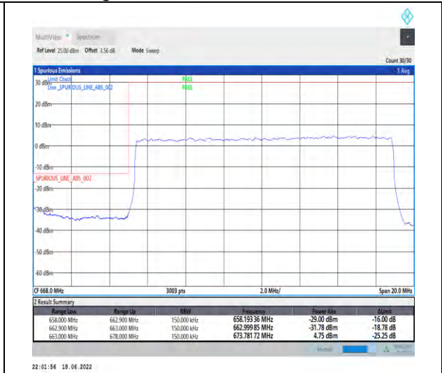
1-N71--15-15-L-3-DFT-PI2BPSK-Outer_Full-75@0-Ant1-PASS-see graph
