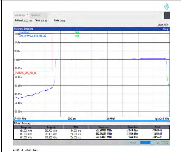
1-N71--15-15-L-6-CP-QPSK-Outer_Full-79@0-Ant1-PASS-see graph
