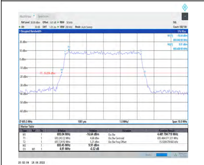
1-N71--15-5-H-5-DFT-256QAM-Outer_Full-25@0-Ant t1-4.482-4.910-≤5-PASS
