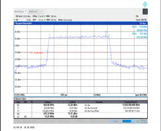
1-N71--15-15-L-2-DFT-PI2BPSK-Outer_Full-75@0-Ant1 nt1-13.454-14.250-≤15-PASS
