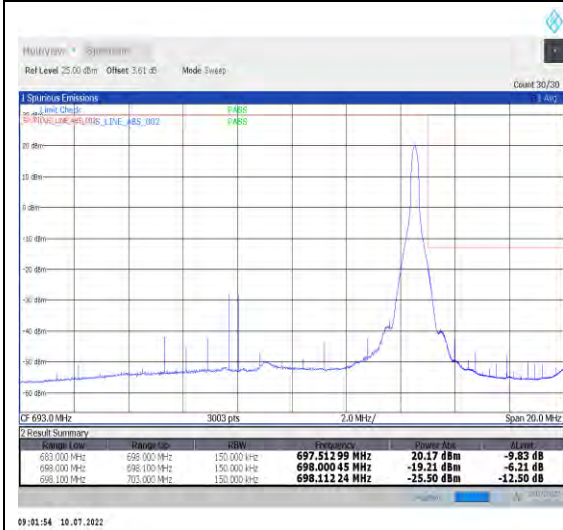
1-N71-PC3-15-15-H-5-CP-QPSK-Edge_1RB_Right-1@78-Ant1-PASS-see graph
