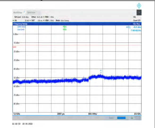
1-N71--15-20-L-1-DFT-PI2BPSK-Inner_1RB_Left-1@ 1-12000-20000-Ant1--45.31--13-PASS
