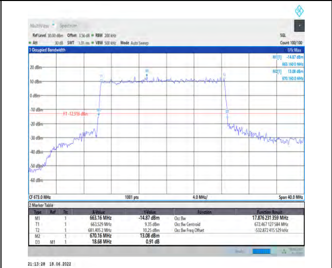
1-N71--15-20-L-3-DFT-16QAM-Outer_Full-100@0-Ant nt1-17.876-18.680-≤20-PASS
