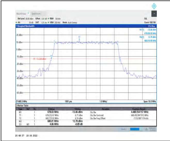
1-N71--15-5-M-4-DFT-64QAM-Outer_Full-25@0-Ant 1-4.48-4.860-≤5-PASS
