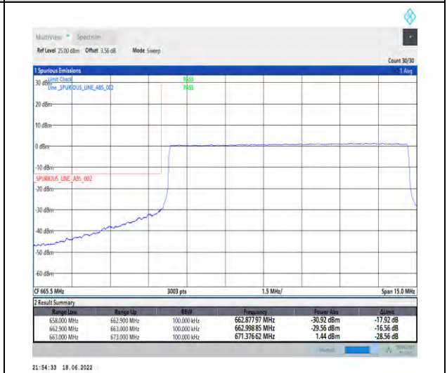
1-N71--15-10-L-6-CP-QPSK-Outer_Full-52@0-Ant1-PASS-see graph
