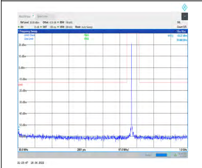
1-N71--15-20-H-1-DFT-PI2BPSK-Inner_1RB_Left-1 @1-30-1000-Ant1--55.27--13-PASS
