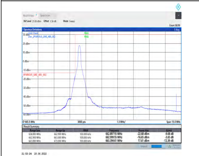
1-N71--15-10-L-4-CP-QPSK-Edge_1RB_Left-1@0-Ant1-PASS-see graph
