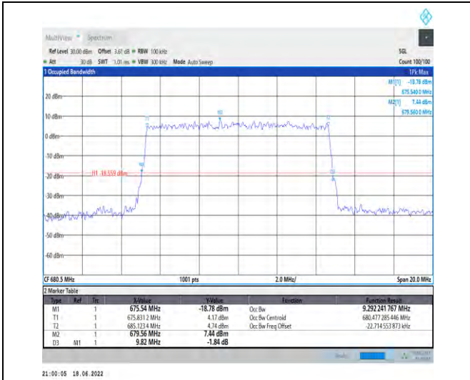
1-N71--15-10-M-9-CP-256QAM-Outer_Full-52@0-An t1-9.292-9.820-≤10-PASS
