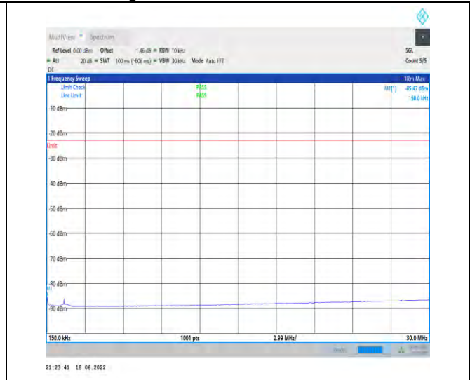
1-N71--15-20-H-1-DFT-PI2BPSK-Inner_1RB_Left-1 @1-0.15-30-Ant1--85.47--23-PASS
