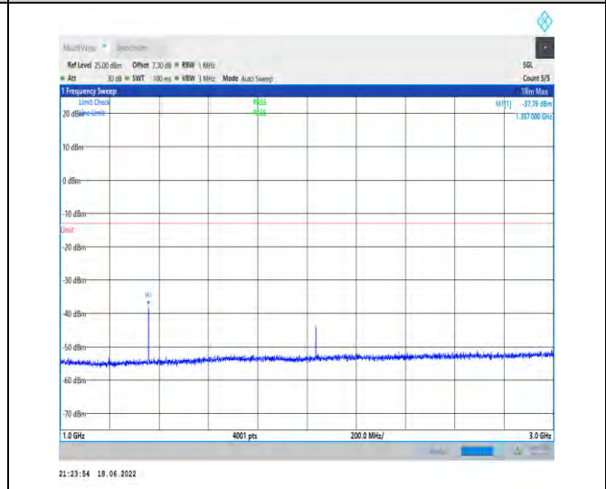
1-N71--15-20-H-1-DFT-PI2BPSK-Inner_1RB_Left-1 @1-1000-3000-Ant1--37.79--13-PASS
