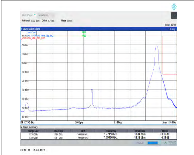
1-N66--15-10-H-5-CP-QPSK-Edge_1RB_Right-1@51-Ant1-seegraph-PASS-see graph
