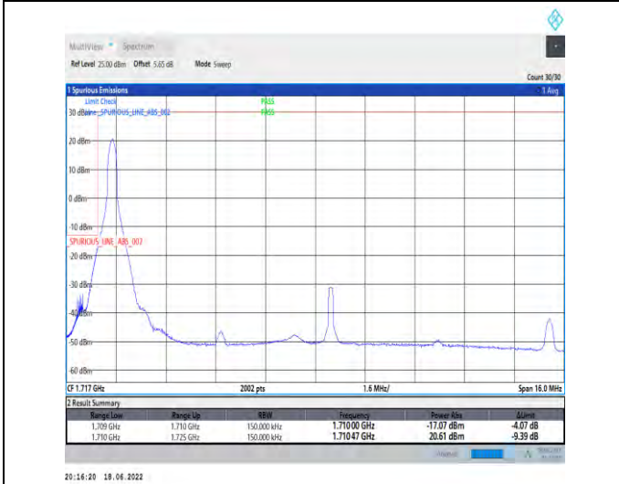
1-N66--15-15-L-4-CP-QPSK-Edge_1RB_Left-1@0-Ant1-seegraph-PASS-see graph
