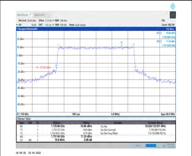
1-N66--15-20-M-6-CP-QPSK-Outer_Full-106@0-Ant 1-18.926-19.800-≤20-PASS
