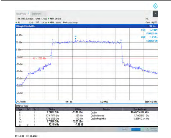
1-N66--15-40-L-8-CP-64QAM-Outer_Full-216@0-Ant1 -38.446-40.160-≤40-PASS
