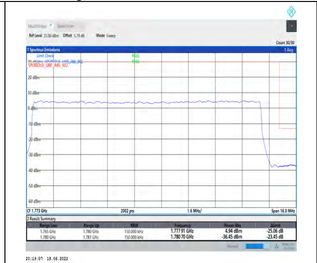
1-N66--15-15-H-3-DFT-PI2BPSK-Outer_Full-75@0-Ant1-seegraph-PASS-see graph
