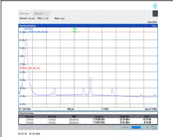
1-N66--15-30-L-4-CP-QPSK-Edge_1RB_Left-1@0-Ant1-seegraph-PASS-see graph
