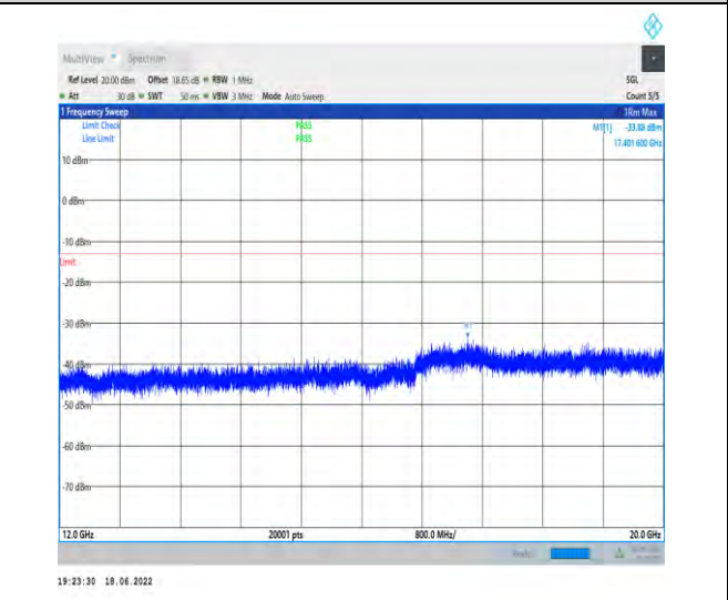
1-N66--15-40-M-1-DFT-PI2BPSK-Inner_1RB_Left-1 @1-12000-20000-Ant1--33.88--13-PASS
