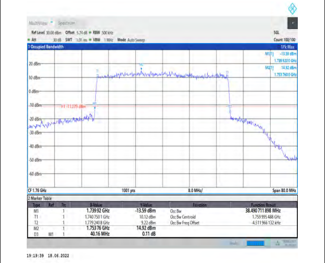
1-N66--15-40-H-3-DFT-16QAM-Outer_Full-216@0-A nt1-38.491-40.160-<math>\leq 40</math>-PASS
