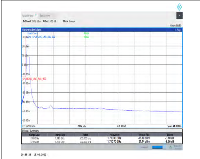
1-N66--15-40-L-4-CP-QPSK-Edge_1RB_Left-1@0-Ant1-seegraph-PASS-see graph
