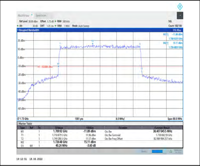
1-N66--15-40-L-1-DFT-QPSK-Outer_Full-216@0-Ant 1-38.407-40.240-<math>\leq 40</math>-PASS
