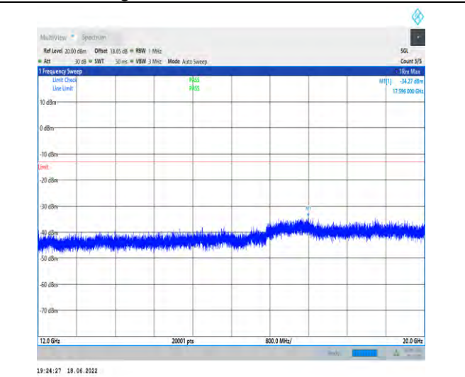
1-N66--15-40-H-1-DFT-PI2BPSK-Inner_1RB_Left-1 @1-12000-20000-Ant1--34.27--13-PASS
