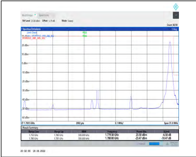
1-N66--15-30-H-2-DFT-PI2BPSK-Edge_1RB_Right-1 @159-Ant1-seegraph-PASS-see graph
