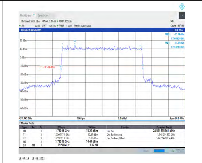
1-N66--15-30-M-3-DFT-16QAM-Outer_Full-160@0-A nt1-28.595-29.580-≤30-PASS
