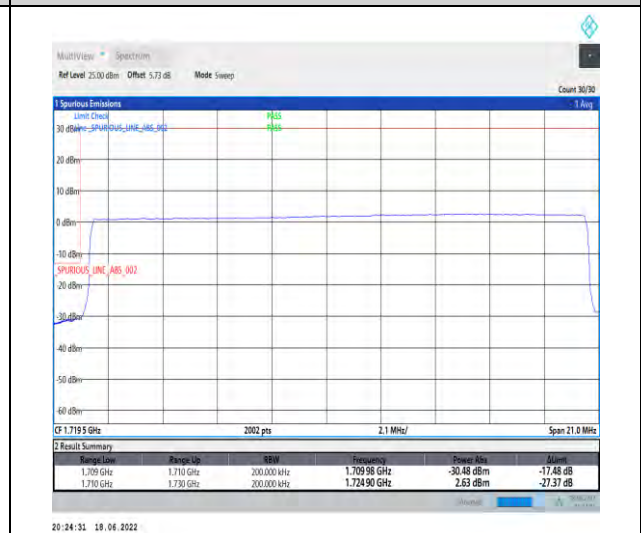
1-N66--15-20-L-6-CP-QPSK-Outer_Full-106@0-Ant1-seegraph-PASS-see graph
