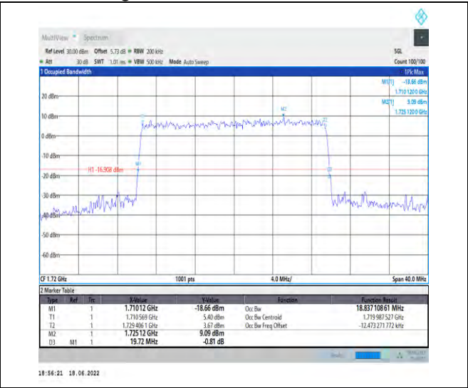
1-N66--15-20-L-9-CP-256QAM-Outer_Full-106@0-A nt1-18.837-19.720-<=20-PASS
