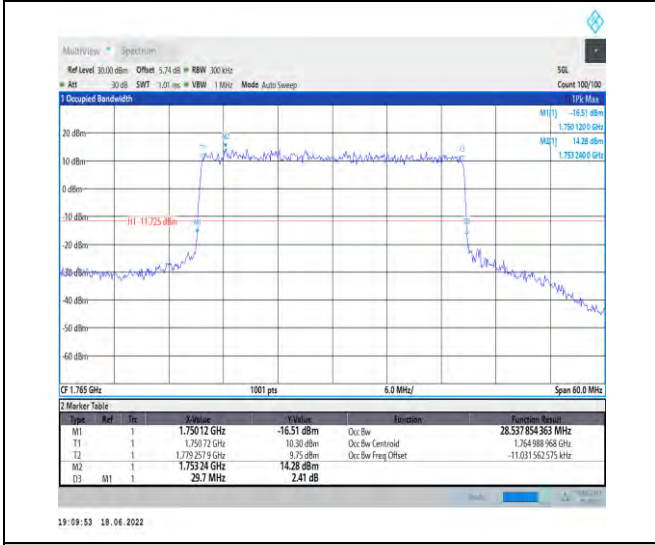
1-N66--15-30-H-1-DFT-QPSK-Outer_Full-160@0-An t1-28.538-29.700-≤30-PASS
