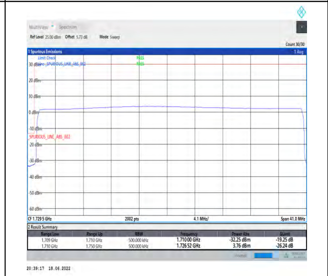
1-N66--15-40-L-6-CP-QPSK-Outer_Full-216@0-Ant1-seegraph-PASS-see graph
