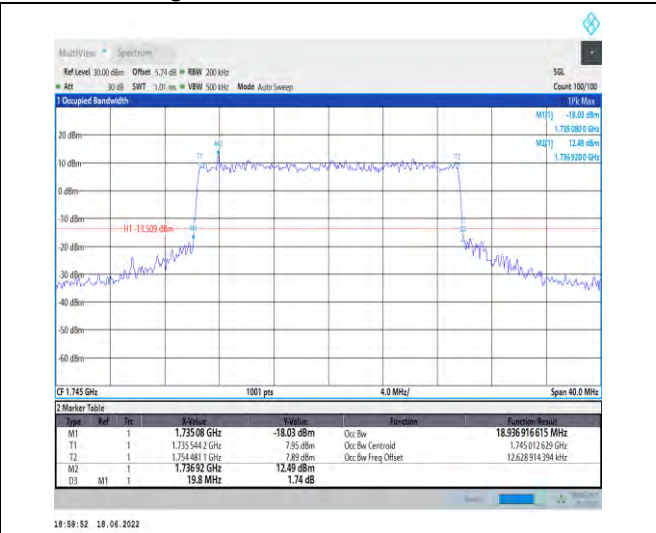
1-N66--15-20-M-8-CP-64QAM-Outer_Full-106@0-A nt1-18.937-19.800-≤20-PASS
