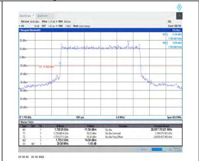
1-N66--15-30-M-1-DFT-QPSK-Outer_Full-160@0-An t1-28.591-29.580-≤30-PASS
