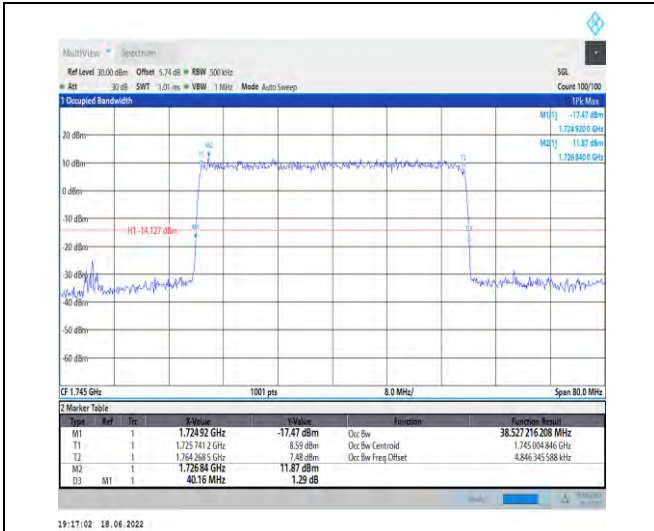
1-N66--15-40-M-5-DFT-256QAM-Outer_Full-216@0-Ant1-38.527-40.160-≤40-PASS
