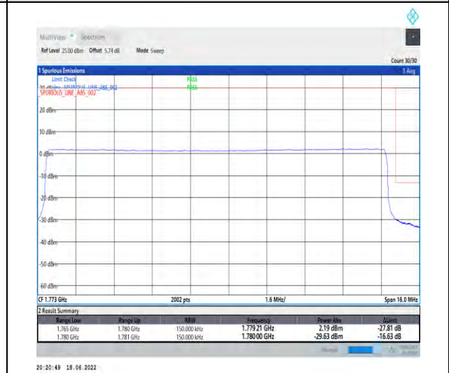
1-N66--15-15-H-6-CP-QPSK-Outer_Full-79@0-Ant1-seegraph-PASS-see graph
