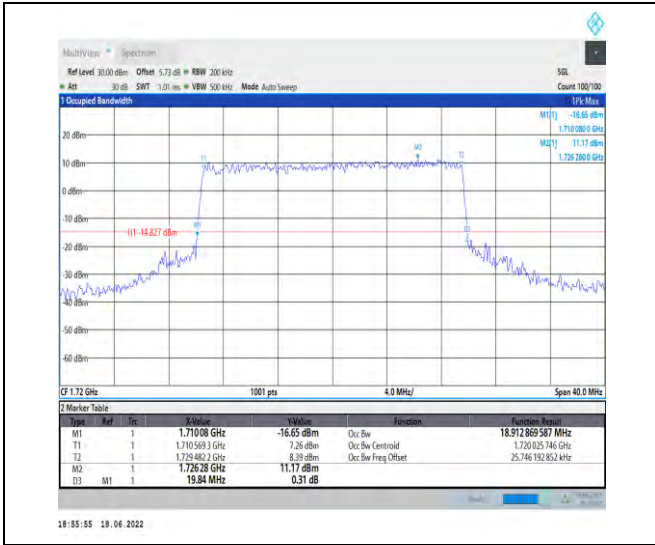
1-N66--15-20-L-8-CP-64QAM-Outer_Full-106@0-An t1-18.913-19.840-<=20-PASS
