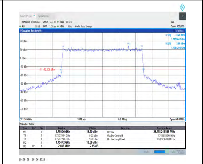
1-N66--15-30-M-7-CP-16QAM-Outer_Full-160@0-A nt1-28.493-29.880-≤30-PASS
