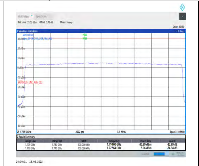
1-N66--15-30-L-3-DFT-PI2BPSK-Outer_Full-160@0-Ant1-seegraph-PASS-see graph
