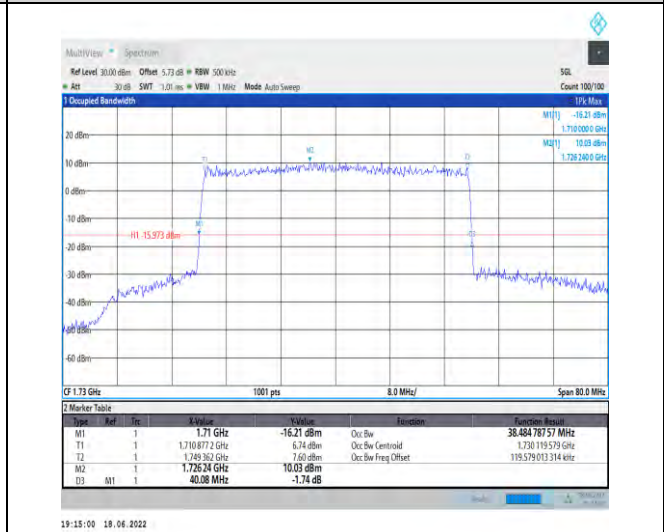
1-N66--15-40-L-9-CP-256QAM-Outer_Full-216@0-Ant1 -38.485-40.080-≤40-PASS
