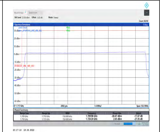
1-N66--15-15-L-6-CP-QPSK-Outer_Full-79@0-Ant1-seegraph-PASS-see graph
