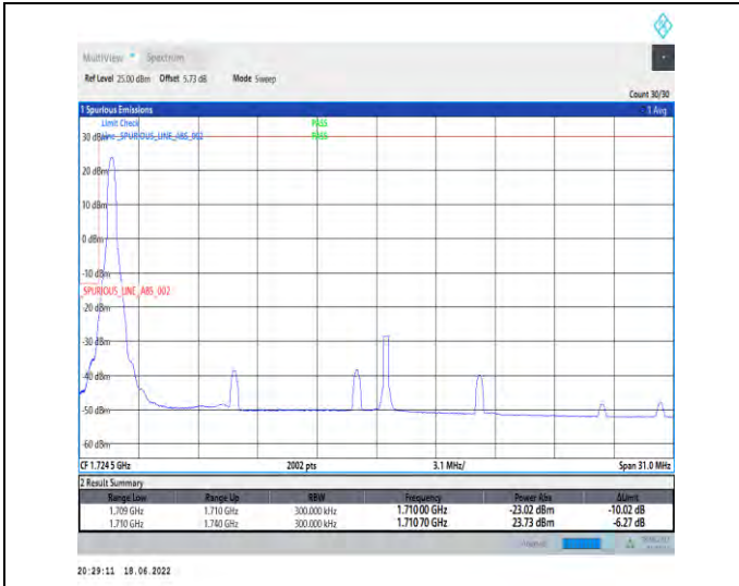
1-N66--15-30-L-1-DFT-PI2BPSK-Edge_1RB_Left-1@0-Ant1-seegraph-PASS-see graph
