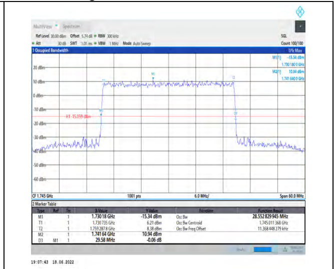
1-N66--15-30-M-5-DFT-256QAM-Outer_Full-160@0-A Ant1-28.553-29.580-≤30-PASS
