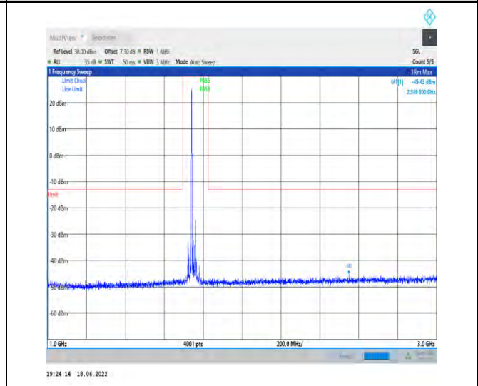
1-N66--15-40-H-1-DFT-PI2BPSK-Inner_1RB_Left-1 @1-1000-3000-Ant1--45.43--13-PASS
