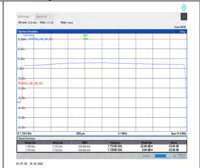
1-N66--15-40-L-3-DFT-PI2BPSK-Outer_Full-216@0-Ant1-seegraph-PASS-see graph
