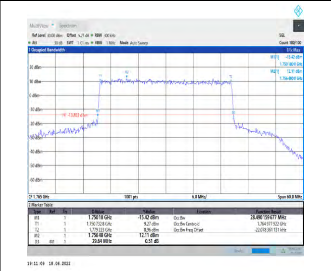
1-N66--15-30-H-6-CP-QPSK-Outer_Full-160@0-Ant 1-28.49-29.640-≤30-PASS
