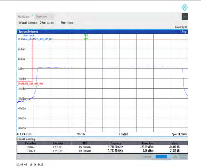
1-N66--15-10-L-6-CP-QPSK-Outer_Full-52@0-Ant1-seegraph-PASS-see graph
