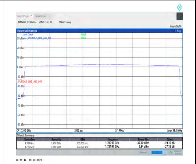
1-N66--15-30-L-6-CP-QPSK-Outer_Full-160@0-Ant1-seegraph-PASS-see graph
