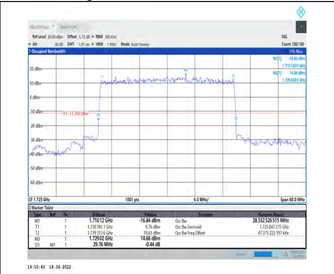
1-N66--15-30-L-2-DFT-PI2BPSK-Outer_Full-160@0-Ant 1-28.533-29.760-≤30-PASS
