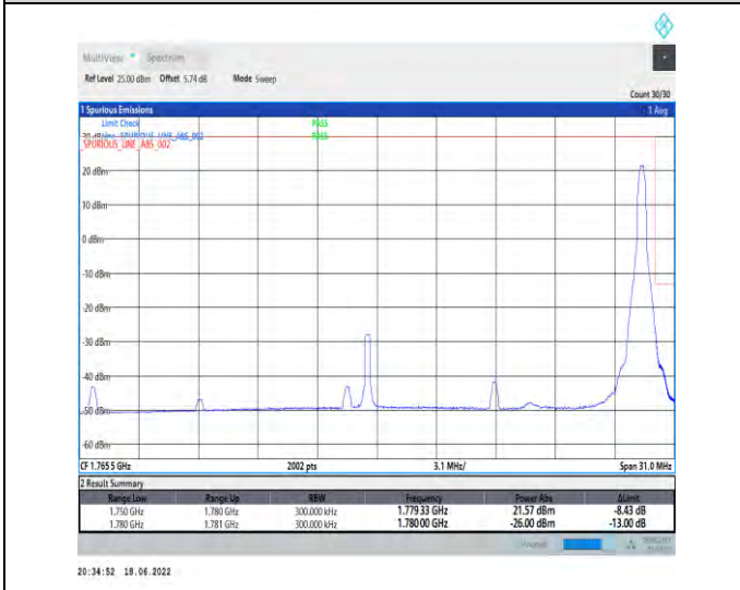
1-N66--15-30-H-5-CP-QPSK-Edge_1RB_Right-1@159 -Ant1-seegraph-PASS-see graph
