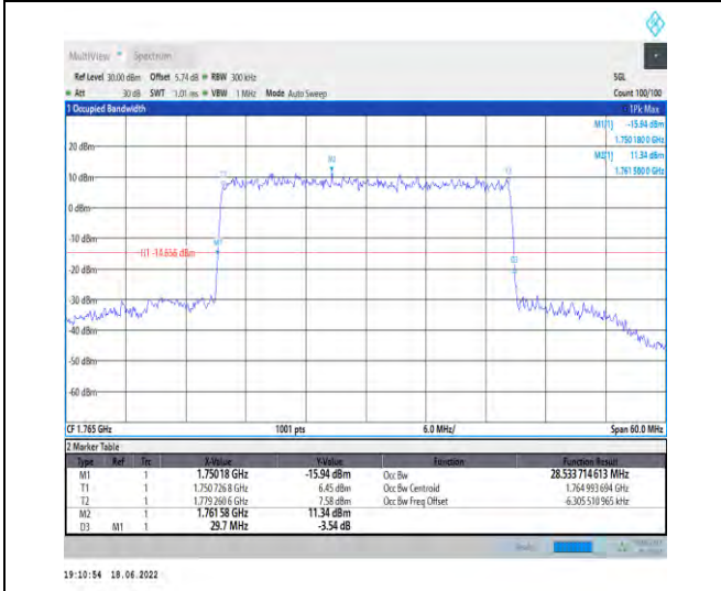
1-N66--15-30-H-5-DFT-256QAM-Outer_Full-160@0-A Ant1-28.534-29.700-≤30-PASS
