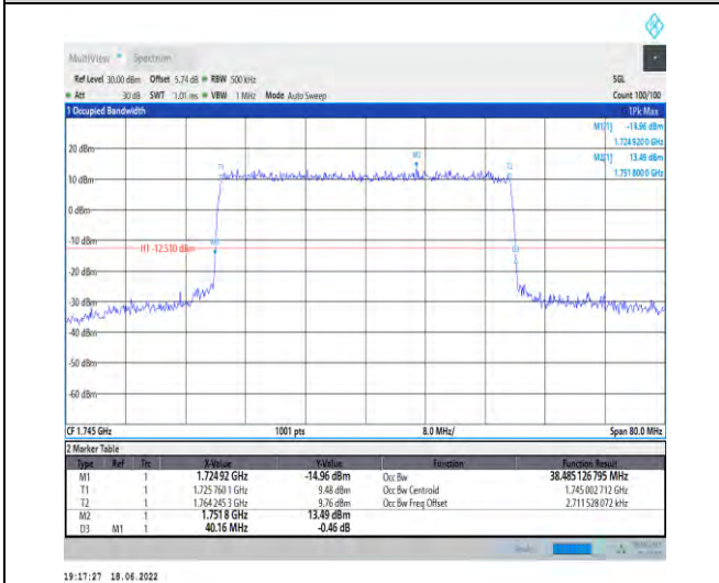
1-N66--15-40-M-7-CP-16QAM-Outer_Full-216@0-Ant1-38.485-40.160-≤40-PASS
