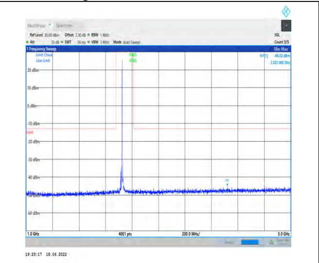
1-N66--15-40-M-1-DFT-PI2BPSK-Inner_1RB_Left-1 @1-1000-3000-Ant1--45.02--13-PASS
