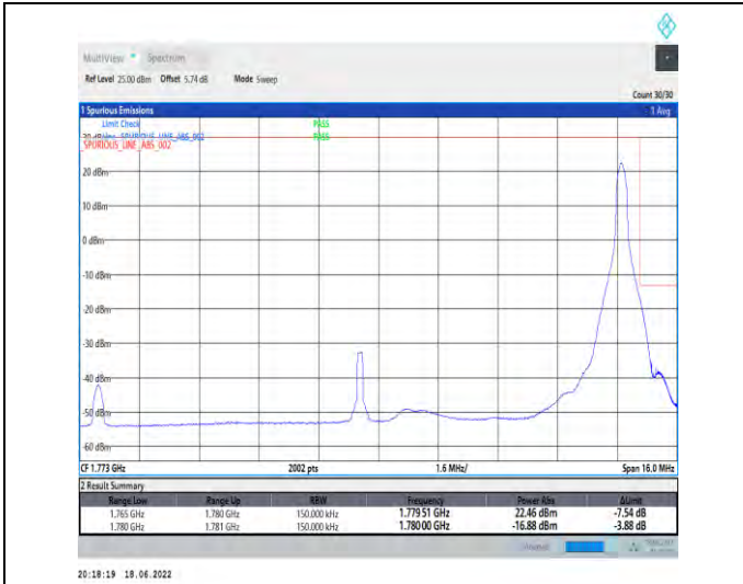
1-N66--15-15-H-2-DFT-PI2BPSK-Edge_1RB_Right-1@78-Ant1-seegraph-PASS-see graph
