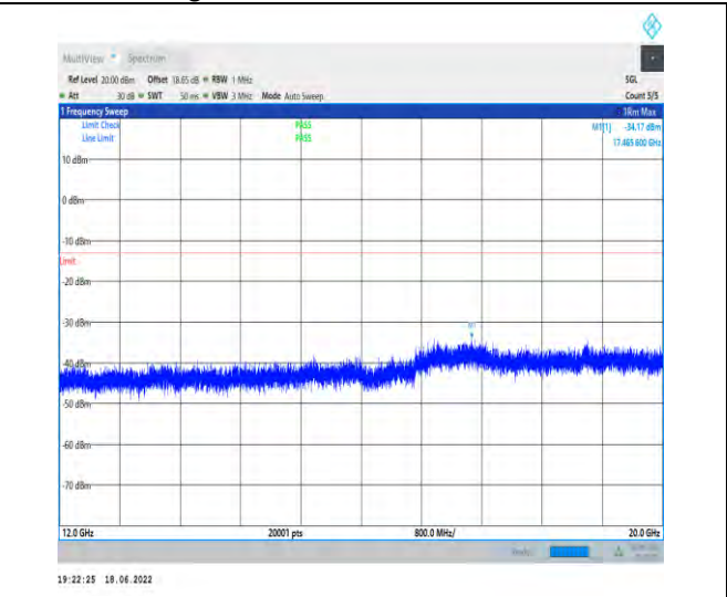
1-N66--15-40-L-1-DFT-PI2BPSK-Inner_1RB_Left-1@ 1-12000-20000-Ant1--34.17--13-PASS
