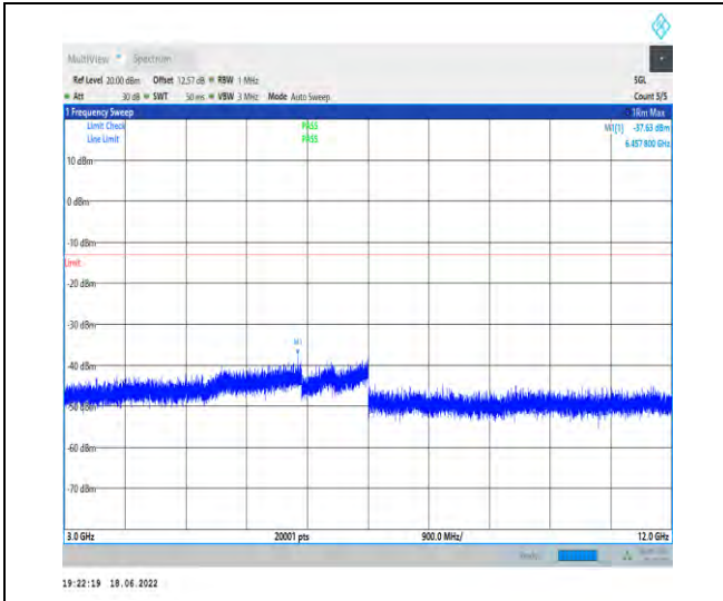
1-N66--15-40-L-1-DFT-PI2BPSK-Inner_1RB_Left-1 @1-3000-12000-Ant1--37.63--13-PASS
