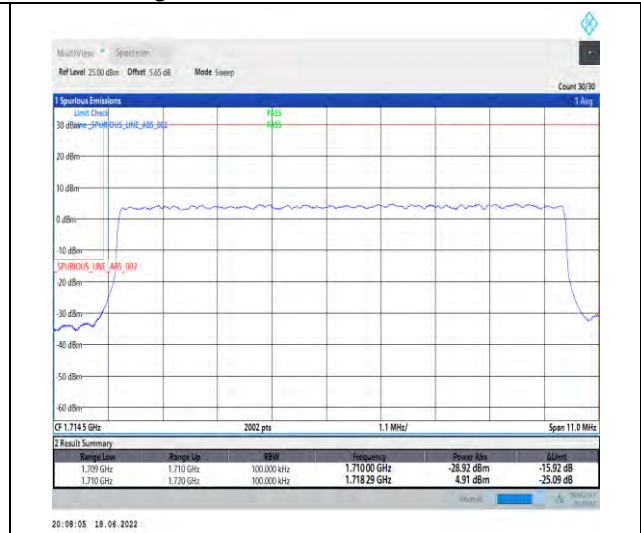
1-N66--15-10-L-3-DFT-PI2BPSK-Outer_Full-50@0-Ant1-seegraph-PASS-see graph
