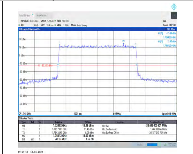
1-N66--15-40-M-6-CP-QPSK-Outer_Full-216@0-Ant1-38.499-40.160-≤40-PASS
