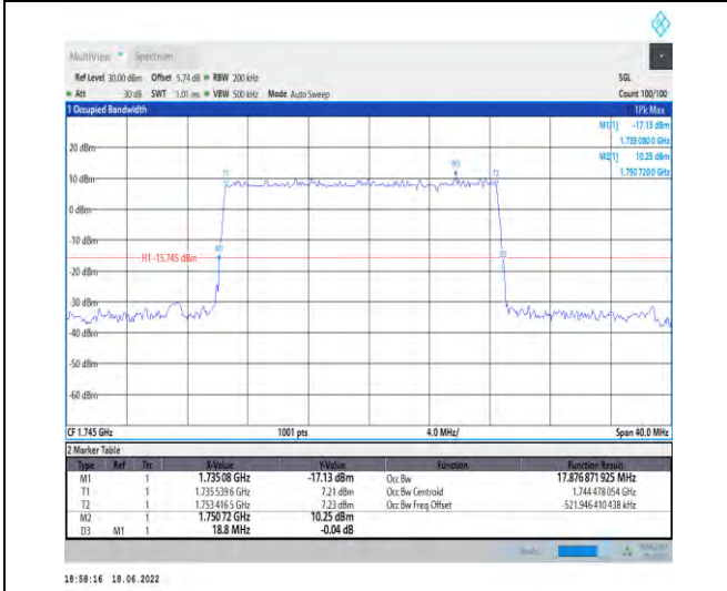
1-N66--15-20-M-5-DFT-256QAM-Outer_Full-100@0-A Ant1-17.877-18.800-≤20-PASS
