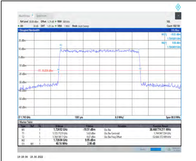
1-N66--15-40-M-9-CP-256QAM-Outer_Full-216@0-Ant1-38.469-40.160-<math>\leq 40</math>-PASS
