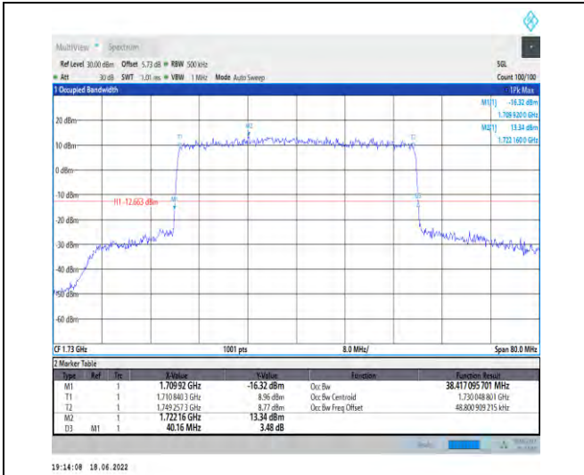
1-N66--15-40-L-6-CP-QPSK-Outer_Full-216@0-Ant1 -38.417-40.160-≤40-PASS
