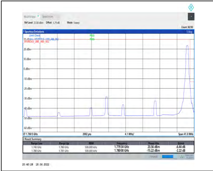
1-N66--15-40-H-2-DFT-PI2BPSK-Edge_1RB_Right-1 @215-Ant1-seegraph-PASS-see graph
