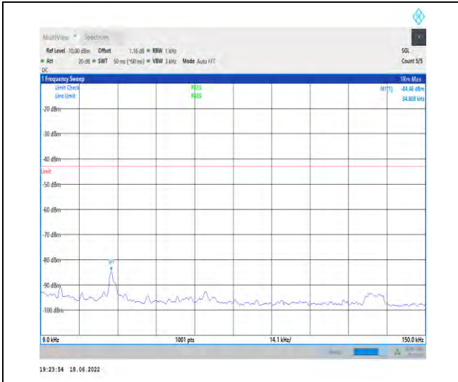
1-N66--15-40-H-1-DFT-PI2BPSK-Inner_1RB_Left-1 @1-0.009-0.15-Ant1--84.46--43-PASS
