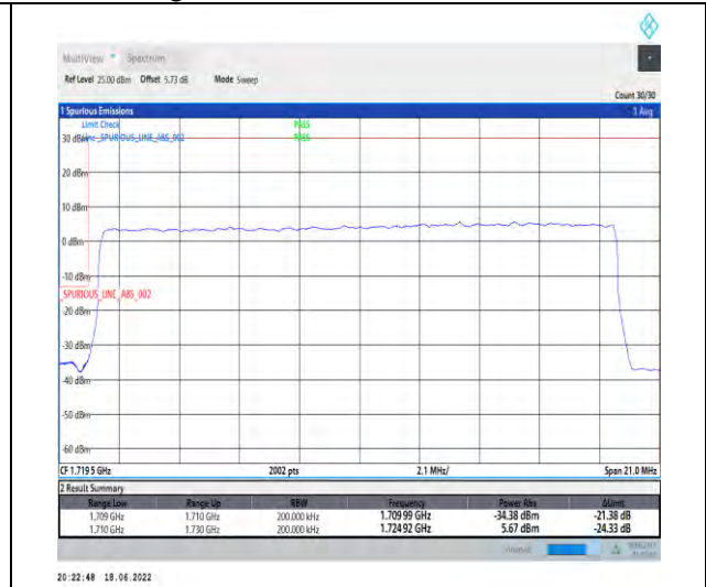
1-N66--15-20-L-3-DFT-PI2BPSK-Outer_Full-100@0-Ant1-seegraph-PASS-see graph
