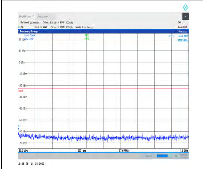
1-N66--15-40-H-1-DFT-PI2BPSK-Inner_1RB_Left-1 @1-30-1000-Ant1--58.74--23-PASS
