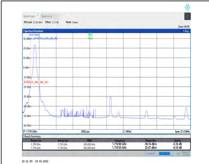
1-N66--15-20-L-1-DFT-PI2BPSK-Edge_1RB_Left-1@0-Ant1-seegraph-PASS-see graph
