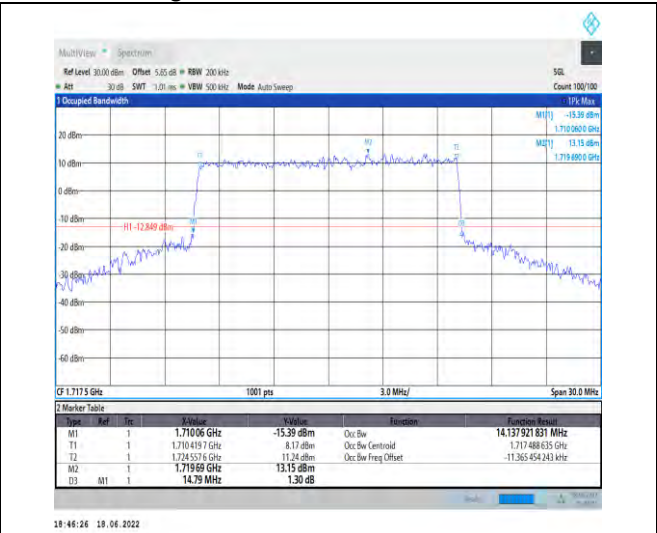
1-N66--15-15-L-8-CP-64QAM-Outer_Full-79@0-Ant 1-14.138-14.790-≤15-PASS
