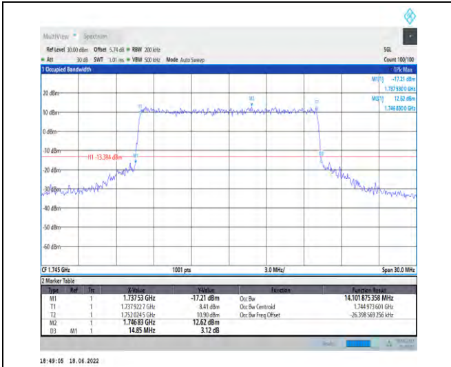
1-N66--15-15-M-6-CP-QPSK-Outer_Full-79@0-Ant1 -14.102-14.850-≤15-PASS
