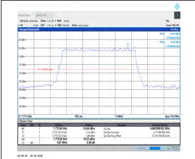
1-N66--15-5-H-5-DFT-256QAM-Outer_Full-25@0-An t1-4.469-4.870-≤5-PASS
