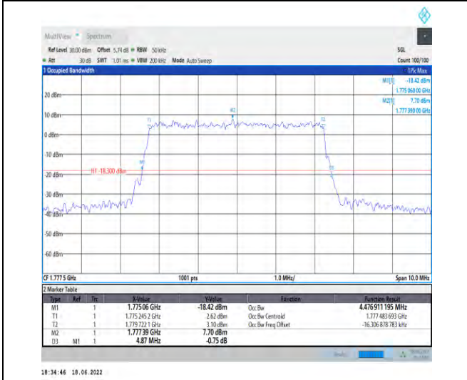
1-N66--15-5-H-9-CP-256QAM-Outer_Full-25@0-Ant1-4.477-4.870-≤5-PASS
