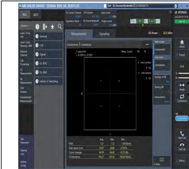
1-N66-PC3-15-20-M-1-DFT-PI2BPSK-Outer_Full-10@0-Ant1-see graph-PASS
