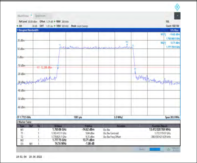
1-N66--15-15-H-4-DFT-64QAM-Outer_Full-75@0-An t1-13.412-14.160-≤15-PASS
