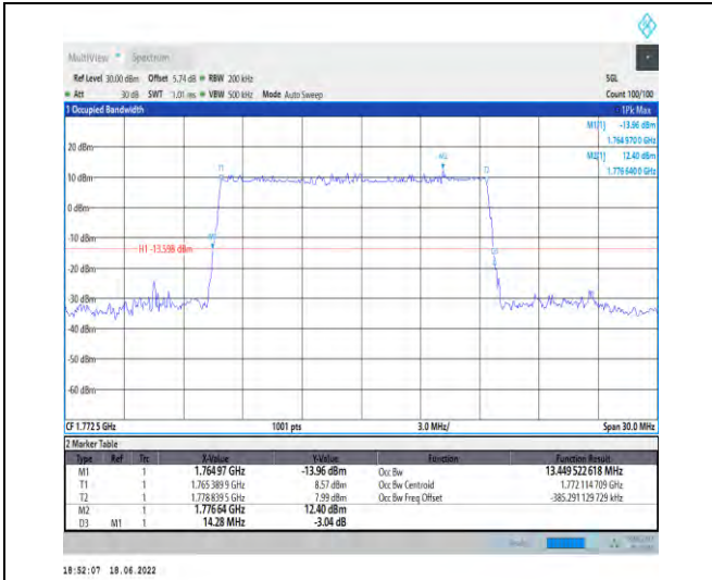
1-N66--15-15-H-5-DFT-256QAM-Outer_Full-75@0-A nt1-13.45-14.280-≤15-PASS
