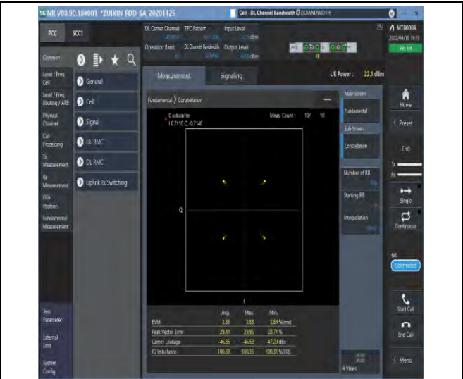
1-N66-PC3-15-20-M-2-DFT-QPSK-Outer_Full-100@0-Ant1-see graph-PASS
