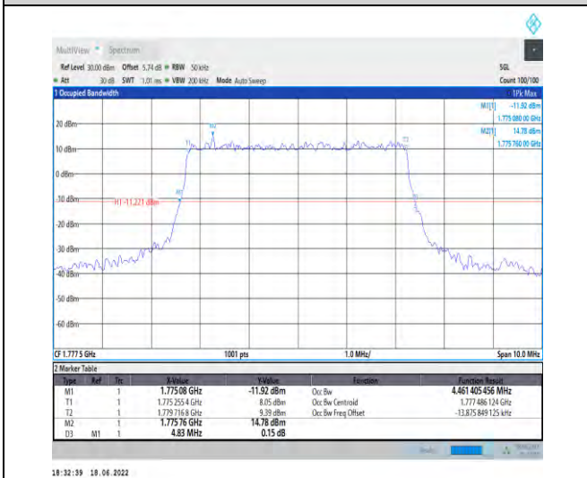
1-N66--15-5-H-1-DFT-QPSK-Outer_Full-25@0-Ant1- 4.461-4.830-≤5-PASS
