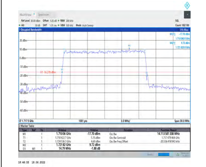
1-N66--15-15-L-9-CP-256QAM-Outer_Full-79@0-An t1-14.114-14.790-≤15-PASS
