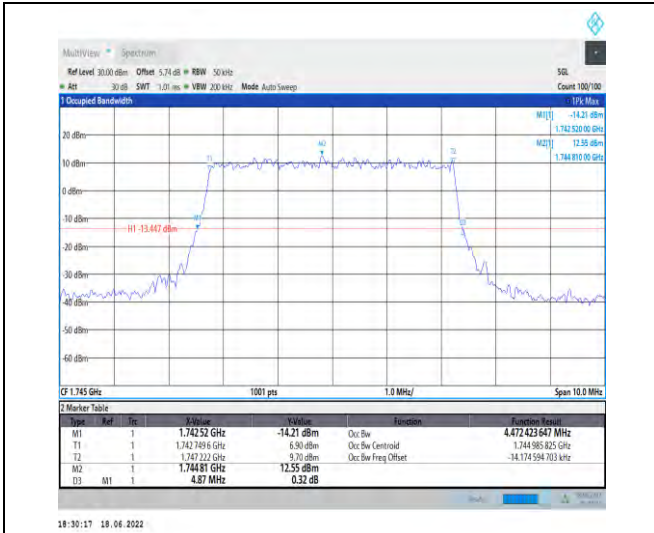
1-N66--15-5-M-4-DFT-64QAM-Outer_Full-25@0-Ant 1-4.472-4.870-≤5-PASS
