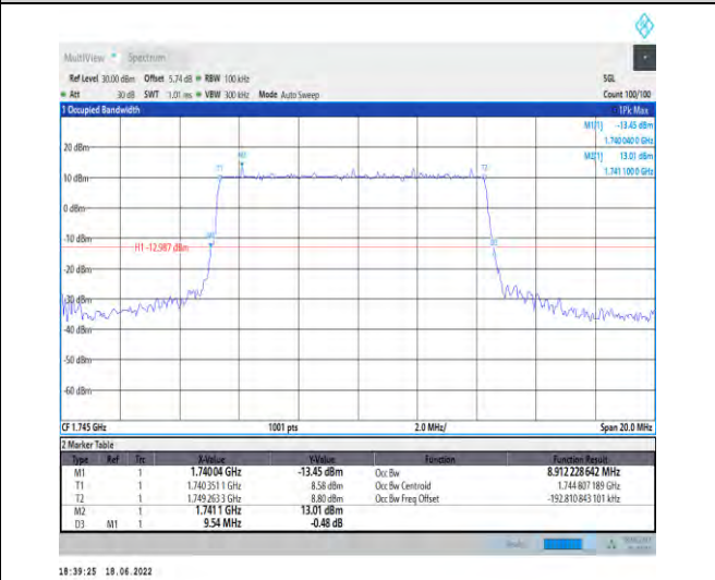
1-N66--15-10-M-4-DFT-64QAM-Outer_Full-50@0-An t1-8.912-9.540-≤10-PASS
