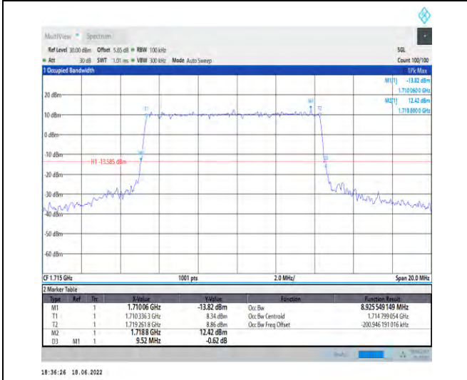
1-N66--15-10-L-4-DFT-64QAM-Outer_Full-50@0-Ant 1-8.926-9.520-≤10-PASS
