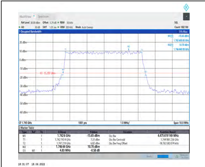
1-N66--15-5-M-8-CP-64QAM-Outer_Full-25@0-Ant1 -4.476-4.830-≤5-PASS
