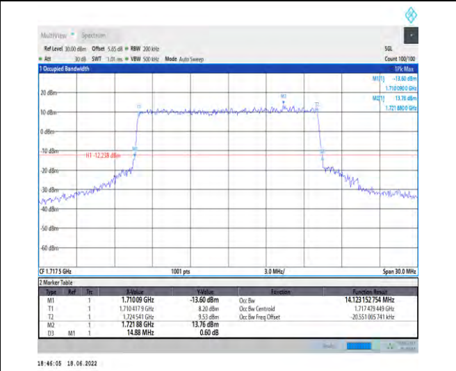
1-N66--15-15-L-6-CP-QPSK-Outer_Full-79@0-Ant1 14.123-14.880-≤15-PASS
