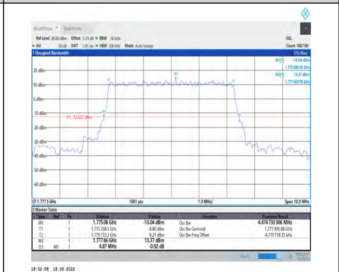
1-N66--15-5-H-2-DFT-PI2BPSK-Outer_Full-25@0-A nt1-4.475-4.870-≤5-PASS
