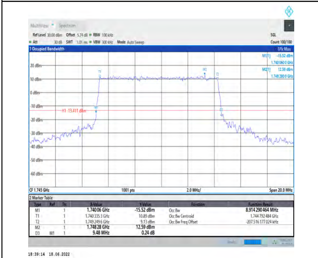
1-N66--15-10-M-3-DFT-16QAM-Outer_Full-50@0-An t1-8.914-9.480-≤10-PASS
