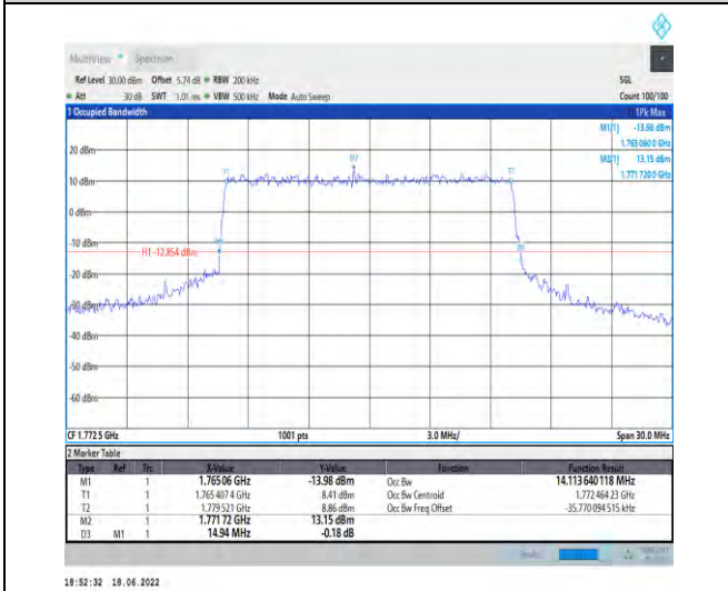
1-N66--15-15-H-7-CP-16QAM-Outer_Full-79@0-Ant 1-14.114-14.940-≤15-PASS
